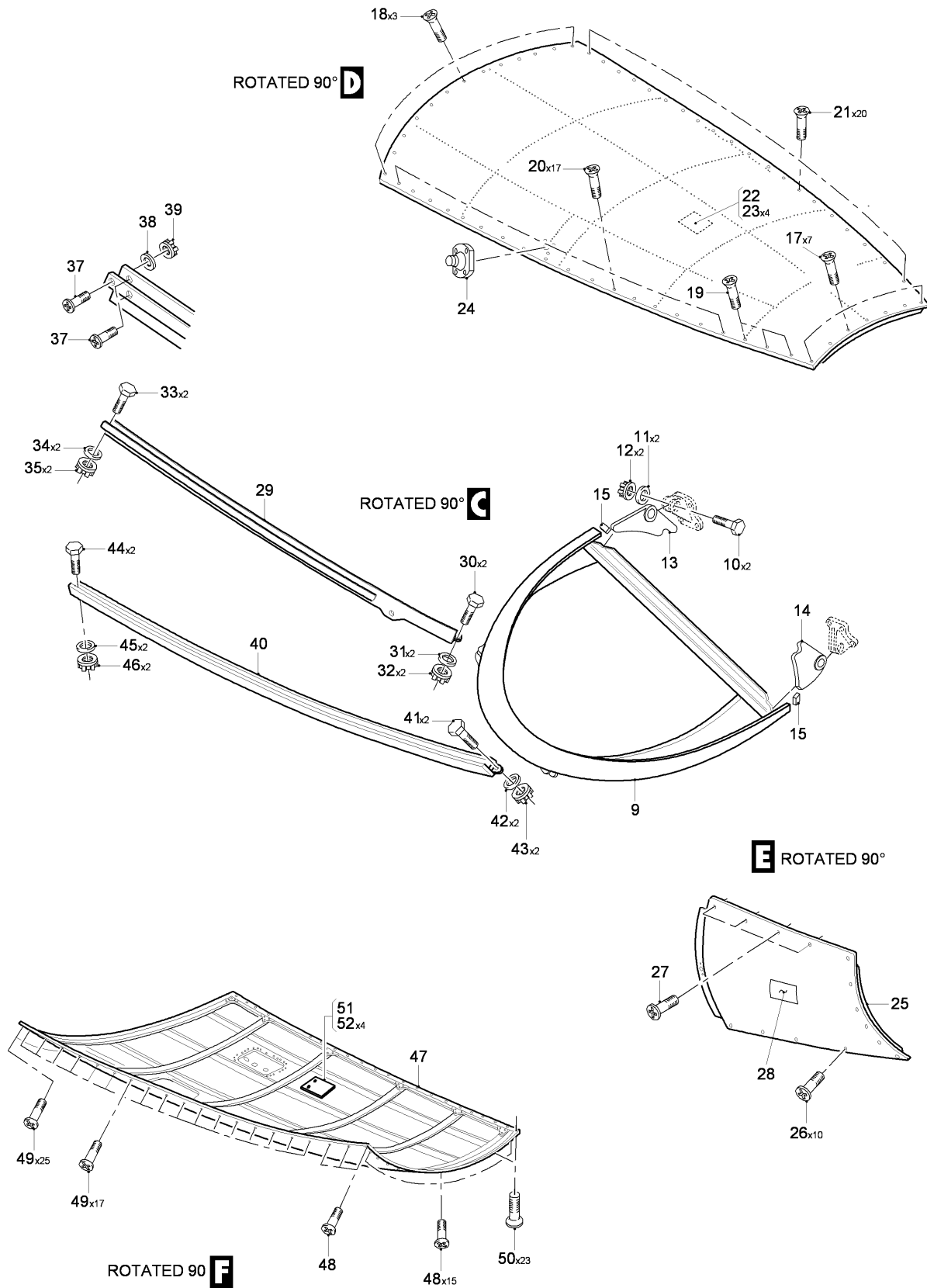
FIG 02 STRUCTURE INSTL - MLG, Z23AA-23AB, RH (SHEET 2 OF 4)
