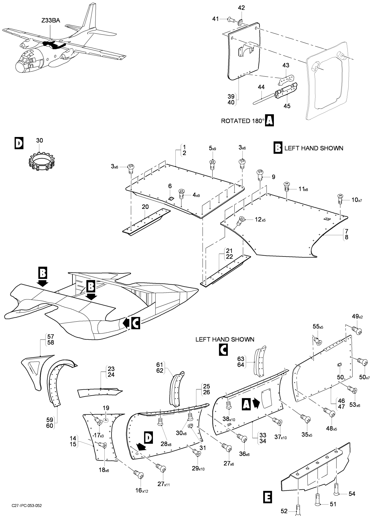
FIG 07 FAIRINGS INSTL - FWD, Z33BA, LH-RH (SHEET 1 OF 1)
