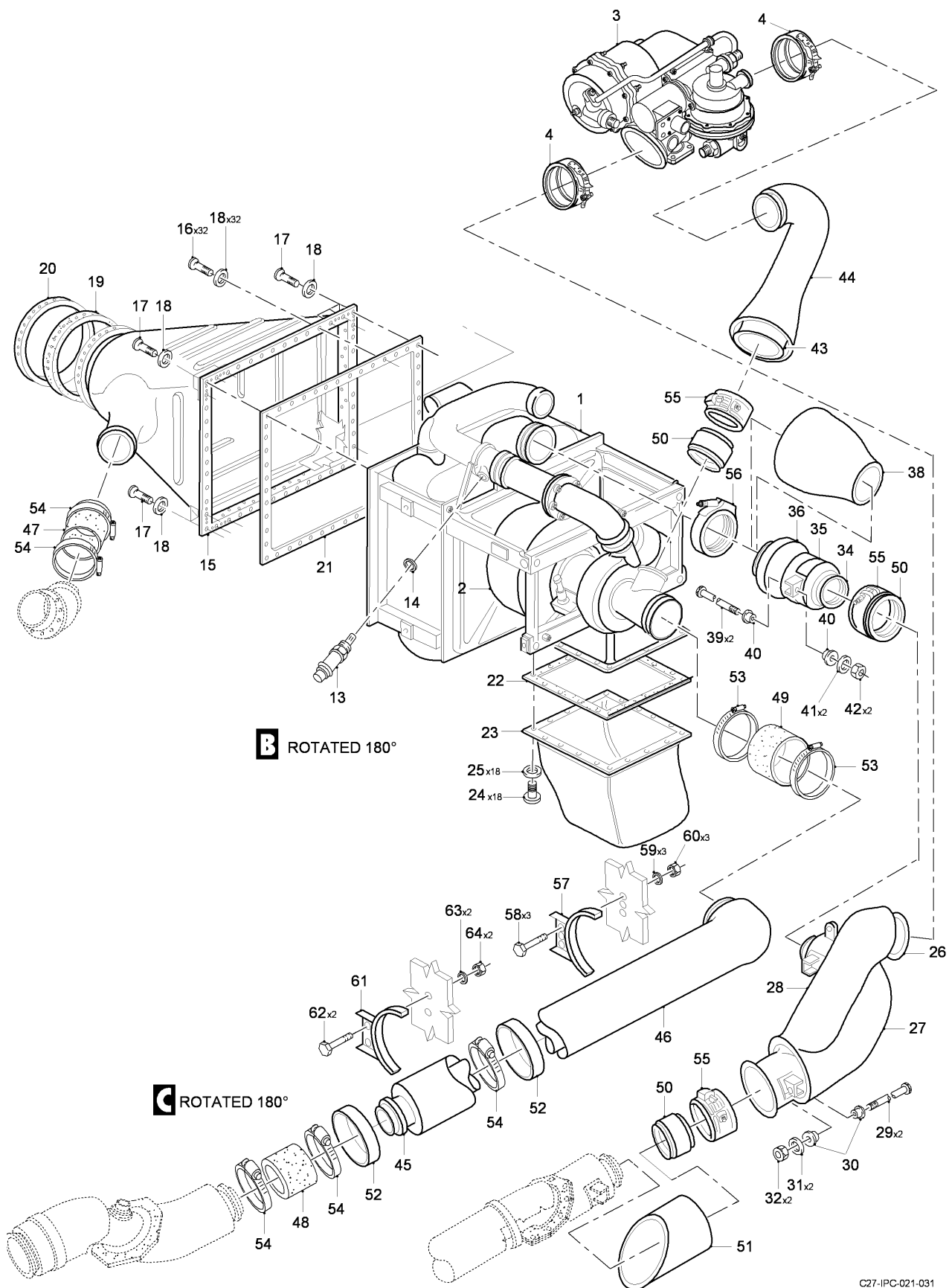
FIG 02 AIR CONDITIONING INSTL - MLG RH FAIRING, Z23AA (SHEET 2 OF 3)
