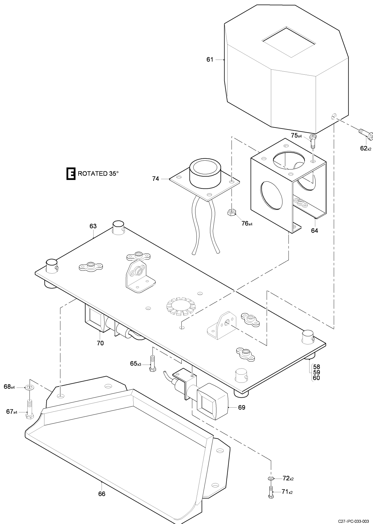
FIG 01 INTERNAL LIGHT INSTL, Z31AA (SHEET 3 OF 3)
