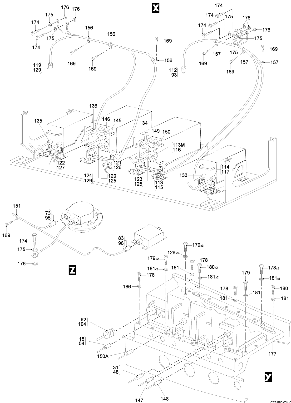
FIG 19M ELECTRICAL AND ELECTRONICS INSTL - REAR FUSELAGE, Z34AA (SHEET 8 OF 10)
