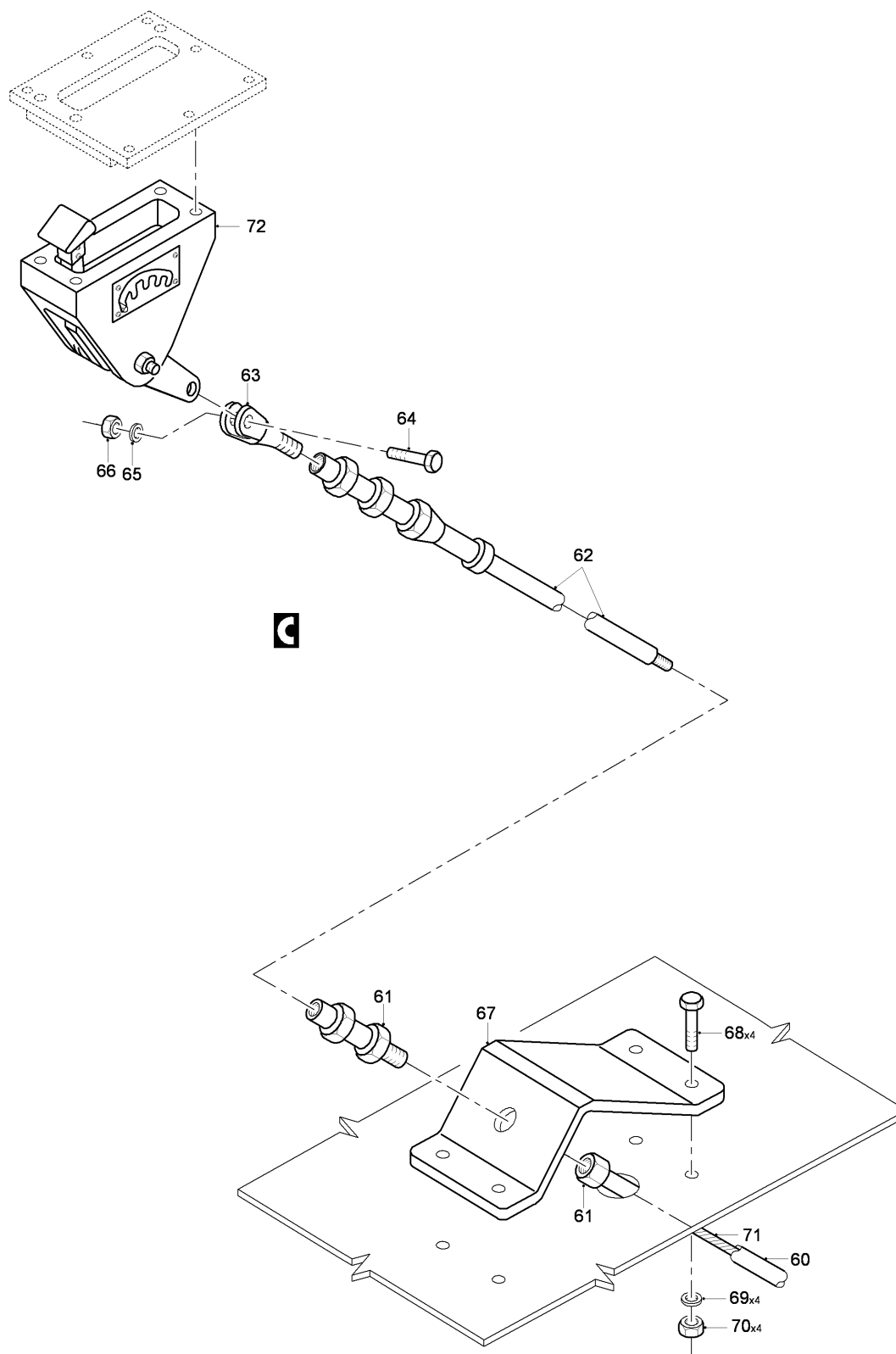
FIG 02 FLAP CONTROLS INSTL, Z31BB (SHEET 3 OF 4)
