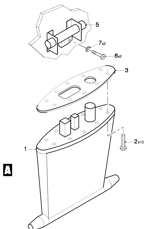
FIG 03 TACAN V/UHF ANTENNA 2 LOWER INSTL, Z32BA (SHEET 1 OF 1)
