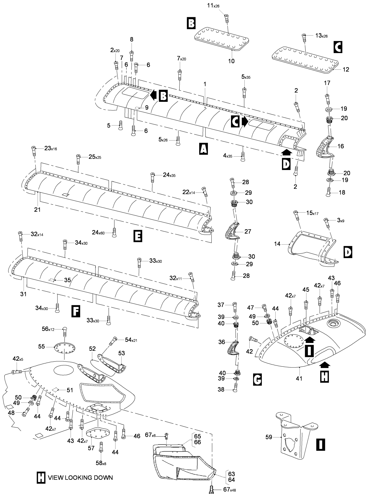
FIG 02 LANDING EDGE INSTL - OUTER WING, Z11AA-21AA, LH-RH (SHEET 2 OF 2)
