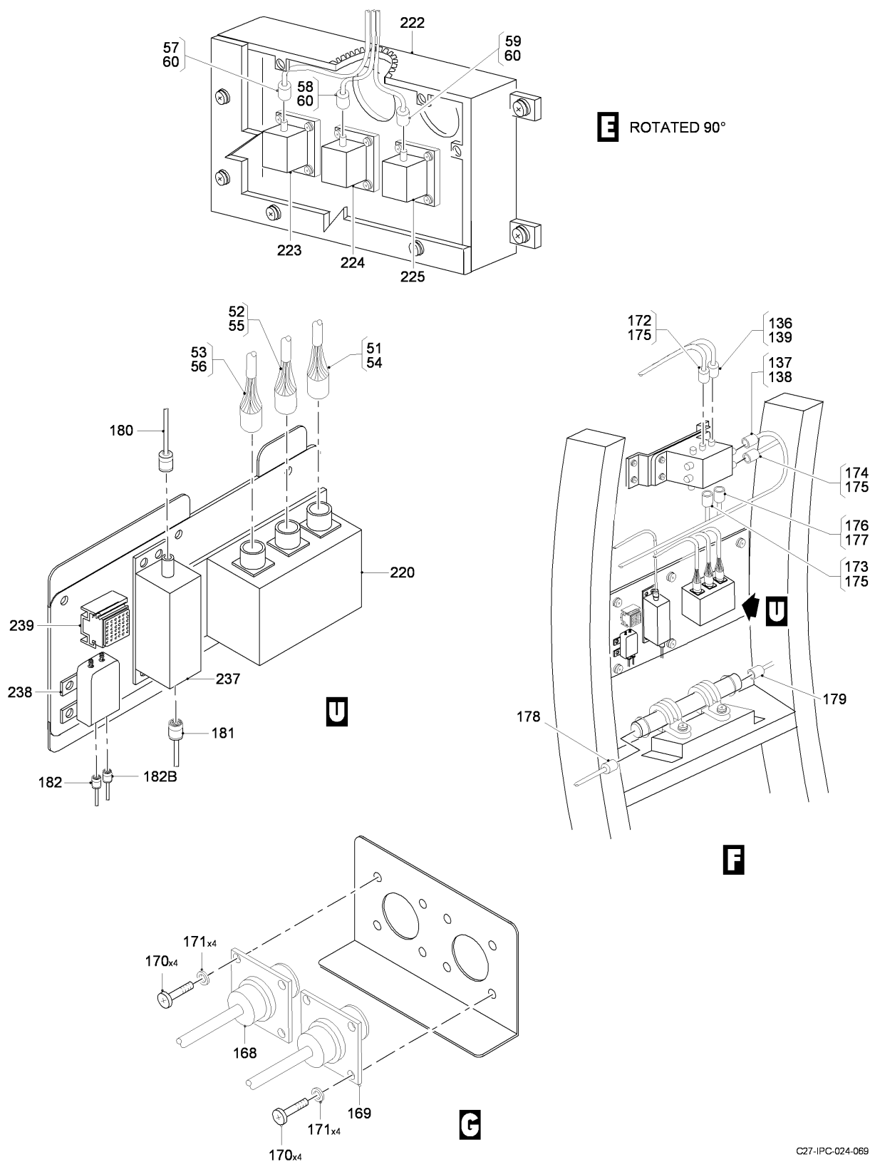
FIG 16 ELECTRICAL AND ELECTRONICS INSTL, Z31AB-32AA-32AB-32AC, RH (SHEET 5 OF 8)
