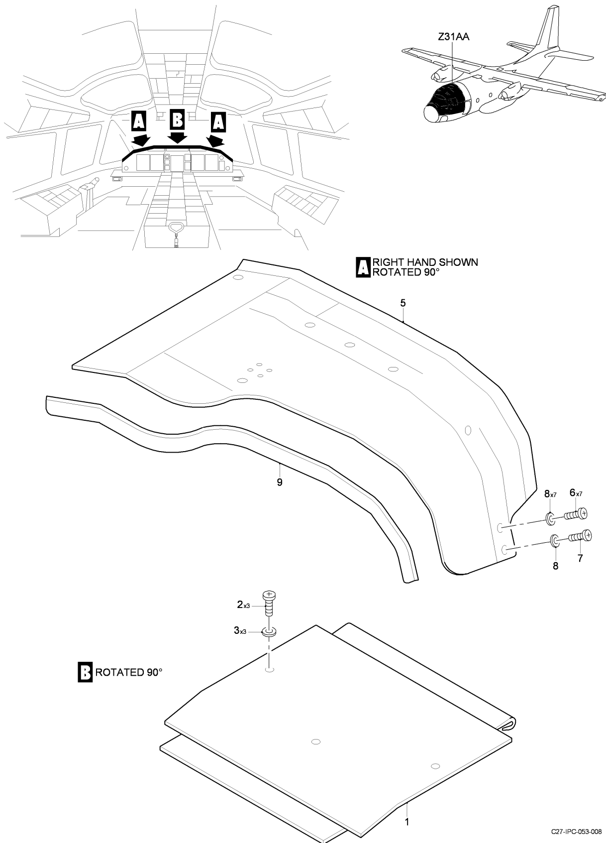
FIG 01 GLARE SHIELD INSTL, Z31AA (SHEET 1 OF 1)
