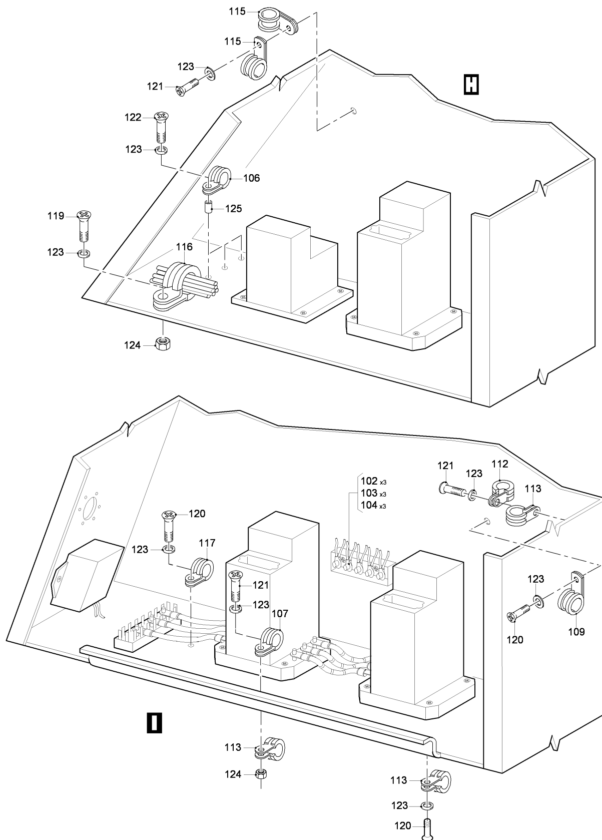
FIG 11 ELECTRICAL AND ELECTRONICS INSTL, Z31AA (SHEET 4 OF 6)
