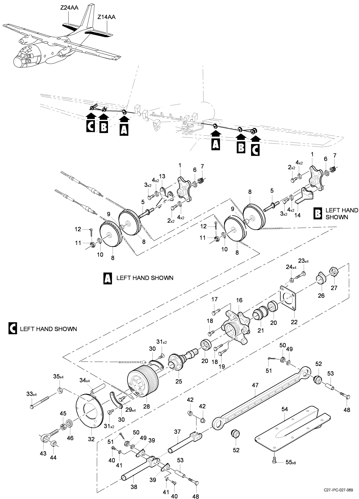
FIG 10 ELEVATOR TRIM CONTROLS INSTL, Z14AB-24AB, LH-RH (SHEET 1 OF 1)
