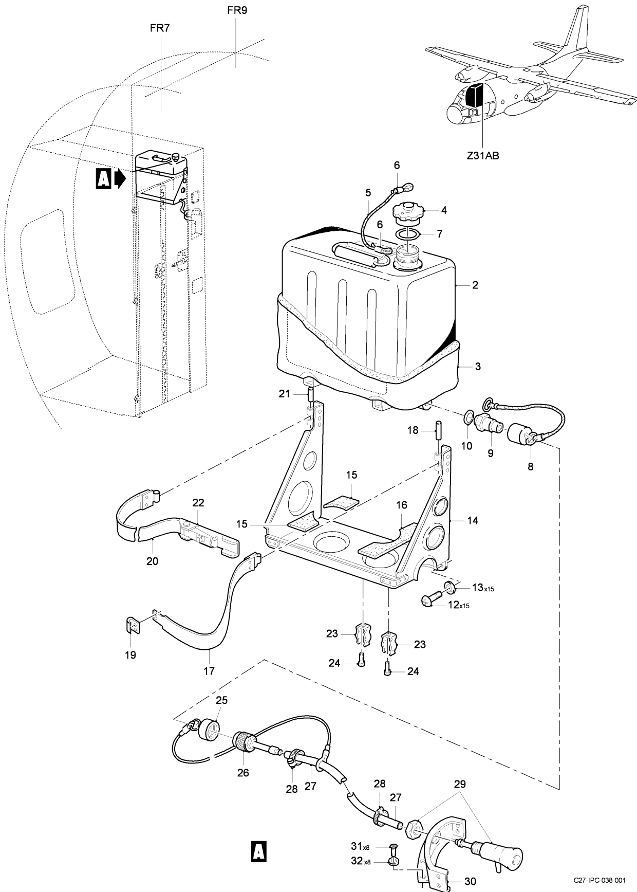
FIG 01 DRINKABLE WATER INSTL, Z31AB (SHEET 1 OF 1)
