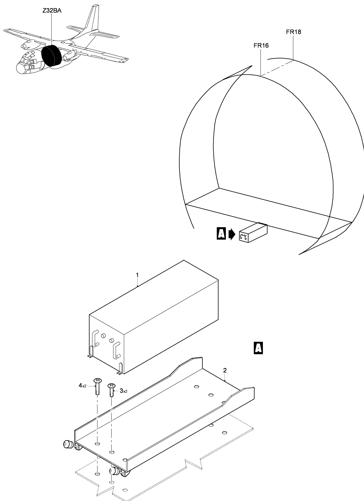
FIG 02 FREQUENCY CONVERTER INSTL, Z32BA (SHEET 1 OF 1)
