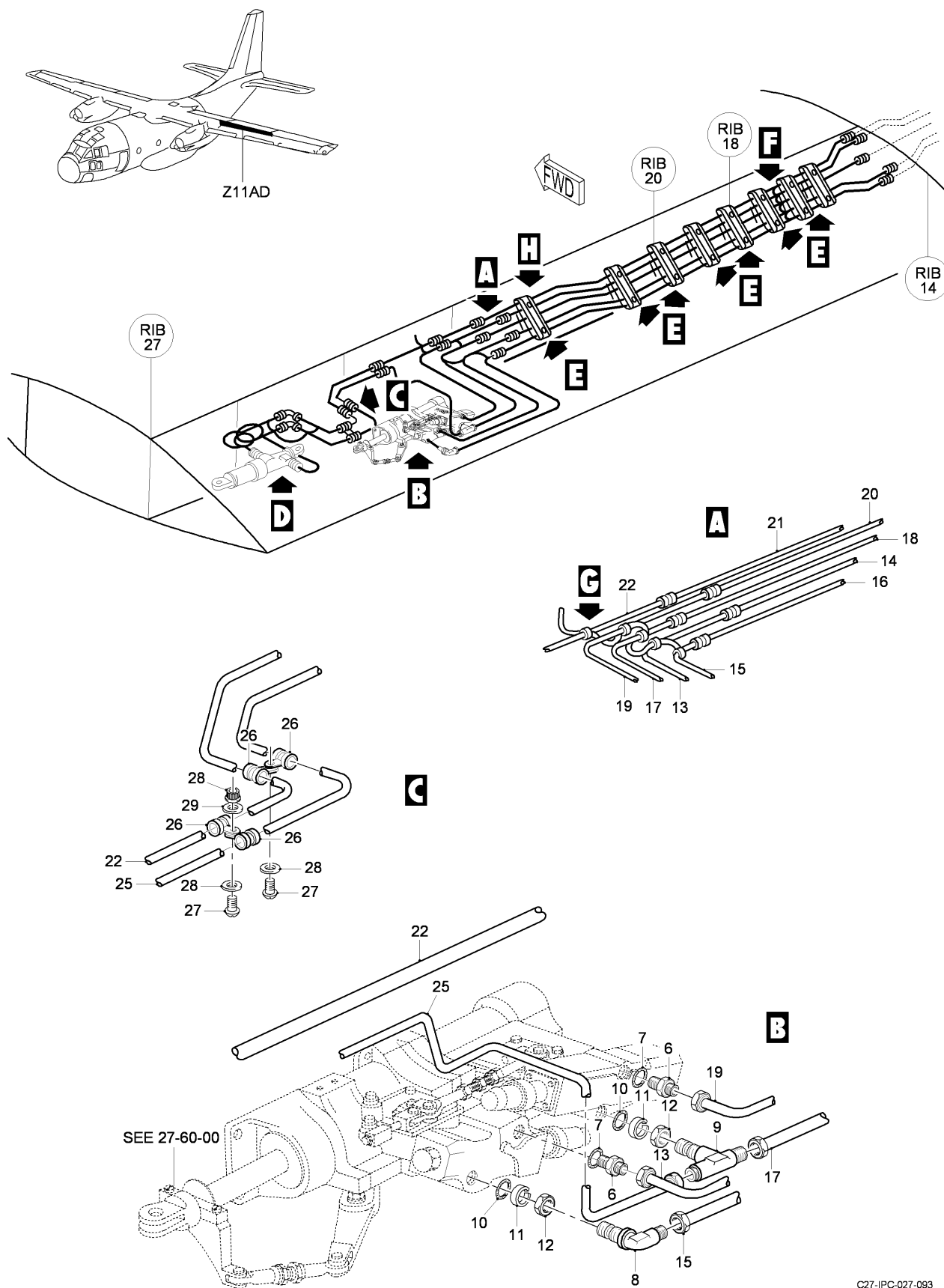
FIG 04 HYDRAULIC PIPING INSTL - SPOILER CONTROL, Z11AD, LH (SHEET 1 OF 3)
