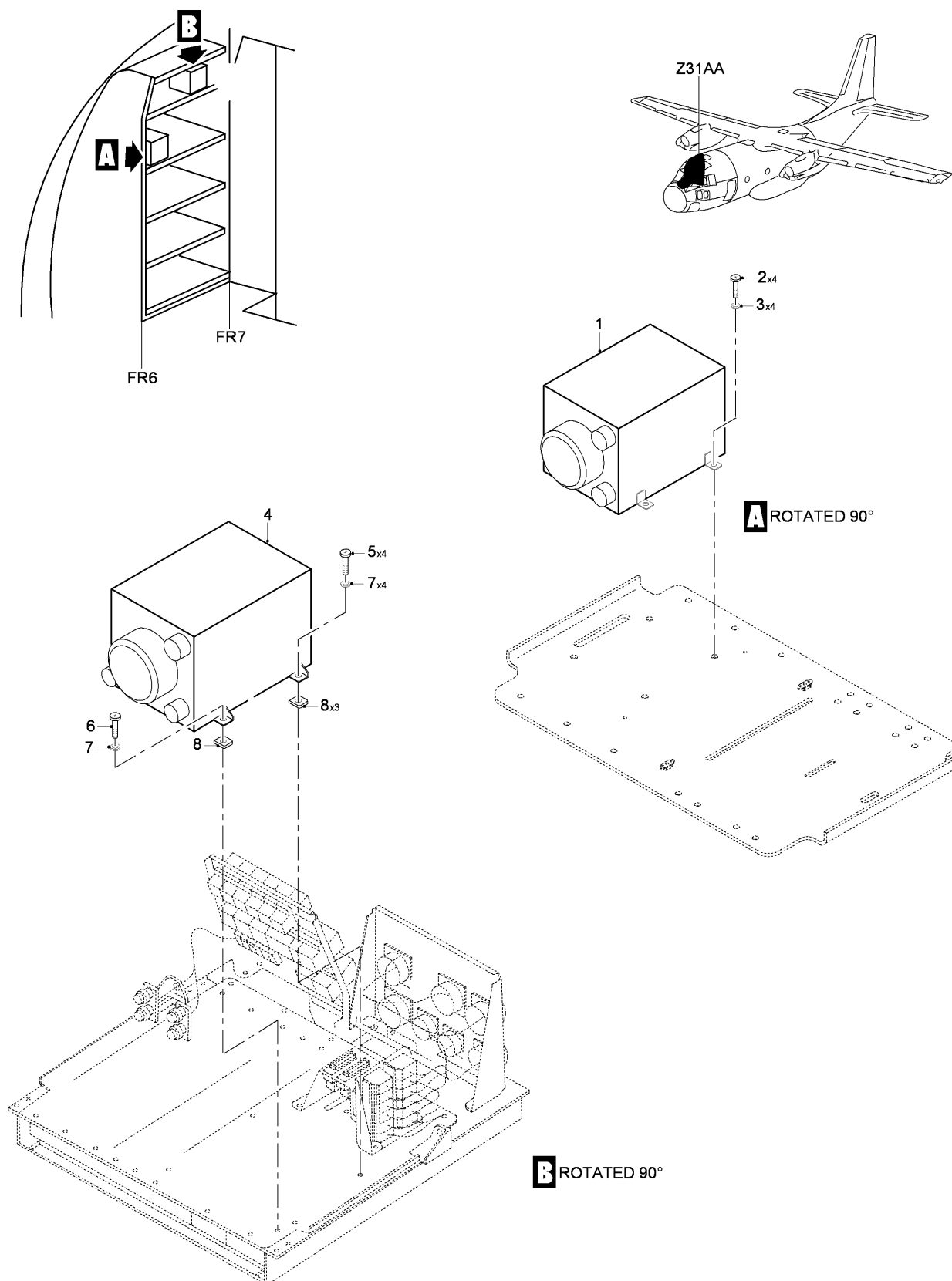
FIG 04 TRU INSTL, Z31AA (SHEET 1 OF 1)
