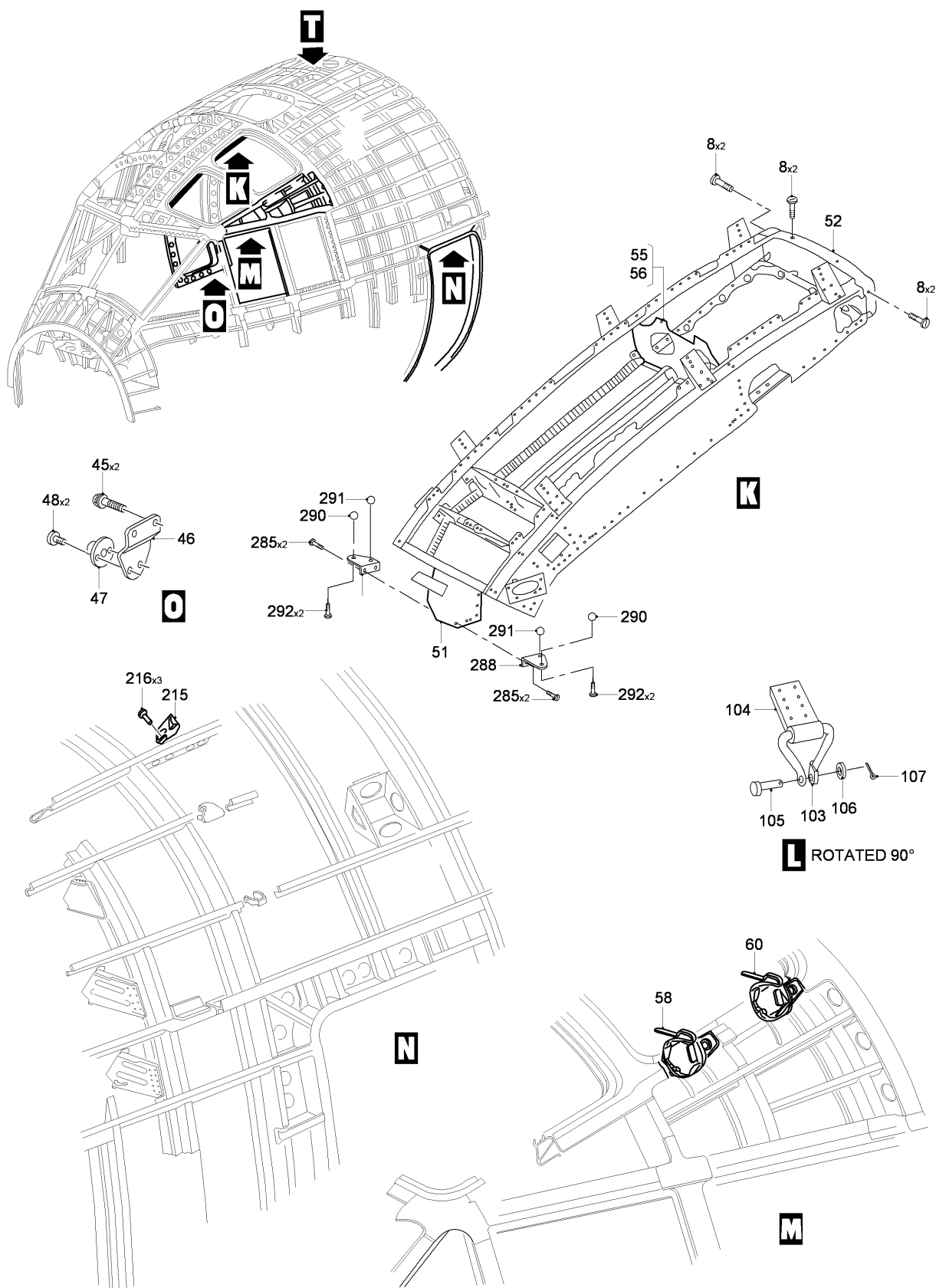
FIG 06 STRUCTURE INSTL, Z31AA (SHEET 3 OF 10)
