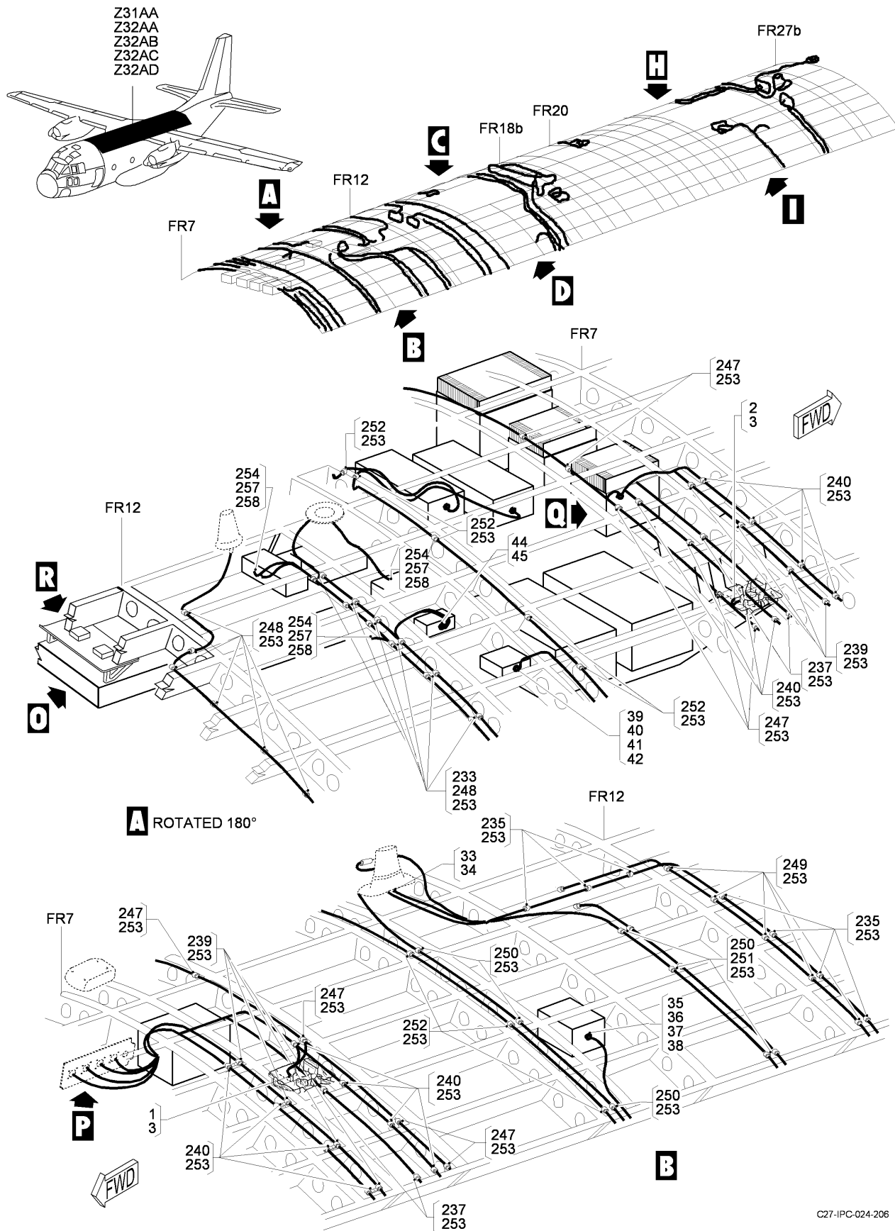
FIG 17 ELECTRICAL AND ELECTRONICS INSTL, Z31AA-32AA-32AB-32AC-32AD (SHEET 1 OF 8)
