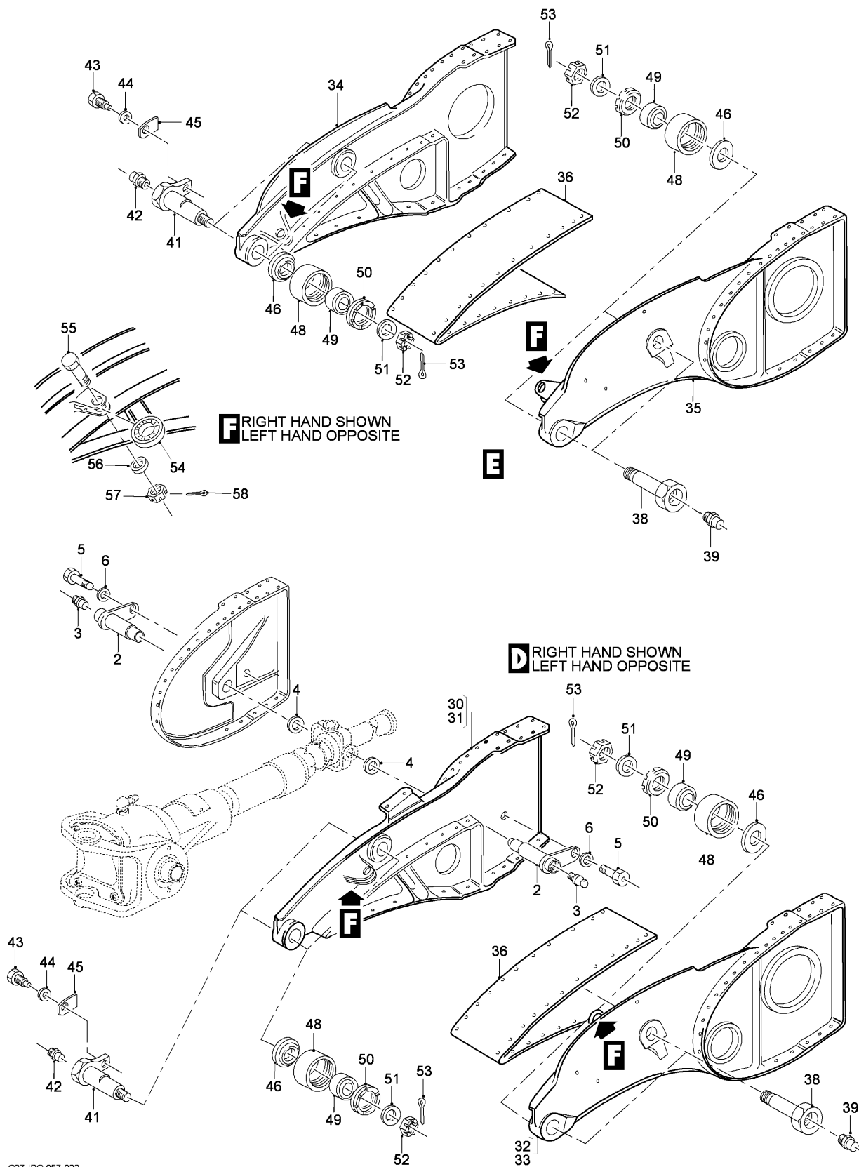
FIG 01 FLAP INSTL - CENTER WING, Z33AC, LH-RH (SHEET 2 OF 2)
