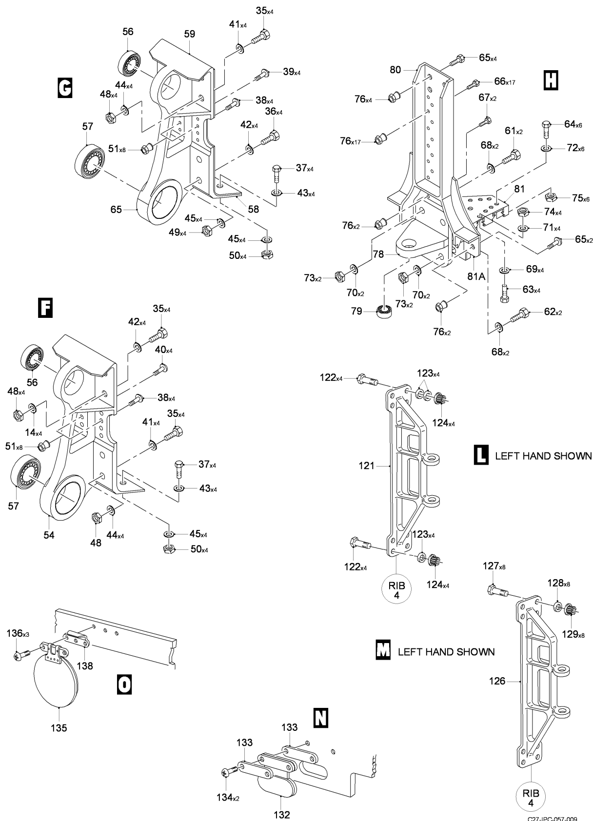
FIG 03 STRUCTURE INSTL - CENTER WING, Z33AB (SHEET 3 OF 5)
