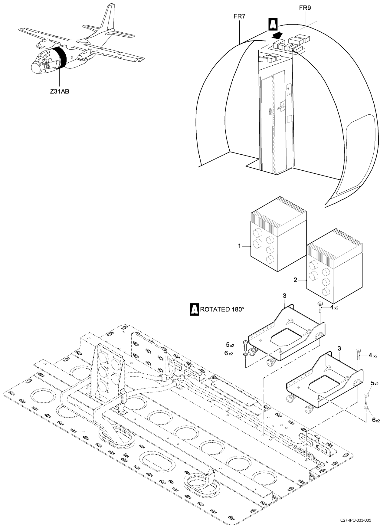
FIG 03 ANNUNCIATOR DIMMER UNIT INSTL, Z31AB (SHEET 1 OF 1)
