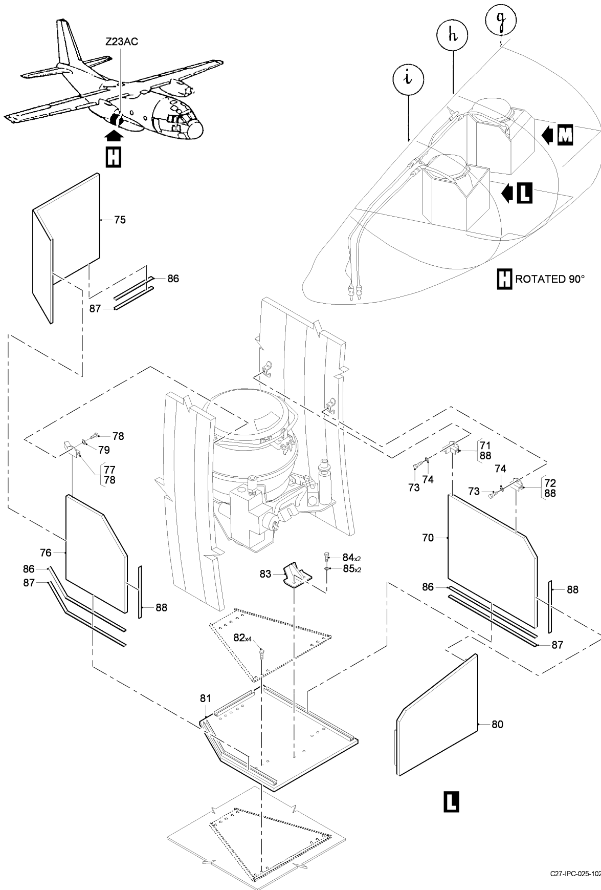
FIG 20 KIT G, BALLISTIC PROTECTION, Z13AC-Z23AC-Z31AA-Z31BA-Z34AA (SHEET 4 OF 6)
