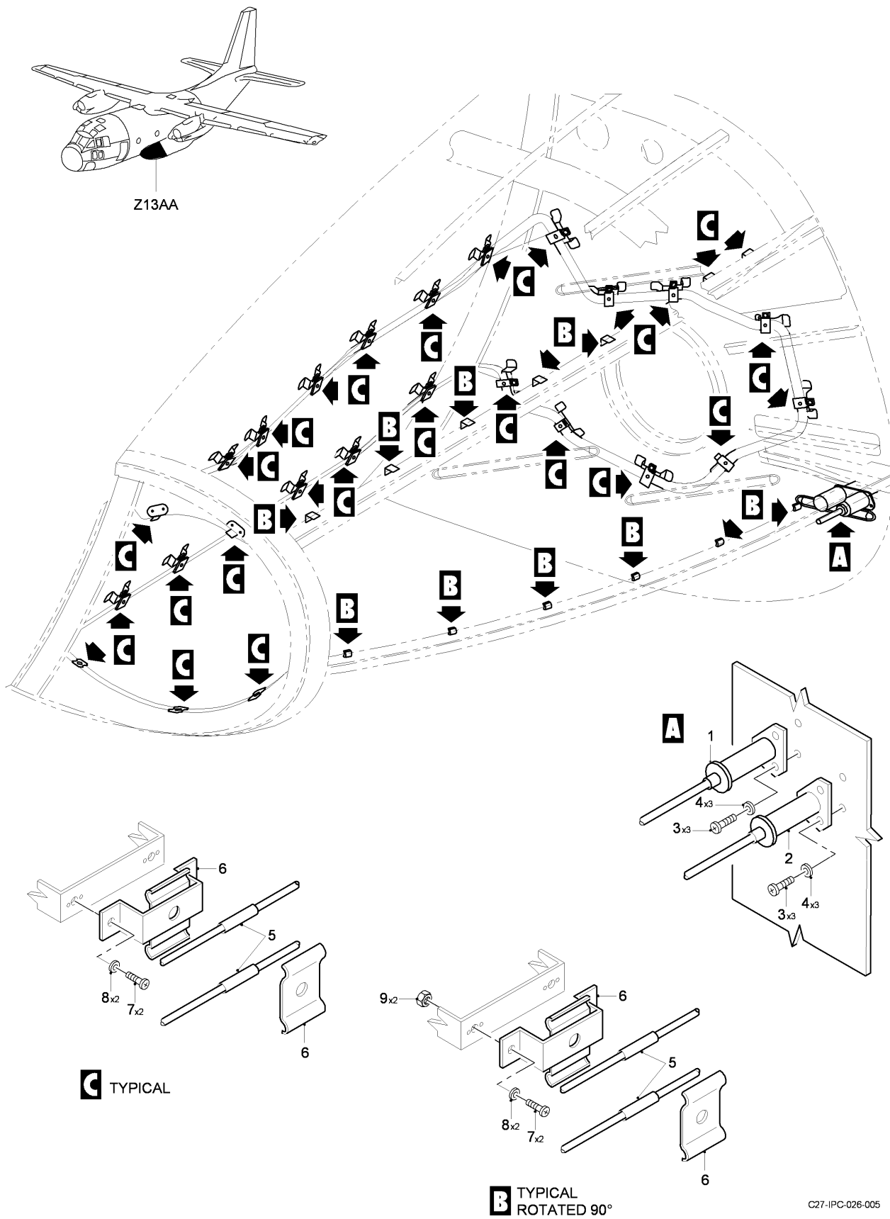
FIG 05 APU FIRE DETECTOR INSTL, MLG FAIRING, Z13AA, LH (SHEET 1 OF 1)
