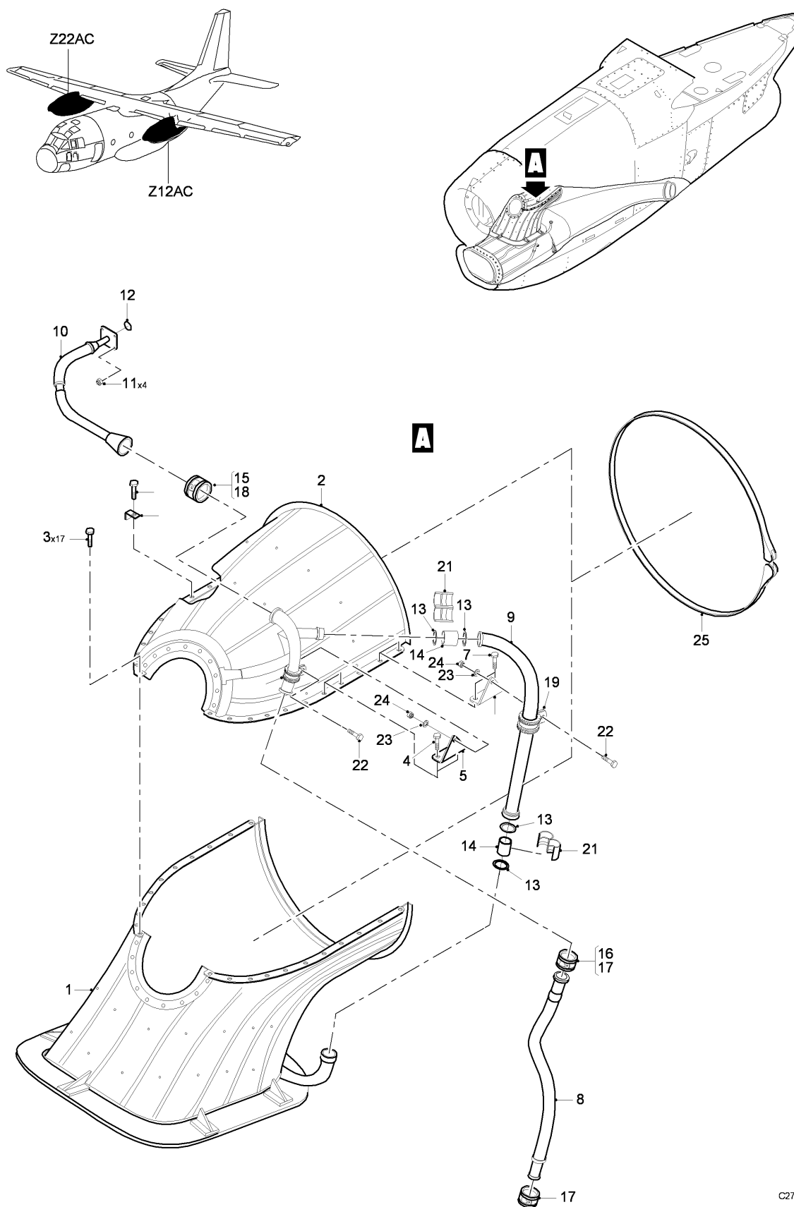
FIG 01 AIR INTAKE UPPER INSTL - ENGINE, Z12AC-22AC, LH-RH (SHEET 1 OF 1)
