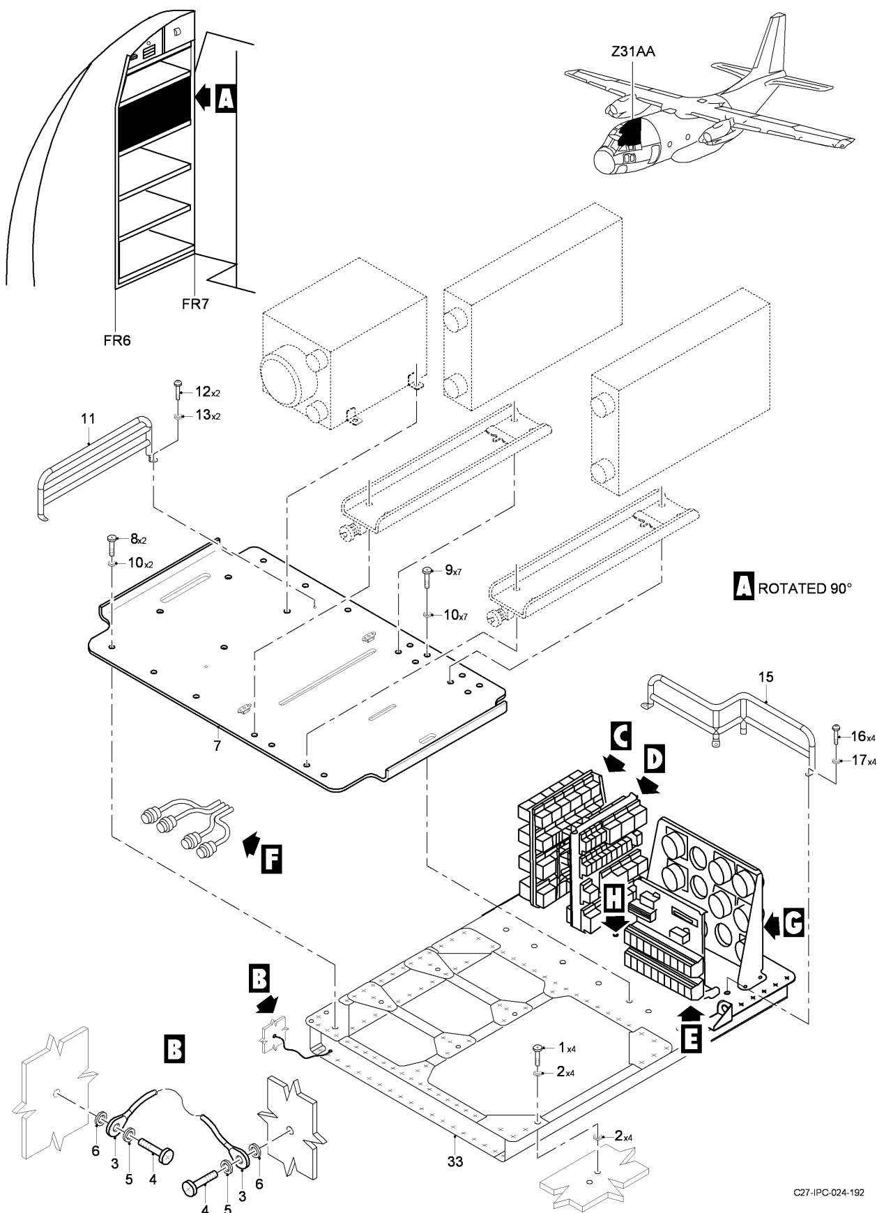
FIG 10 FOURTH SHELF INSTL - ELECTRICAL COMPARTMENT, Z31AA (SHEET 1 OF 4)
