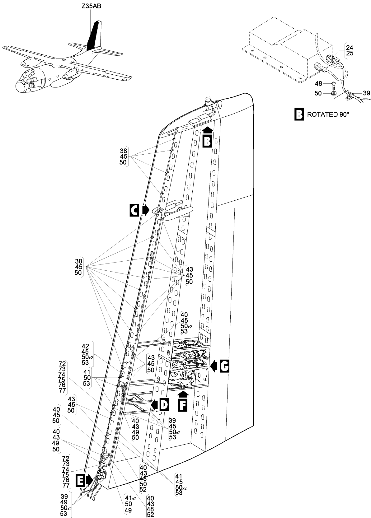
FIG 21 ELECTRICAL AND ELECTRONICS INSTL, Z35AB (SHEET 1 OF 4)
