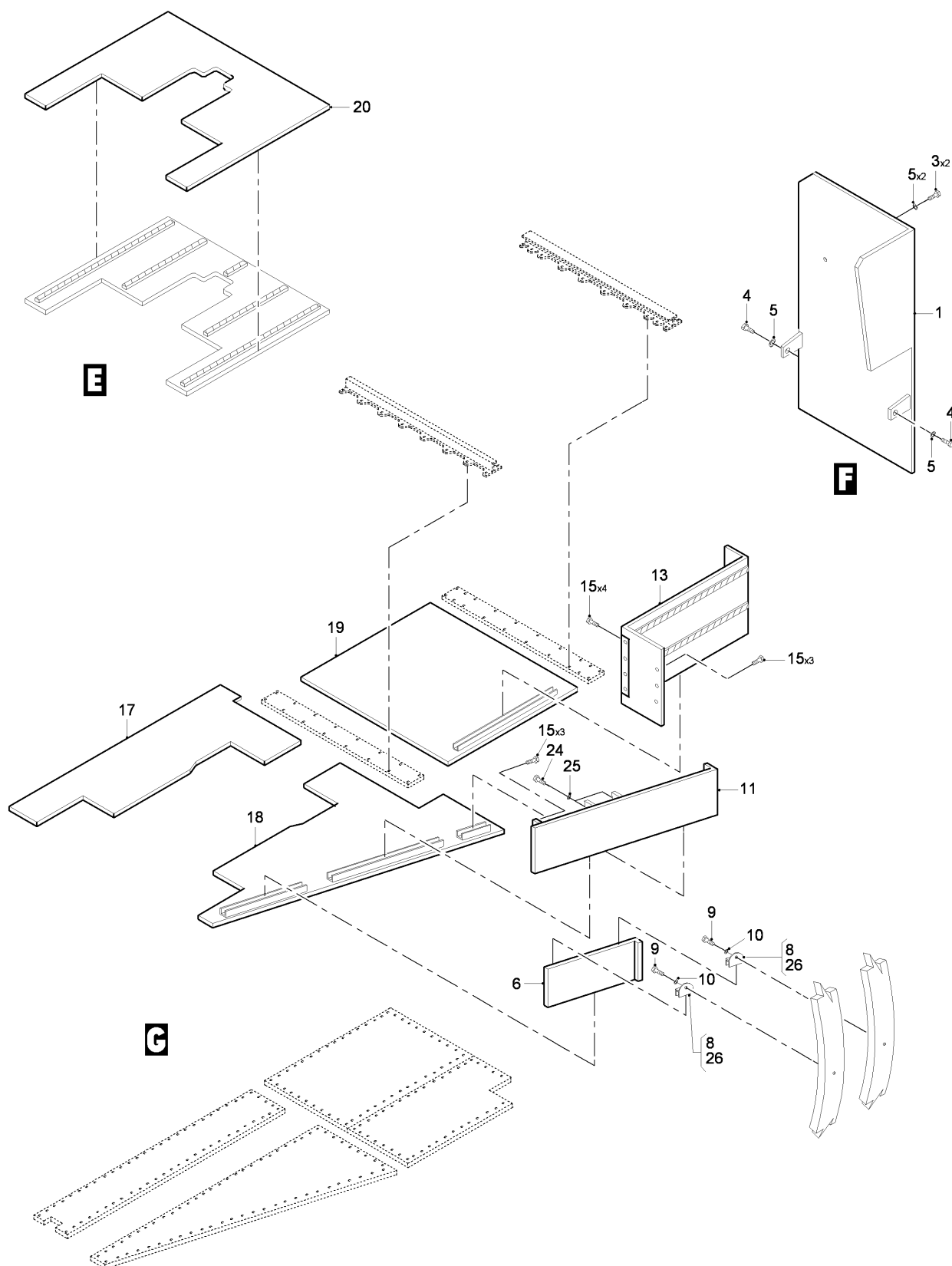
FIG 20 KIT G, BALLISTIC PROTECTION, Z13AC-Z23AC-Z31AA-Z31BA-Z34AA (SHEET 3 OF 6)
