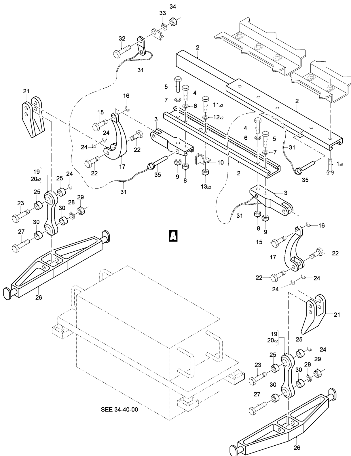
FIG 03 RAIL INSTL - RECEIVER TRANSMITTER PROCESSOR, Z31BA (SHEET 2 OF 2)
