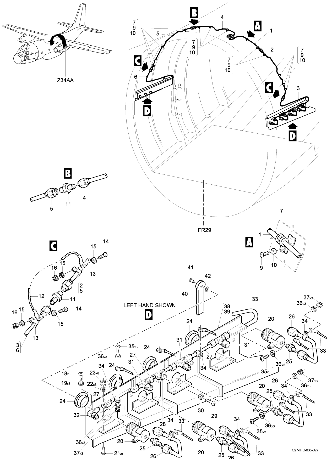
FIG 04 OXYGEN INSTL - REAR FUSELAGE, Z34AA (SHEET 1 OF 1)
