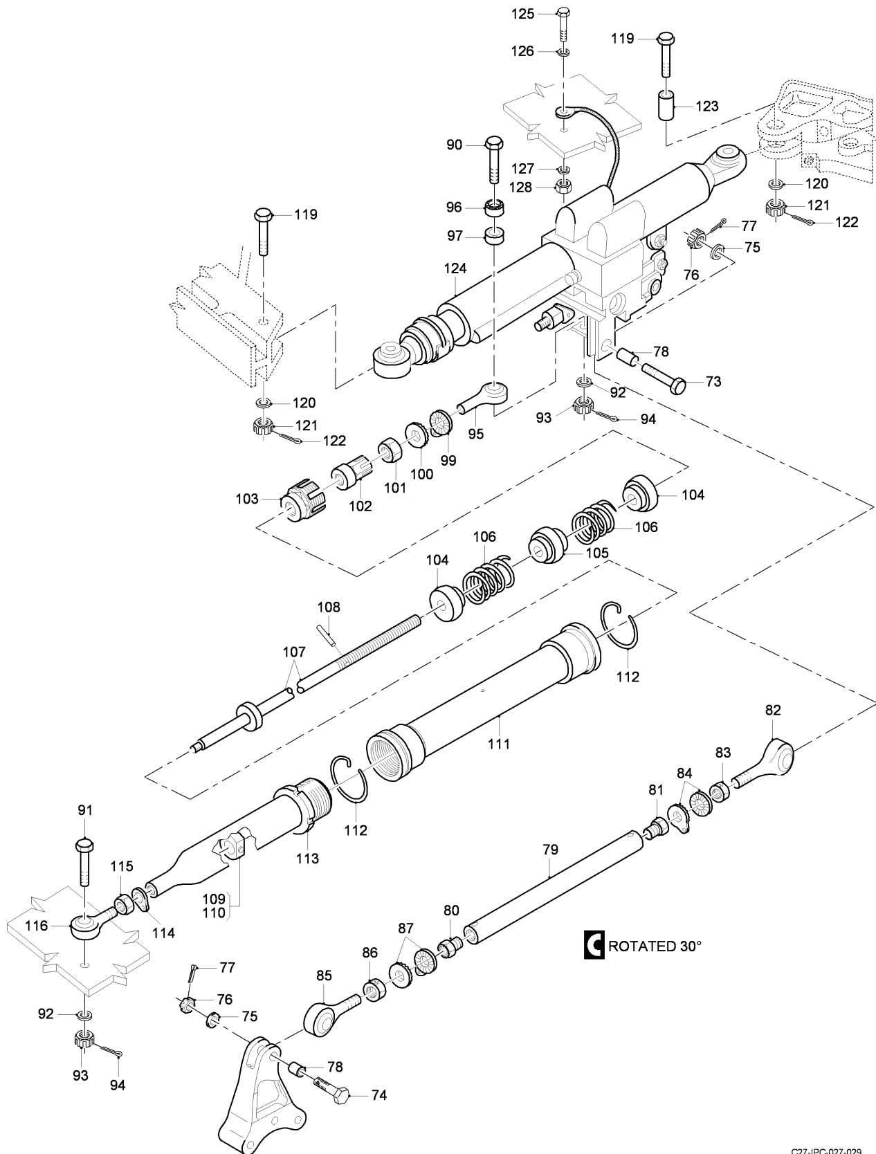
FIG 06 RUDDER CONTROL INSTL, Z35AB (SHEET 3 OF 4)
