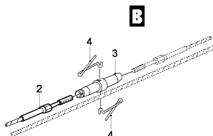
FIG 04 RUDDER CONTROLS INSTL, Z32AB-32AC-32AD (SHEET 1 OF 1)
