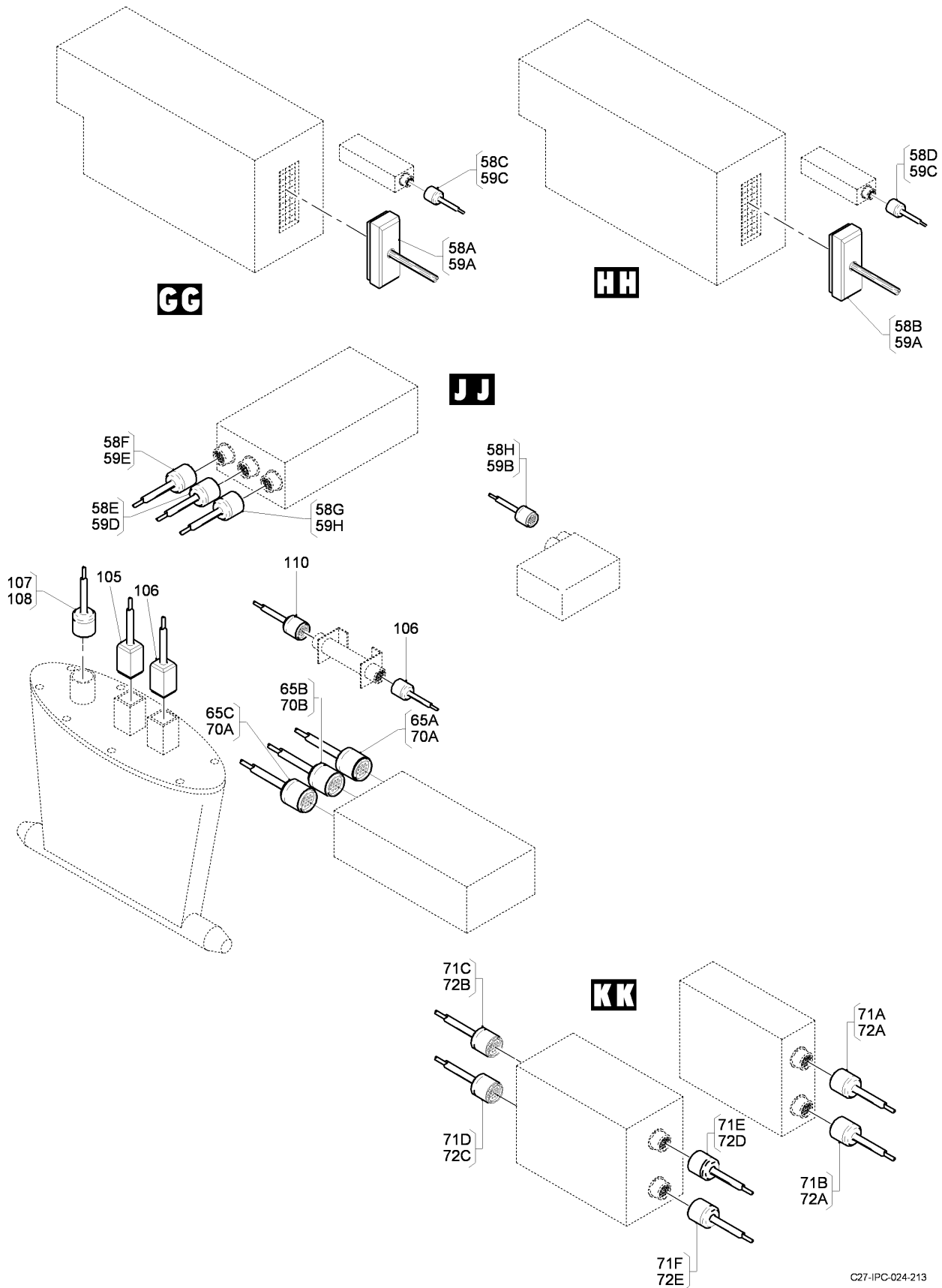
FIG 14 ELECTRICAL AND ELECTRONICS INSTL, Z31BC-31BD-32BA (SHEET 11 OF 11)
