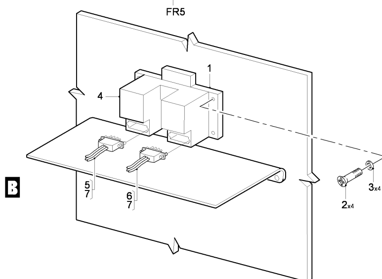
FIG 02 POWER DISTRIBUTION UNIT INSTL, Z31AA (SHEET 1 OF 1)
