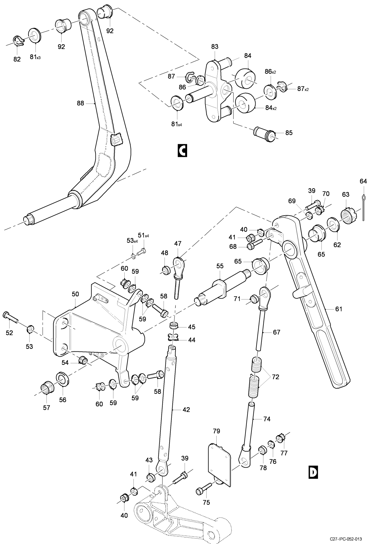
FIG 03 PARATROOPS DOOR ASSY, LH-RH (SHEET 2 OF 8)
