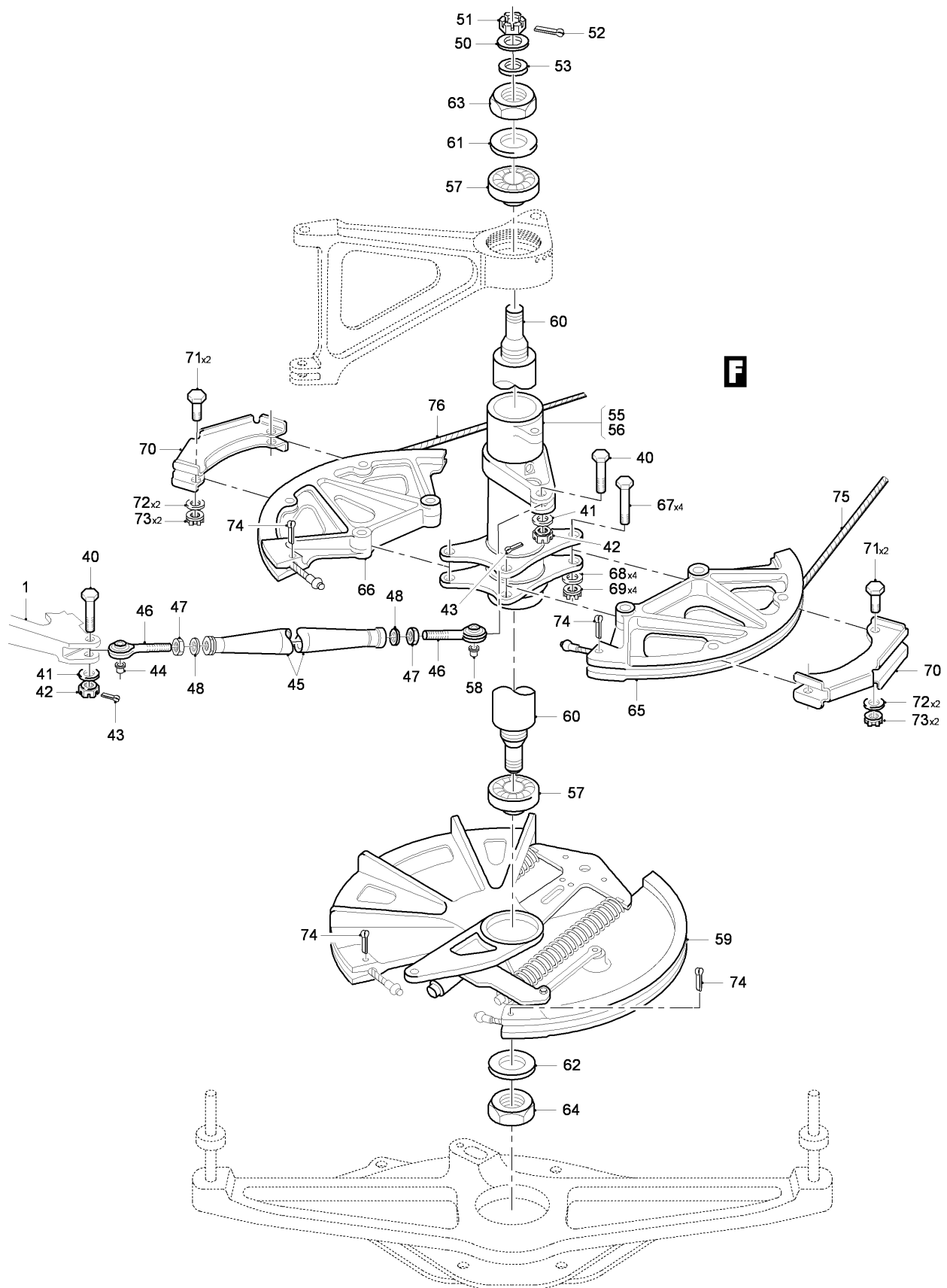
FIG 03 RUDDER CONTROLS INSTL, Z31AA-31BC-31AB (SHEET 4 OF 5)
