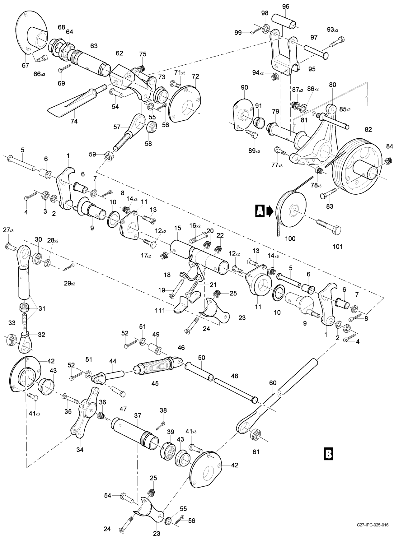
FIG 05 CONTROLS INSTL - LIFE RAFT DOOR, Z32AC, LH-RH (SHEET 2 OF 2)
