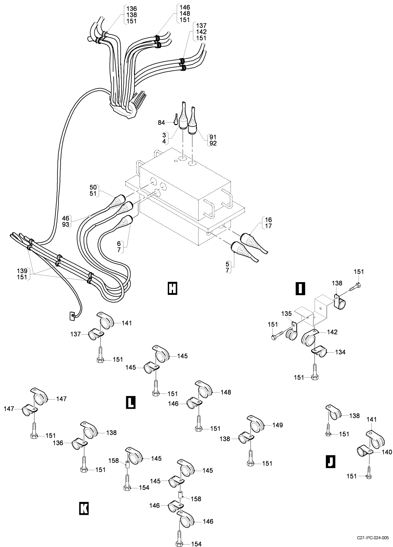
FIG 01 ELECTRICAL AND ELECTRONICS INSTL - RADOME AND FWD BAY, Z31BA (SHEET 5 OF 5)
