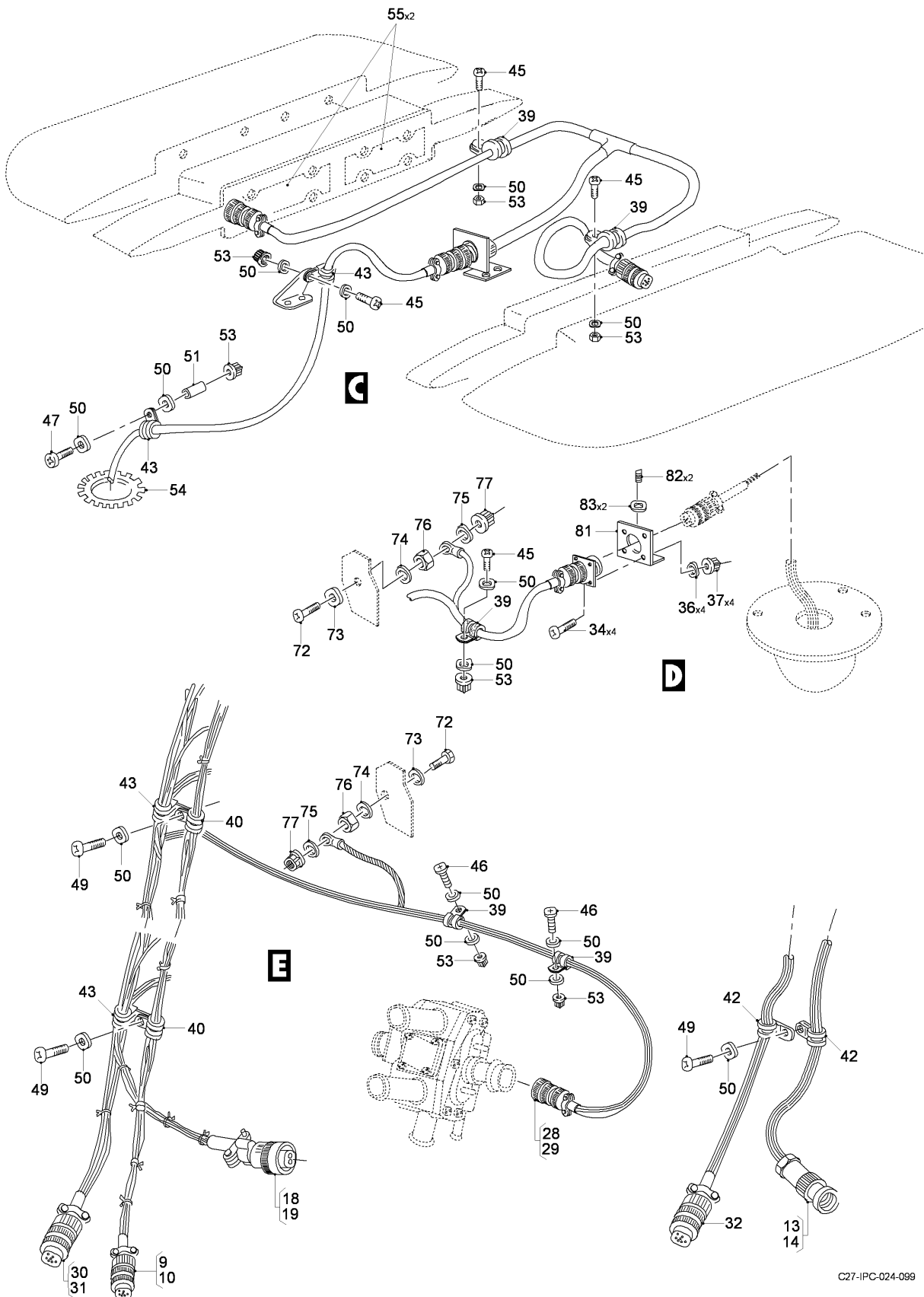
FIG 21 ELECTRICAL AND ELECTRONICS INSTL, Z35AB (SHEET 2 OF 4)
