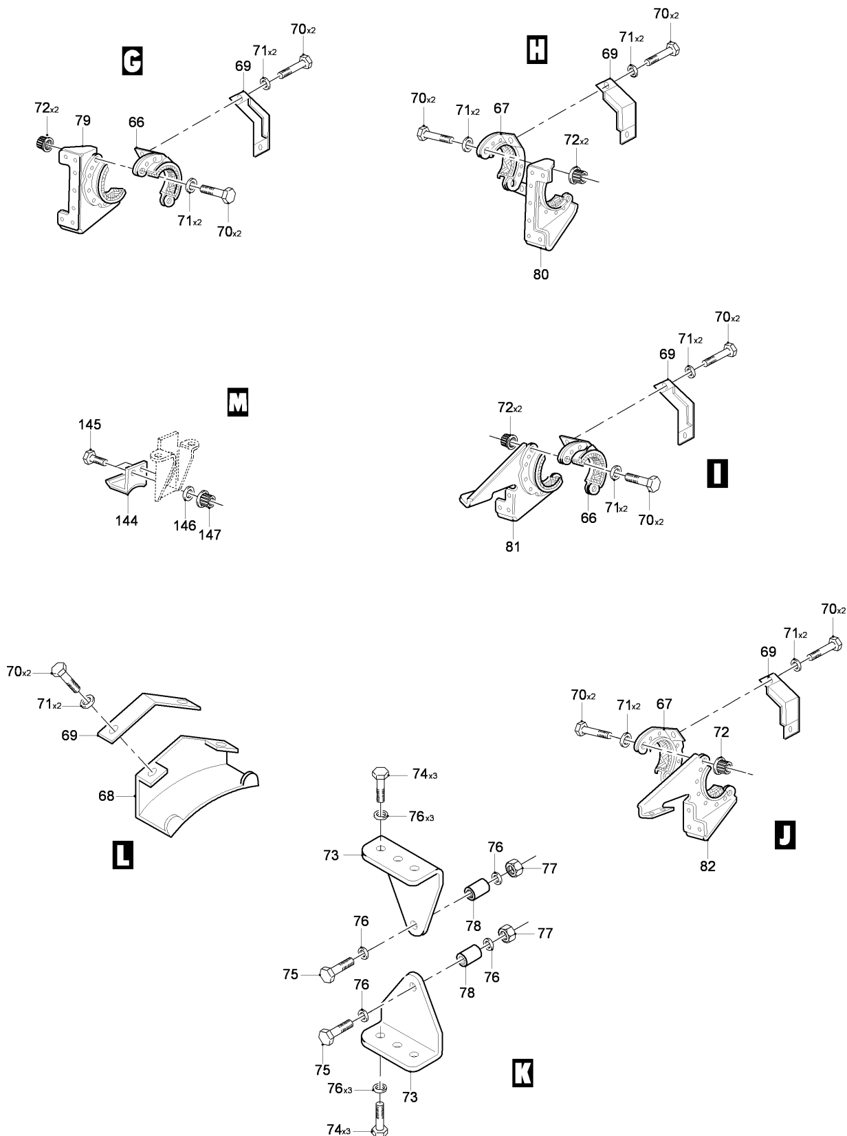
FIG 04 AIR CONDITIONING INSTL - CENTER FUSELAGE, Z32BA-32AB (SHEET 4 OF 7)
