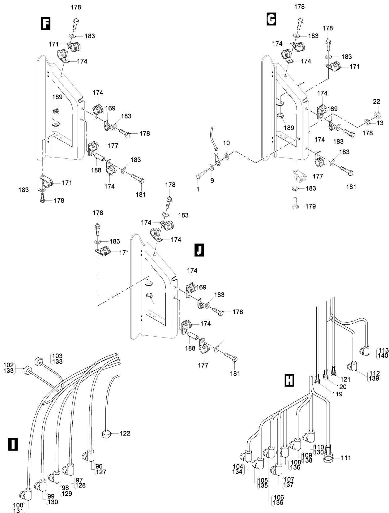
FIG 22 ELECTRICAL AND ELECTRONICS INSTL - CENTER WING, Z33AB, LH (SHEET 3 OF 7)
