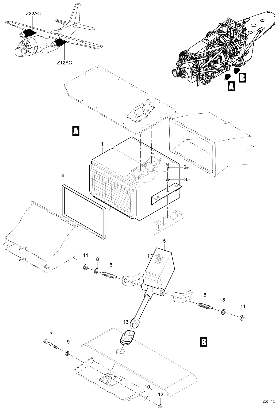
FIG 01 ENGINE LUBRICATION INSTL, Z12AC-22AC (SHEET 1 OF 1)
