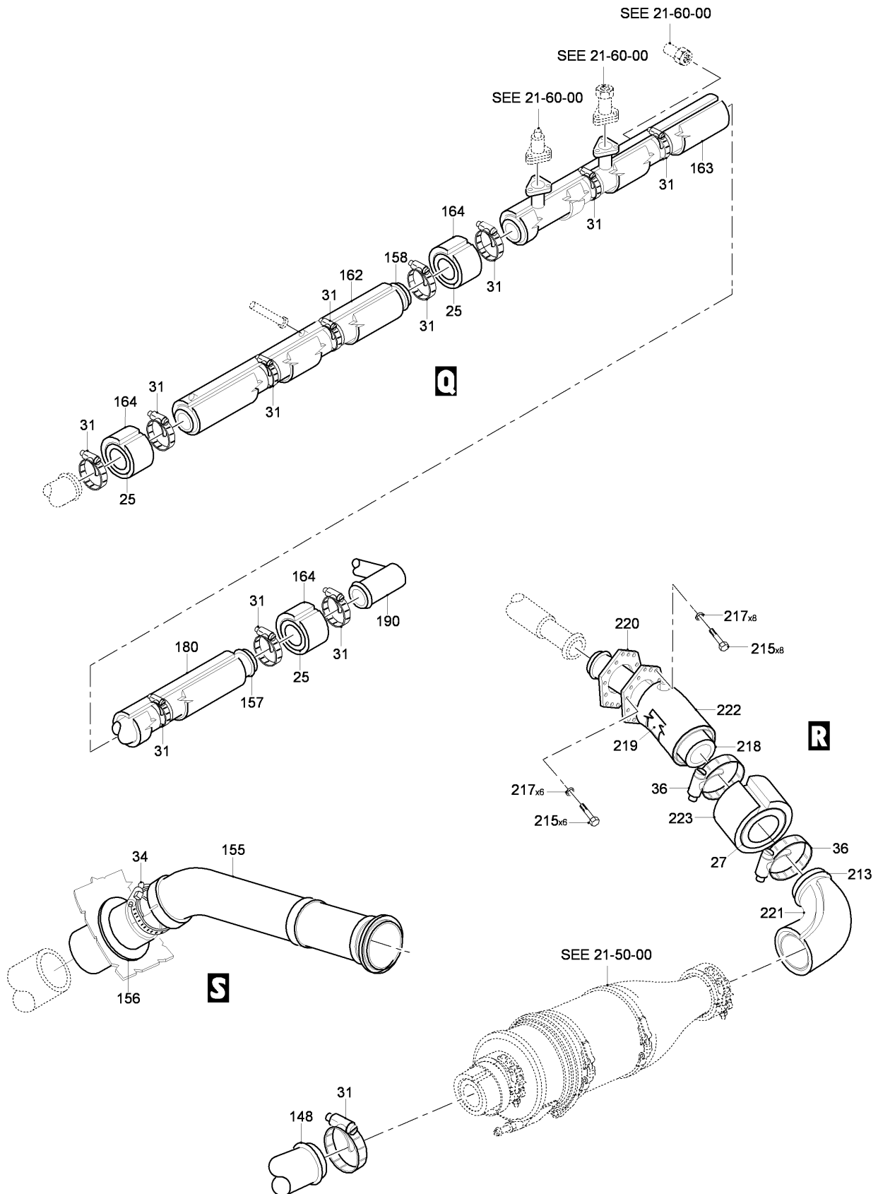
FIG 04 AIR CONDITIONING INSTL - CENTER FUSELAGE, Z32BA-32AB (SHEET 6 OF 7)
