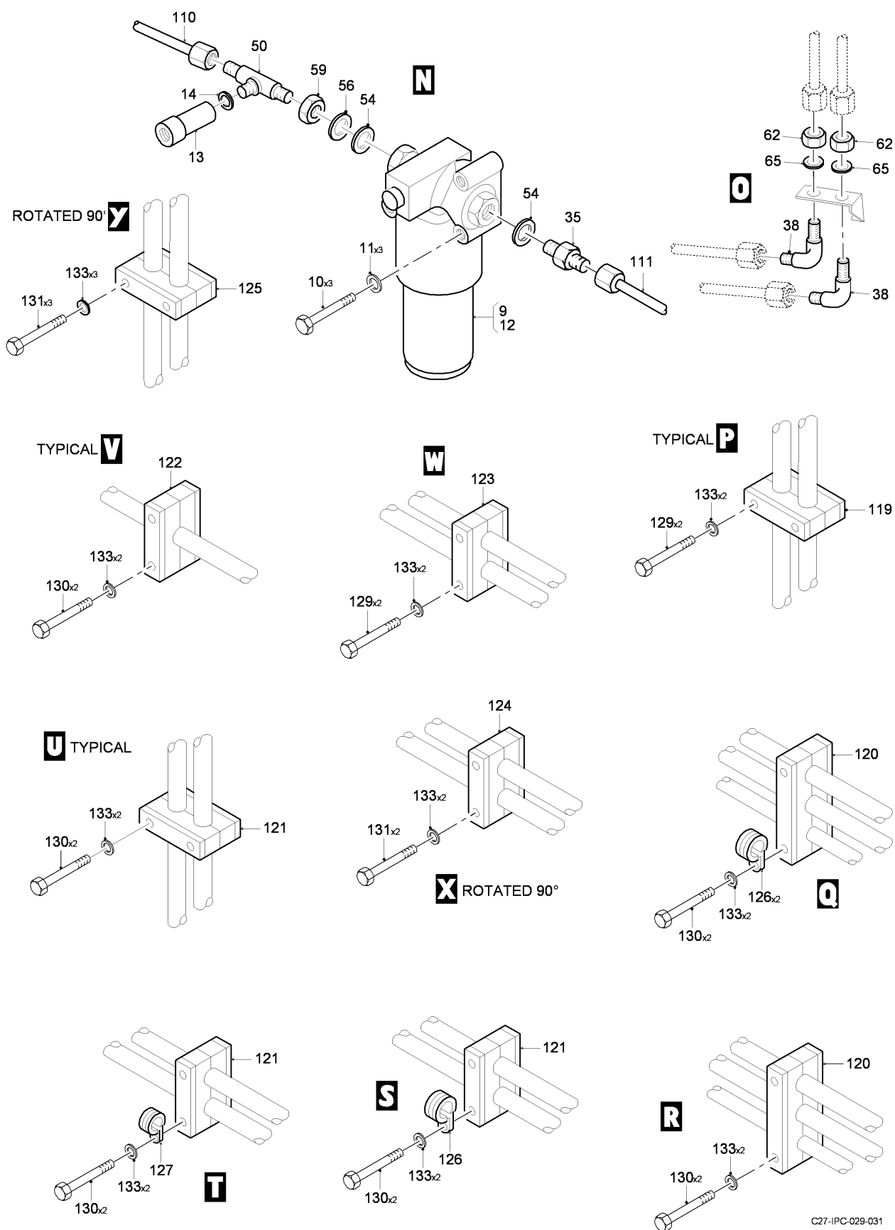
FIG 07 HYDRAULIC INSTL - MLG, Z13AB, LH (SHEET 7 OF 8)
