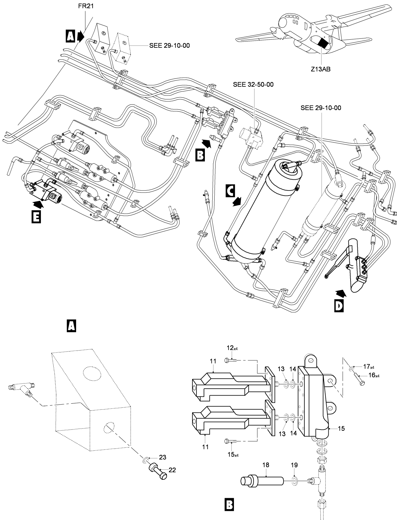
FIG 06 HYDRAULIC COMPONENT INSTL - MLG, Z13AB (SHEET 1 OF 2)
