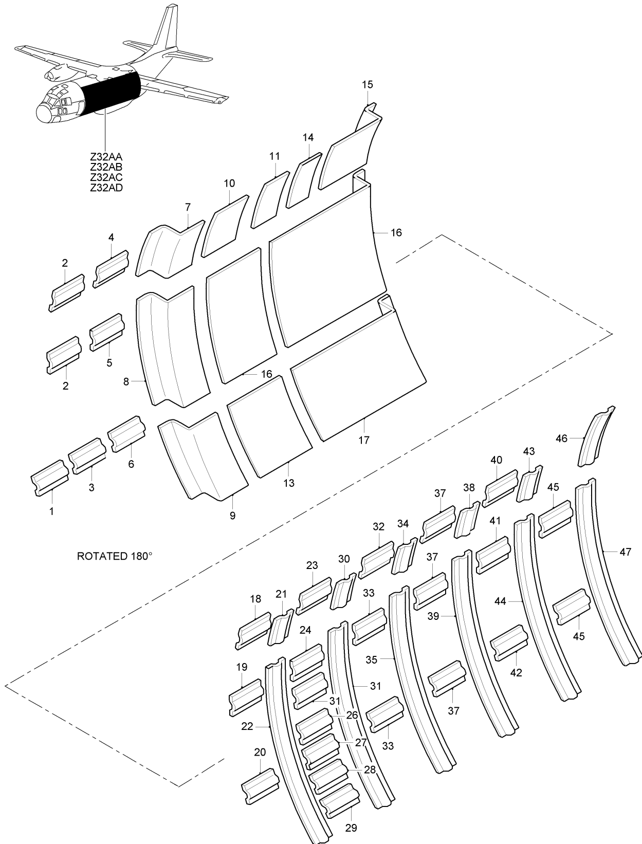
FIG 18 PRIMARY THERMAL INSULATION INSTL, Z32AA-32AB-32AC-32AD (SHEET 1 OF 1)
