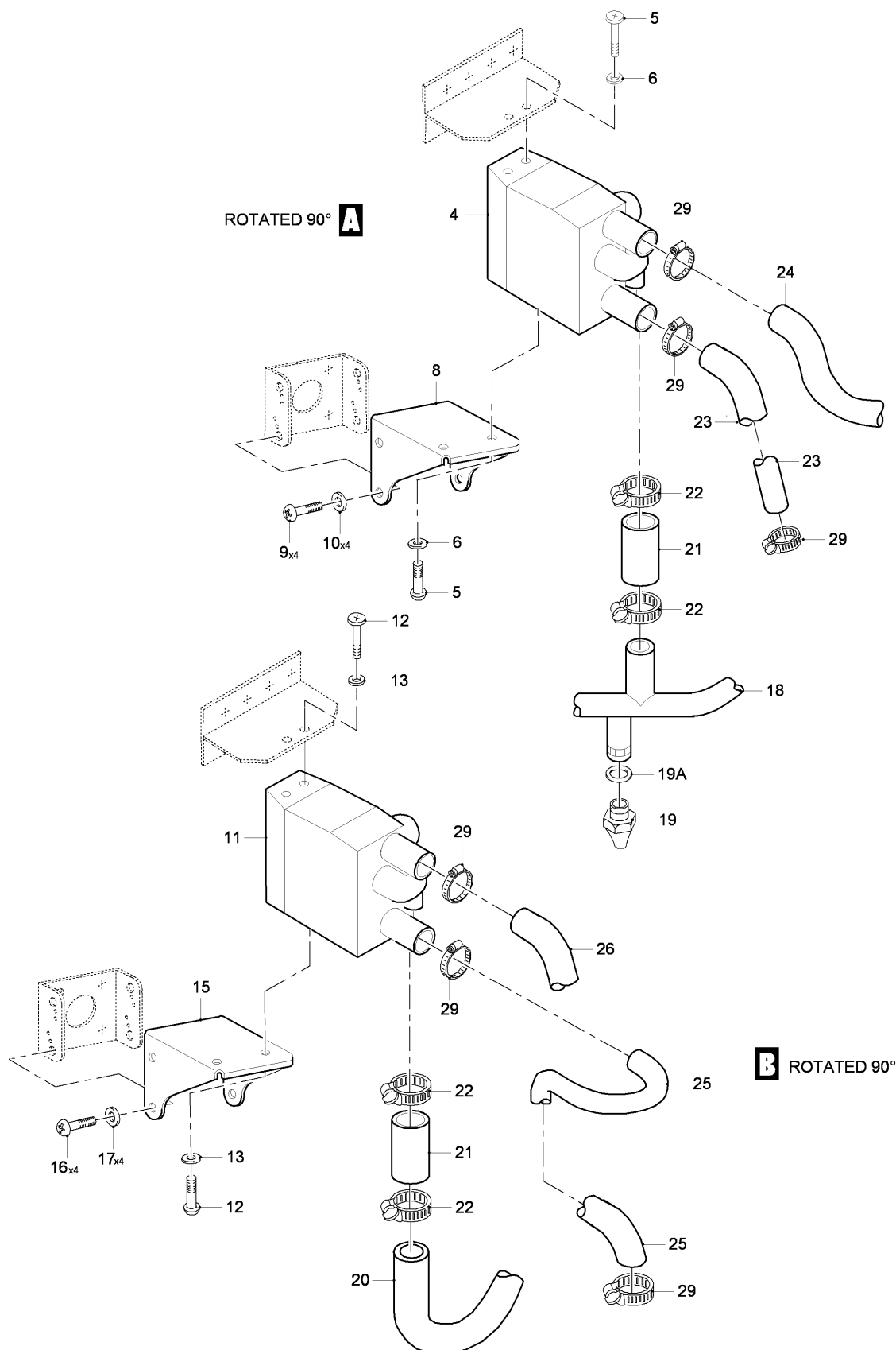
FIG 07 ANTI-ICING INSTL - OUTER WING, Z11AA, LH (SHEET 2 OF 3)
