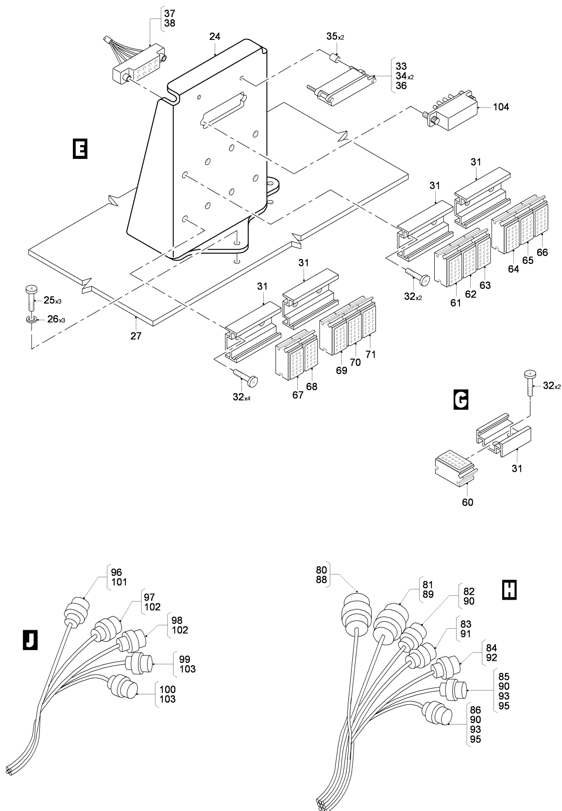
FIG 04 FOURTH SHELF INSTL - ELECTRONIC COMPARTMENT, Z31AA (SHEET 2 OF 3)
