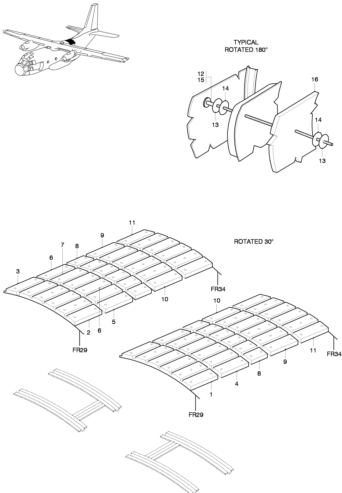
FIG 31 PRIMARY THERMAL INSULATION INSTL, Z34AA (SHEET 1 OF 1)
