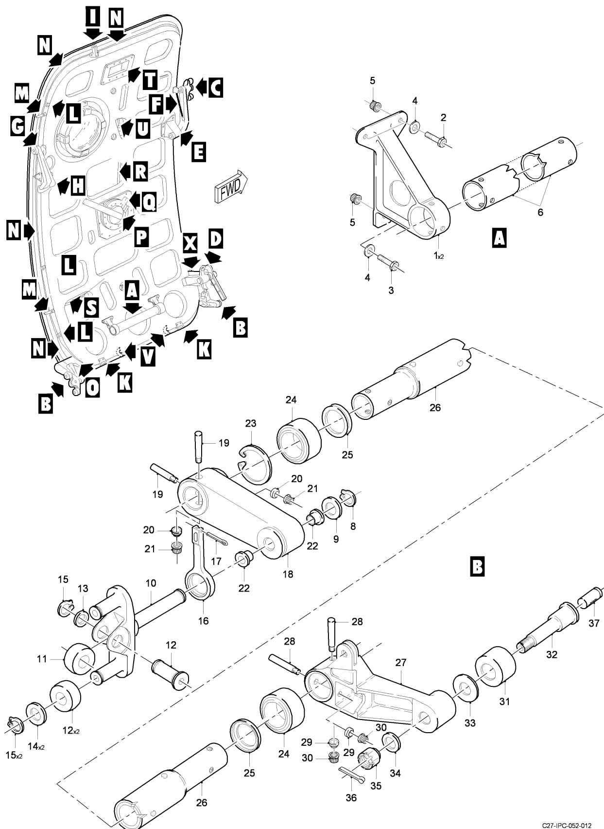
FIG 03 PARATROOPS DOOR ASSY, LH-RH (SHEET 1 OF 8)
