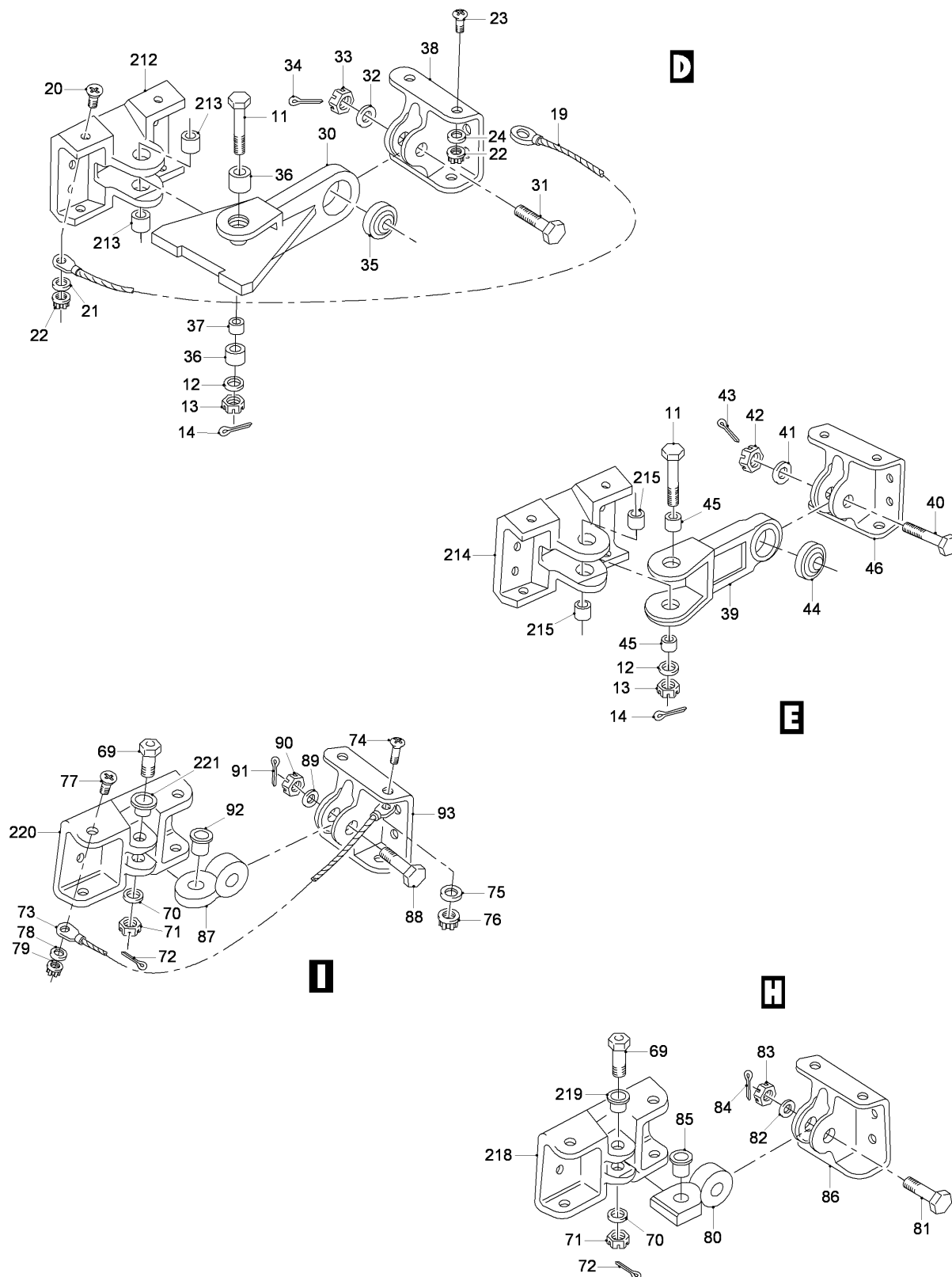
FIG 01 AILERON ASSY, LH-RH (SHEET 2 OF 5)
