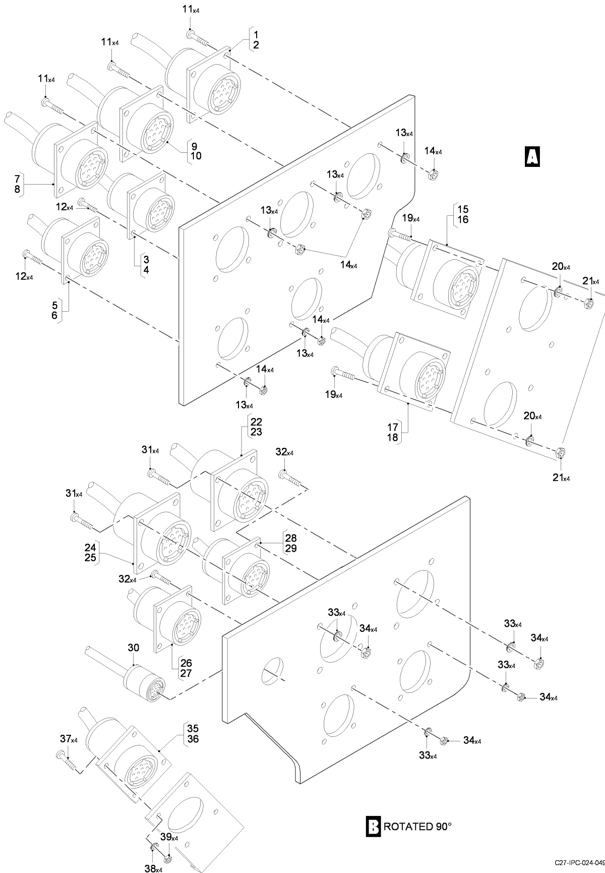
FIG 14 ELECTRICAL AND ELECTRONICS INSTL, Z31BC-31BD-32BA (SHEET 3 OF 11)
