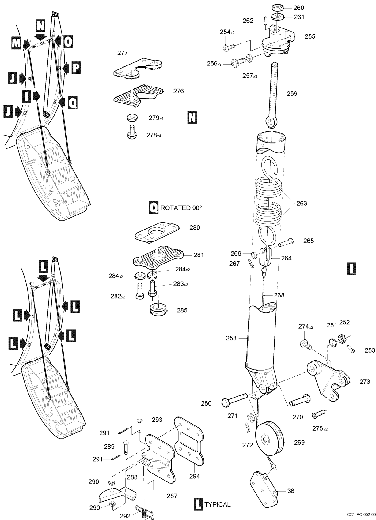
FIG 01 CREW DOOR INSTL, Z31AB (SHEET 6 OF 7)
