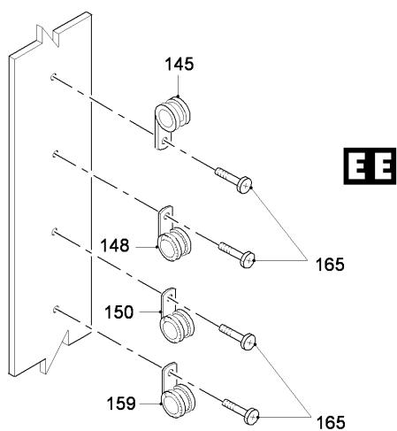
FIG 14 ELECTRICAL AND ELECTRONICS INSTL, Z31BC-31BD-32BA (SHEET 10 OF 11)
