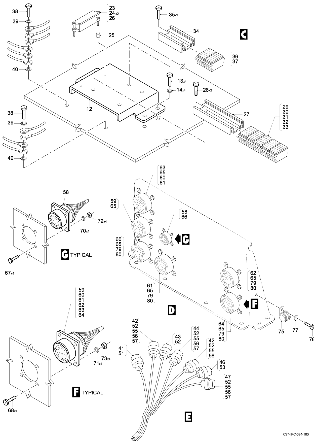
FIG 01 FIRST SHELF INSTL - ELECTRONIC COMPARTMENT, Z31AA (SHEET 2 OF 2)
