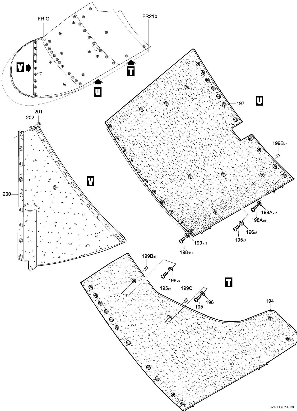
FIG 08 HYDRAULIC INSTL - MLG, Z23AB, RH (SHEET 7 OF 11)
