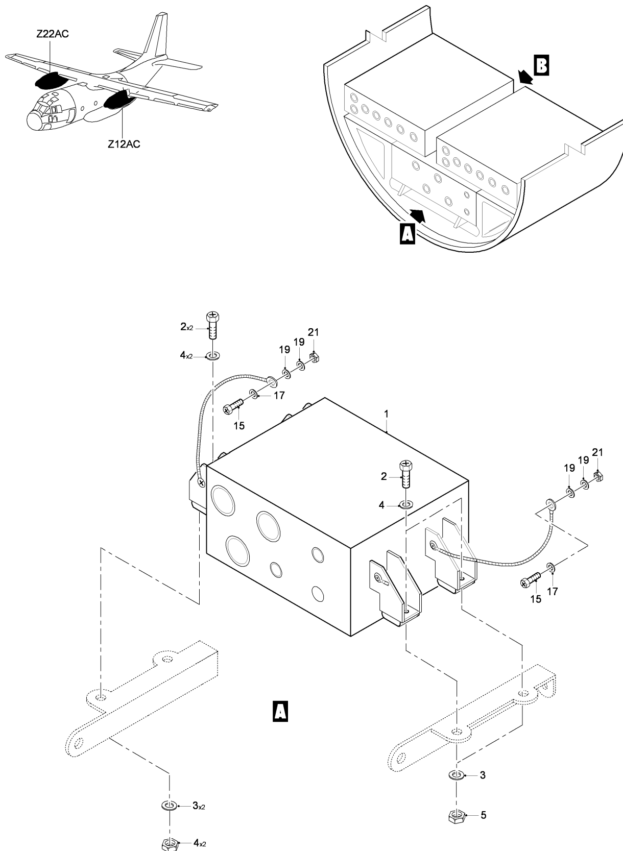
FIG 03 NIU AND FADEC INSTL, Z12AC-22AC (SHEET 1 OF 2)
