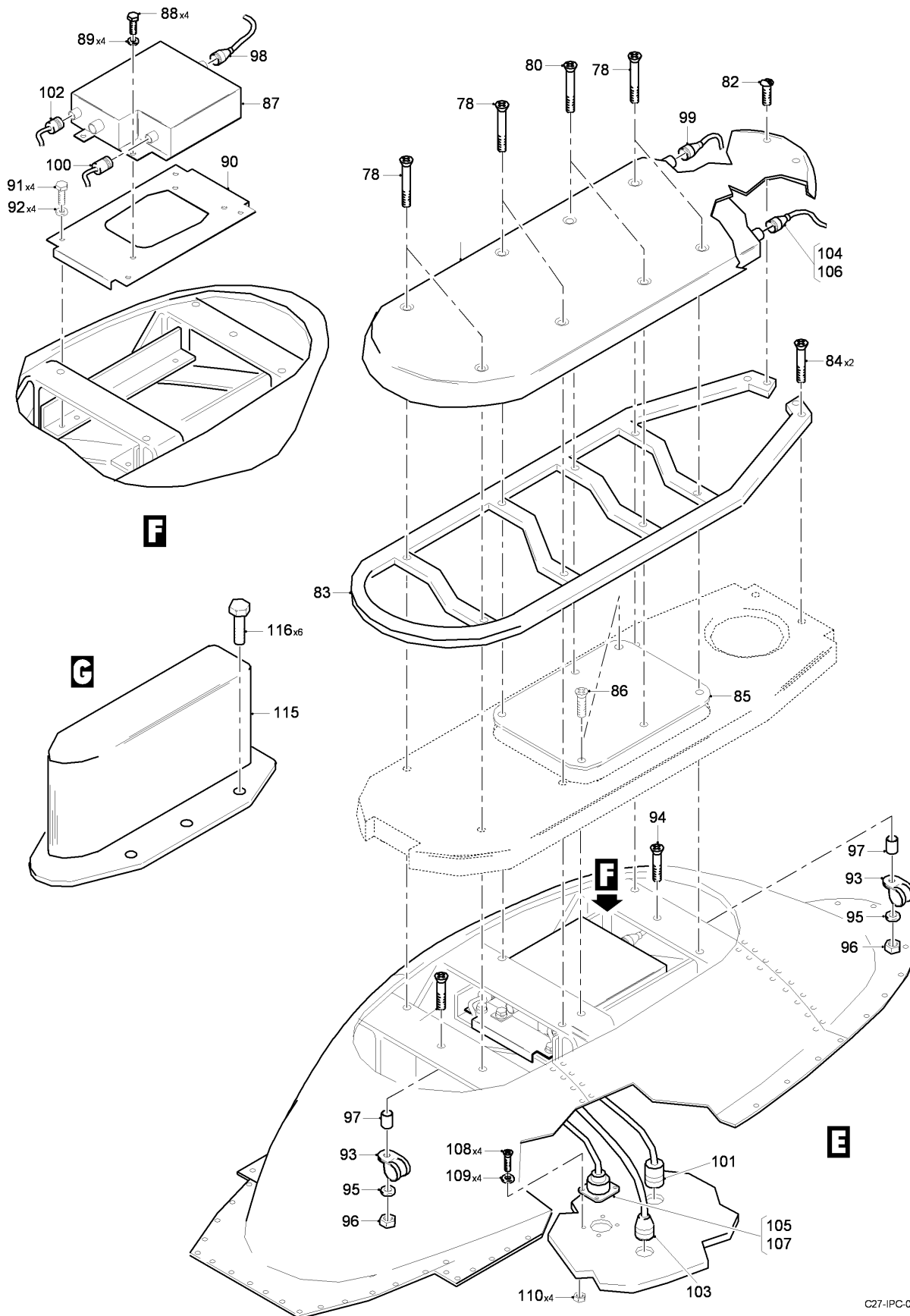
FIG 01 SATELLITE COMMUNICATION SYSTEM, Z32AA, Z32AD, Z32BA, Z34AA (SHEET 3 OF 3)
