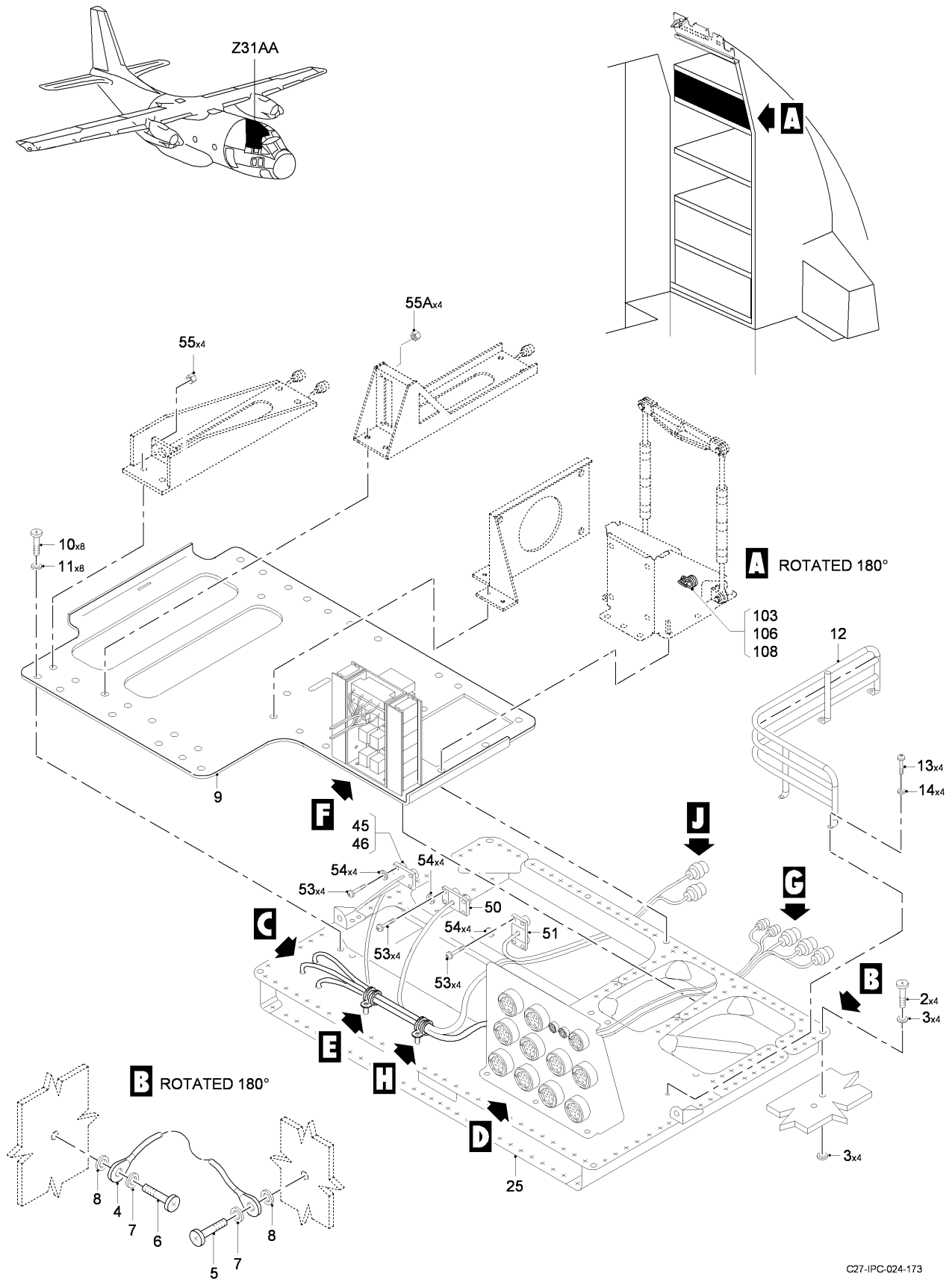
FIG 05 FIFTH SHELF INSTL - ELECTRONIC COMPARTMENT, Z31AA (SHEET 1 OF 3)
