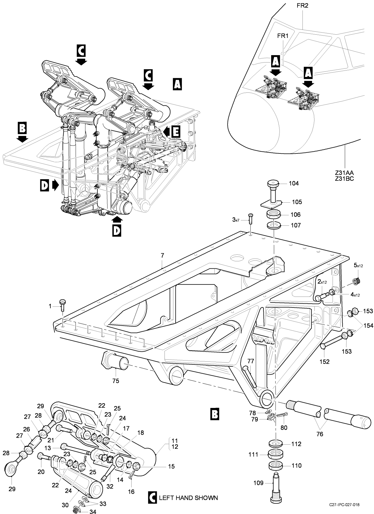
FIG 02 RUDDER PEDAL INSTL, Z31AA-31BC, LH-RH (SHEET 1 OF 2)
