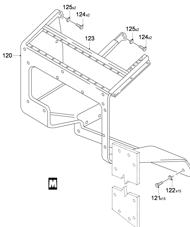
FIG 03 INSTRUMENTS PANELS INSTL, Z31AA (SHEET 5 OF 5)
