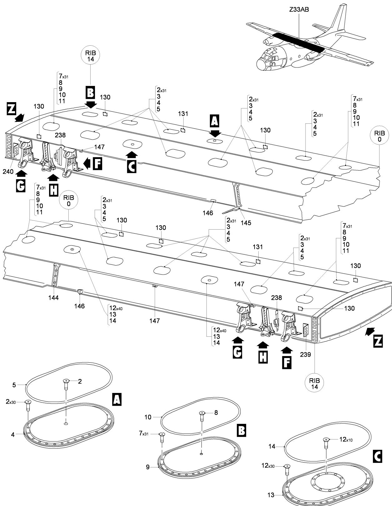
FIG 03 STRUCTURE INSTL - CENTER WING, Z33AB (SHEET 1 OF 5)
