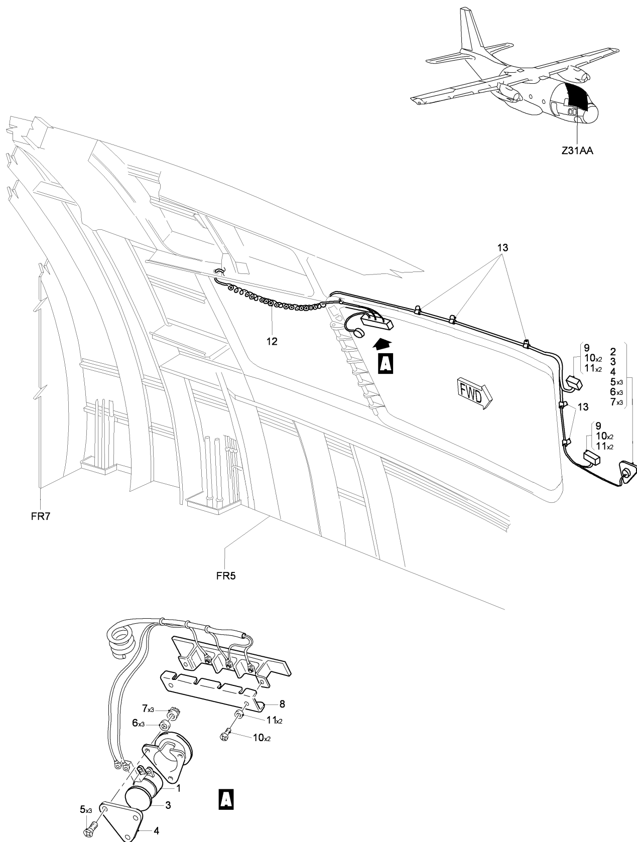
FIG 04 SWITCH THERMOSTATIC INSTL, Z31AA, LH (SHEET 1 OF 1)
