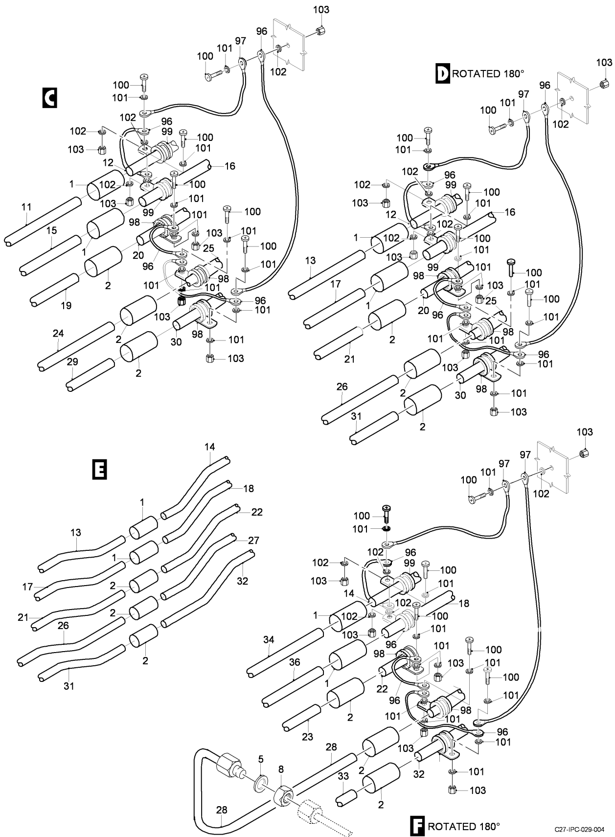
FIG 02 HYDRAULIC INSTL - CENTER FUSELAGE, LOWER, Z32BA (SHEET 2 OF 8)
