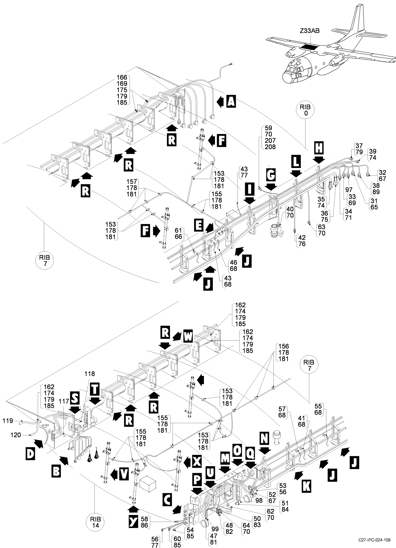
FIG 23 ELECTRICAL AND ELECTRONICS INSTL - CENTER WING, Z33AB, RH (SHEET 1 OF 6)
