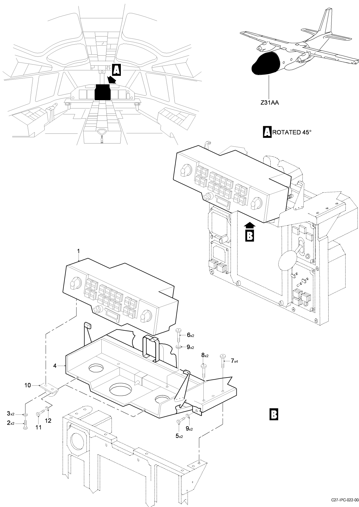
FIG 04 DA/FD CONTROL PANEL INSTL, Z31AA (SHEET 1 OF 1)
