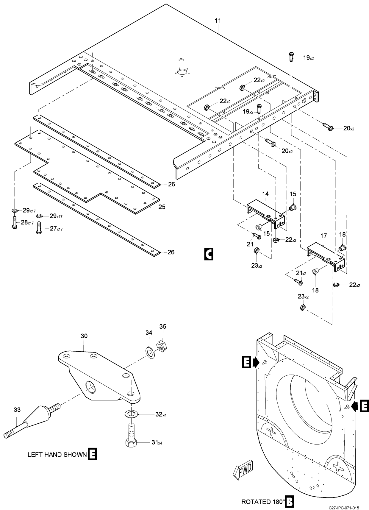
FIG 01 FIREWALL INSTL - NACELLE ENGINE, Z12AB-22AB (SHEET 2 OF 2)
