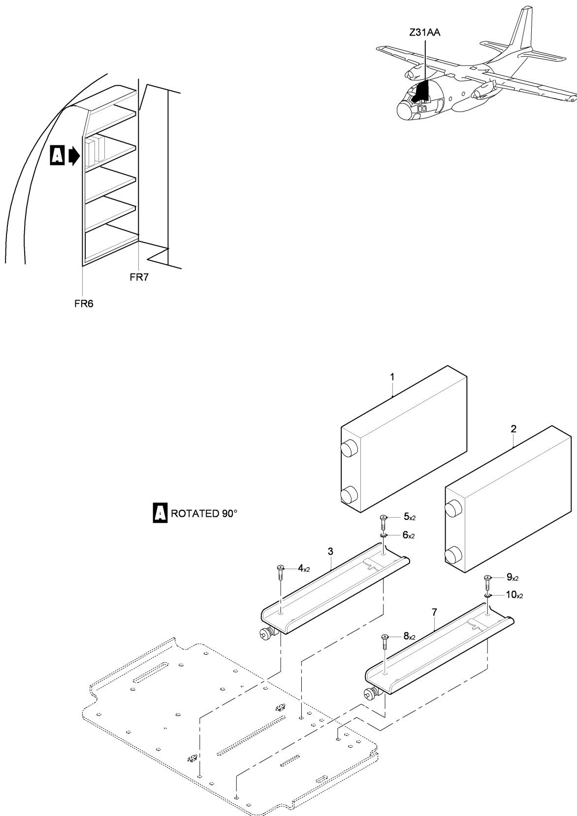
FIG 07 WINDSHIELD ANTI-ICE CONTROLLER INSTL, Z31AA (SHEET 1 OF 1)
