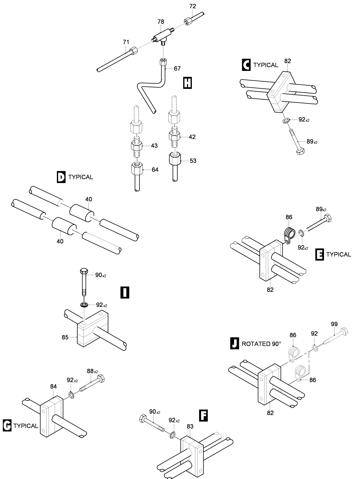
FIG 05 ELEVATOR AND RUDDER HYDRAULIC ACCUMULATOR INSTL, Z34AA, LH (SHEET 3 OF 3)
