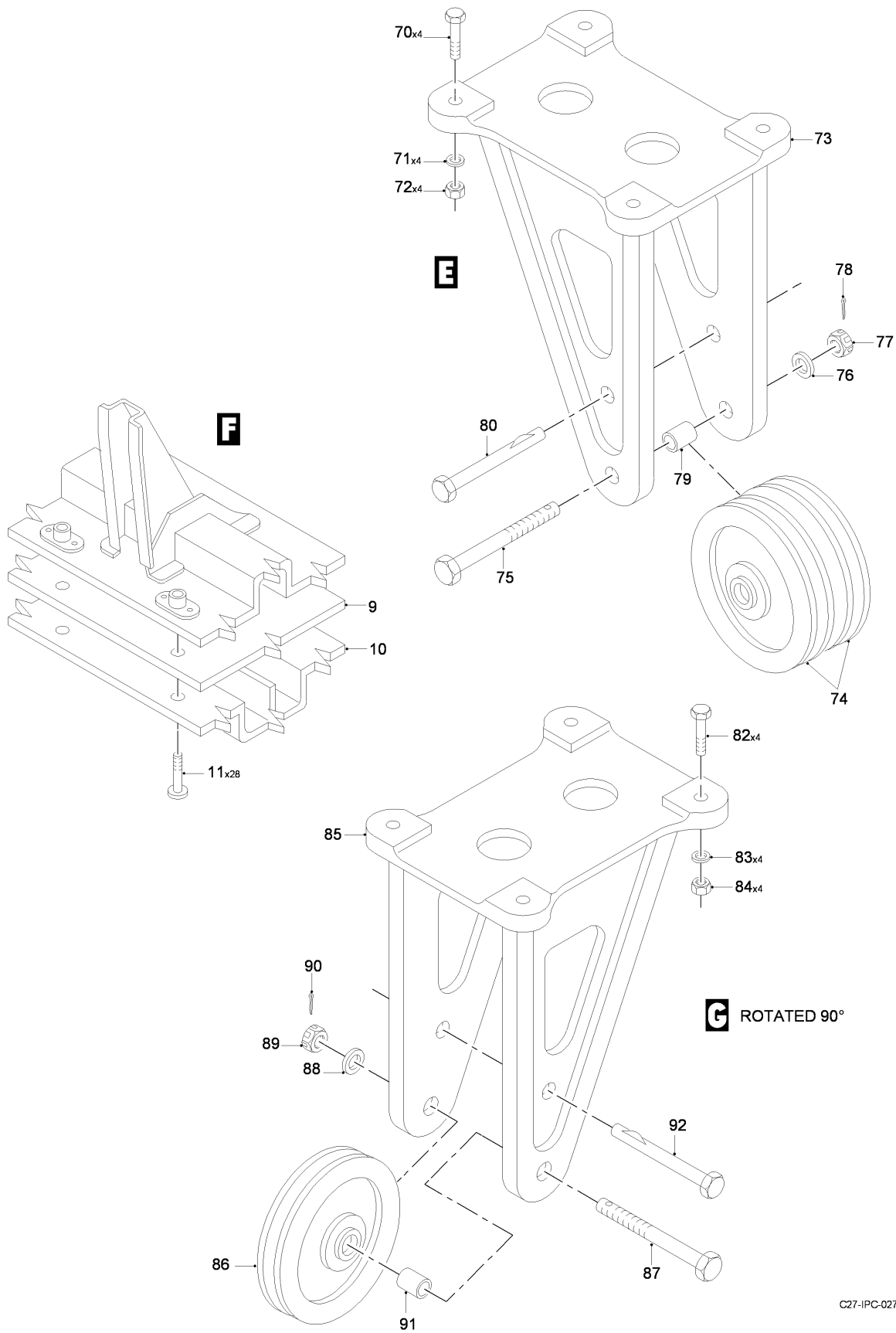
FIG 09 ELEVATOR EMERGENCY TRIM INSTL, Z34AA (SHEET 4 OF 4)
