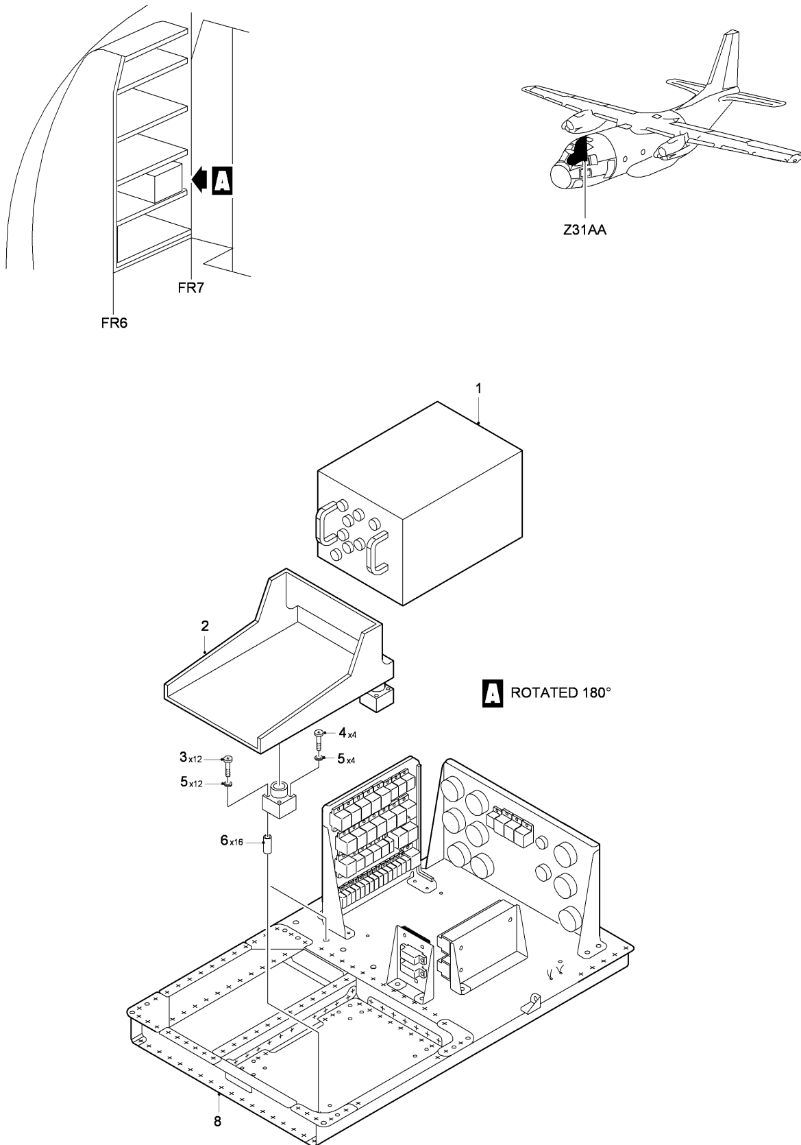
FIG 03 BUS INTERFACE UNIT INSTL - ELECTRICAL COMPARTMENT, Z31AA (SHEET 1 OF 1)
