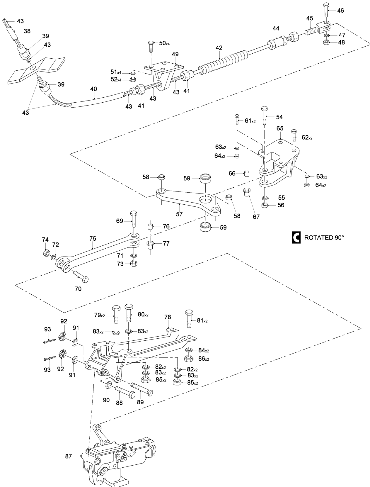
FIG 02 EMERGENCY CONTROL INSTL - MAIN LANDING GEAR, Z31AA (SHEET 3 OF 3)
