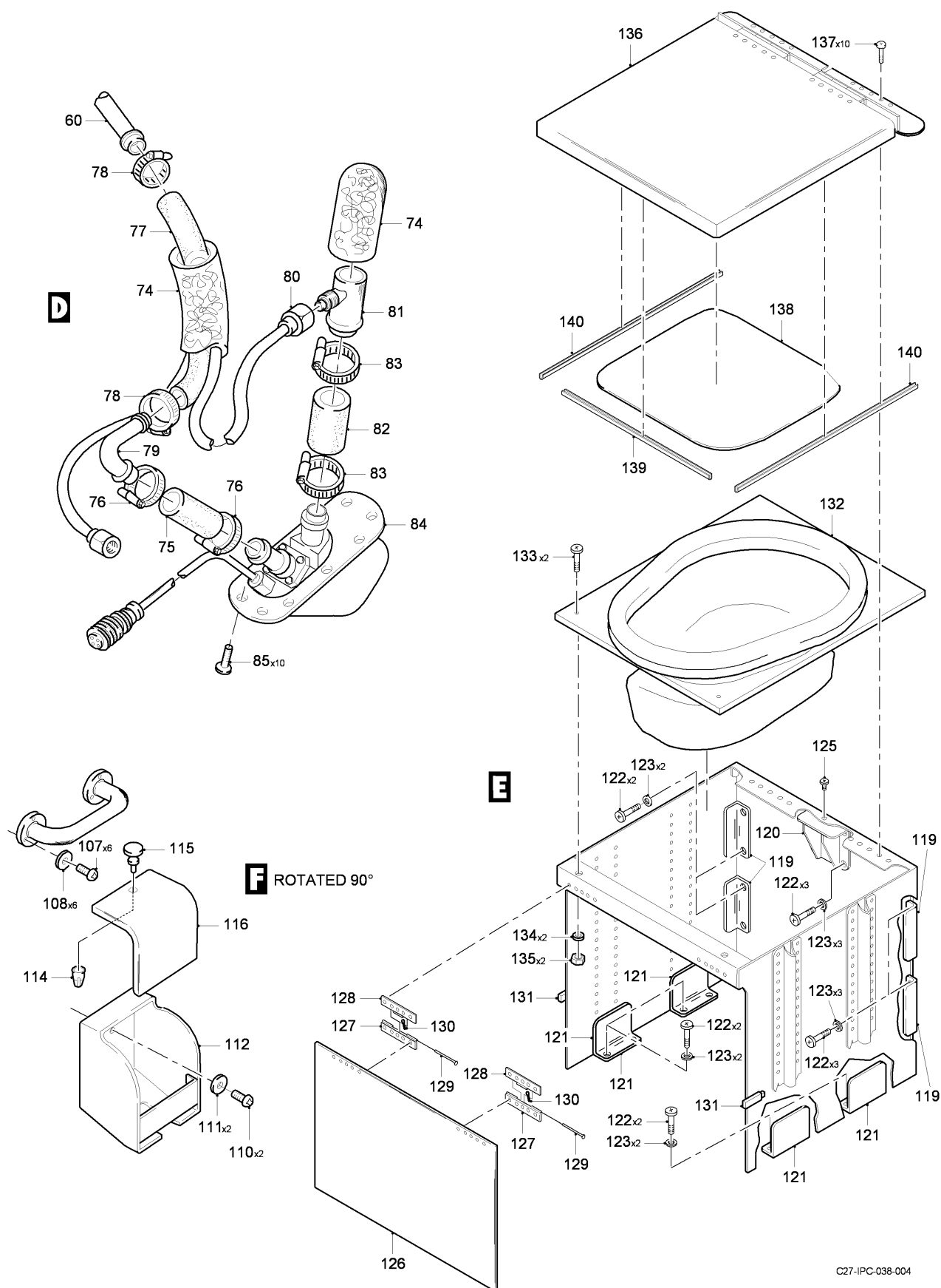
FIG 01 TOILET INSTL, Z31AB (SHEET 3 OF 3)
