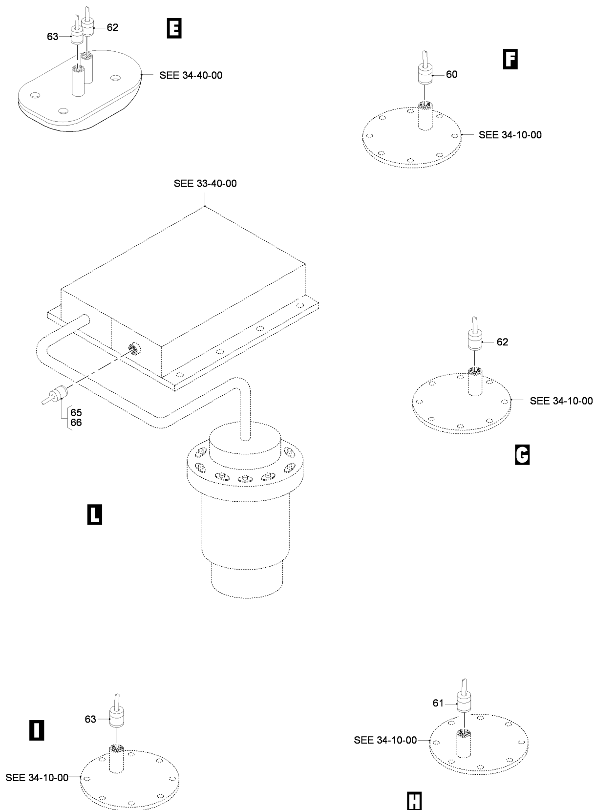
FIG 14 ELECTRICAL AND ELECTRONICS INSTL, Z31BC-31BD-32BA (SHEET 5 OF 11)
