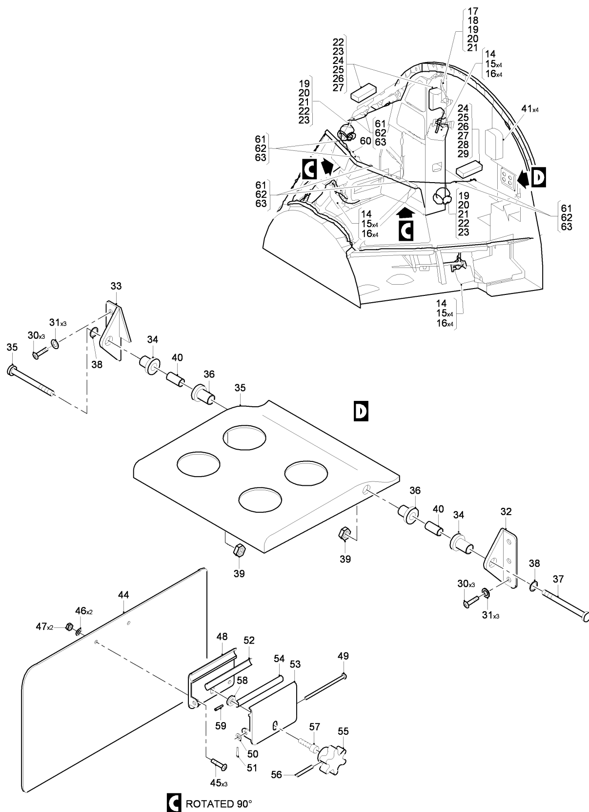
FIG 01 EMERGENCY EQUIPMENT INSTL, Z31-32-34 (SHEET 2 OF 2)
