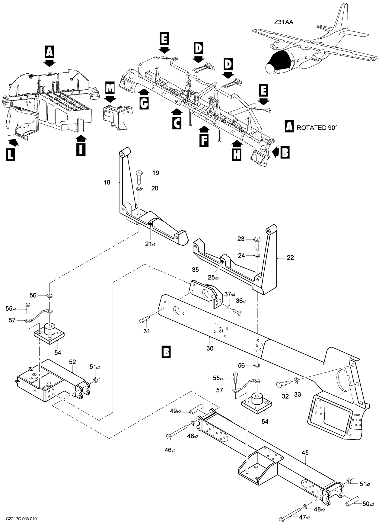
FIG 03 INSTRUMENTS PANELS INSTL, Z31AA (SHEET 1 OF 5)
