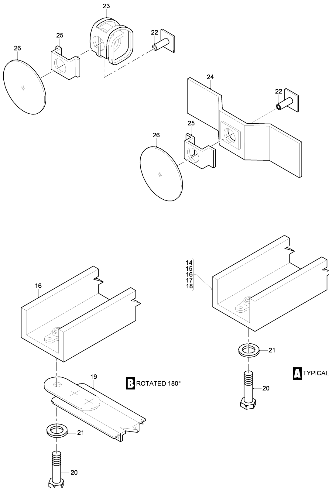
FIG 36 SECONDARY THERMAL INSULATION INSTL, OVERHEAD, Z34AA (SHEET 2 OF 2)
