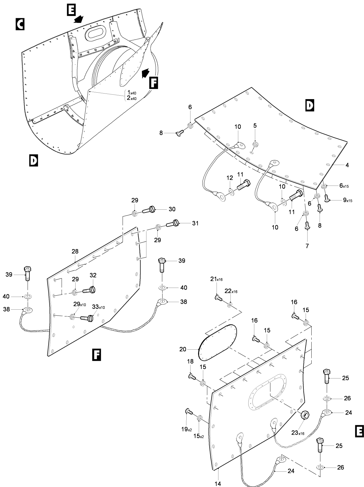
FIG 03 FAIRING LOWER INSTL - NACELLE ENGINE, Z12AD-22AD (SHEET 2 OF 2)
