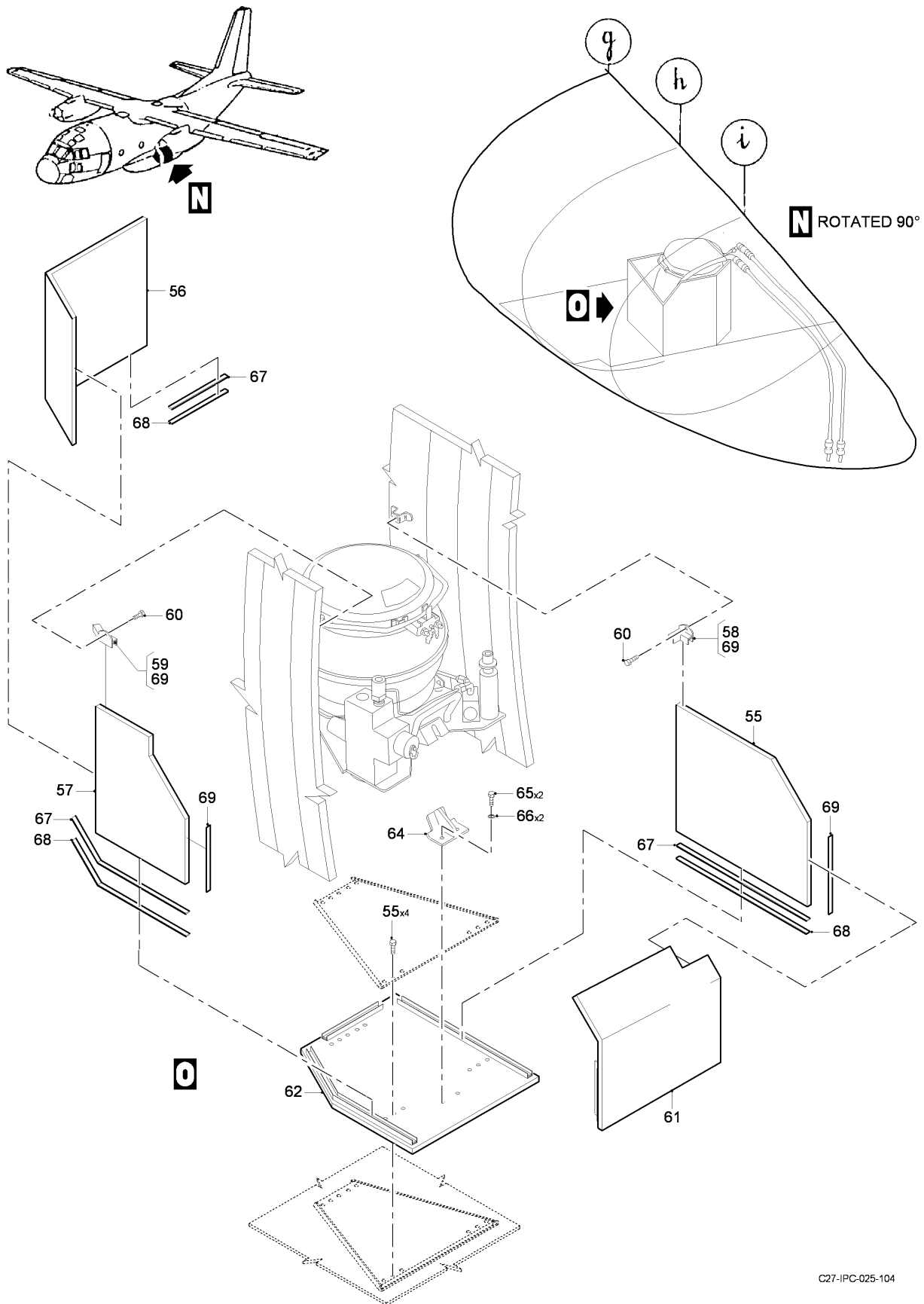
FIG 20 KIT G, BALLISTIC PROTECTION, Z13AC-Z23AC-Z31AA-Z31BA-Z34AA (SHEET 6 OF 6)
