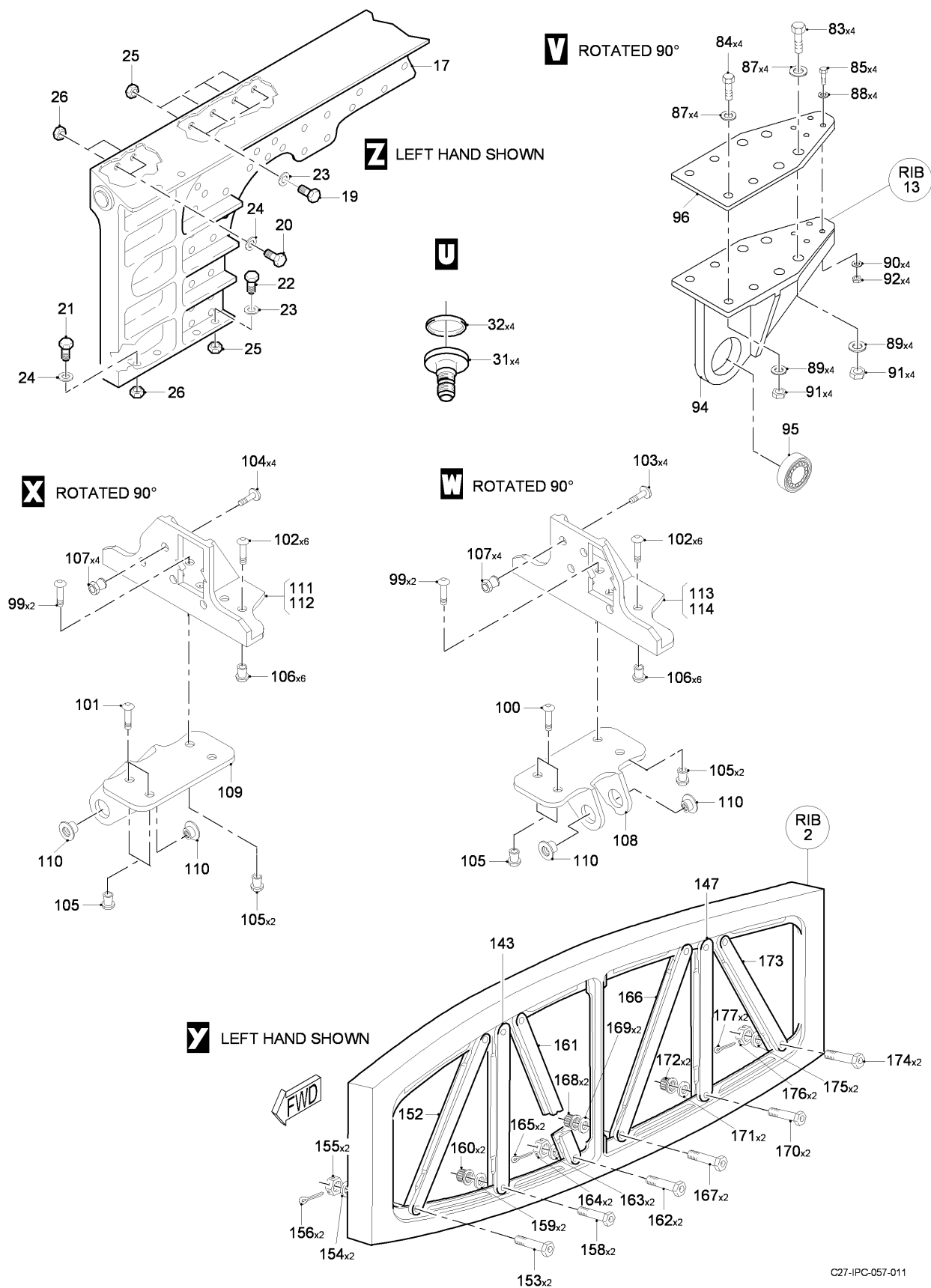
FIG 03 STRUCTURE INSTL - CENTER WING, Z33AB (SHEET 5 OF 5)
