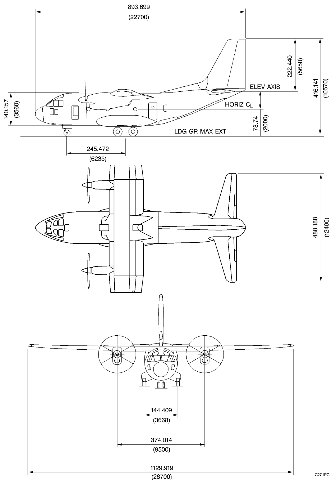
Figure 1-2. AIRCRAFT OVERALL DIMENSION (Sheet 1 of 1)
