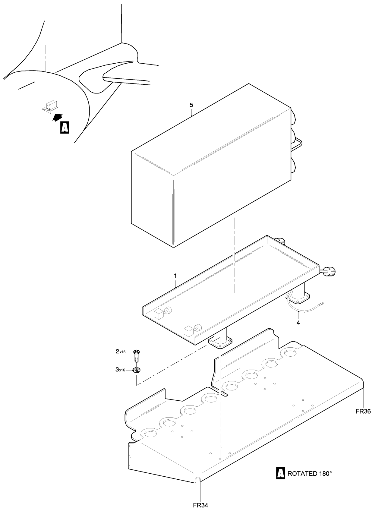
FIG 13 RADIO HF, HP ACP INSTL, Z34AA (SHEET 1 OF 1)
