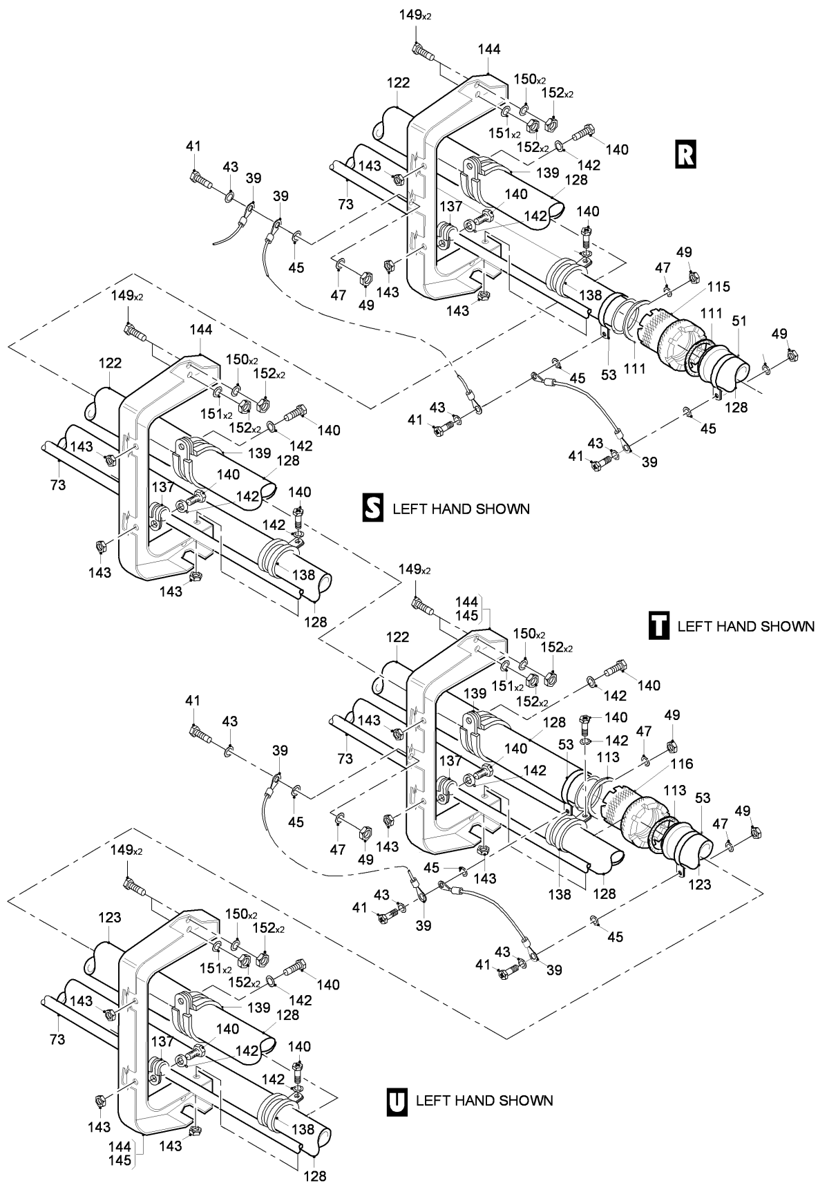
FIG 04 SINGLE POINT REFUELLING AND FUEL SUPPLY INSTL, Z33AB, LH-RH (SHEET 4 OF 6)
