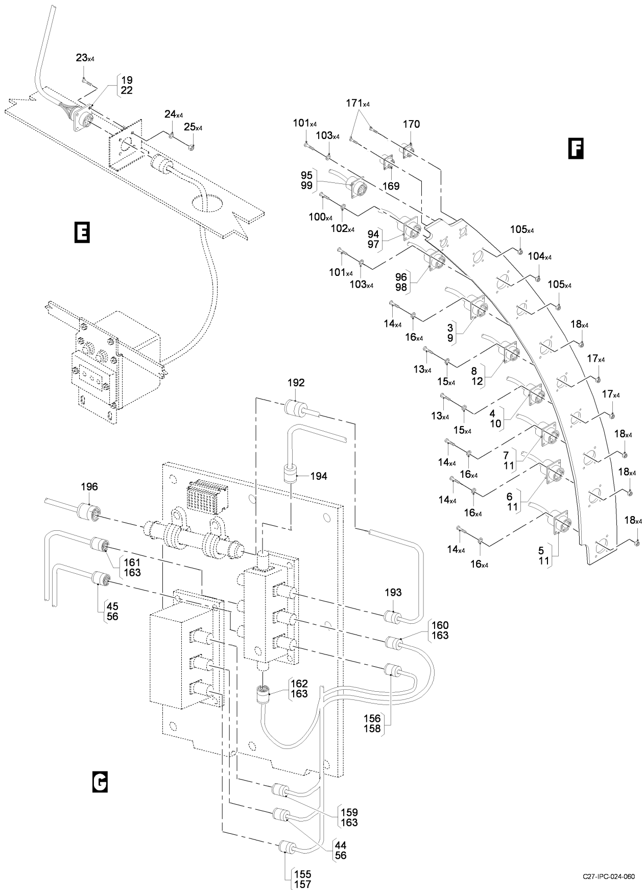
FIG 15 ELECTRICAL AND ELECTRONICS INSTL, Z31AB-32AA-32AB-32AC, LH (SHEET 4 OF 9)
