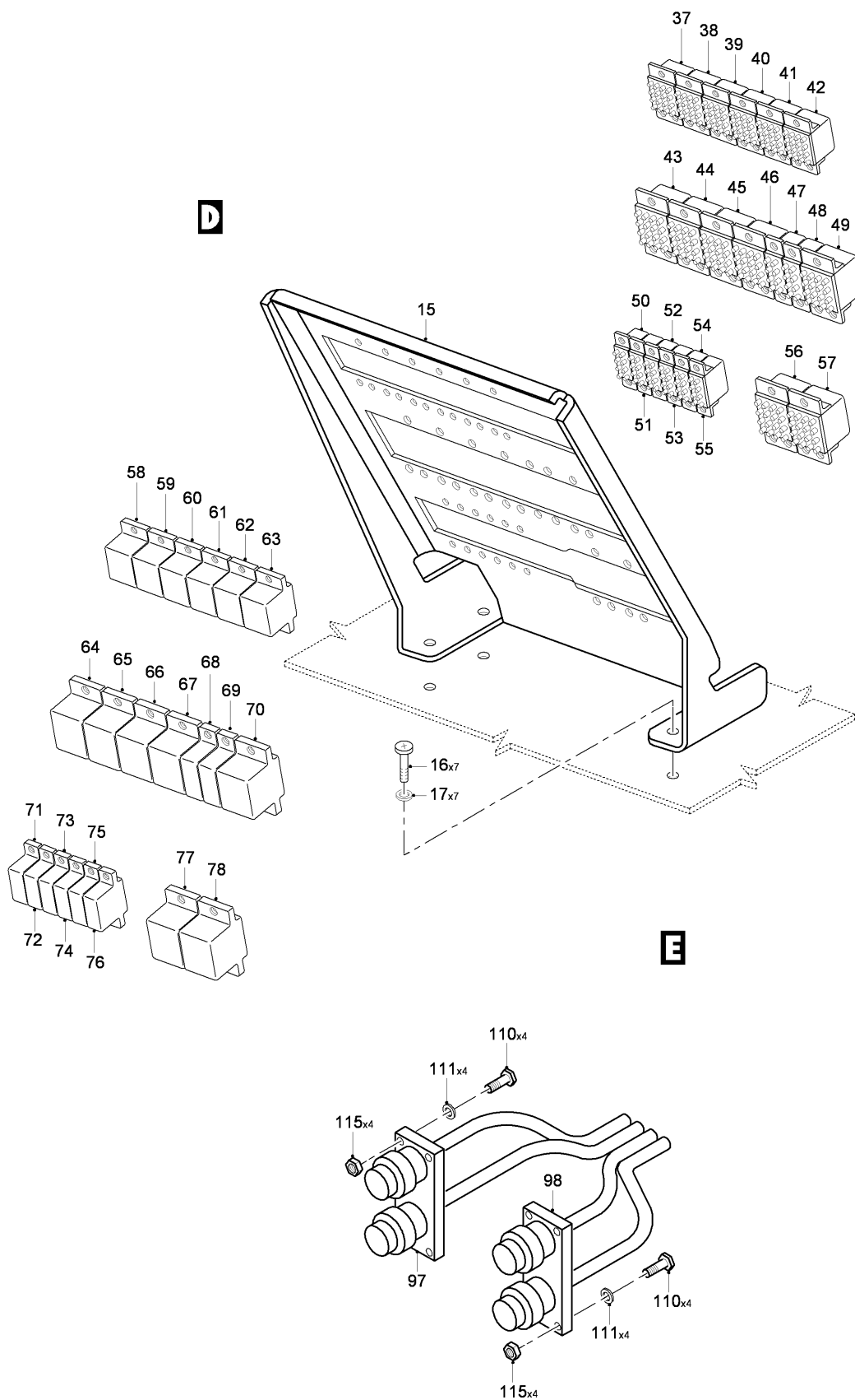
FIG 11 FIFTH AND SIXTH SHELF INSTL - ELECTRICAL COMPARTMENT, Z31AA (SHEET 3 OF 4)
