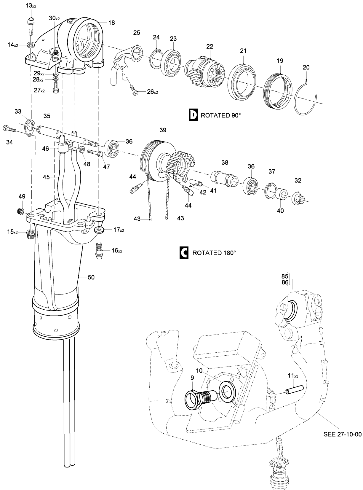
FIG 01 CONTROL COLUMN INSTL, Z31AA, LH-RH (SHEET 2 OF 3)
