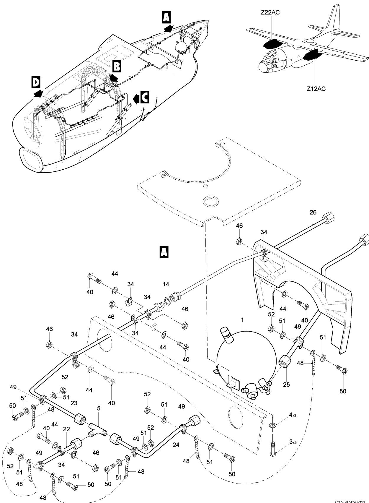
FIG 03 ENGINE FIRE EXTINGUISHING INSTL, Z12AC-12AD-22AC-22AD (SHEET 1 OF 3)
