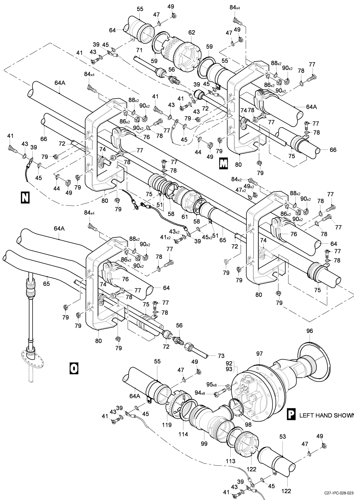
FIG 04 SINGLE POINT REFUELLING AND FUEL SUPPLY INSTL, Z33AB, LH-RH (SHEET 3 OF 6)
