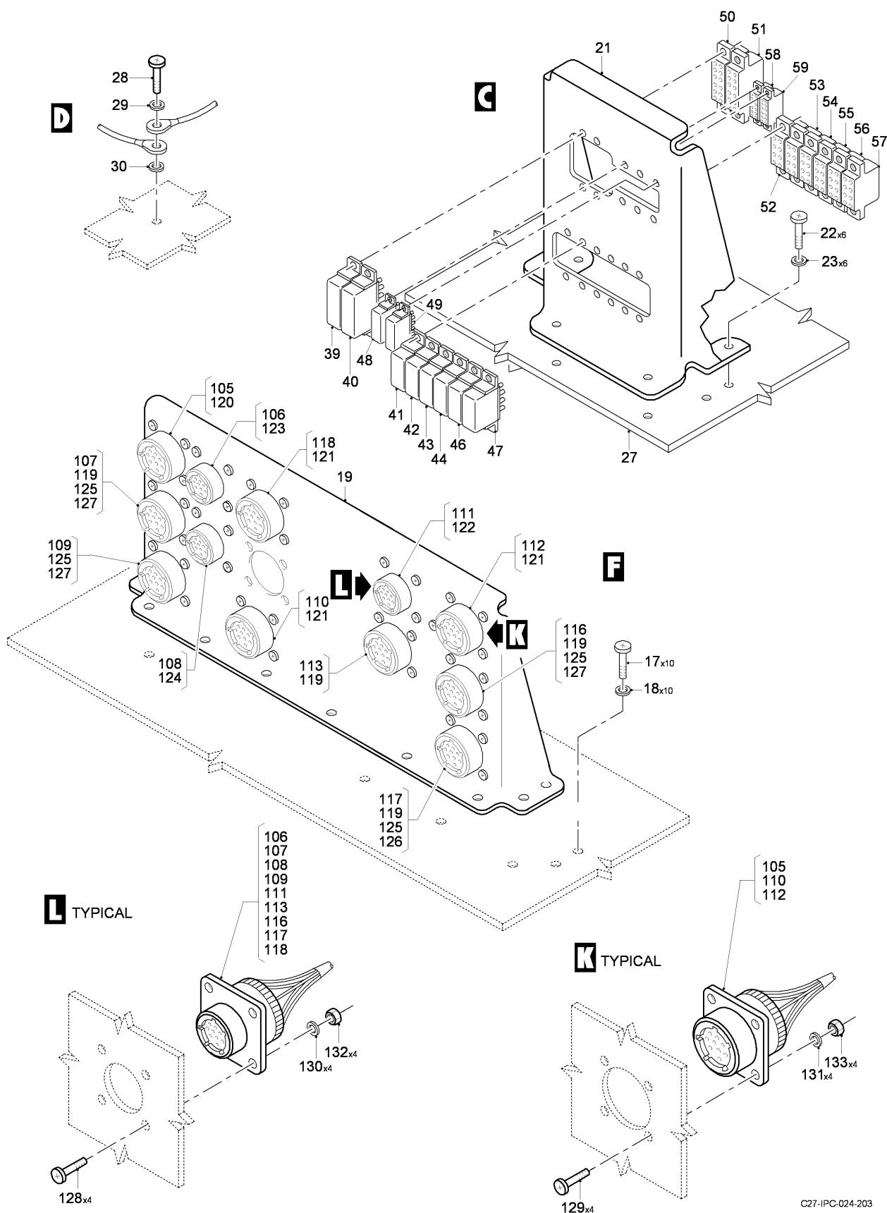
FIG 04 FOURTH SHELF INSTL - ELECTRONIC COMPARTMENT, Z31AA (SHEET 3 OF 3)
