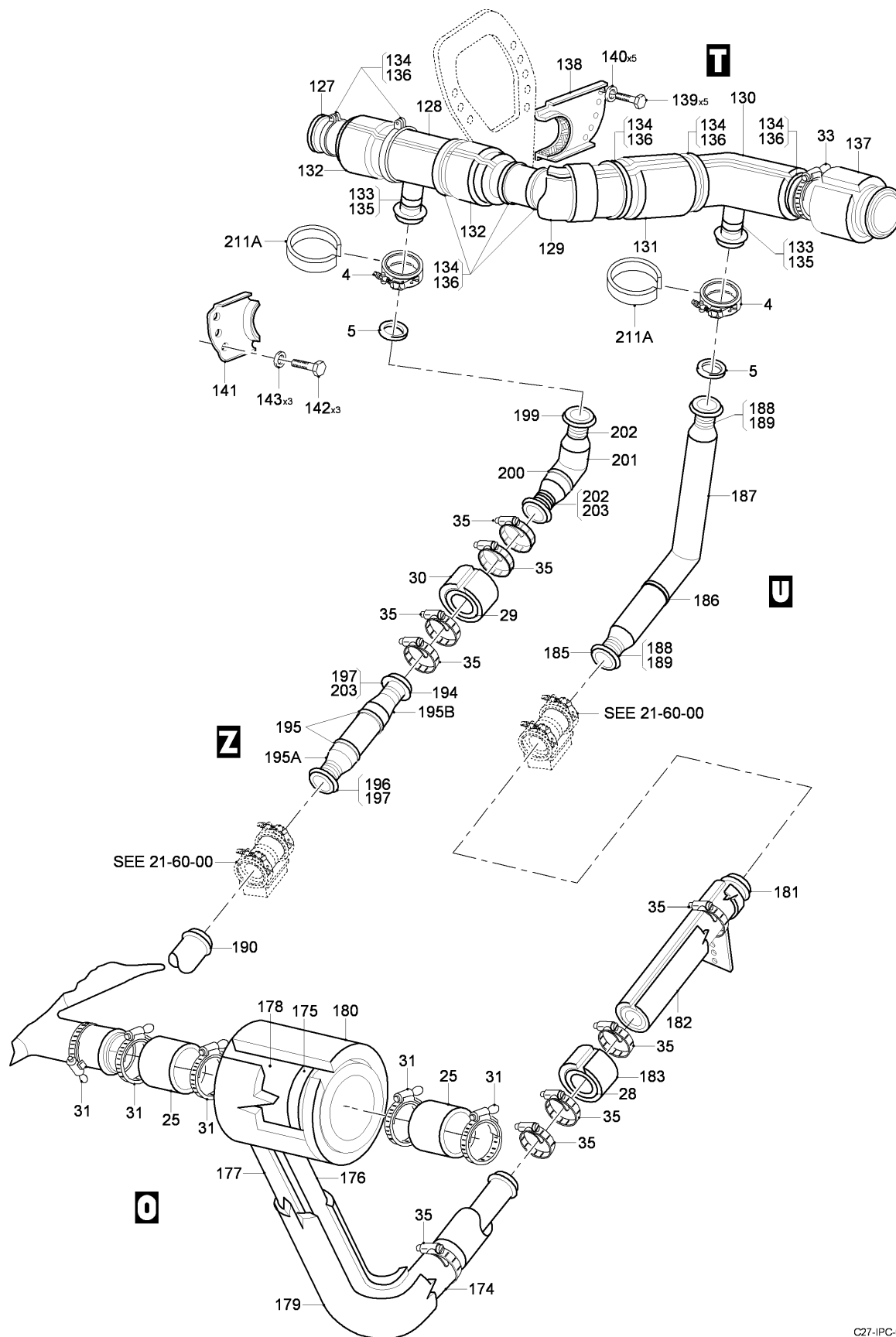
FIG 04 AIR CONDITIONING INSTL - CENTER FUSELAGE, Z32BA-32AB (SHEET 7 OF 7)
