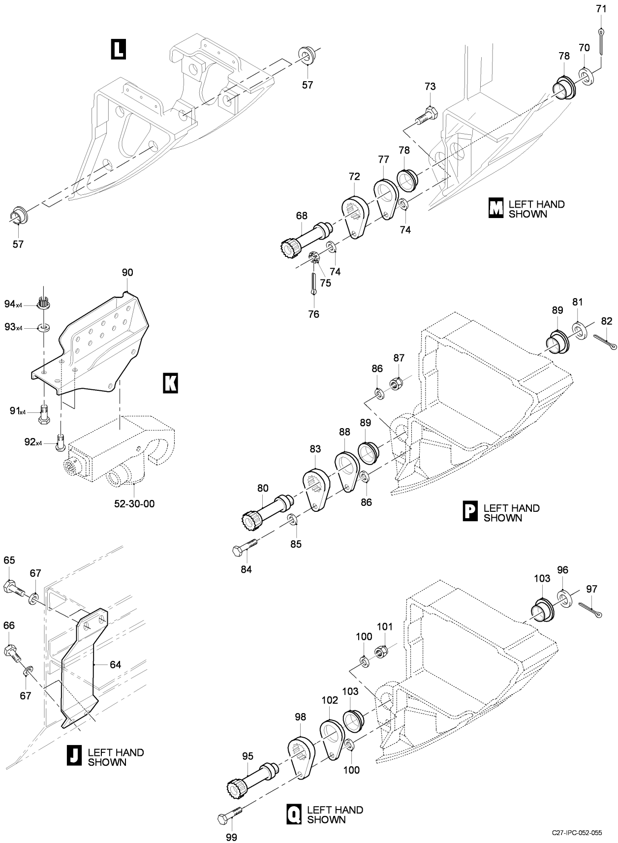
FIG 11 CARGO DOOR INSTL, Z34AA-34BB (SHEET 3 OF 3)
