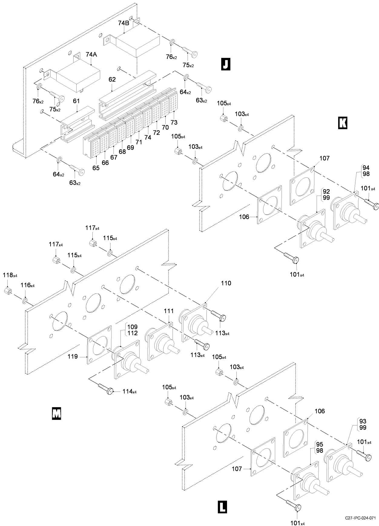
FIG 16 ELECTRICAL AND ELECTRONICS INSTL, Z31AB-32AA-32AB-32AC, RH (SHEET 7 OF 8)
