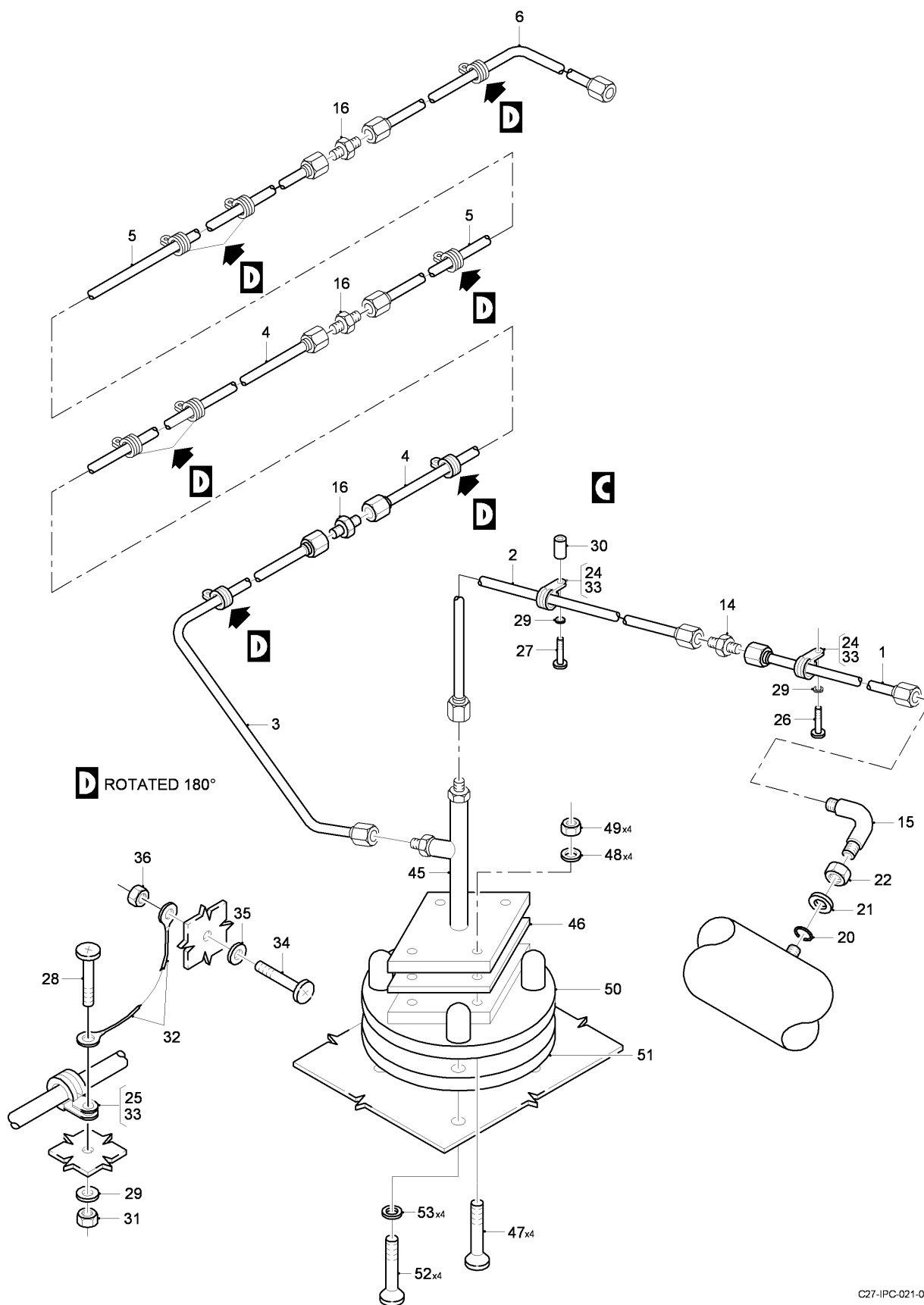
FIG 03 PRESSURIZATION INSTL - FWD FUSELAGE, Z32AB-32AC (SHEET 3 OF 3)
