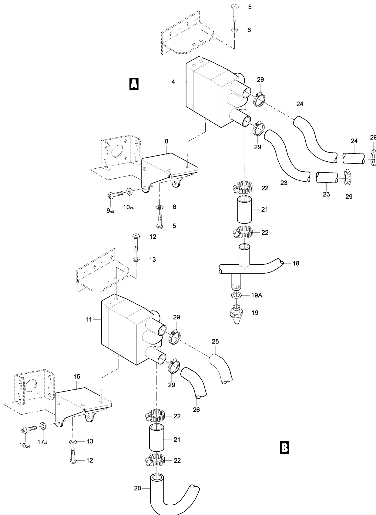
FIG 08 ANTI-ICING INSTL - OUTER WING, Z21AA, RH (SHEET 2 OF 3)
