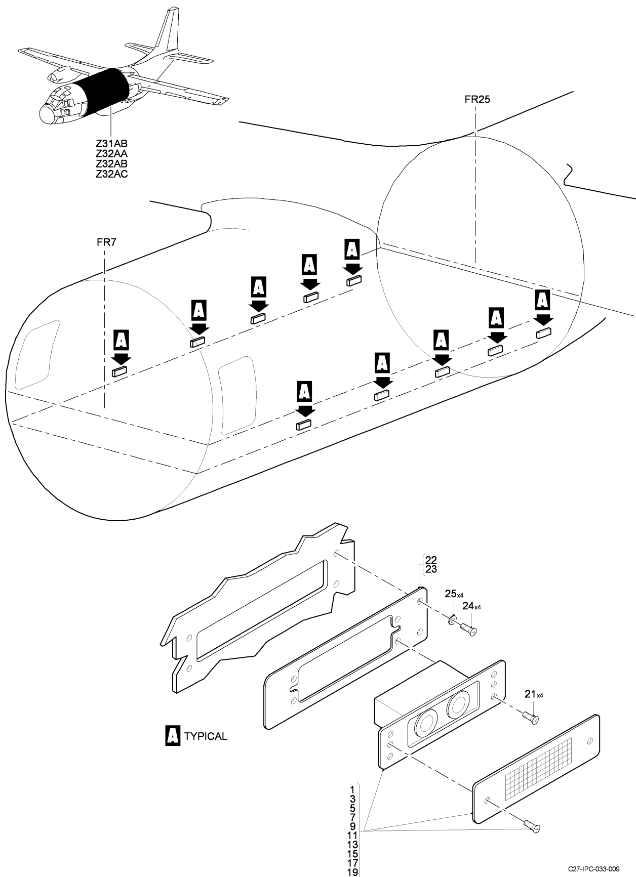
FIG 03 FLOOR LIGHT INSTL, Z31AB-32AA-32AB-32AC (SHEET 1 OF 1)
