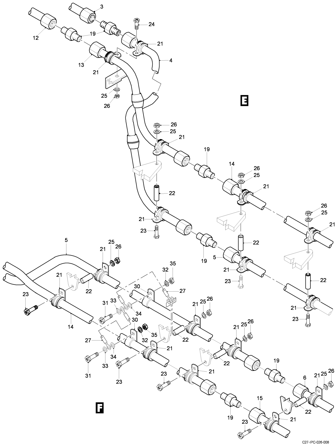
FIG 01 ENGINE FIRE EXTINGUISHING INSTL - CENTER WING, Z33AB (SHEET 3 OF 4)
