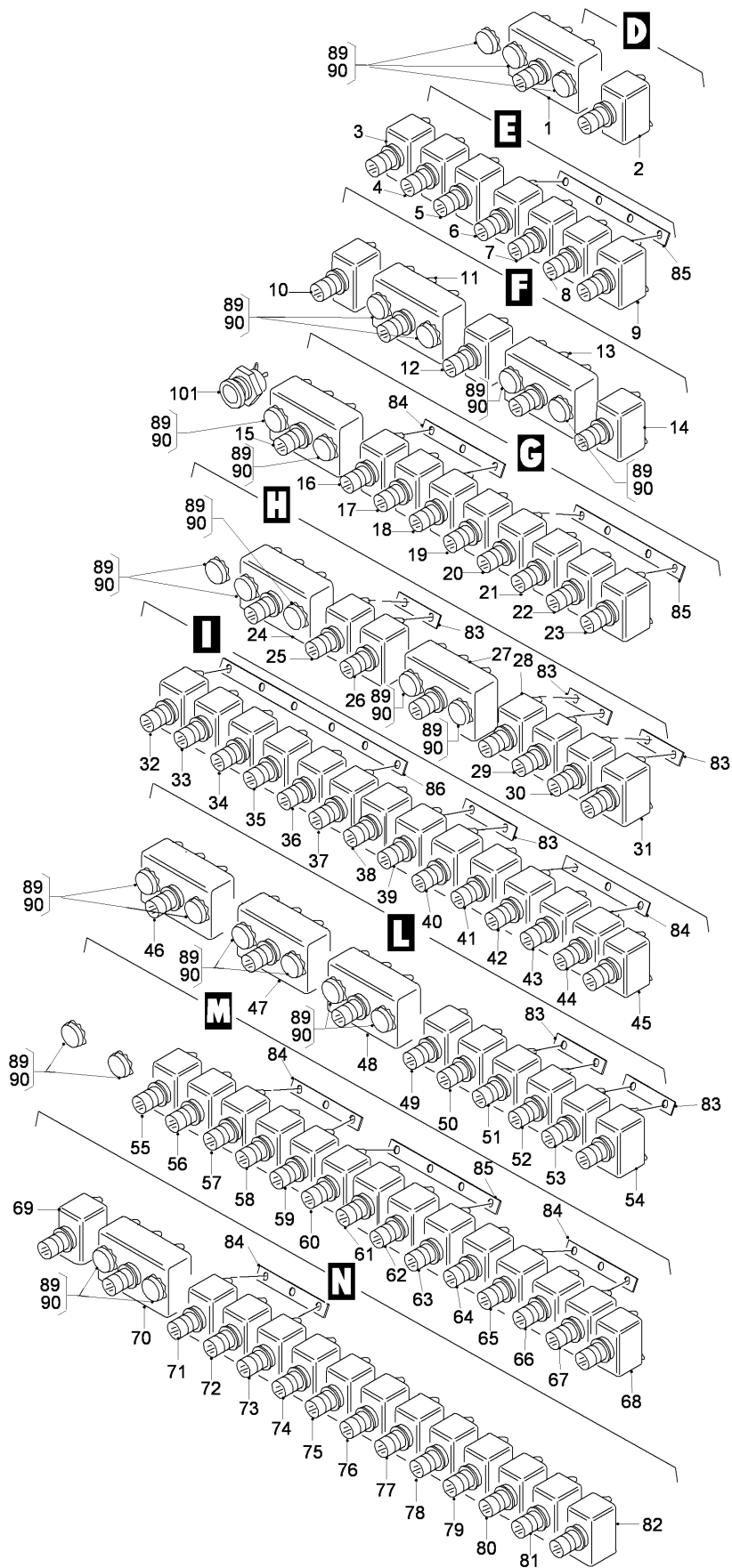
FIG 02 CIRCUIT BREAKER PANEL NO. 1 INSTL, Z31AA (SHEET 3 OF 3)
