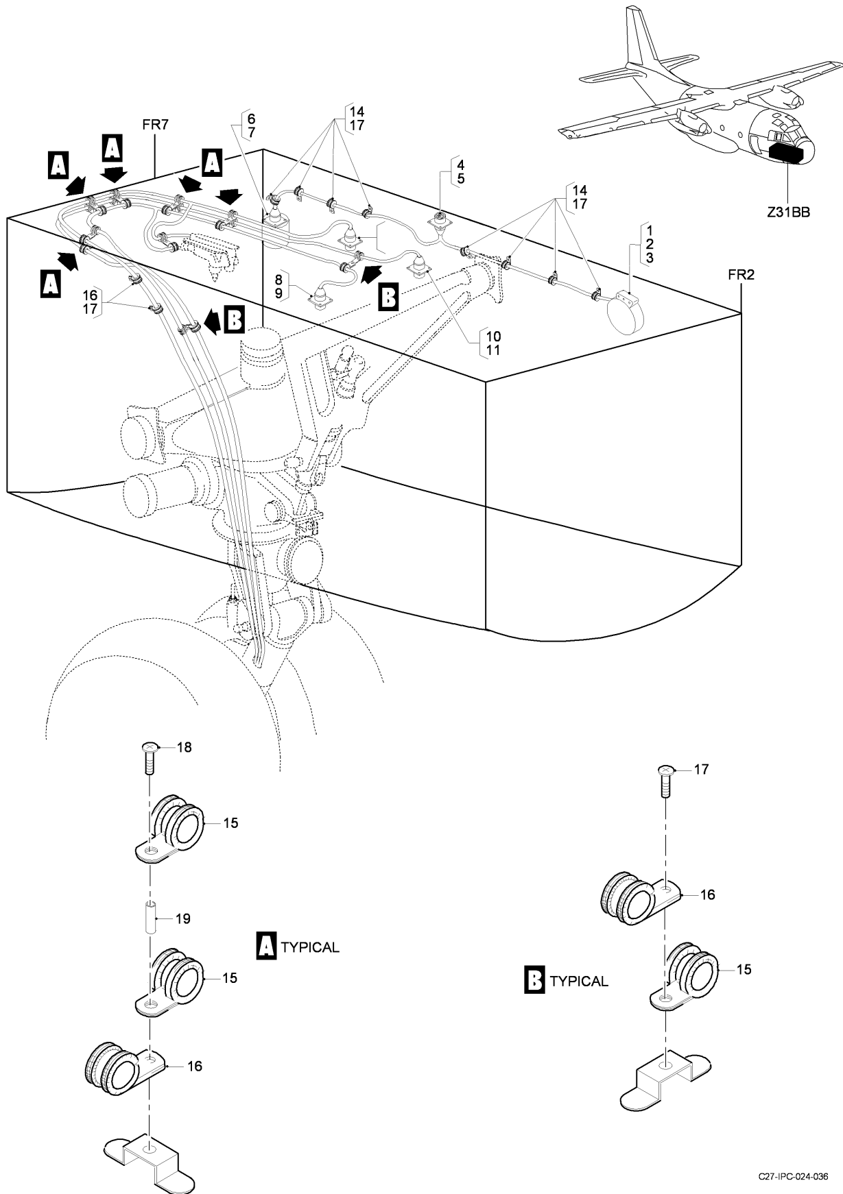
FIG 10 ELECTRICAL AND ELECTRONICS INSTL - NLG BAY, Z31BB (SHEET 1 OF 1)
