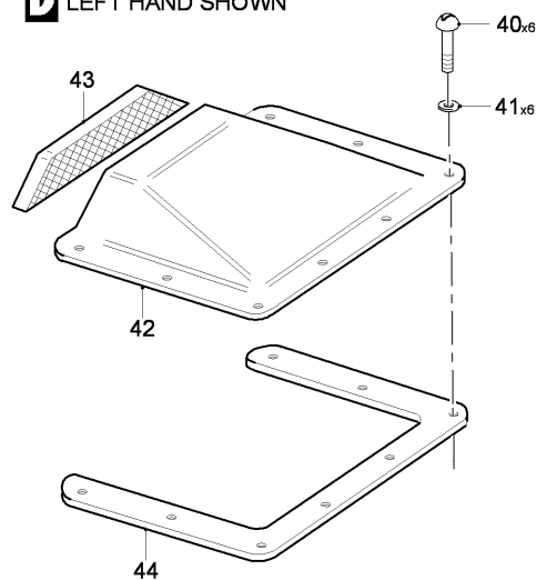
FIG 05 AIR DISTRUBTION INSTL, Z32AA-32AB-32AC-32AD (SHEET 2 OF 4)
