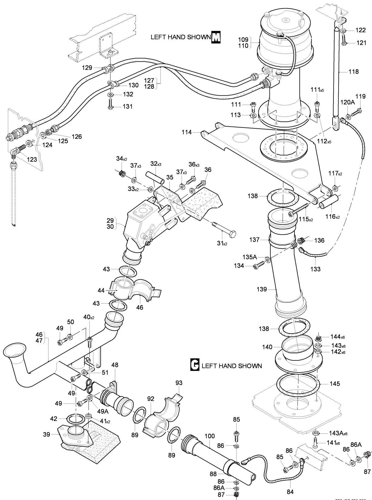
FIG 01 FUEL VENT AND DRAINS INSTL - CENTER WING, Z33AB, LH-RH (SHEET 3 OF 4)
