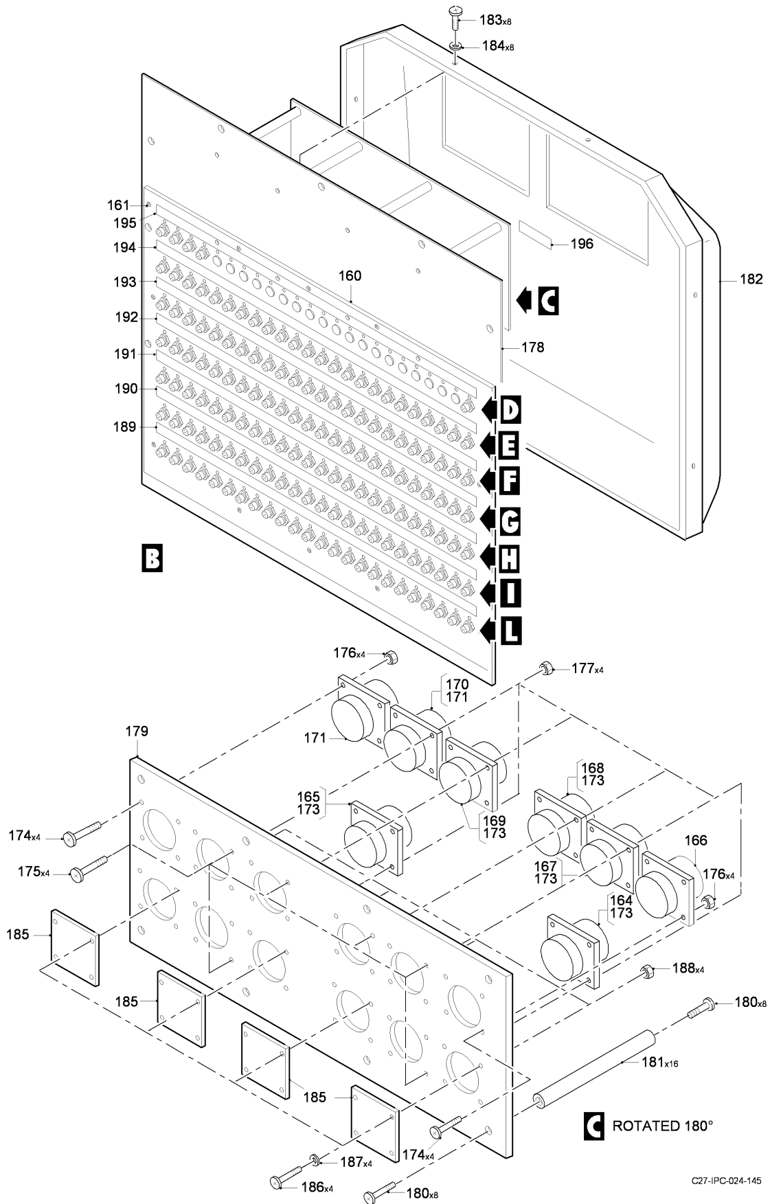
FIG 01 TRU INSTL, Z31AB (SHEET 2 OF 5)
