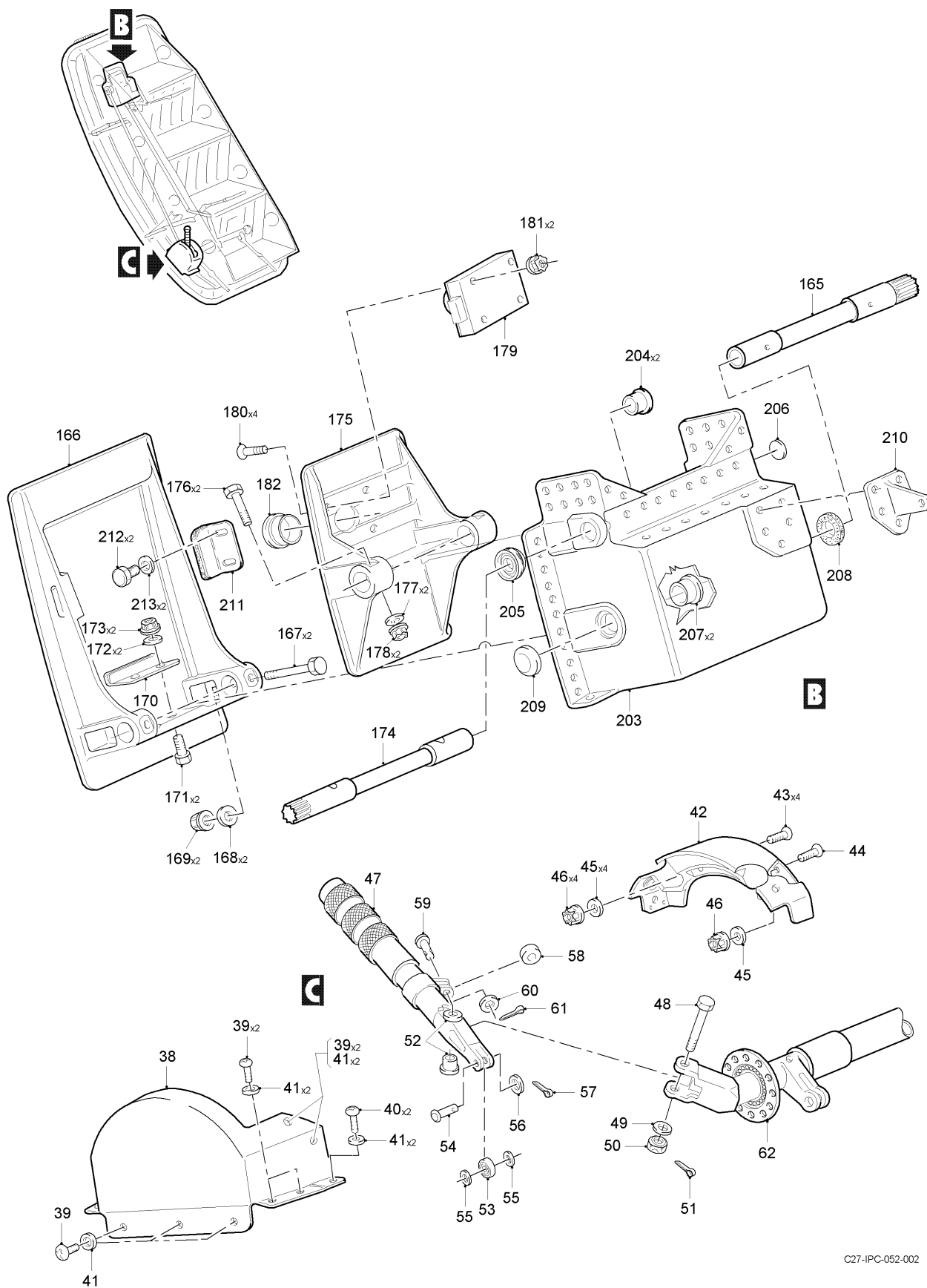
FIG 01 CREW DOOR INSTL, Z31AB (SHEET 2 OF 7)
