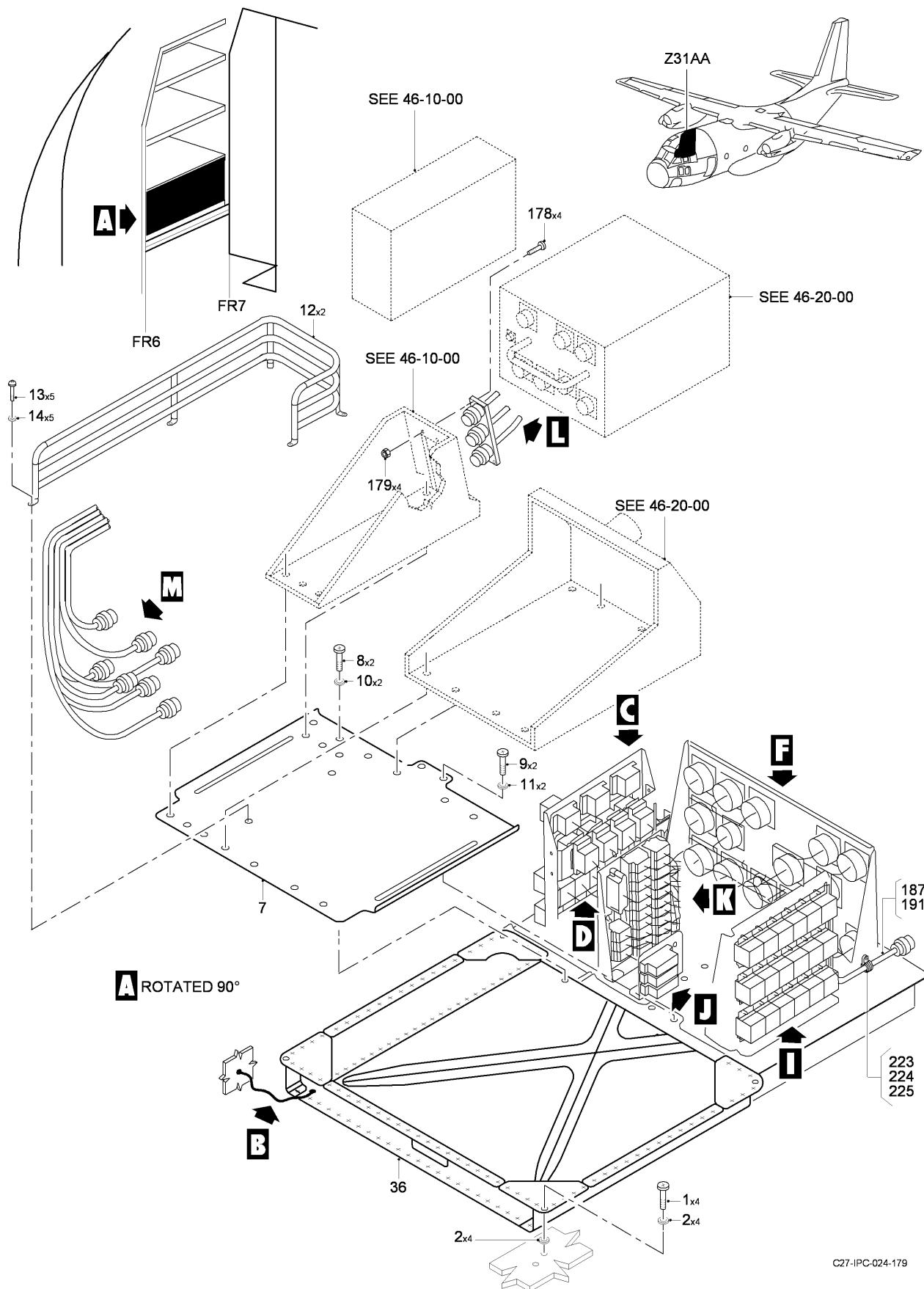
FIG 07 FIRST SHELF INSTL - ELECTRICAL COMPARTMENT, Z31AA (SHEET 1 OF 5)
