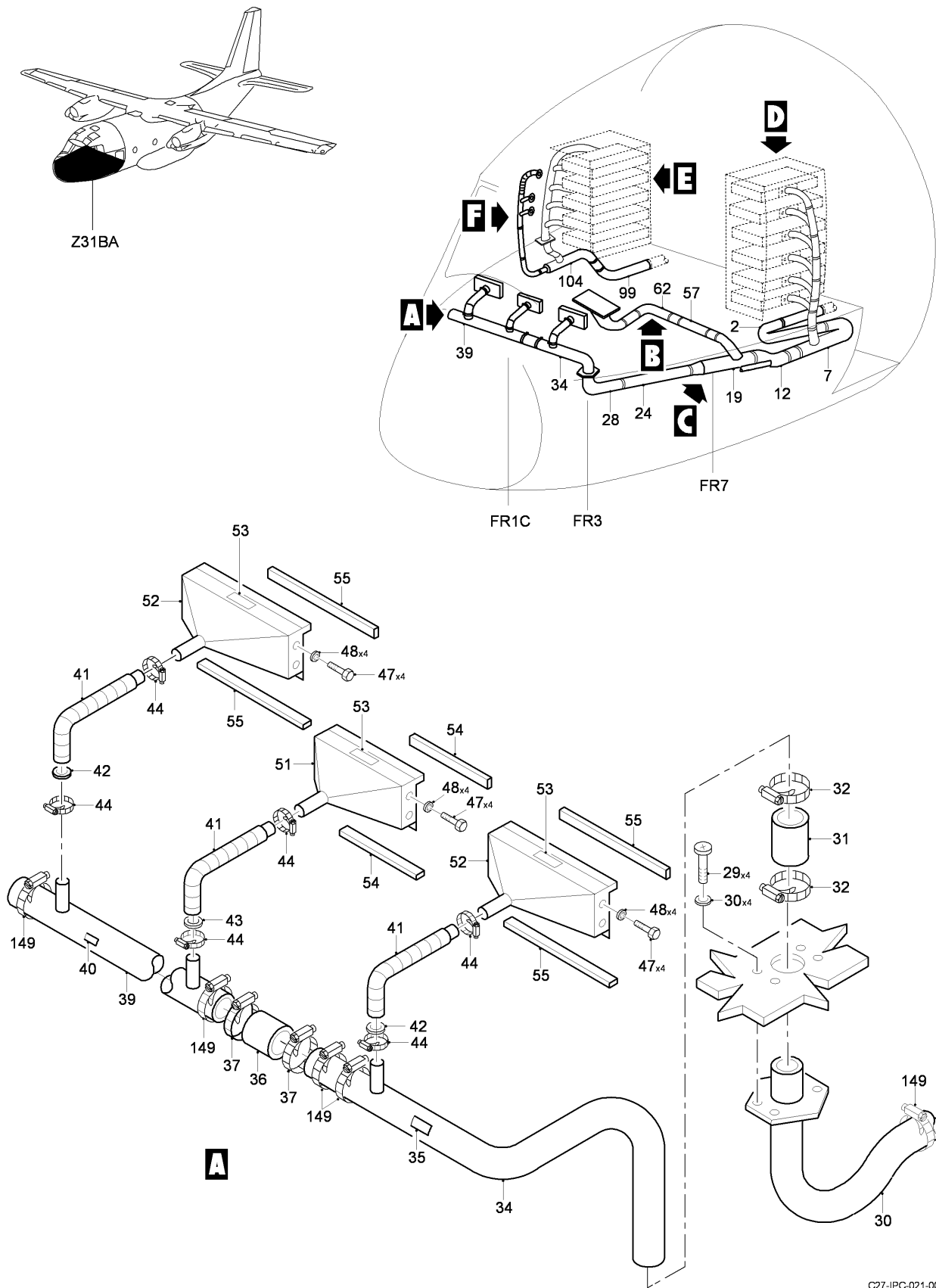
FIG 02 VENTILATION INSTL - FWD FUSELAGE, Z31AA-31AB (SHEET 1 OF 3)
