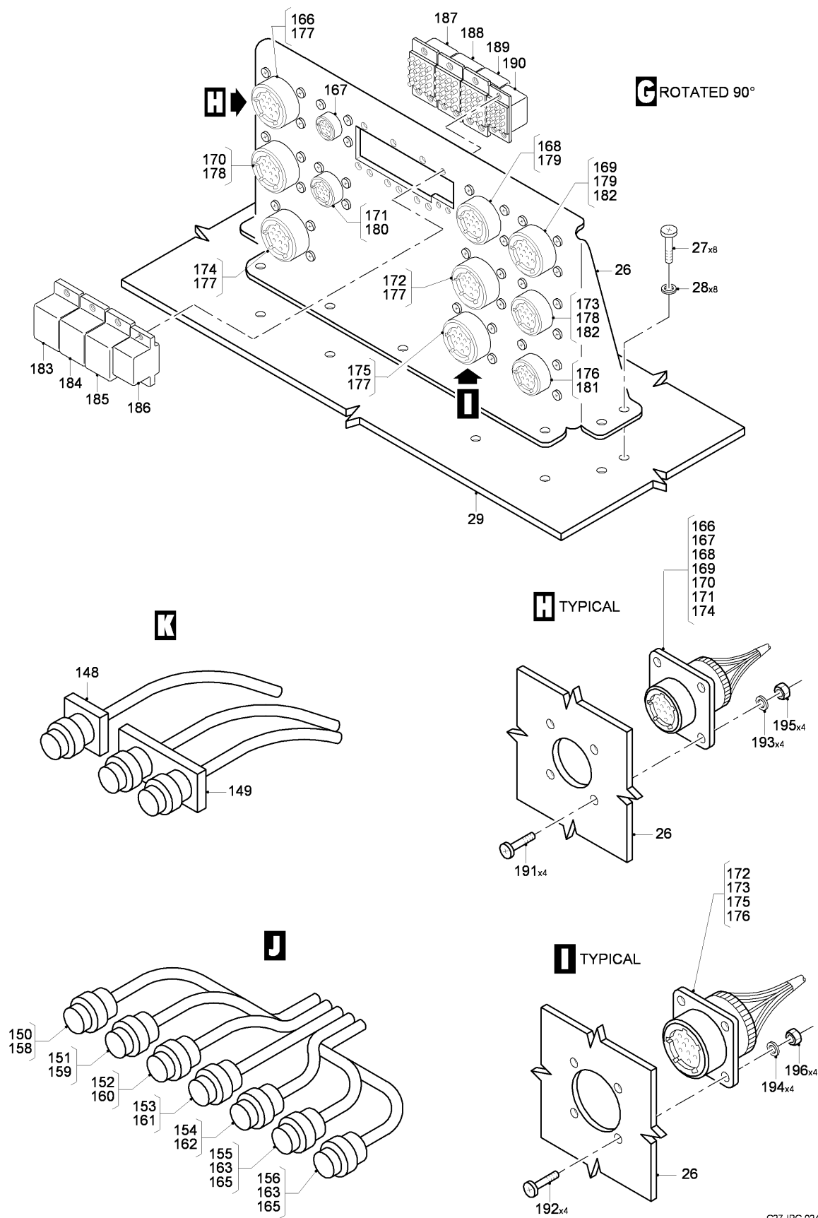
FIG 08 SECOND SHELF INSTL - ELECTRICAL COMPARTMENT, Z31AA (SHEET 4 OF 4)
