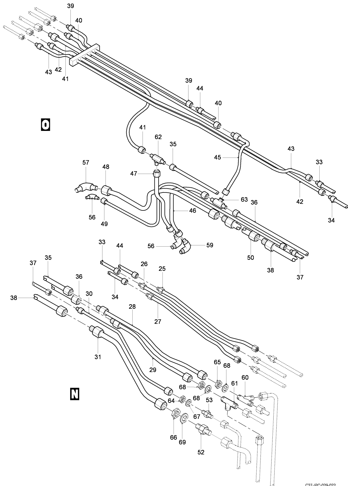
FIG 05 HYDRAULIC PIPING INSTL - CENTER WING, Z33AB, LH-RH (SHEET 5 OF 5)
