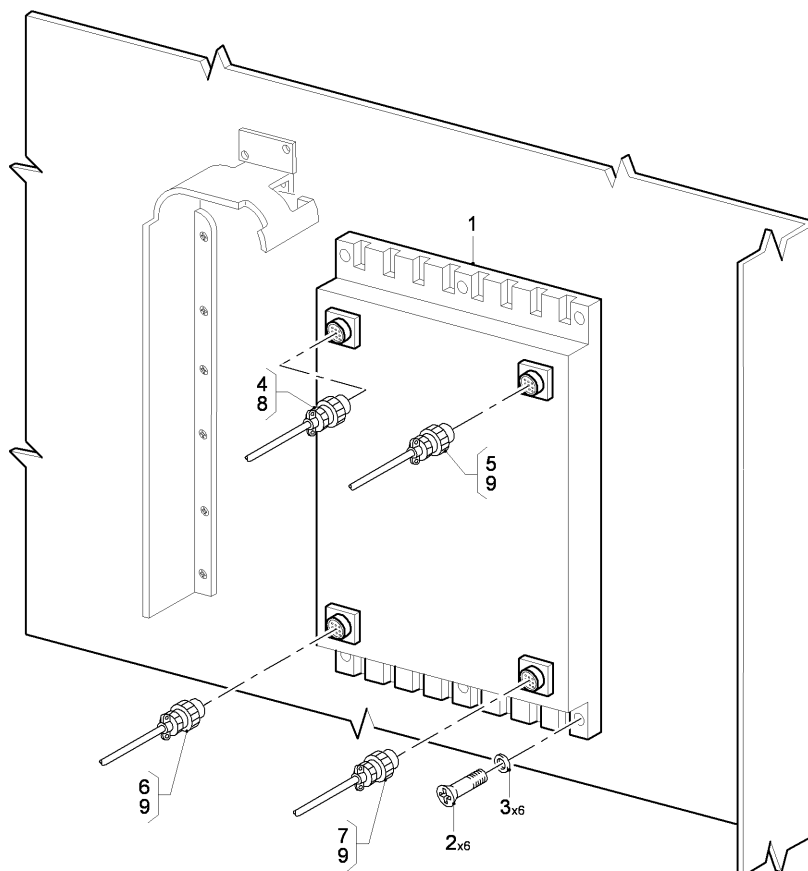
FIG 01 POWER DISTRUBUTION UNIT INSTL, Z31AA (SHEET 1 OF 1)
