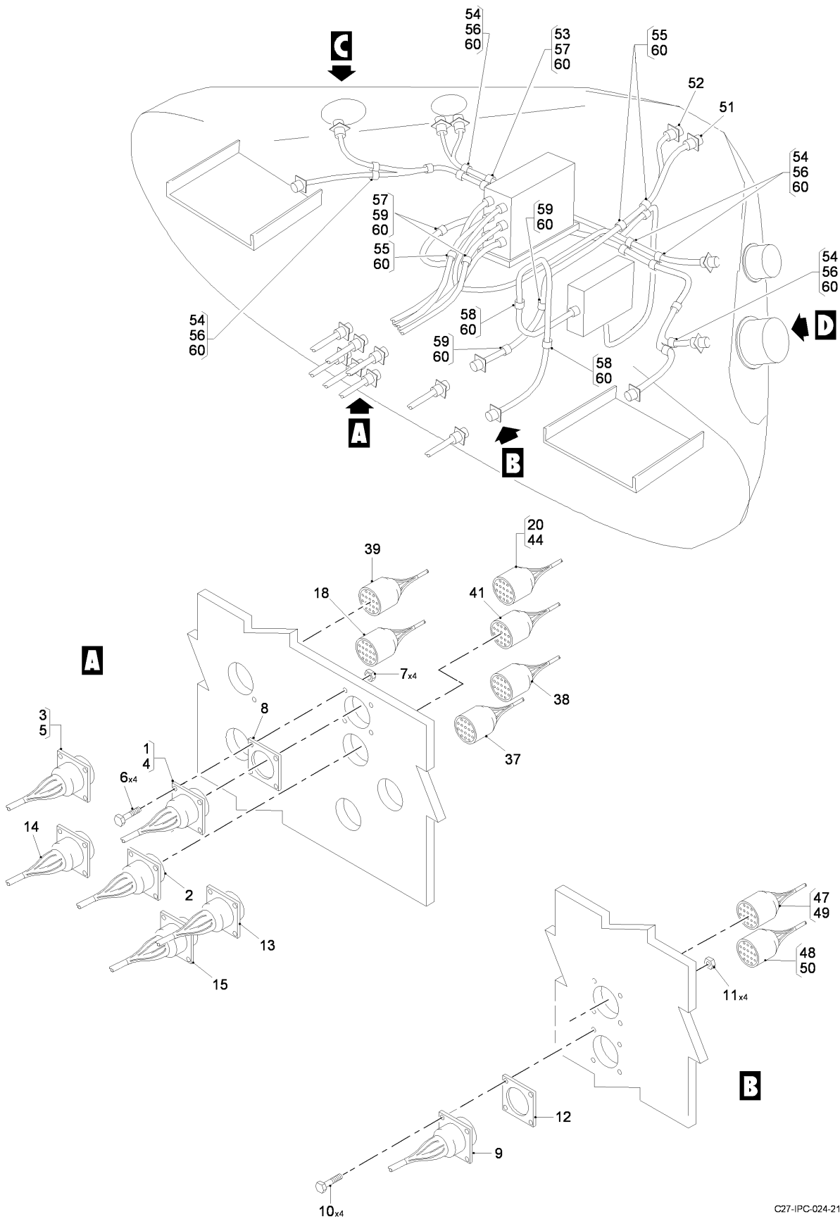
FIG 28 ELECTRICAL AND ELECTRONICS INSTL - TAIL CONE , Z34AB (SHEET 1 OF 2)
