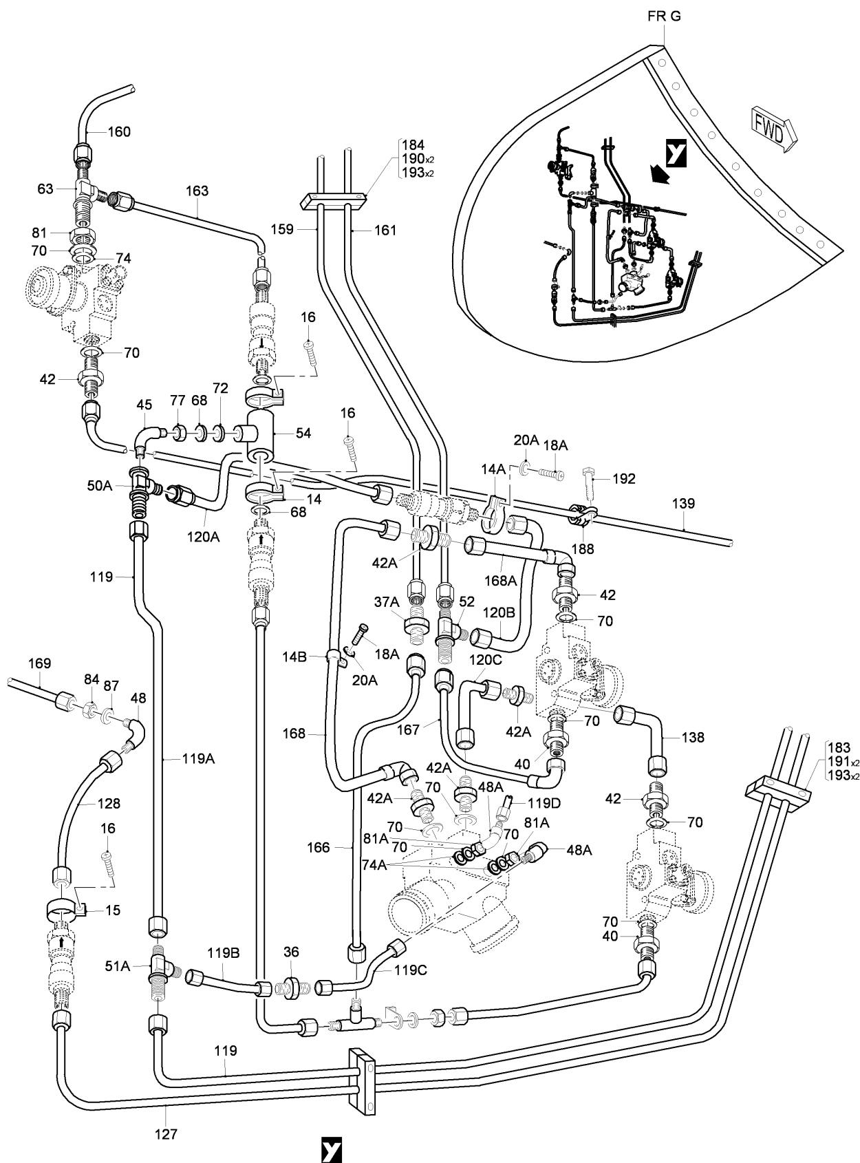
FIG 08 HYDRAULIC INSTL - MLG, Z23AB, RH (SHEET 10 OF 11)
