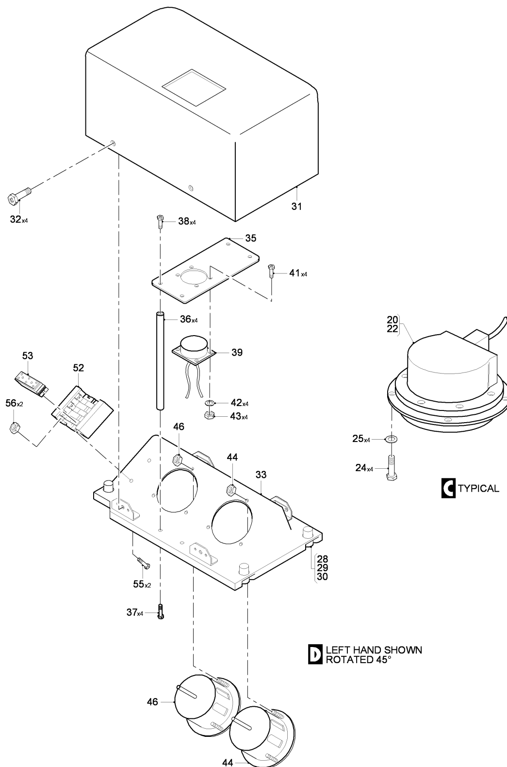
FIG 01 INTERNAL LIGHT INSTL, Z31AA (SHEET 2 OF 3)
