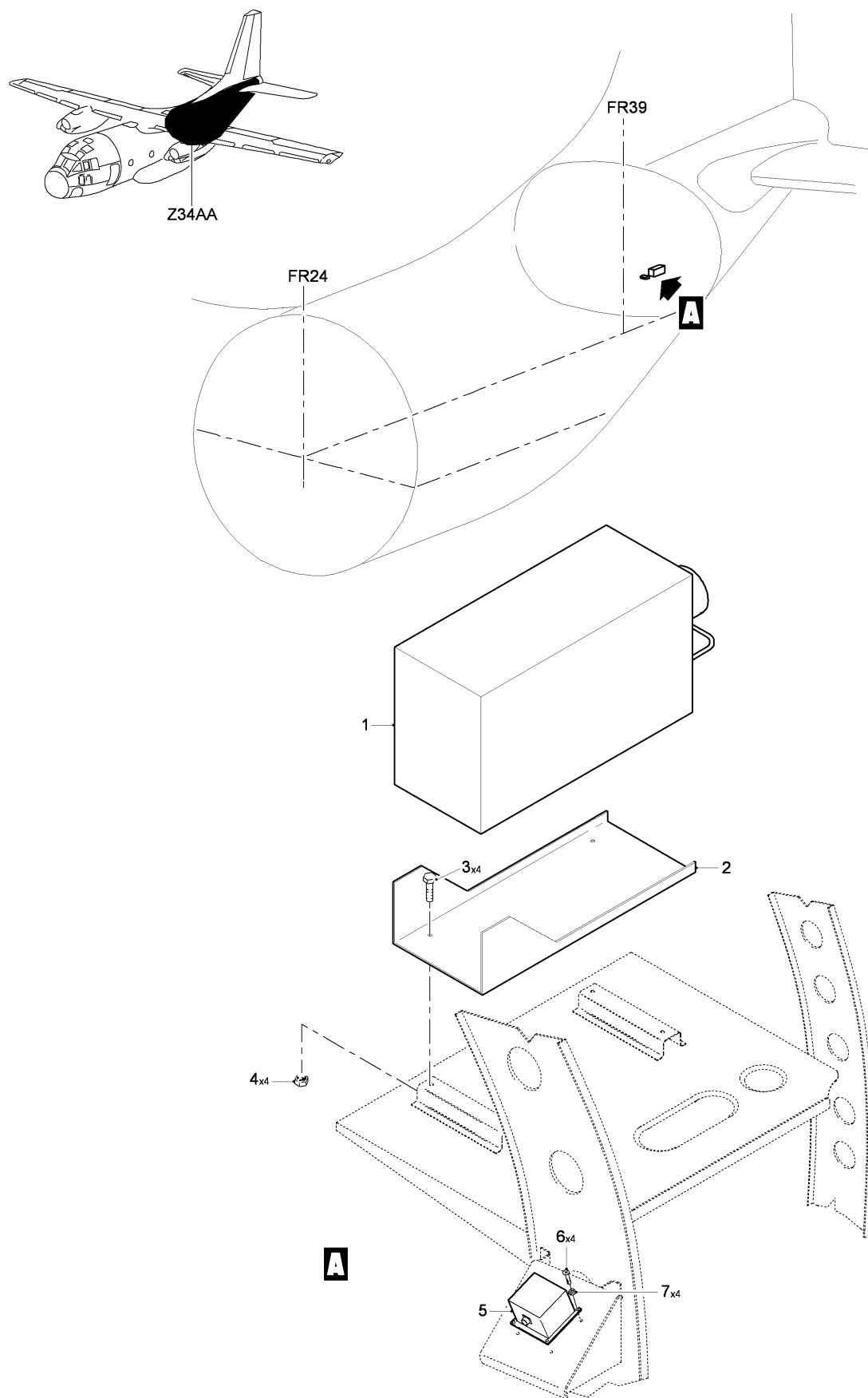
FIG 05 VOICE RECORDER UNIT INSTL, Z34AA (SHEET 1 OF 1)
