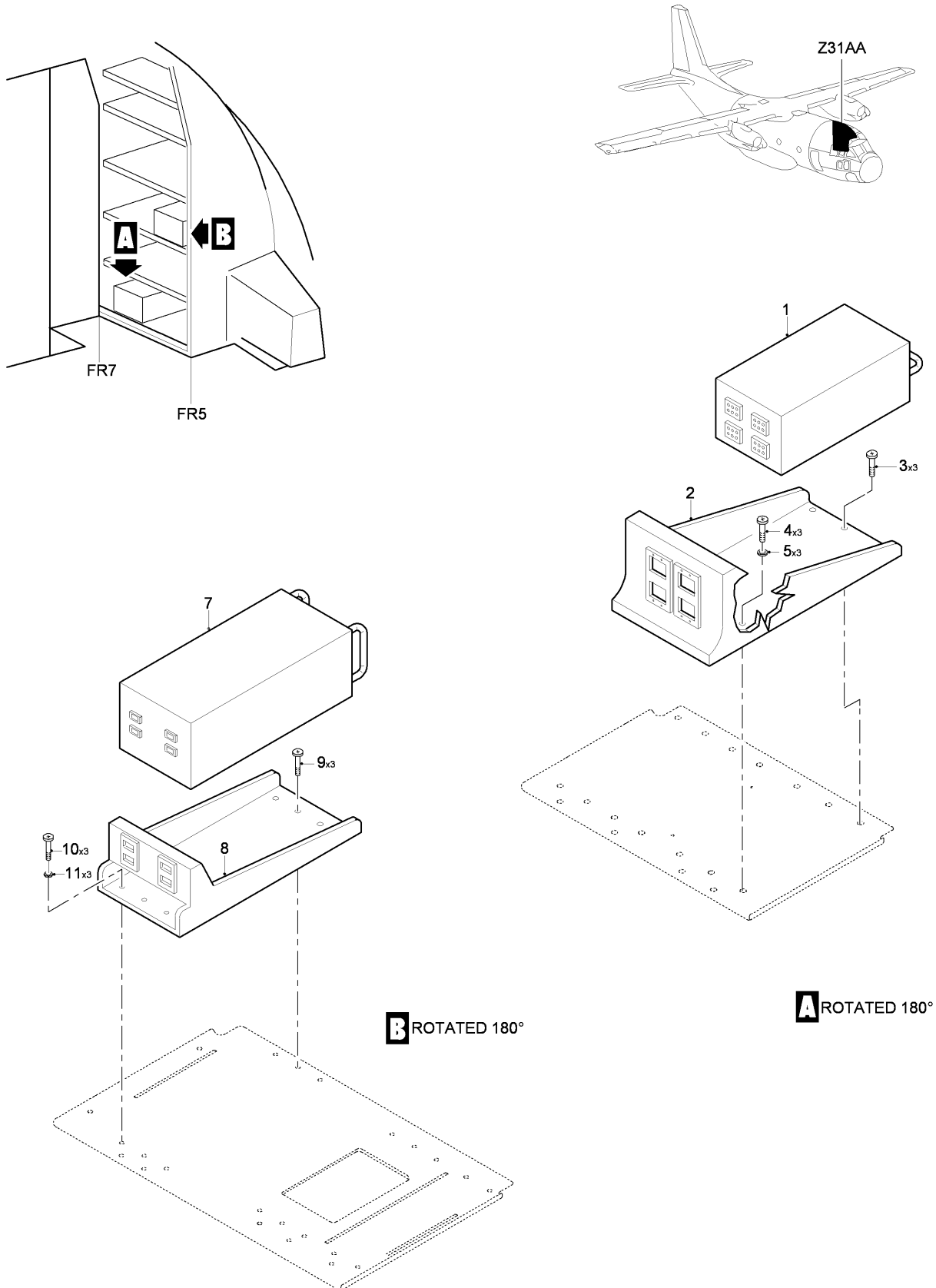
FIG 06 DA/FD PROCESSOR INSTL - ELCTRONIC COMPARTMENT, Z31AA (SHEET 1 OF 1)
