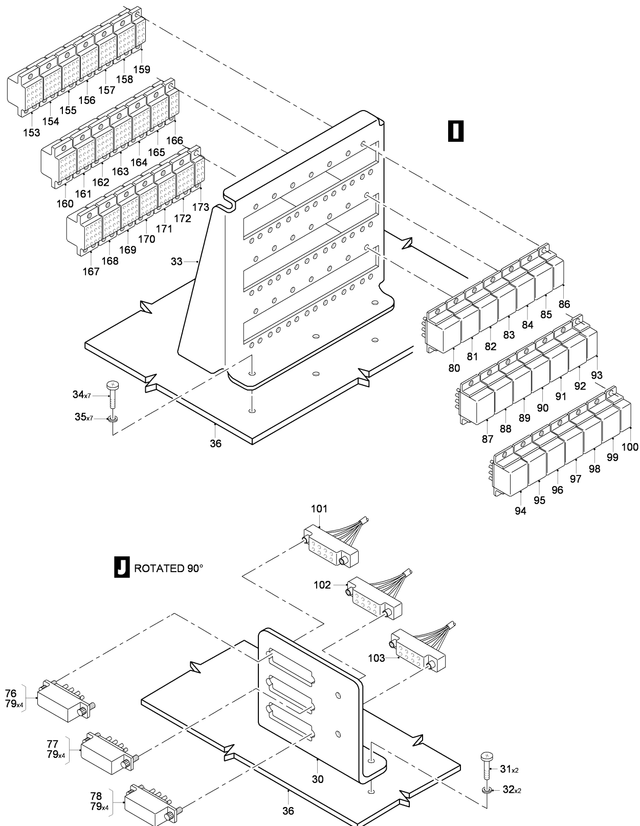
FIG 07 FIRST SHELF INSTL - ELECTRICAL COMPARTMENT, Z31AA (SHEET 4 OF 5)
