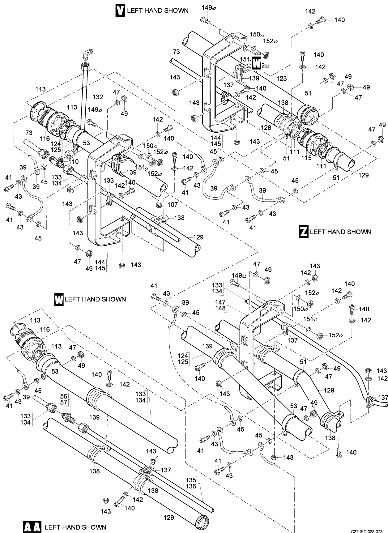
FIG 04 SINGLE POINT REFUELLING AND FUEL SUPPLY INSTL, Z33AB, LH-RH (SHEET 5 OF 6)
