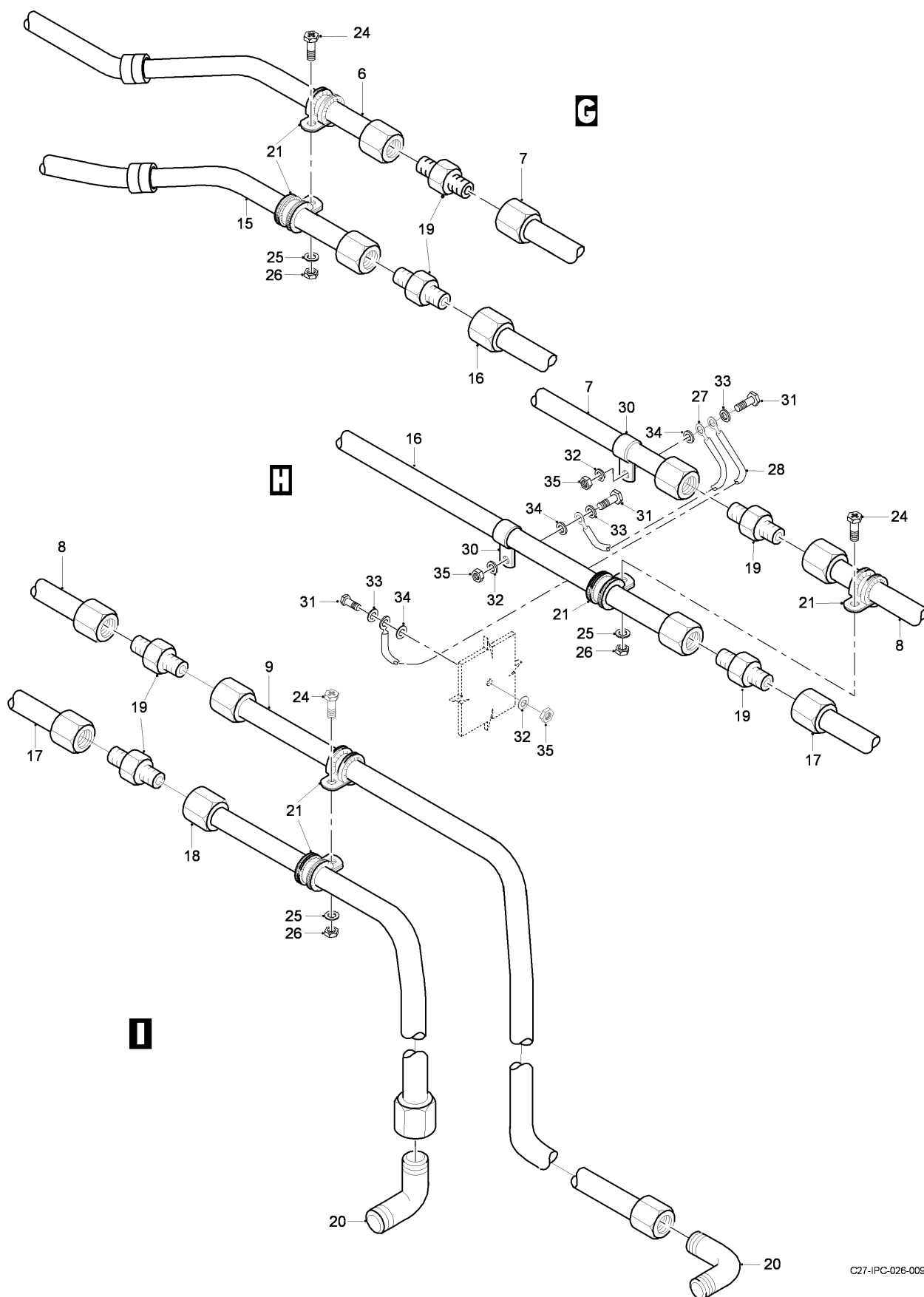
FIG 01 ENGINE FIRE EXTINGUISHING INSTL - CENTER WING, Z33AB (SHEET 4 OF 4)
