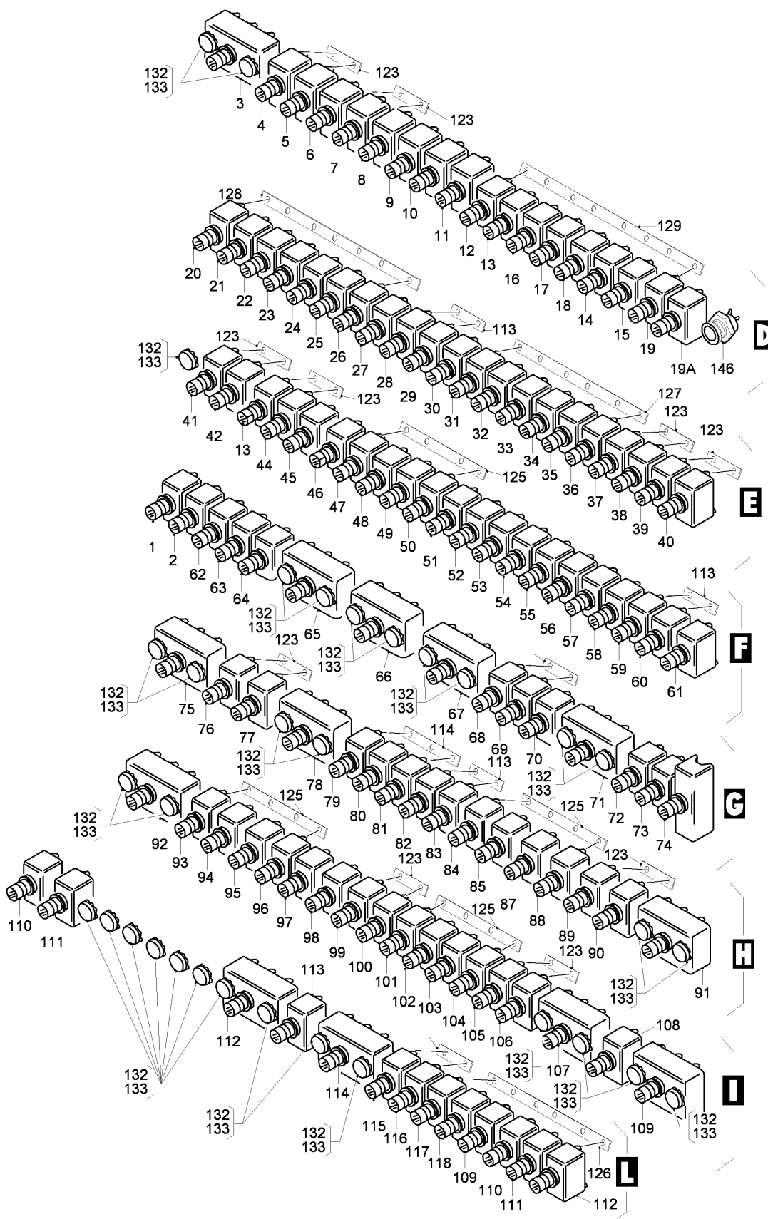
FIG 03 CIRCUIT BREAKER PANEL NO. 2 INSTL, Z31AA (SHEET 3 OF 3)
