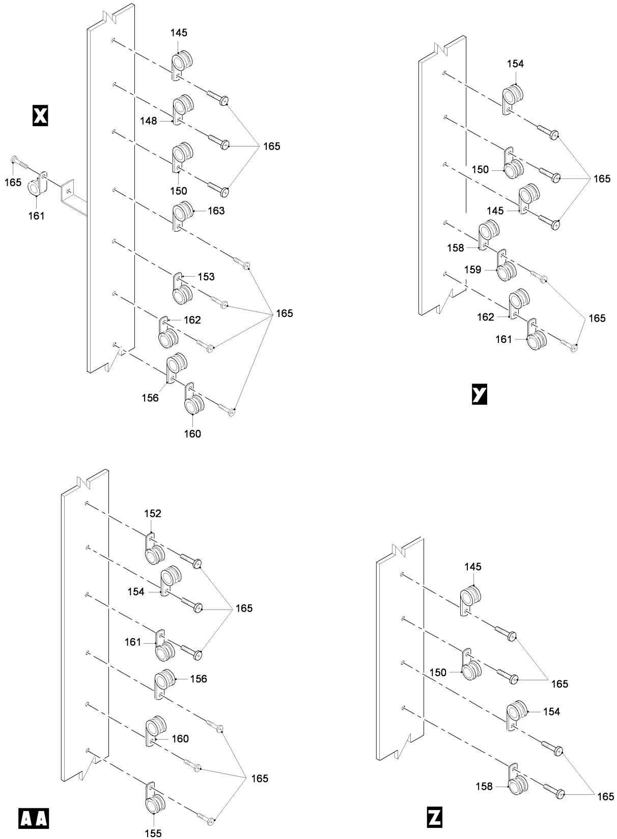
FIG 14 ELECTRICAL AND ELECTRONICS INSTL, Z31BC-31BD-32BA (SHEET 9 OF 11)
