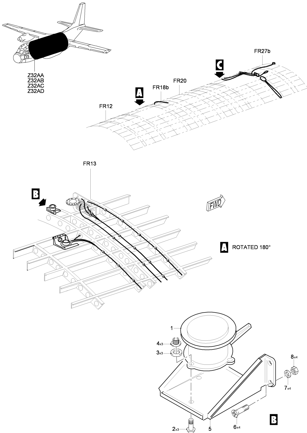
FIG 03 BAIL OUT SIGNAL INSTL, Z32AA-32AB-32AC-32AD (SHEET 1 OF 2)
