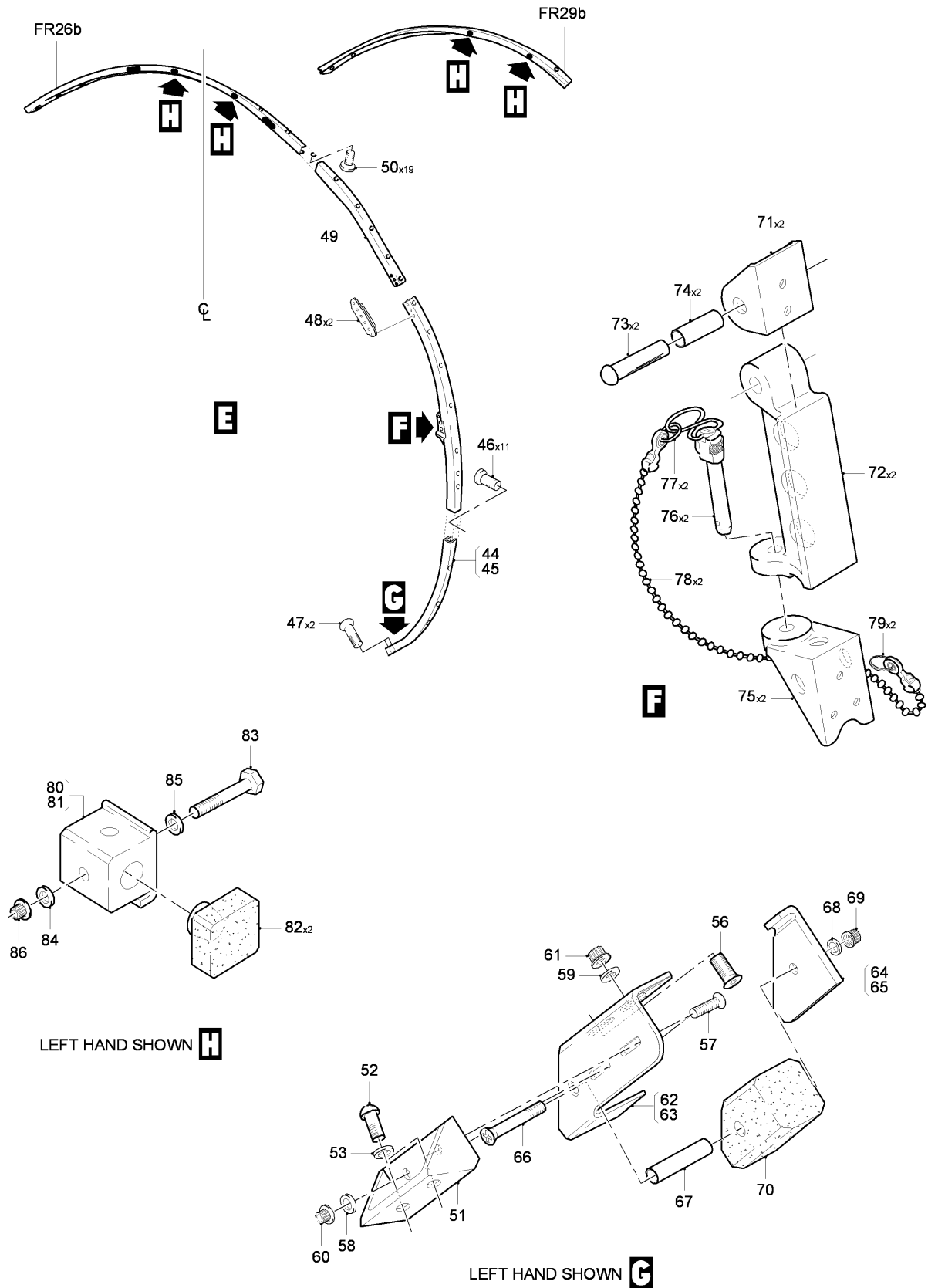
FIG 02 PARATROOPS DOOR INSTL, Z32AD, LH-RH (SHEET 2 OF 5)
