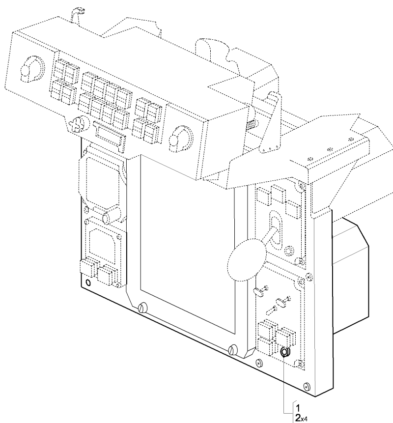
FIG 01 TAXI LANDING LIGHT AND ANTISKID CONTROL PANEL INSTL, Z31AA (SHEET 1 OF 1)
