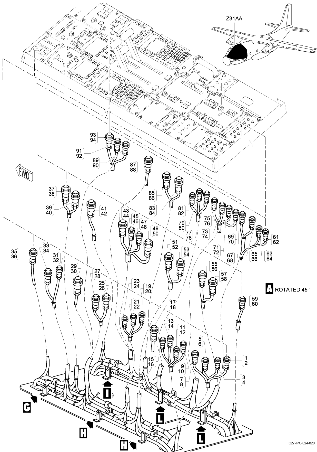
FIG 07 ELECTRICAL AND ELECTRONICS INSTL - CABIN LOWER SIDE, Z31AA (SHEET 1 OF 4)
