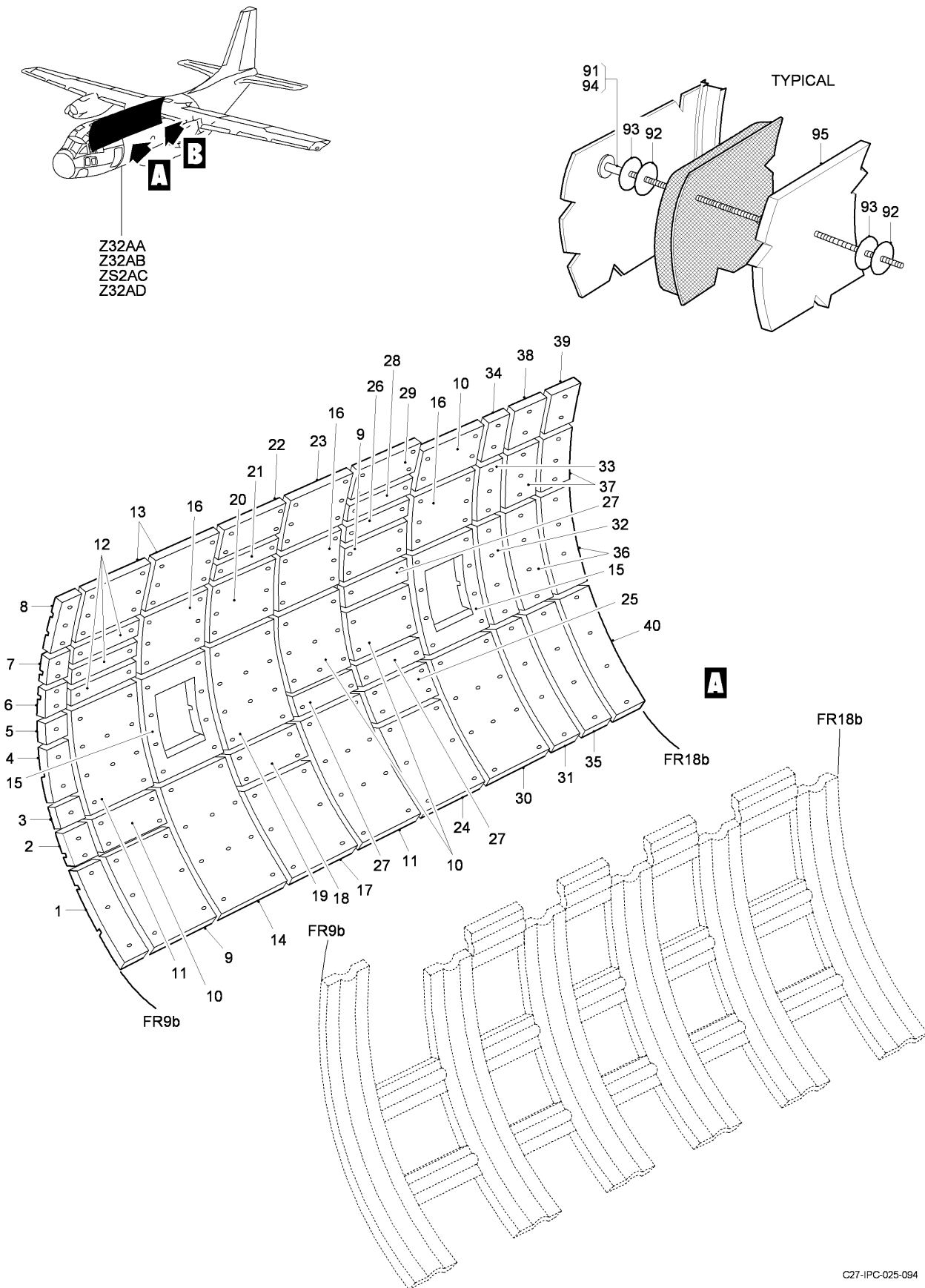
FIG 17 PRIMARY THERMAL INSULATION INSTL, Z32AA-32AB-32AC-32AD (SHEET 1 OF 2)
