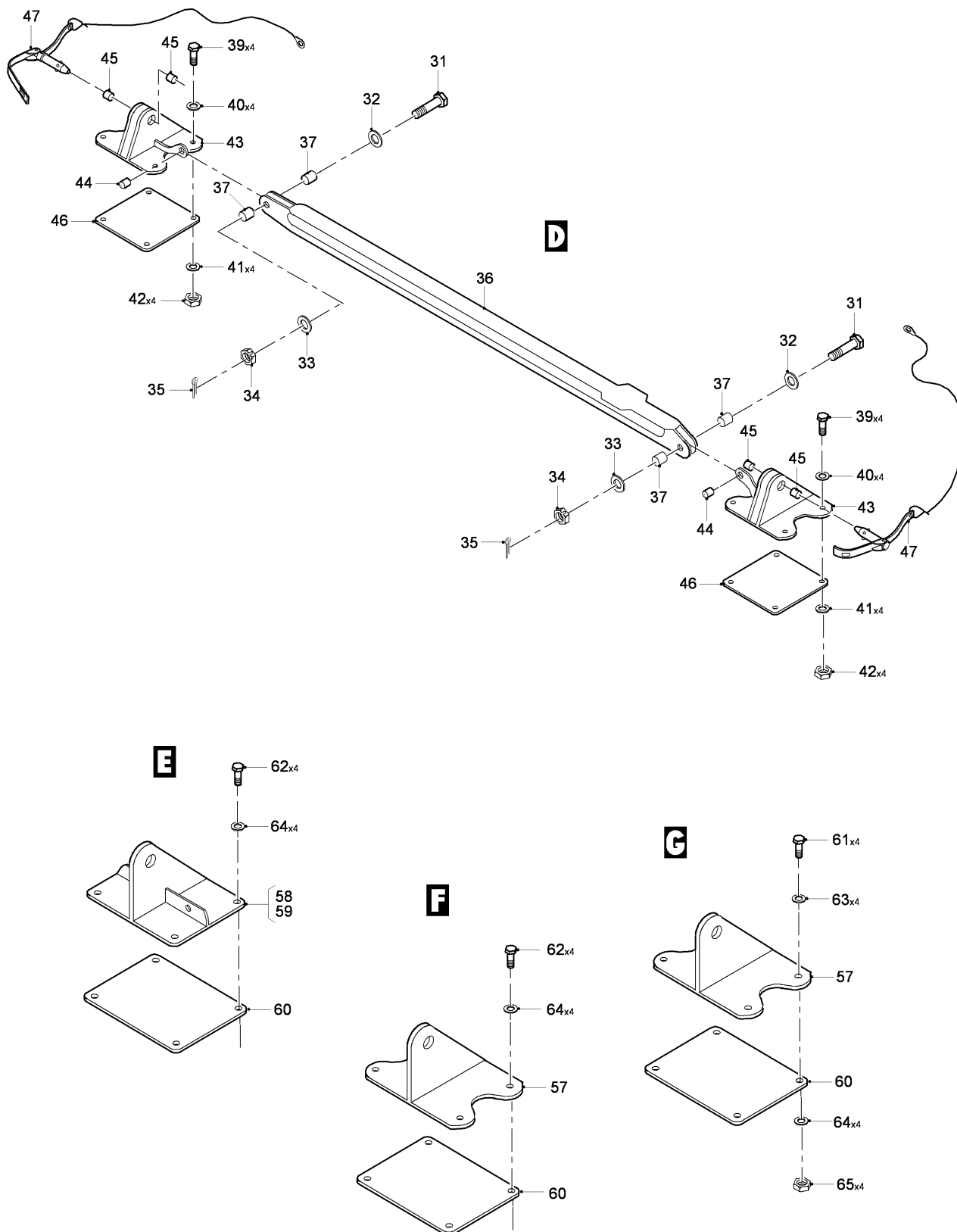
FIG 01 NACELLE ENGINE LWR PANEL INSTL, Z12AC-12AD-22AC-22AD, LH-RH (SHEET 2 OF 3)
