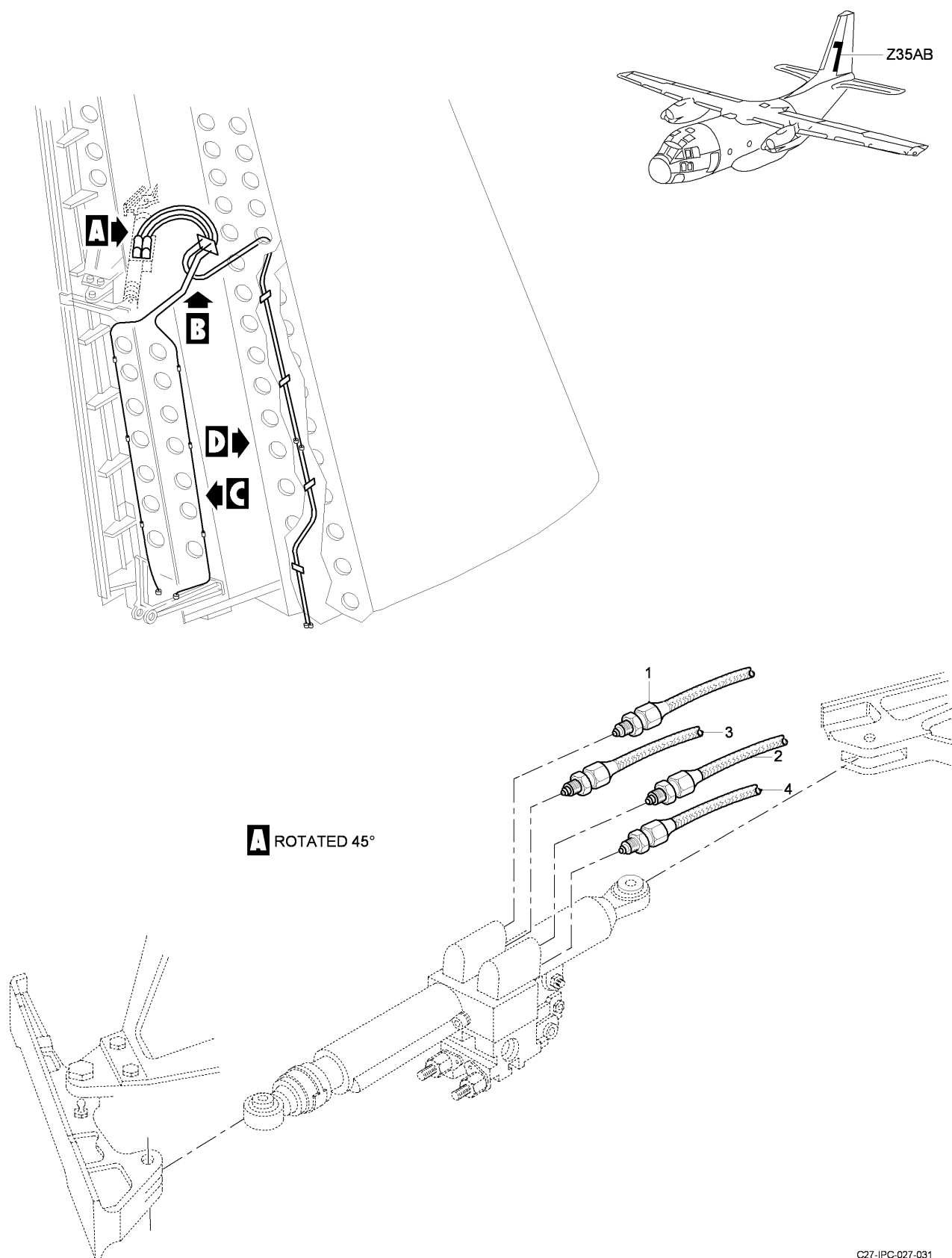
FIG 07 HYDRAULIC INSTL - VERTICAL STABILIZER, Z35AB (SHEET 1 OF 2)
