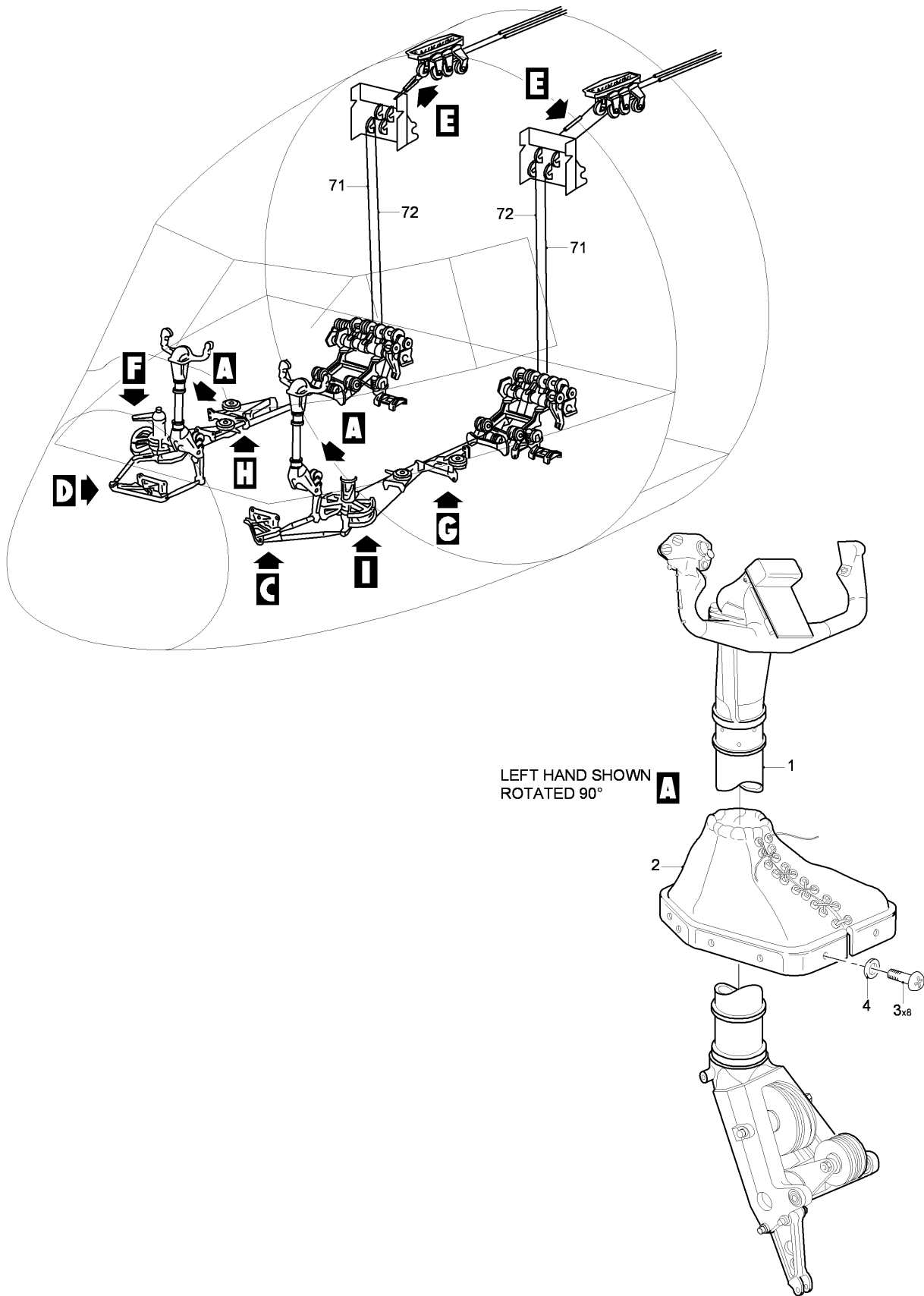
FIG 02 ELEVATOR CONTROLS INSTL, Z31AA-31BB-31AB (SHEET 1 OF 5)
