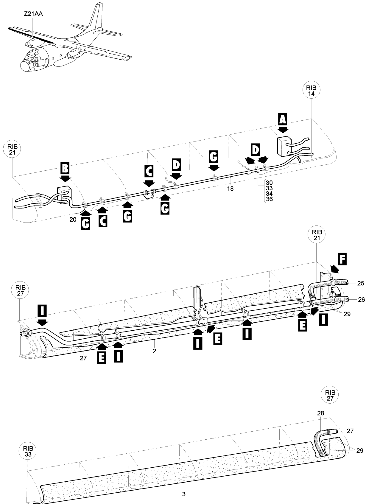
FIG 08 ANTI-ICING INSTL - OUTER WING, Z21AA, RH (SHEET 1 OF 3)
