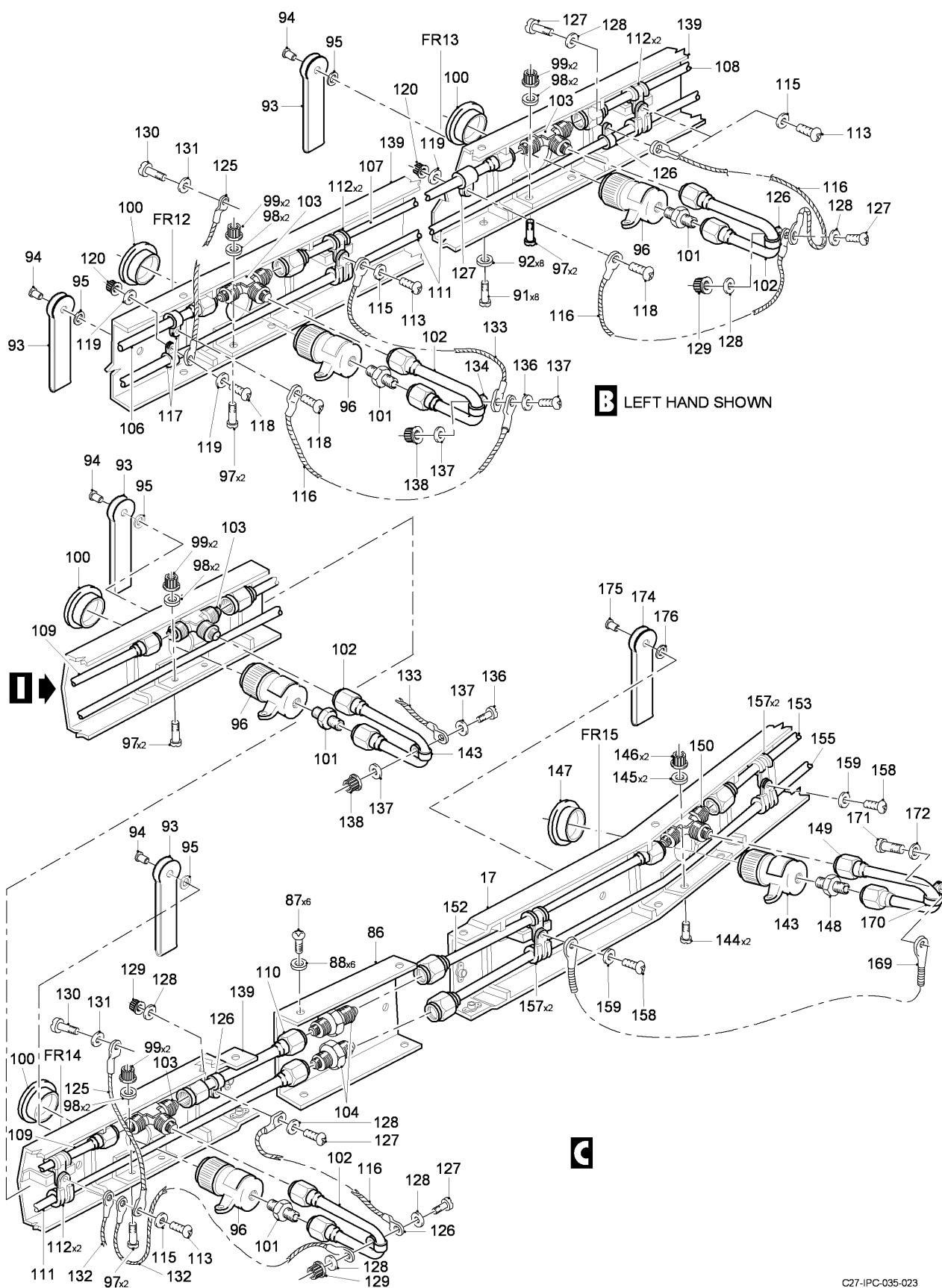
FIG 03 OXYGEN INSTL - CENTER FUSELAGE, Z32AA-32AB-32AC-32AD (SHEET 2 OF 5)
