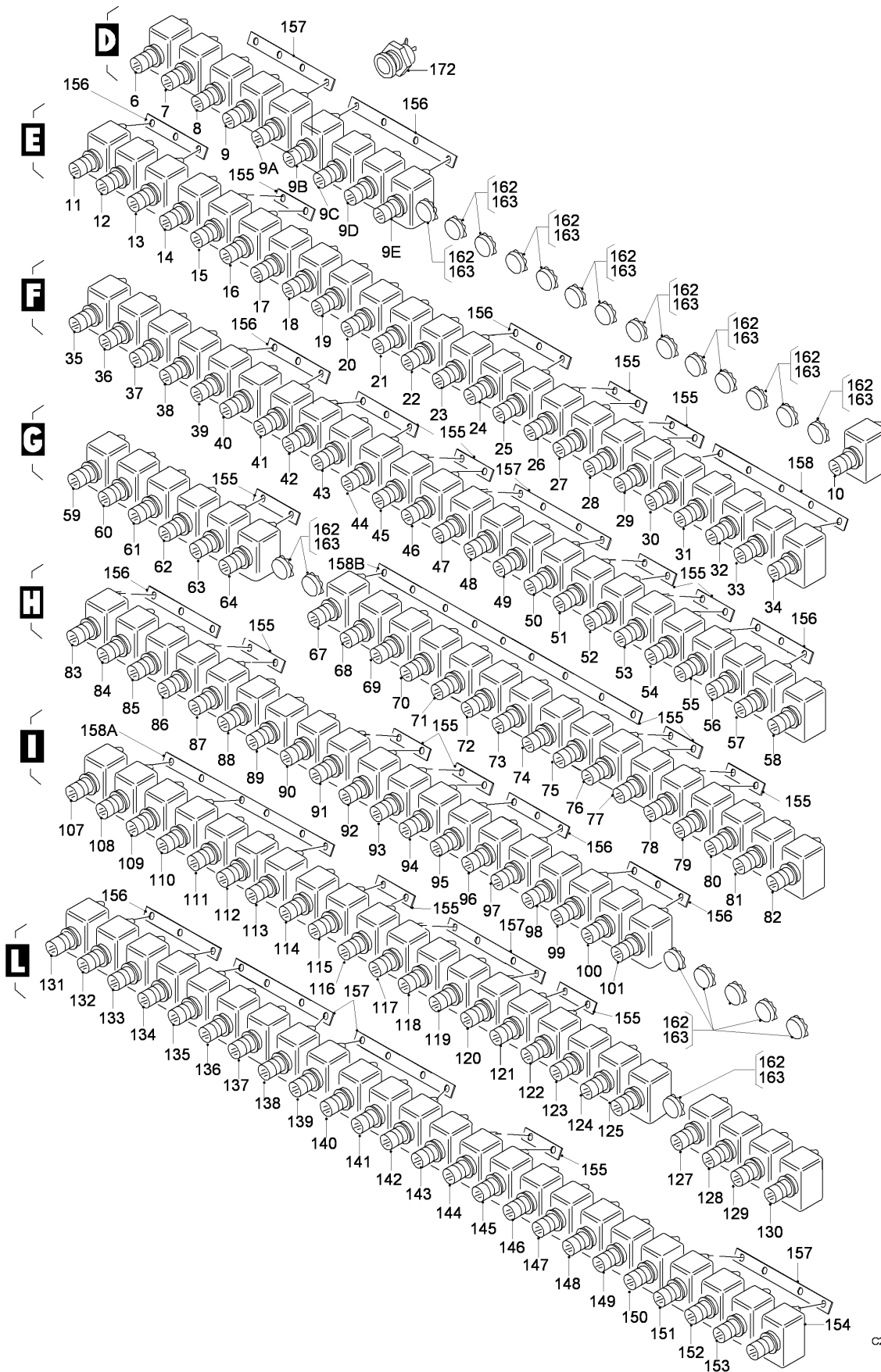
FIG 01 TRU INSTL, Z31AB (SHEET 3 OF 5)
