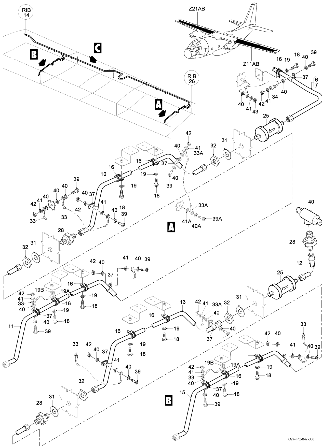
FIG 04 FUEL TANK EXPLOSION PROTECTION SYS INSTL, Z11AB-21AB, LH-RH (SHEET 1 OF 2)
