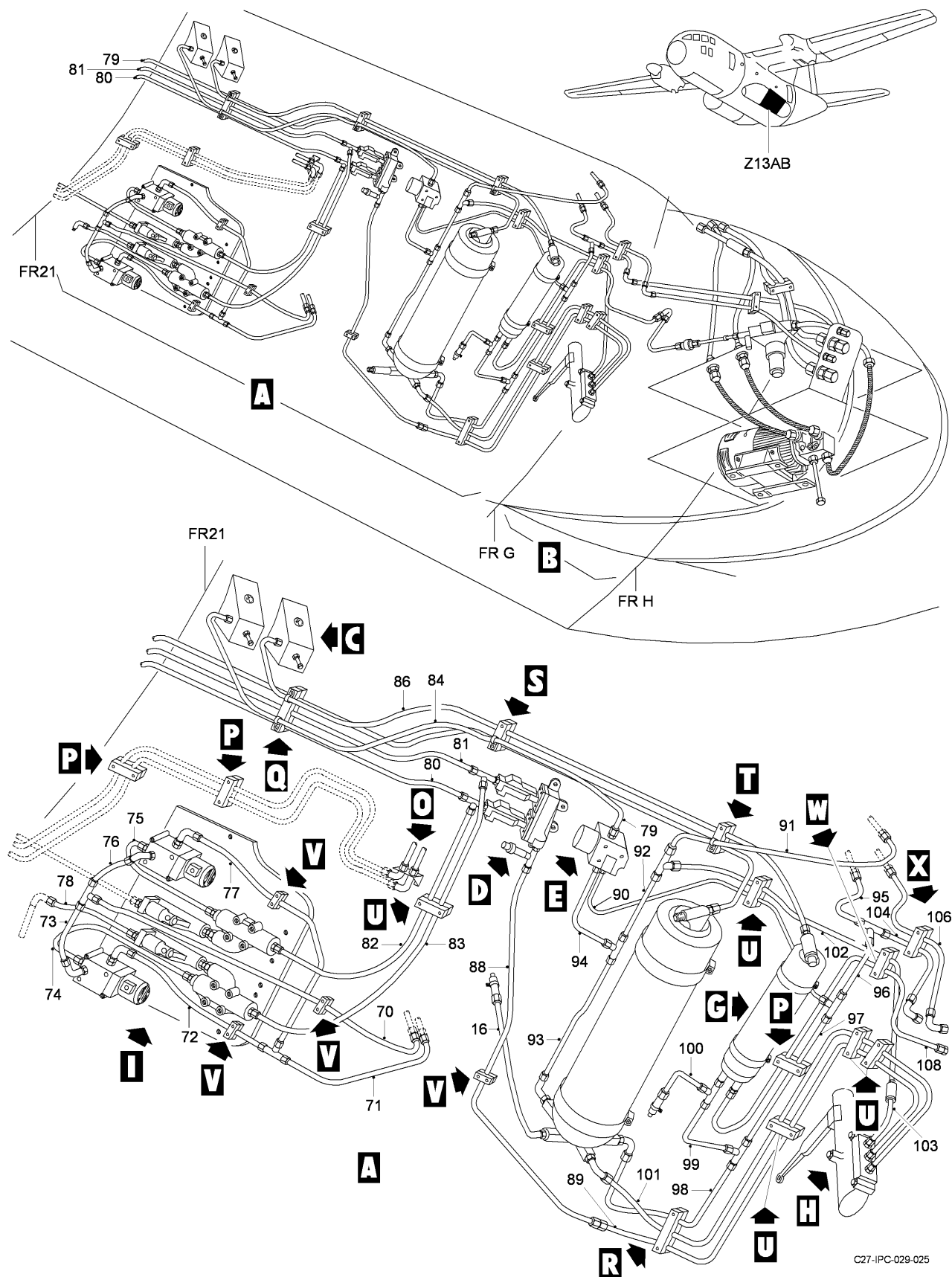
FIG 07 HYDRAULIC INSTL - MLG, Z13AB, LH (SHEET 1 OF 8)
