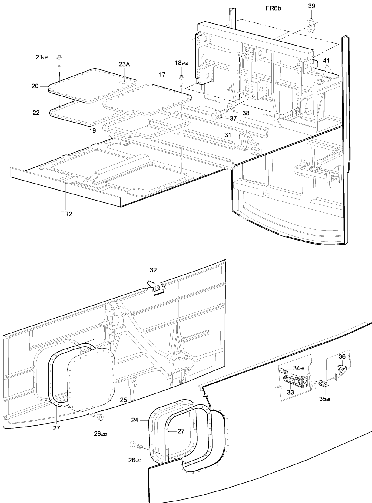
FIG 09 STRUCTURE INSTL, Z31AA (SHEET 2 OF 3)
