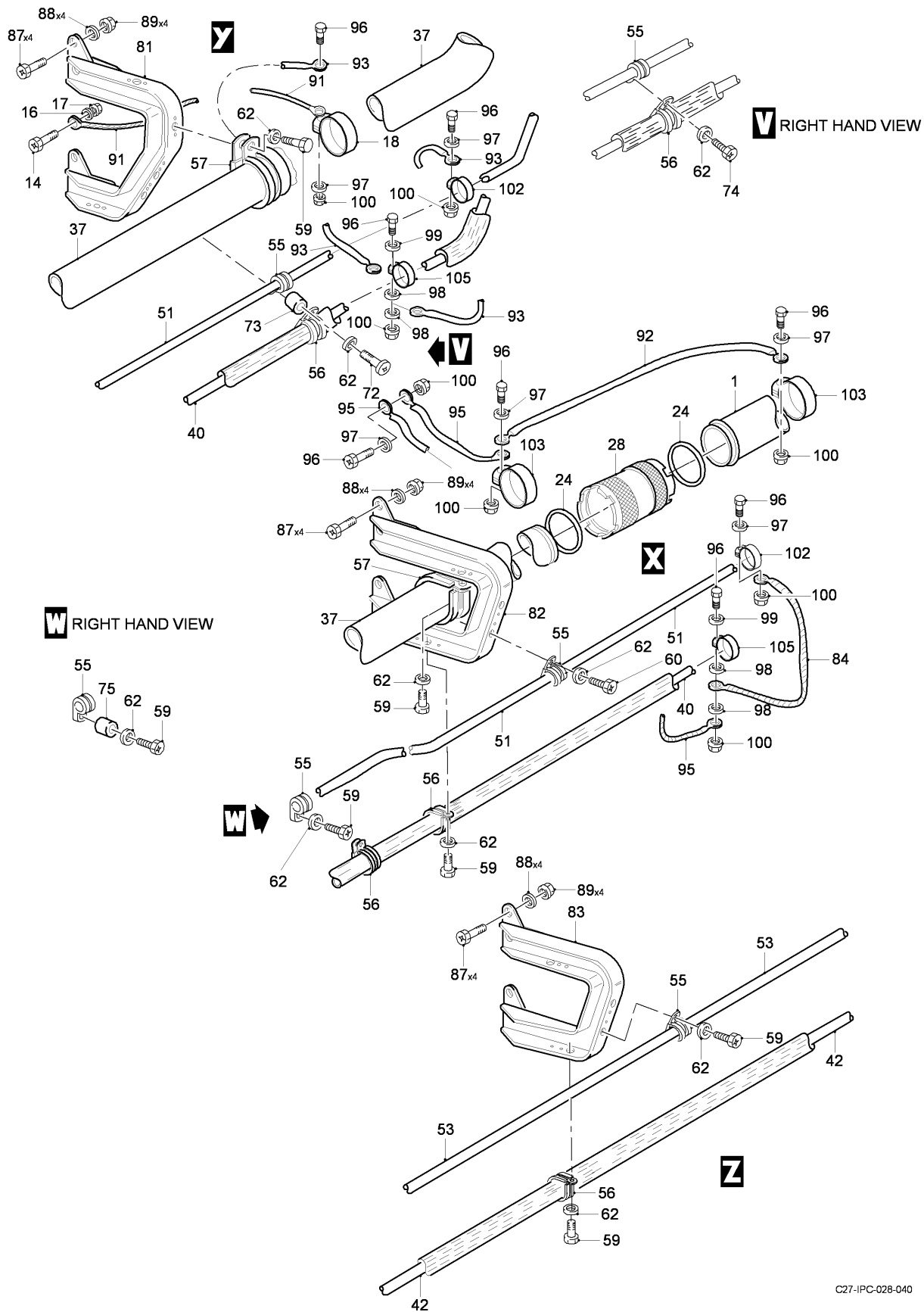
FIG 08 SINGLE POINT REFUEL AND FUEL SUPPLY INSTL, Z11AA-21AA, LH-RH (SHEET 6 OF 6)
