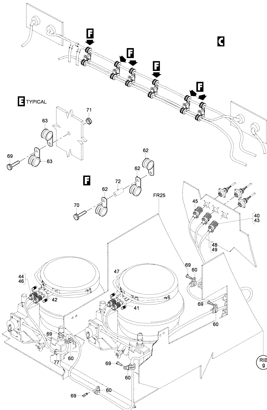
FIG 27 ELECTRICAL AND ELECTRONICS INSTL - MLG, Z23AA-23AB-23AC, RH (SHEET 2 OF 5)
