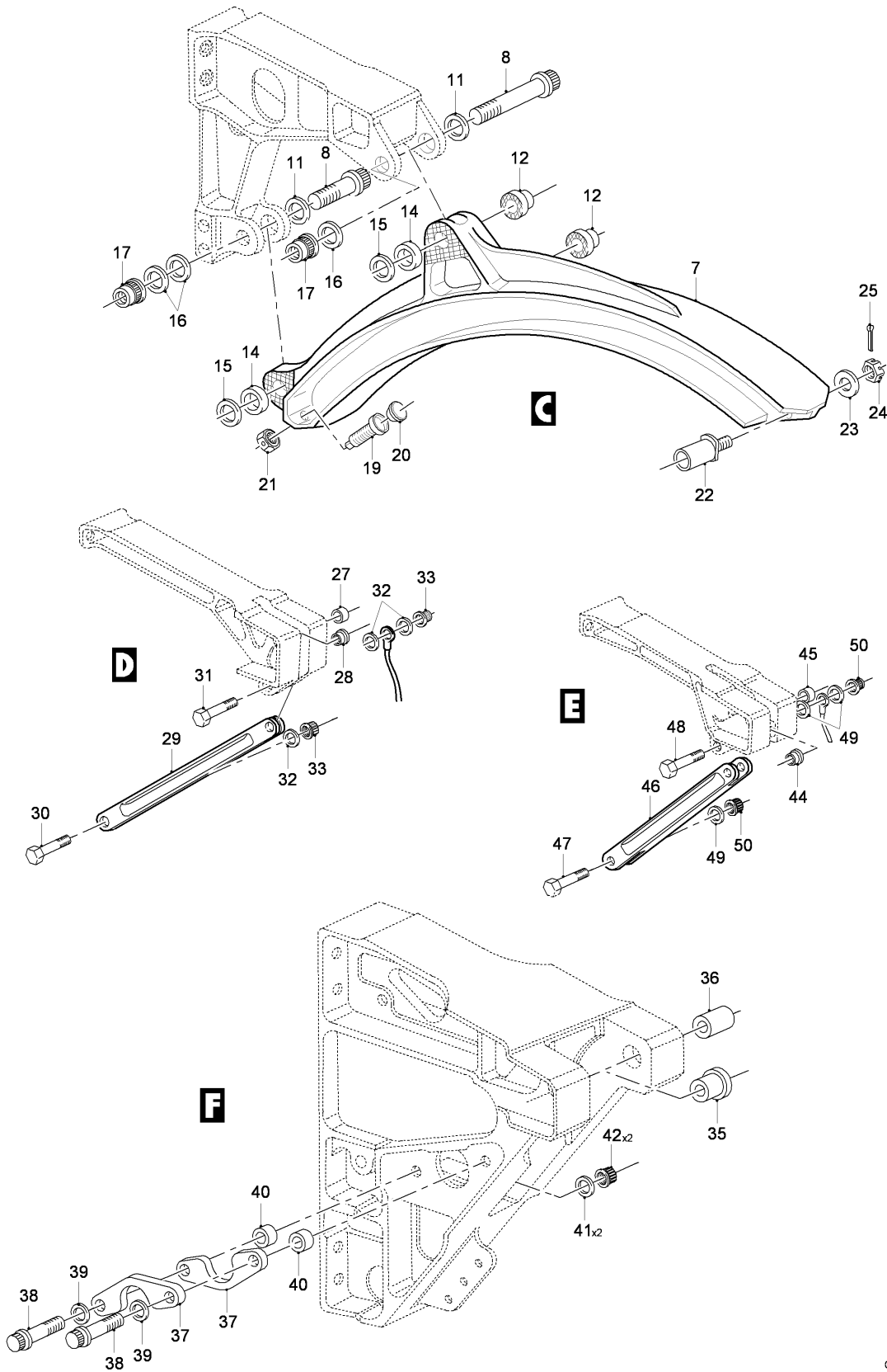
FIG 04 TRAILING EDGE INSTL, Z11AC-11AD-21AC-21AD, LH-RH (SHEET 2 OF 5)
