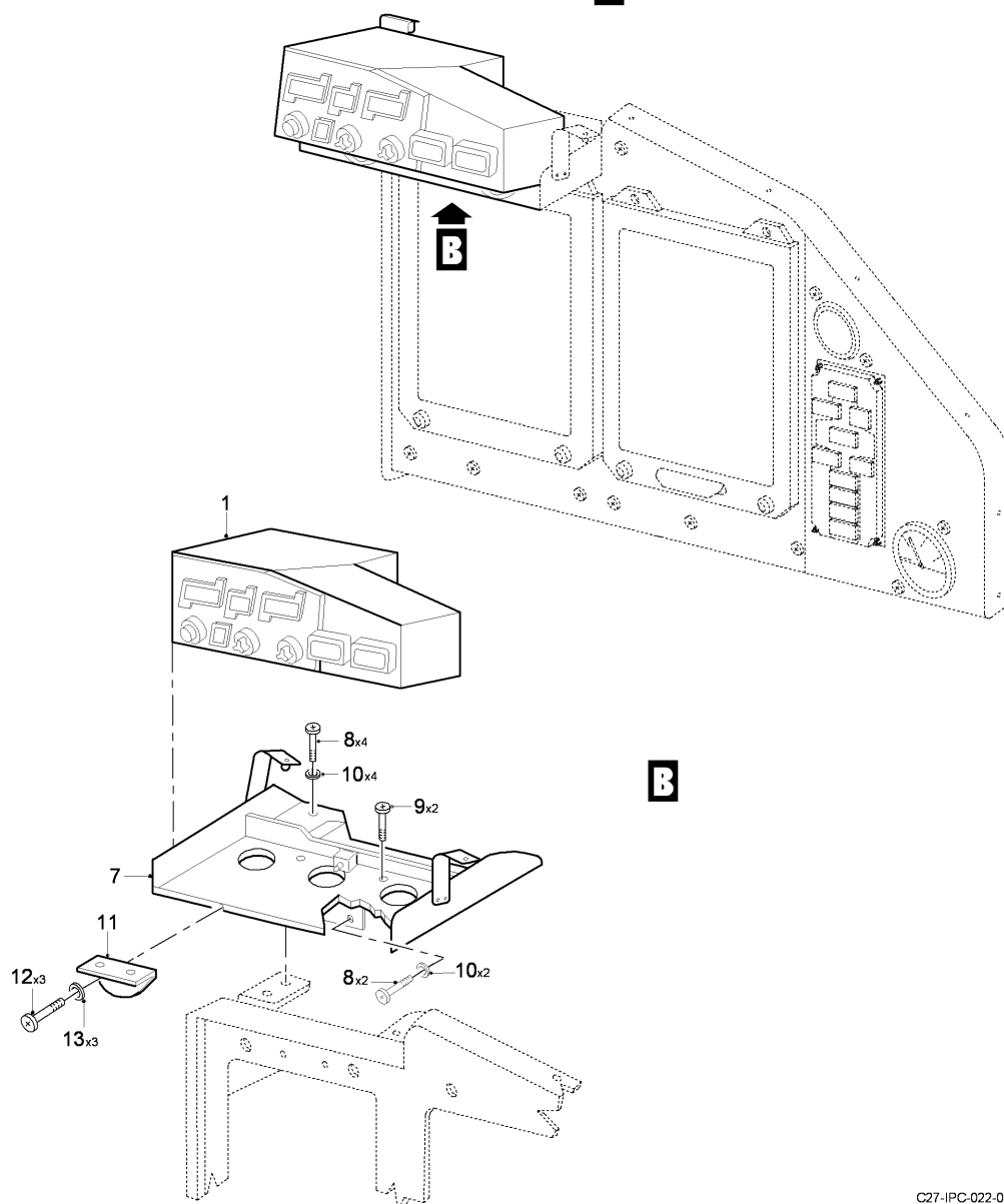
FIG 03 SET/WARNING PANEL COPILOT INSTL, Z31AA (SHEET 1 OF 1)
