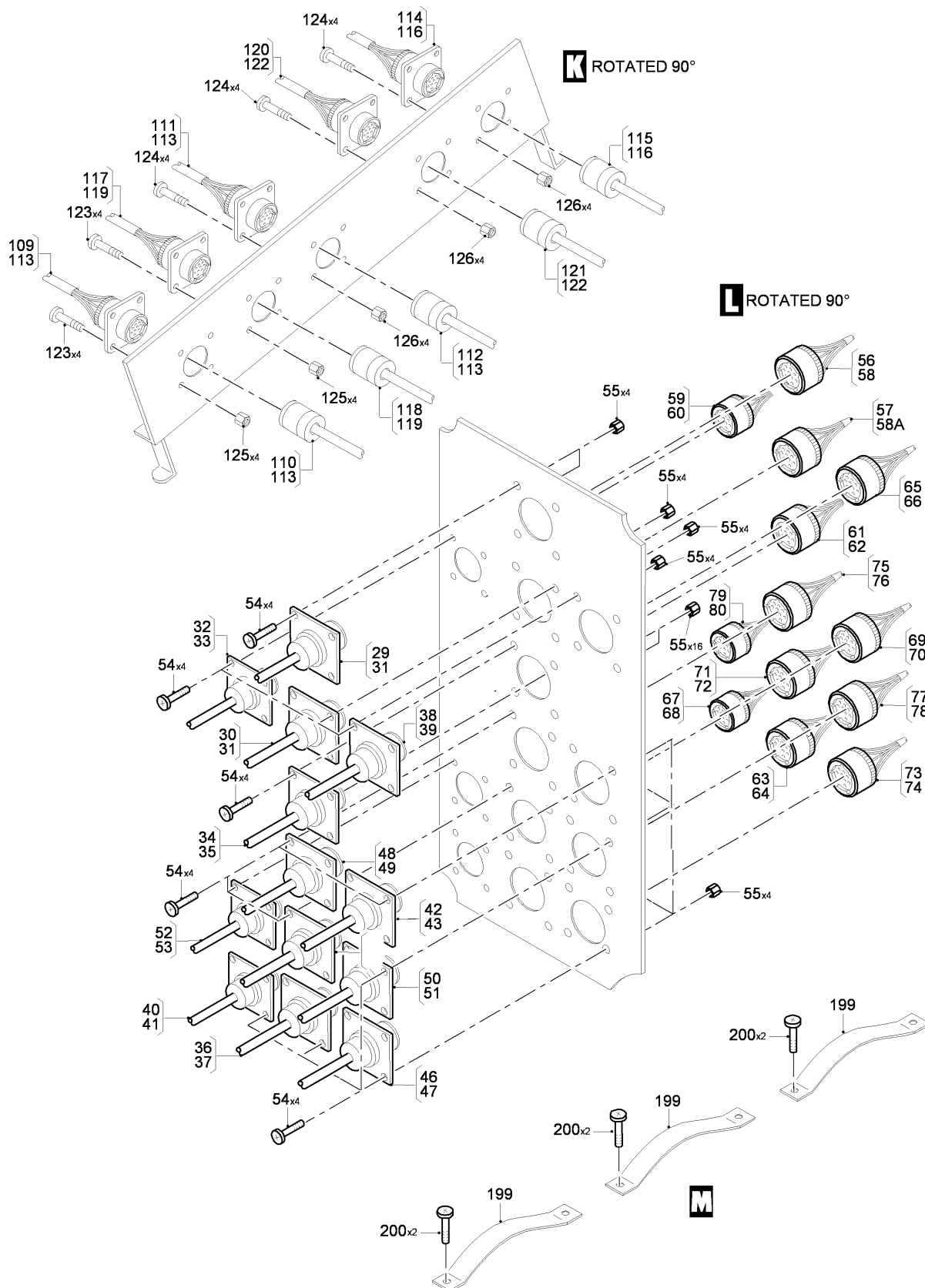
FIG 09 ELECTRICAL AND ELECTRONICS INSTL, Z31AA-31BC, RH (SHEET 5 OF 7)
