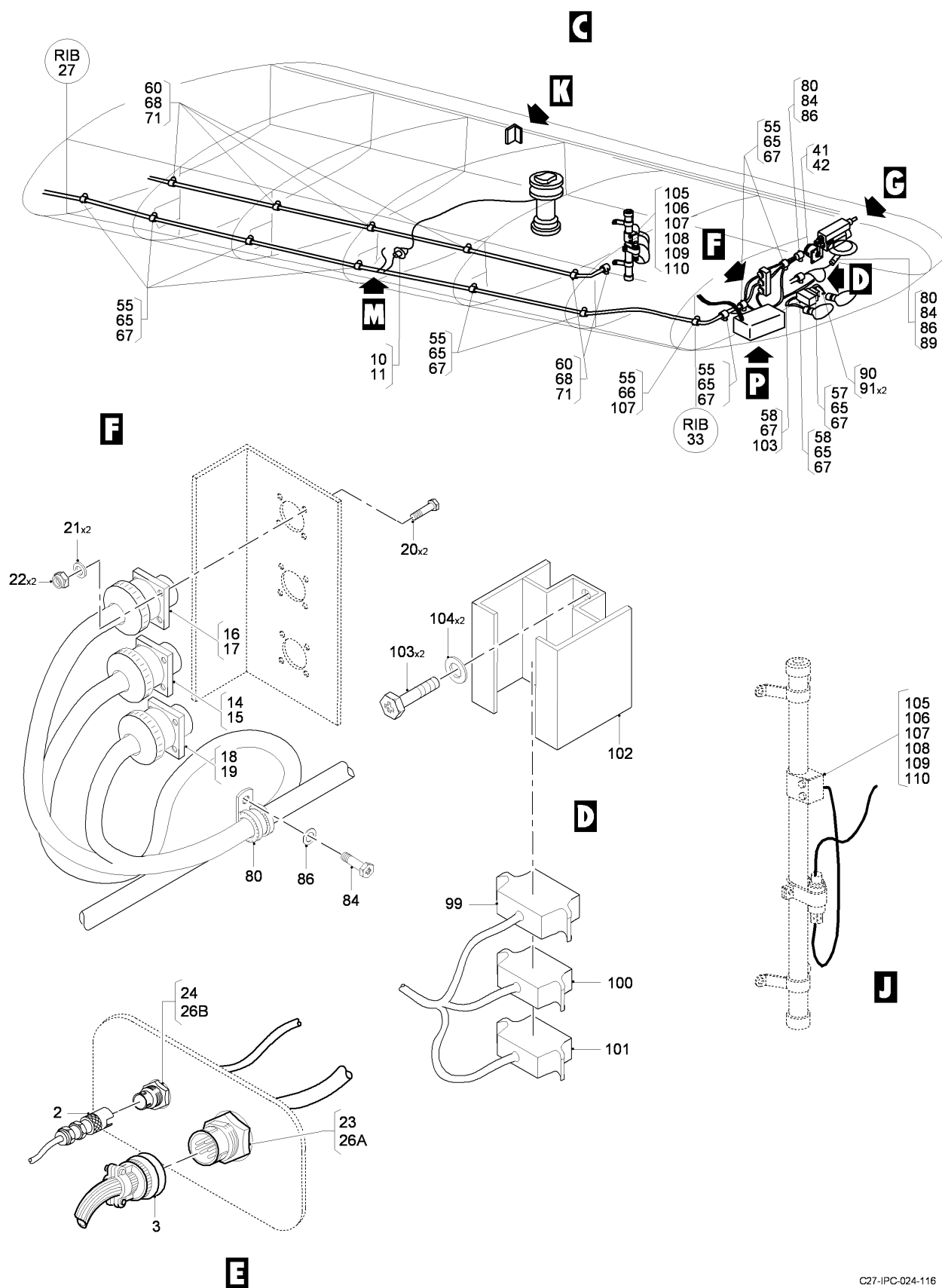
FIG 24 ELECTRICAL AND ELECTRONICS INSTL, Z11AA-11AB, LH (SHEET 2 OF 3)
