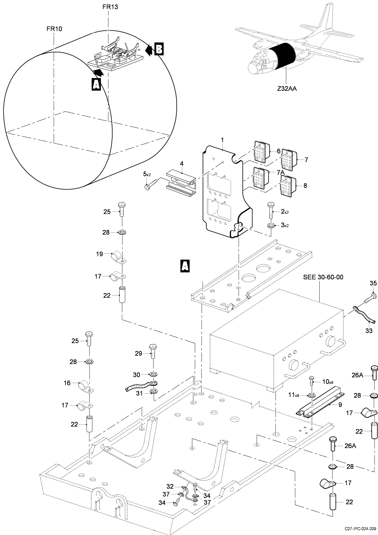
FIG 18 ELECTRICAL AND ELECTRONICS INSTL, Z32AA (SHEET 1 OF 2)
