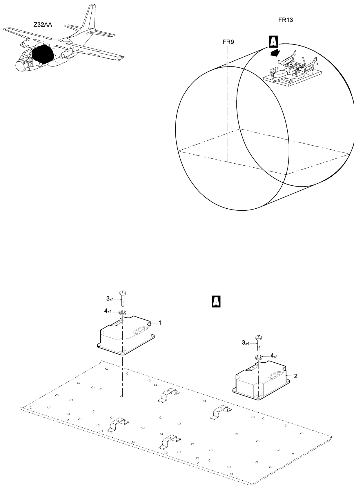
FIG 03 HYDRAULIC PUMP CONTACTOR INSTL, Z32AA (SHEET 1 OF 1)
