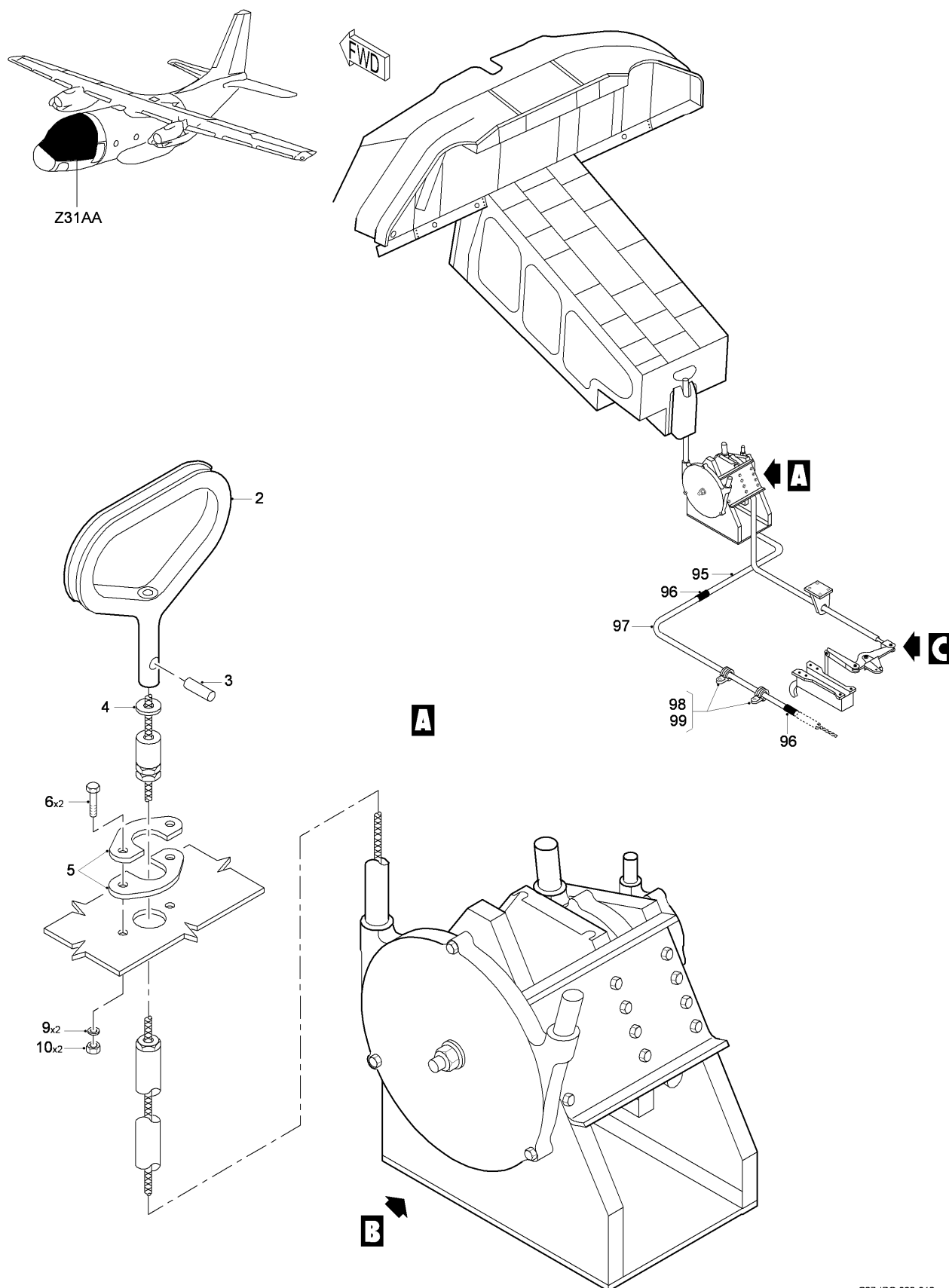
FIG 02 EMERGENCY CONTROL INSTL - MAIN LANDING GEAR, Z31AA (SHEET 1 OF 3)
