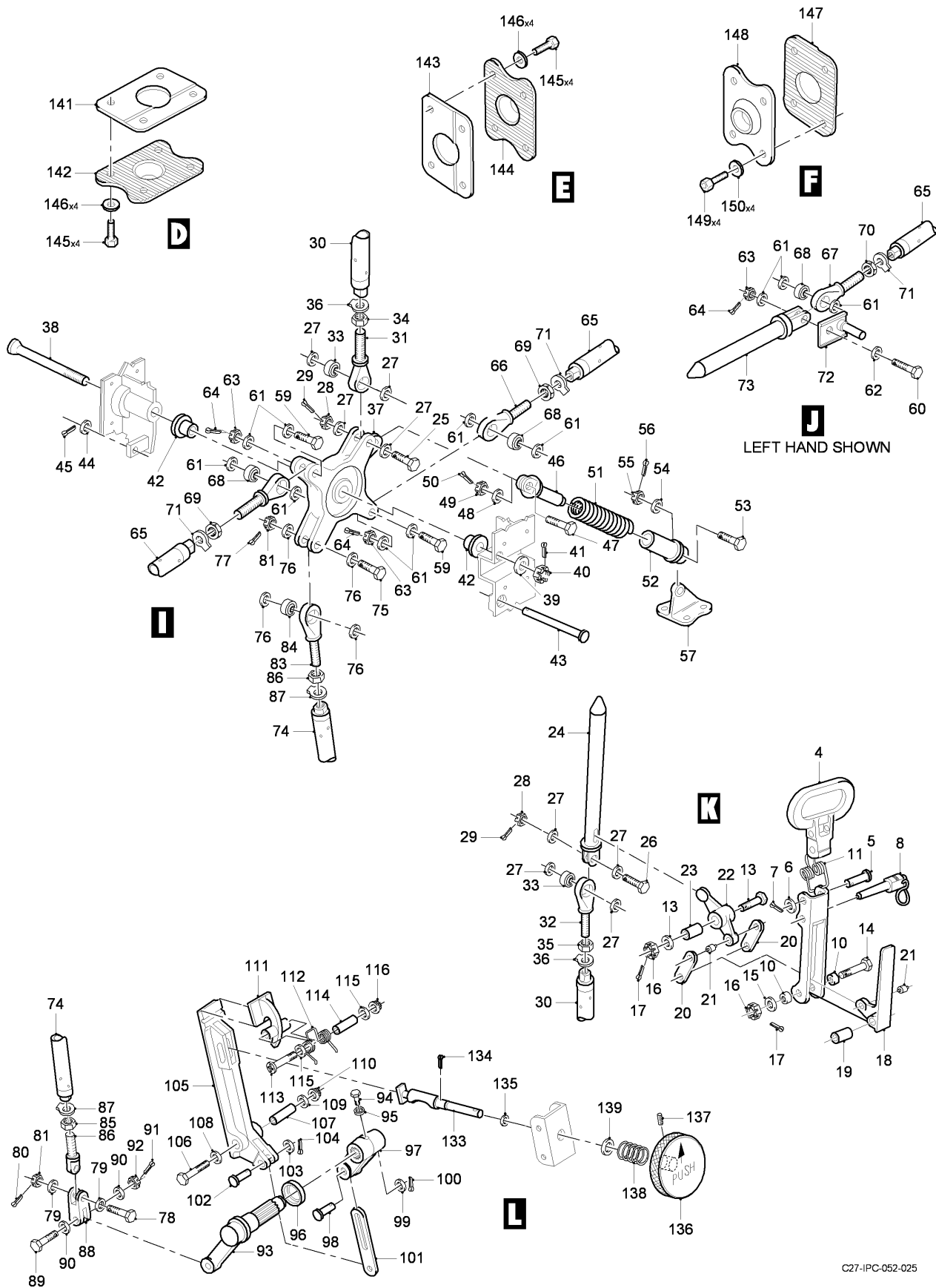
FIG 02 EMERGENCY EXIT DOOR INSTL - RH SIDE, Z31AB (SHEET 2 OF 2)
