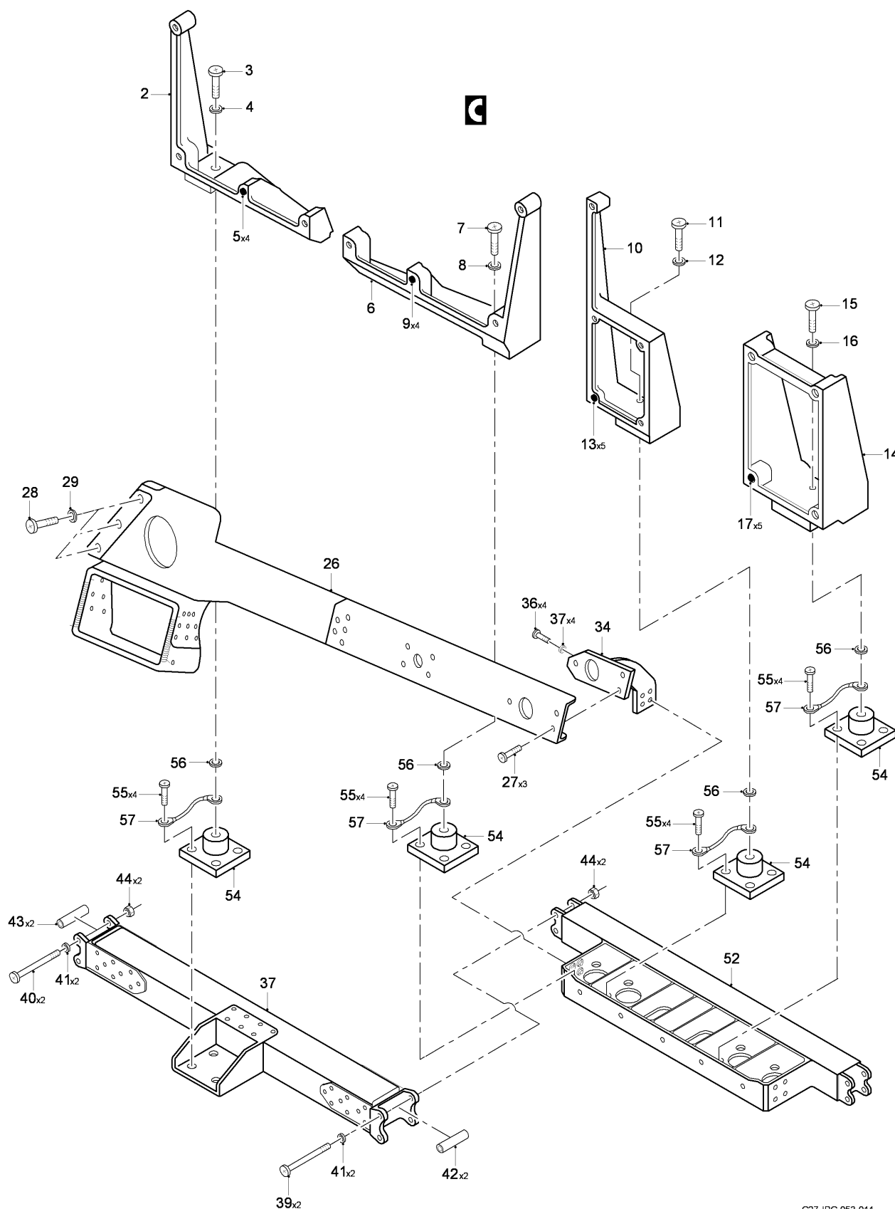
FIG 03 INSTRUMENTS PANELS INSTL, Z31AA (SHEET 2 OF 5)
