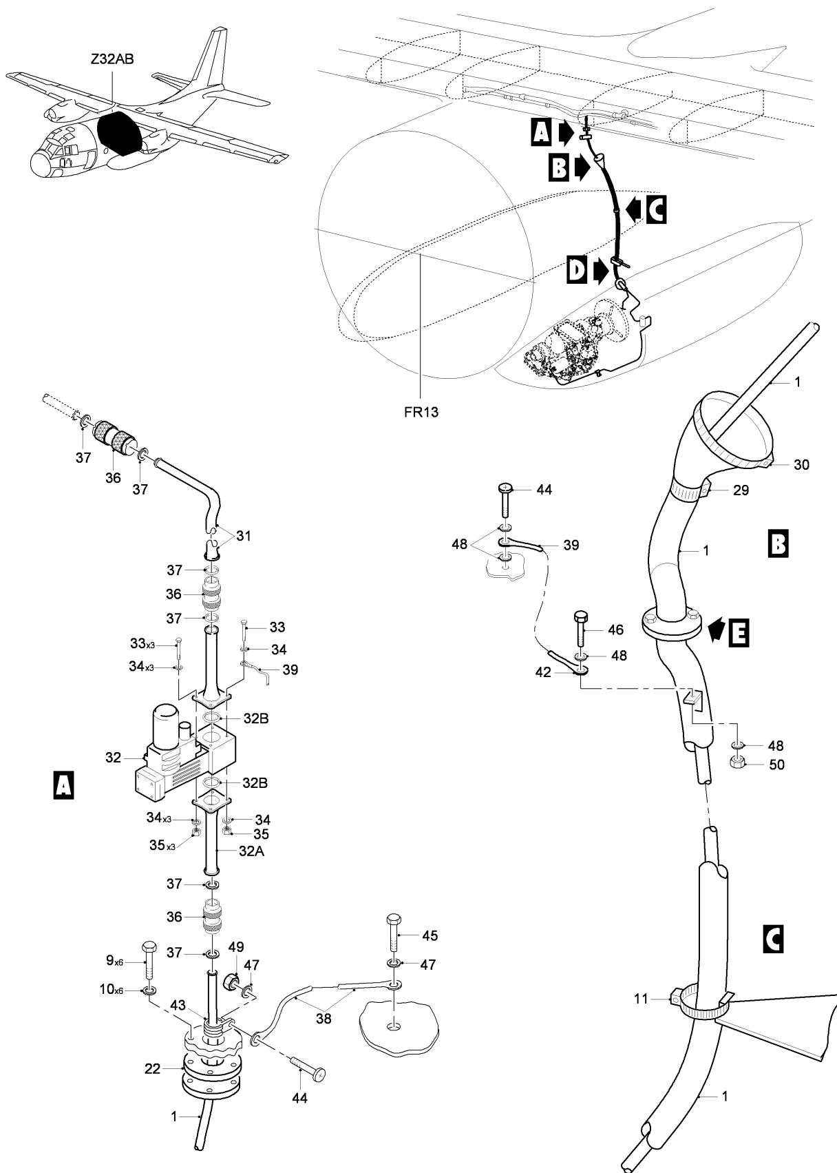
FIG 01 APU FUEL SUPPLY INSTL - CENTER FUSELAGE, Z32AB (SHEET 1 OF 2)
