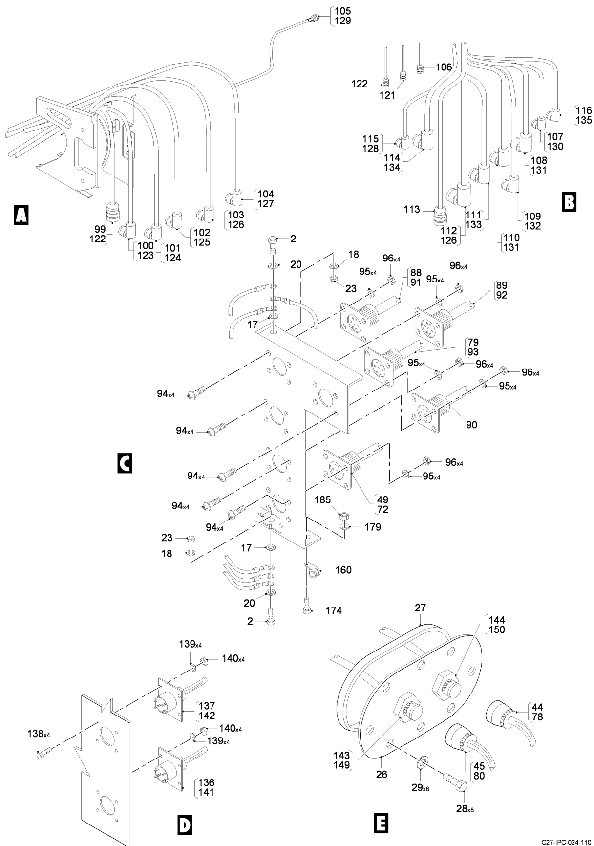
FIG 23 ELECTRICAL AND ELECTRONICS INSTL - CENTER WING, Z33AB, RH (SHEET 2 OF 6)
