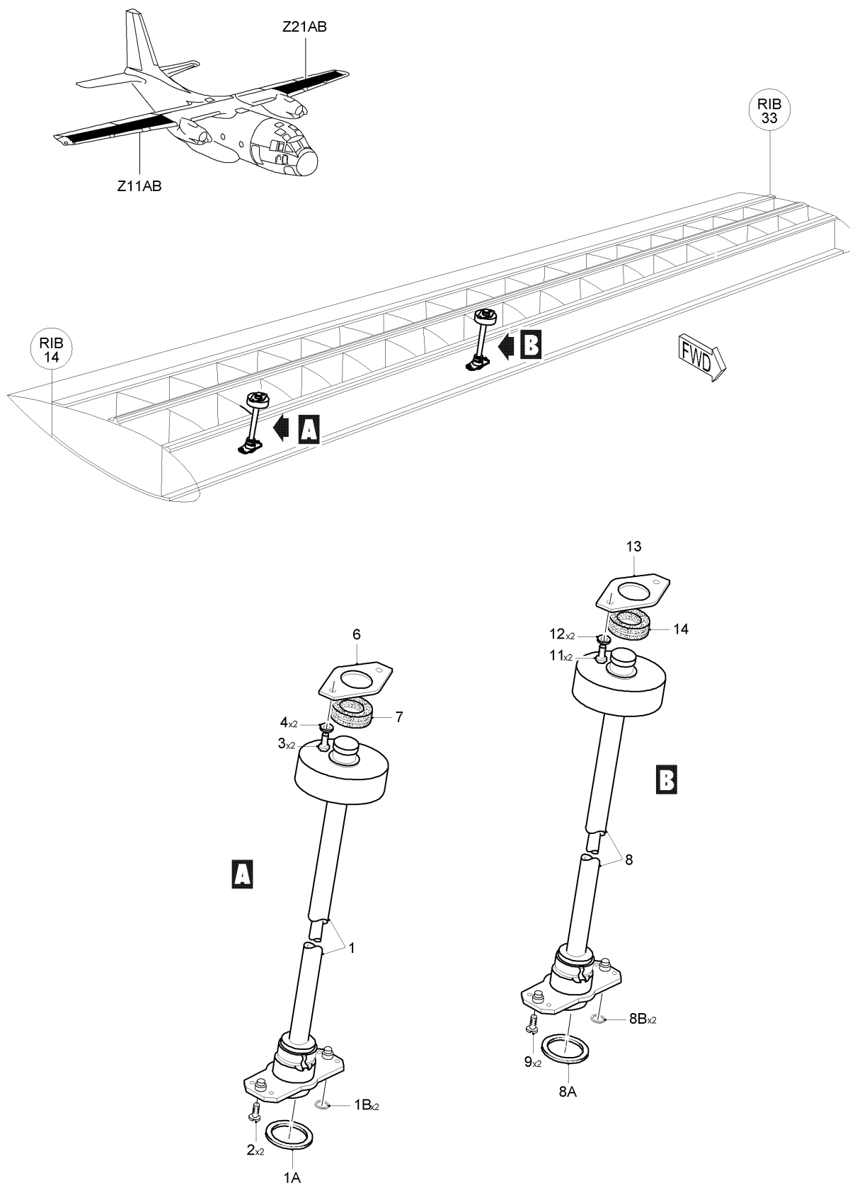
FIG 04 INDICATOR FUEL QUANTITY INSTL, Z11AB-21AB, LH-RH (SHEET 1 OF 1)
