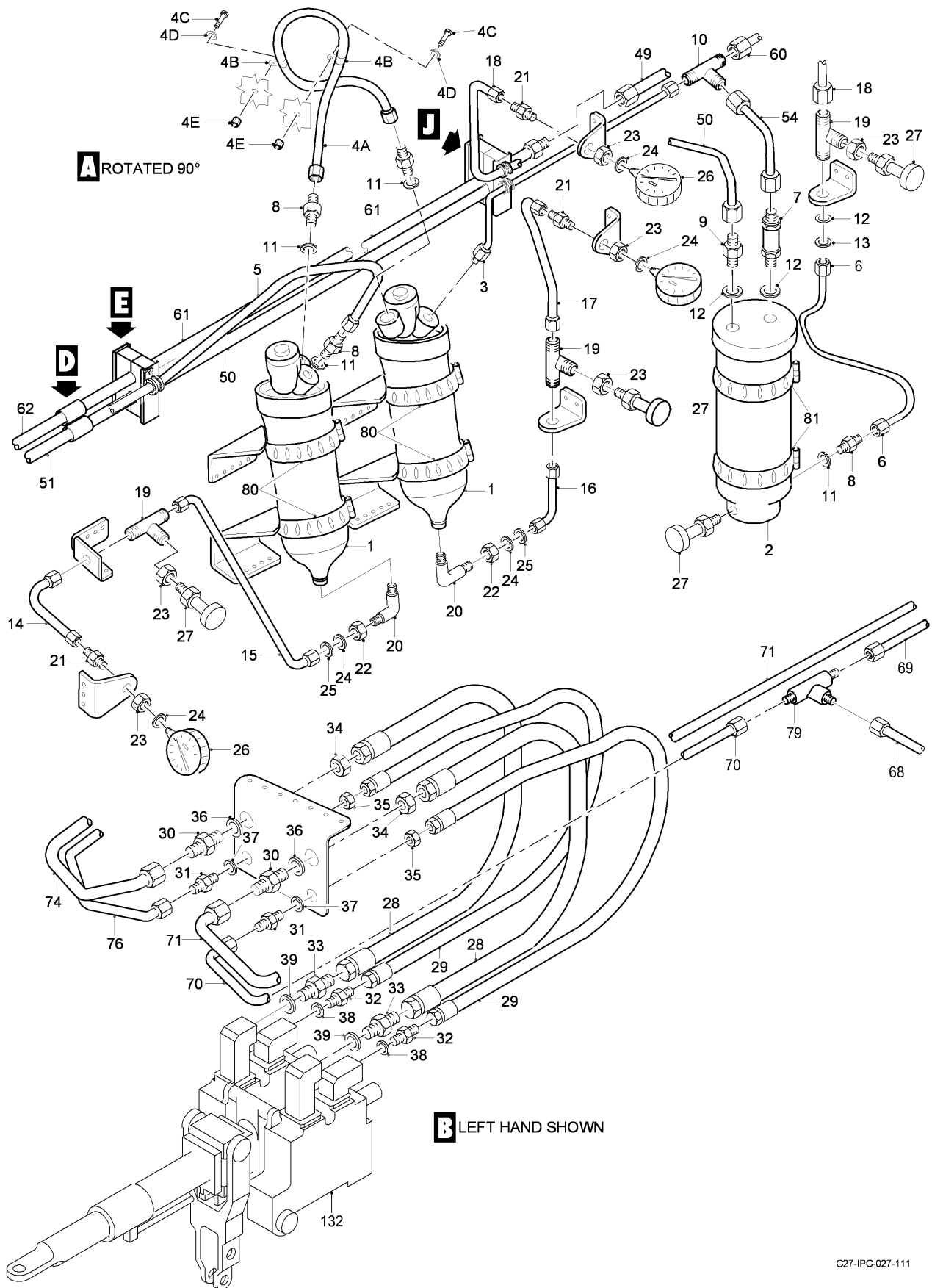
FIG 05 ELEVATOR AND RUDDER HYDRAULIC ACCUMULATOR INSTL, Z34AA, LH (SHEET 2 OF 3)
