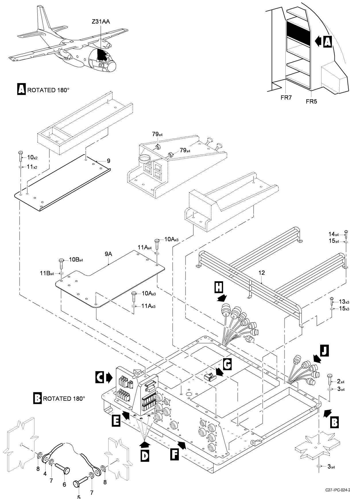
FIG 04 FOURTH SHELF INSTL - ELECTRONIC COMPARTMENT, Z31AA (SHEET 1 OF 3)
