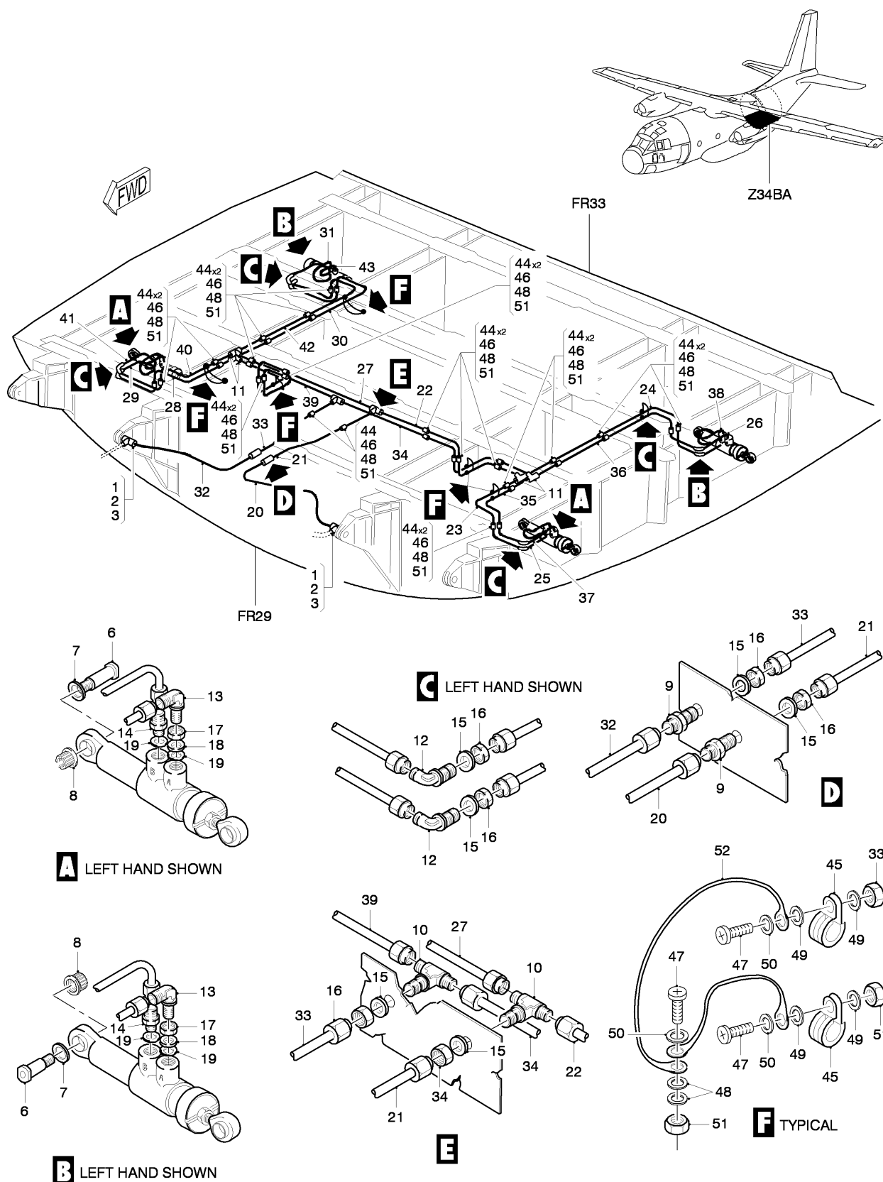
FIG 03 HYDRAULIC PIPING INSTL - CARGO RAMP, Z34BA (SHEET 1 OF 1)
