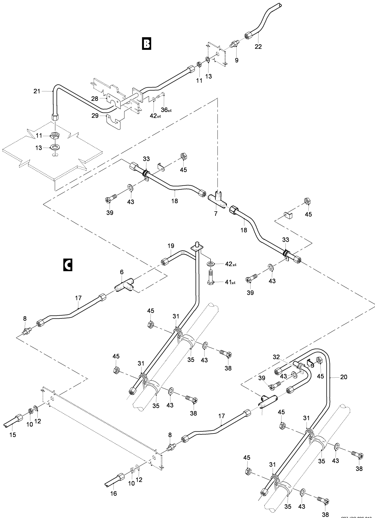
FIG 03 ENGINE FIRE EXTINGUISHING INSTL, Z12AC-12AD-22AC-22AD (SHEET 2 OF 3)
