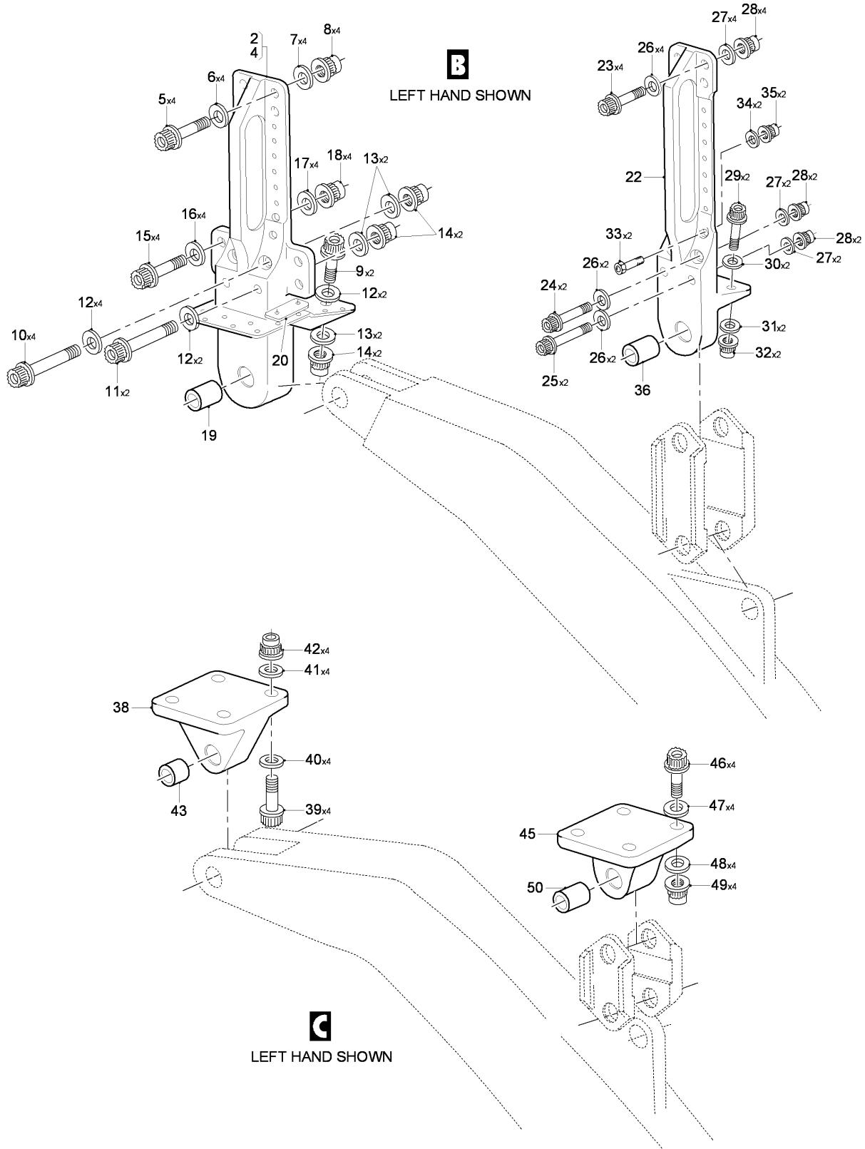
FIG 01 STRUCTURE INSTL - CENTER WING, Z33AB (SHEET 2 OF 3)
