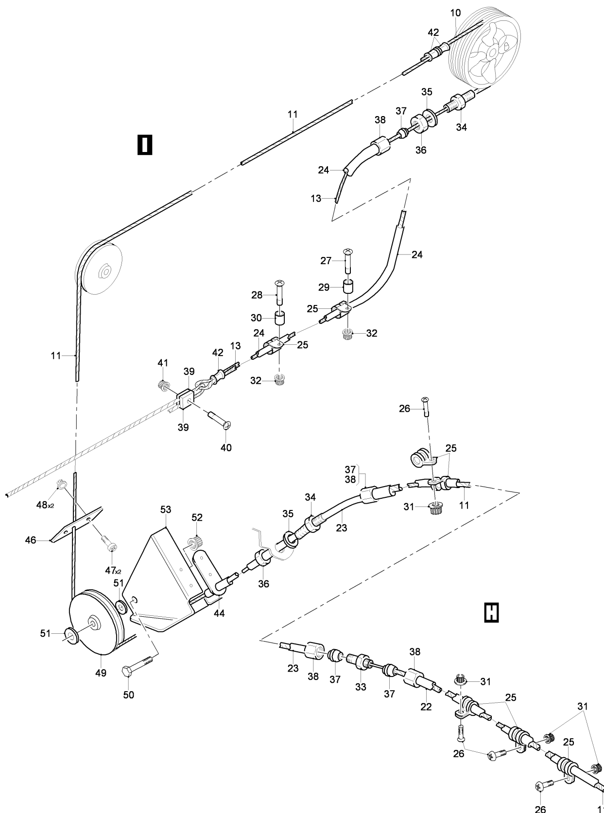
FIG 02 LIFE RAFTS OPENING EMERG CONTROL INSTL, Z31AB-32AA-32AB-32AC (SHEET 3 OF 3)
