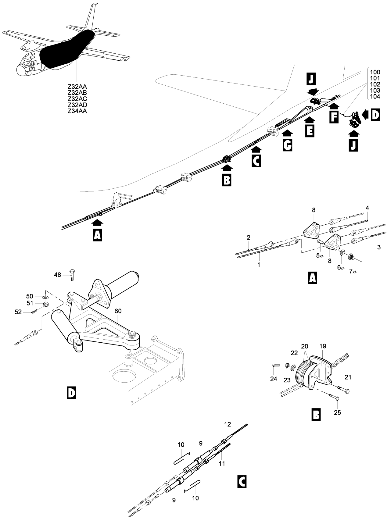
FIG 02 CONTROLS LOKING INSTL, Z32AA-32AB-32AC-32AD-34AA (SHEET 1 OF 3)
