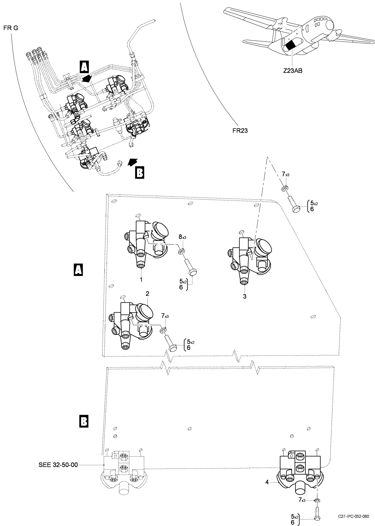
FIG 14 SELECTOR FLOW INSTL - CARGO DOOR AND CARGO RAMP, Z23AB (SHEET 1 OF 1)
