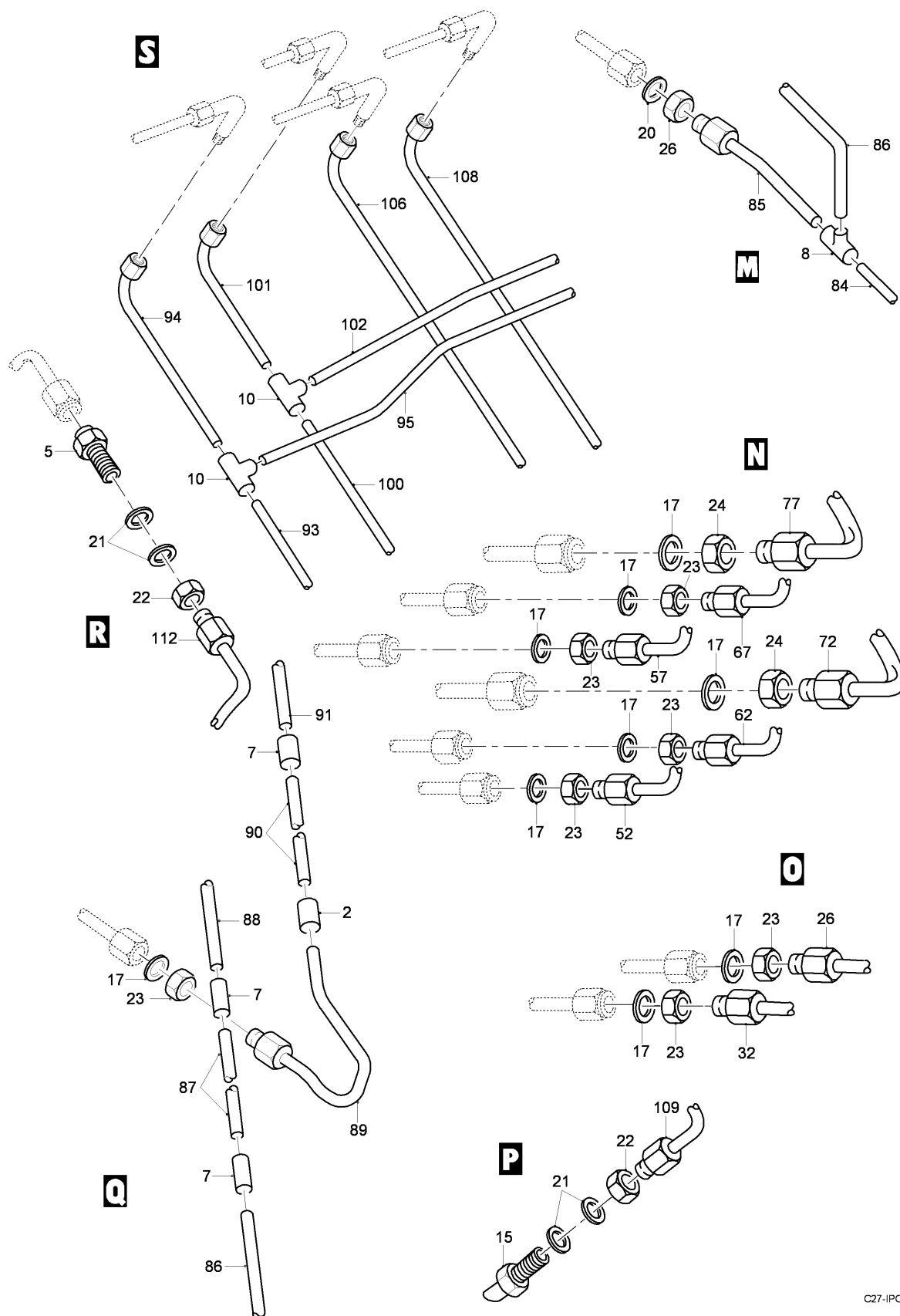
FIG 04 HYDRAULIC INSTL - CENTER FUSELAGE, Z32AC-32AD (SHEET 3 OF 6)
