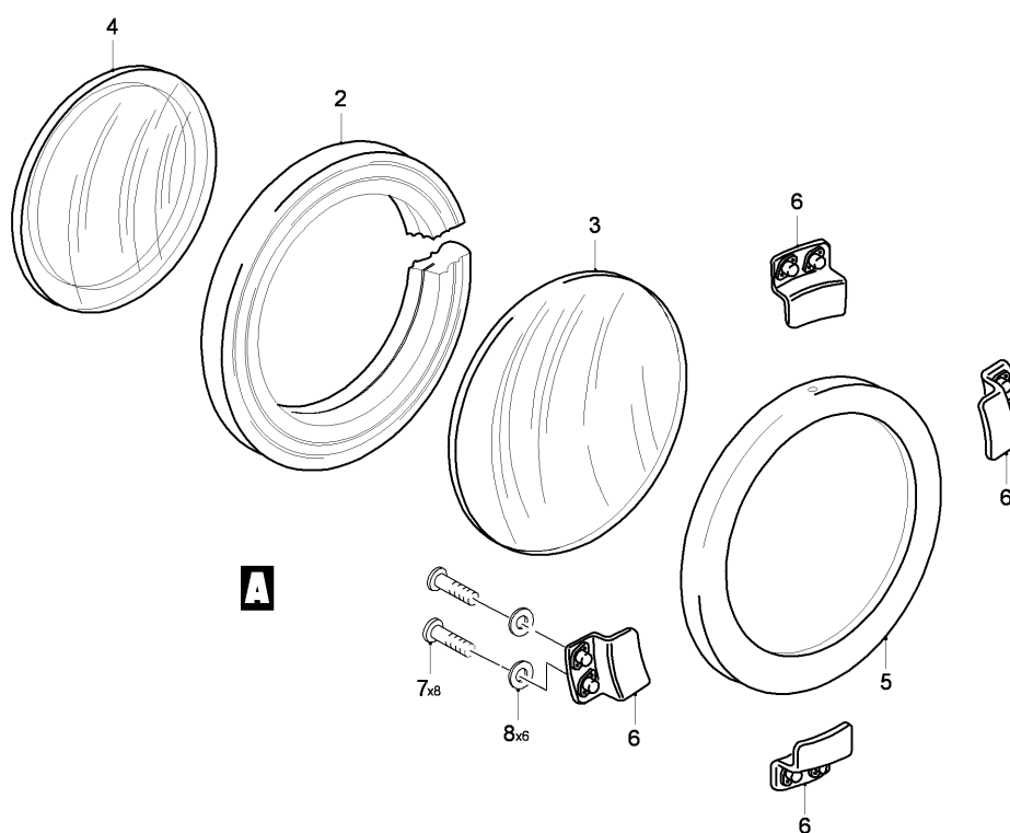
FIG 01 WINDOW INSTL - PARATROOP DOOR, Z32AD, LH-RH (SHEET 1 OF 1)
