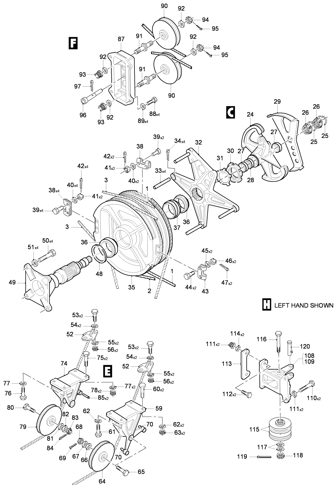
FIG 04 AILERON CONTROLS INSTL, Z33AB (SHEET 2 OF 2)
