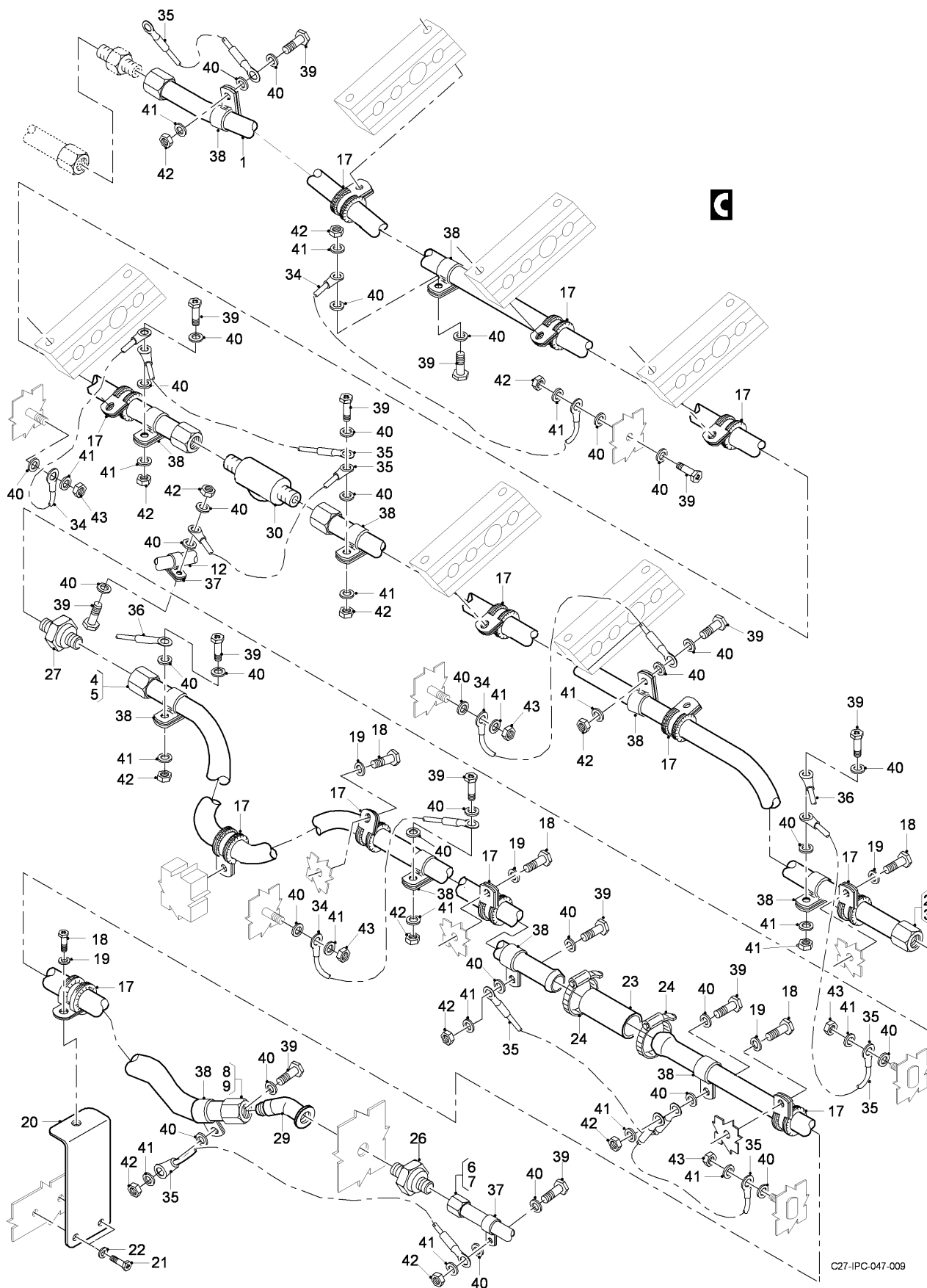
FIG 04 FUEL TANK EXPLOSION PROTECTION SYS INSTL, Z11AB-21AB, LH-RH (SHEET 2 OF 2)
