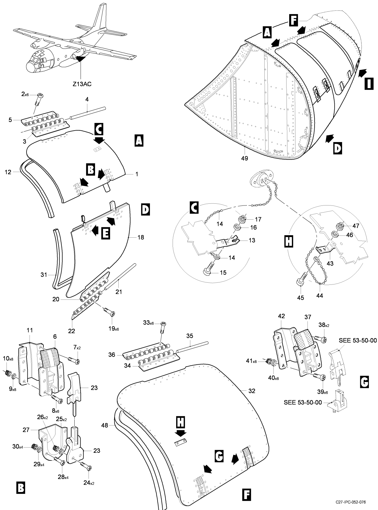
FIG 10 DOOR INSTL - MLG REAR, Z13AC, LH (SHEET 1 OF 2)
