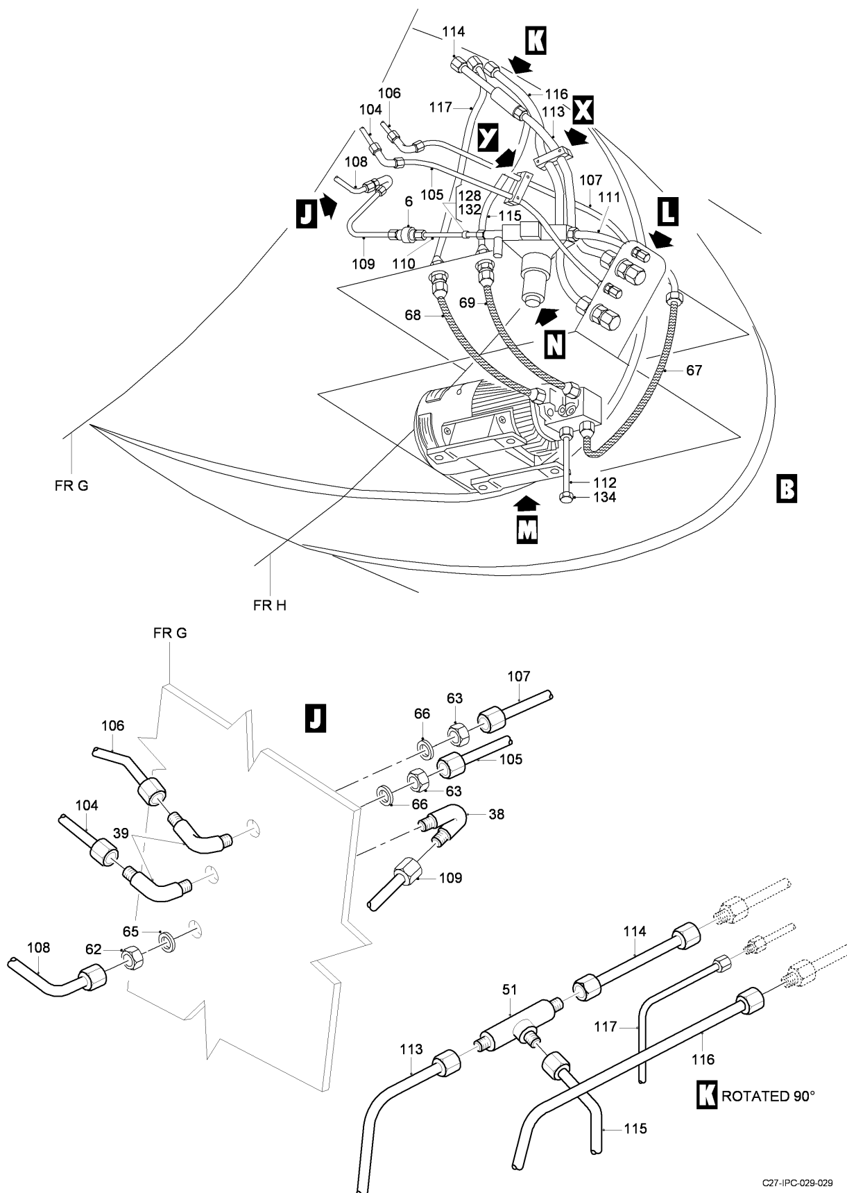
FIG 07 HYDRAULIC INSTL - MLG, Z13AB, LH (SHEET 5 OF 8)
