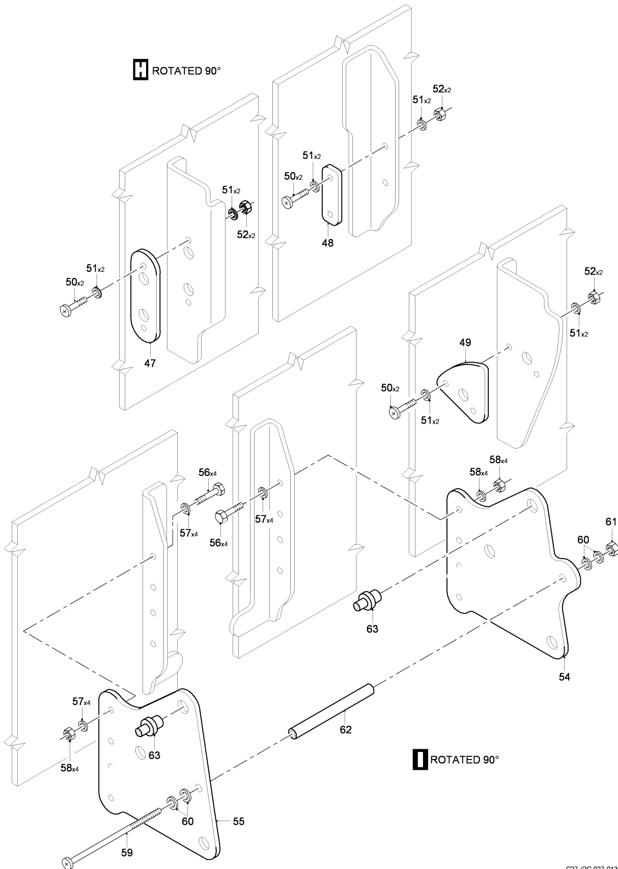
FIG 01 CONTROLS LOCKING INSTL, Z31AB-31BB (SHEET 4 OF 4)
