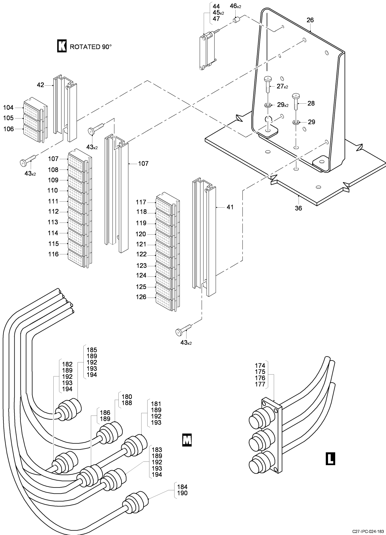
FIG 07 FIRST SHELF INSTL - ELECTRICAL COMPARTMENT, Z31AA (SHEET 5 OF 5)
