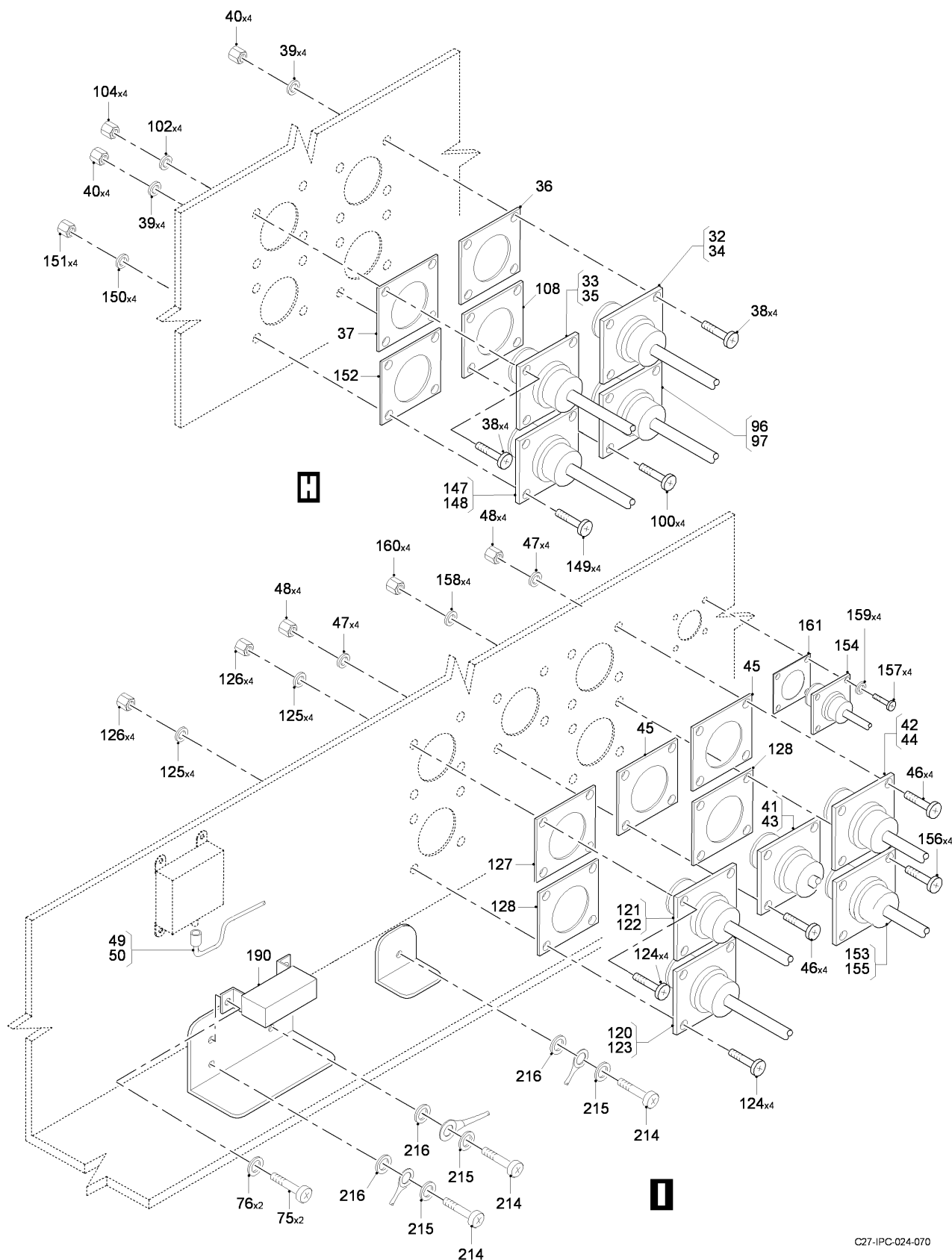
FIG 16 ELECTRICAL AND ELECTRONICS INSTL, Z31AB-32AA-32AB-32AC, RH (SHEET 6 OF 8)
