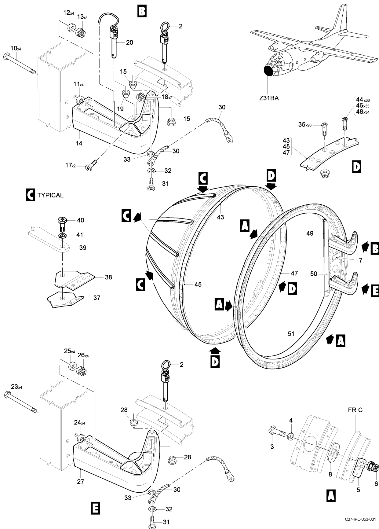
FIG 01 RADOME INSTL, Z31BA (SHEET 1 OF 1)
