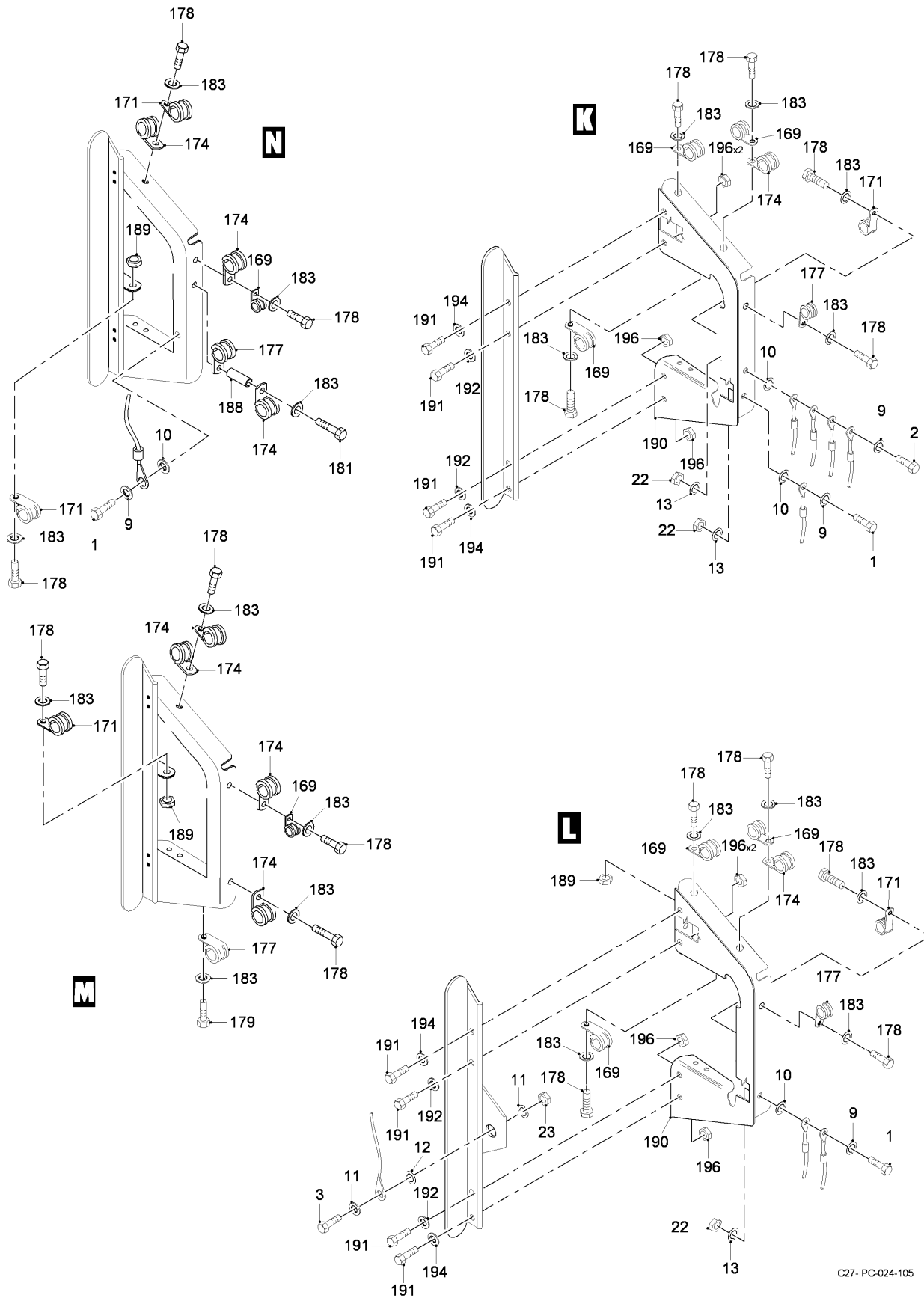
FIG 22 ELECTRICAL AND ELECTRONICS INSTL - CENTER WING, Z33AB, LH (SHEET 4 OF 7)
