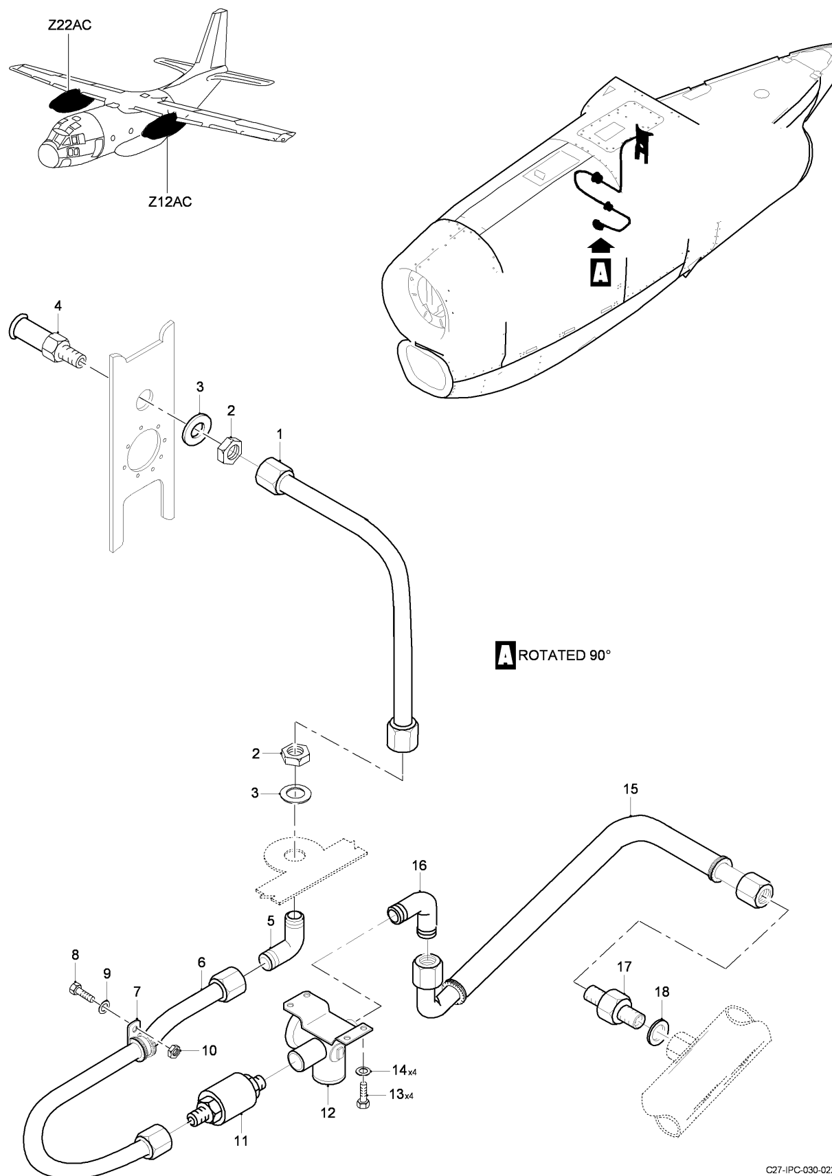
FIG 03 ANTI-ICING NACELLE INSTL, Z12AC-22AC (SHEET 1 OF 1)
