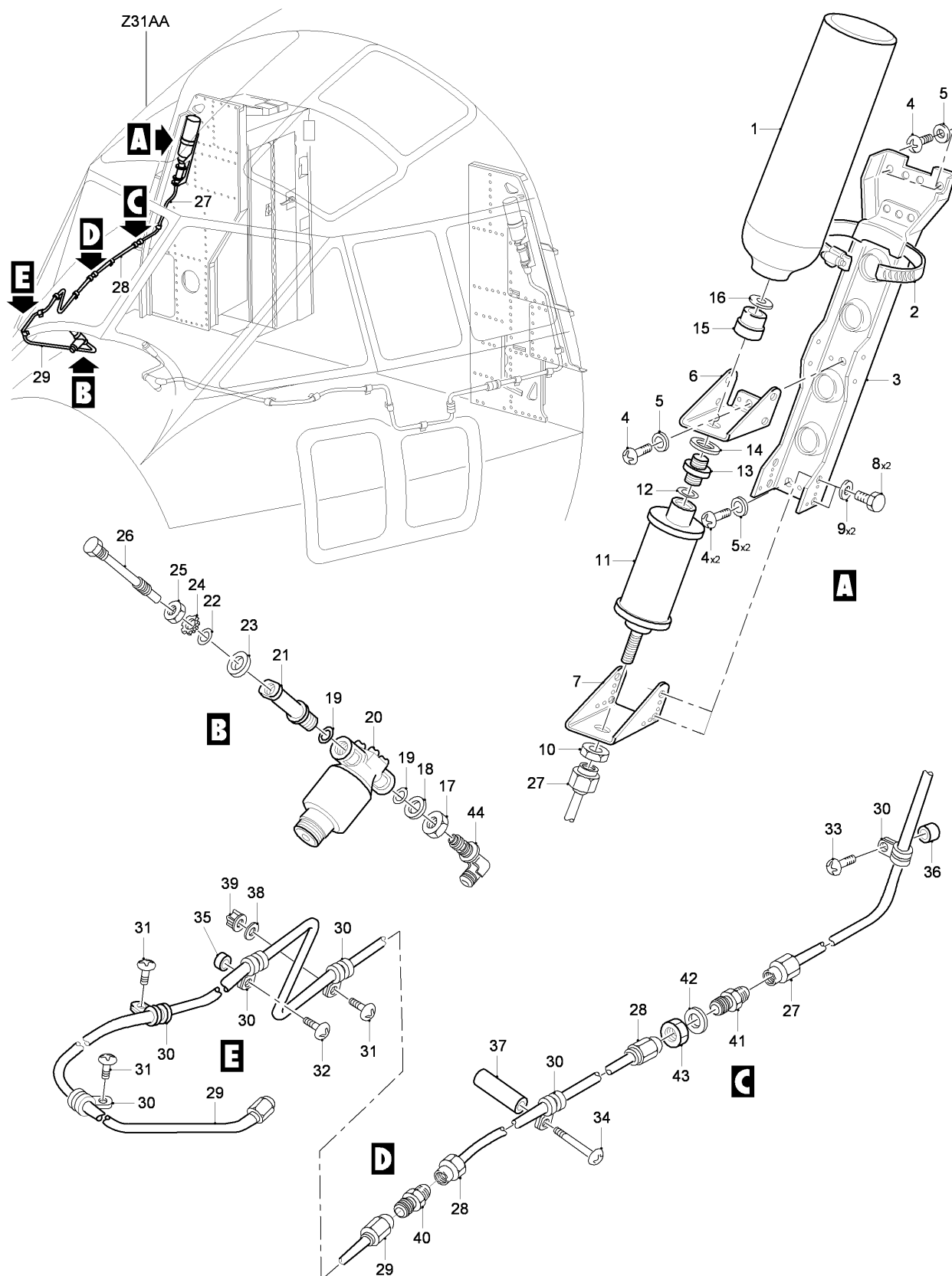
FIG 03 RAIN REMOVAL INSTL, Z31AA, RH (SHEET 1 OF 1)
