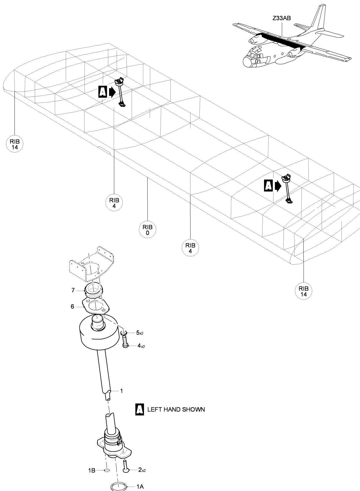
FIG 03 INDICATOR FUEL QUANTITY INSTL - CENTER WING, Z33AB, LH-RH (SHEET 1 OF 1)
