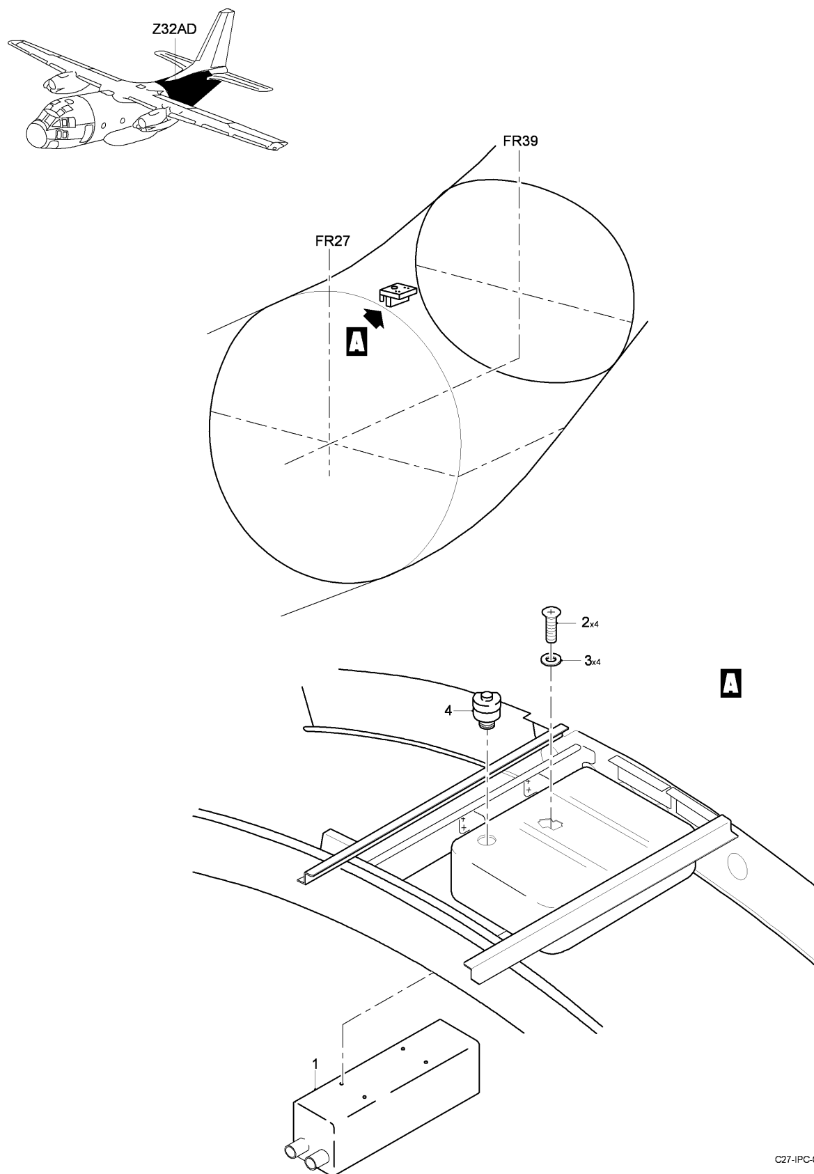
FIG 06 EMERGENCY LOCATOR TRANSMITTER INSTL, Z32AD (SHEET 1 OF 1)
