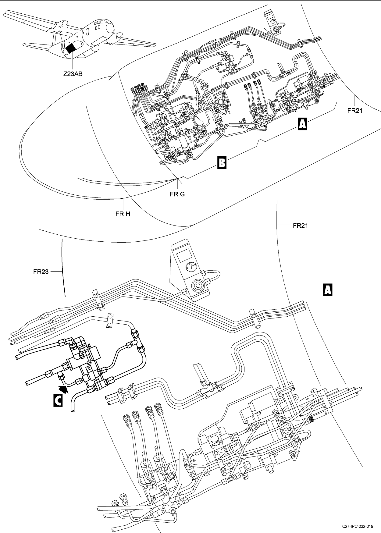
FIG 04 HYDRAULIC VALVE - MLG, Z23AB, RH (SHEET 1 OF 2)
