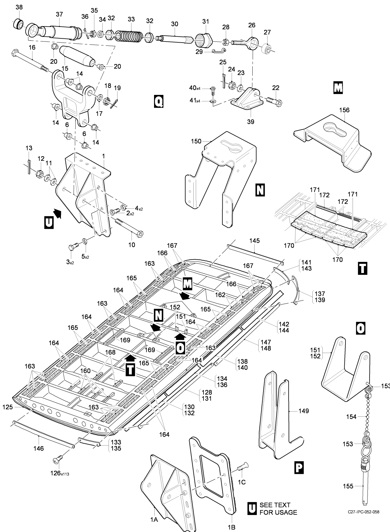
FIG 12 CARGO DOOR ASSY (SHEET 3 OF 4)
