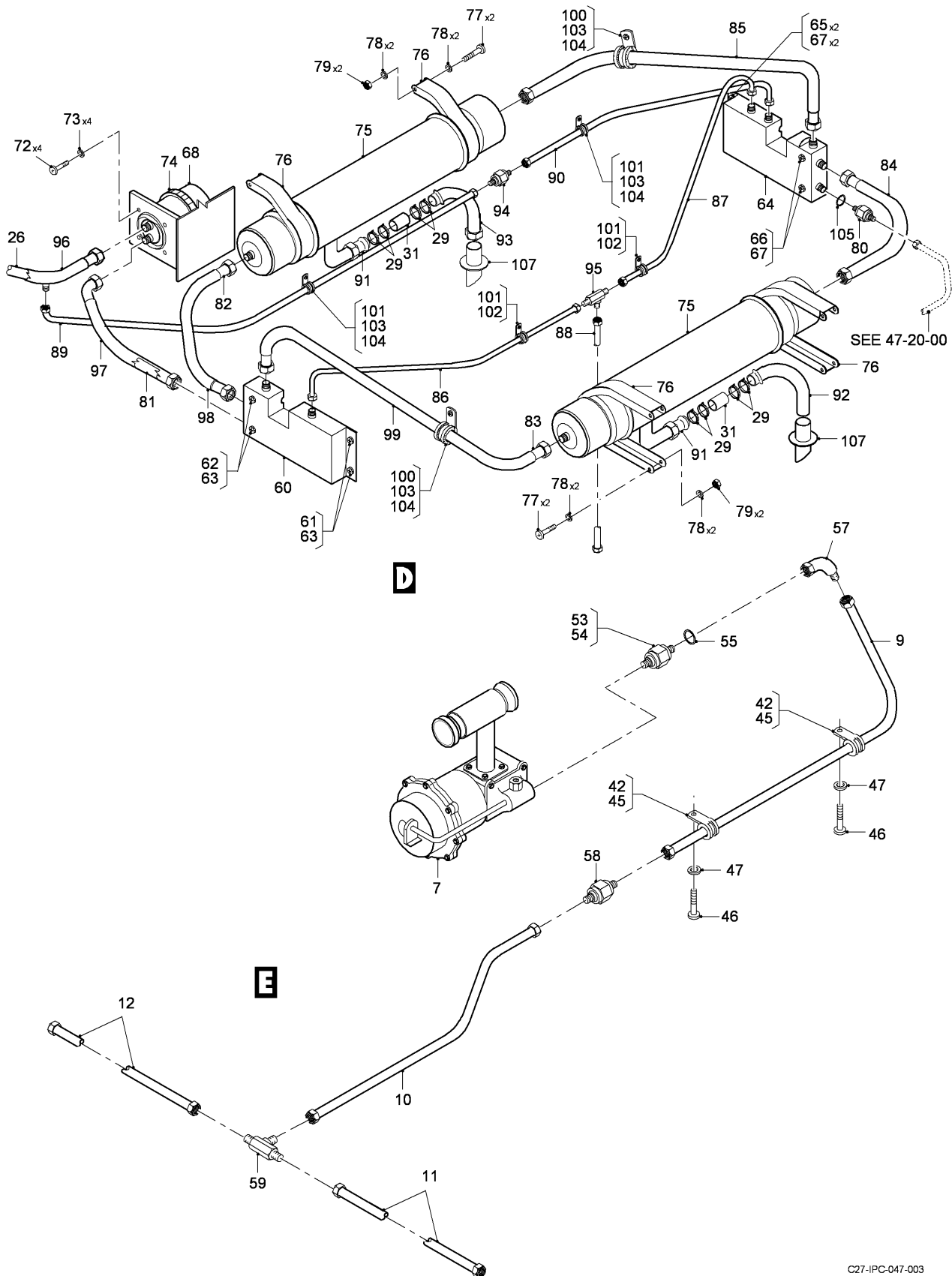
FIG 01 FUEL TANK EXPLOSION PROTECTION SYSTEM INSTL, Z32BA (SHEET 3 OF 3)
