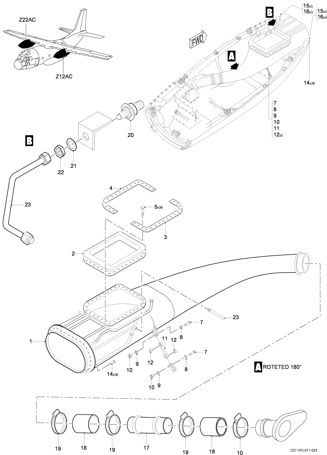
FIG 02 AIR INTAKE LOWER INSTL - ENGINE, Z12AC-22AC, LH-RH (SHEET 1 OF 1)
