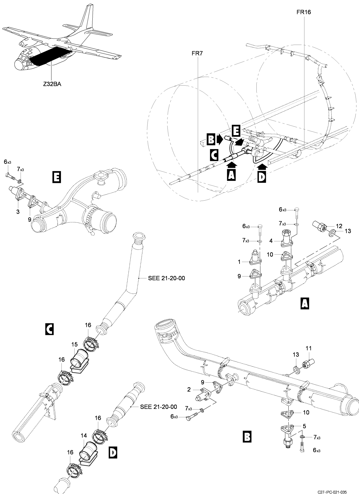
FIG 03 TEMPERATURE SENSOR BOX INSTL, Z31AB (SHEET 1 OF 1)
