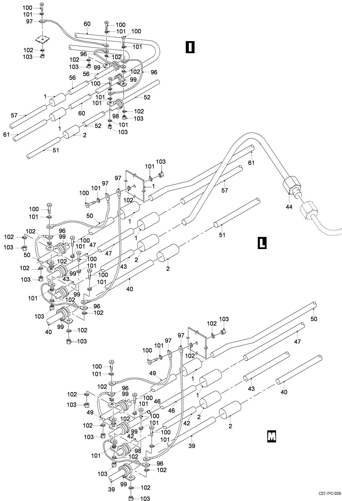
FIG 02 HYDRAULIC INSTL - CENTER FUSELAGE, LOWER, Z32BA (SHEET 4 OF 8)
