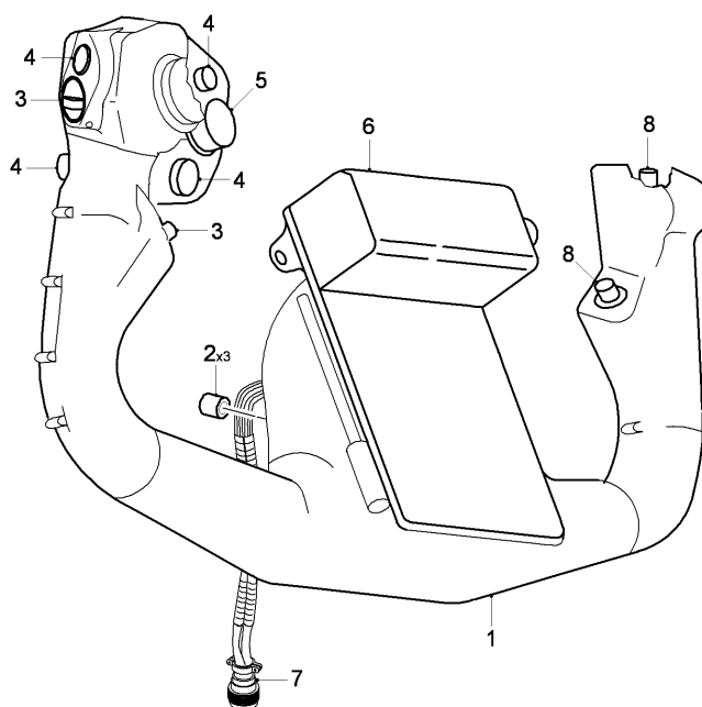
FIG 01 WHEEL ASSY INSTL - CONTROL COLUMN, Z31AA, LH-RH (SHEET 1 OF 1)
