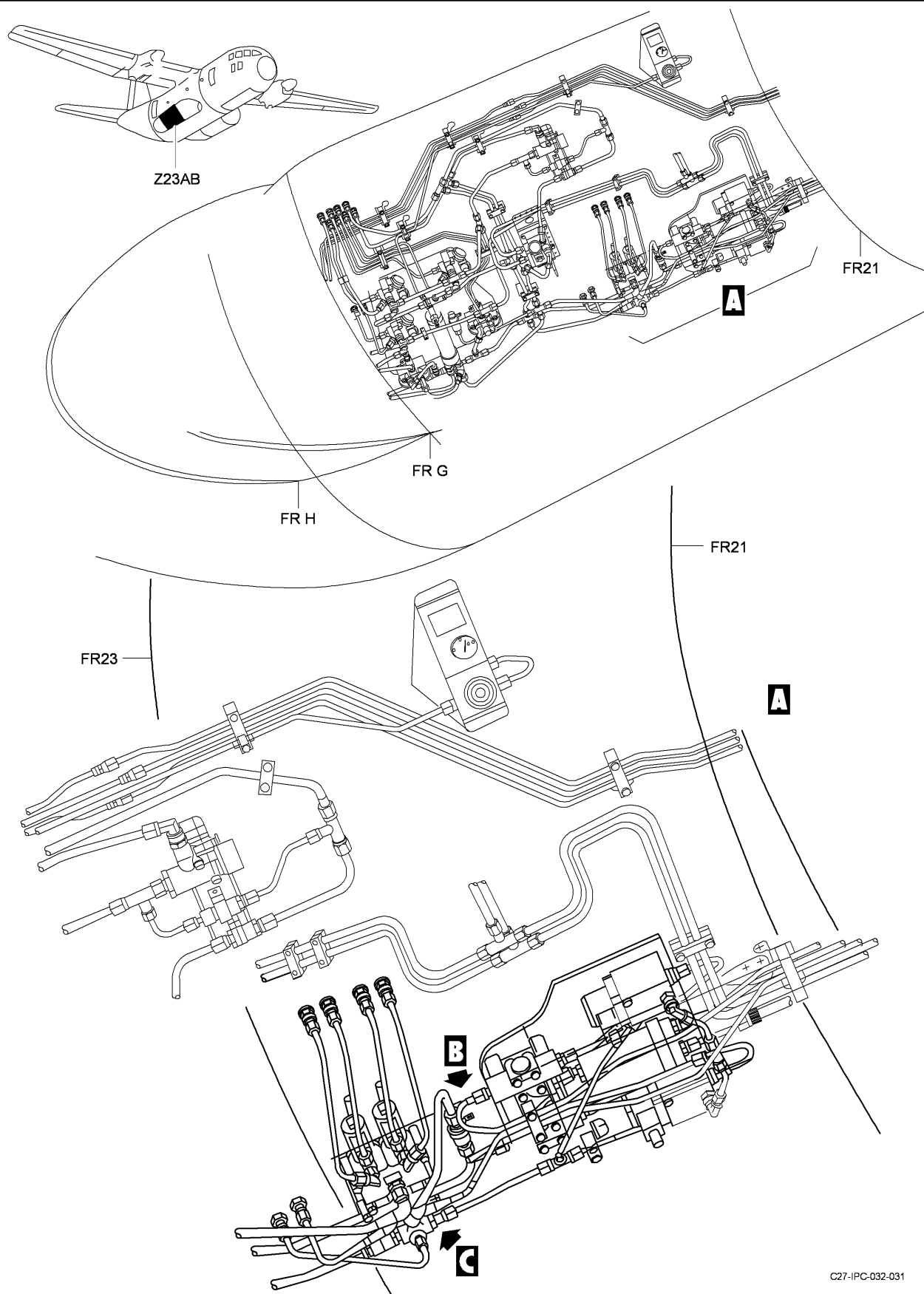
FIG 07 HYDRAULIC COMPONENT INSTL - MLG, Z23AB, RH (SHEET 1 OF 2)
