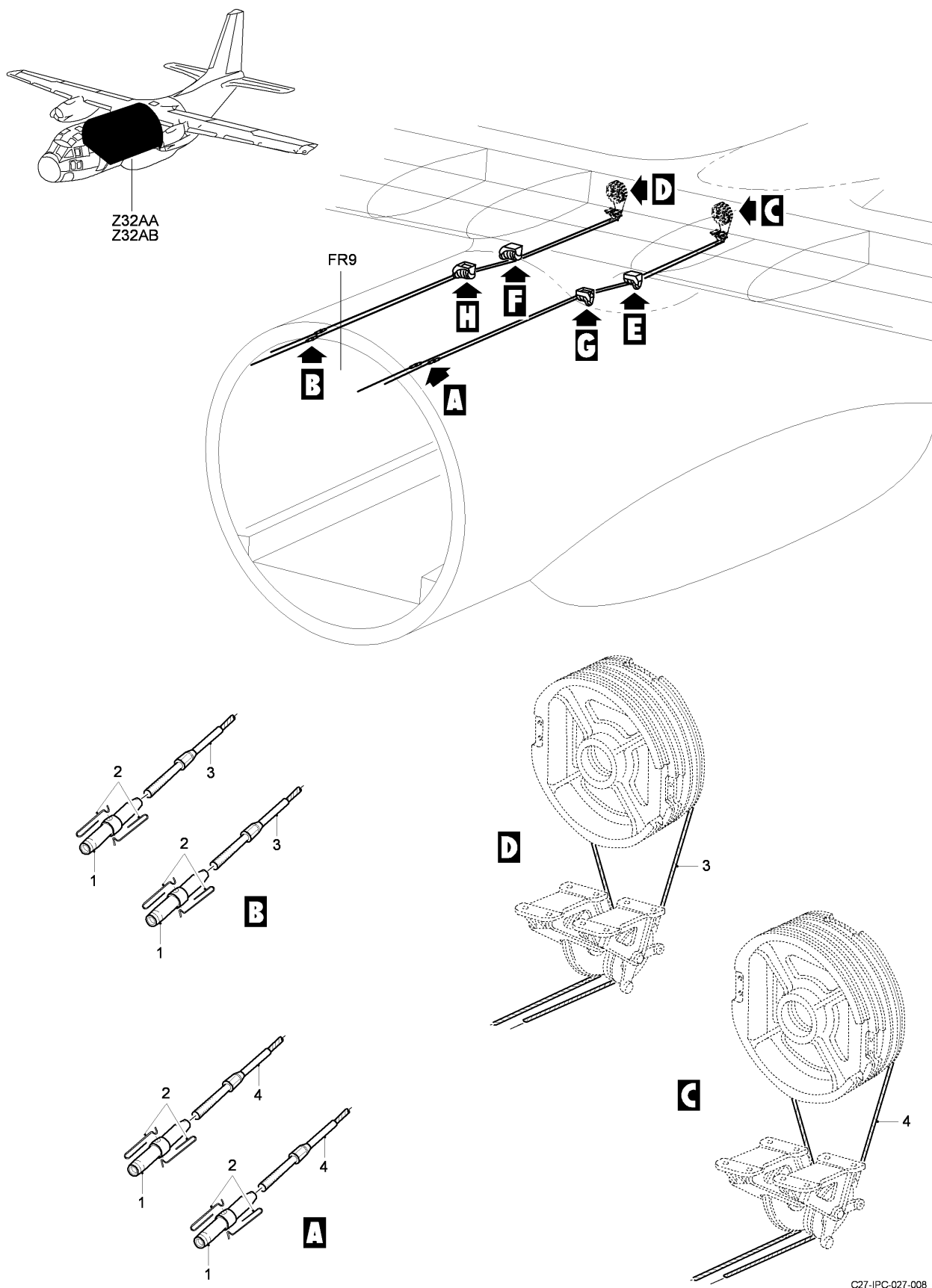
FIG 03 AILERON CONTROLS INSTL, Z32AA-32AB (SHEET 1 OF 3)
