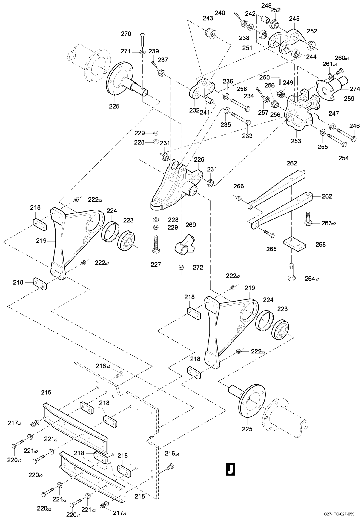
FIG 07 ELEVATOR CONTROLS INSTL, Z34AA (SHEET 4 OF 8)
