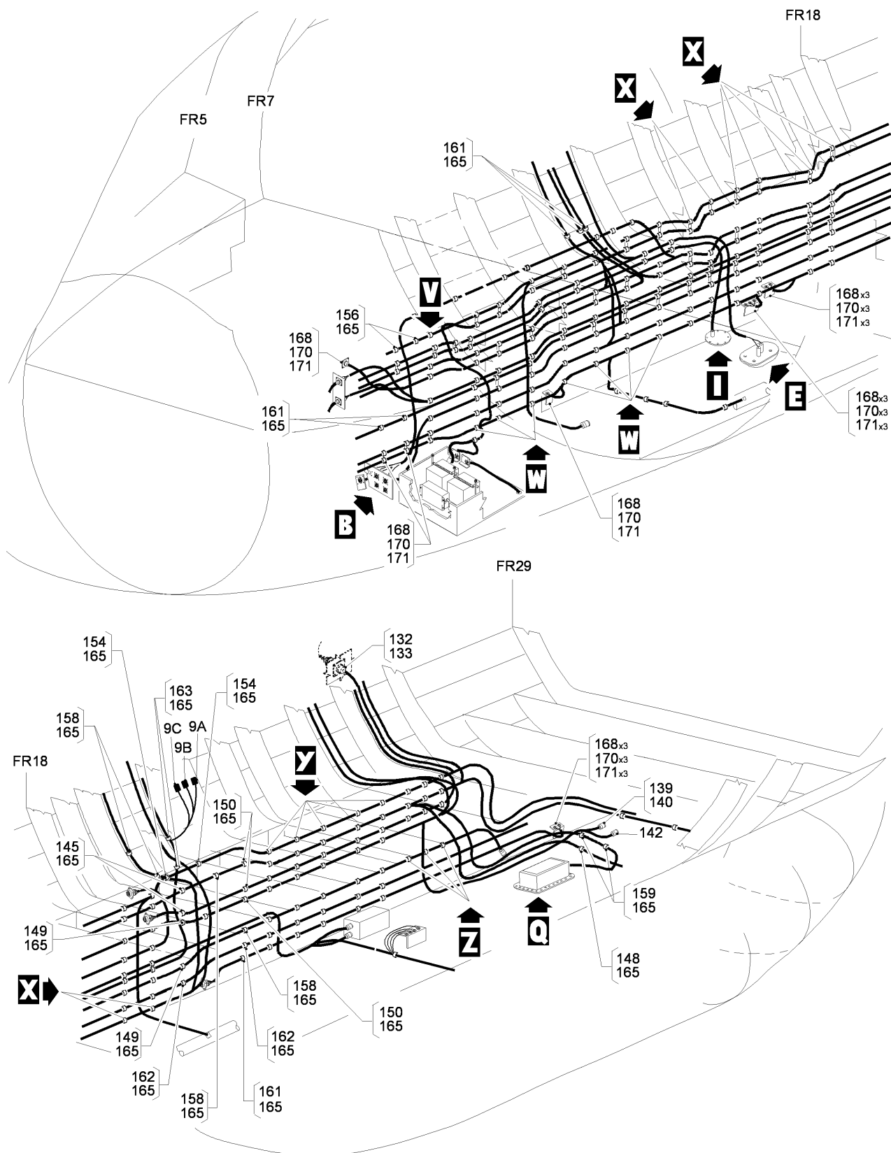
FIG 14 ELECTRICAL AND ELECTRONICS INSTL, Z31BC-31BD-32BA (SHEET 2 OF 11)
