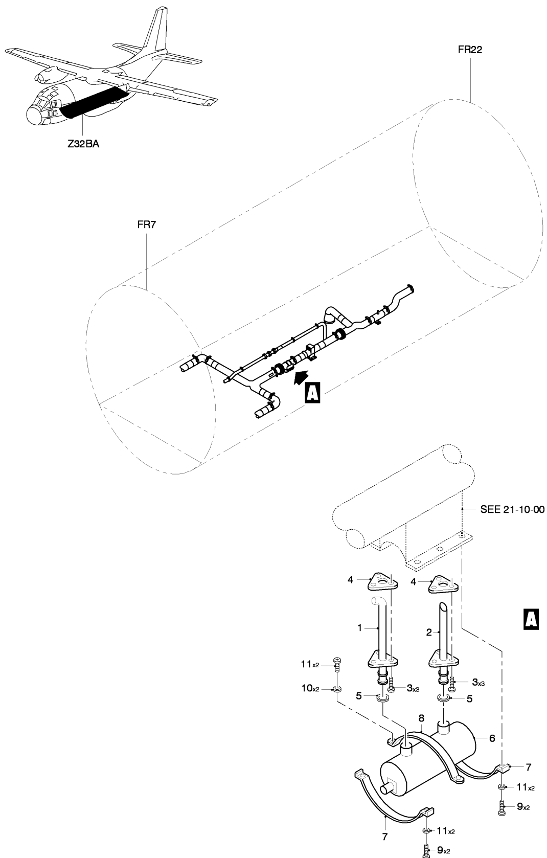
FIG 02 SMOKE DETECTOR INSTL, Z32BA (SHEET 1 OF 1)
