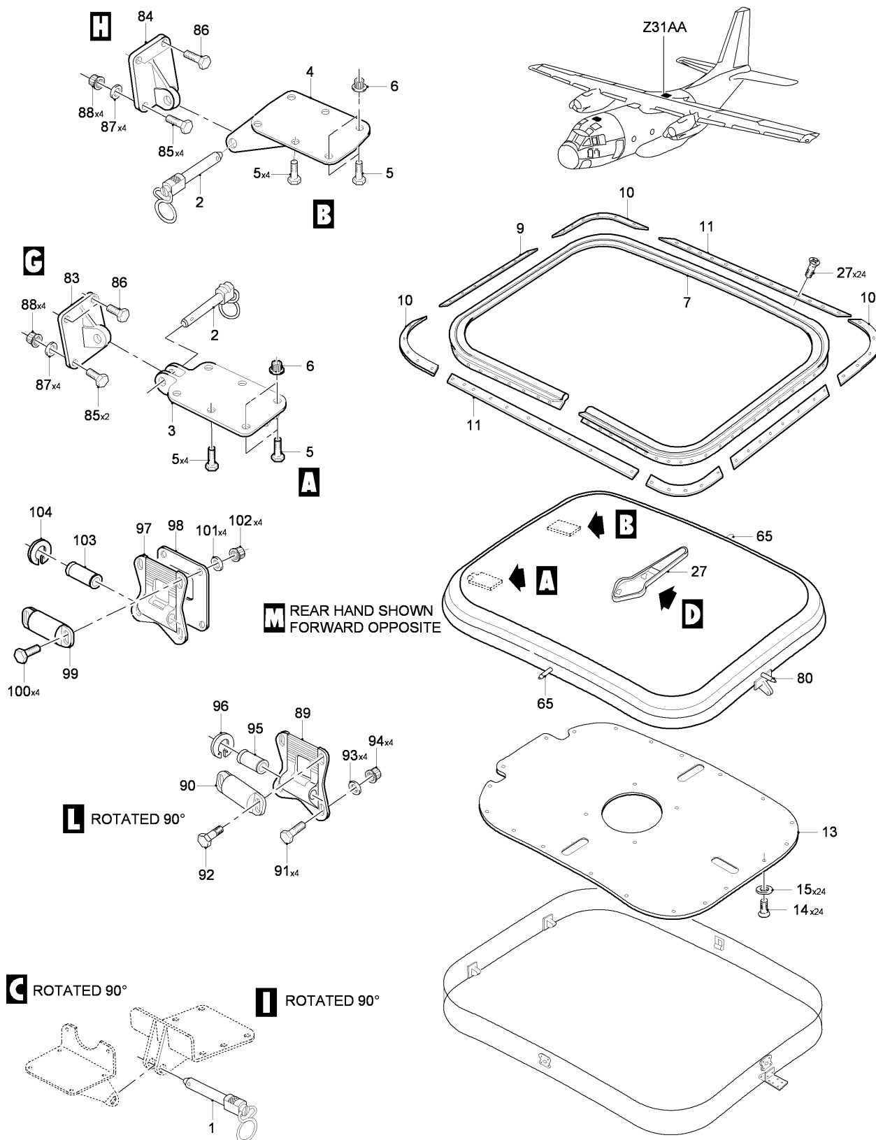
FIG 01 EMERGENCY EXIT DOOR INSTL - TOP FWD, Z31AA (SHEET 1 OF 2)
