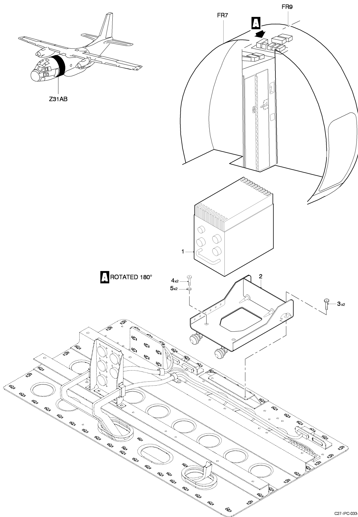
FIG 01 CARGO DIMMER UNIT INSTL, Z31AB (SHEET 1 OF 1)
