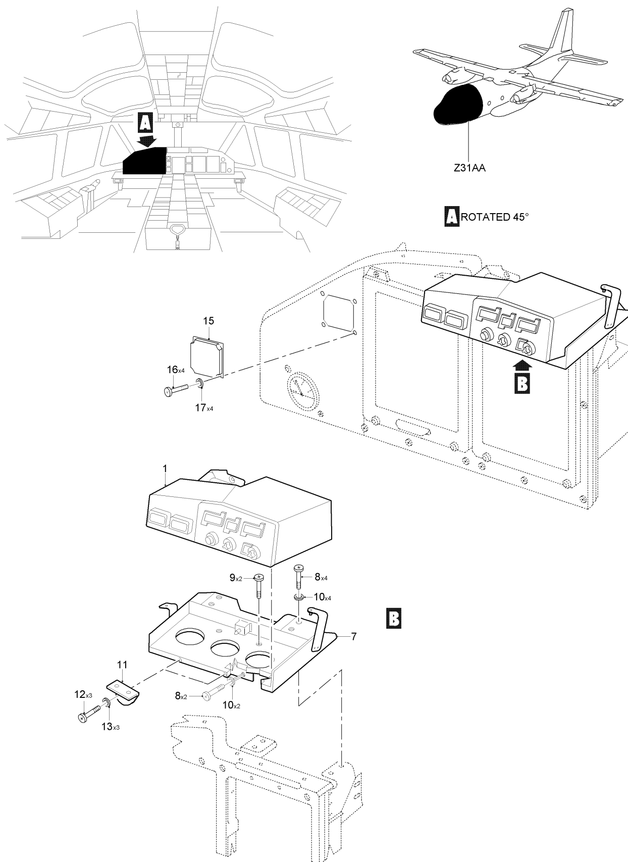
FIG 02 SET/WARNING PANEL PILOT INSTL, Z31AA (SHEET 1 OF 1)
