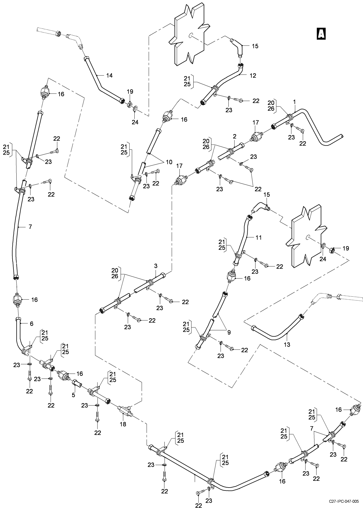
FIG 02 FUEL TANK EXPLOSION PROTECTION SYSTEM INSTL, Z32AB (SHEET 2 OF 2)
