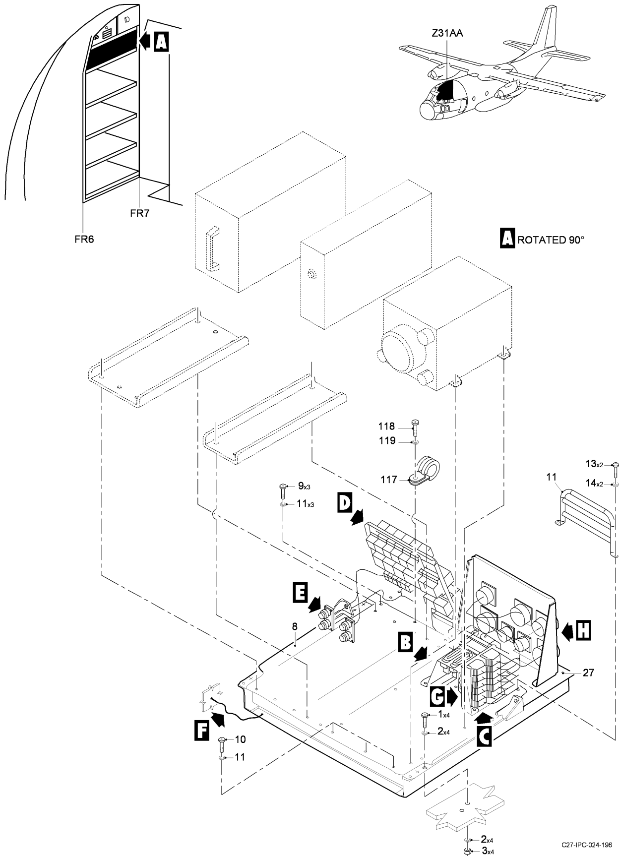
FIG 11 FIFTH AND SIXTH SHELF INSTL - ELECTRICAL COMPARTMENT, Z31AA (SHEET 1 OF 4)
