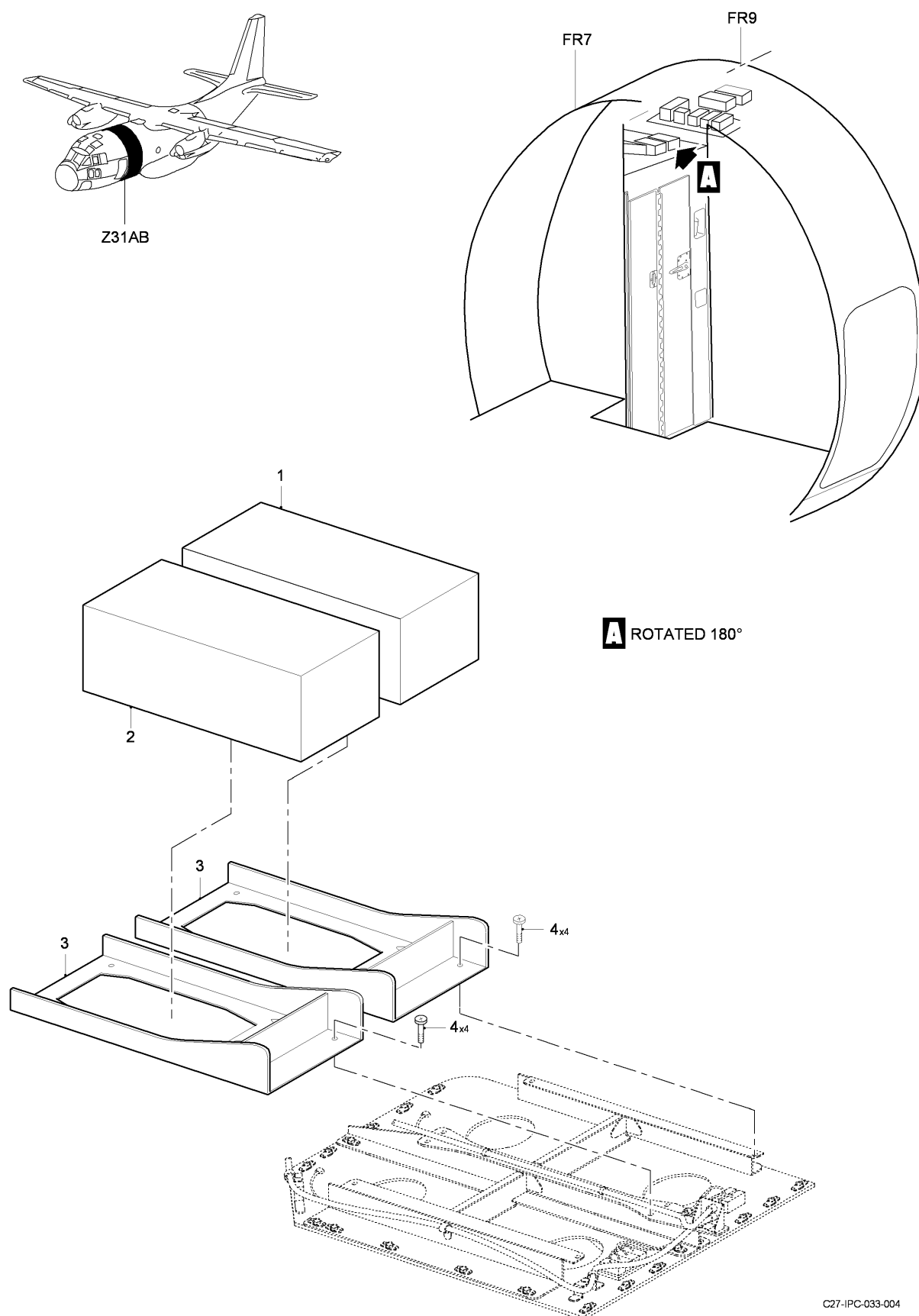
FIG 02 FLIGHT STATION DIMMER UNIT INSTL, Z31AB (SHEET 1 OF 1)
