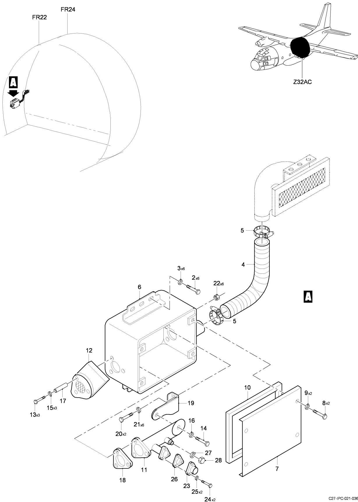
FIG 04 BOX ASSY SENSOR TEMPERATURE INSTL, Z32AC (SHEET 1 OF 1)
