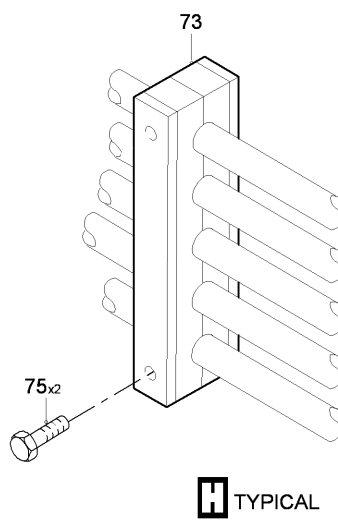
FIG 05 HYDRAULIC PIPING INSTL - CENTER WING, Z33AB, LH-RH (SHEET 3 OF 5)
