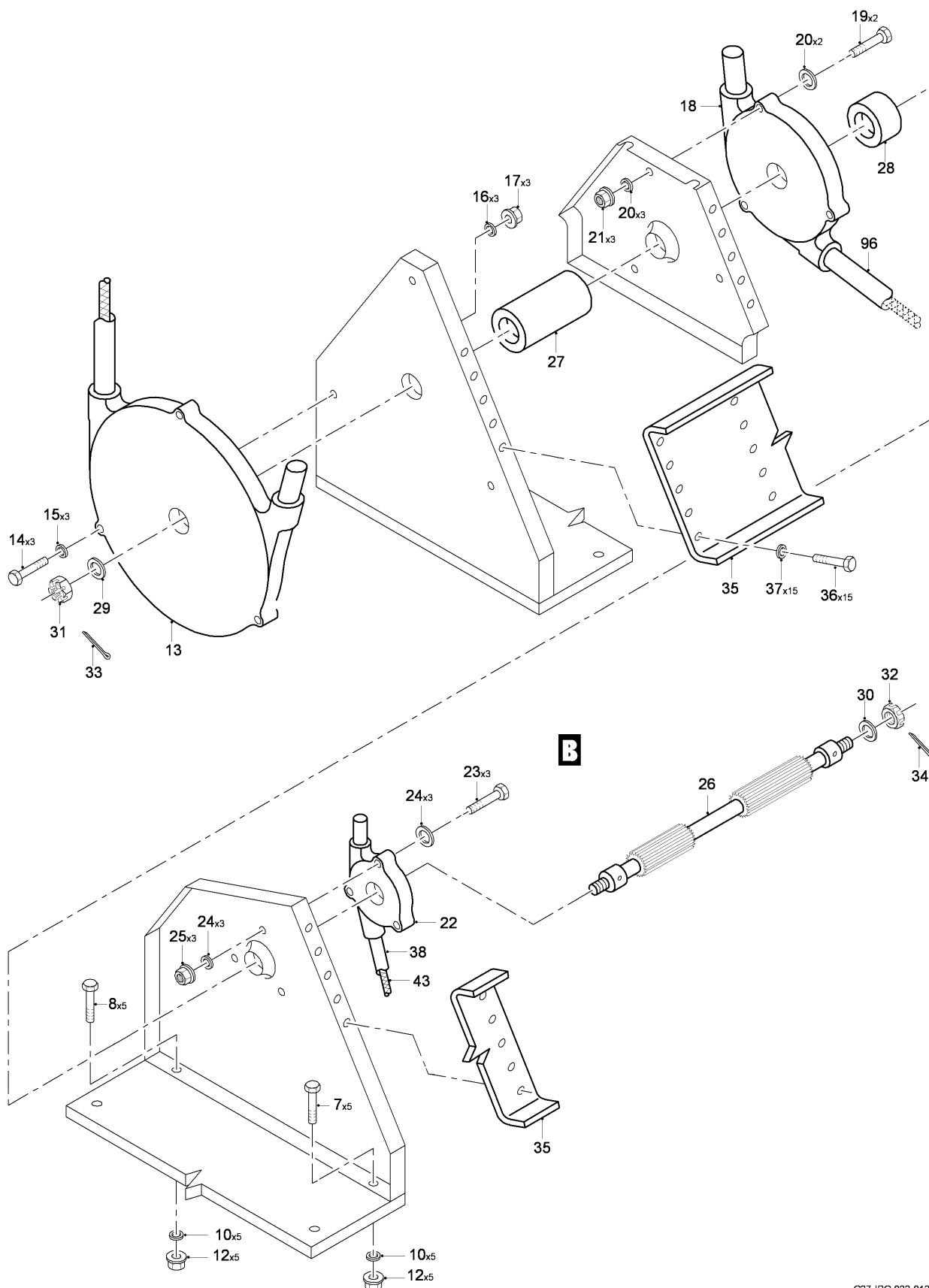
FIG 02 EMERGENCY CONTROL INSTL - MAIN LANDING GEAR, Z31AA (SHEET 2 OF 3)
