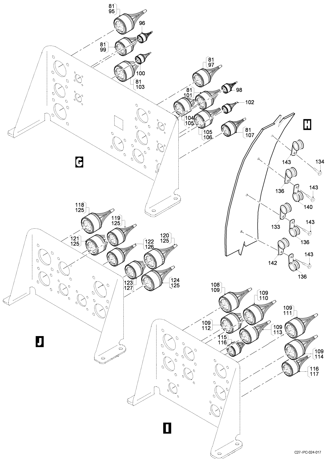
FIG 05 ELECTRICAL AND ELECTRONICS INSTL - CABIN, Z31AA, RH (SHEET 5 OF 5)
