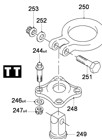
FIG 05 FLOOR CARGO INSTL, Z32BA (SHEET 9 OF 9)
