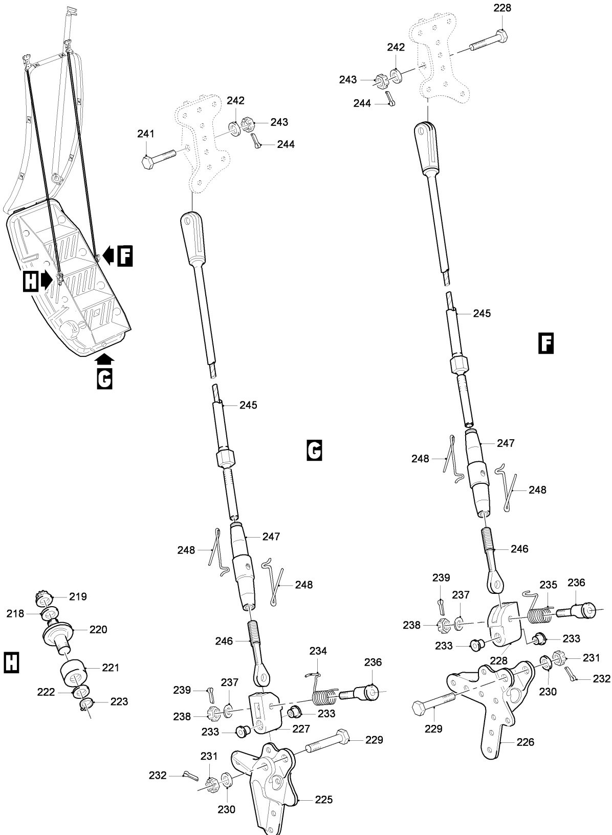
FIG 01 CREW DOOR INSTL, Z31AB (SHEET 5 OF 7)
