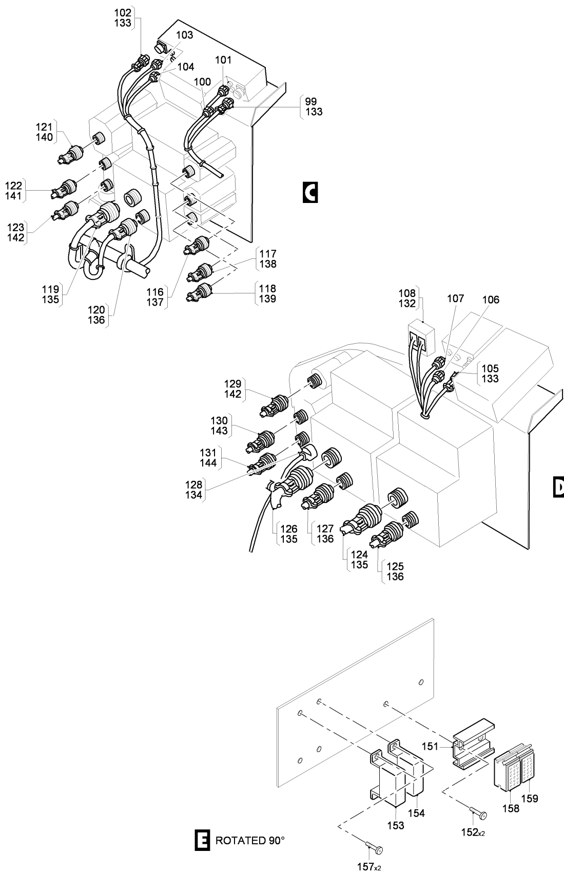
FIG 07 ELECTRICAL AND ELECTRONICS INSTL - CABIN LOWER SIDE, Z31AA (SHEET 3 OF 4)
