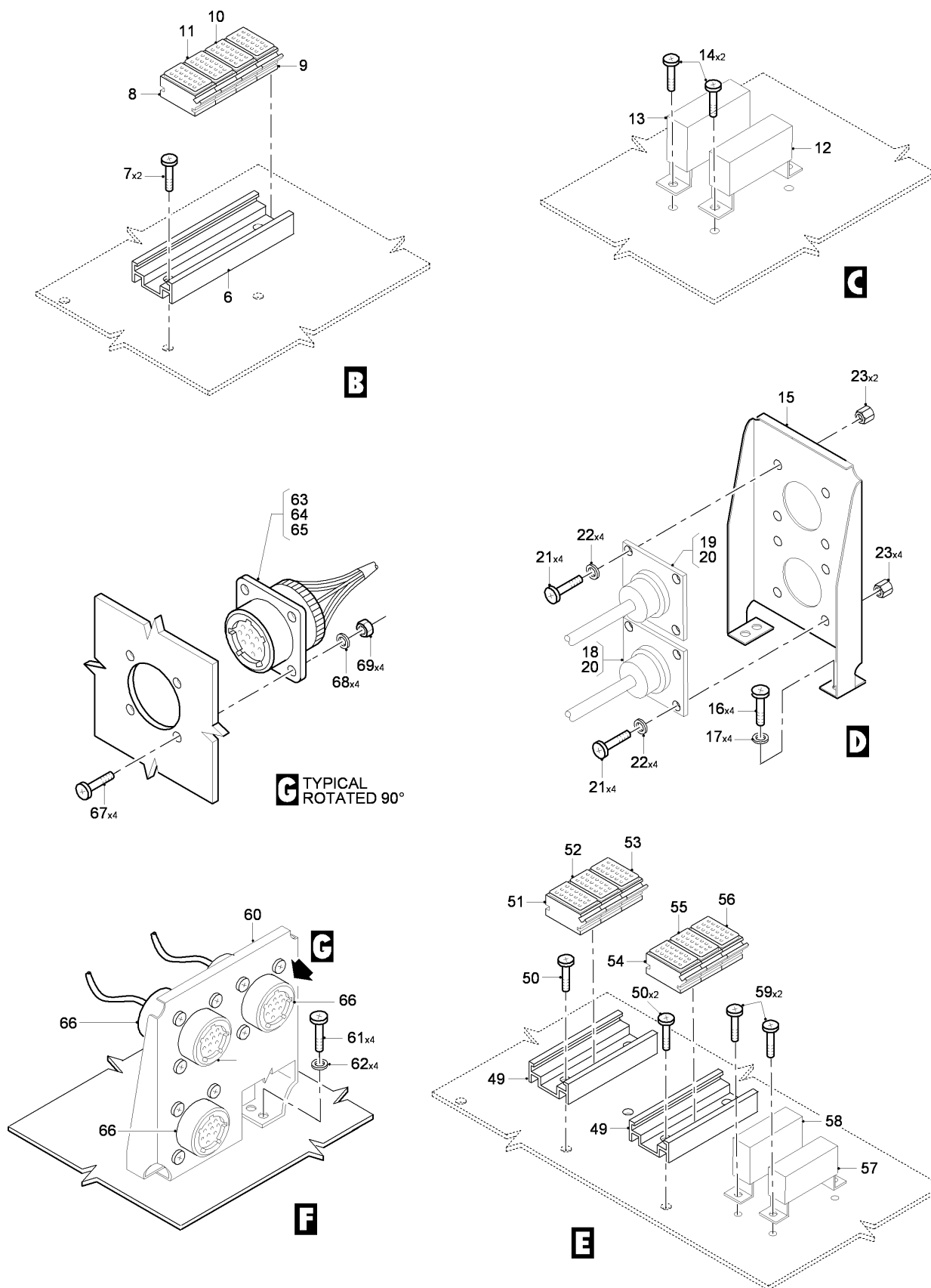
FIG 13 ELECTRONIC INSTL - SHELF FRAME 7 TO 8, Z31AB (SHEET 2 OF 2)
