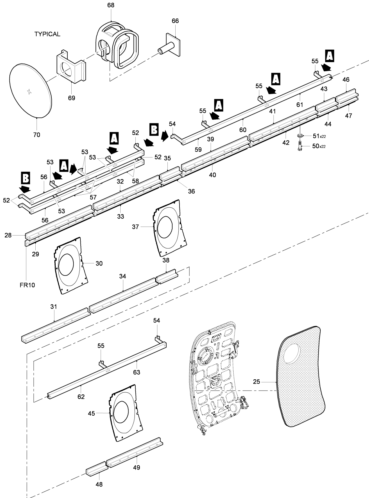
FIG 24 SECONDARY THERMAL INSULATION INSTL, Z32AA-32AB-32AC-32AD (SHEET 2 OF 3)
