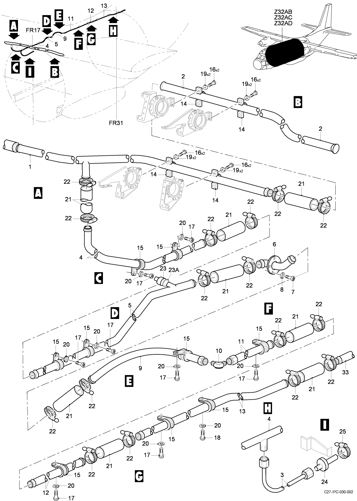
FIG 02 ANTI-ICING INSTL - CENTER FUSELAGE, Z32AB-32AC-32AD (SHEET 1 OF 1)
