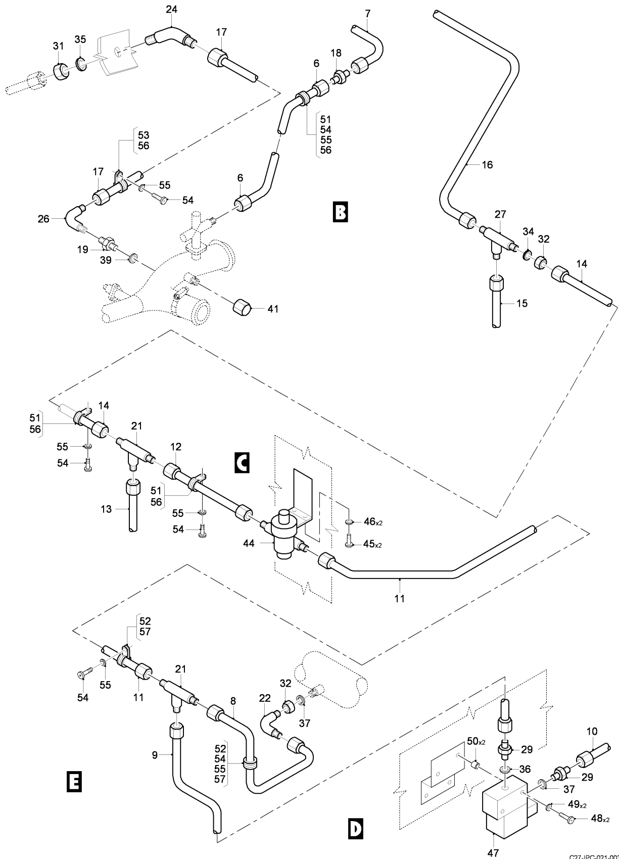
FIG 02 AIR CONDITIONING SENSITIVE LINE INSTL, Z32AA-32AB (SHEET 2 OF 4)
