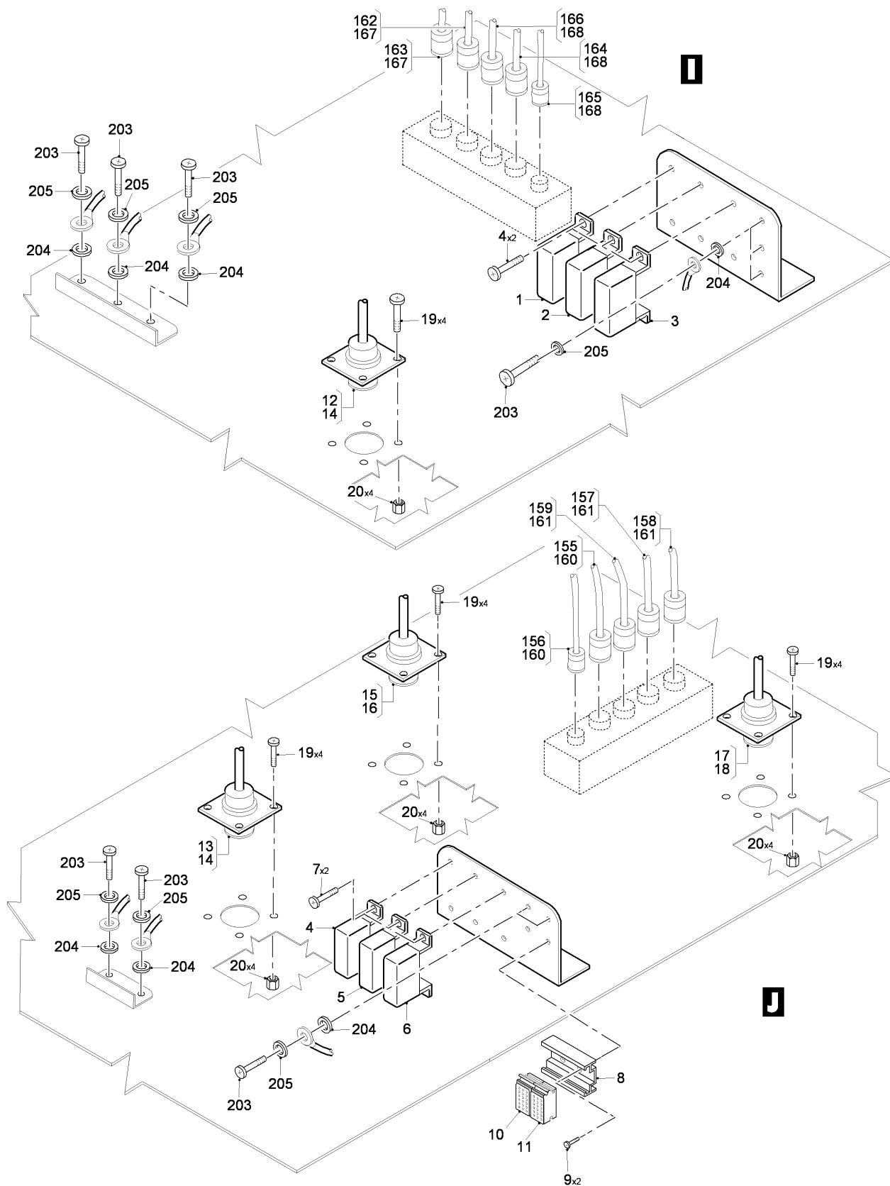
FIG 09 ELECTRICAL AND ELECTRONICS INSTL, Z31AA-31BC, RH (SHEET 4 OF 7)
