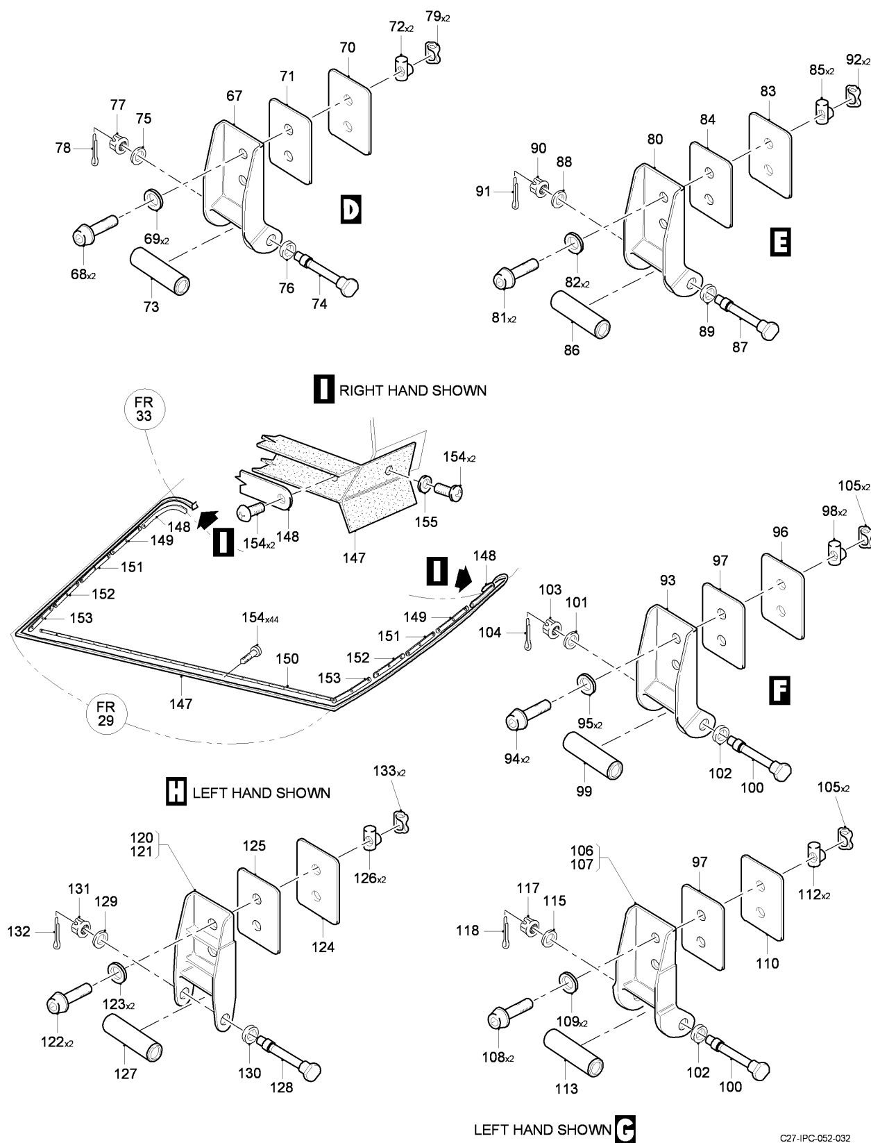
FIG 01 CARGO RAMP INSTL, Z34BA (SHEET 3 OF 3)
