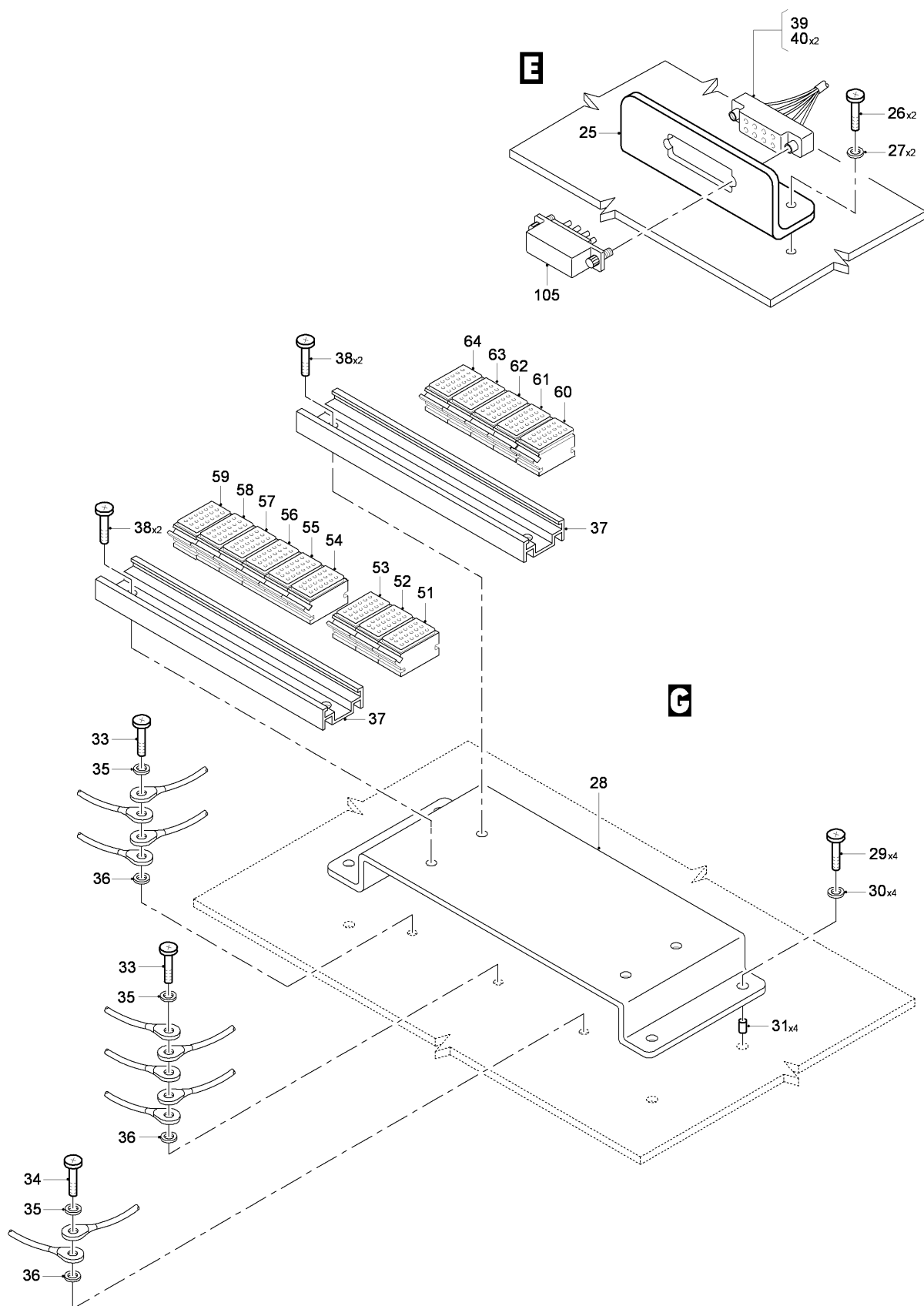
FIG 03 THIRD SHELF INSTL - ELECTRONIC COMPARTMENT, Z31AA (SHEET 2 OF 3)
