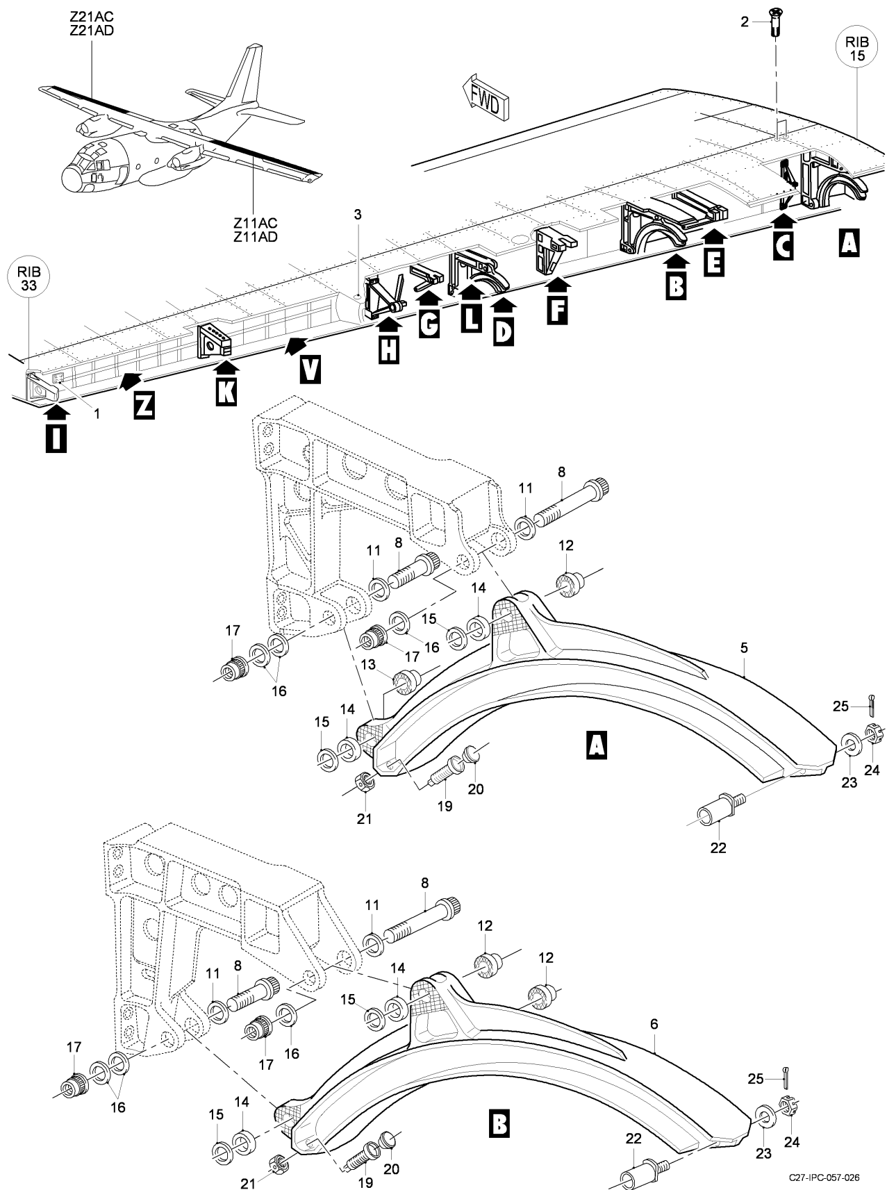
FIG 04 TRAILING EDGE INSTL, Z11AC-11AD-21AC-21AD, LH-RH (SHEET 1 OF 5)
