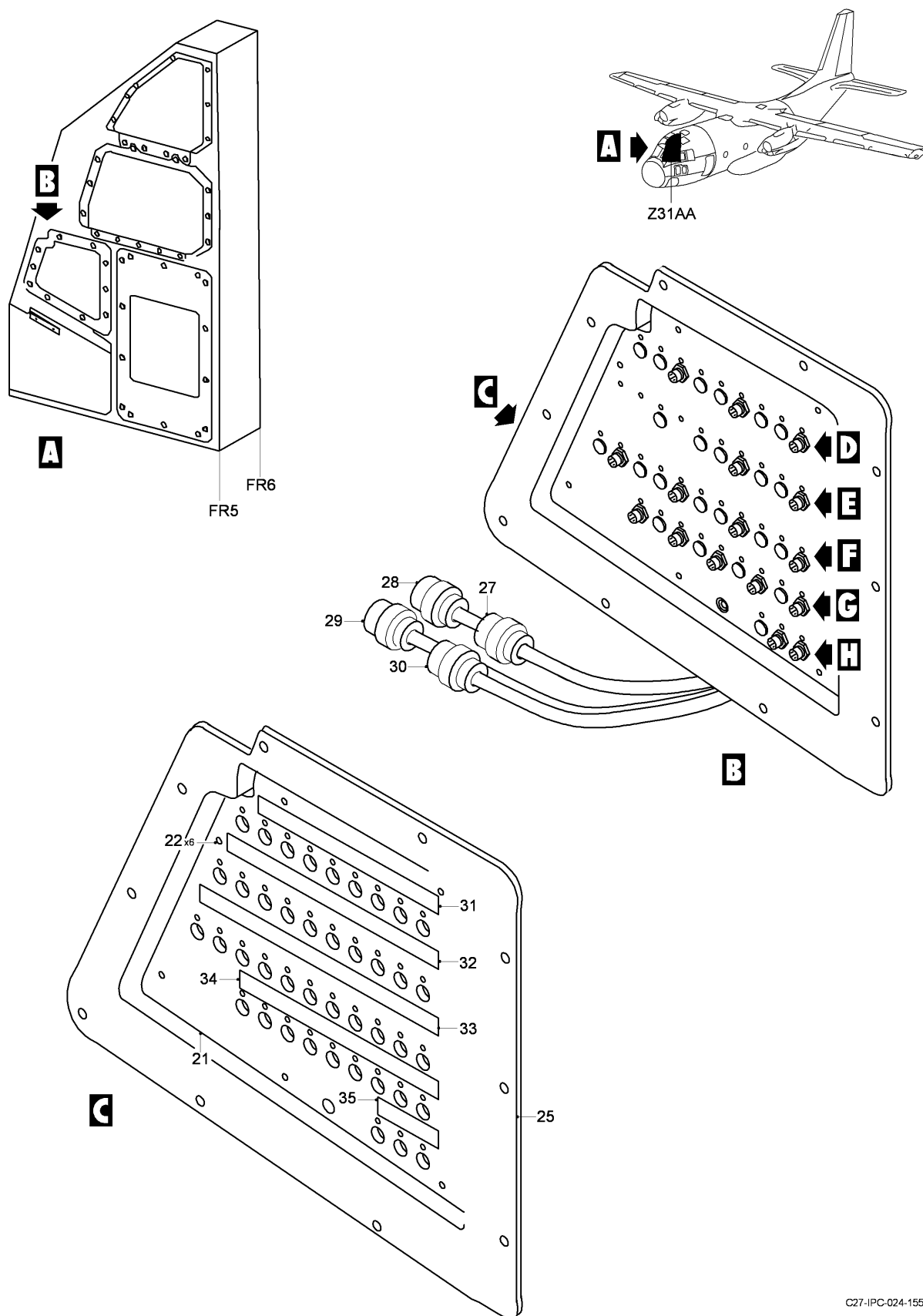
FIG 04 CIRCUIT BREAKER PANEL NO. 3 INSTL, Z31AA (SHEET 1 OF 2)
