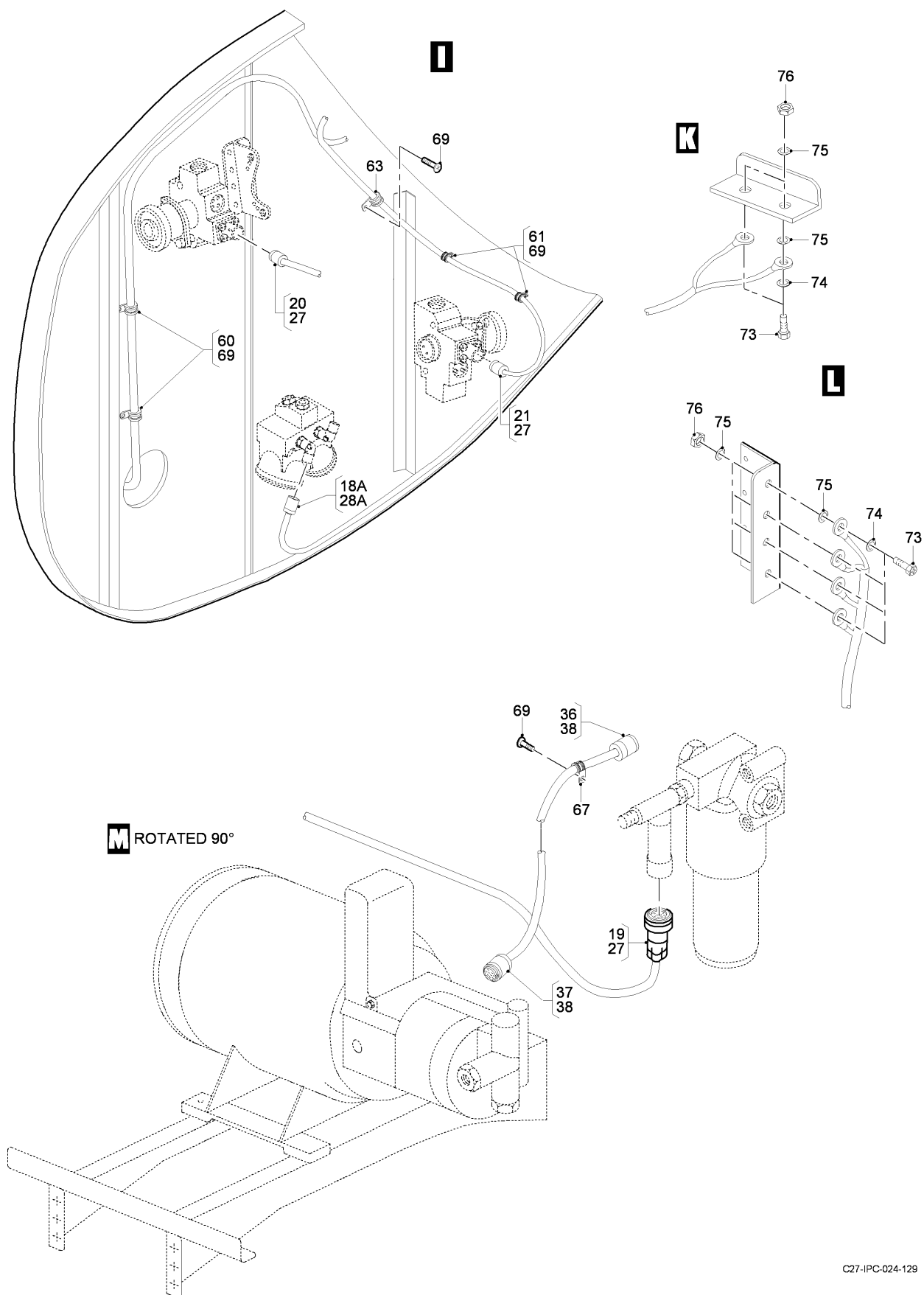
FIG 27 ELECTRICAL AND ELECTRONICS INSTL - MLG, Z23AA-23AB-23AC, RH (SHEET 4 OF 5)
