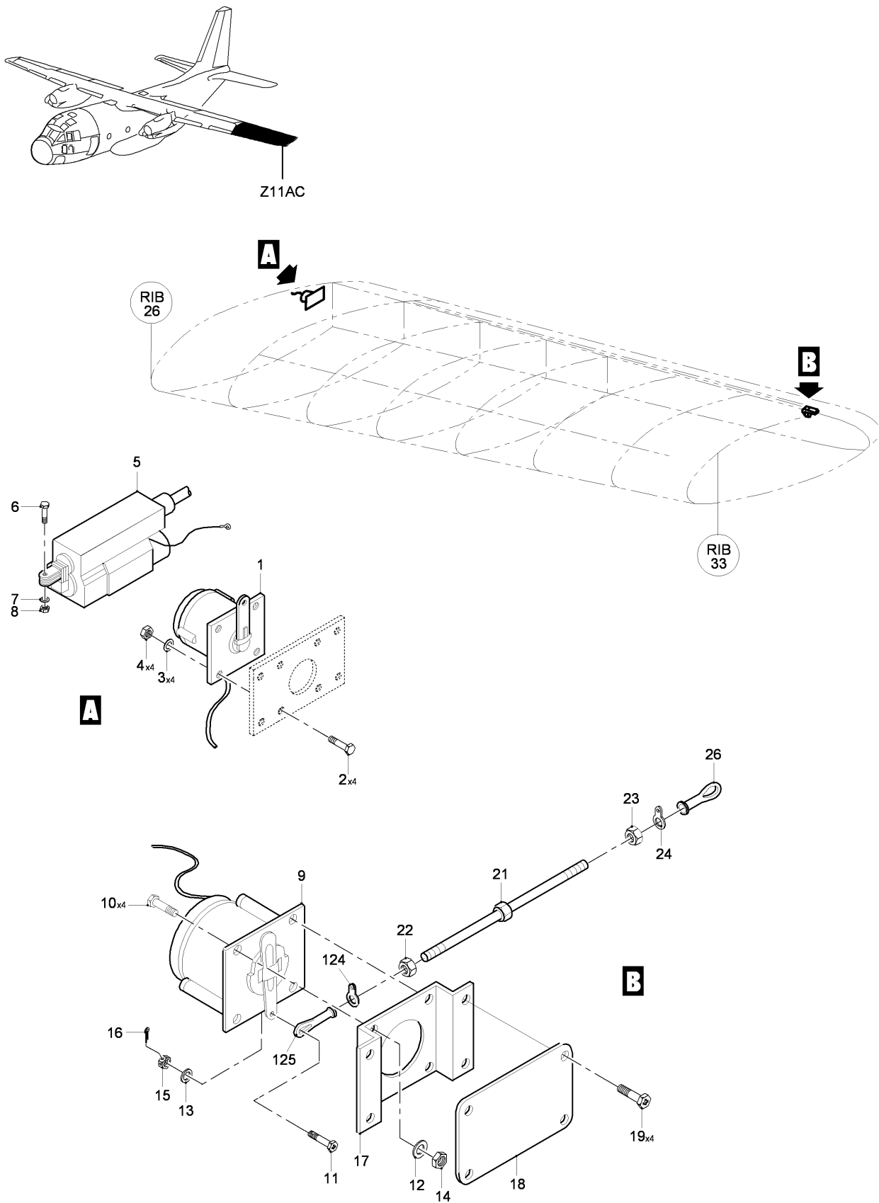
FIG 11 TRANSMITTER TRIM POSITION INSTL - AILERON, Z11AC (SHEET 1 OF 1)
