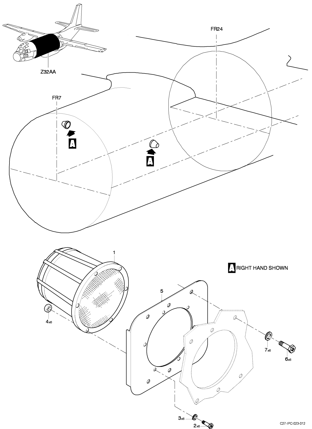
FIG 01 LOUDSPEAKER INSTL, Z32AA, LH-RH (SHEET 1 OF 1)
