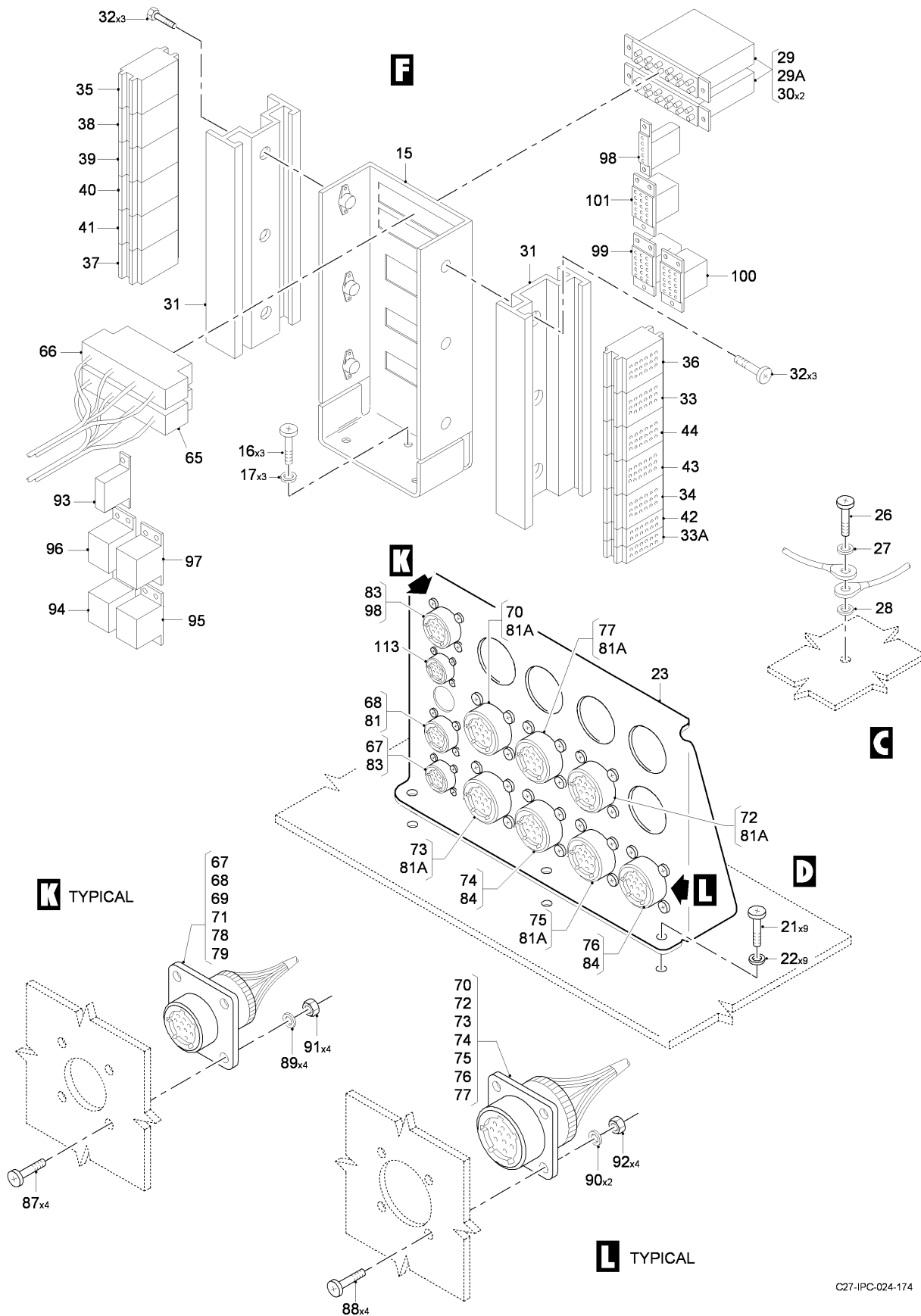
FIG 05 FIFTH SHELF INSTL - ELECTRONIC COMPARTMENT, Z31AA (SHEET 2 OF 3)
