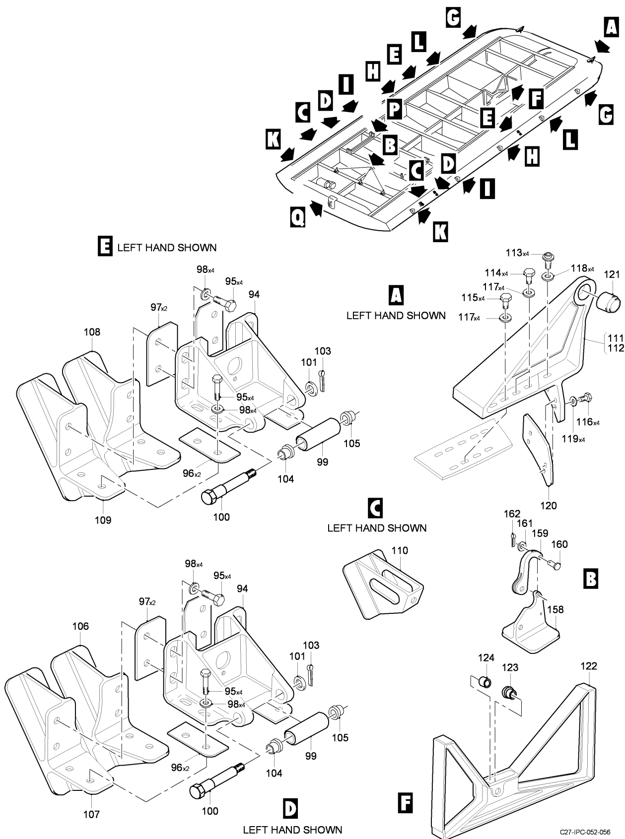
FIG 12 CARGO DOOR ASSY (SHEET 1 OF 4)
