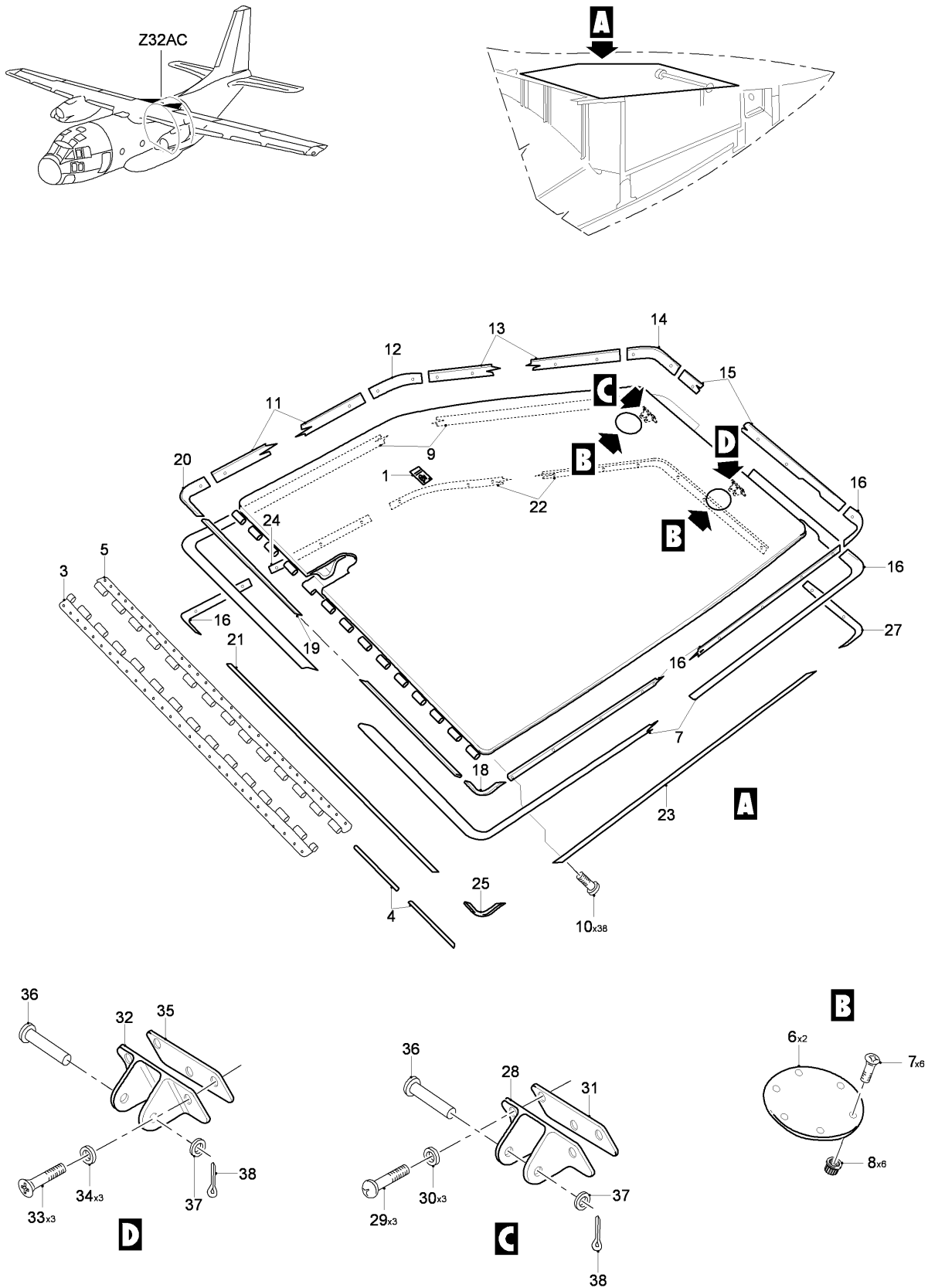
FIG 04 LIFE RAFT DOOR INSTL, Z32AC, LH-RH (SHEET 1 OF 1)
