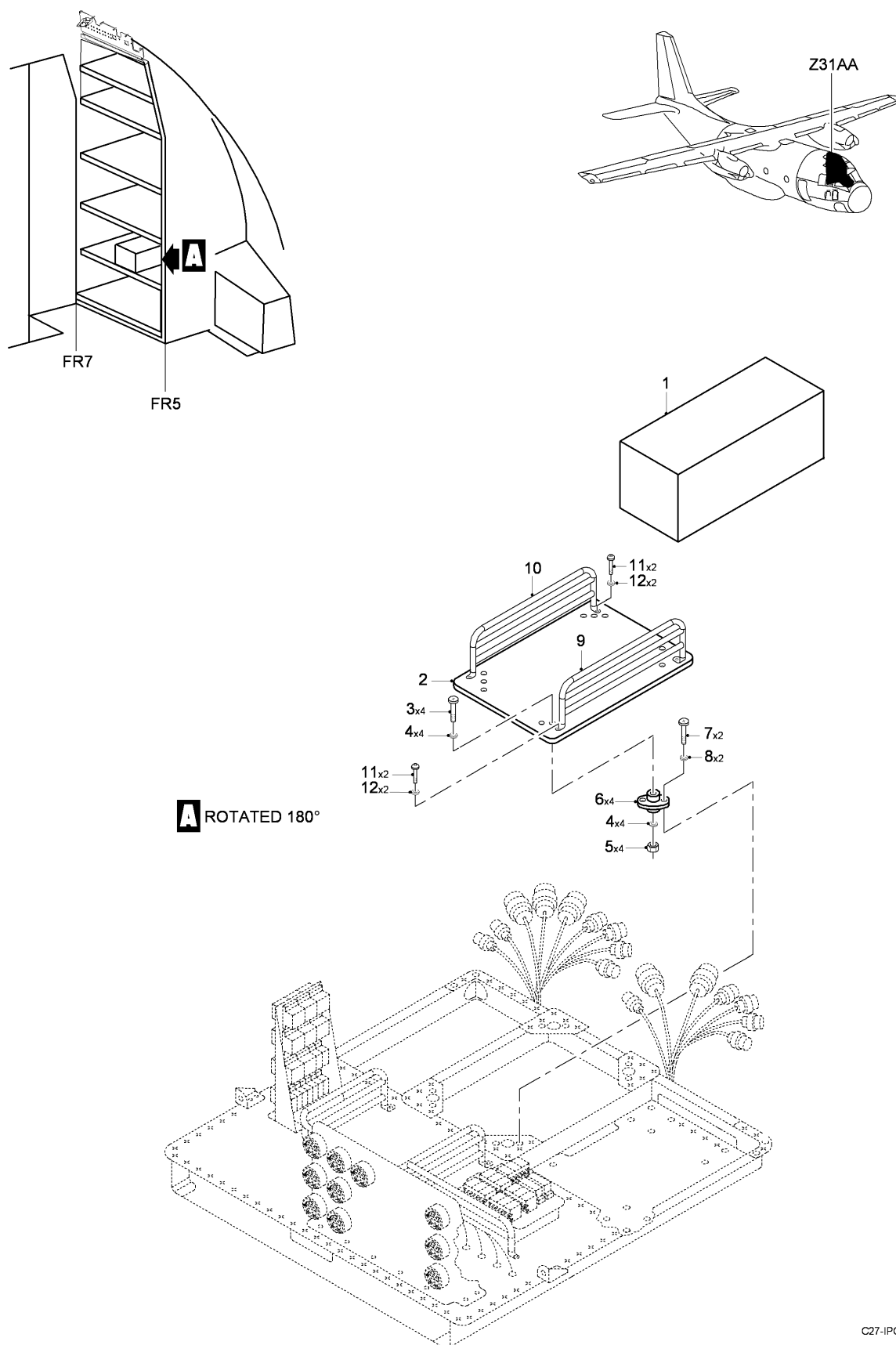
FIG 02 CNI SIGNAL PROCESSOR NO. 1 INSTL, Z31AA (SHEET 1 OF 1)
