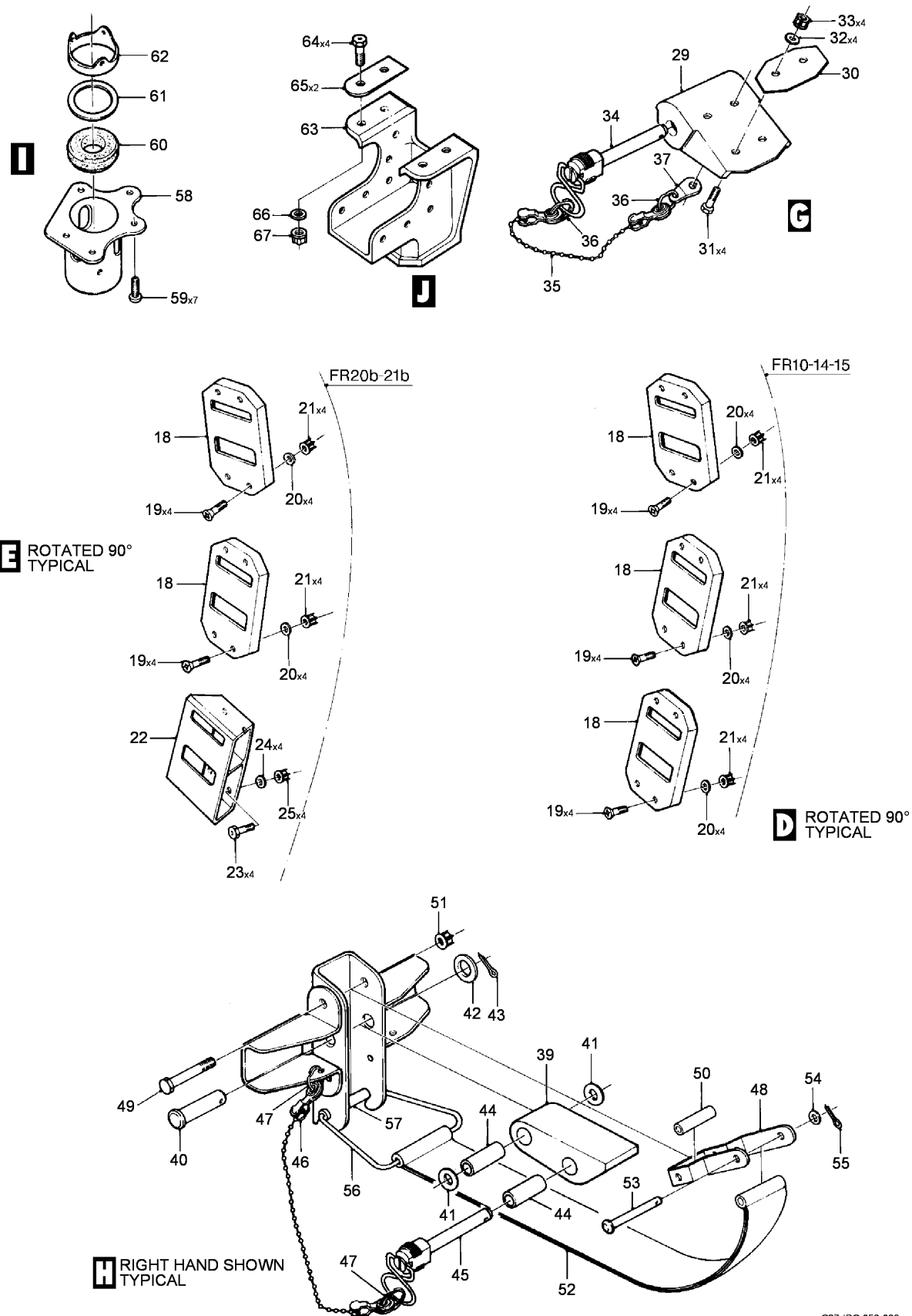
FIG 03 STRUCTURE INSTL, Z32AA-32AB-32AC-32AD (SHEET 2 OF 2)
