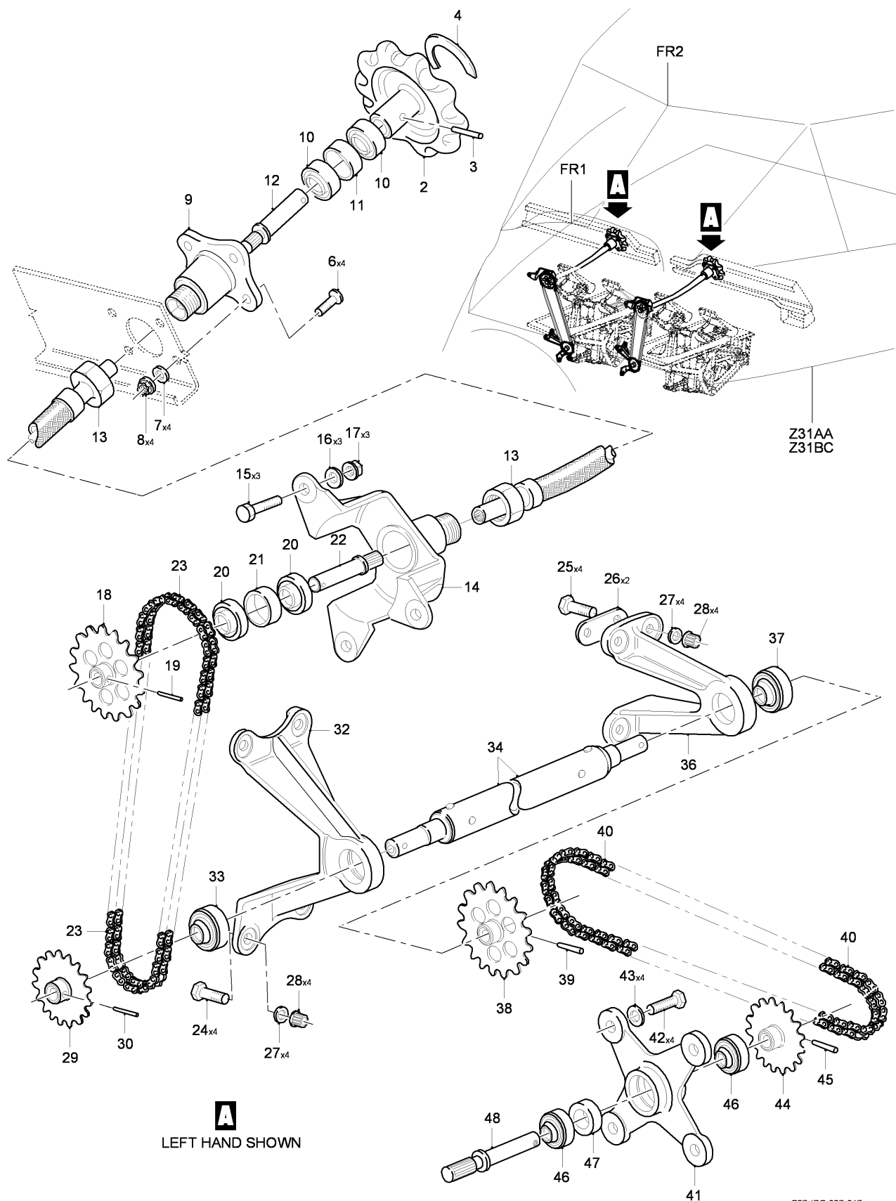
FIG 01 RUDDER PEDAL ADJUSTMENT CONTROLS INSTL, Z31AA-31BC, LH-RH (SHEET 1 OF 1)
