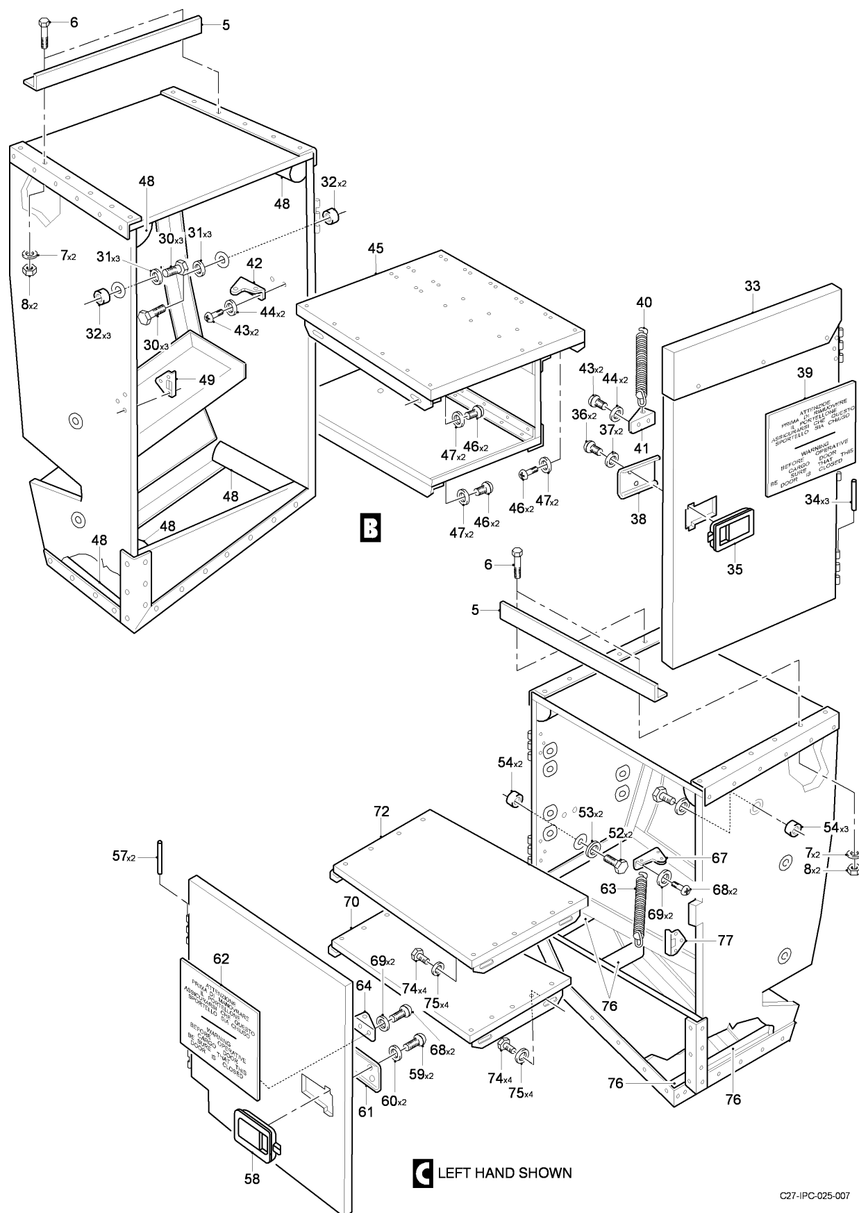
FIG 03 STORAGE CABINETS INSTL, Z34AA, LH-RH (SHEET 2 OF 2)
