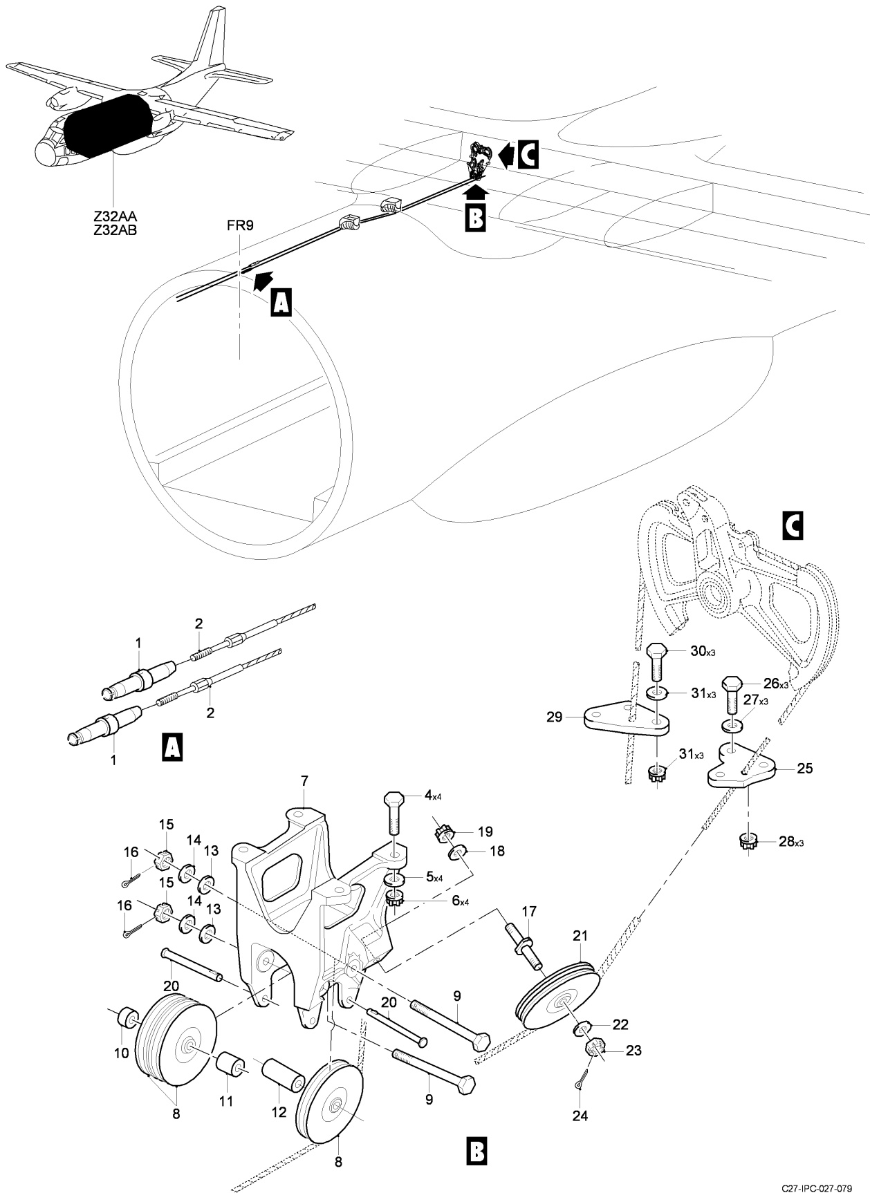
FIG 04 FLAP CONTROLS INSTL, Z32AA-32AB (SHEET 1 OF 1)
