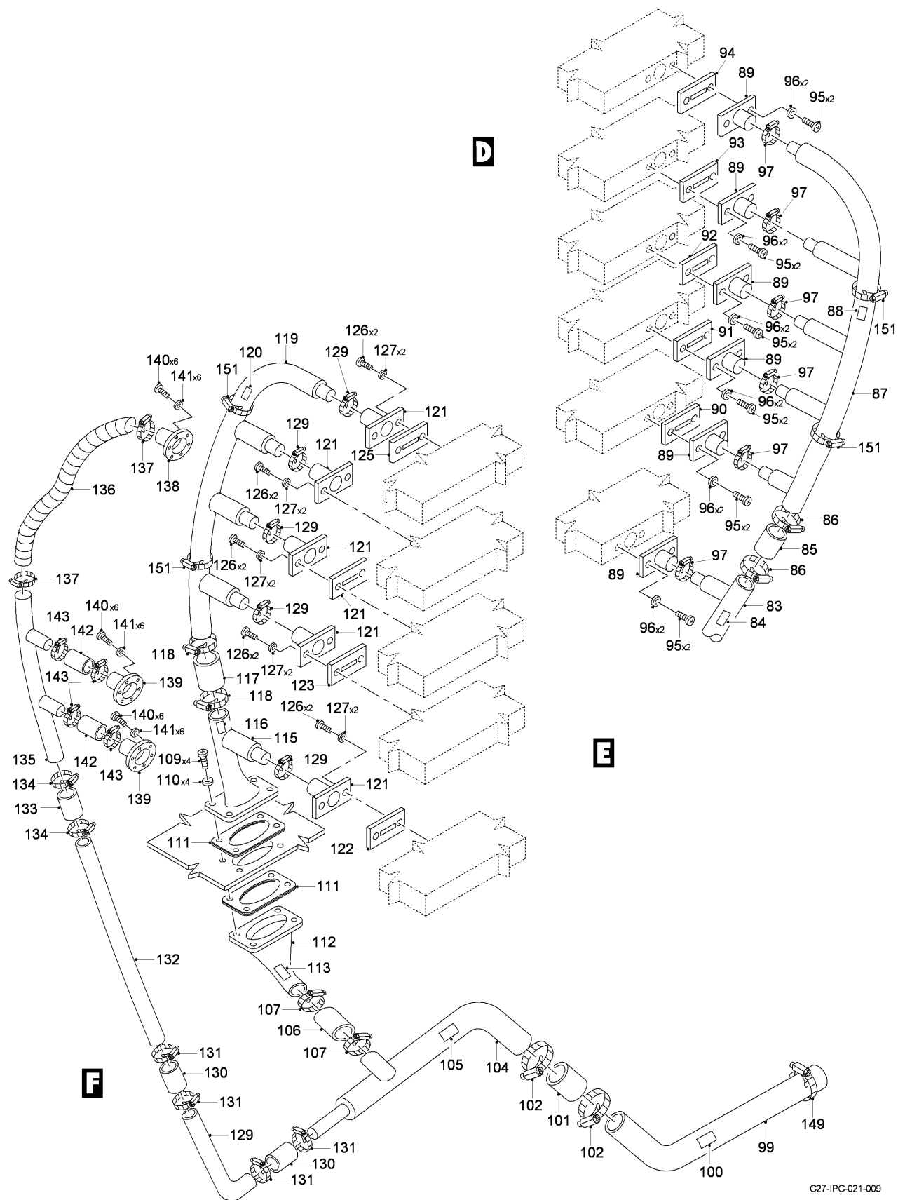
FIG 02 VENTILATION INSTL - FWD FUSELAGE, Z31AA-31AB (SHEET 3 OF 3)
