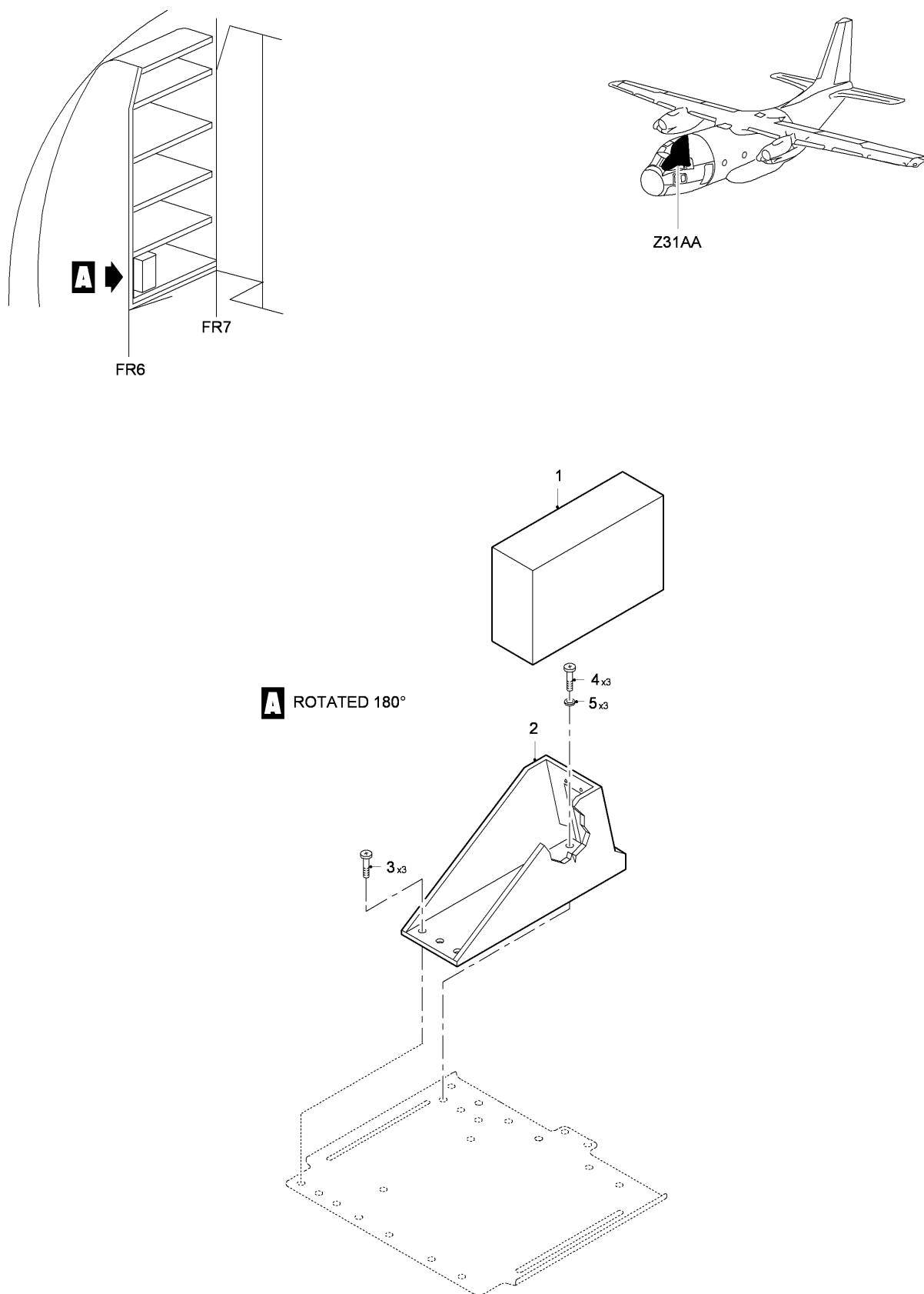
FIG 05 BUS ADAPTER UNIT INSTL - ELECTRICAL COMPARTMENT, Z31AA (SHEET 1 OF 1)
