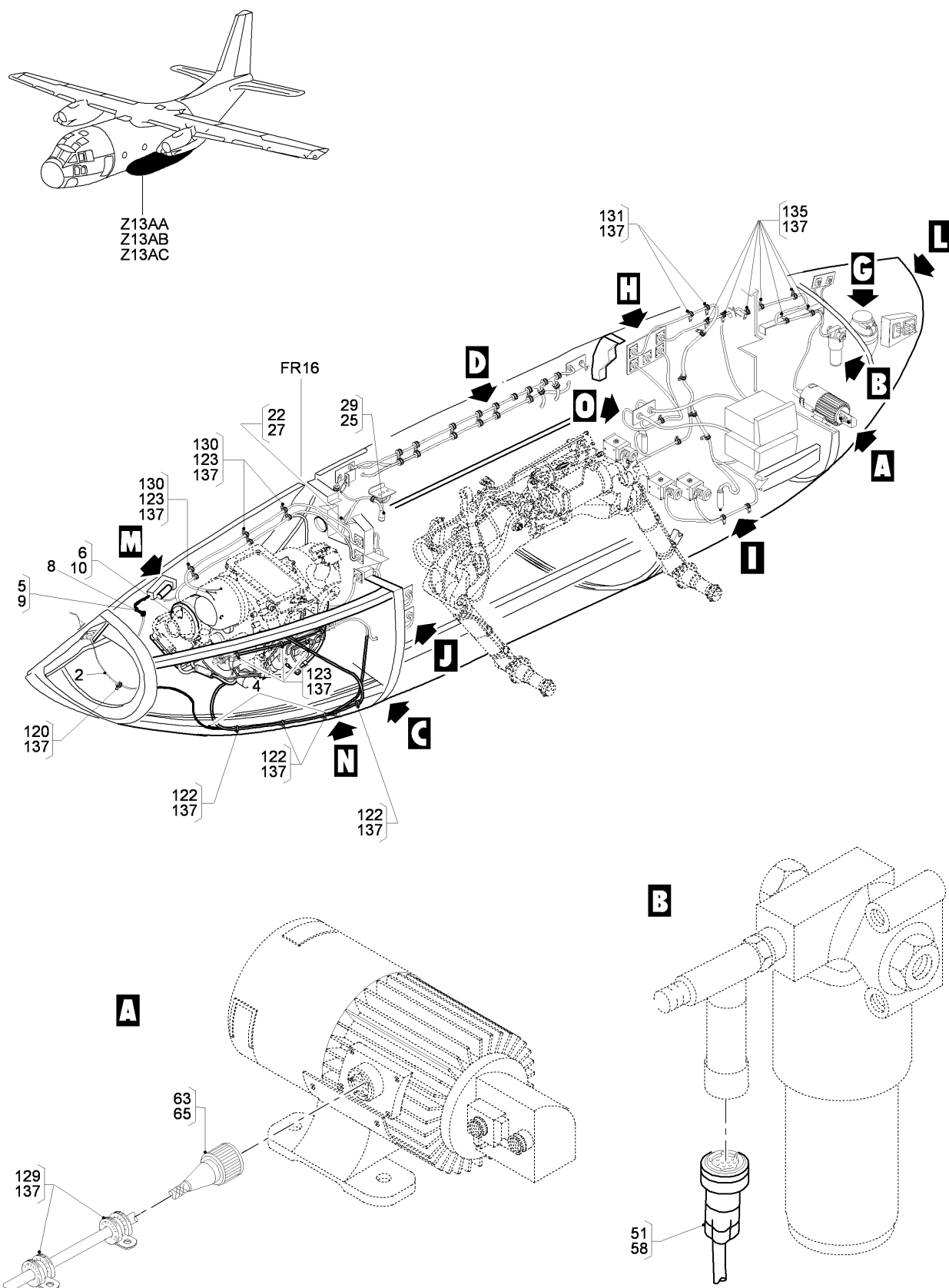
FIG 26 ELECTRICAL AND ELECTRONICS INSTL - MLG, Z13AA-13AB-13AC, LH (SHEET 1 OF 5)
