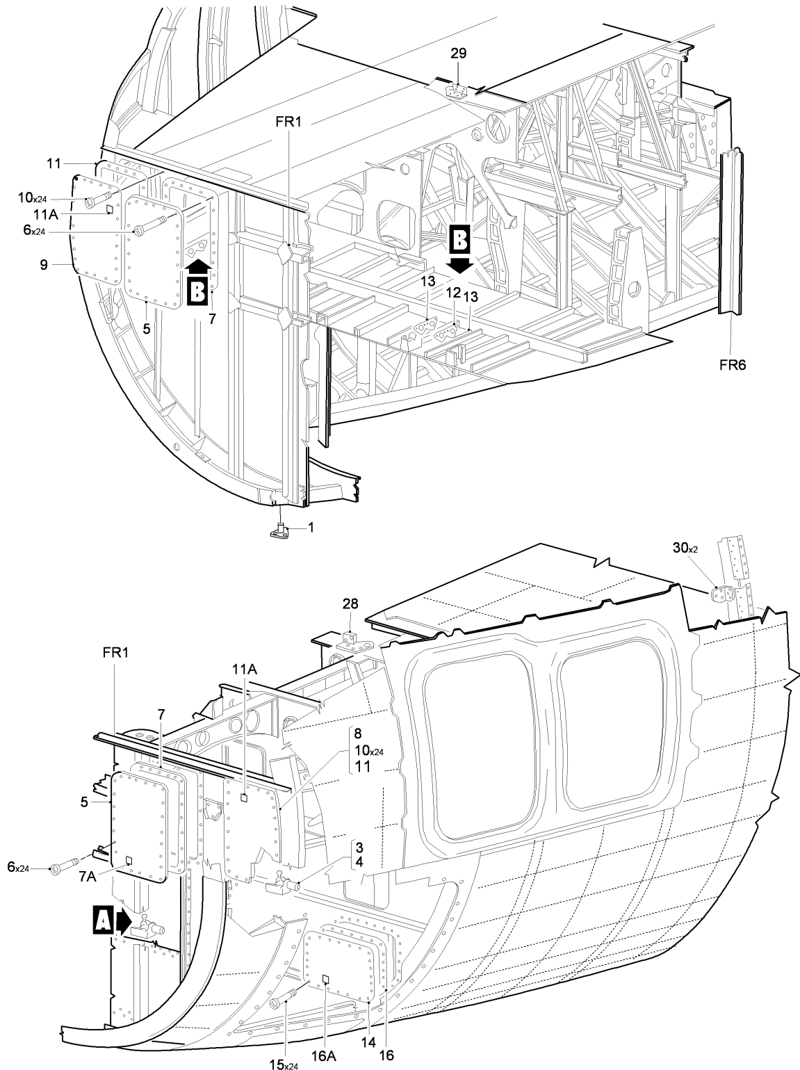
FIG 09 STRUCTURE INSTL, Z31AA (SHEET 1 OF 3)
