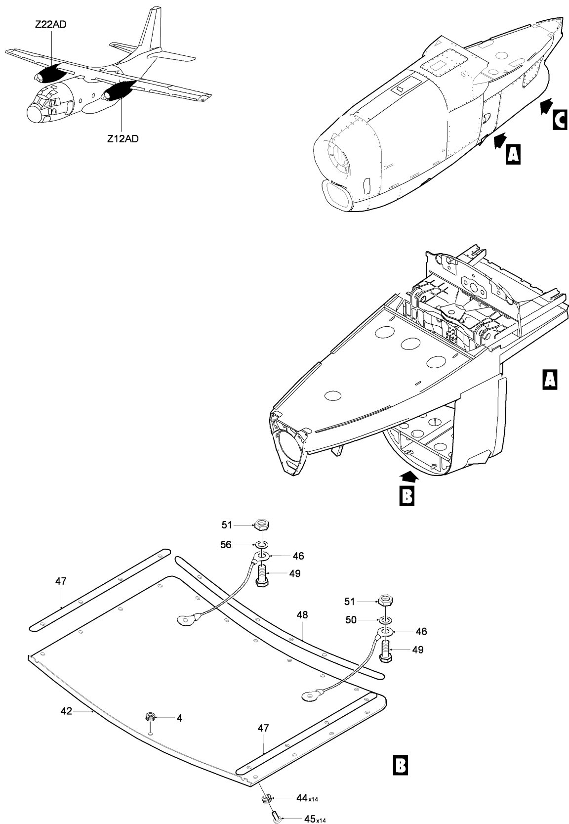
FIG 03 FAIRING LOWER INSTL - NACELLE ENGINE, Z12AD-22AD (SHEET 1 OF 2)
