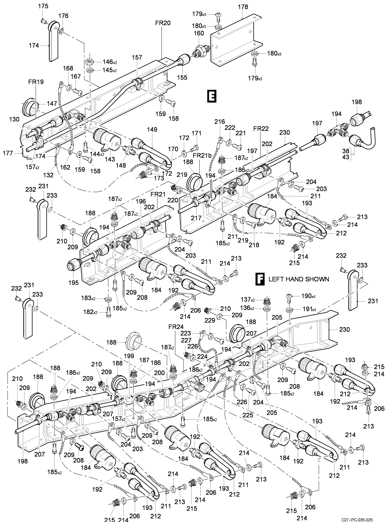
FIG 03 OXYGEN INSTL - CENTER FUSELAGE, Z32AA-32AB-32AC-32AD (SHEET 4 OF 5)
