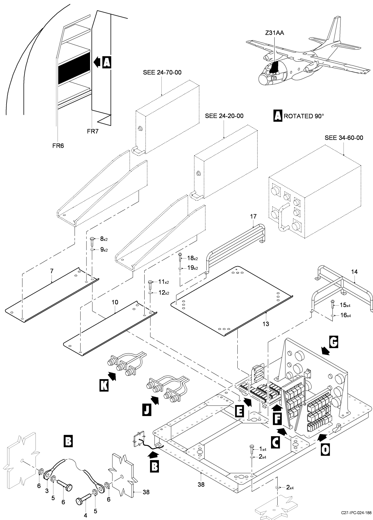
FIG 09 THIRD SHELF INSTL - ELECTRICAL COMPARTMENT, Z31AA (SHEET 1 OF 4)
