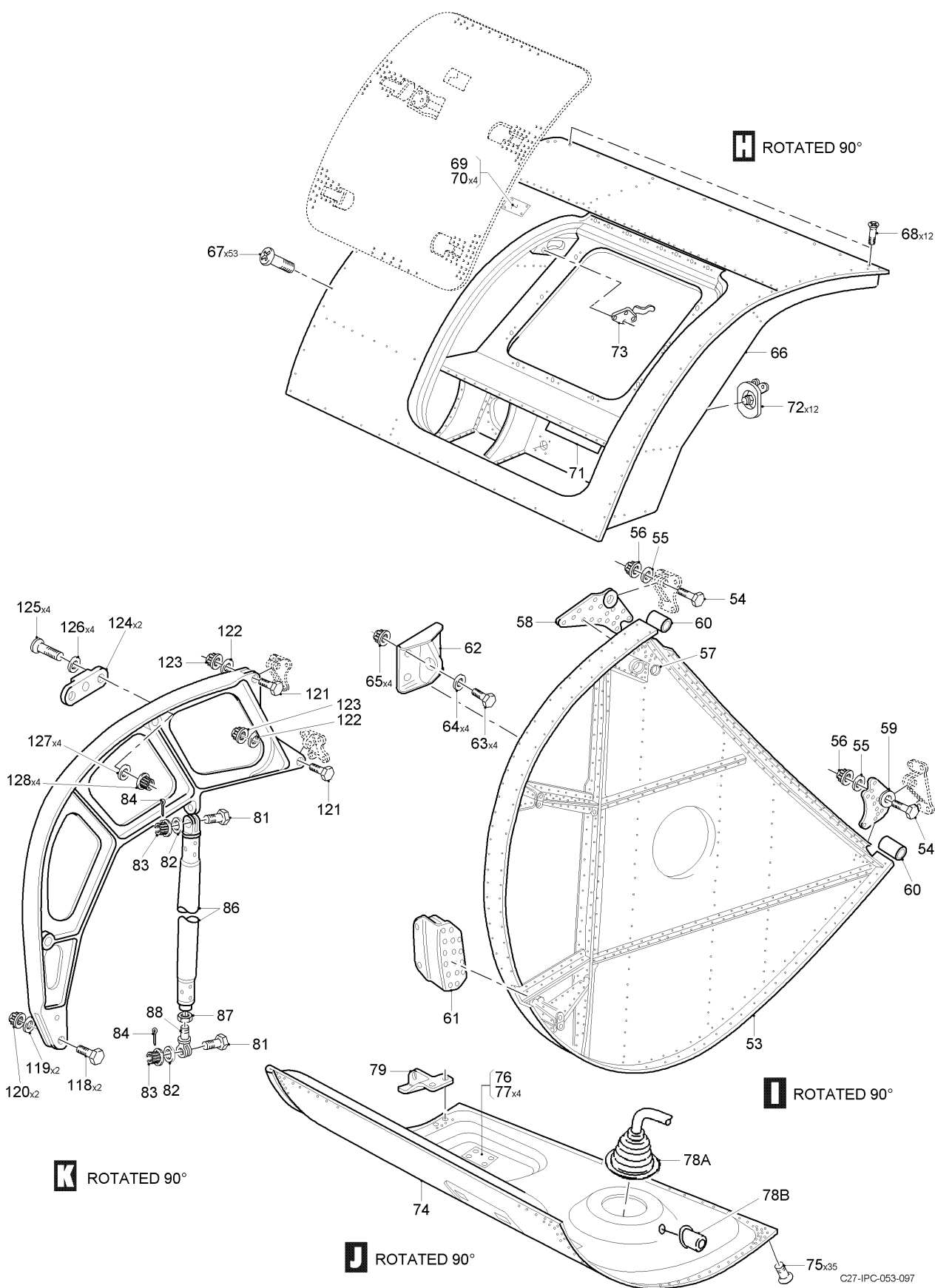
FIG 02 STRUCTURE INSTL - MLG, Z23AA-23AB, RH (SHEET 3 OF 4)
