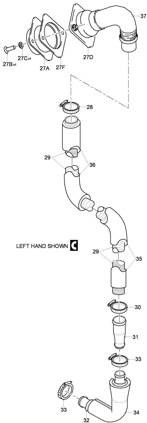
FIG 05 AIR DISTRUBTION INSTL, Z32AA-32AB-32AC-32AD (SHEET 2 OF 4)
