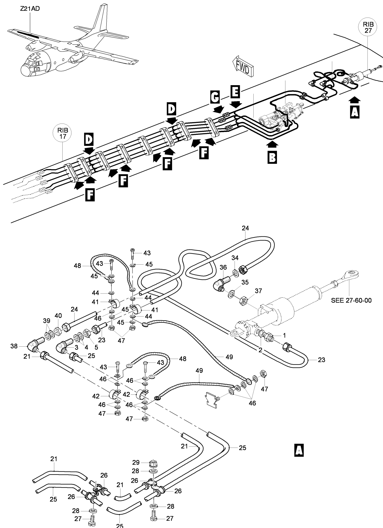
FIG 05 HYDRAULIC PIPING INSTL - SPOILER CONTROL, Z21AD, RH (SHEET 1 OF 3)
