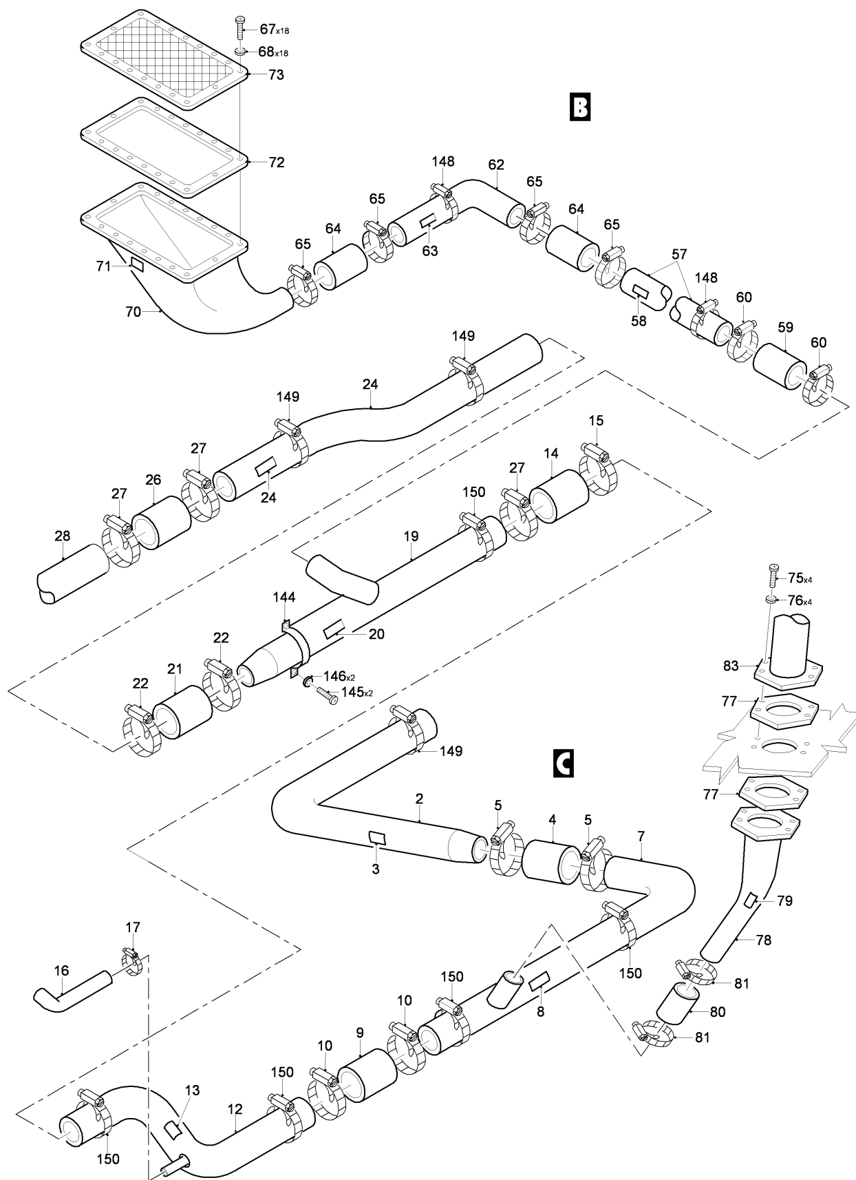
FIG 02 VENTILATION INSTL - FWD FUSELAGE, Z31AA-31AB (SHEET 2 OF 3)
