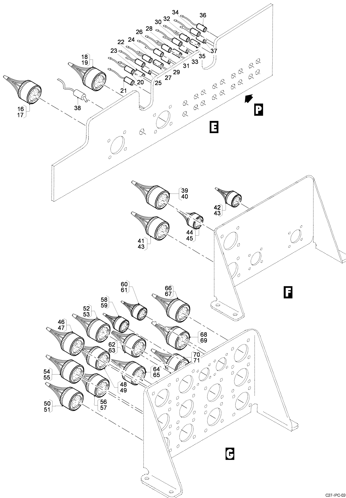
FIG 04 ELECTRICAL AND ELECTRONICS INSTL - CABIN, Z31AA, LH (SHEET 3 OF 5)
