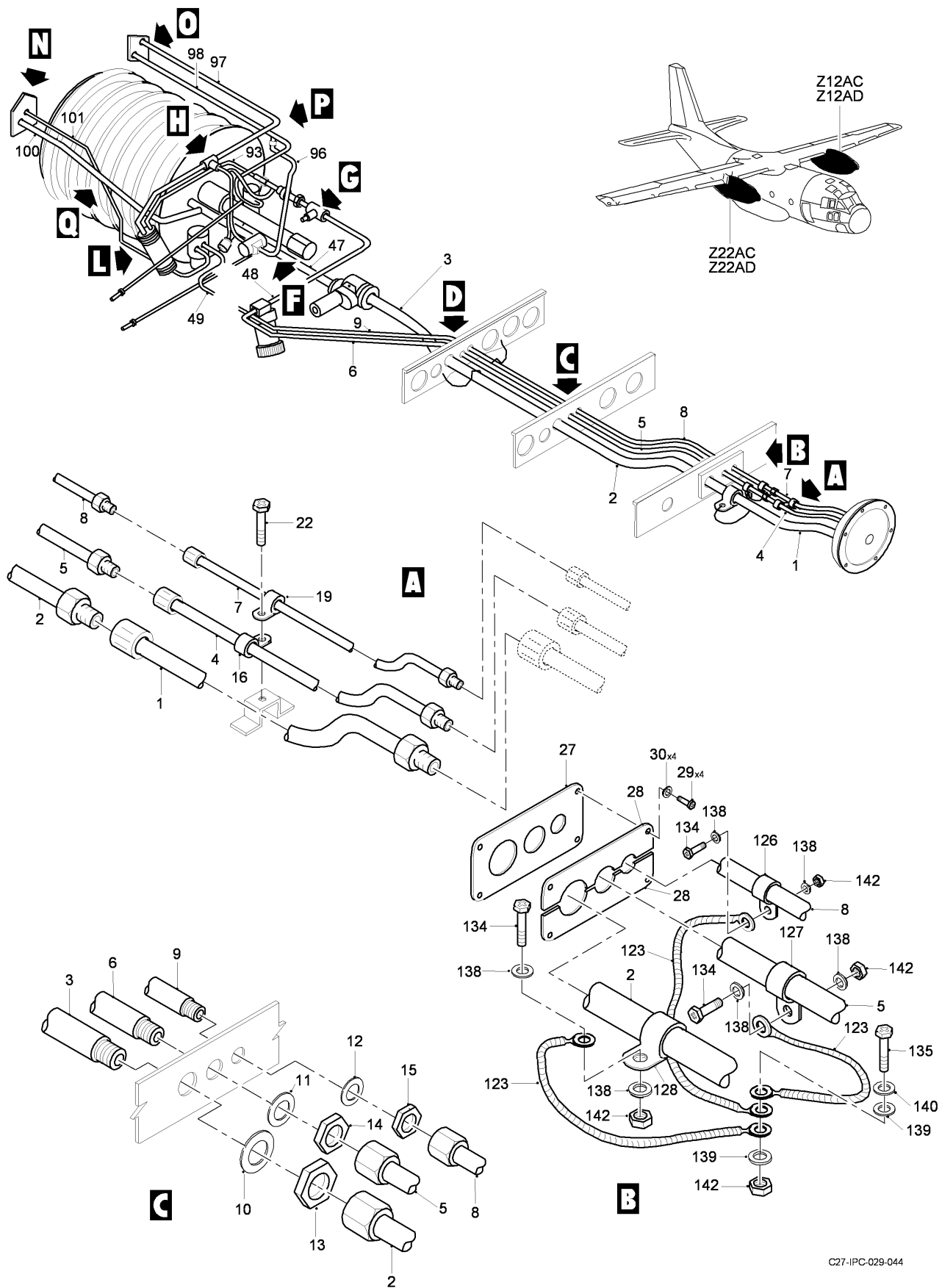
FIG 09 HYDRAULIC INSTL - ENGINE, Z12AC-22AC-12AD-22AD, LH-RH (SHEET 1 OF 5)
