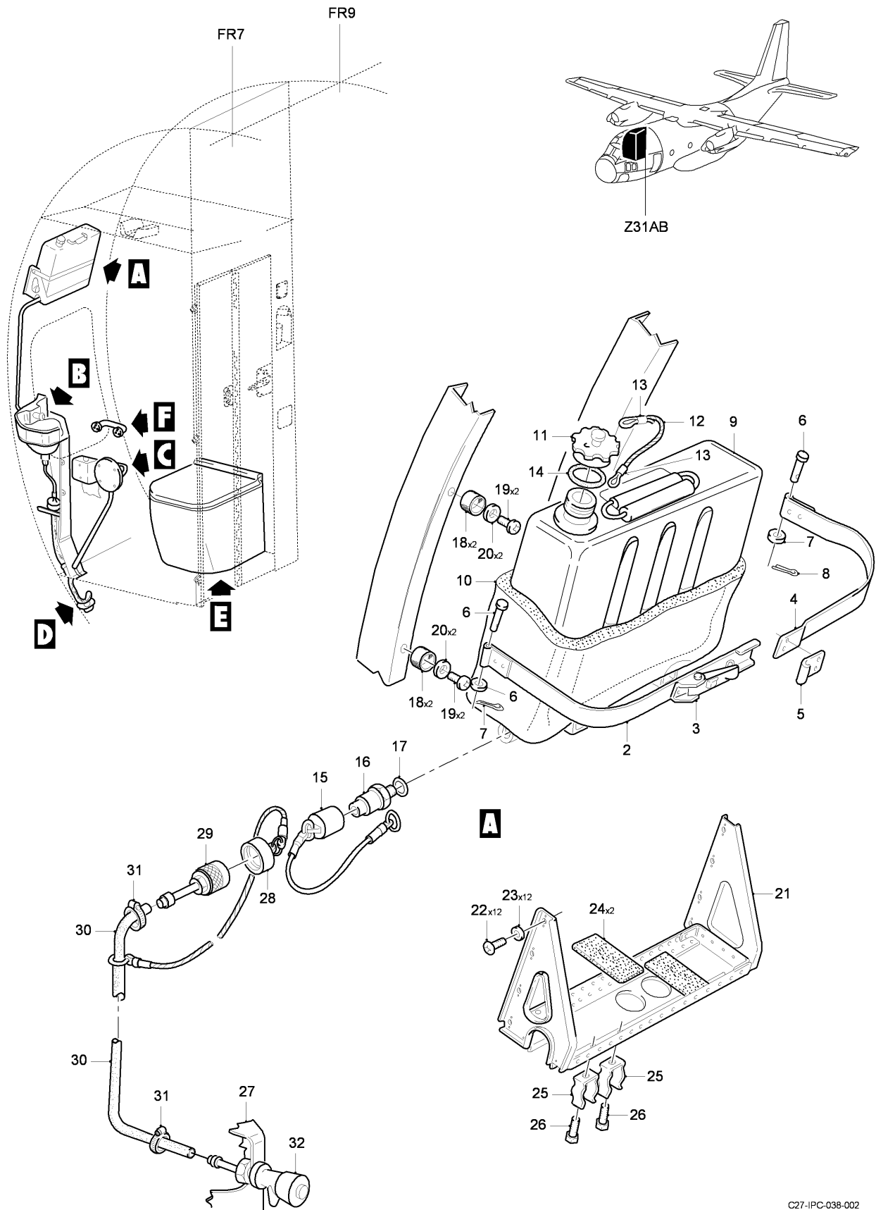
FIG 01 TOILET INSTL, Z31AB (SHEET 1 OF 3)
