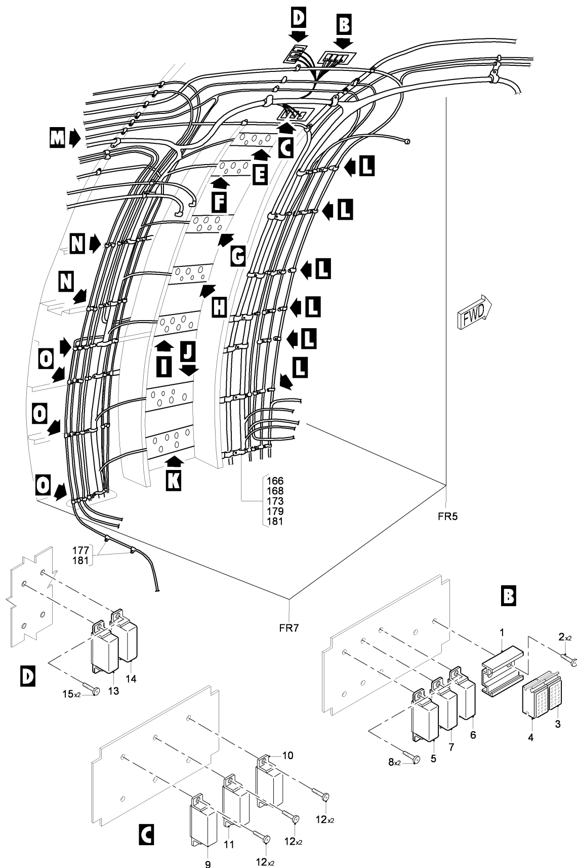
FIG 04 ELECTRICAL AND ELECTRONICS INSTL - CABIN, Z31AA, LH (SHEET 2 OF 5)
