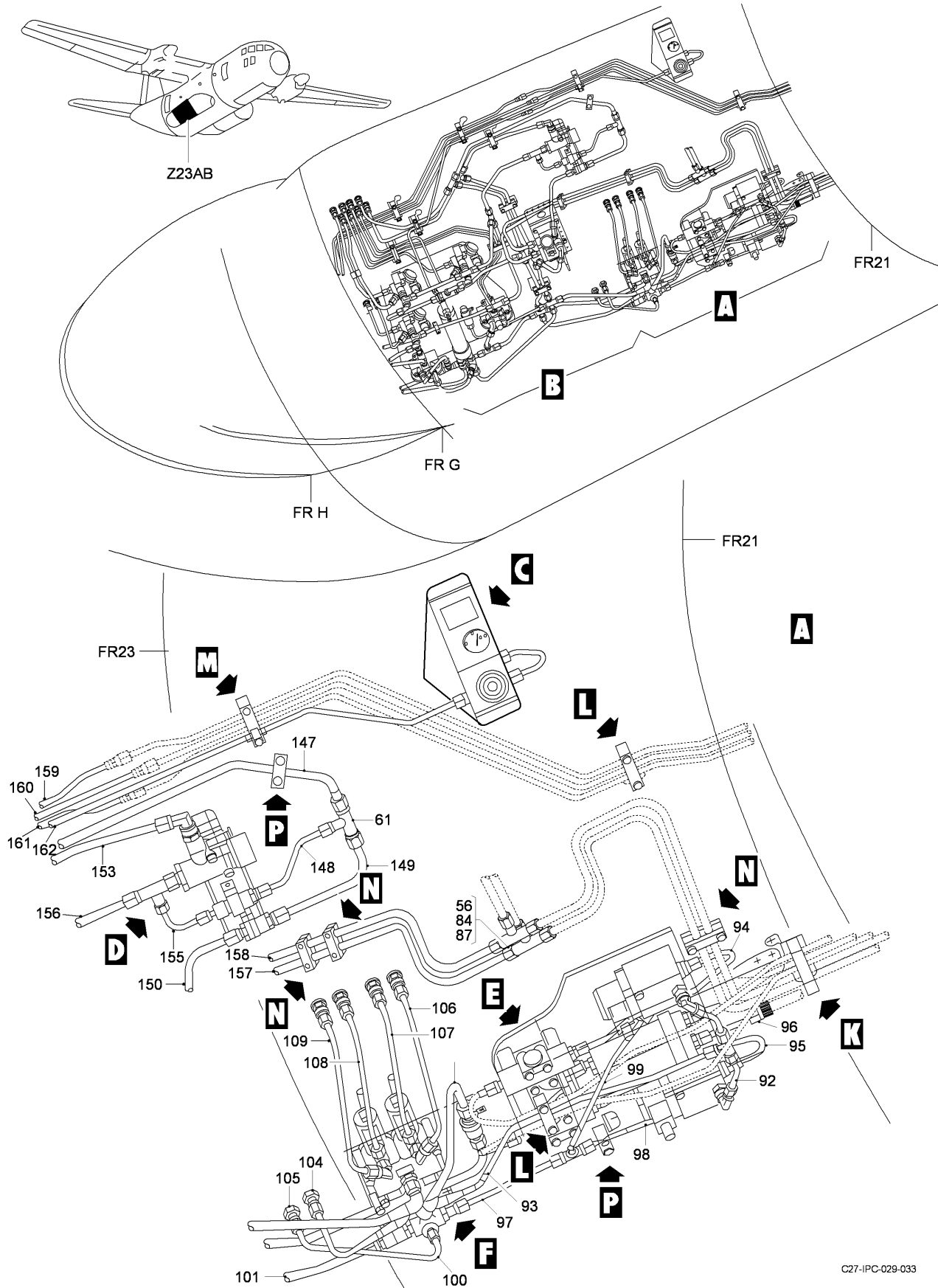
FIG 08 HYDRAULIC INSTL - MLG, Z23AB, RH (SHEET 1 OF 11)
