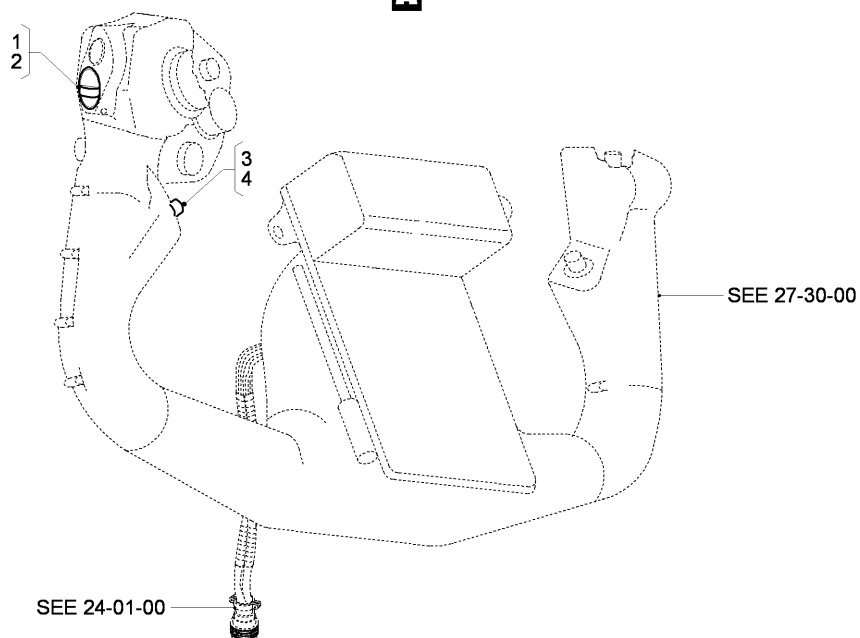
FIG 05 RADIO INTERPHONE SWITCH INSTL, Z31AA, LH-RH (SHEET 1 OF 1)
