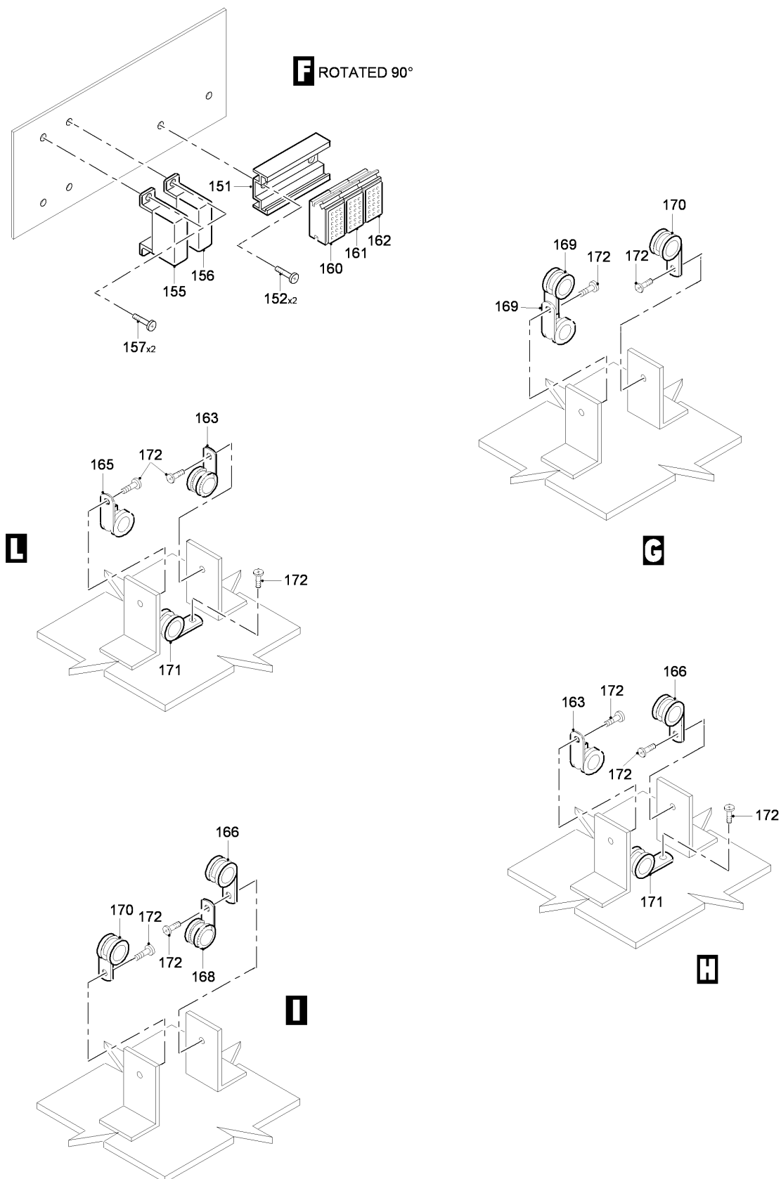
FIG 07 ELECTRICAL AND ELECTRONICS INSTL - CABIN LOWER SIDE, Z31AA (SHEET 4 OF 4)
