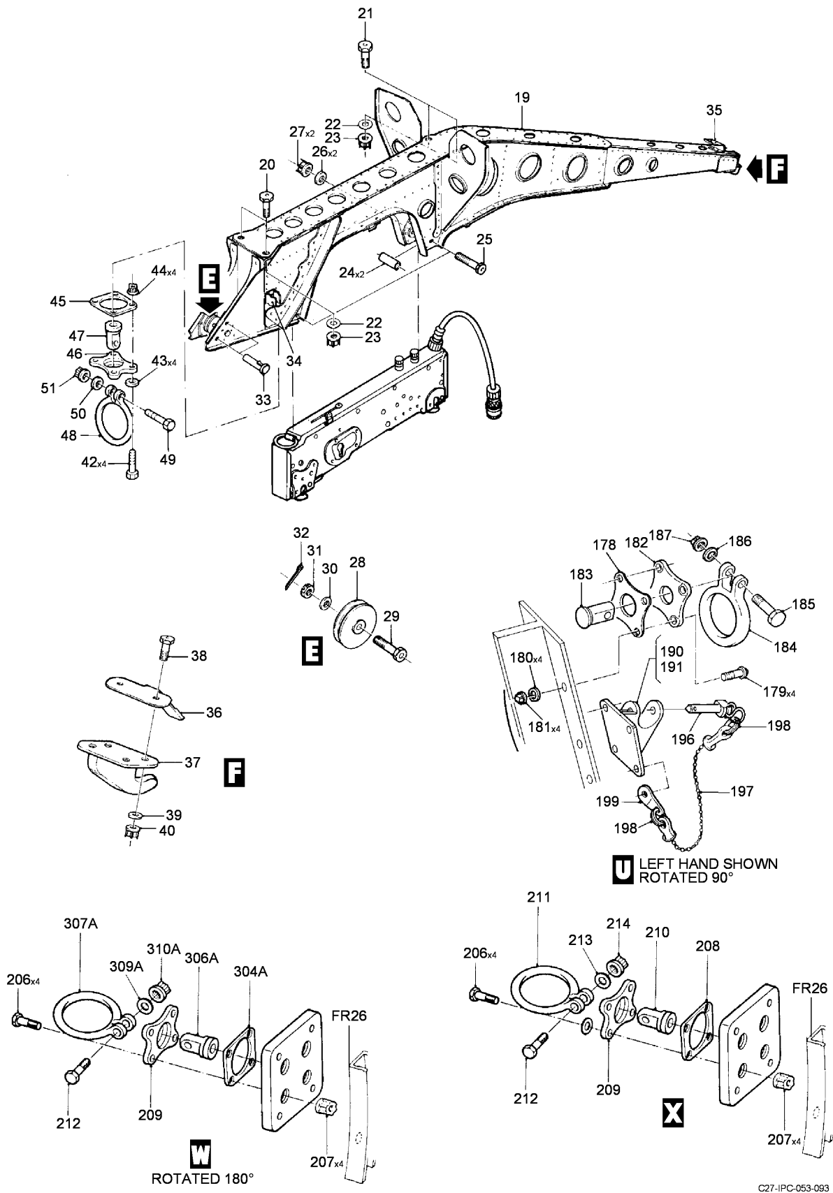
FIG 01 STRUCTURE INSTL, Z34AA (SHEET 5 OF 6)
