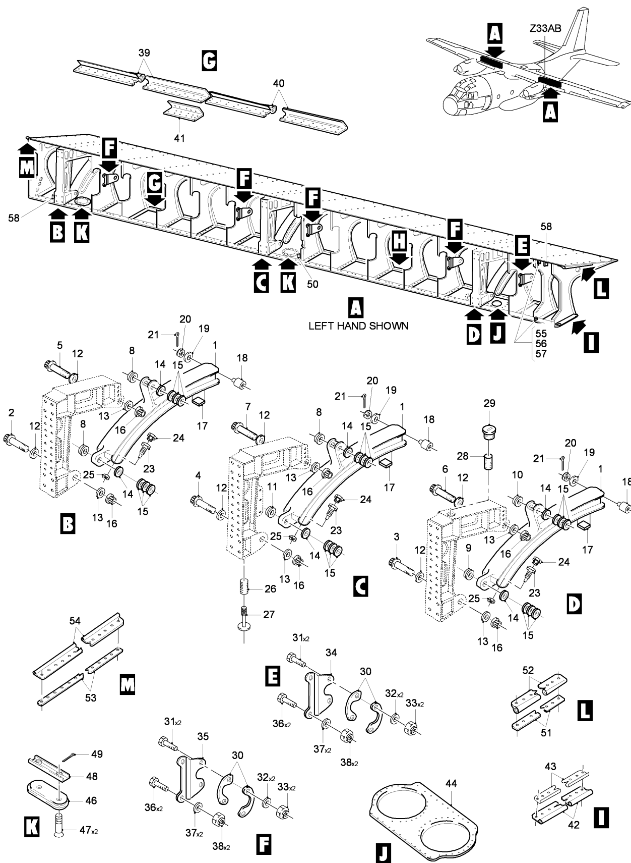
FIG 03 TRAILING EDGE INSTL - CENTER WING, Z33AB (SHEET 1 OF 1)
