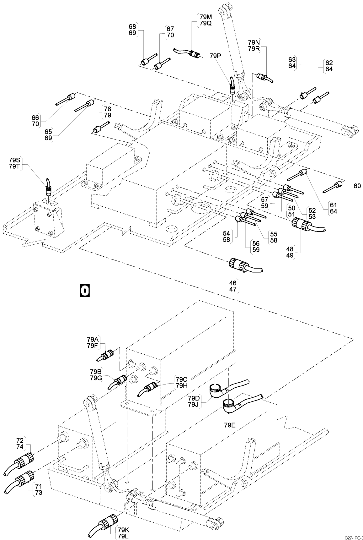
FIG 17 ELECTRICAL AND ELECTRONICS INSTL, Z31AA-32AA-32AB-32AC-32AD (SHEET 6 OF 8)
