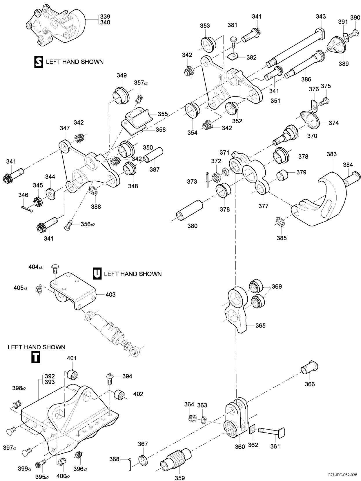
FIG 02 CARGO RAMP ASSY (SHEET 6 OF 6)
