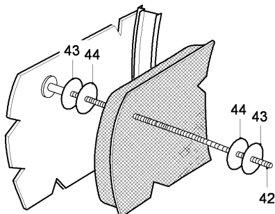
FIG 03 PRIMARY THERMAL INSULATION INSTL - LH SIDE, Z31AA-31AB (SHEET 1 OF 1)
