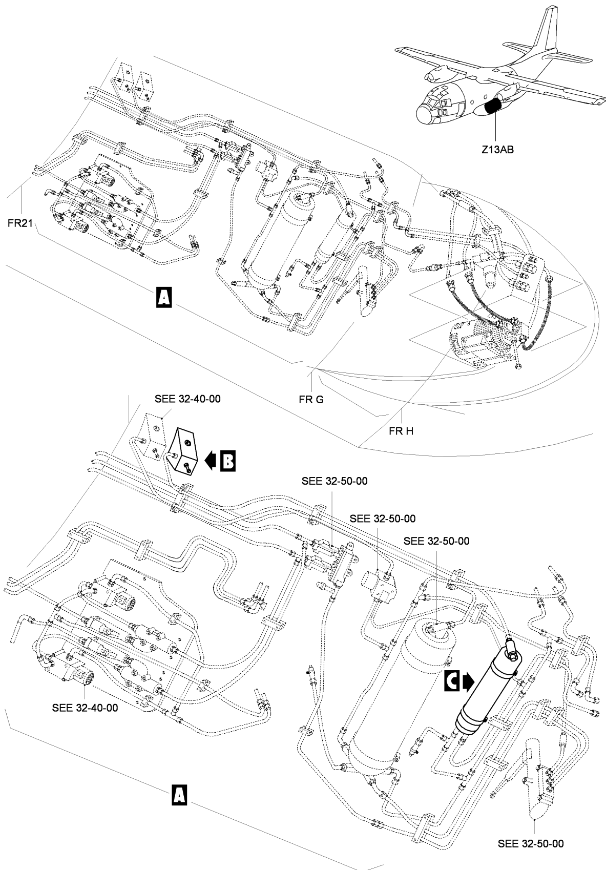
FIG 06 HYDRAULIC INSTL - MLG, Z23AB, RH (SHEET 1 OF 2)
