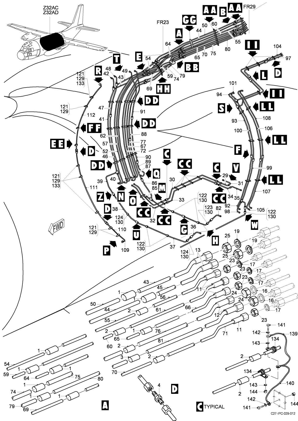
FIG 04 HYDRAULIC INSTL - CENTER FUSELAGE, Z32AC-32AD (SHEET 1 OF 6)
