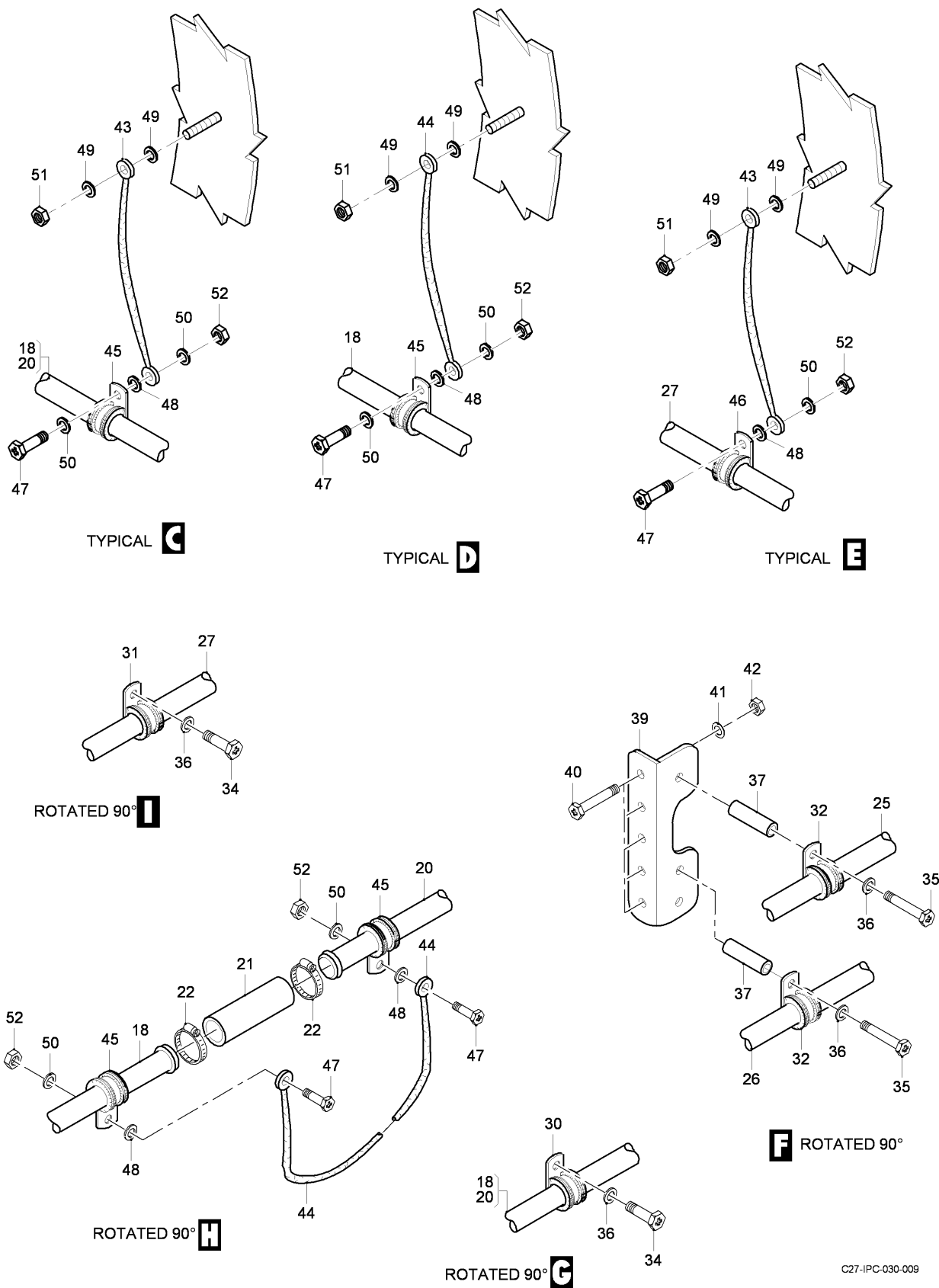
FIG 07 ANTI-ICING INSTL - OUTER WING, Z11AA, LH (SHEET 3 OF 3)
