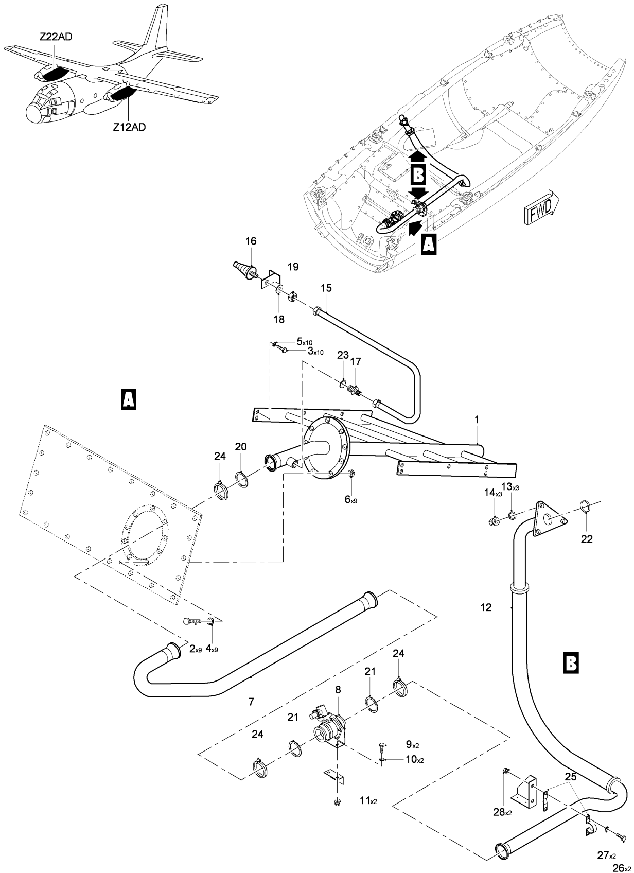
FIG 03 ENGINE AUGMENTATION INSTL, Z12AD-22AD (SHEET 1 OF 1)
