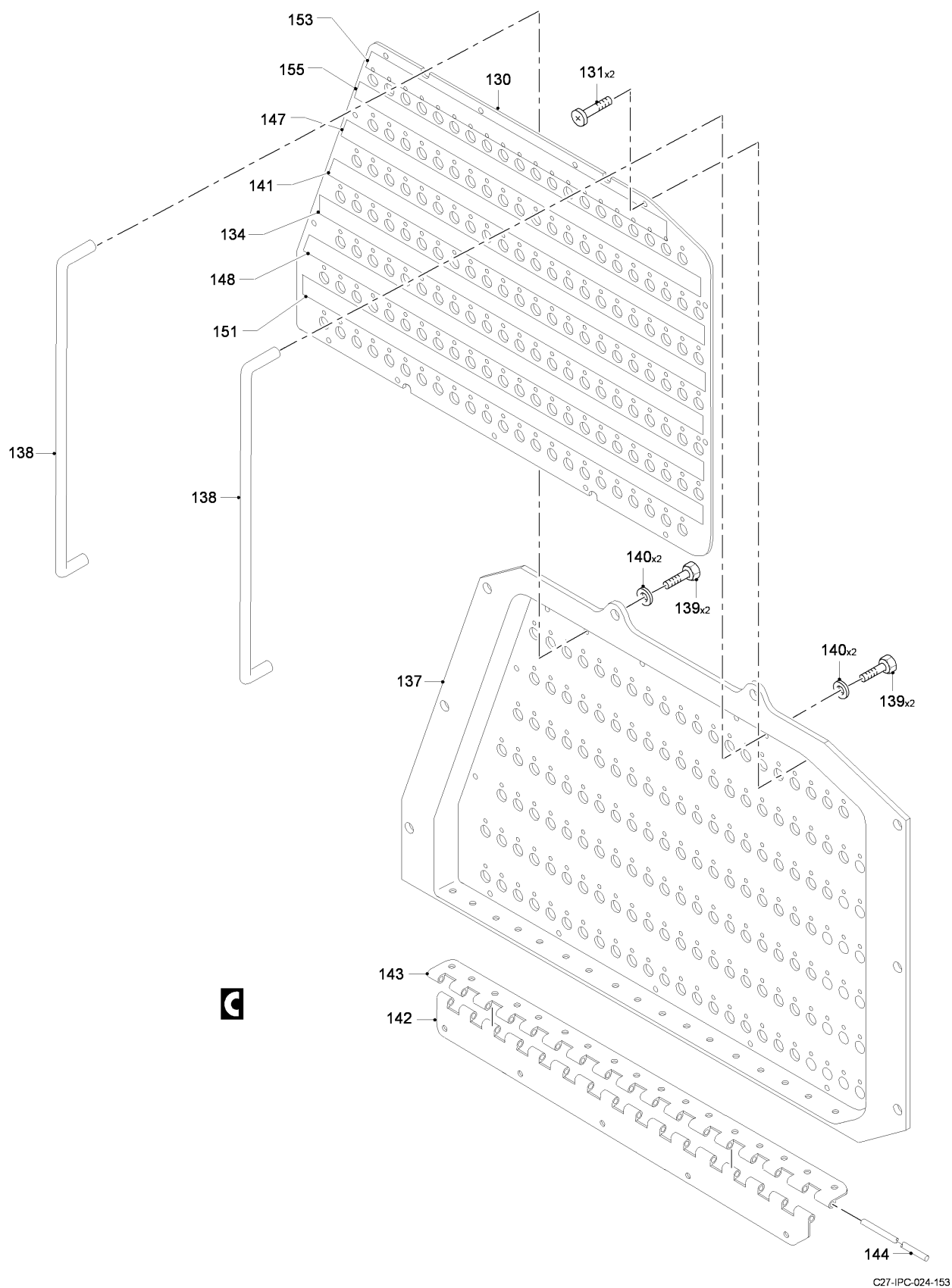
FIG 03 CIRCUIT BREAKER PANEL NO. 2 INSTL, Z31AA (SHEET 2 OF 3)
