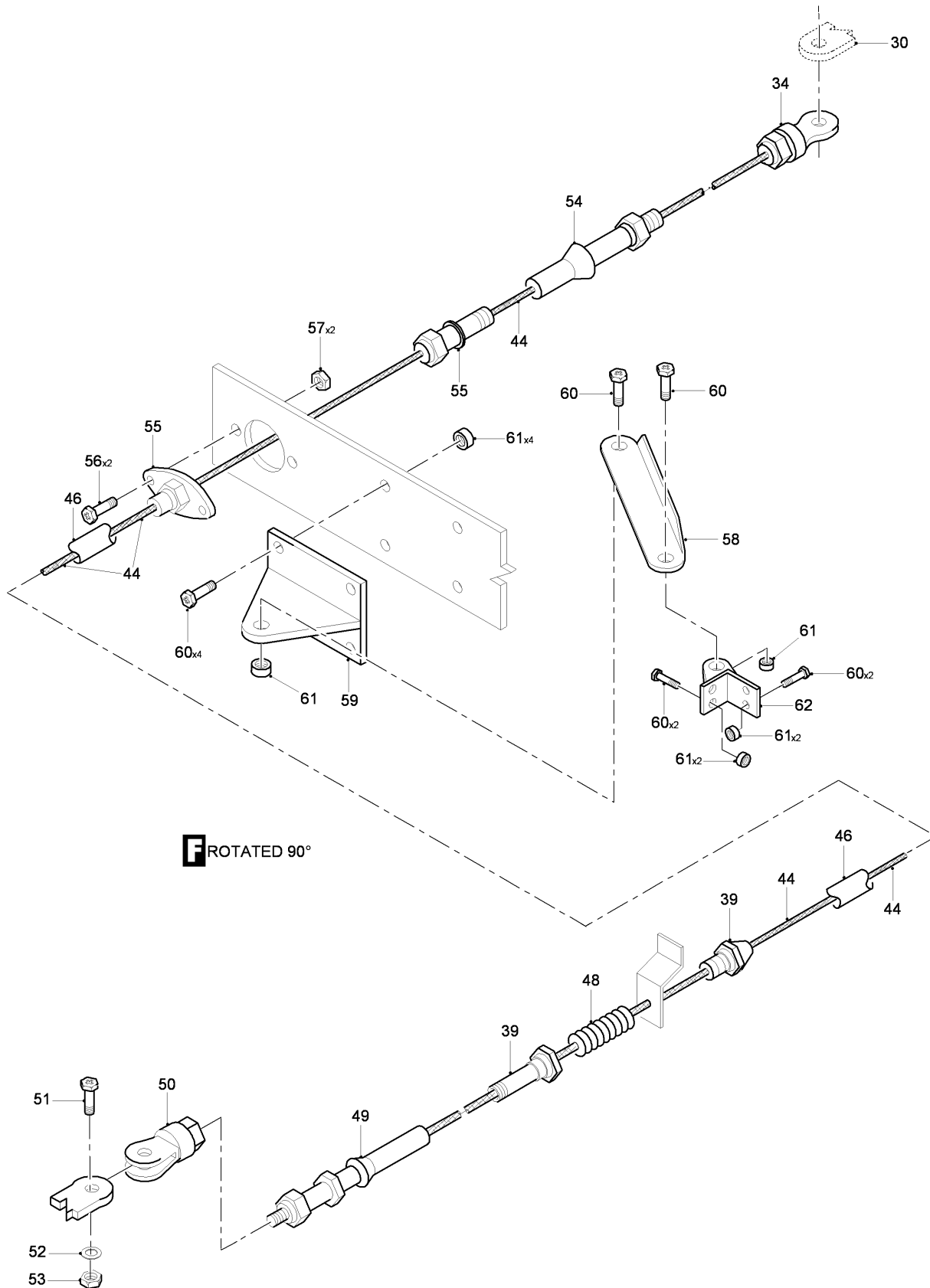
FIG 03 EMERGENCY CONTROL INSTL - MAIN LANDING GEAR, Z32BA (SHEET 4 OF 4)
