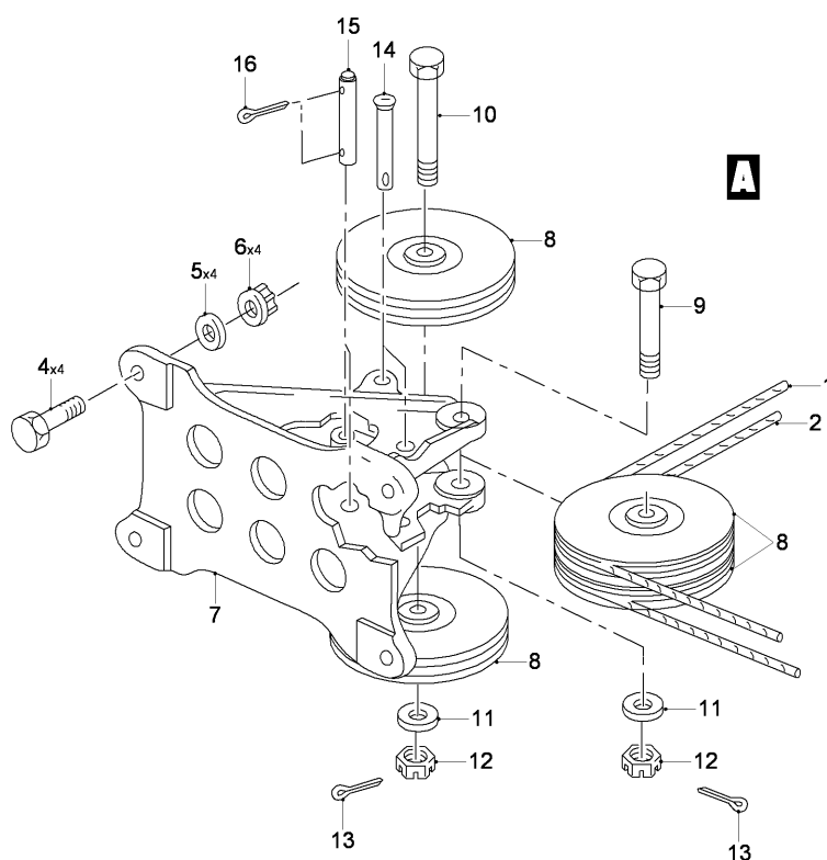
FIG 02 FLAP CONTROLS INSTL, Z31BB (SHEET 1 OF 4)
