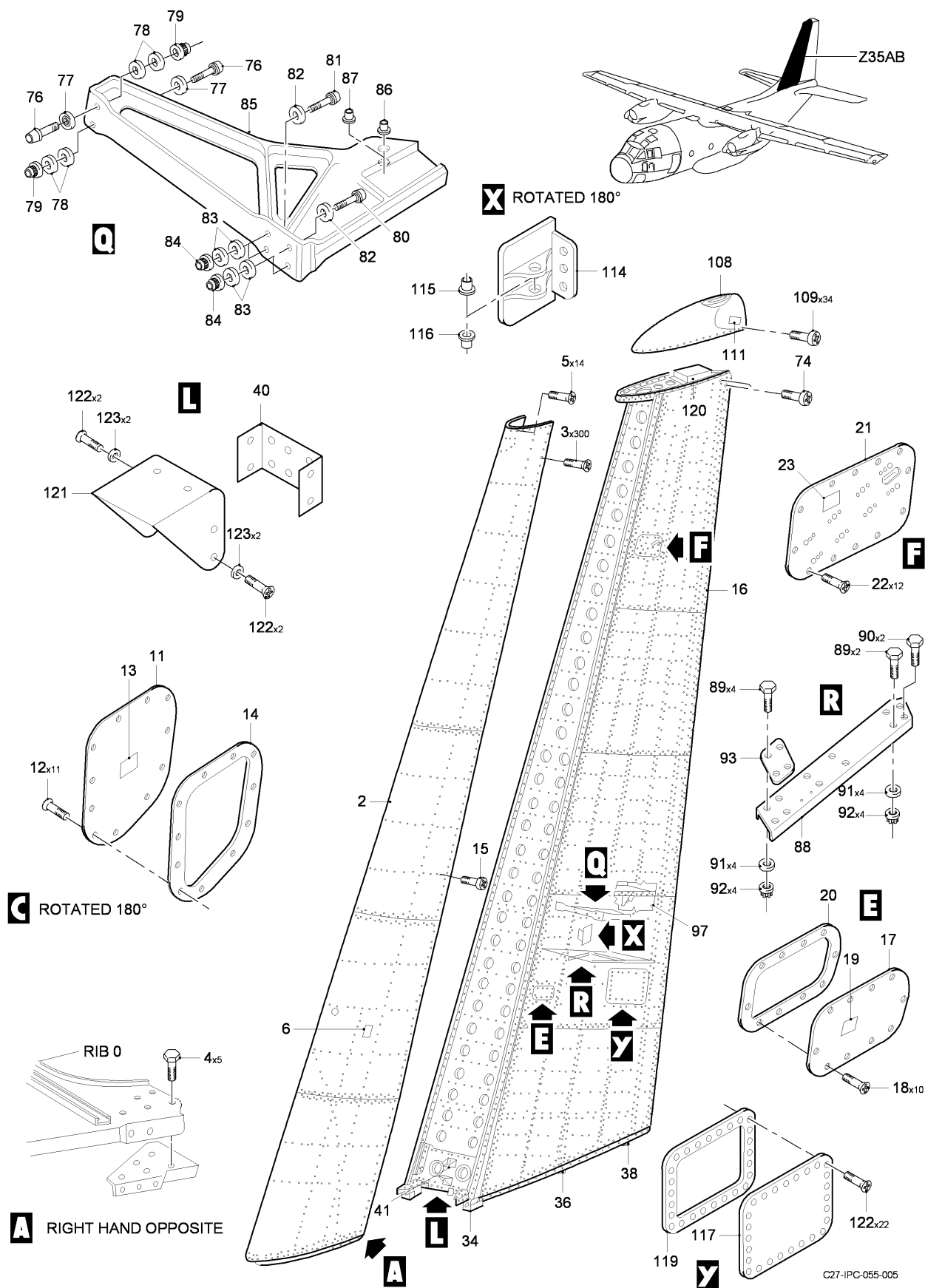
FIG 01 VERTICAL STABILIZER INSTL, Z35AB (SHEET 1 OF 2)
