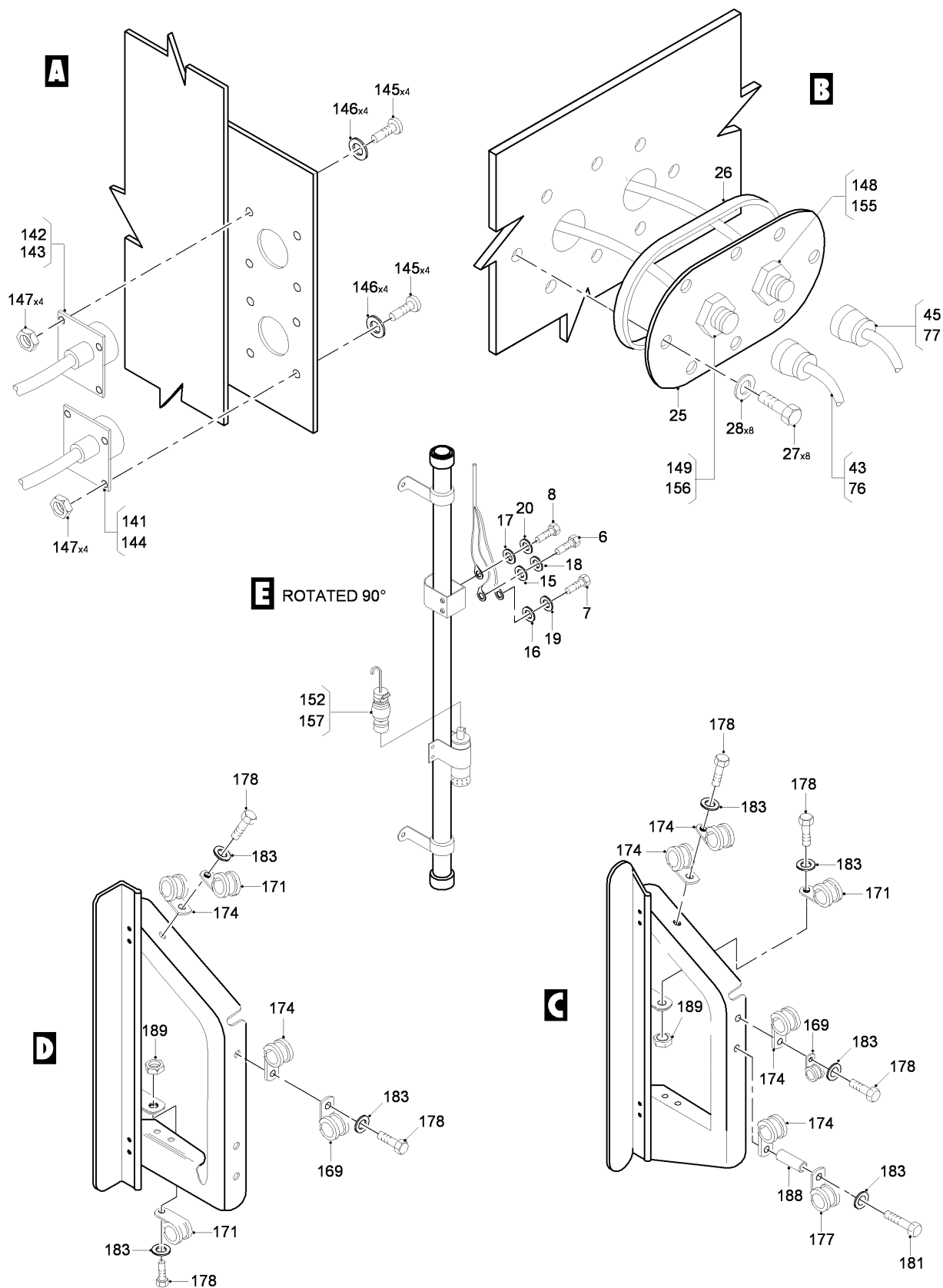
FIG 22 ELECTRICAL AND ELECTRONICS INSTL - CENTER WING, Z33AB, LH (SHEET 2 OF 7)
