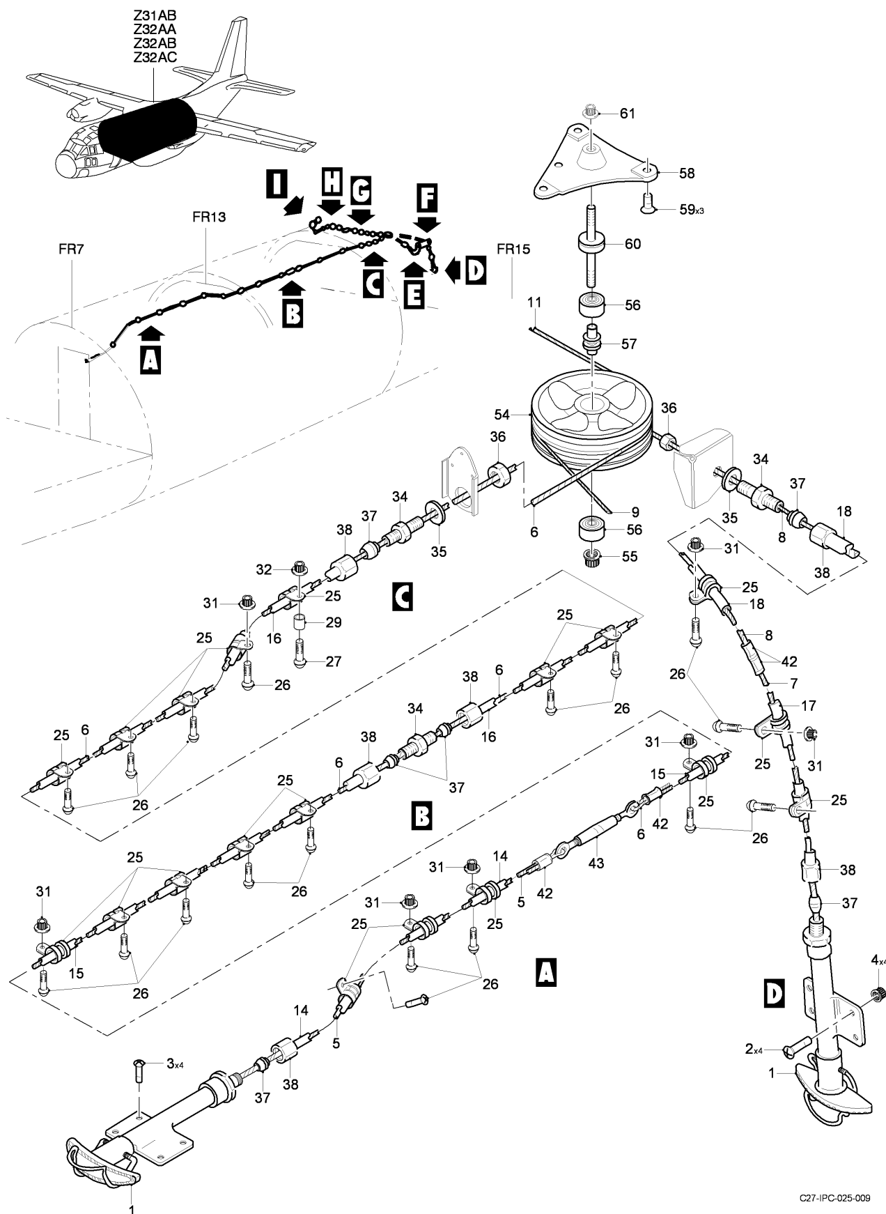
FIG 02 LIFE RAFTS OPENING EMERG CONTROL INSTL, Z31AB-32AA-32AB-32AC (SHEET 1 OF 3)
