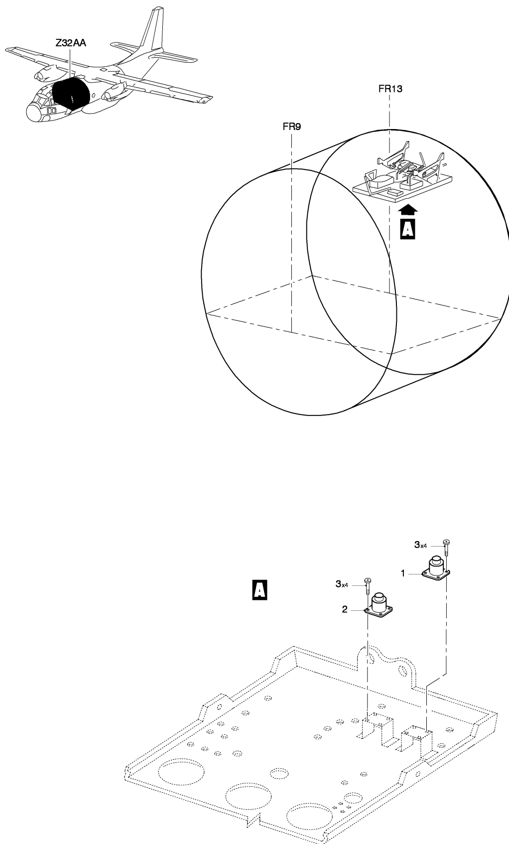
FIG 05 SPST CONTACTOR INSTL, Z32AA (SHEET 1 OF 1)
