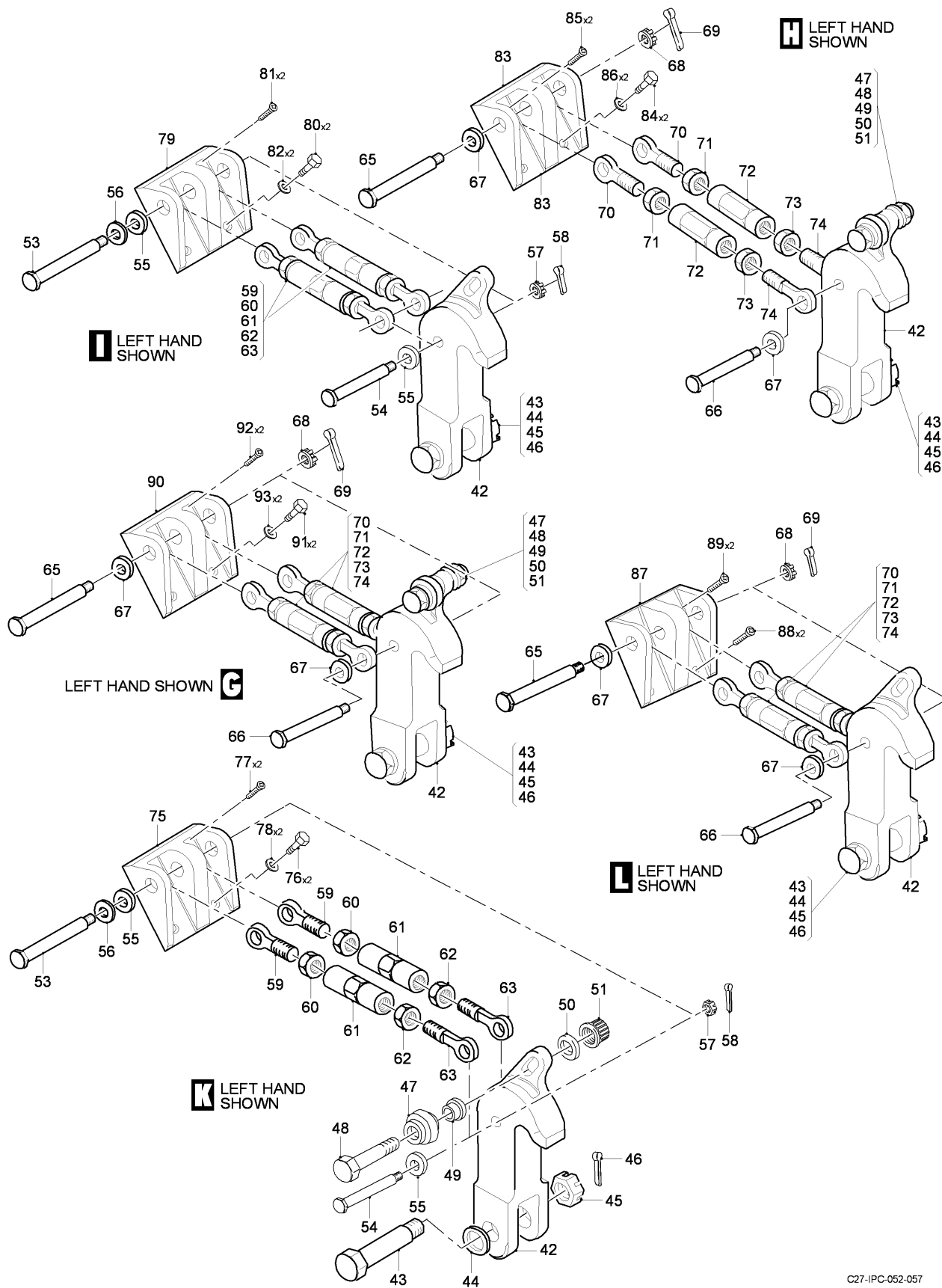
FIG 12 CARGO DOOR ASSY (SHEET 2 OF 4)
