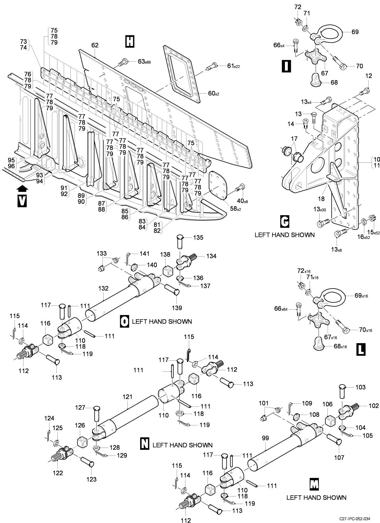
FIG 02 CARGO RAMP ASSY (SHEET 2 OF 6)
