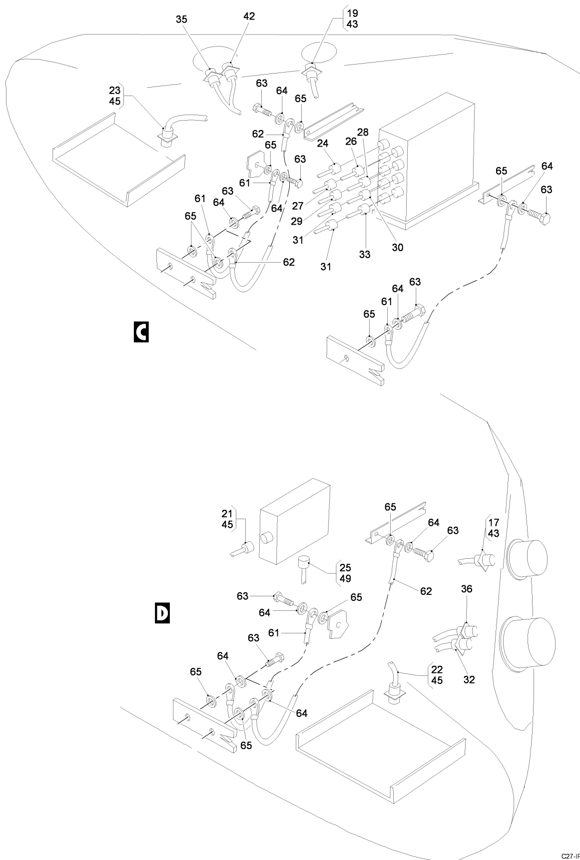
FIG 28 ELECTRICAL AND ELECTRONICS INSTL - TAIL CONE , Z34AB (SHEET 2 OF 2)
