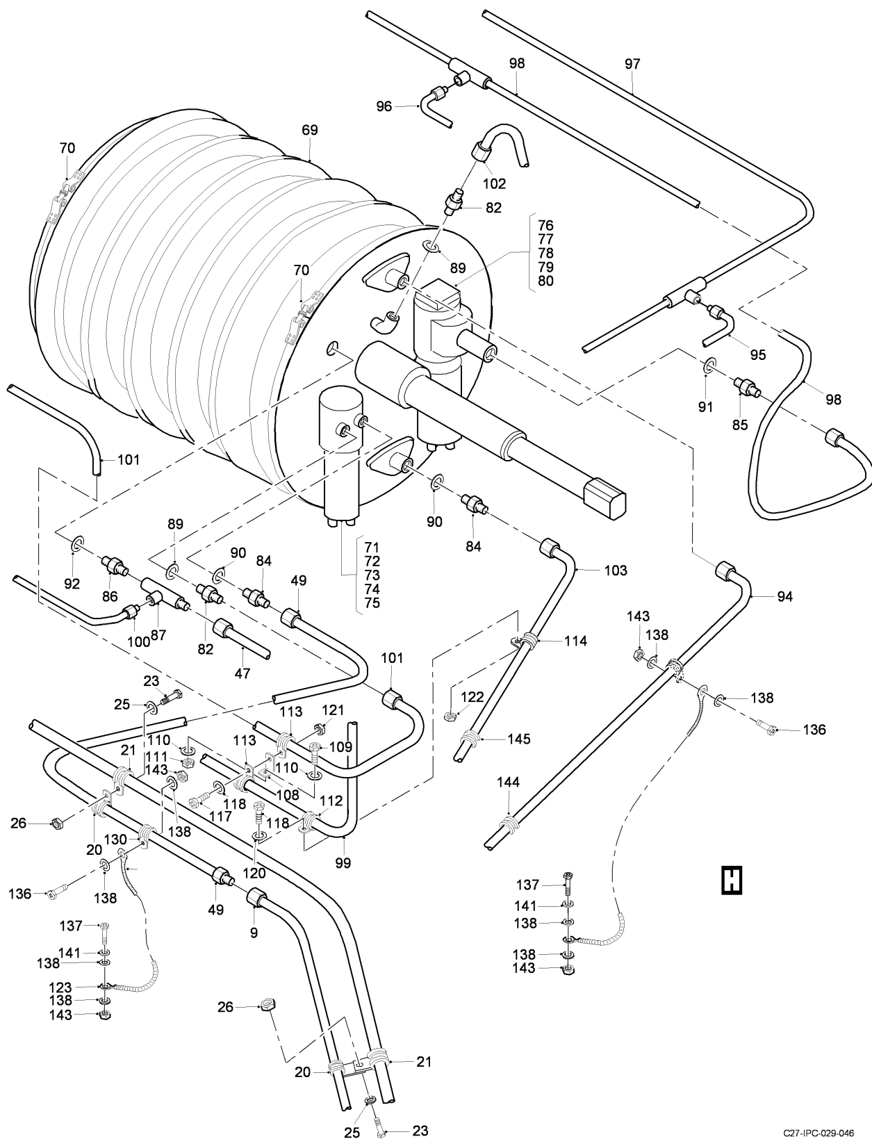
FIG 09 HYDRAULIC INSTL - ENGINE, Z12AC-22AC-12AD-22AD, LH-RH (SHEET 3 OF 5)
