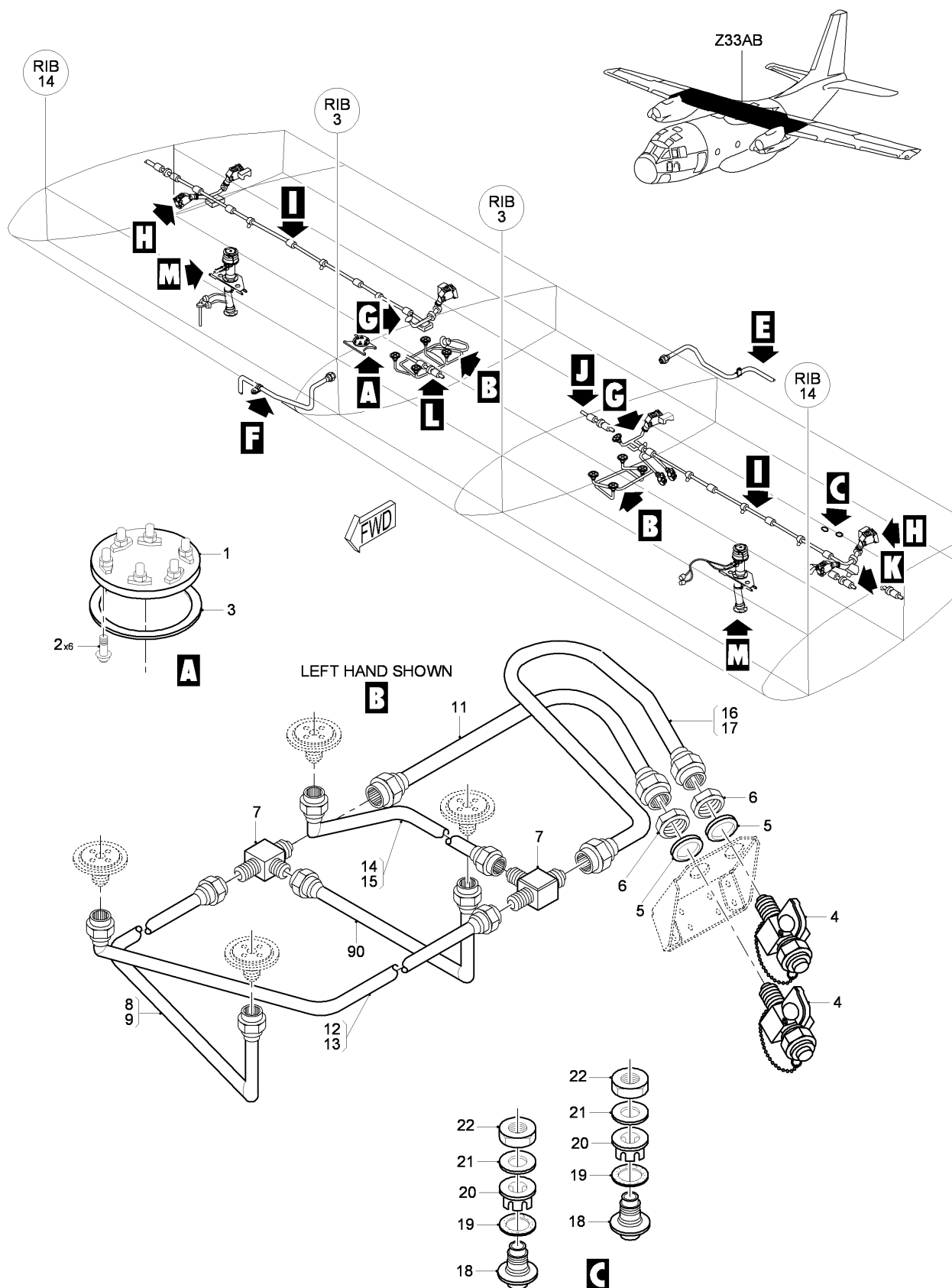
FIG 01 FUEL VENT AND DRAINS INSTL - CENTER WING, Z33AB, LH-RH (SHEET 1 OF 4)
