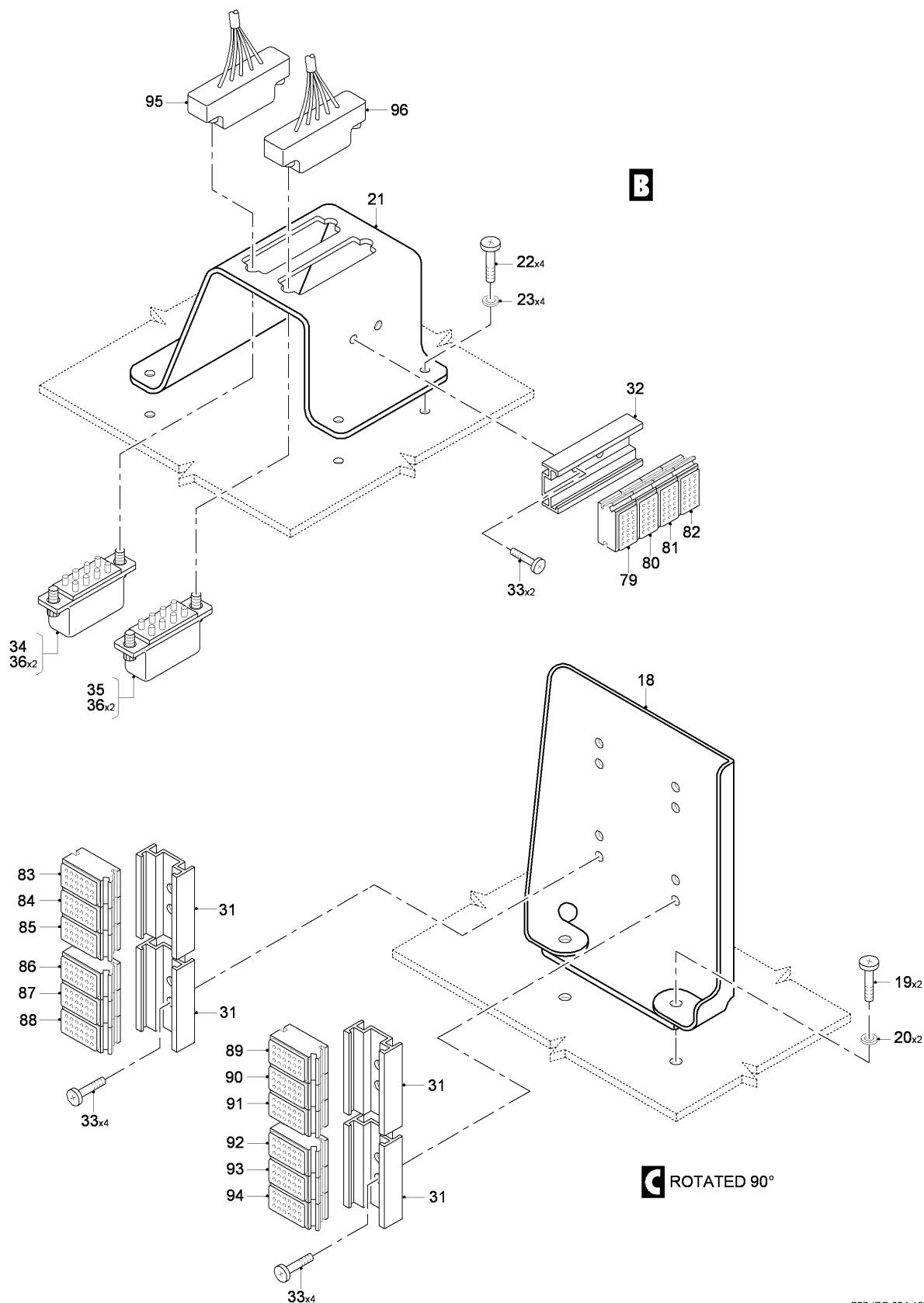
FIG 11 FIFTH AND SIXTH SHELF INSTL - ELECTRICAL COMPARTMENT, Z31AA (SHEET 2 OF 4)
