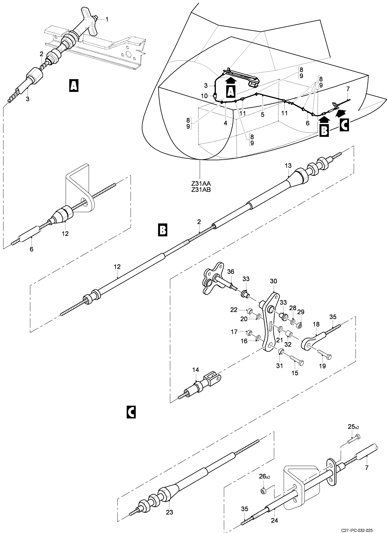
FIG 02 PARKING AND WHEEL BRAKES EMERGENCY INSTL, Z31AA-31BB (SHEET 1 OF 1)
