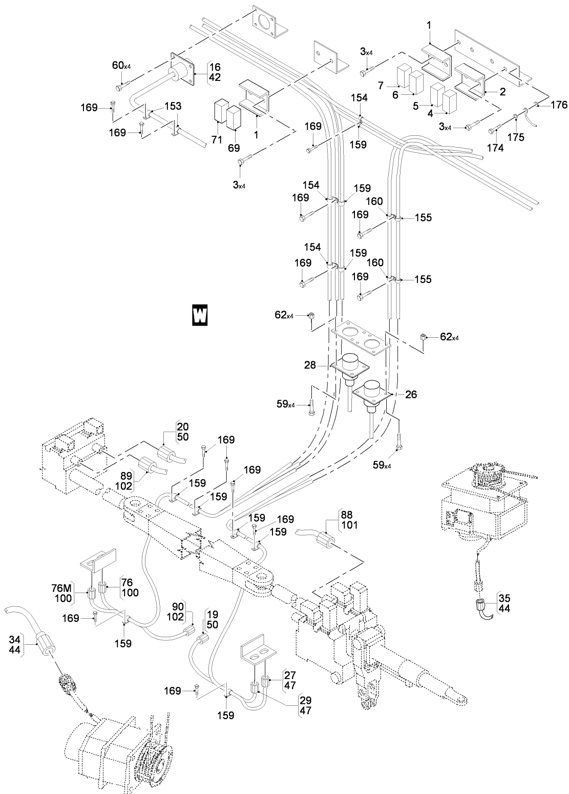
FIG 19M ELECTRICAL AND ELECTRONICS INSTL - REAR FUSELAGE, Z34AA (SHEET 7 OF 10)
