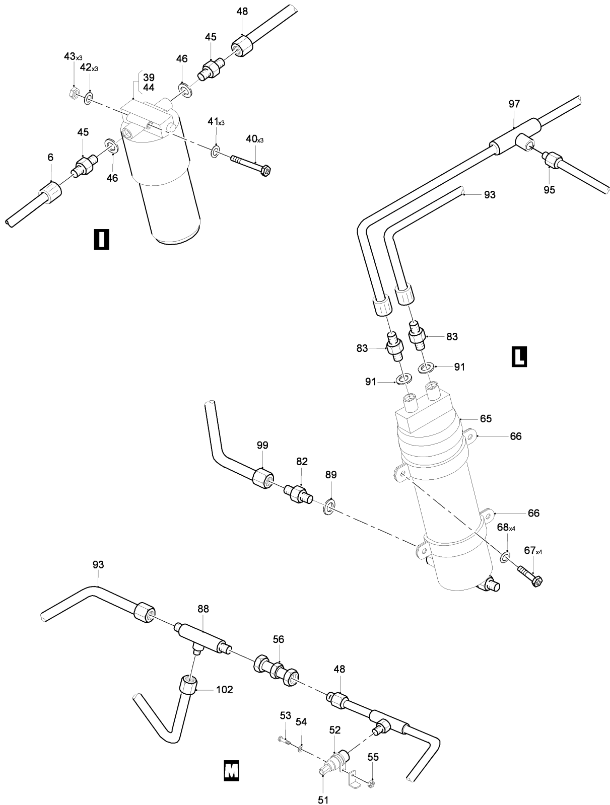
FIG 09 HYDRAULIC INSTL - ENGINE, Z12AC-22AC-12AD-22AD, LH-RH (SHEET 4 OF 5)
