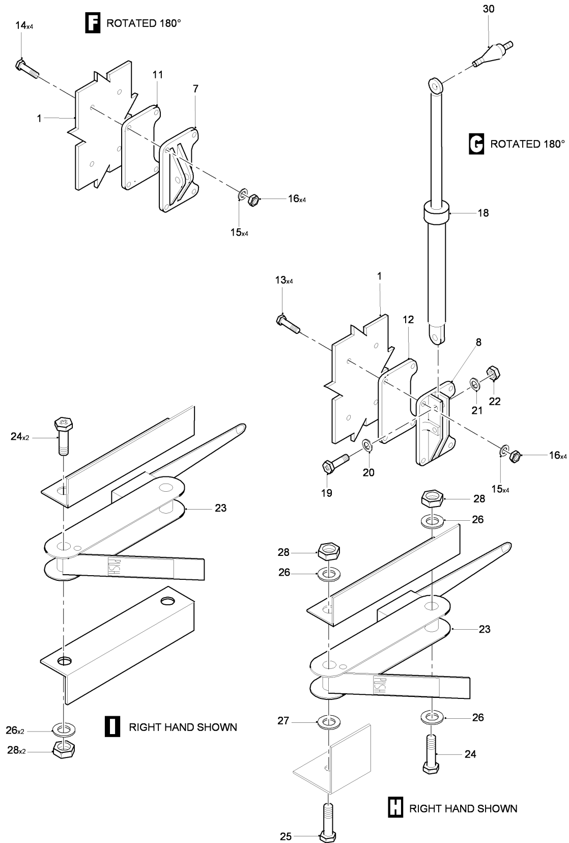
FIG 04 PANEL ASSY INSTL - SIDE FWD, Z12AC-22AC, LH-RH (SHEET 2 OF 2)
