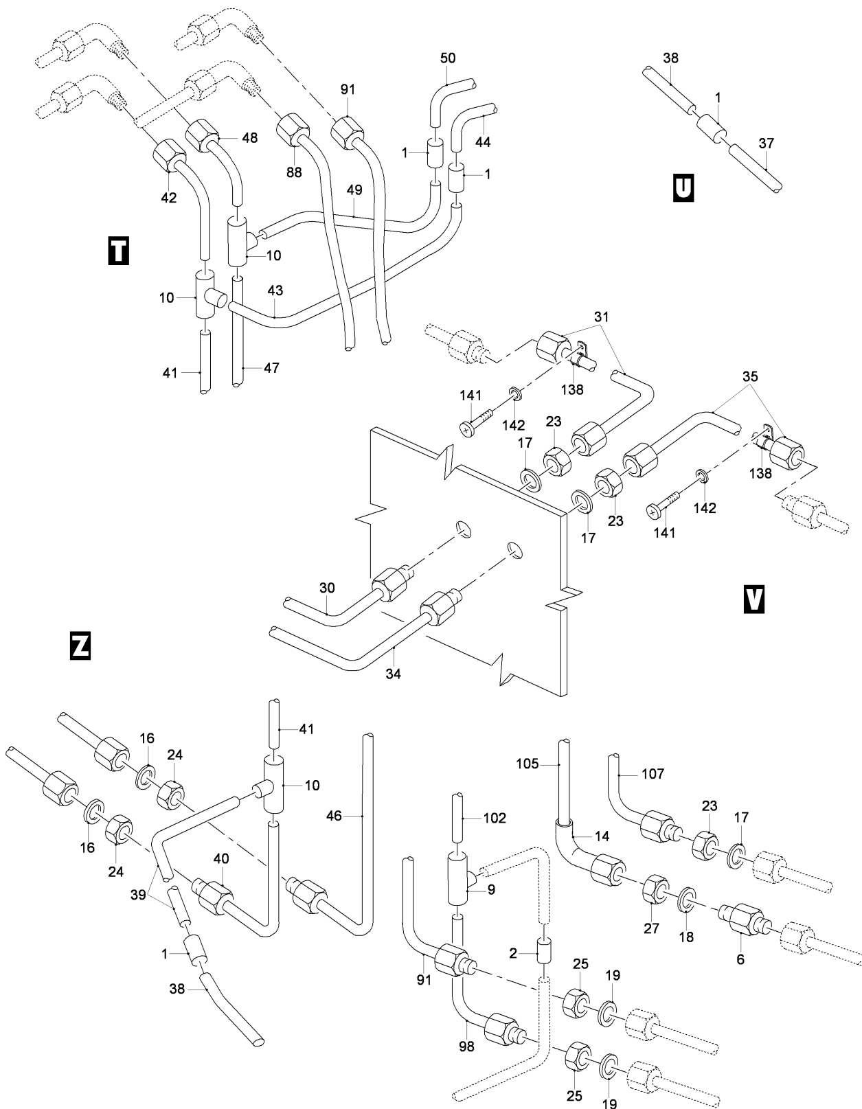
FIG 04 HYDRAULIC INSTL - CENTER FUSELAGE, Z32AC-32AD (SHEET 4 OF 6)
