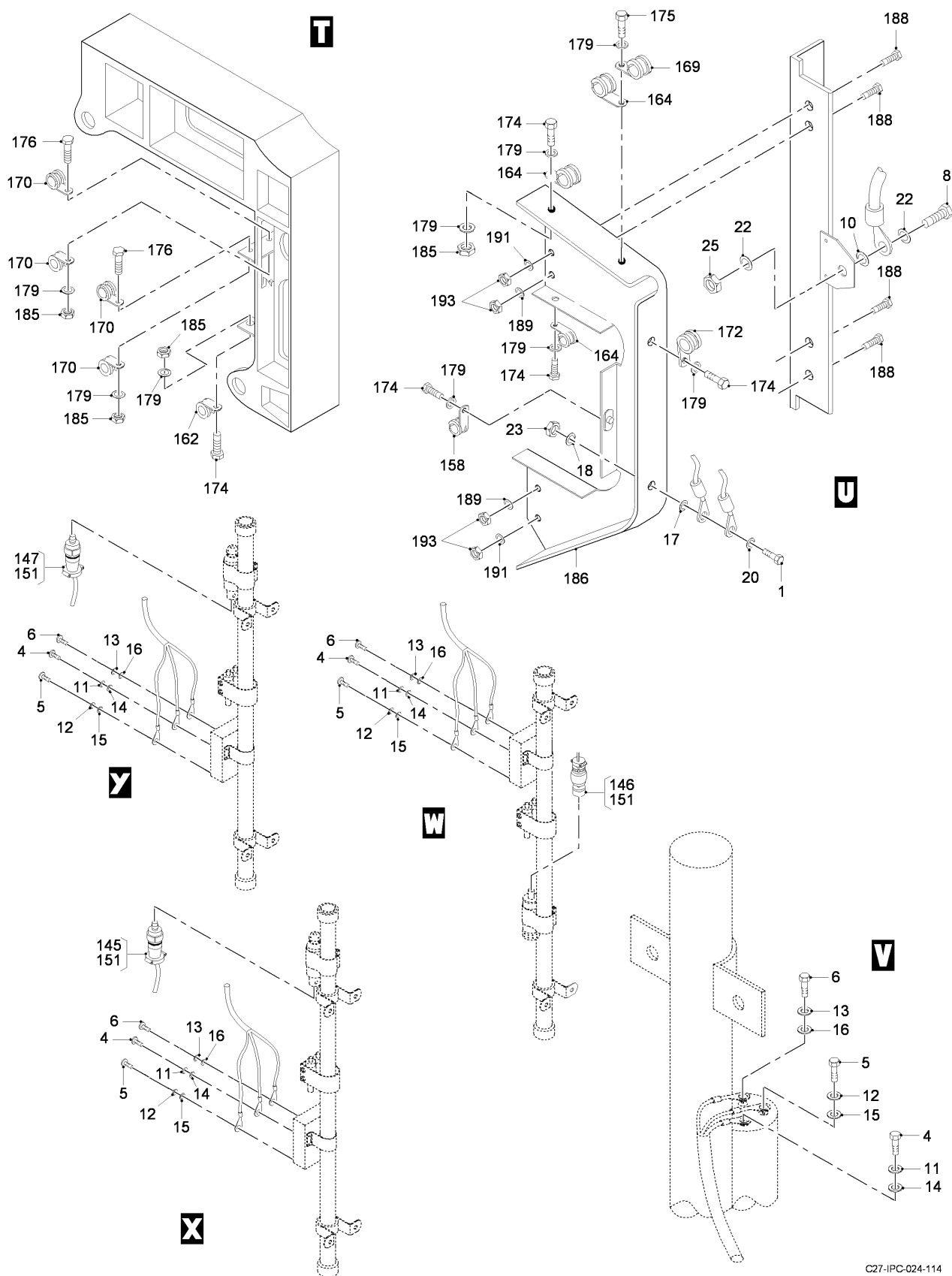
FIG 23 ELECTRICAL AND ELECTRONICS INSTL - CENTER WING, Z33AB, RH (SHEET 6 OF 6)
