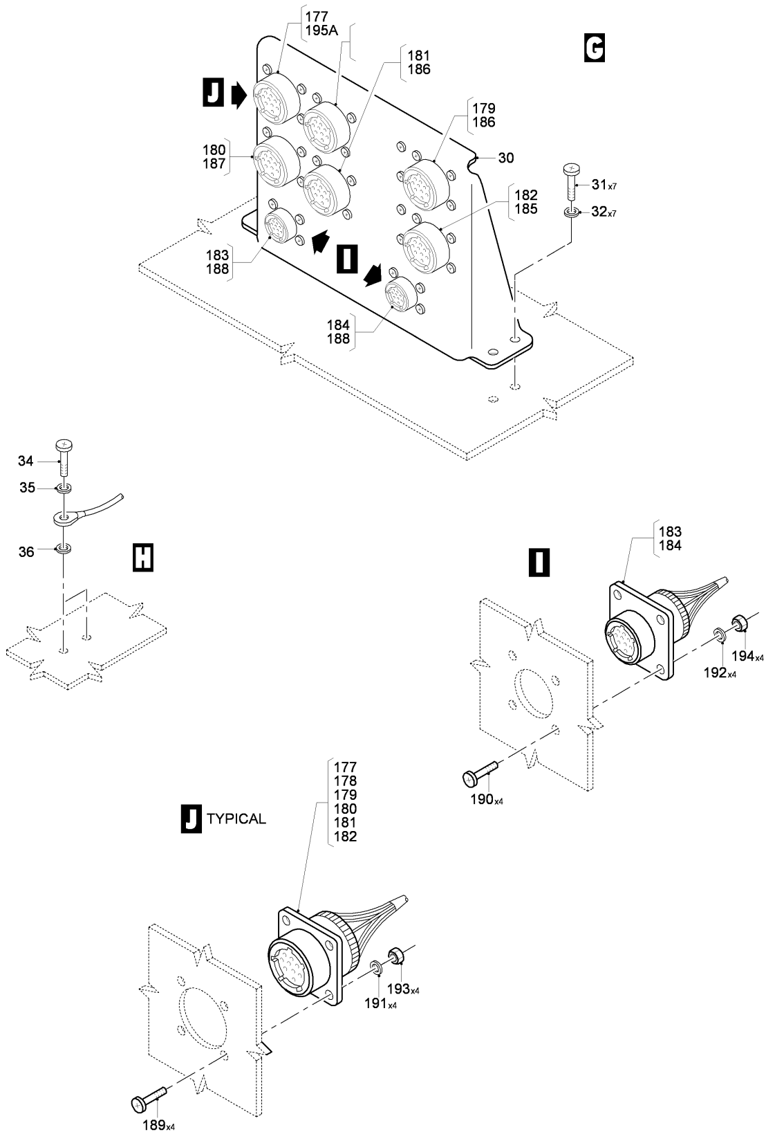
FIG 10 FOURTH SHELF INSTL - ELECTRICAL COMPARTMENT, Z31AA (SHEET 4 OF 4)
