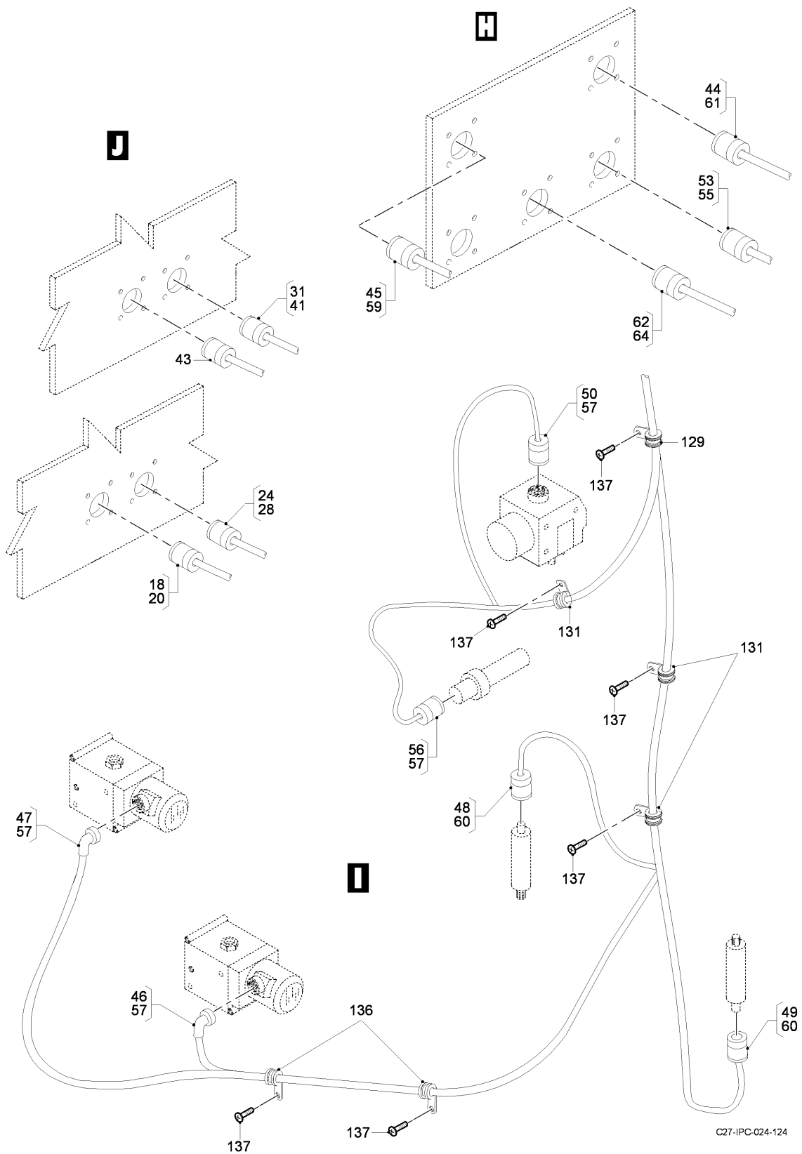
FIG 26 ELECTRICAL AND ELECTRONICS INSTL - MLG, Z13AA-13AB-13AC, LH (SHEET 4 OF 5)
