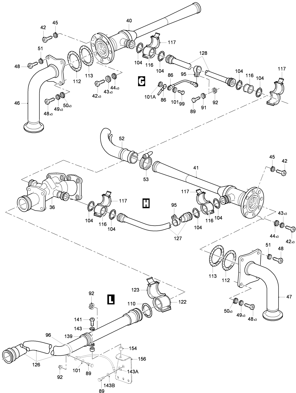
FIG 06 FUEL SUPPLY INSTL - OUTER WING, Z11AB, LH (SHEET 3 OF 4)
