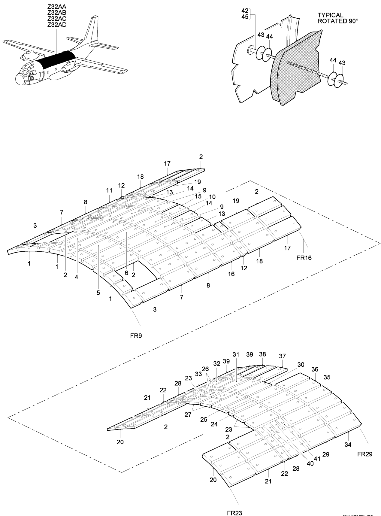
FIG 20 PRIMARY THERMAL INSULATION INSTL, Z32AA-32AB-32AC-32AD (SHEET 1 OF 1)
