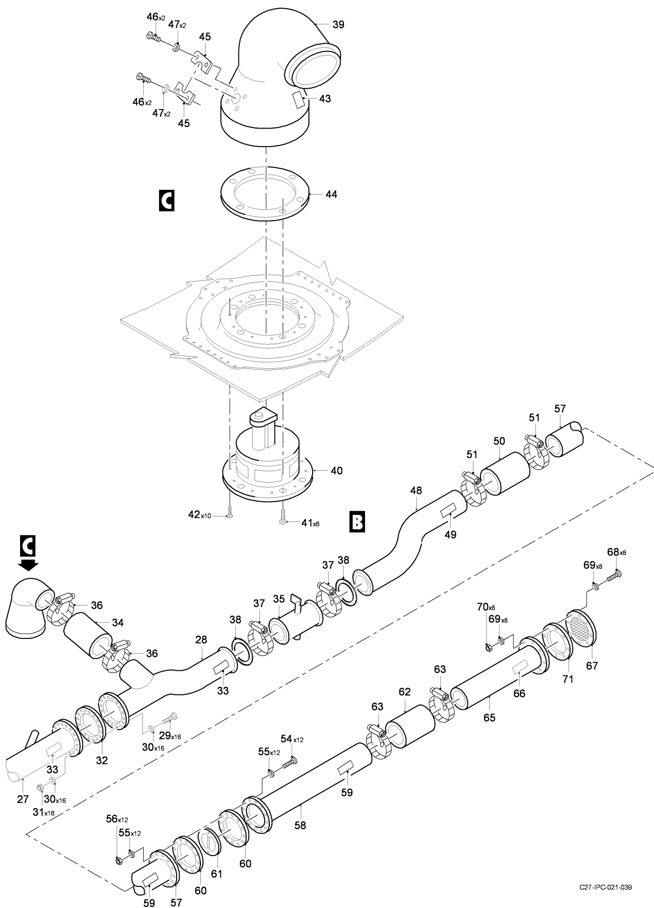
FIG 01 VENTILATION INSTL - CENTER FUSELAGE, Z32BA (SHEET 2 OF 3)
