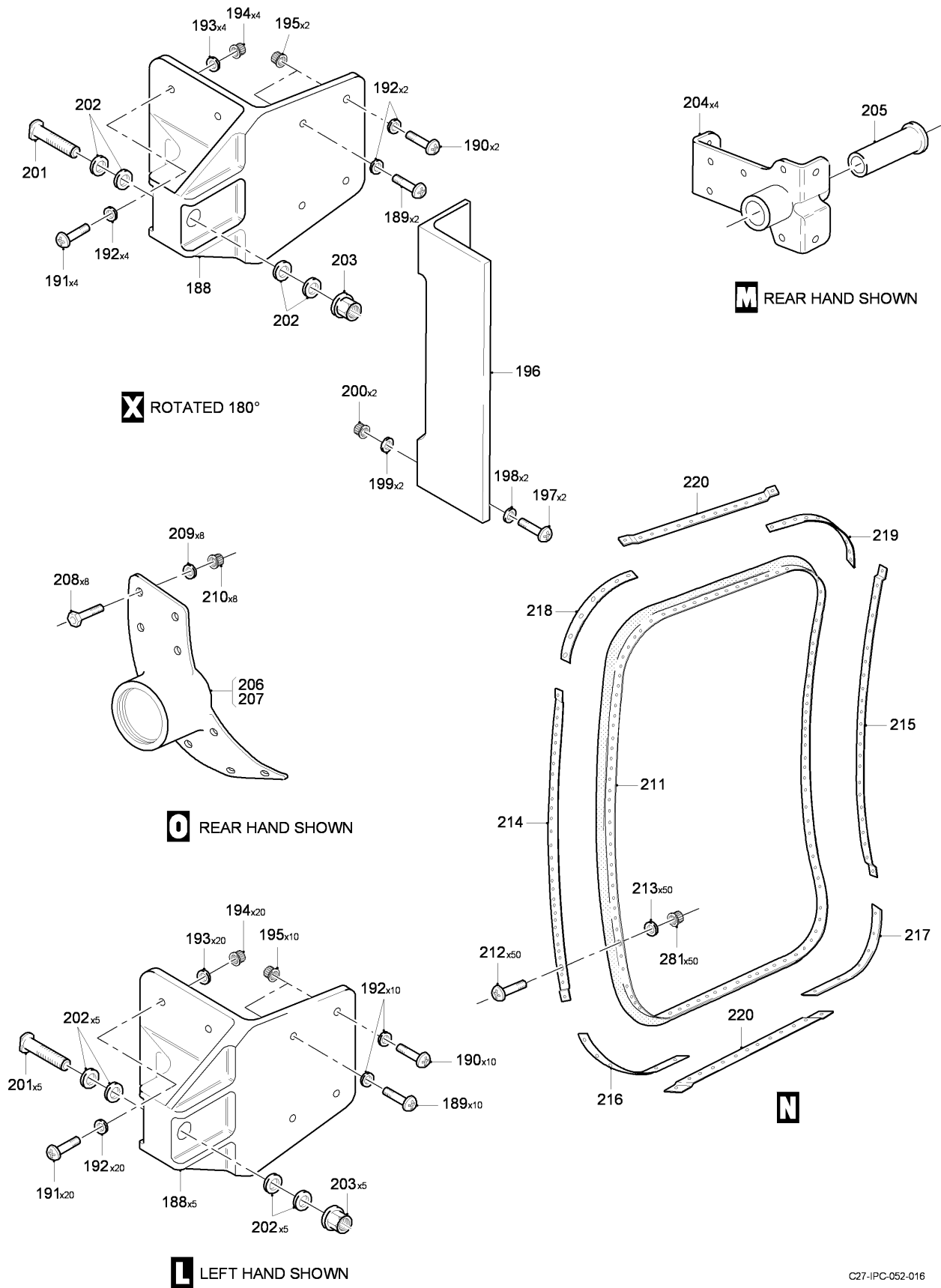
FIG 03 PARATROOPS DOOR ASSY, LH-RH (SHEET 5 OF 8)
