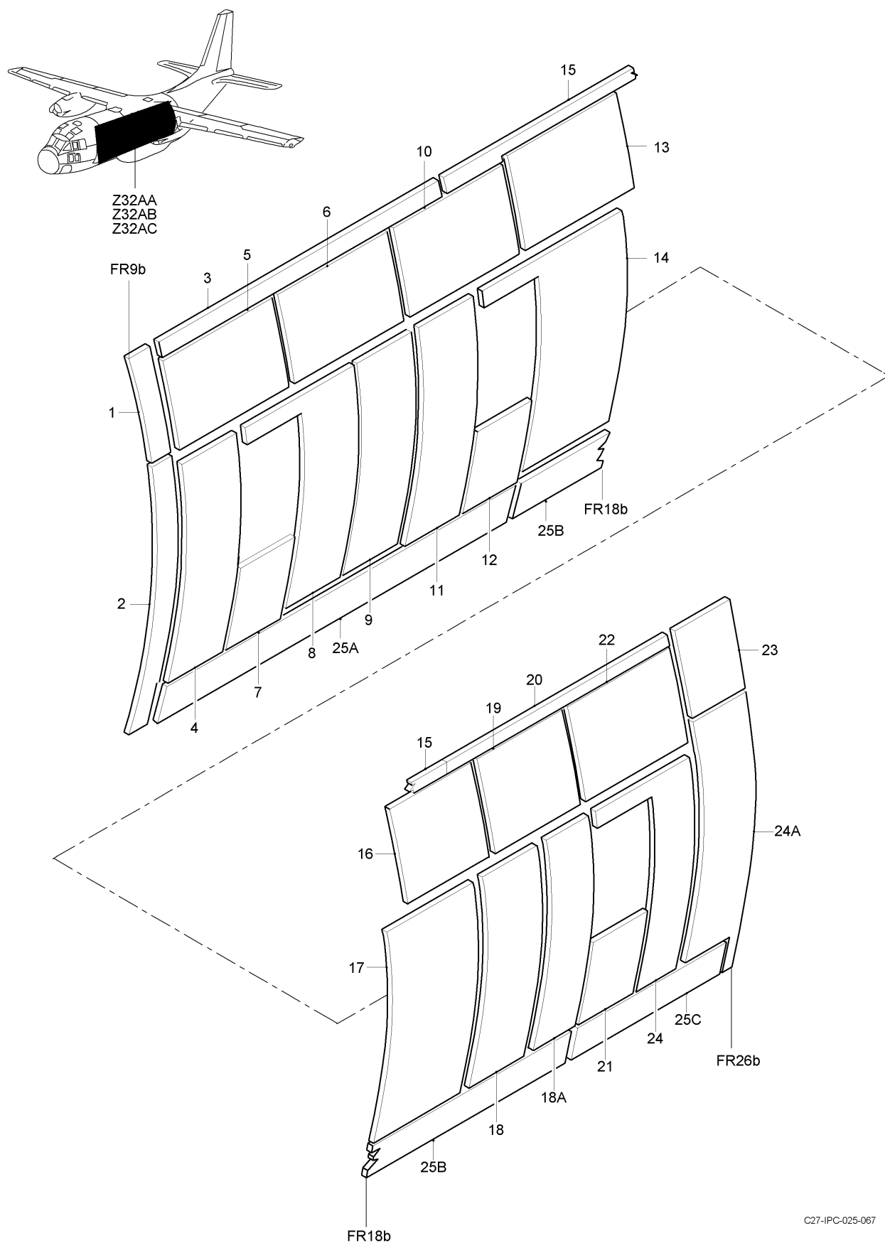
FIG 25 SECONDARY THERMAL INSULATION INSTL, Z32AA-32AB-32AC-32AD (SHEET 1 OF 3)
