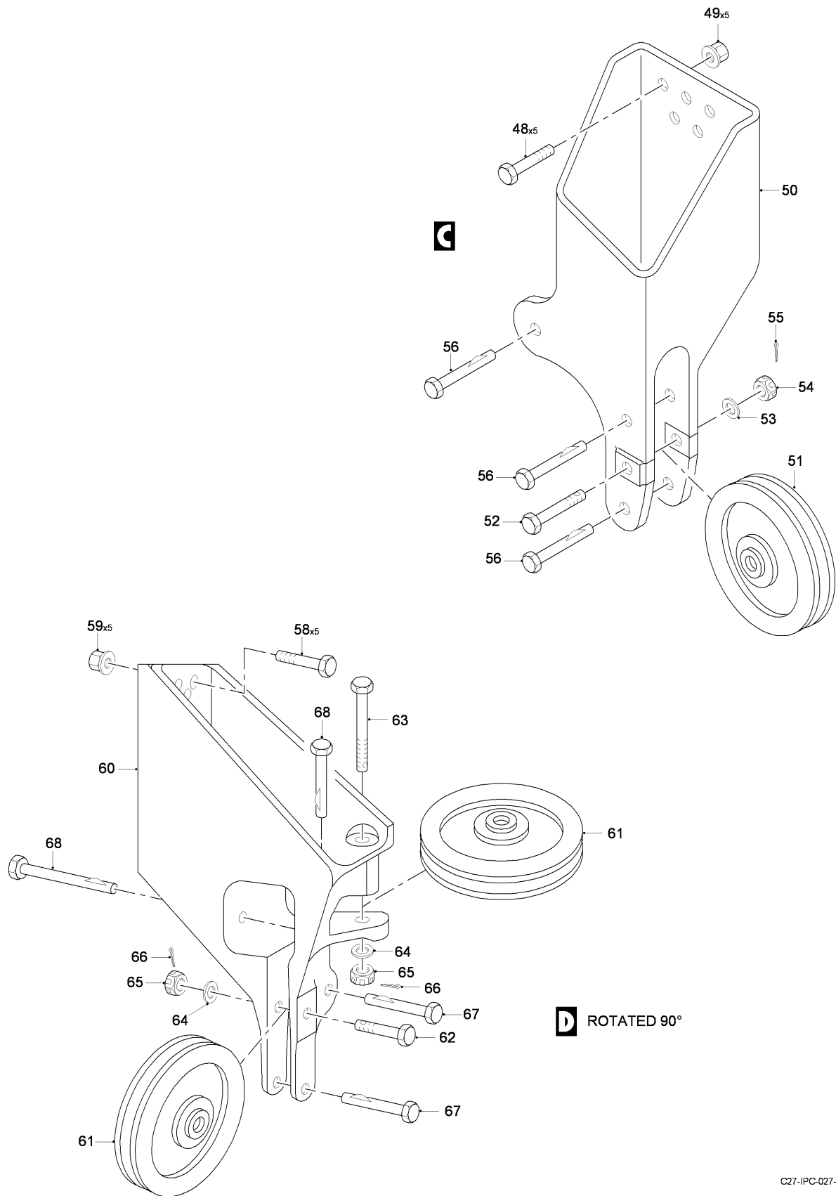
FIG 09 ELEVATOR EMERGENCY TRIM INSTL, Z34AA (SHEET 3 OF 4)
