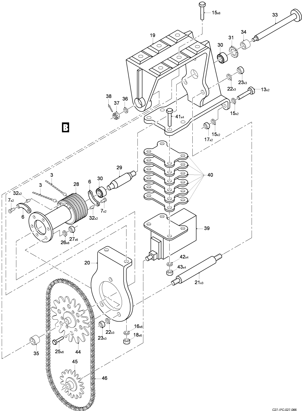
FIG 09 ELEVATOR EMERGENCY TRIM INSTL, Z34AA (SHEET 2 OF 4)
