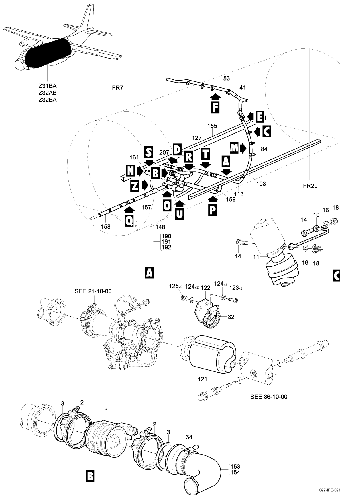
FIG 04 AIR CONDITIONING INSTL - CENTER FUSELAGE, Z32BA-32AB (SHEET 1 OF 7)
