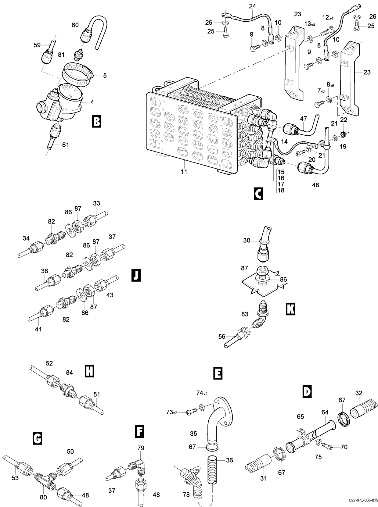
FIG 02 OXYGEN INSTL - FWD FUSELAGE, Z31AA (SHEET 2 OF 4)
