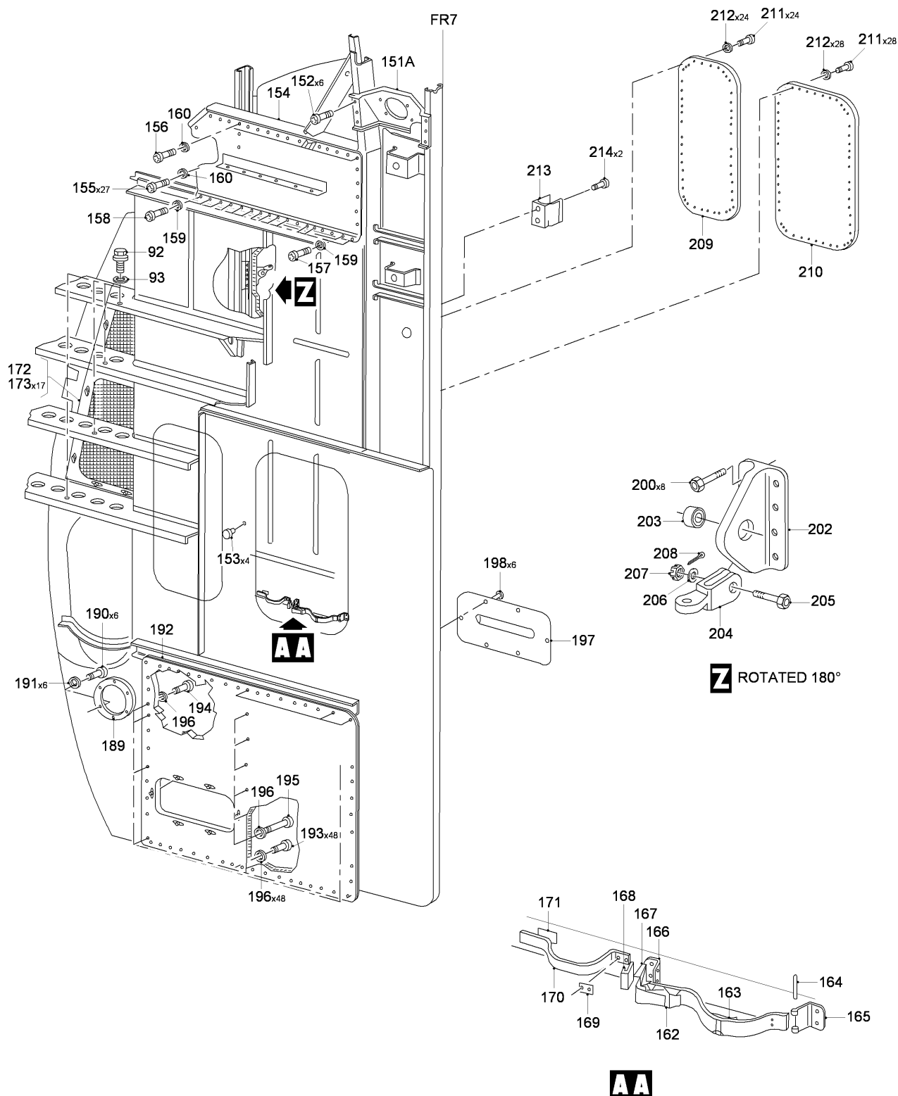
FIG 06 STRUCTURE INSTL, Z31AA (SHEET 7 OF 10)
