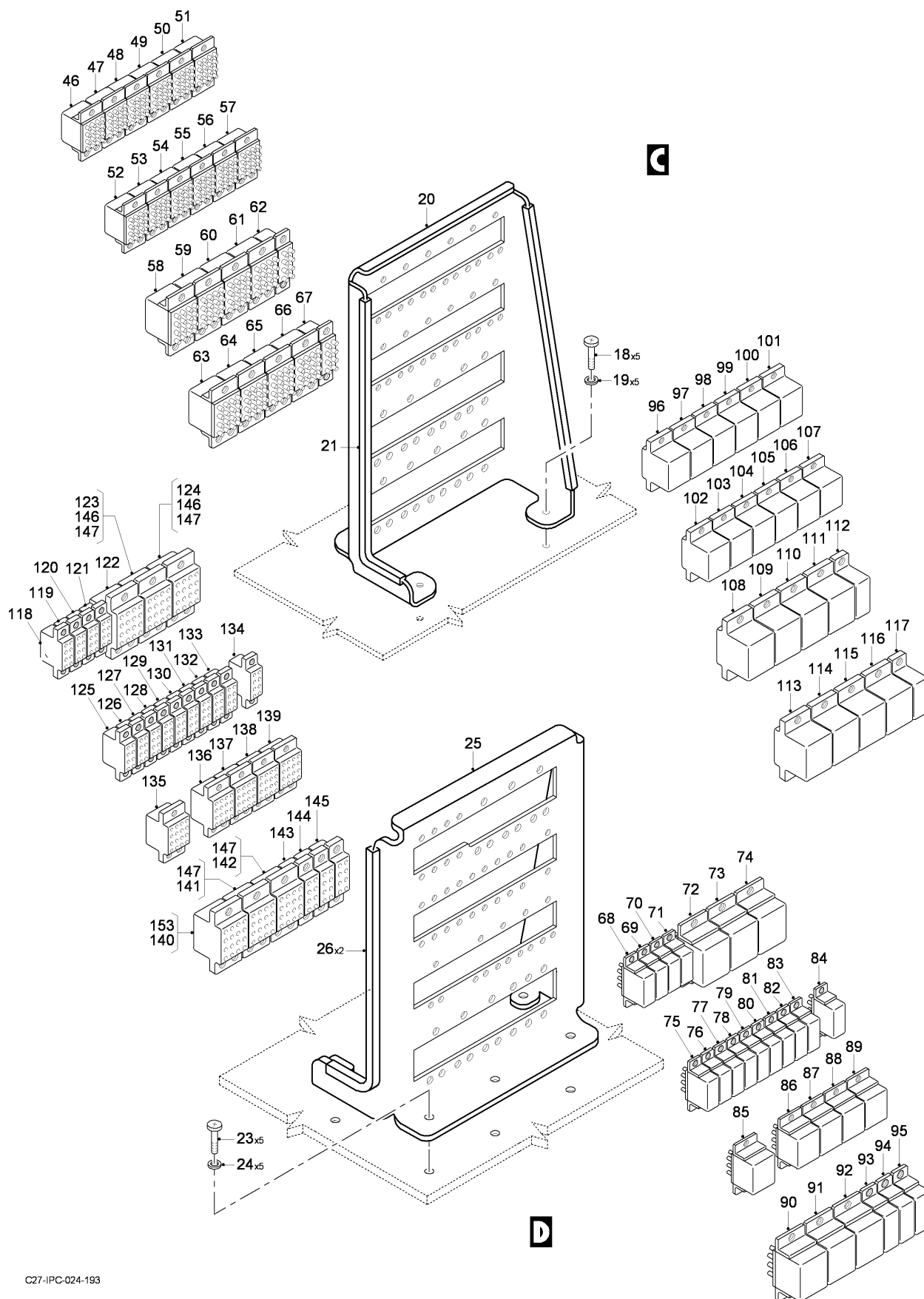
FIG 10 FOURTH SHELF INSTL - ELECTRICAL COMPARTMENT, Z31AA (SHEET 2 OF 4)
