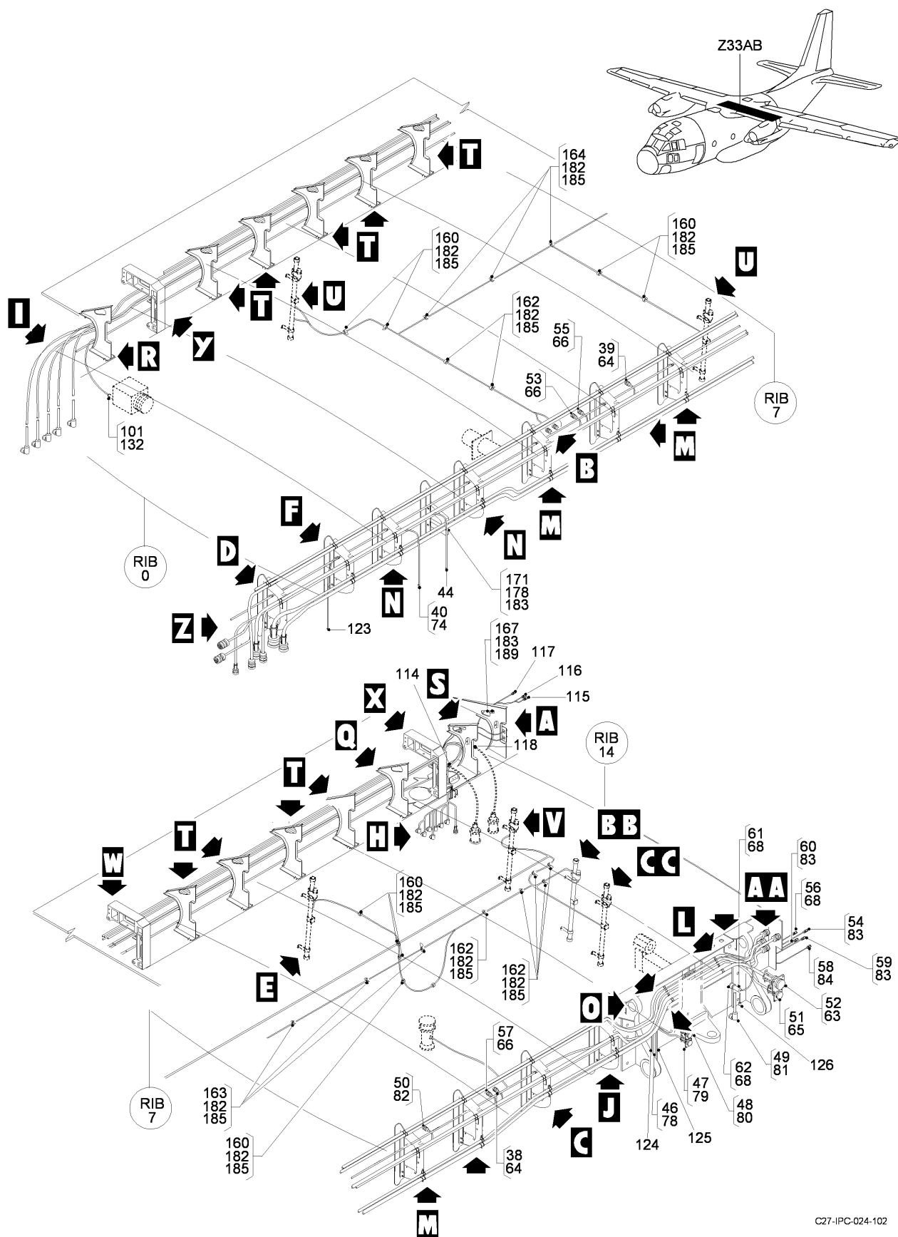
FIG 22 ELECTRICAL AND ELECTRONICS INSTL - CENTER WING, Z33AB, LH (SHEET 1 OF 7)
