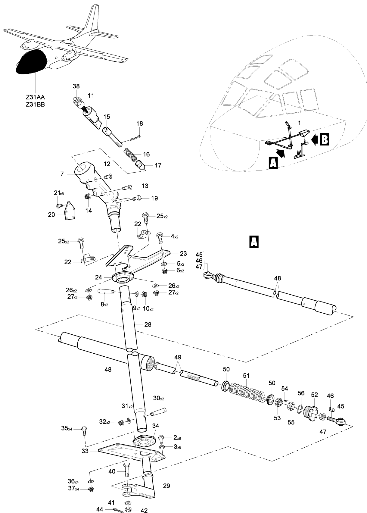
FIG 01 STEERING CONTROLS INSTL, Z31AA-31BB (SHEET 1 OF 2)
