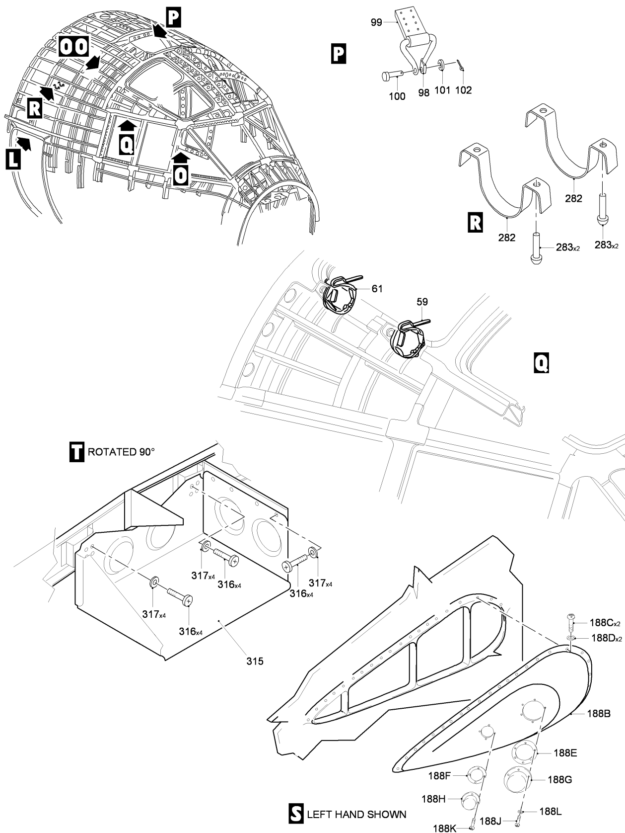
FIG 06 STRUCTURE INSTL, Z31AA (SHEET 4 OF 10)
