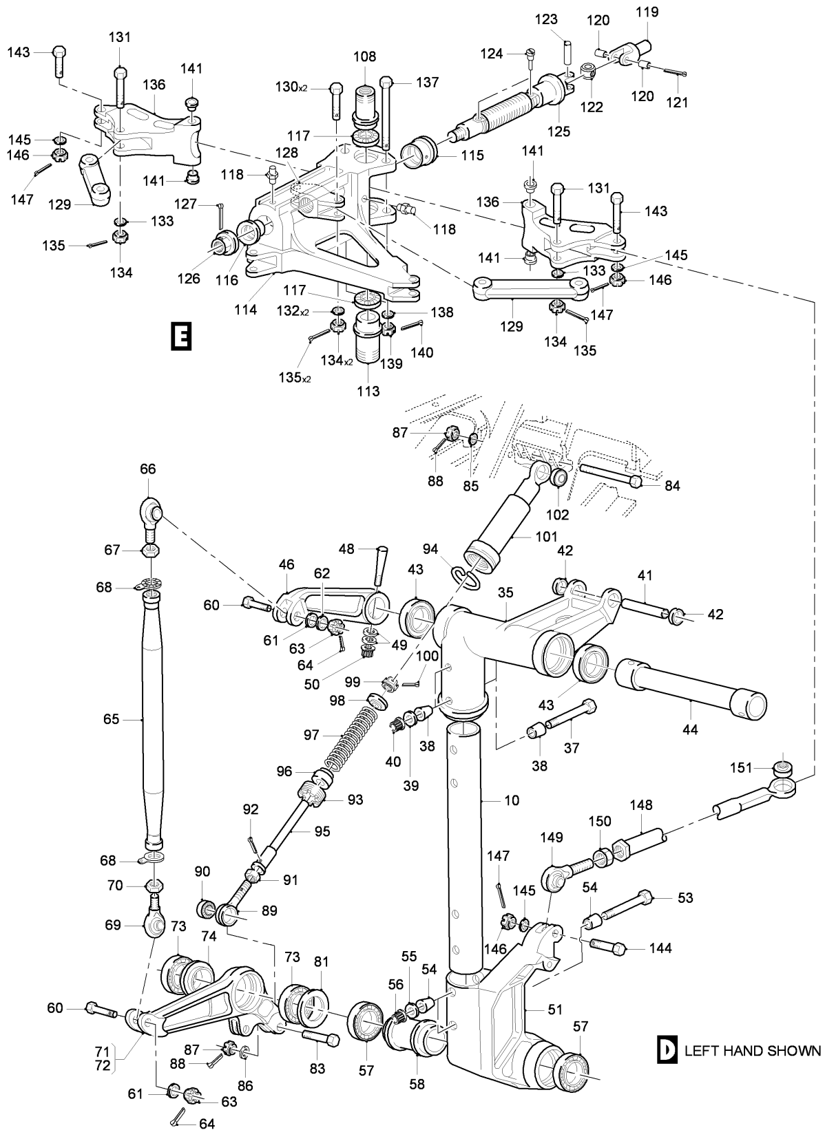
FIG 02 RUDDER PEDAL INSTL, Z31AA-31BC, LH-RH (SHEET 2 OF 2)
