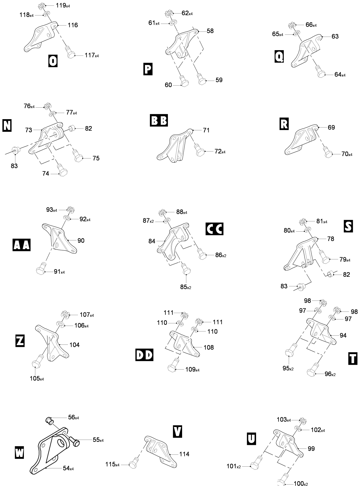
FIG 04 SUPPORT INSTL, Z32BA (SHEET 2 OF 2)
