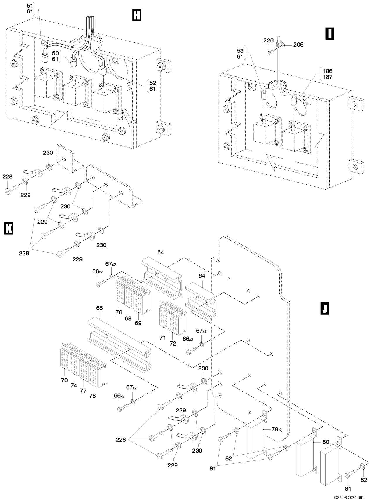
FIG 15 ELECTRICAL AND ELECTRONICS INSTL, Z31AB-32AA-32AB-32AC, LH (SHEET 5 OF 9)
