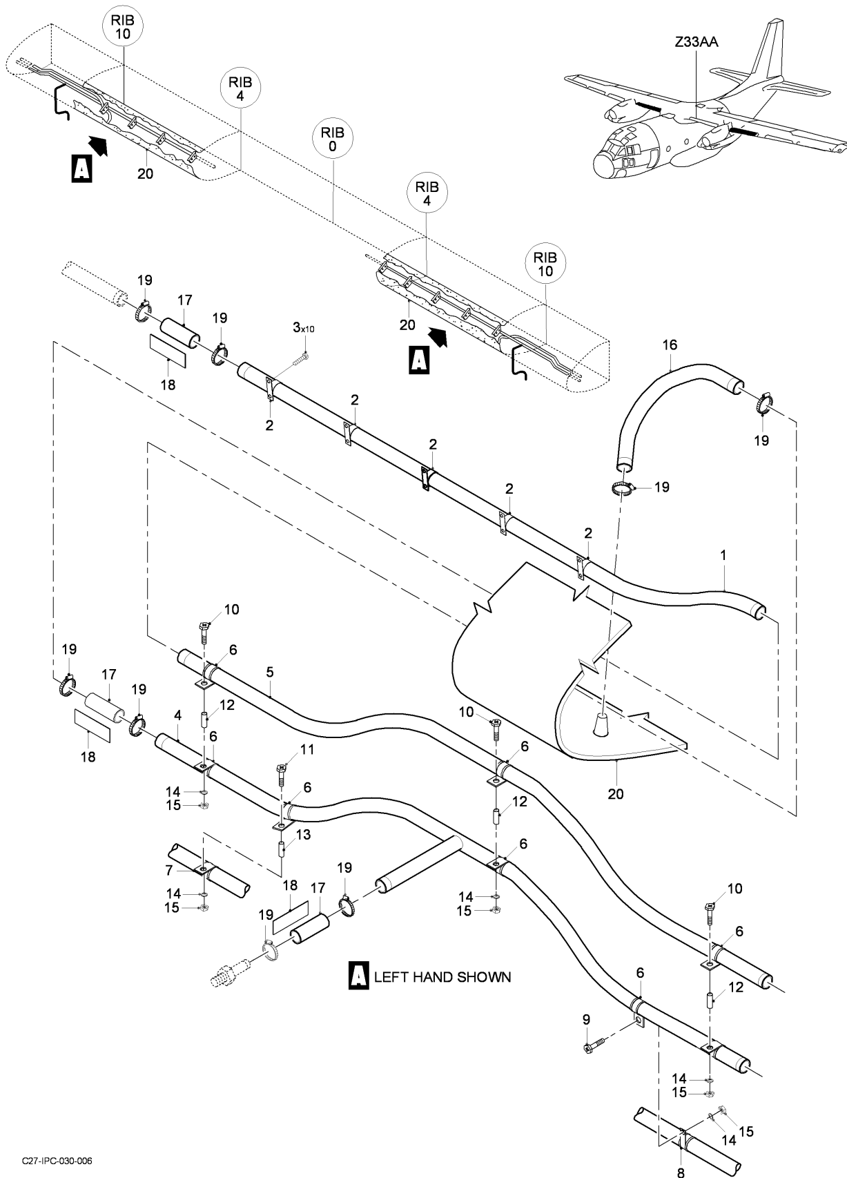
FIG 06 ANTI-ICING INSTL - CENTER WING, Z33AA, LH-RH (SHEET 1 OF 1)
