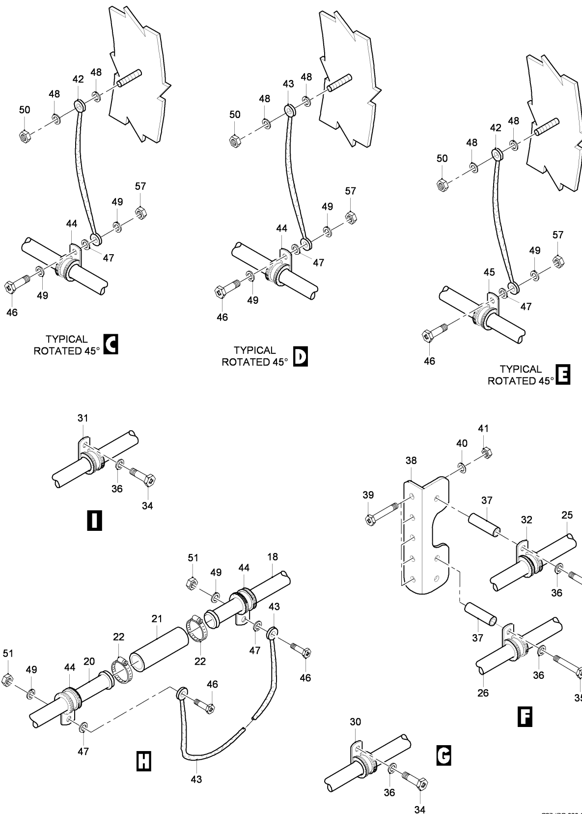
FIG 08 ANTI-ICING INSTL - OUTER WING, Z21AA, RH (SHEET 3 OF 3)
