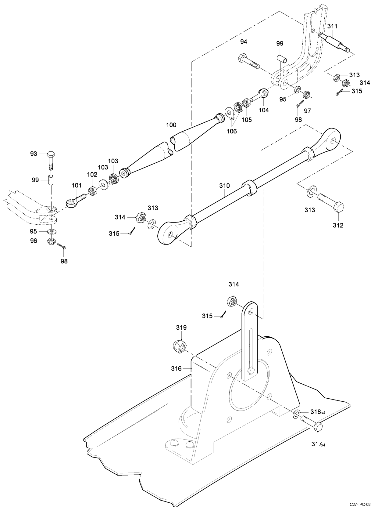
FIG 07 ELEVATOR CONTROLS INSTL, Z34AA (SHEET 8 OF 8)
