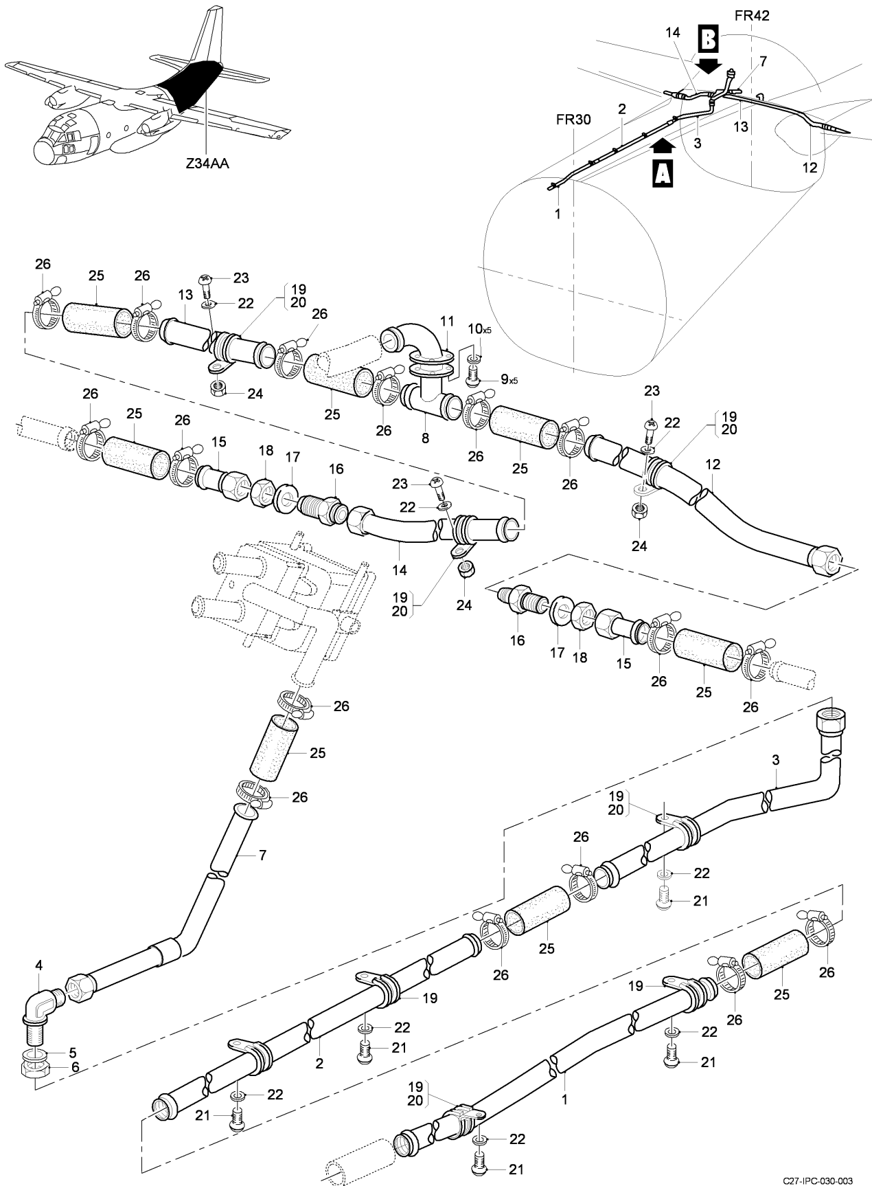
FIG 03 ANTI-ICING INSTL - REAR FUSELAGE, Z34AA (SHEET 1 OF 1)
