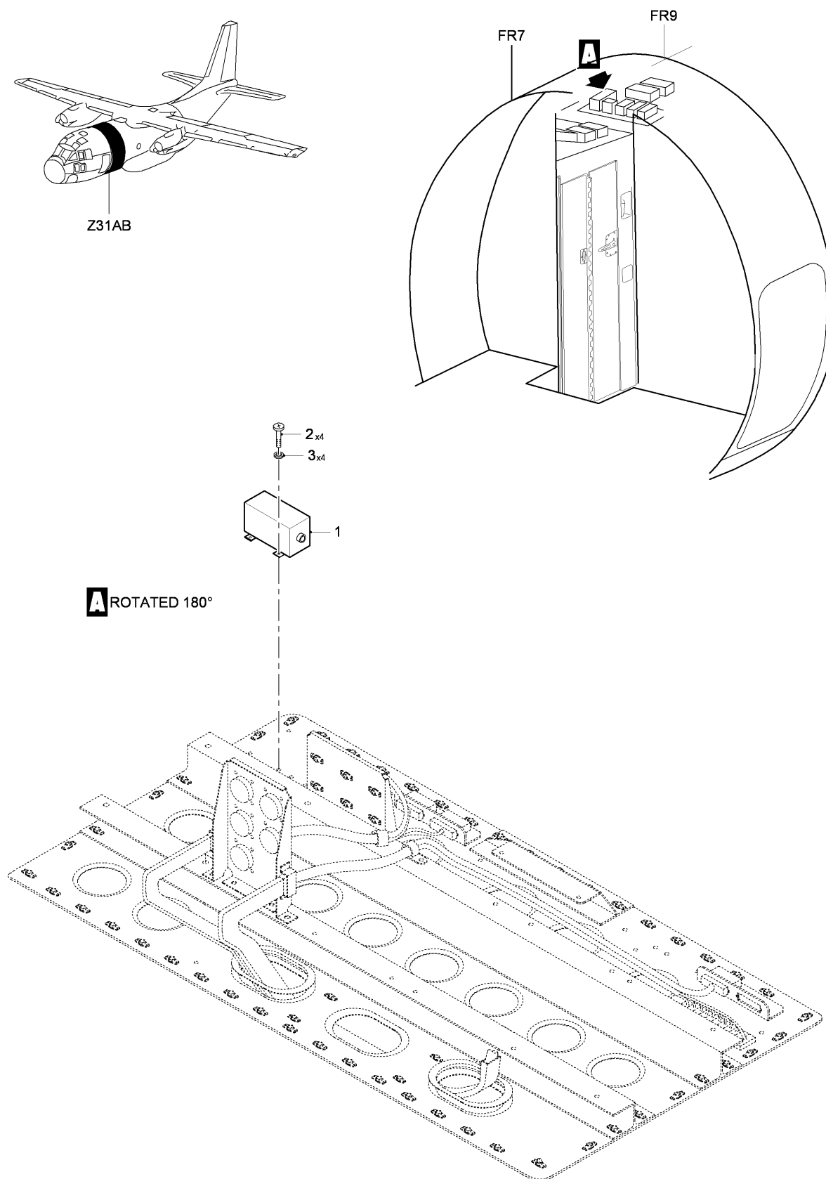
FIG 04 FLASHER INSTL, NAVIGATION LIGHT, Z31AB (SHEET 1 OF 1)
