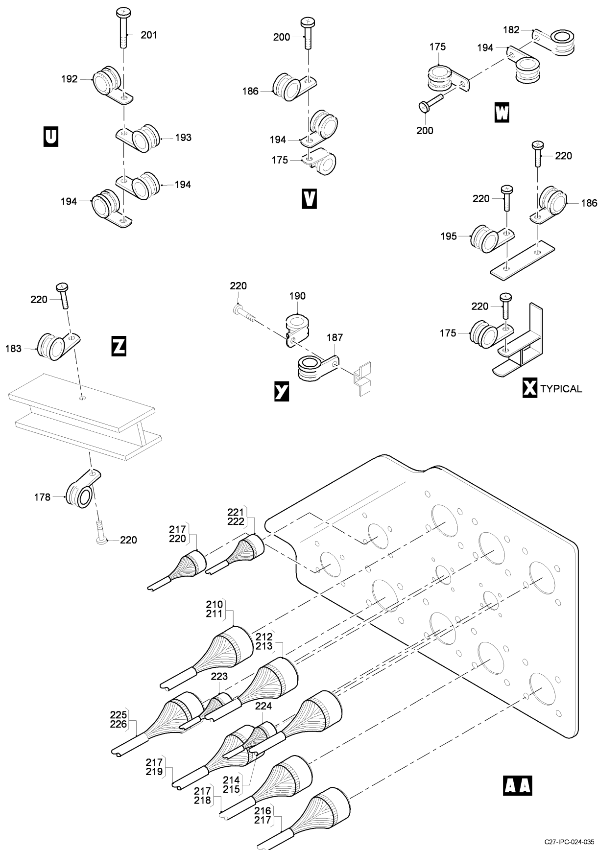
FIG 09 ELECTRICAL AND ELECTRONICS INSTL, Z31AA-31BC, RH (SHEET 7 OF 7)
