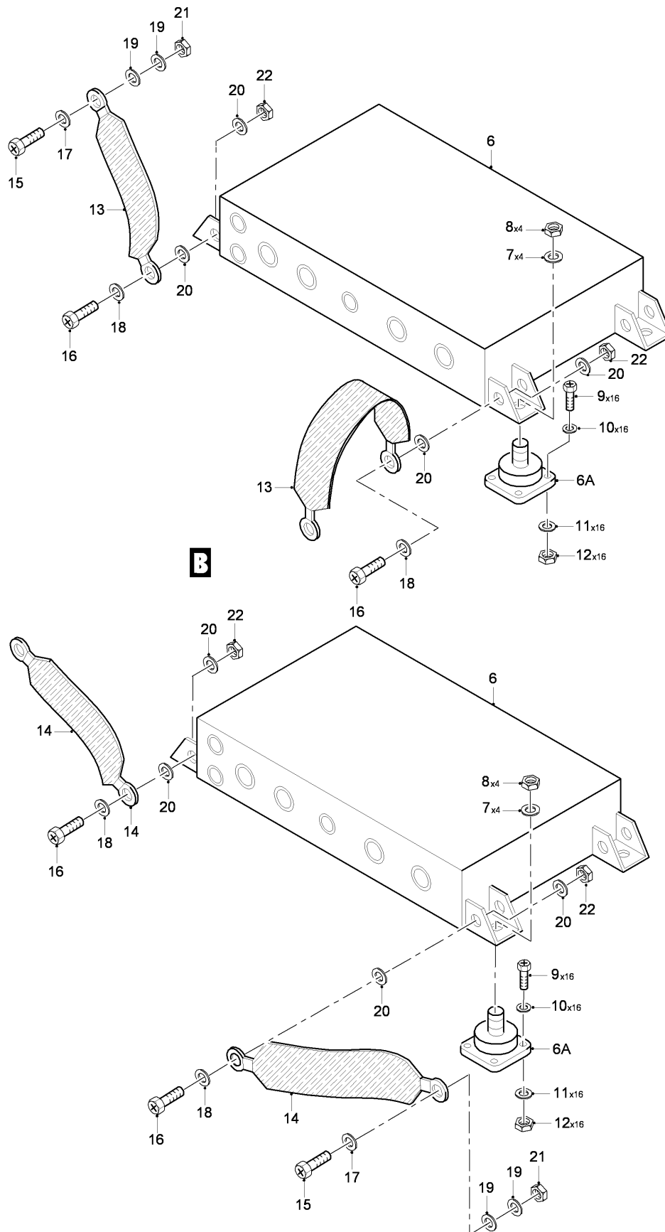
FIG 03 NIU AND FADEC INSTL, Z12AC-22AC (SHEET 2 OF 2)
