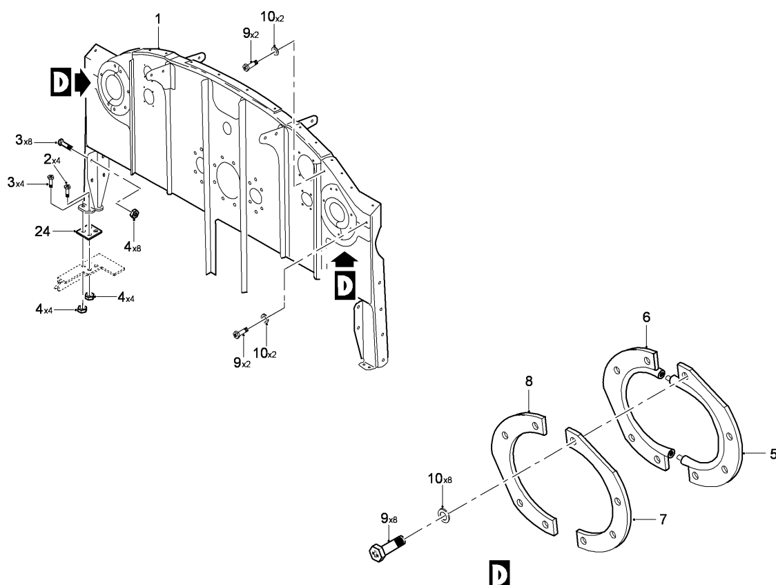
FIG 01 FIREWALL INSTL - NACELLE ENGINE, Z12AB-22AB (SHEET 1 OF 2)
