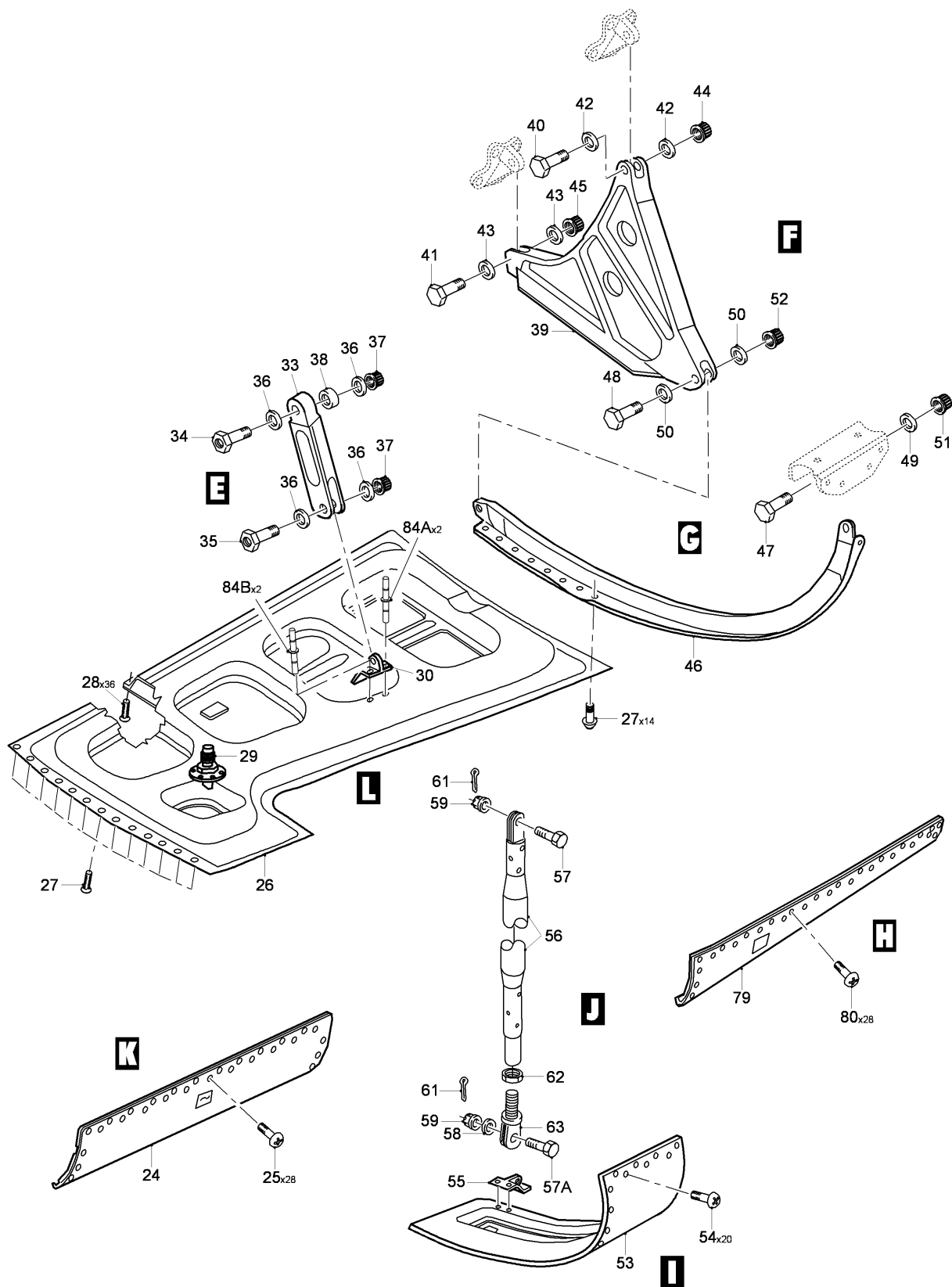
FIG 03 STRUCTURE INSTL - MLG, Z13AB, LH (SHEET 2 OF 3)
