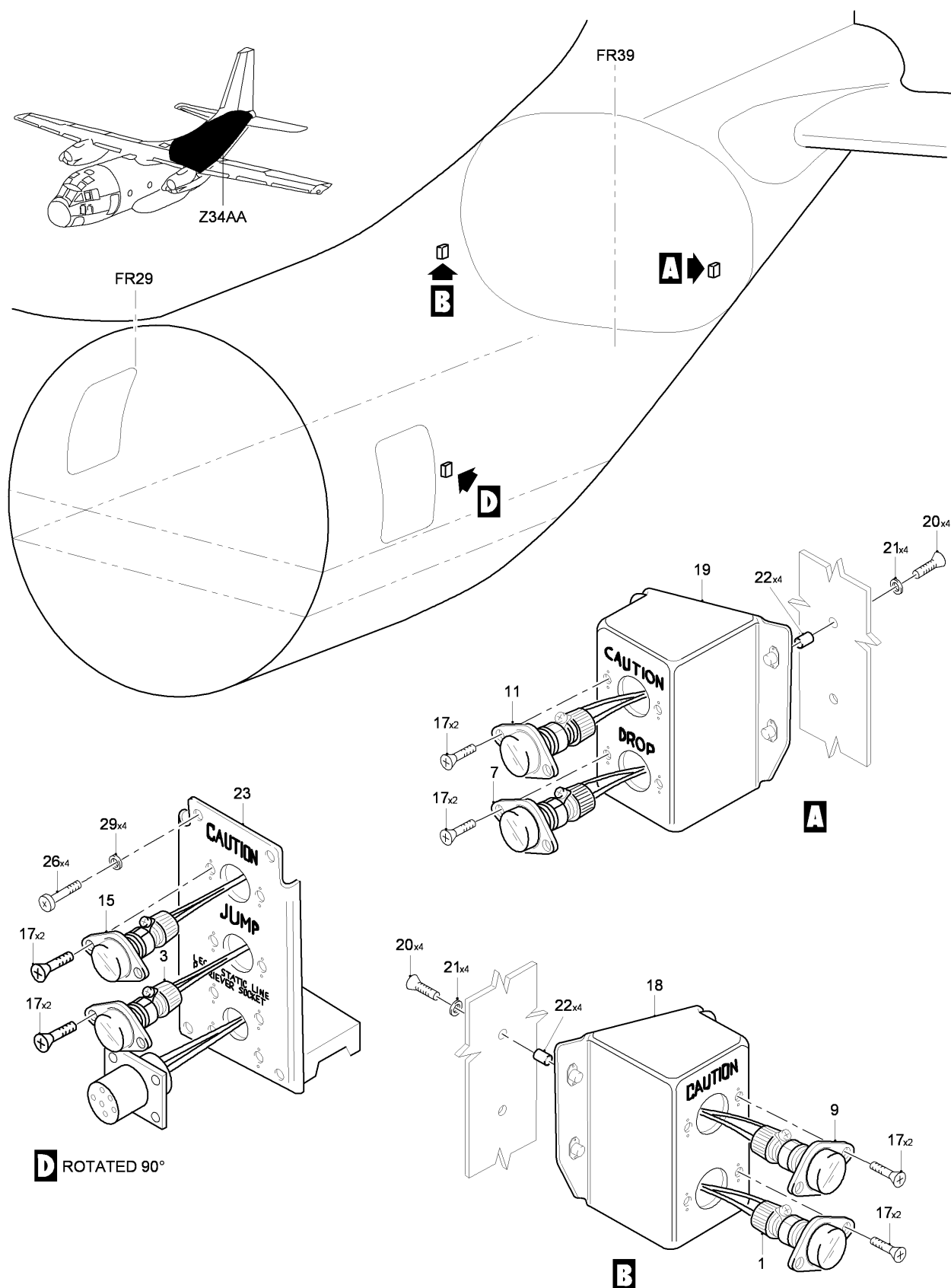
FIG 03 LIGHT CAUTION INSTL, DROP - JUMP, Z34AA (SHEET 1 OF 2)
