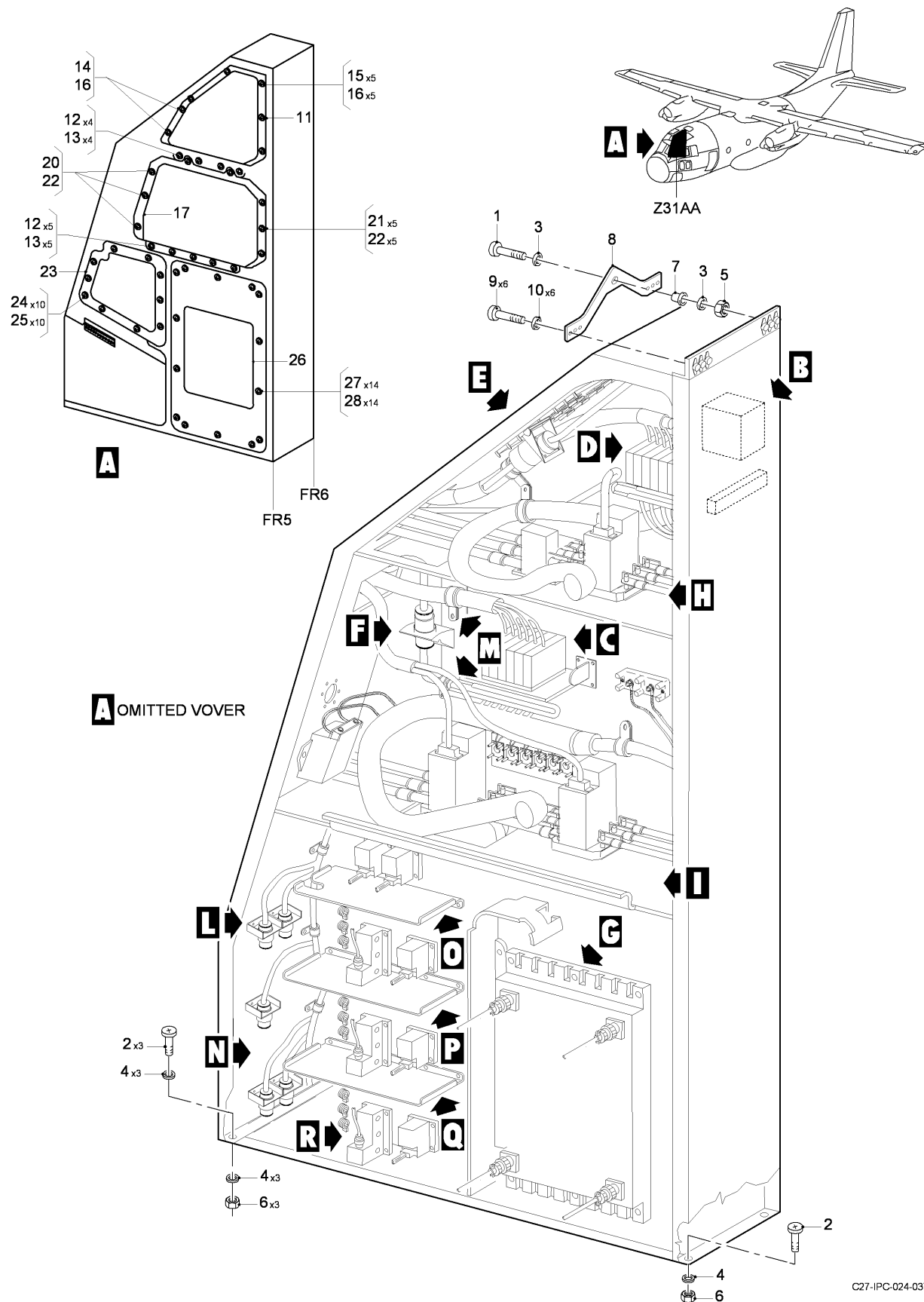
FIG 11 ELECTRICAL AND ELECTRONICS INSTL, Z31AA (SHEET 1 OF 6)
