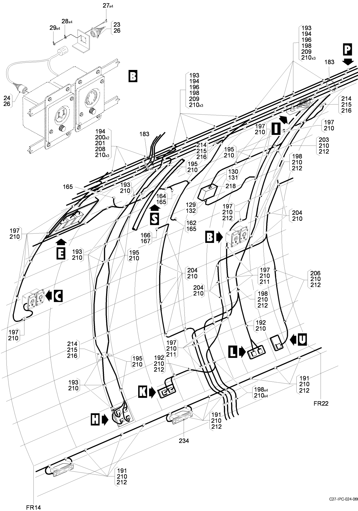
FIG 16 ELECTRICAL AND ELECTRONICS INSTL, Z31AB-32AA-32AB-32AC, RH (SHEET 2 OF 8)
