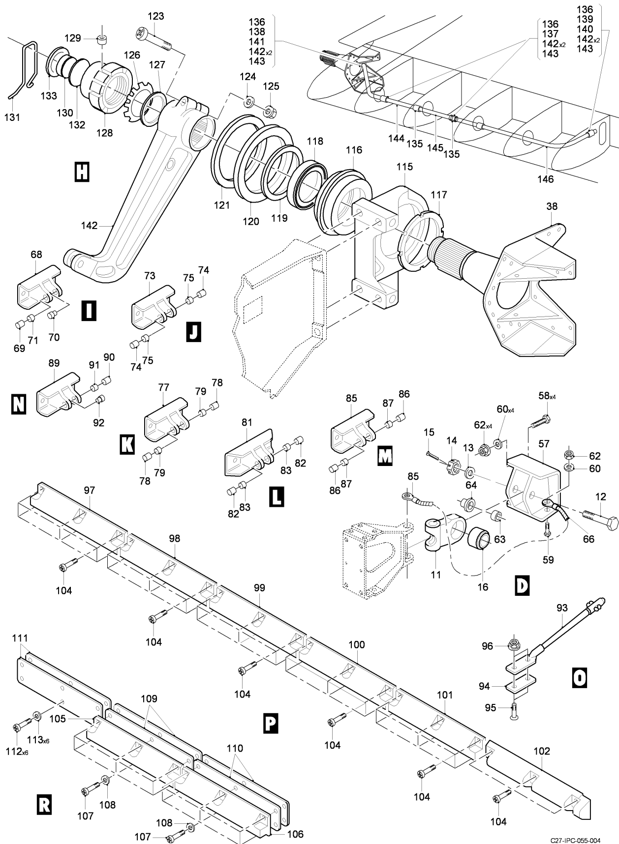
FIG 01 ELEVATOR CONTROL STRUCTURE INSTL, Z14AB-24AB, LH-RH (SHEET 2 OF 2)
