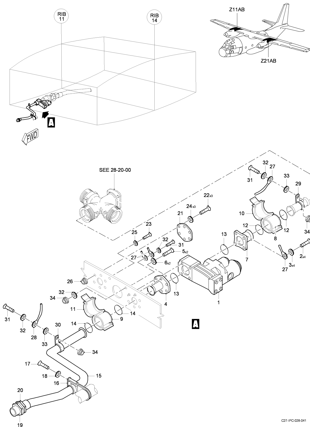
FIG 09 SHUT-OFF VALVE INSTL, FUEL SUPPLY, Z11AB-21AB, LH-RH (SHEET 1 OF 1)
