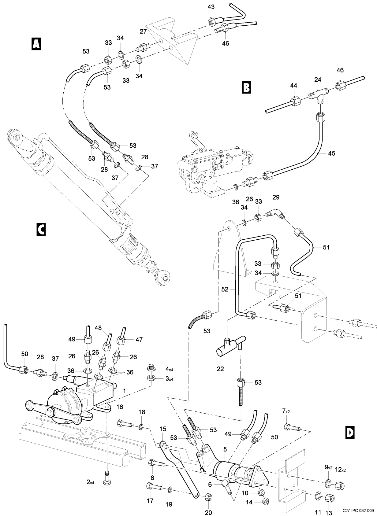
FIG 06 HYDRAULIC COMPONENT INSTL - NLG, Z31BB (SHEET 2 OF 3)
