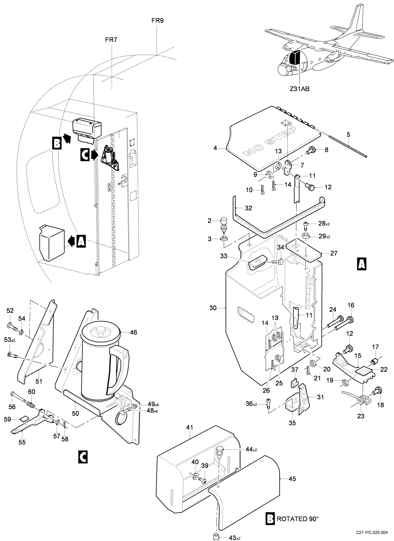
FIG 01 CONTAINER REFUSE AND DISPENSER PAPER TOWEL INSTL, Z31AB (SHEET 1 OF 1)
