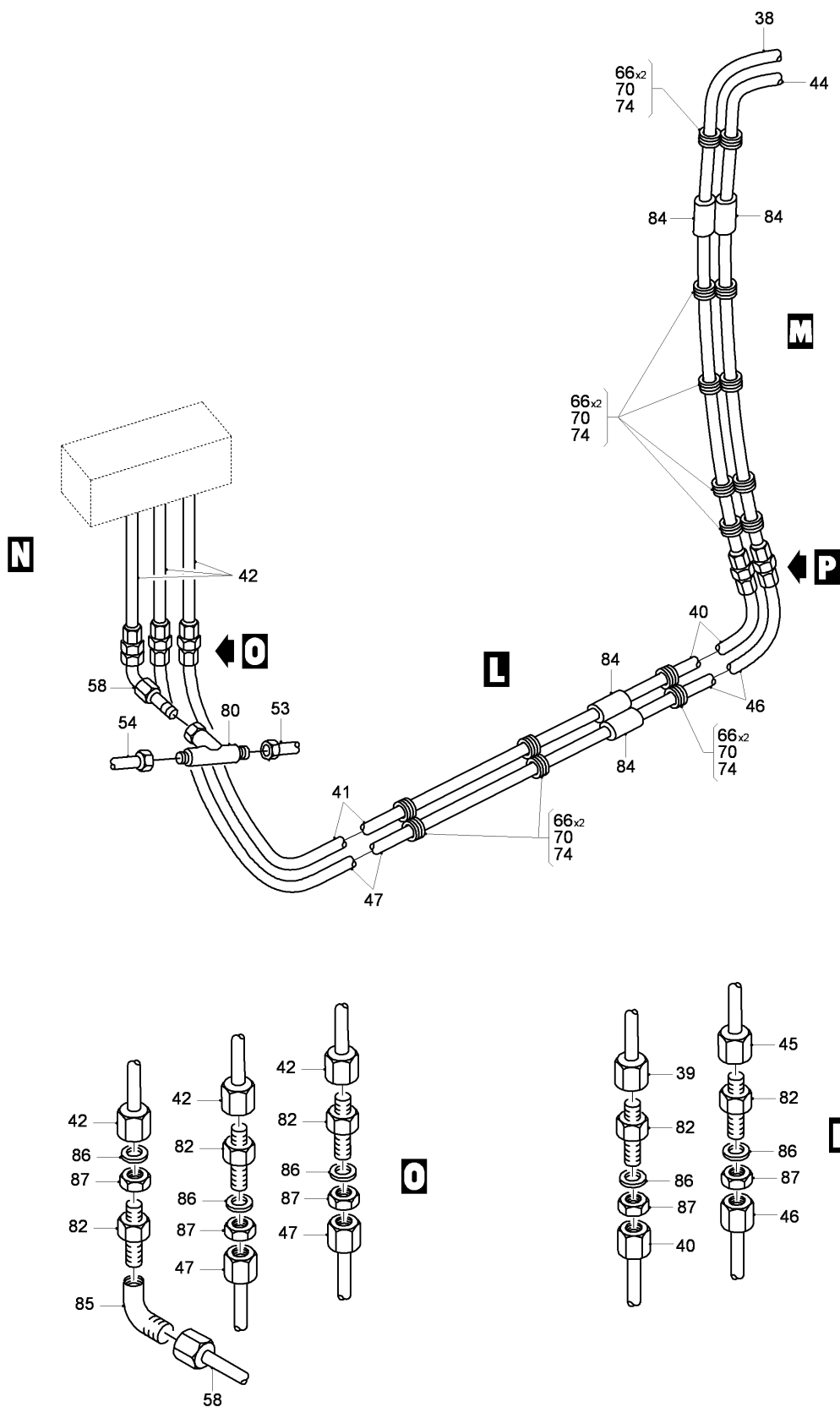
FIG 02 OXYGEN INSTL - FWD FUSELAGE, Z31AA (SHEET 3 OF 4)
