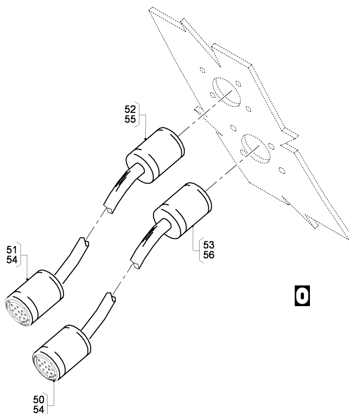
FIG 27 ELECTRICAL AND ELECTRONICS INSTL - MLG, Z23AA-23AB-23AC, RH (SHEET 5 OF 5)
