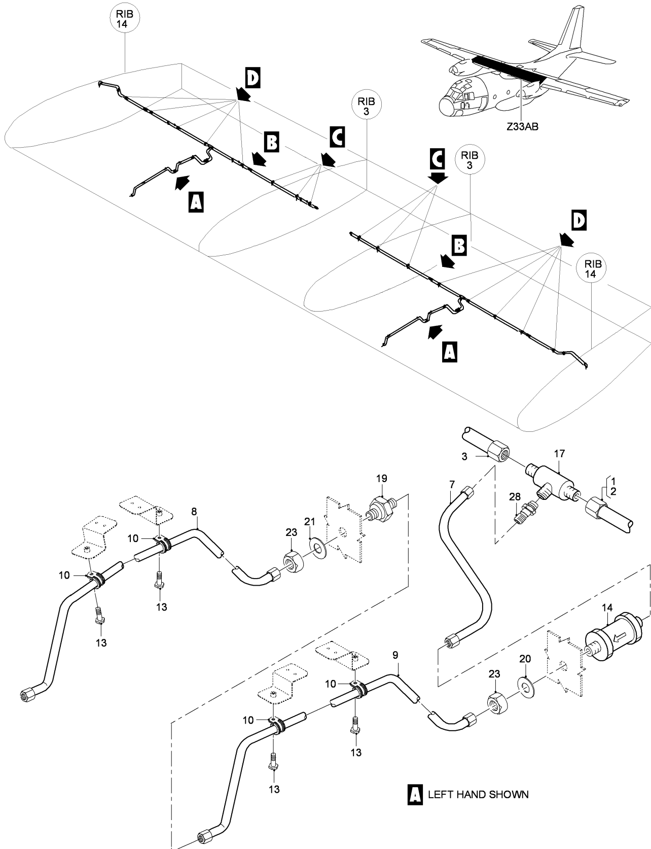
FIG 03 FUEL TANK EXPLOSION PROTECTION SYSTEM INSTL, Z33AB (SHEET 1 OF 2)
