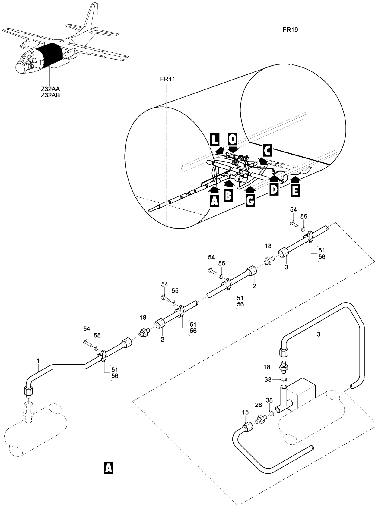
FIG 02 AIR CONDITIONING SENSITIVE LINE INSTL, Z32AA-32AB (SHEET 1 OF 4)
