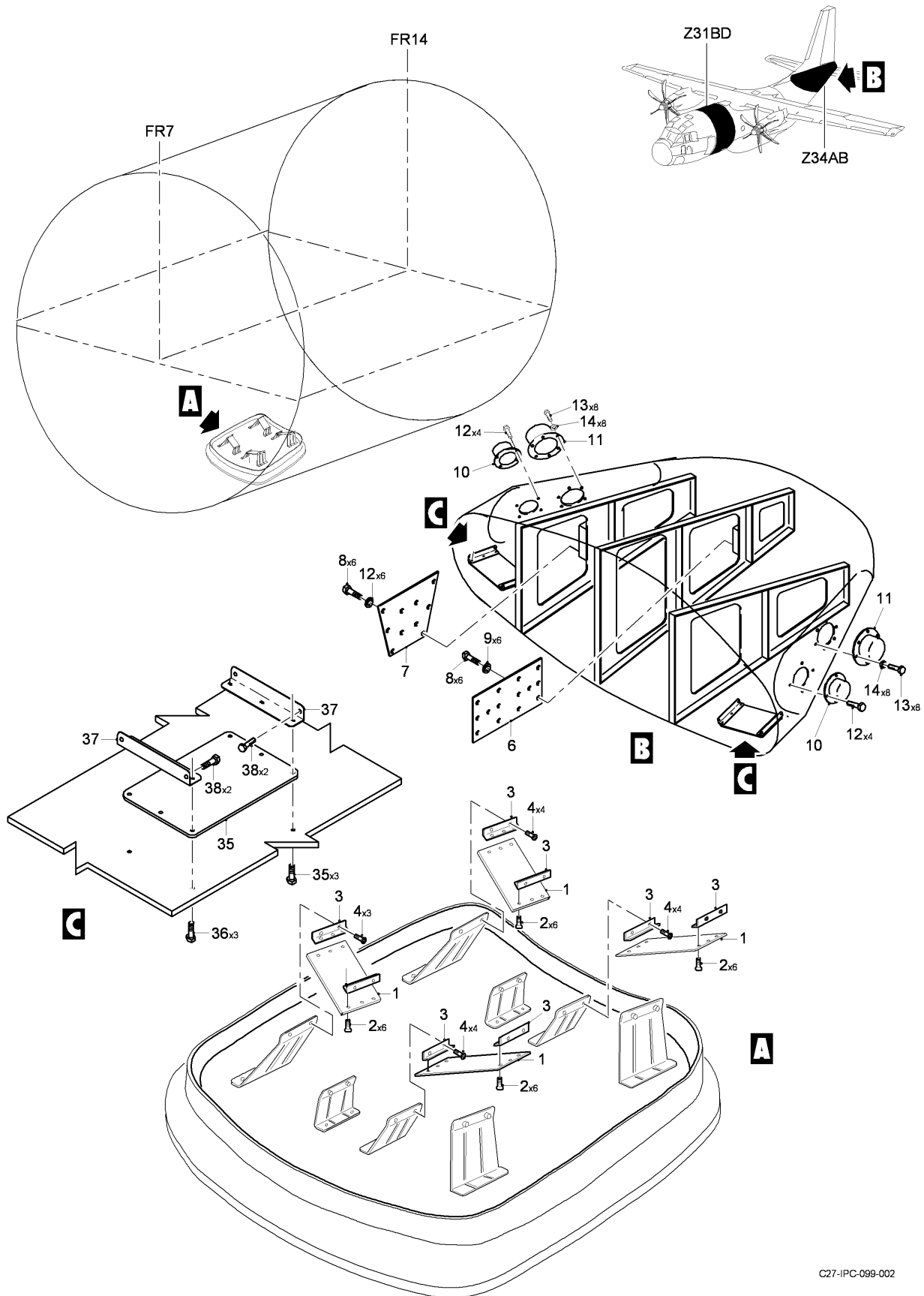
FIG 01 DASS SYSTEM, Z13AB, Z23AB, Z31BD, Z34AB (SHEET 1 OF 2)
