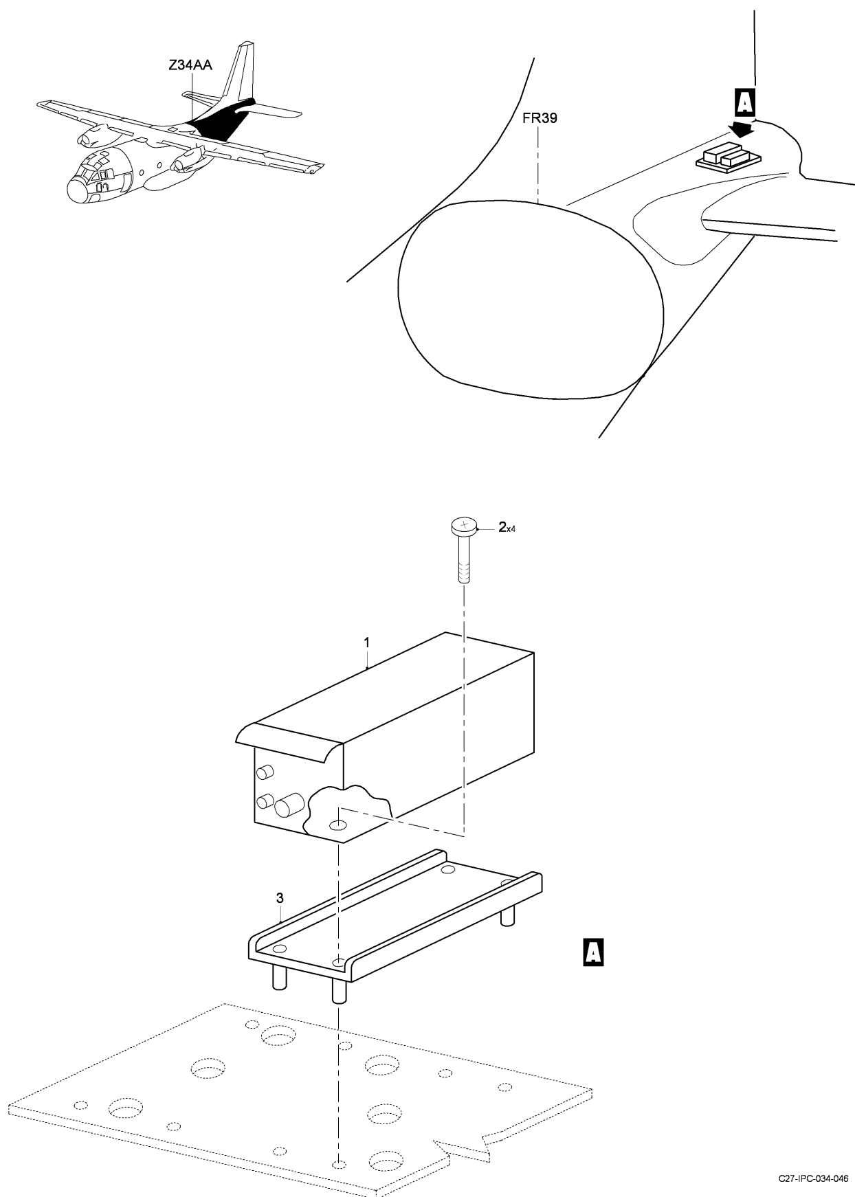
FIG 13 ADF RECEIVER INSTL, Z34AA (SHEET 1 OF 1)
