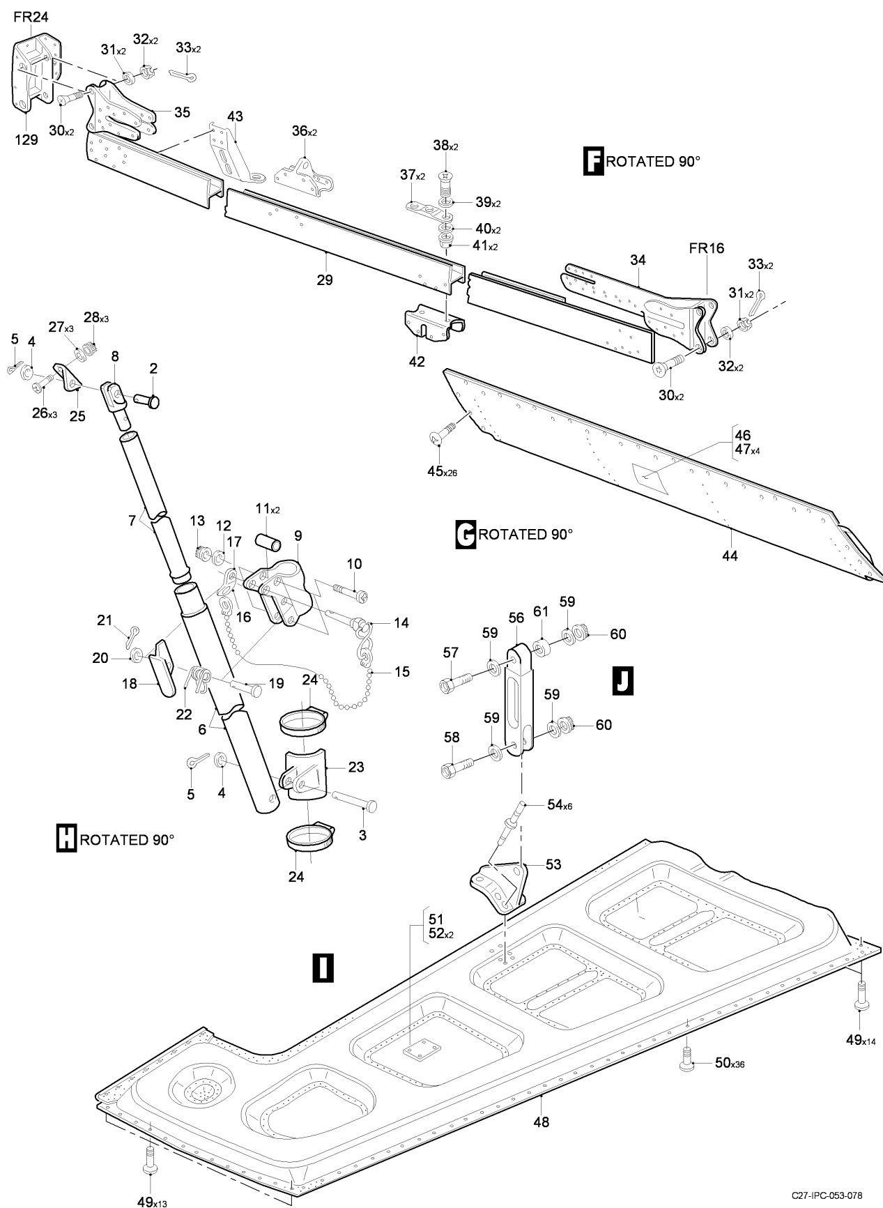
FIG 04 STRUCTURE INSTL - MLG, Z23AB, RH (SHEET 3 OF 4)
