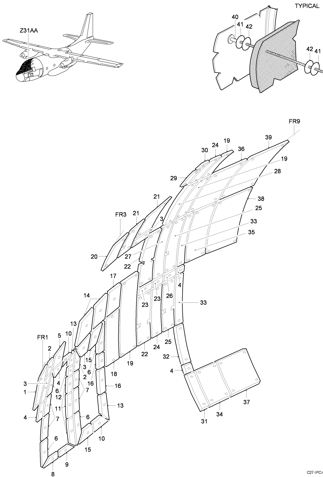
FIG 04 PRIMARY THERMAL INSULATION INSTL - RH SIDE, Z31AA-31AB (SHEET 1 OF 1)
