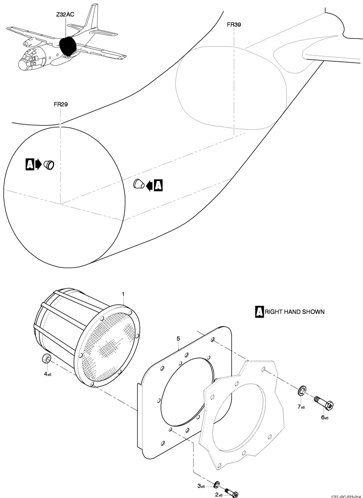
FIG 03 LOUDSPEAKER INSTL, Z32AC, LH-RH (SHEET 1 OF 1)
