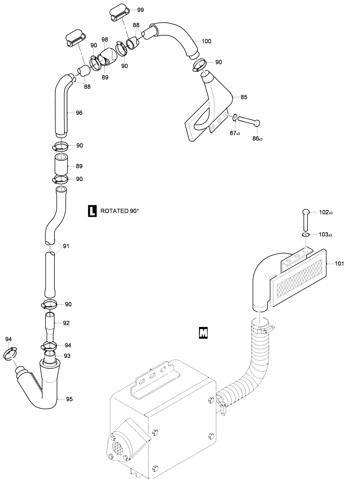
FIG 05 AIR DISTRUBUTION INSTL, Z32AA-32AB-32AC-32AD (SHEET 4 OF 4)
