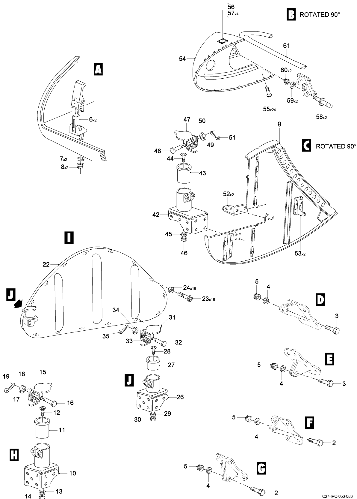
FIG 06 STRUCTURE INSTL - MLG, Z23AC, RH (SHEET 2 OF 2)
