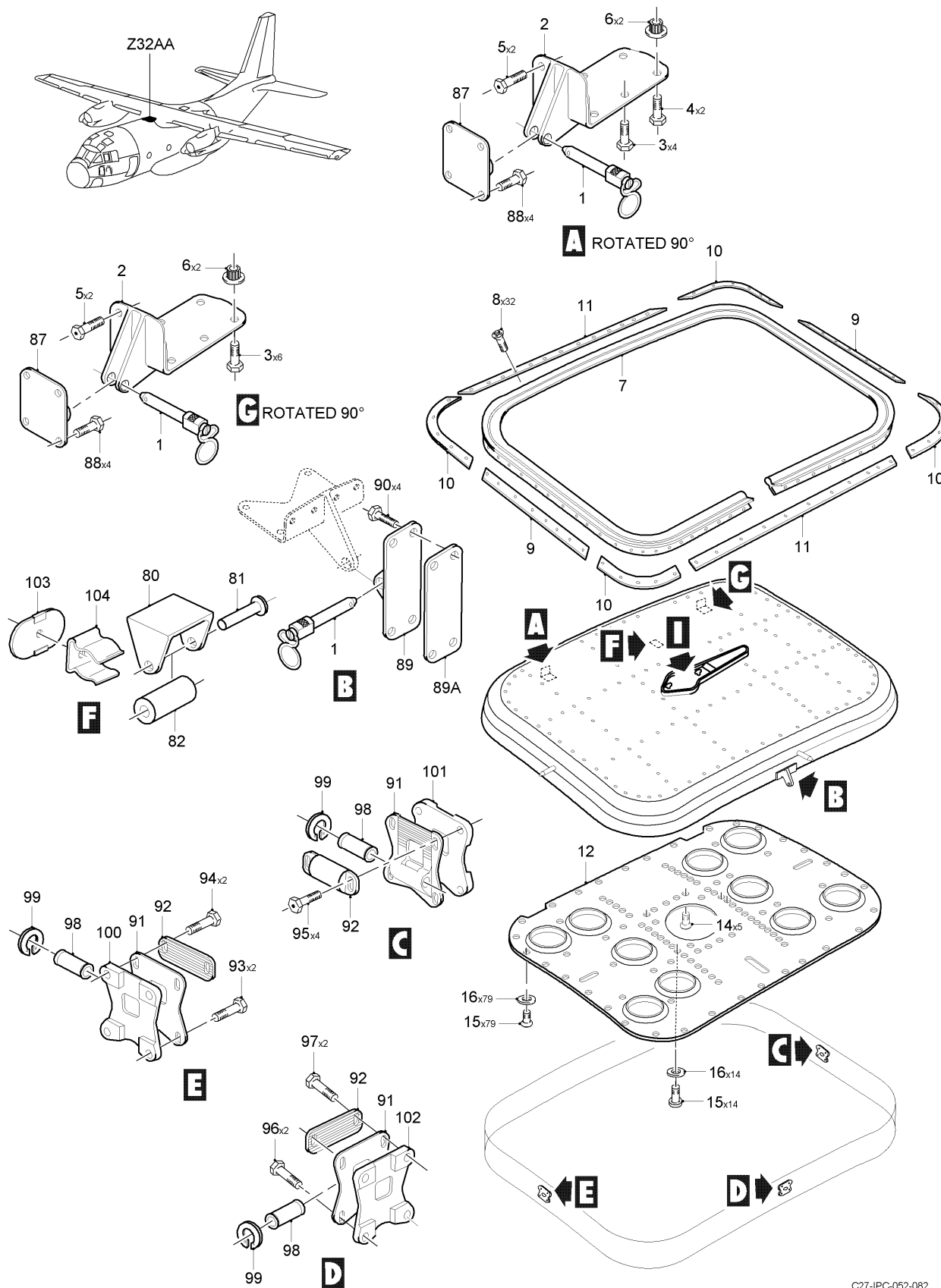
FIG 03 EMERGENCY EXIT DOOR INSTL - TOP CENTER, Z32AA (SHEET 1 OF 2)
