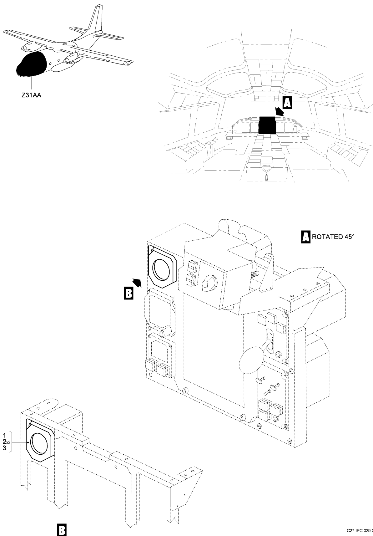
FIG 01 HYDRAULIC TRIPLE PRESSURE INDICATOR INSTL, Z31AA (SHEET 1 OF 1)
