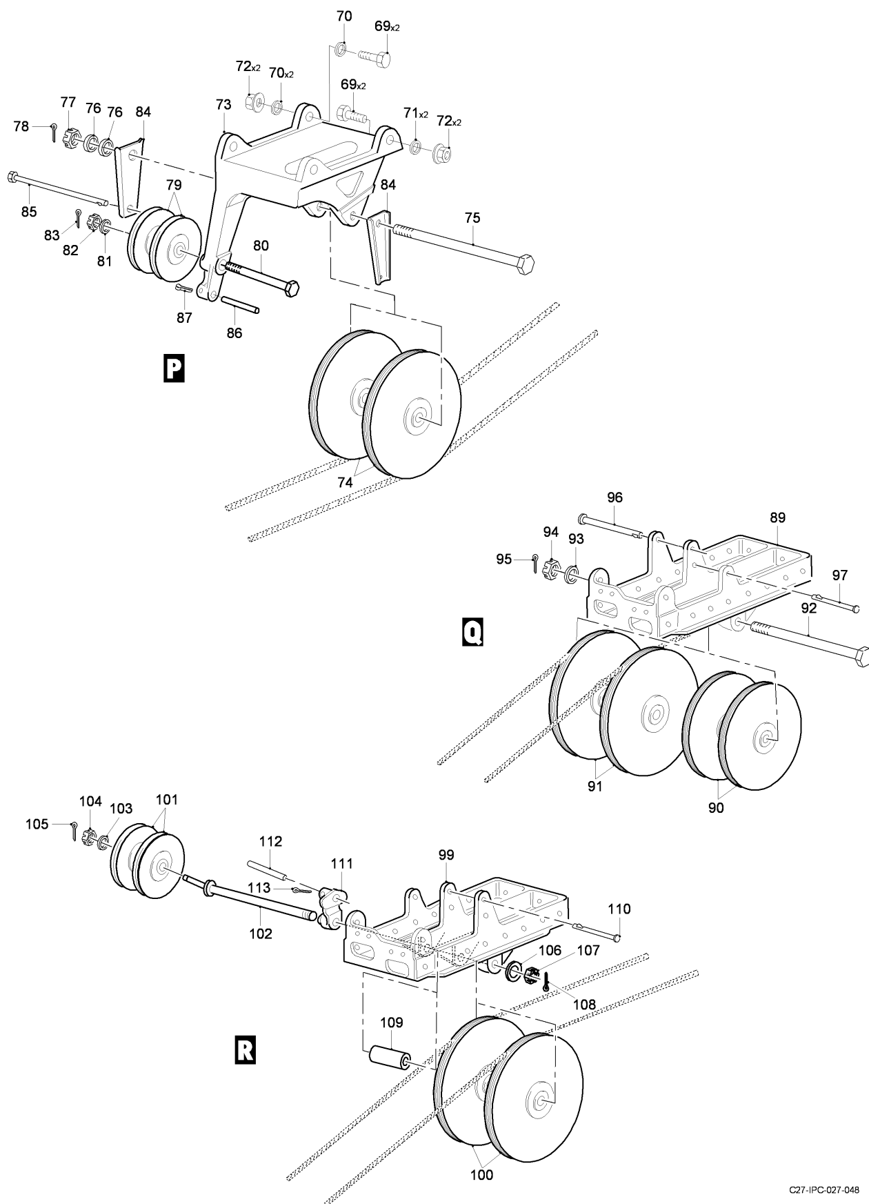
FIG 04 ELEVATOR CONTROLS INSTL, Z32AA-32AB-32AC-32AD-34AA (SHEET 4 OF 5)
