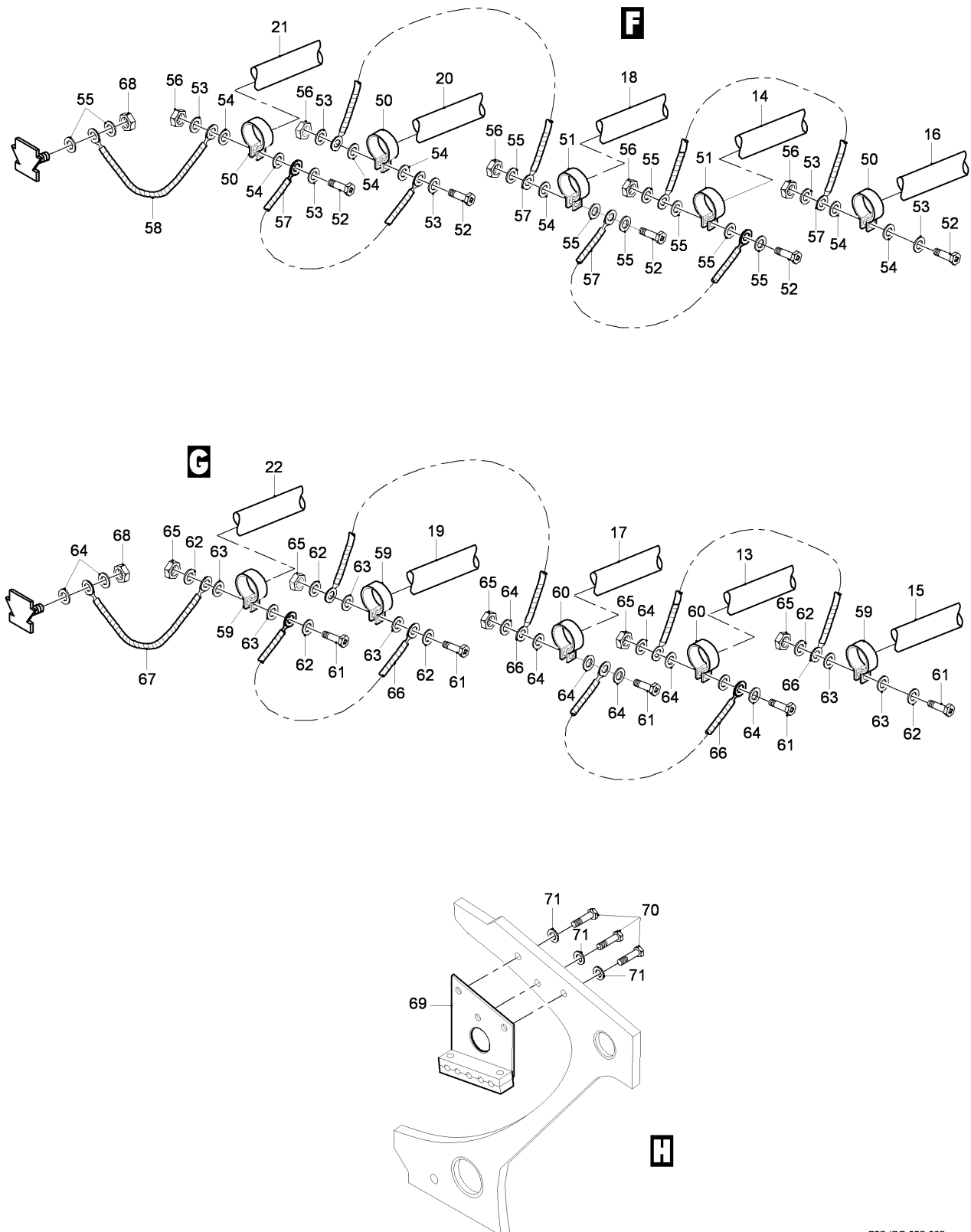
FIG 04 HYDRAULIC PIPING INSTL - SPOILER CONTROL, Z11AD, LH (SHEET 3 OF 3)
