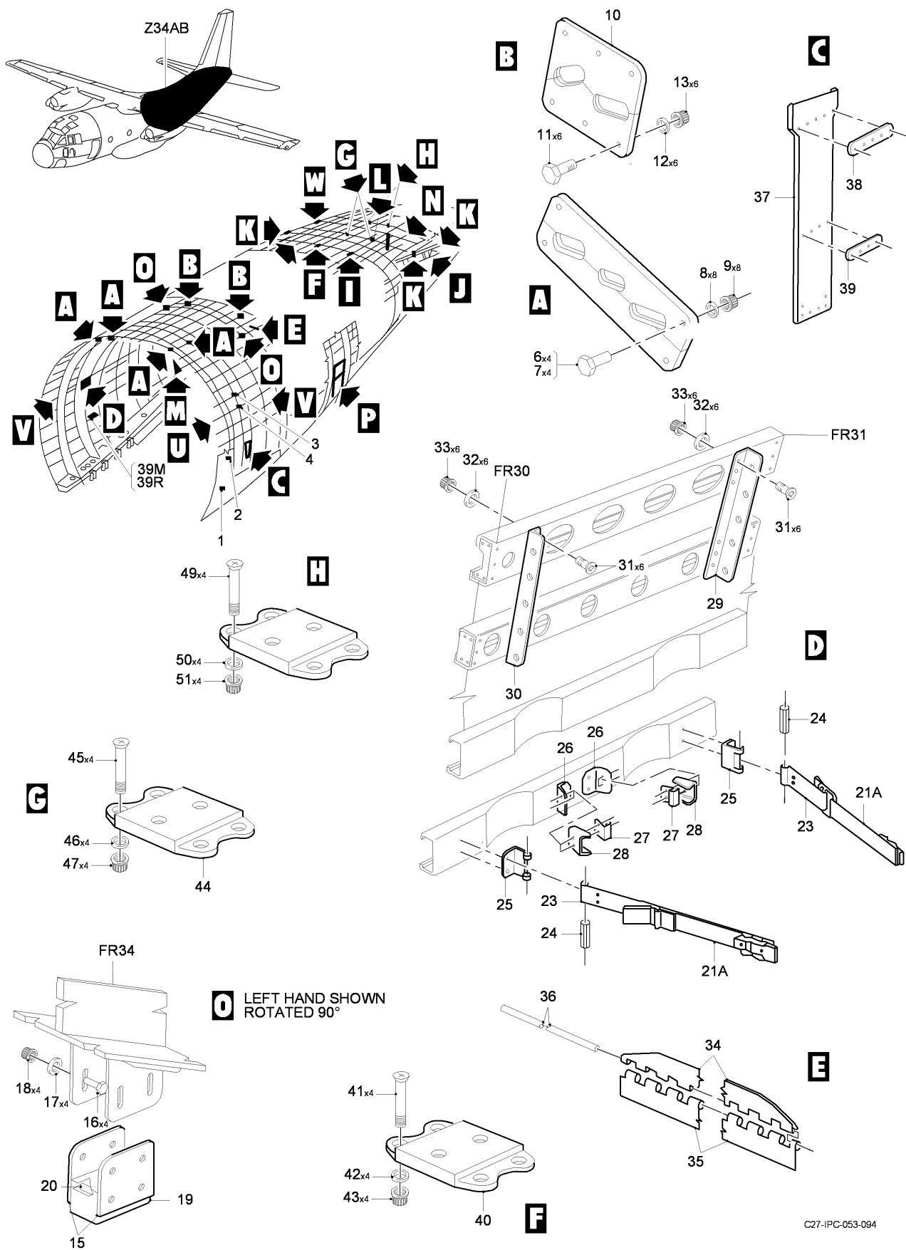
FIG 02 STRUCTURE INSTL, Z34AA (SHEET 1 OF 4)
