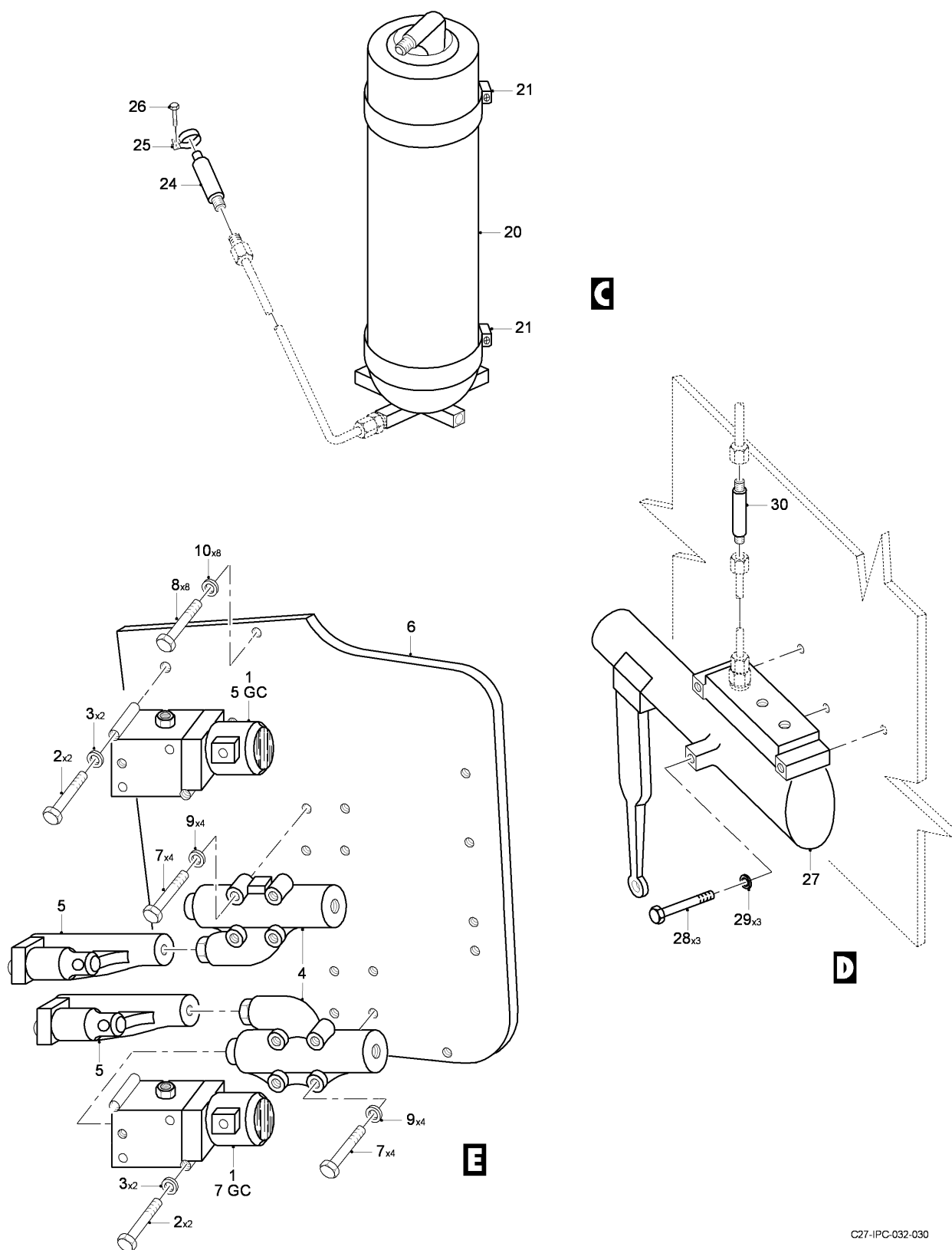
FIG 06 HYDRAULIC COMPONENT INSTL - MLG, Z13AB (SHEET 2 OF 2)
