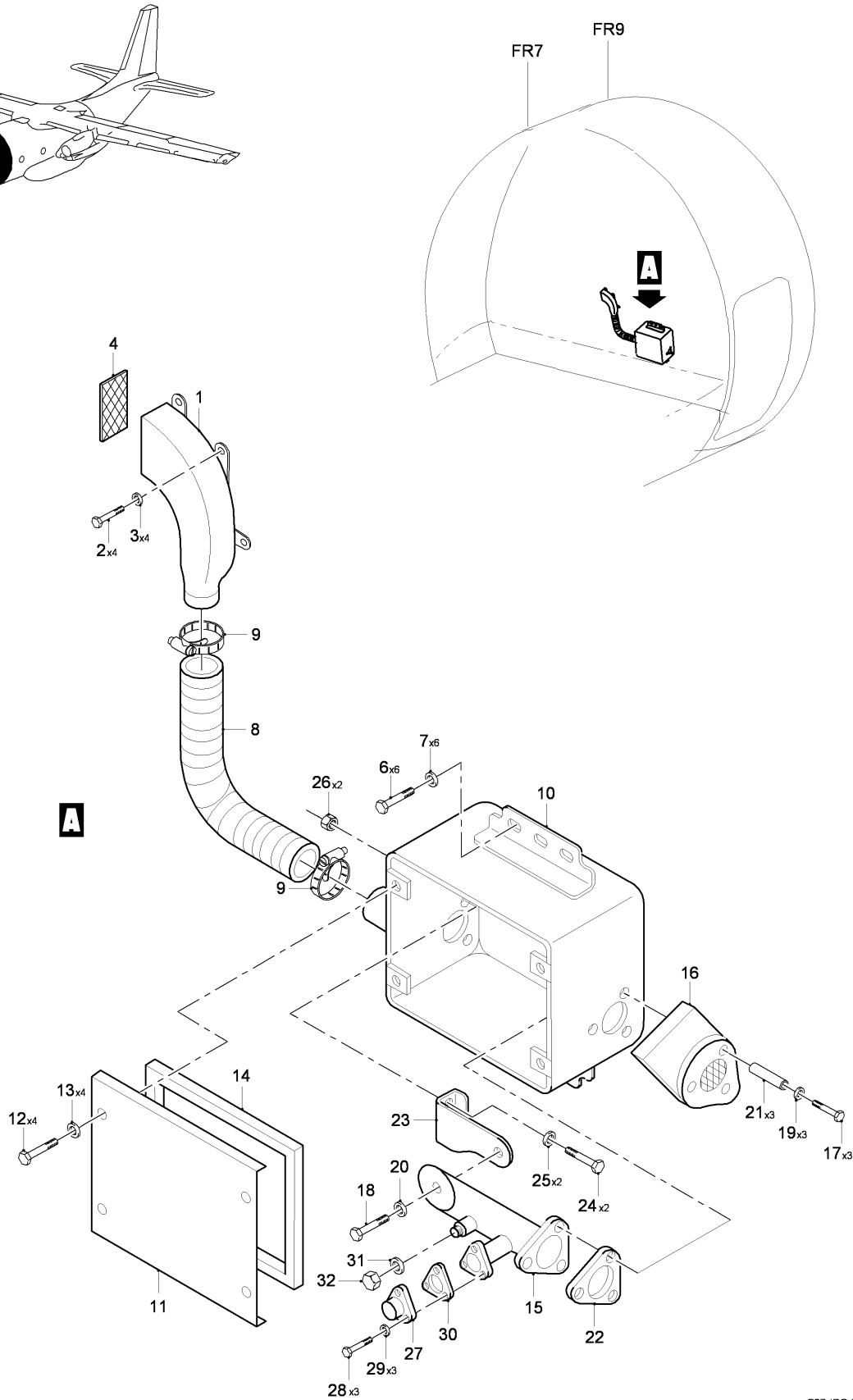
FIG 02 TEMPERATURE SENSOR BOX INSTL, Z31AB (SHEET 1 OF 1)
