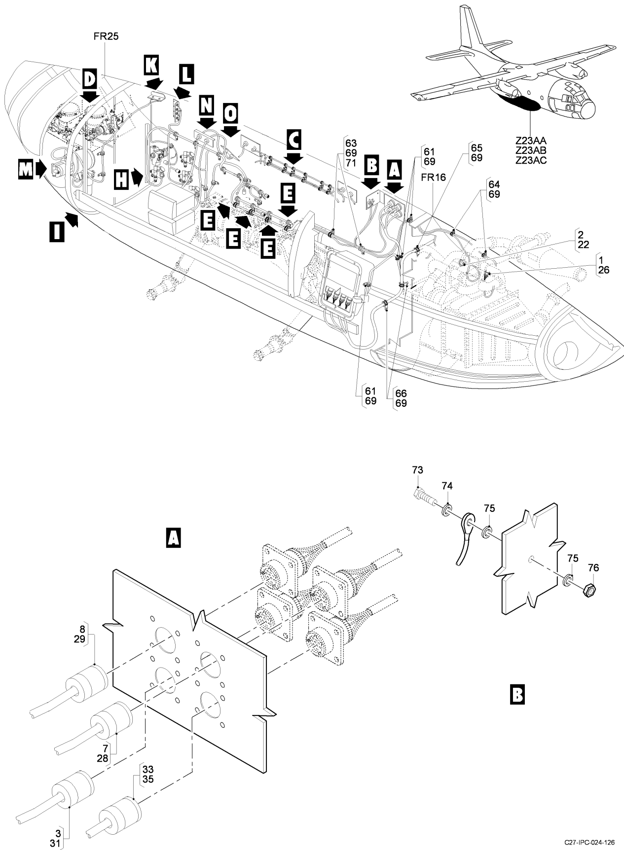
FIG 27 ELECTRICAL AND ELECTRONICS INSTL - MLG, Z23AA-23AB-23AC, RH (SHEET 1 OF 5)
