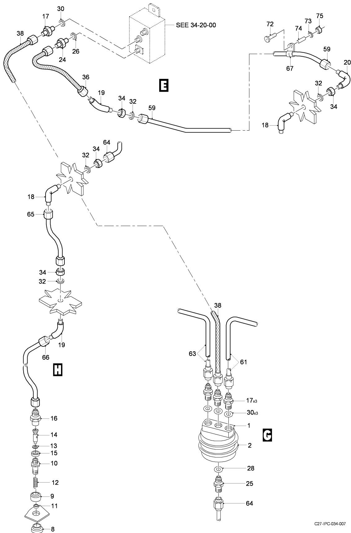
FIG 06 STATIC AND DINAMIC PRESSURE INSTRUMENTS INSTL, Z31AA (SHEET 2 OF 5)
