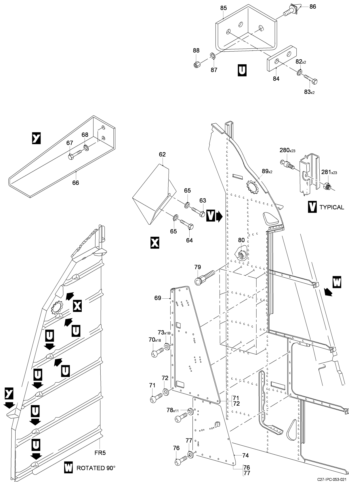
FIG 06 STRUCTURE INSTL, Z31AA (SHEET 5 OF 10)
