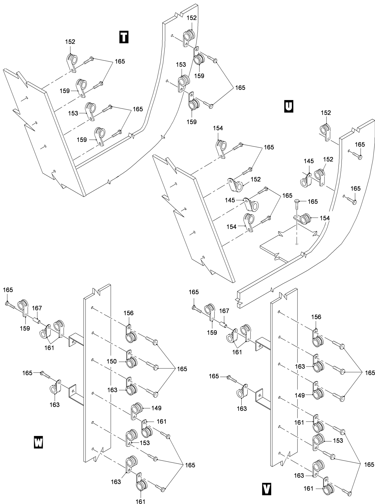
FIG 14 ELECTRICAL AND ELECTRONICS INSTL, Z31BC-31BD-32BA (SHEET 8 OF 11)
