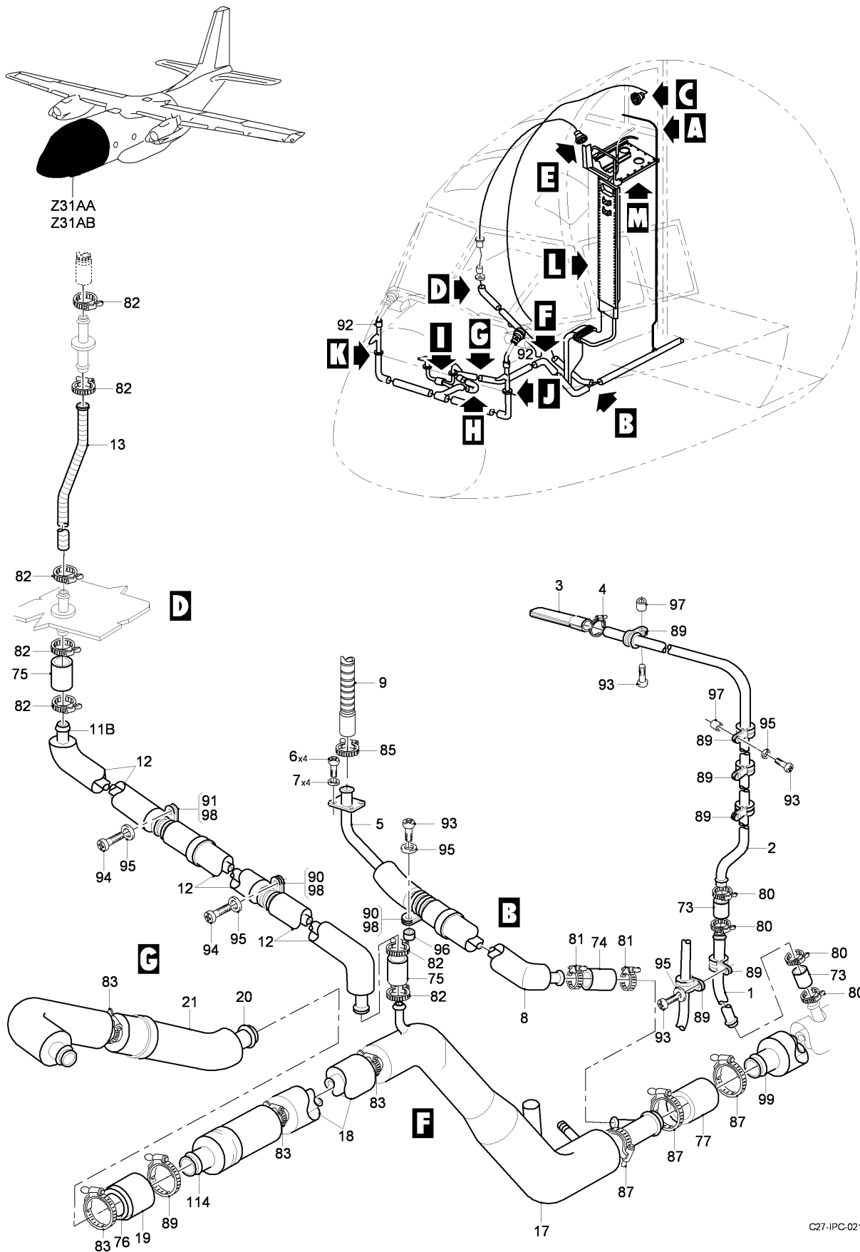
FIG 01 AIR CONDITIONING INSTL - FWD FUSELAGE, Z31AA-31AB (SHEET 1 OF 3)
