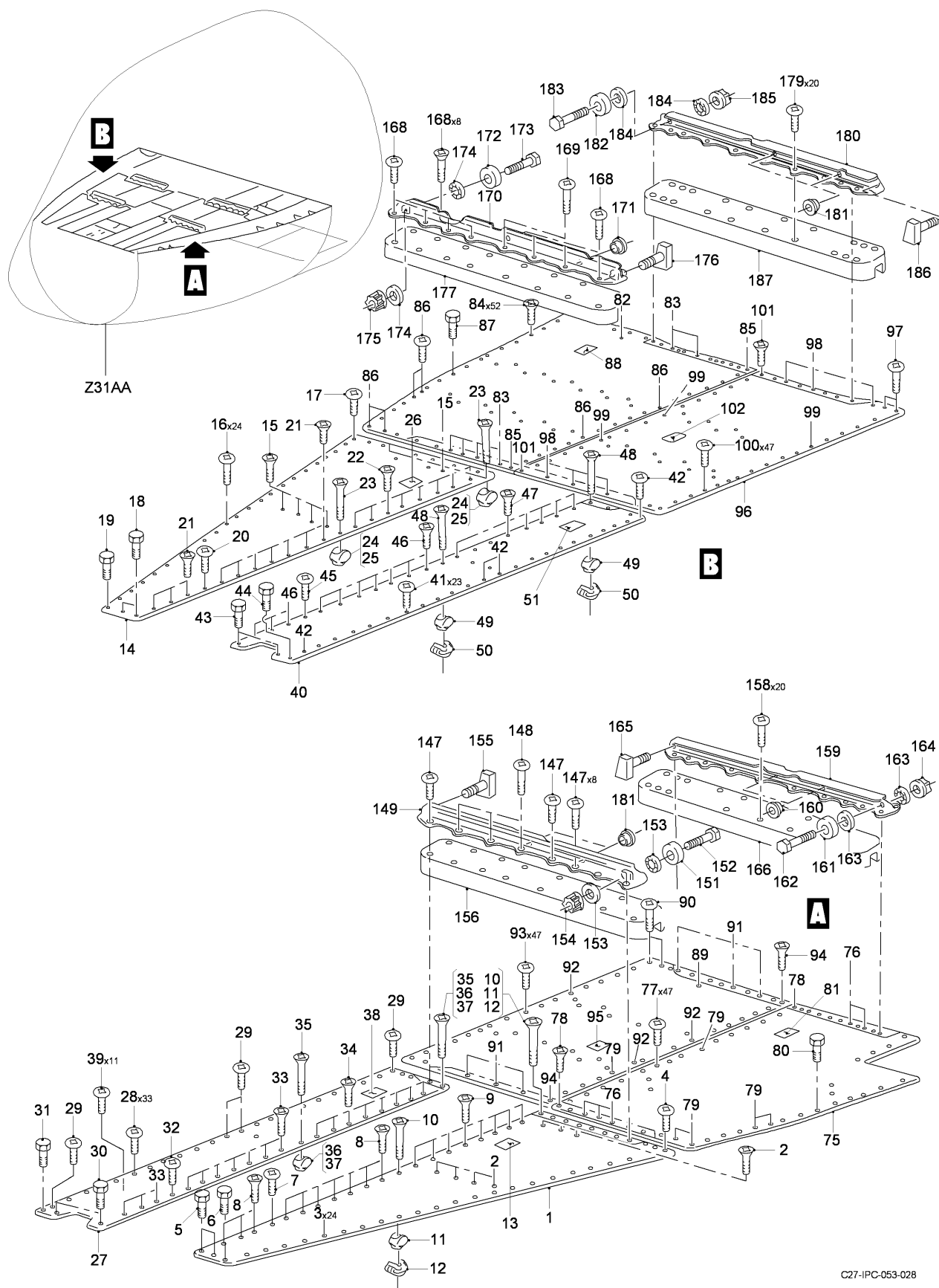
FIG 08 FLOOR FWD FUSELAGE INSTL, Z31AA (SHEET 1 OF 3)
