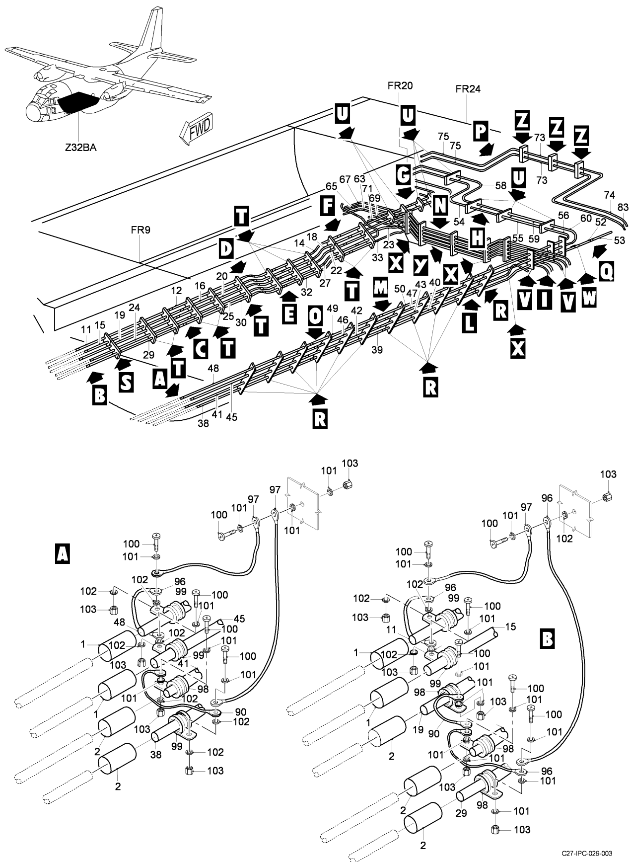
FIG 02 HYDRAULIC INSTL - CENTER FUSELAGE, LOWER, Z32BA (SHEET 1 OF 8)
