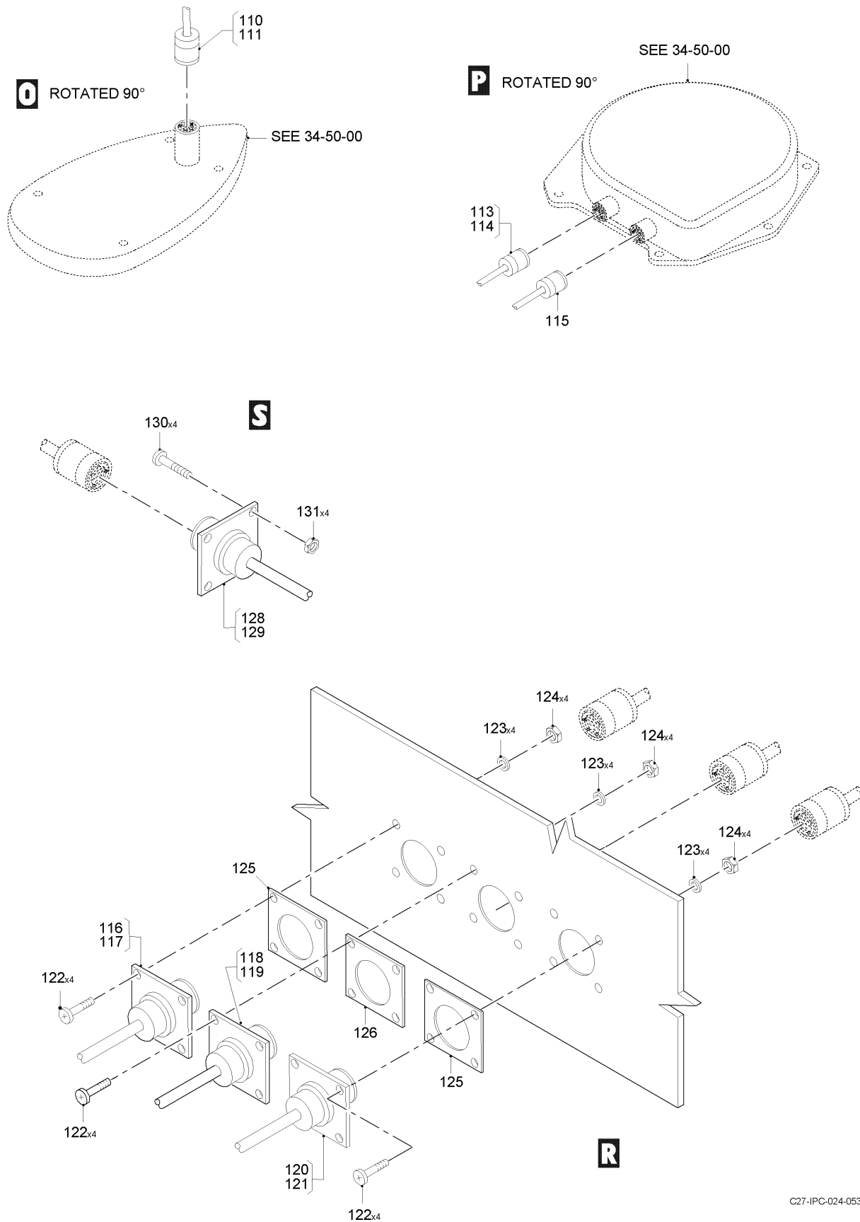
FIG 14 ELECTRICAL AND ELECTRONICS INSTL, Z31BC-31BD-32BA (SHEET 7 OF 11)
