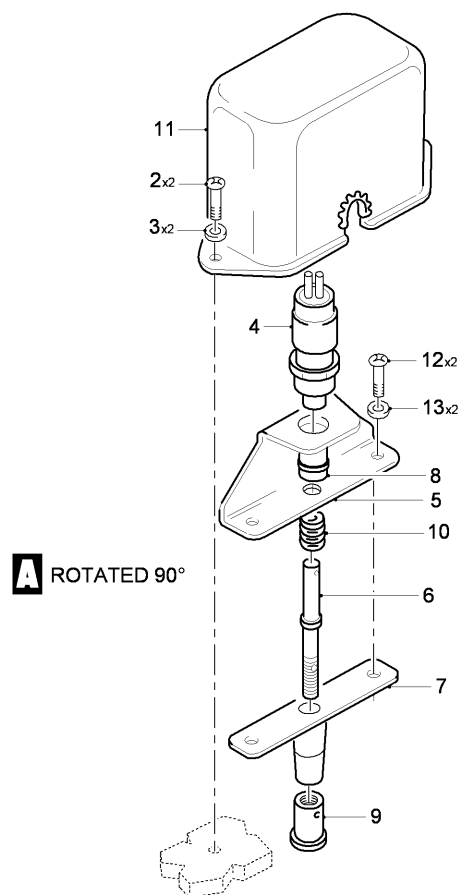
FIG 01 CREW DOOR SWITCH INSTL, Z31AB (SHEET 1 OF 1)
