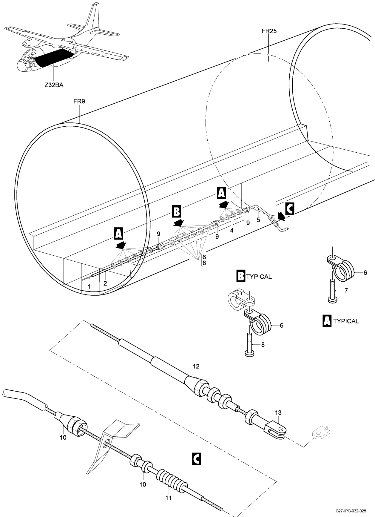
FIG 05 PARKING AND WHEEL BRAKES EMERGENCY INSTL, Z32BA (SHEET 1 OF 1)
