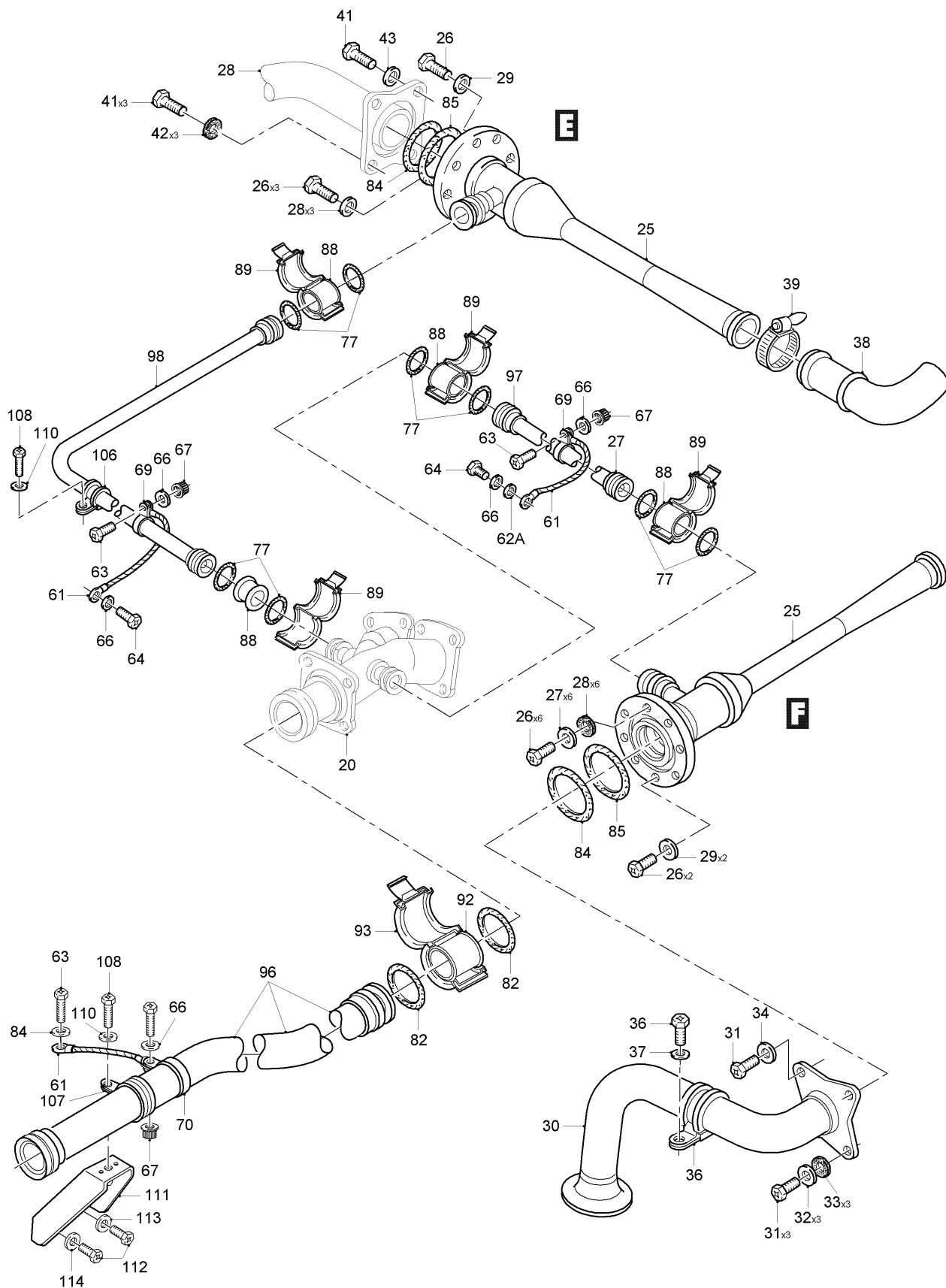
FIG 10 FUEL VENT AND DRAINS INSTL - CENTER WING, Z33AB, LH-RH (SHEET 3 OF 4)
