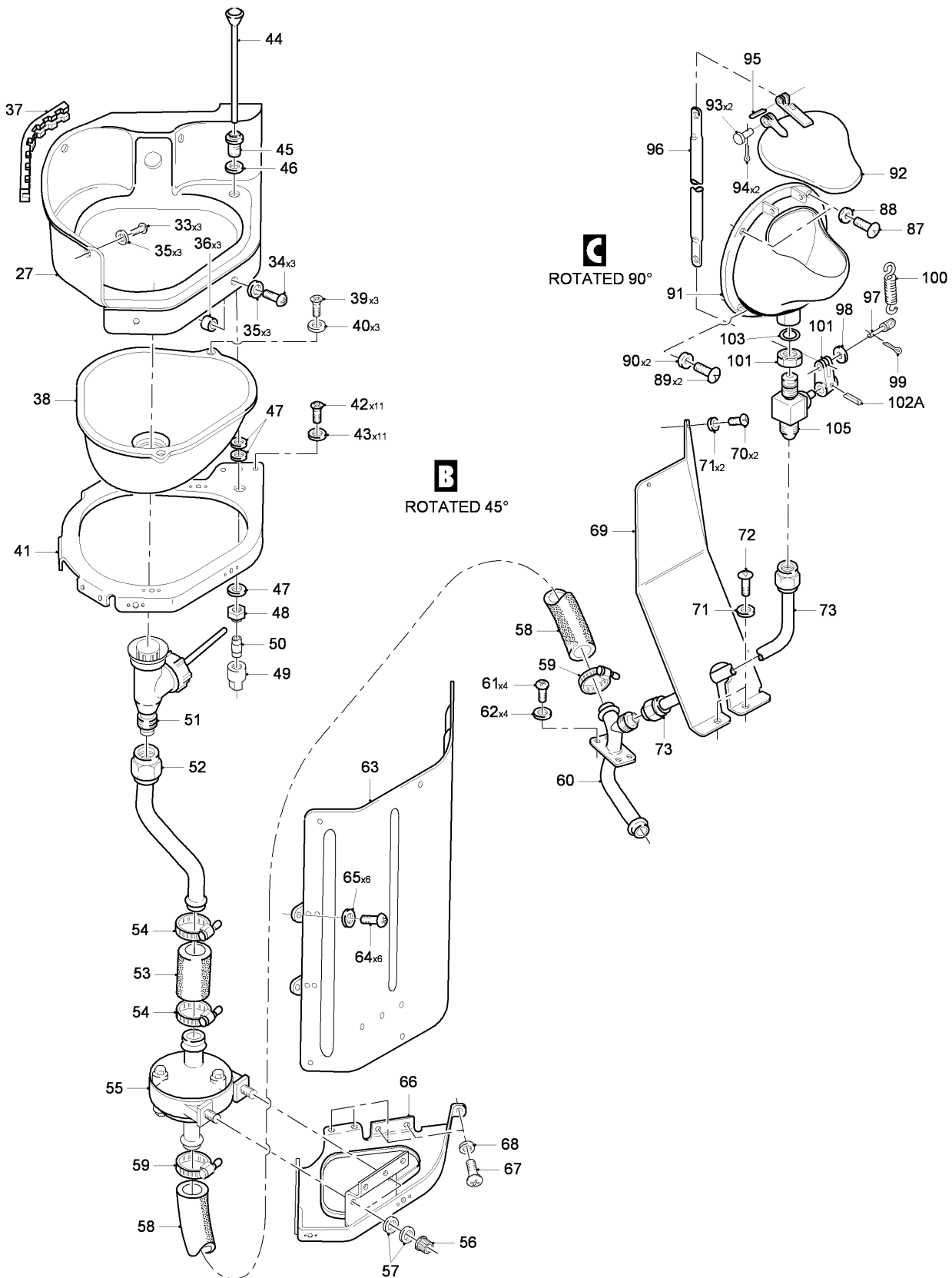
FIG 01 TOILET INSTL, Z31AB (SHEET 2 OF 3)
