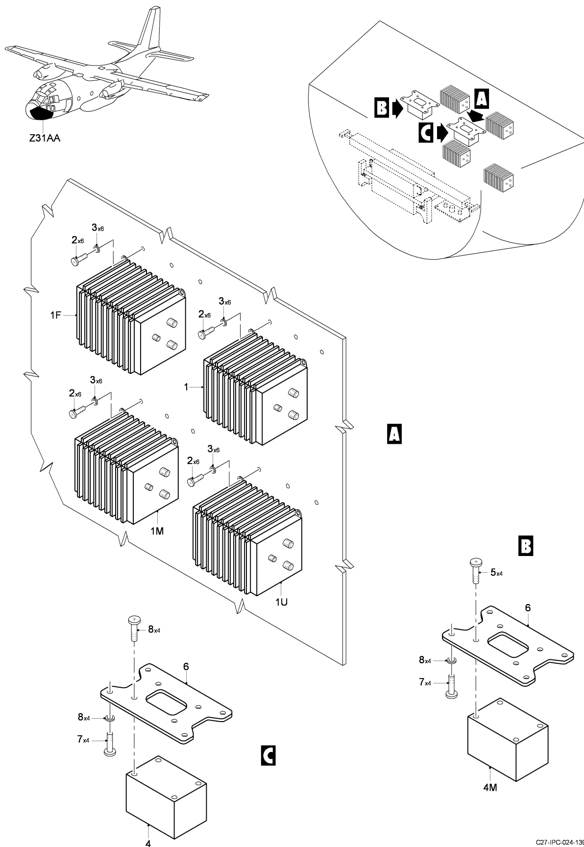
FIG 01 REGULATED POWER SUPPLY COMPONENTS INSTL, Z31AA (SHEET 1 OF 1)
