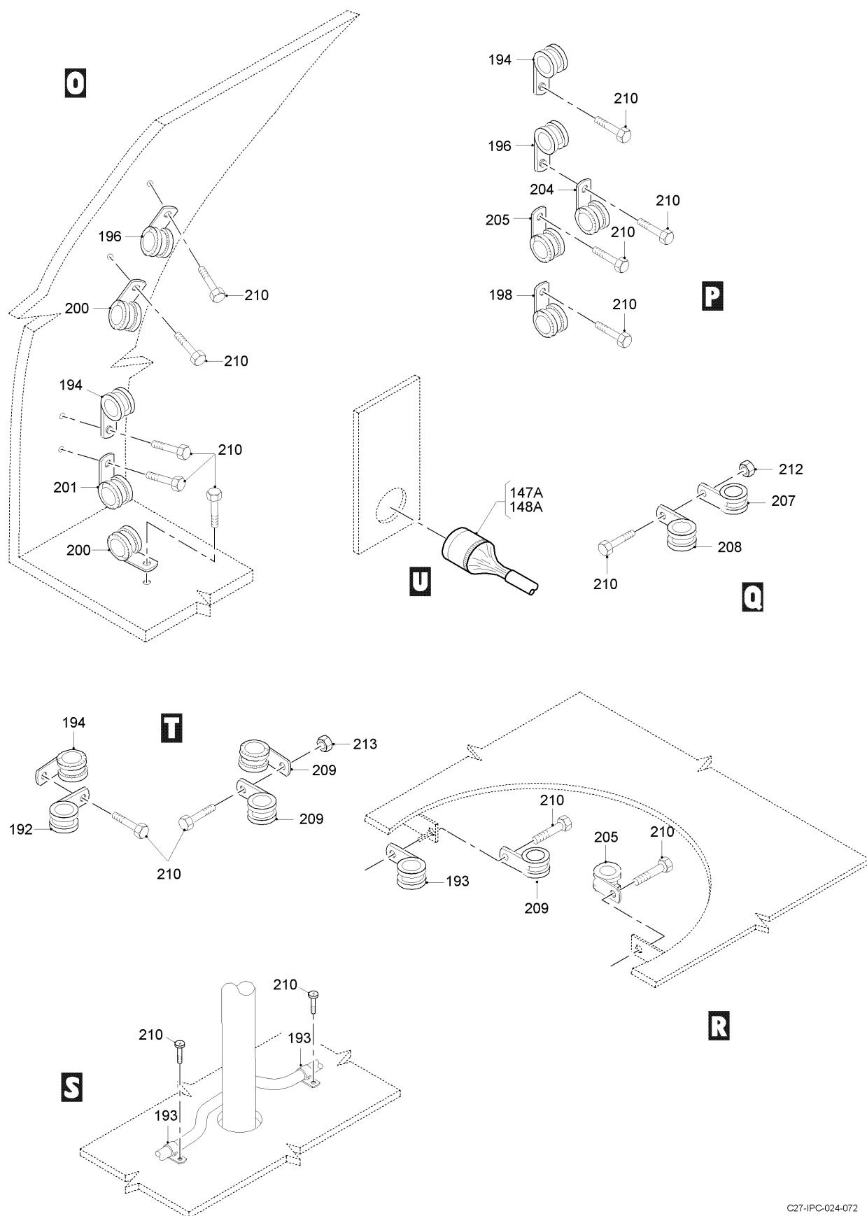
FIG 16 ELECTRICAL AND ELECTRONICS INSTL, Z31AB-32AA-32AB-32AC, RH (SHEET 8 OF 8)
