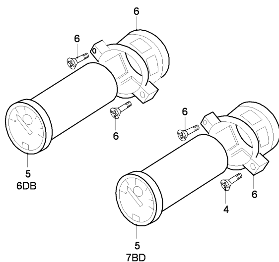
FIG 03 OXYGEN QUANTITY INDICATOR INSTL, UPPER SIDE, Z31AA, LH (SHEET 1 OF 1)
