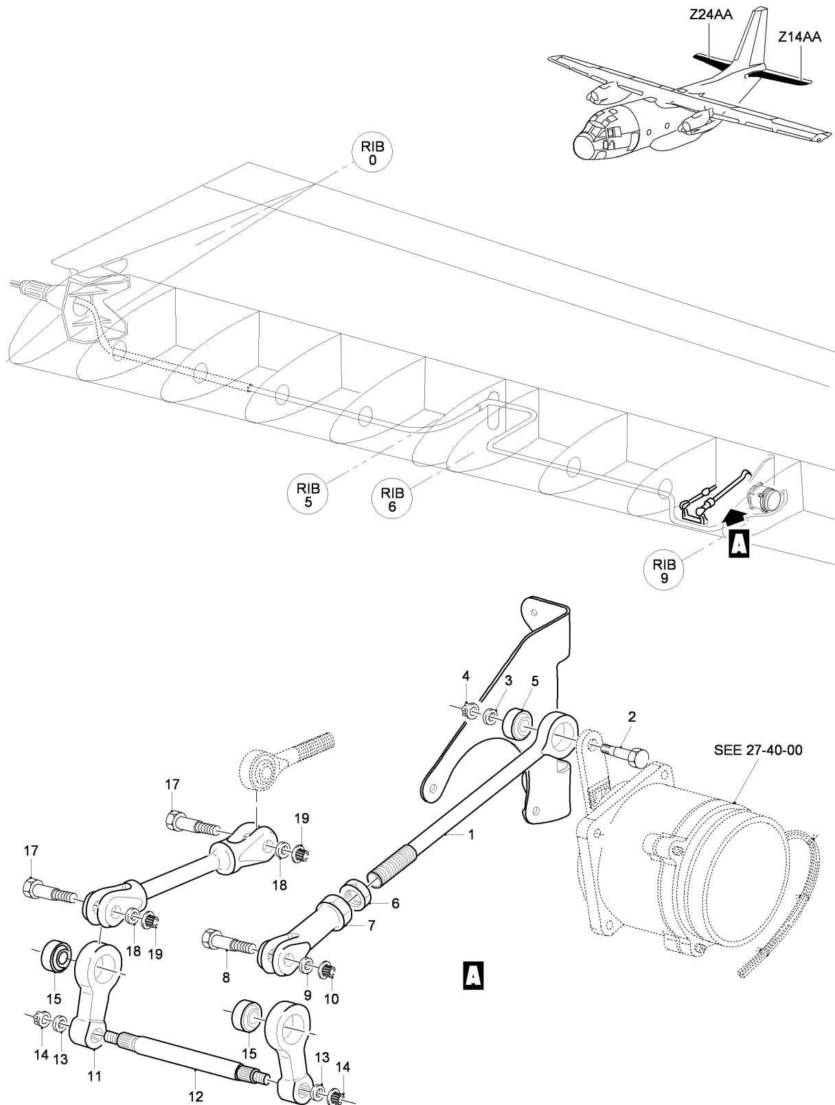
FIG 10 ELEVATOR TRANSMITTER INSTL-TRIM POSITION, Z14AA-24AA, LH-RH (SHEET 1 OF 1)
