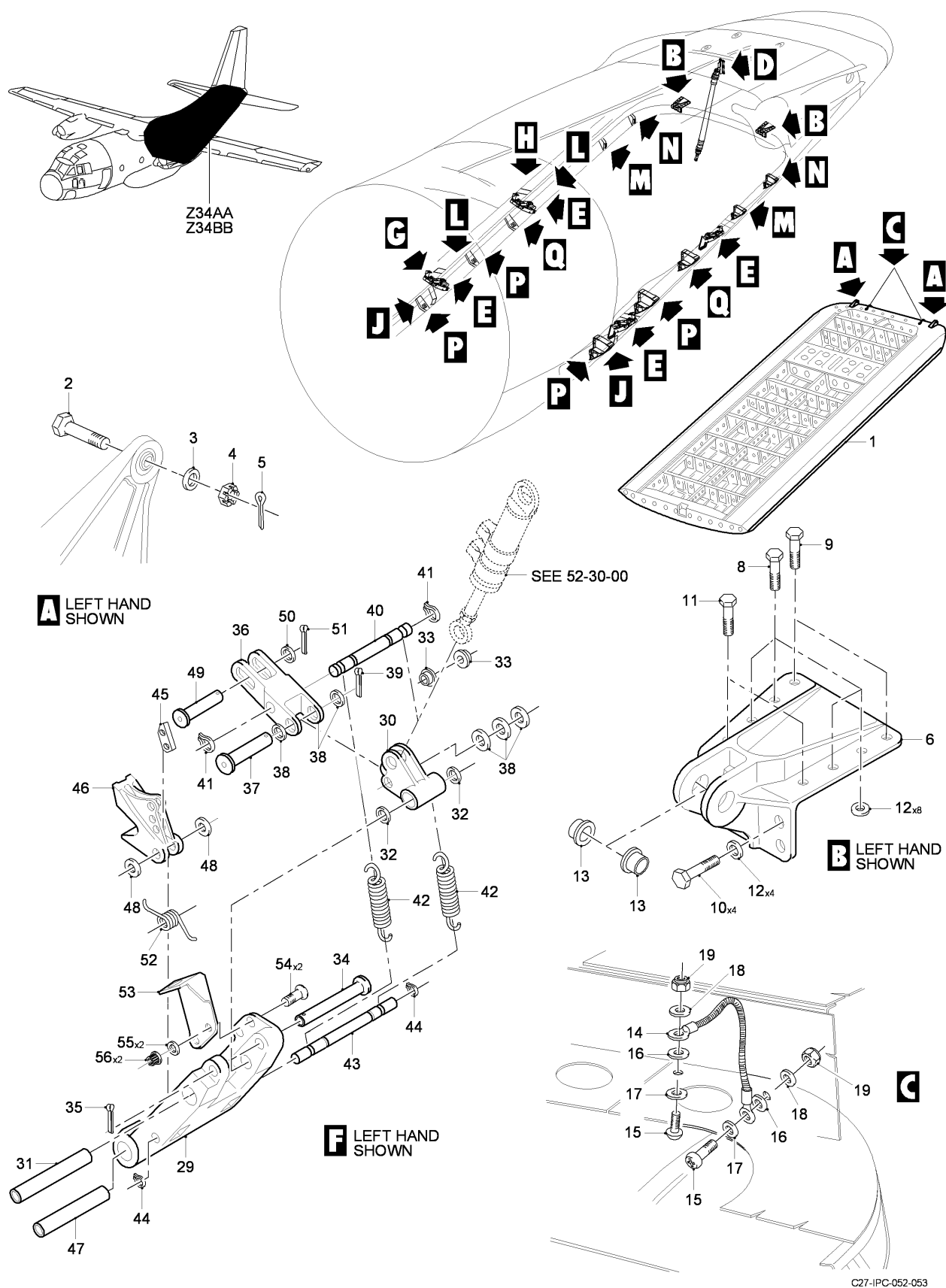
FIG 11 CARGO DOOR INSTL, Z34AA-34BB (SHEET 1 OF 3)
