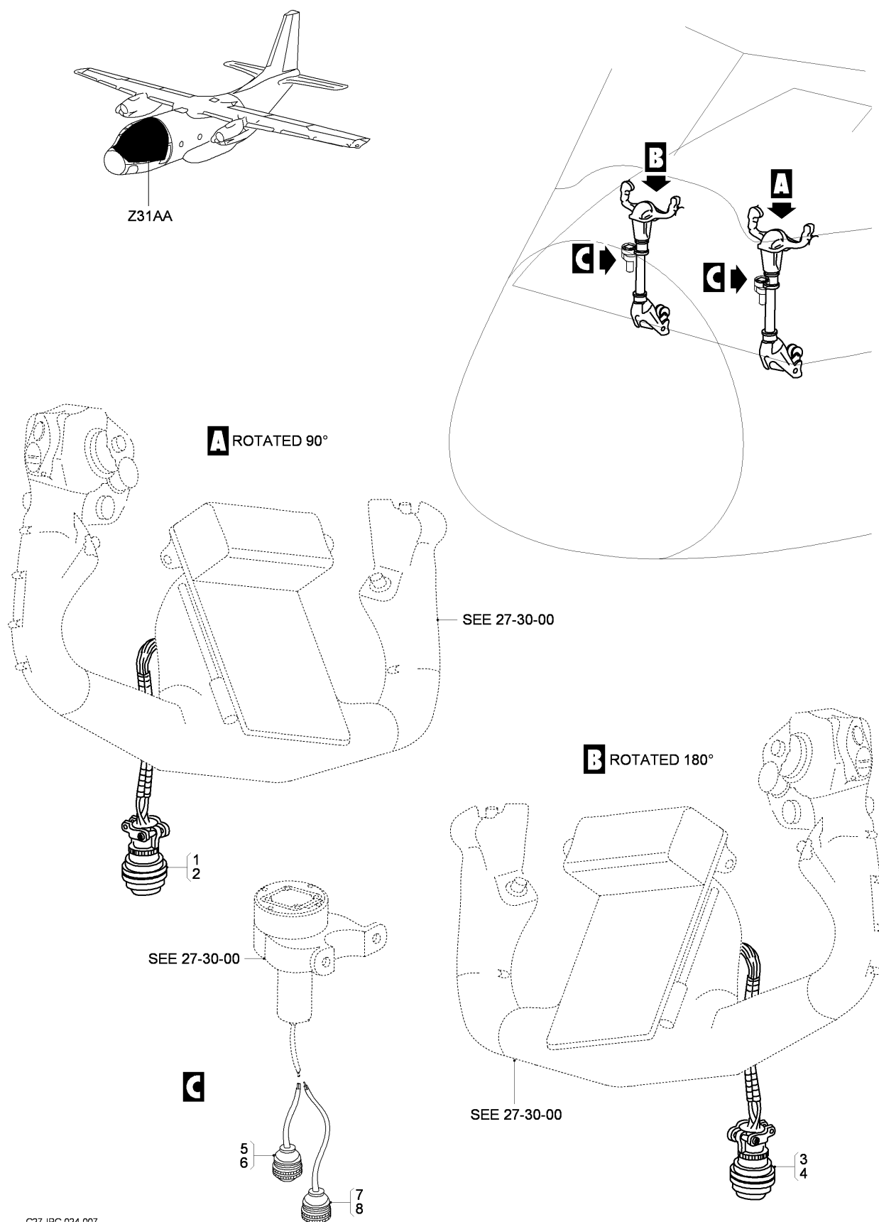
FIG 03 HARNESS CONTROL COLUMN INSTL, Z31AA, LH-RH (SHEET 1 OF 1)
