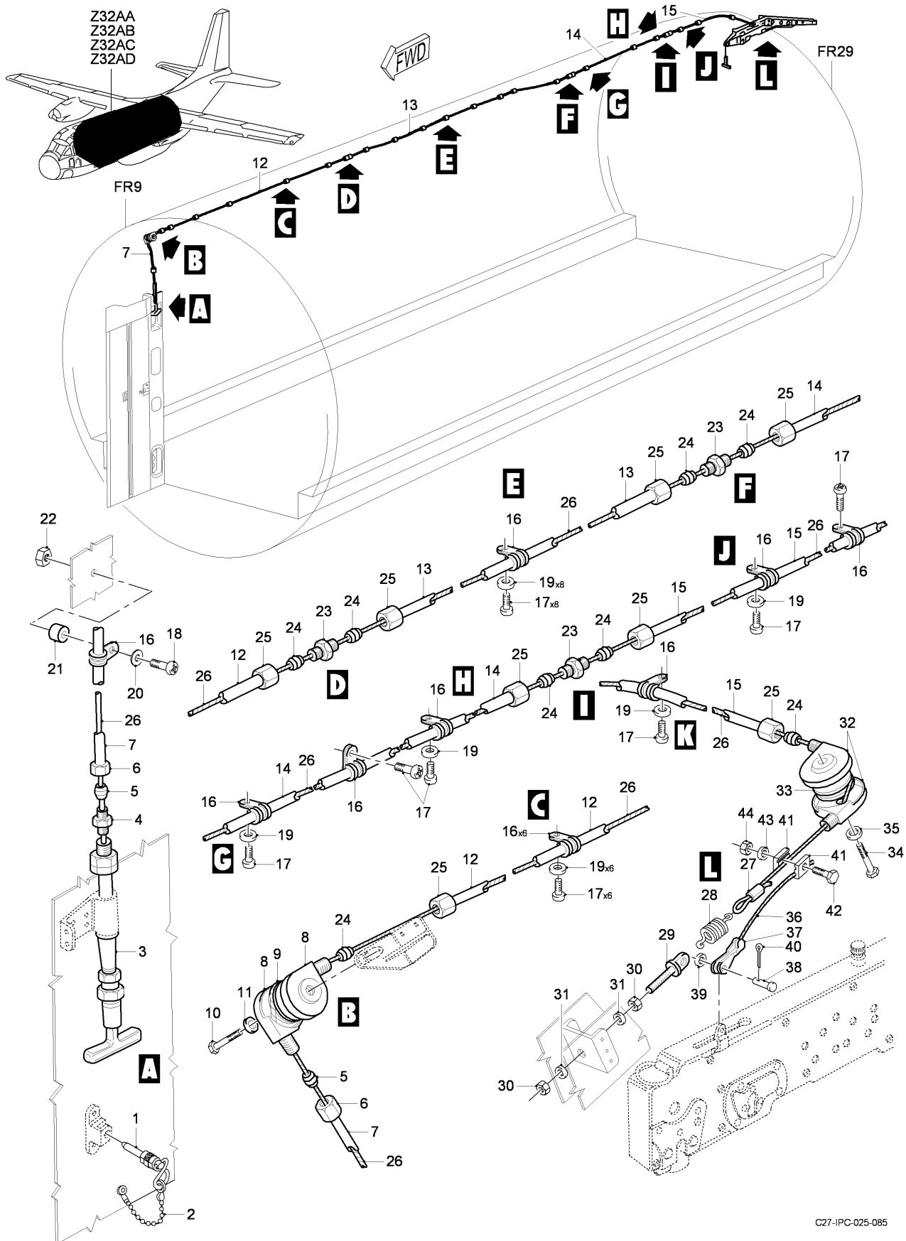
FIG 01 HOOK EMERGENCY CONTROLS INSTL, Z32AA-32AB-32AC-32AD (SHEET 1 OF 1)
