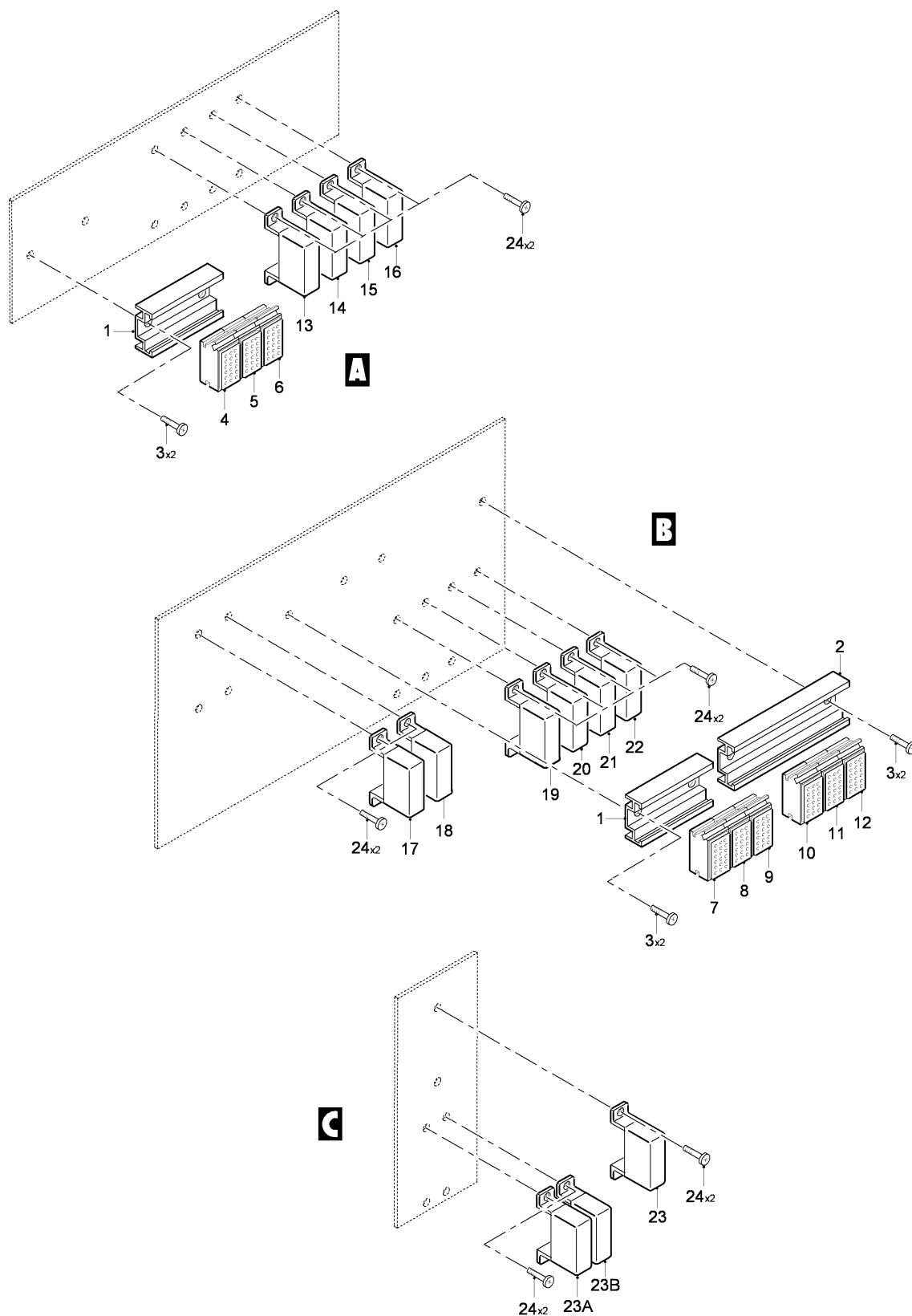
FIG 05 ELECTRICAL AND ELECTRONICS INSTL - CABIN, Z31AA, RH (SHEET 3 OF 5)
