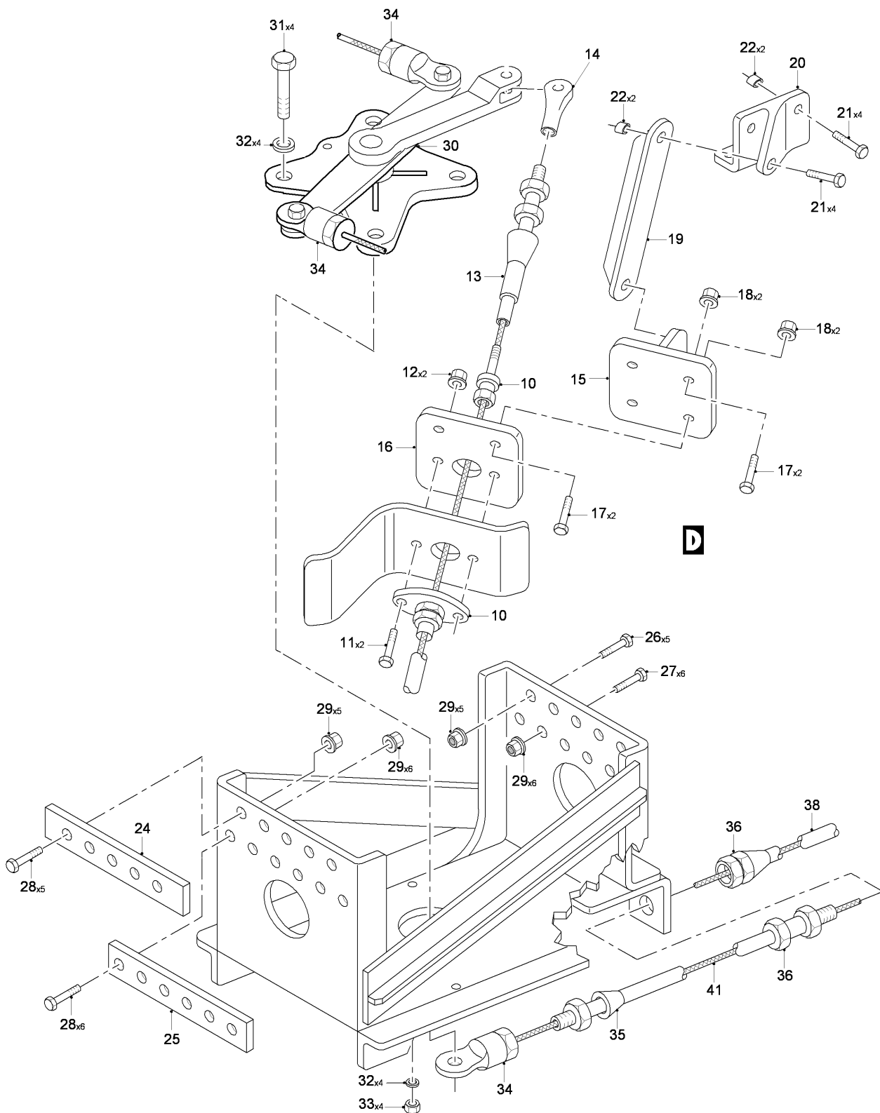
FIG 03 EMERGENCY CONTROL INSTL - MAIN LANDING GEAR, Z32BA (SHEET 2 OF 4)
