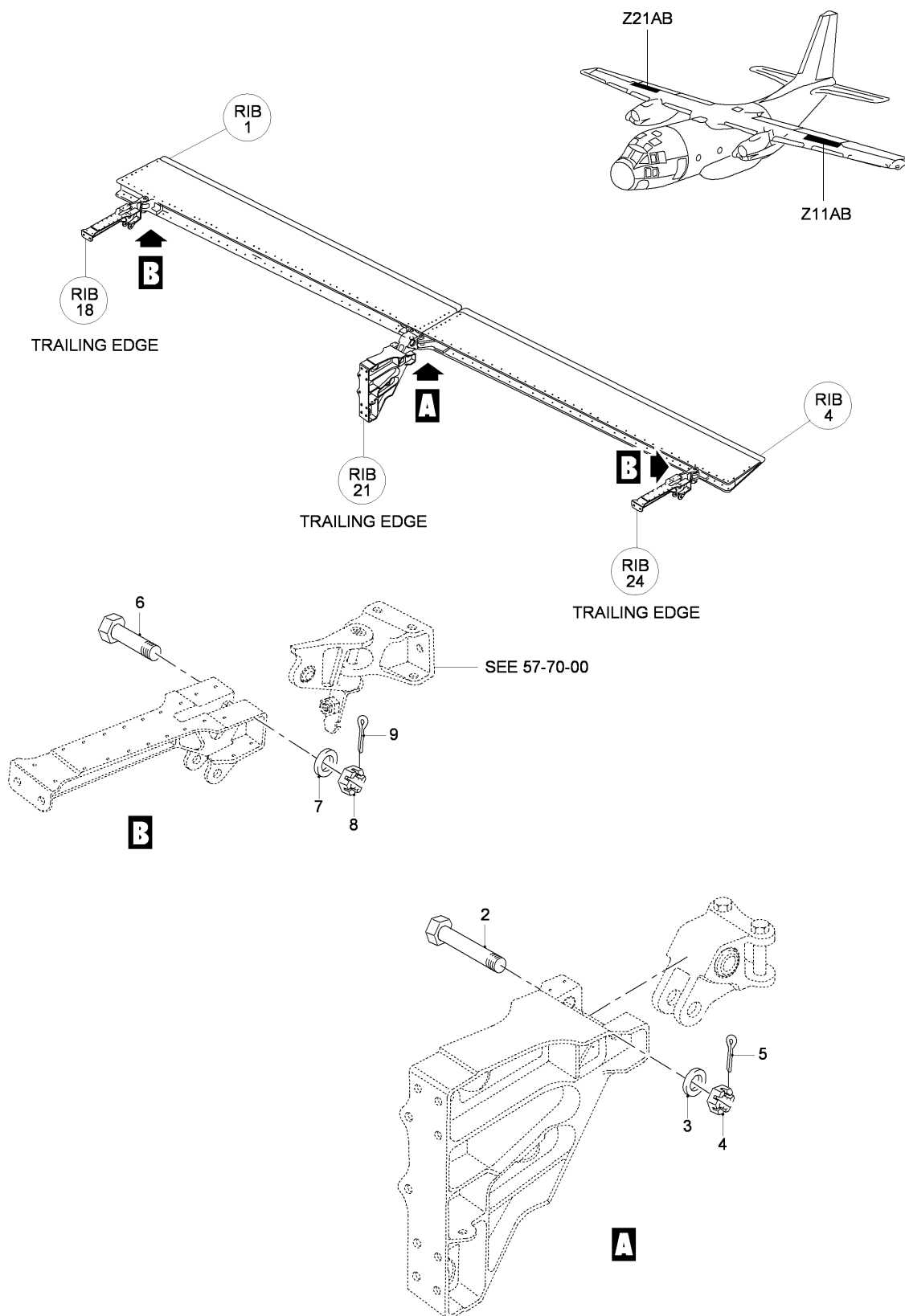
FIG 06 SPOILER INSTL, Z11AB-21AB, LH-RH (SHEET 1 OF 1)
