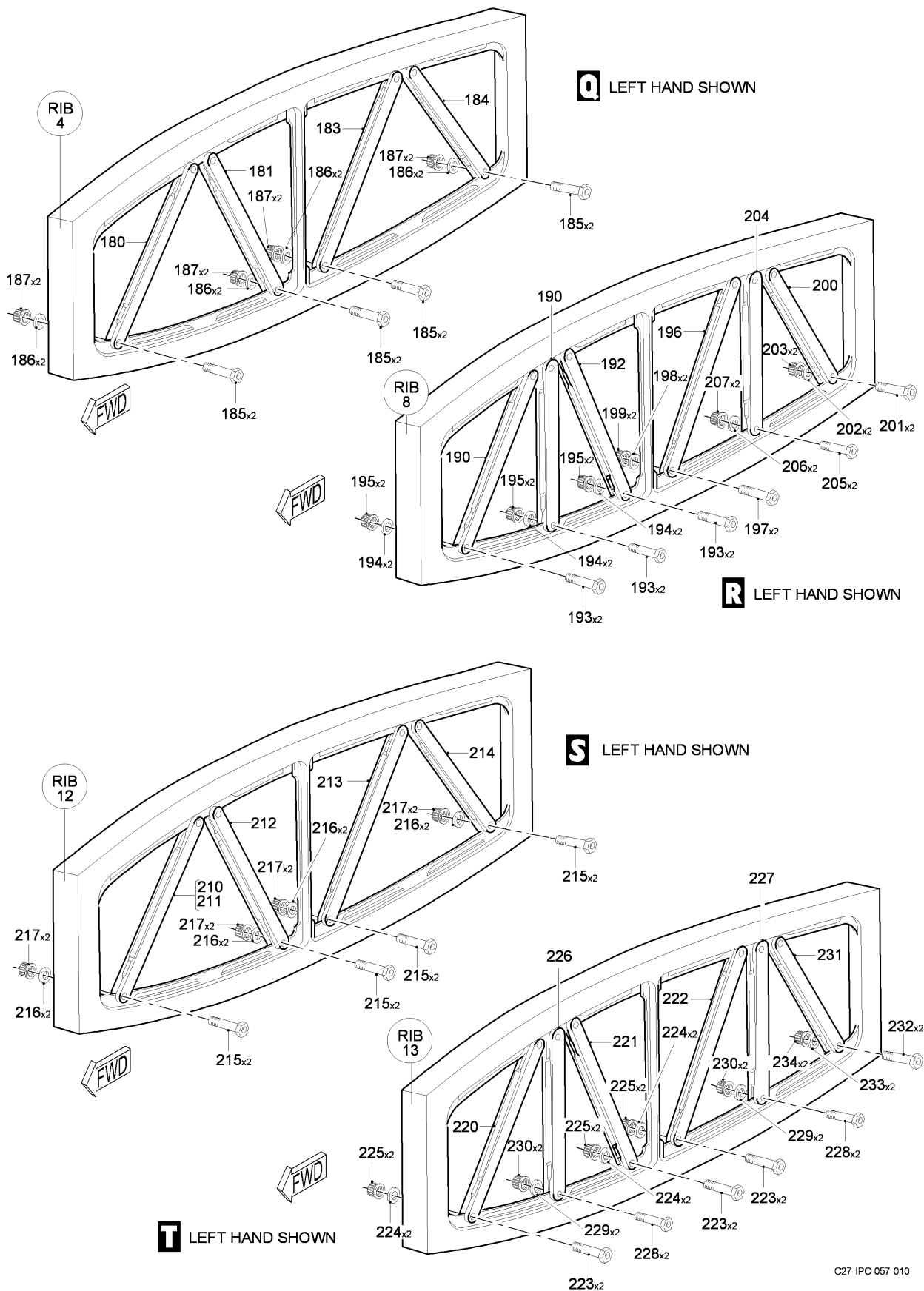
FIG 03 STRUCTURE INSTL - CENTER WING, Z33AB (SHEET 4 OF 5)
