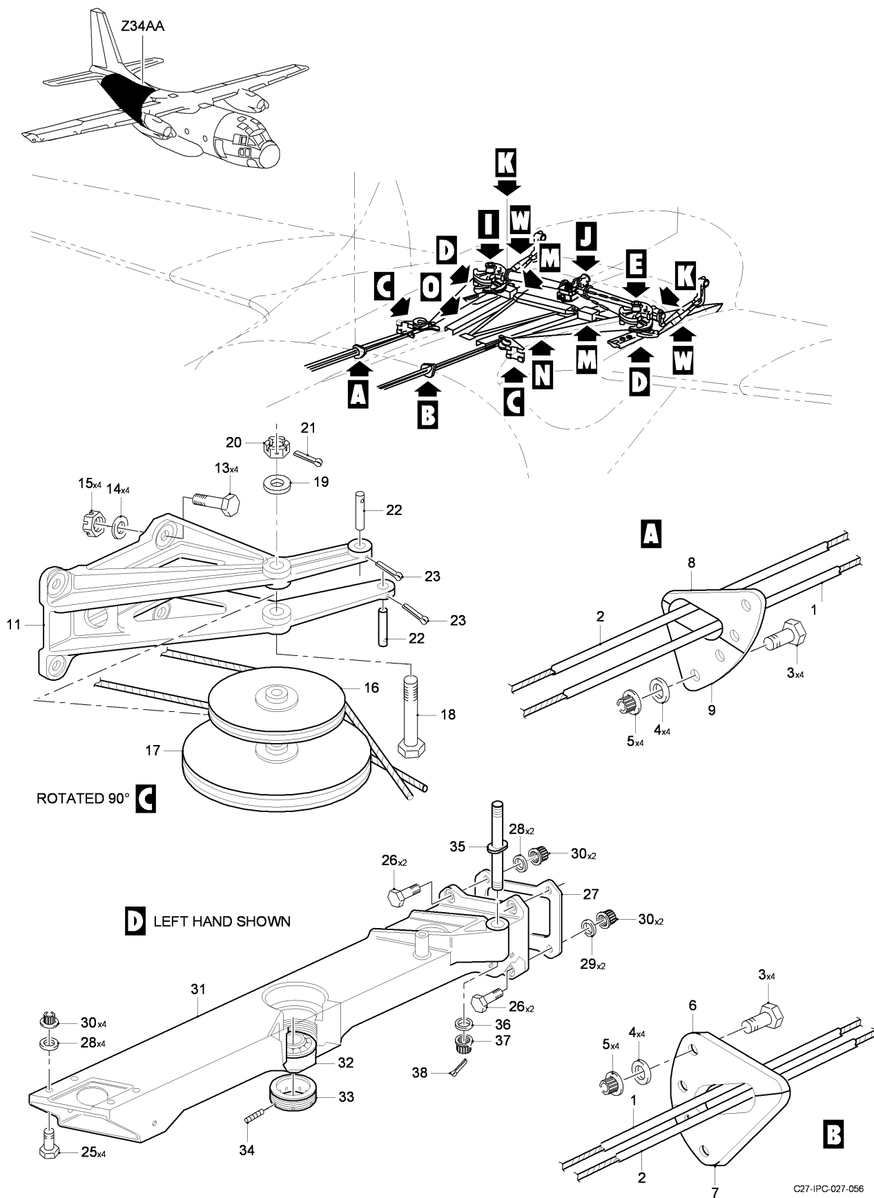
FIG 07 ELEVATOR CONTROLS INSTL, Z34AA (SHEET 1 OF 8)
