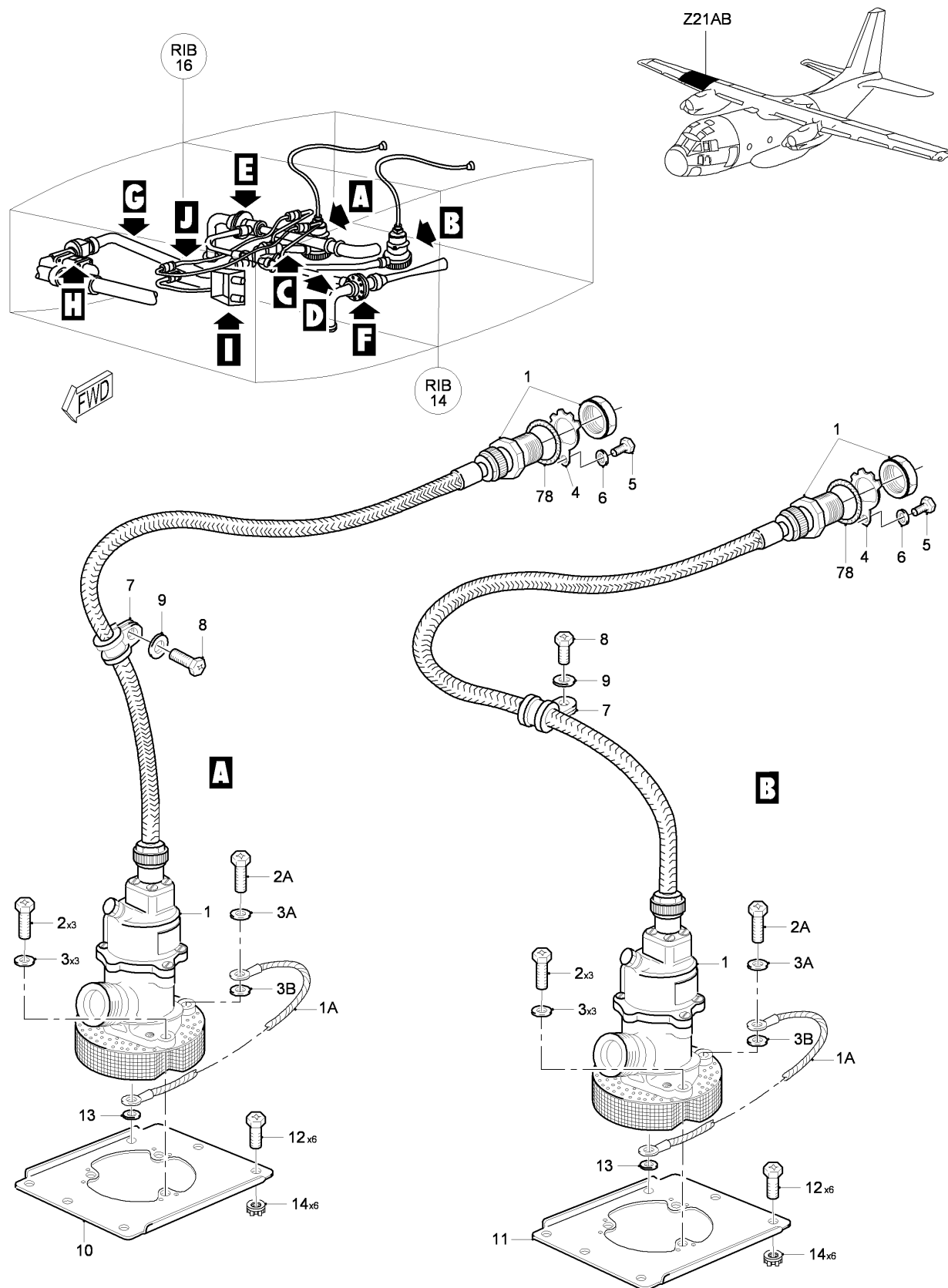
FIG 07 FUEL SUPPLY INSTL - OUTER WING, Z21AB, RH (SHEET 1 OF 4)
