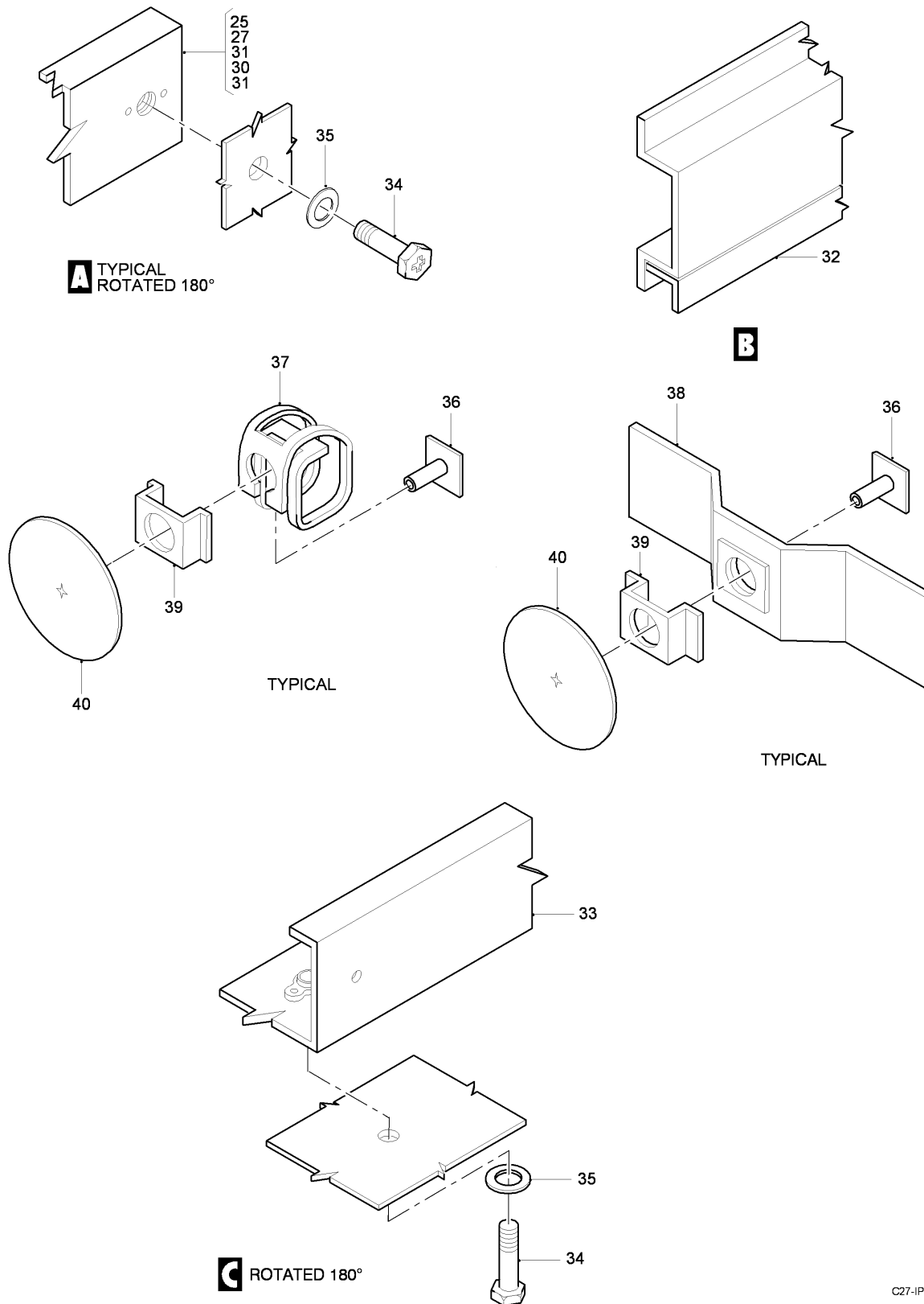
FIG 34 SECONDARY THERMAL INSULATION INSTL, LH SIDE, Z34AA (SHEET 2 OF 2)
