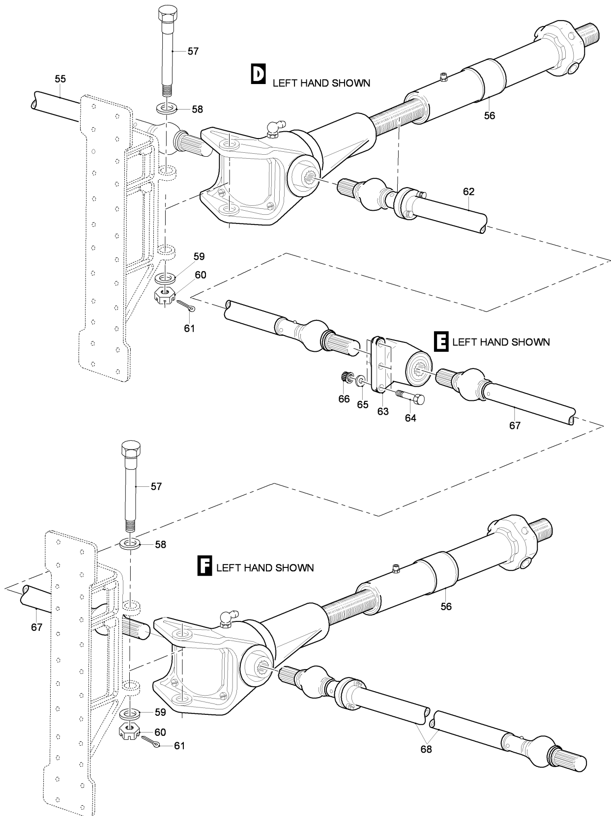
FIG 06 FLAP CONTROLS INSTL, Z33AC (SHEET 3 OF 3)
