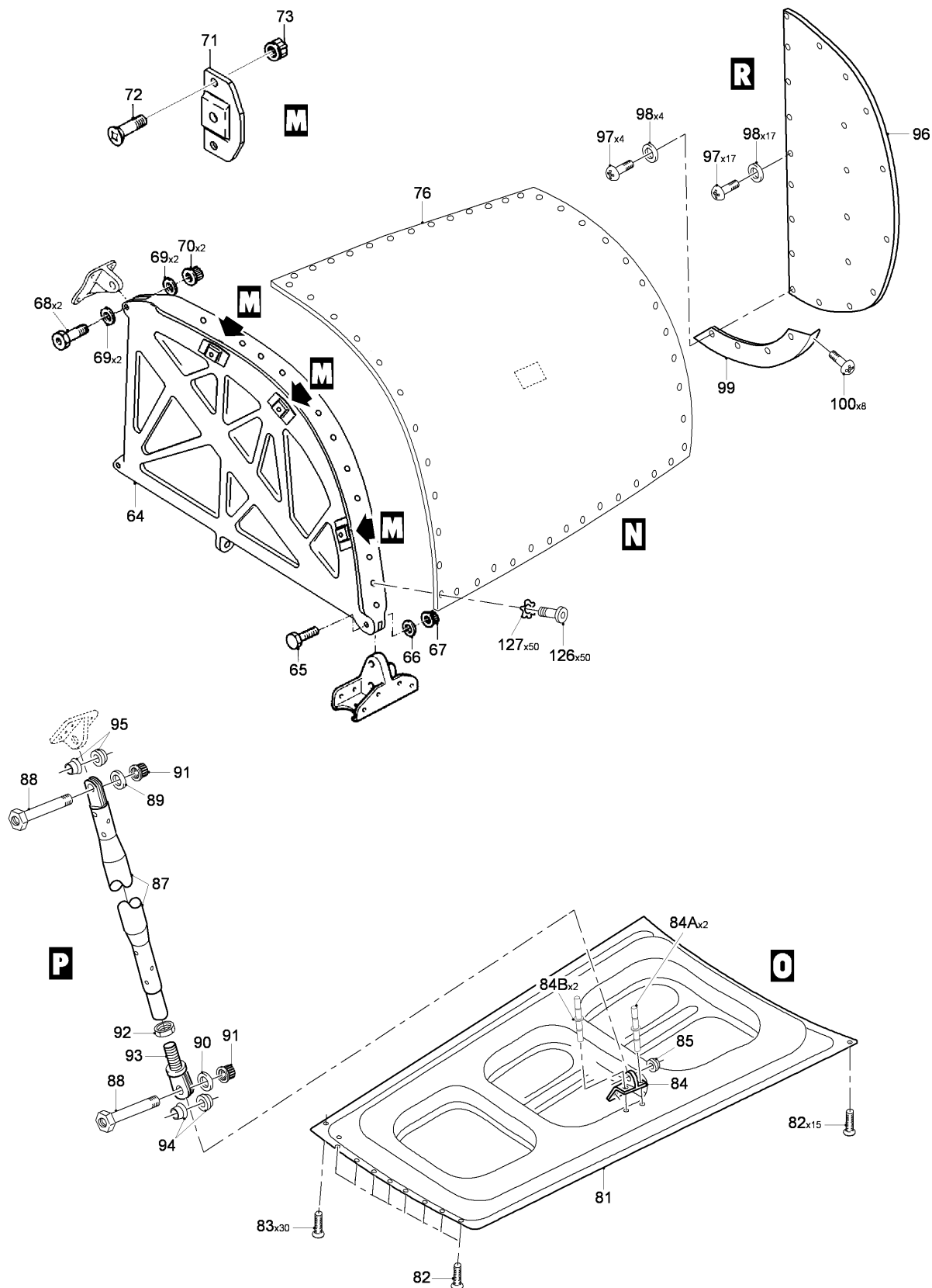
FIG 03 STRUCTURE INSTL - MLG, Z13AB, LH (SHEET 3 OF 3)
