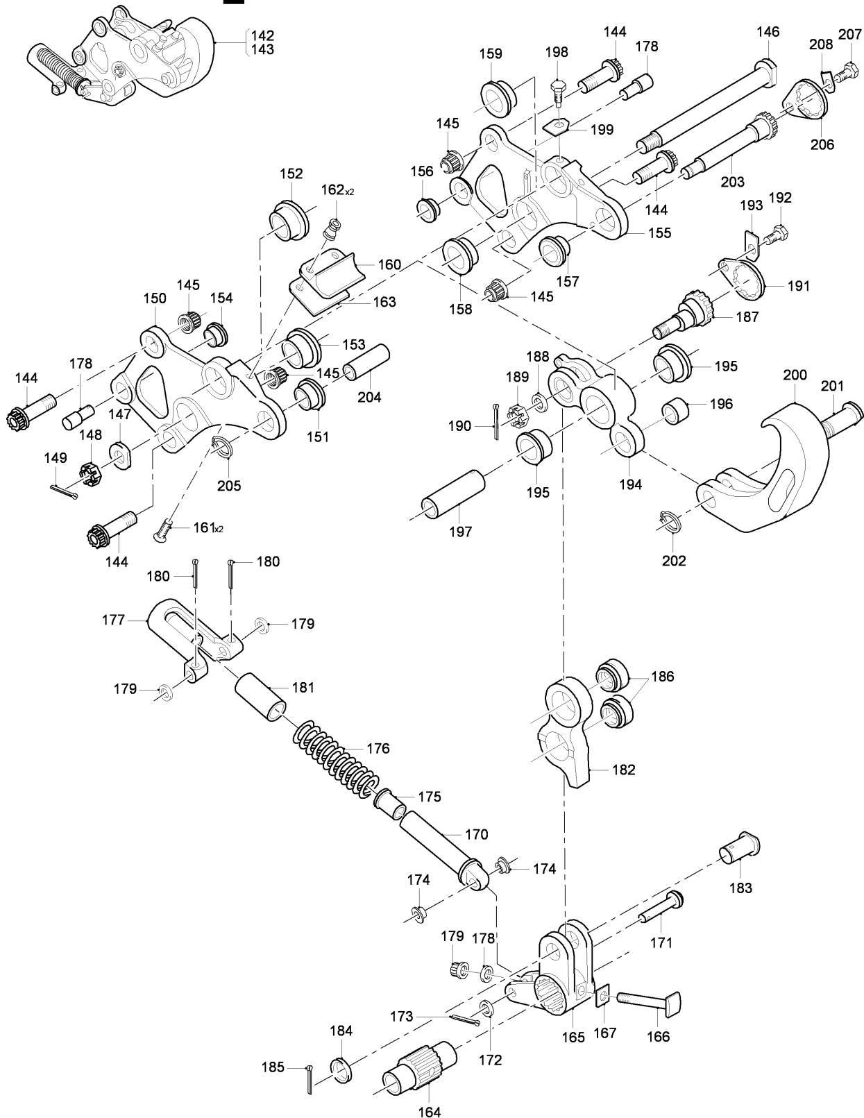
FIG 02 CARGO RAMP ASSY (SHEET 3 OF 6)
