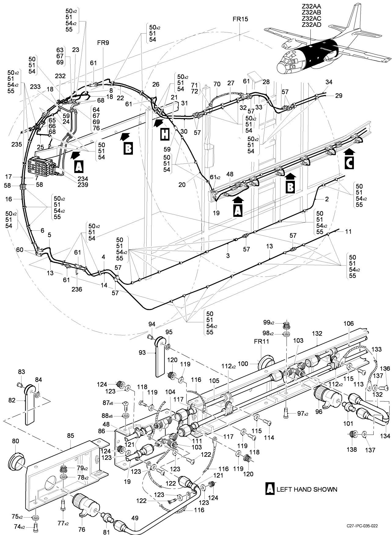
FIG 03 OXYGEN INSTL - CENTER FUSELAGE, Z32AA-32AB-32AC-32AD (SHEET 1 OF 5)
