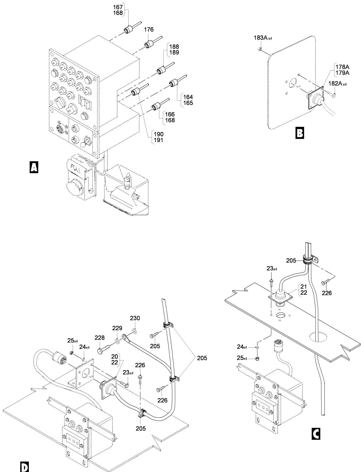
FIG 15 ELECTRICAL AND ELECTRONICS INSTL, Z31AB-32AA-32AB-32AC, LH (SHEET 3 OF 9)
