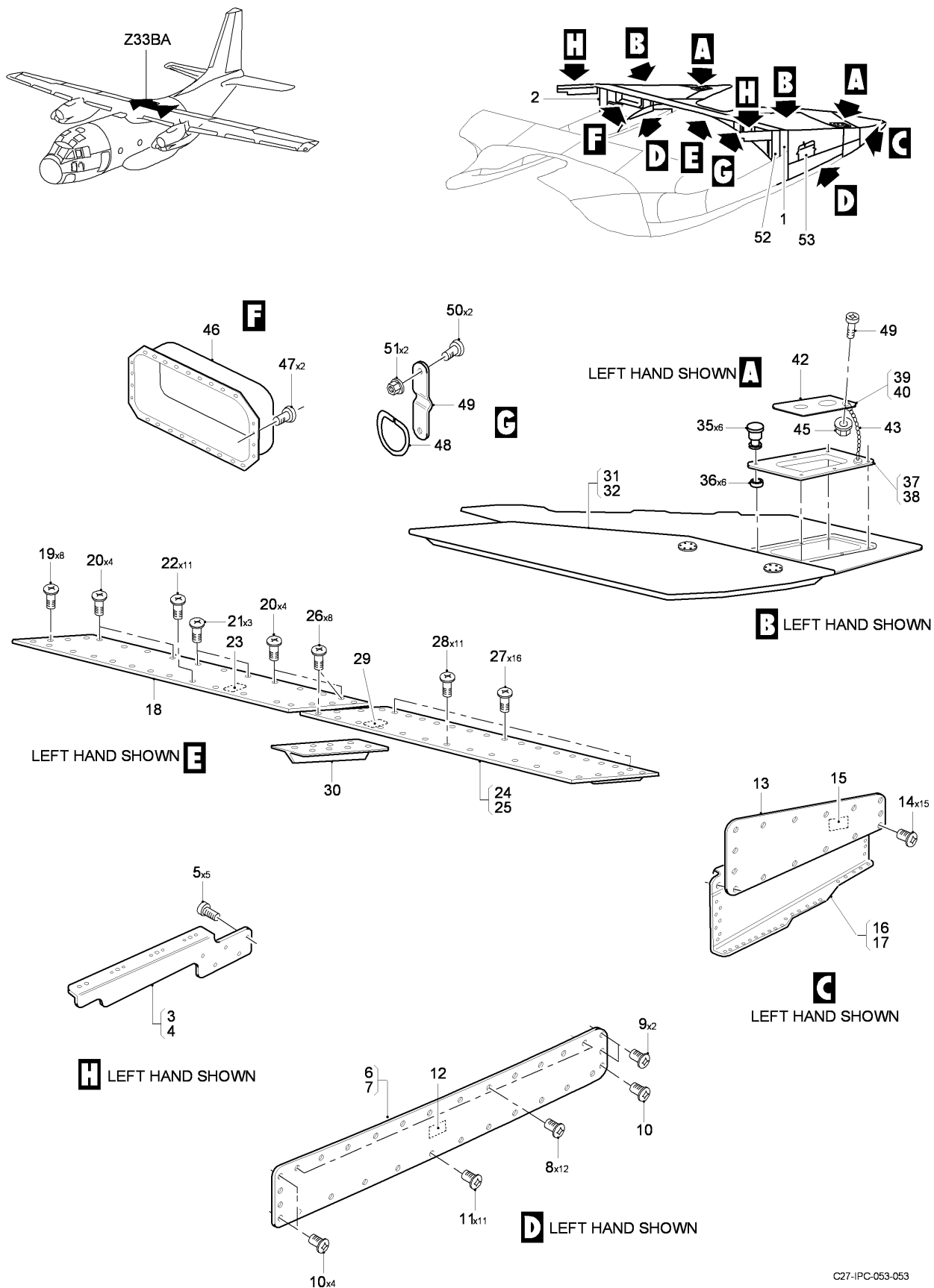
FIG 08 FAIRINGS INSTL - REAR, Z33BA, LH-RH (SHEET 1 OF 1)
