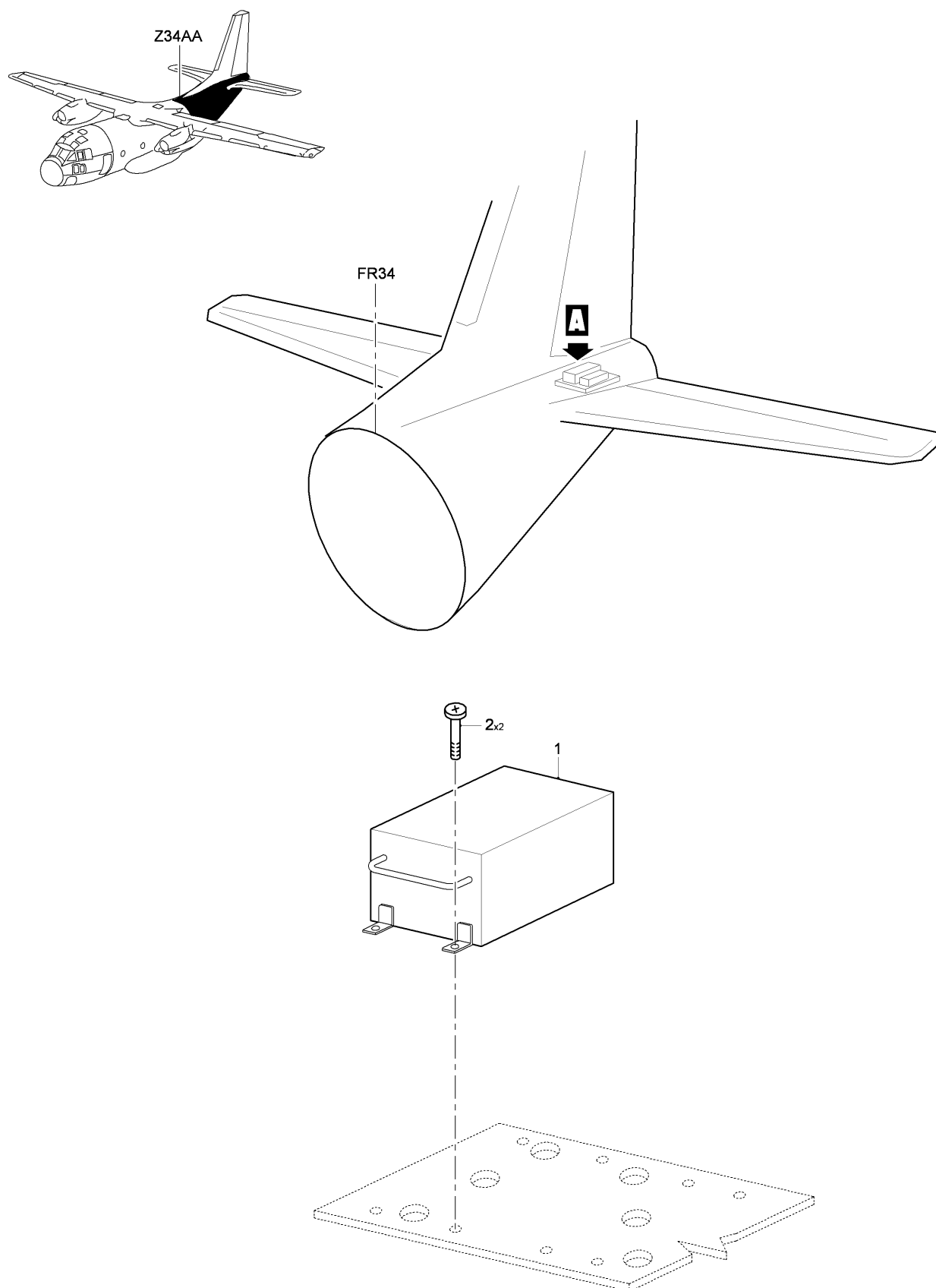
FIG 08 Q-FEEL/RTL ECU BOX INSTL, Z34AA (SHEET 1 OF 1)
