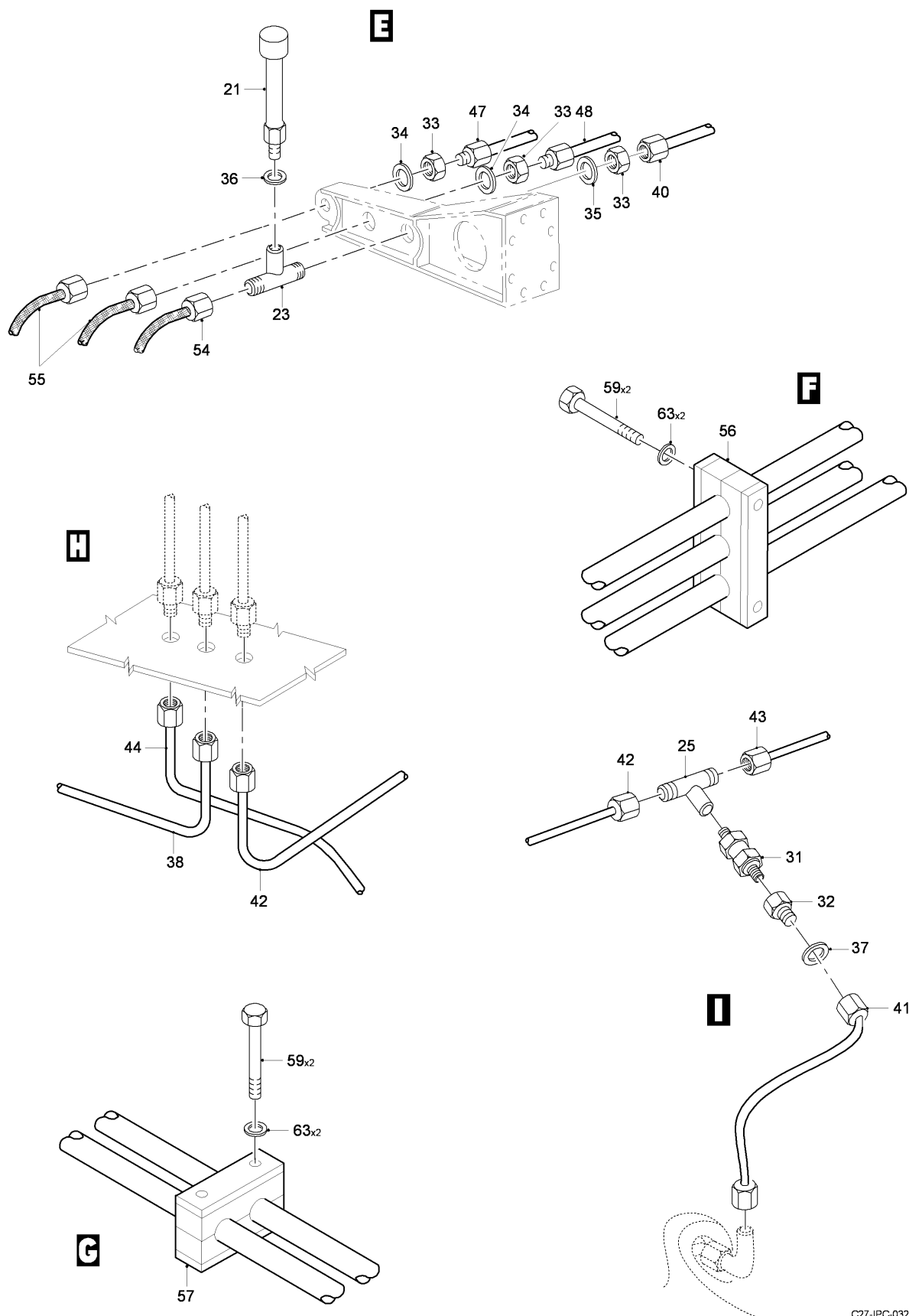
FIG 06 HYDRAULIC COMPONENT INSTL - NLG, Z31BB (SHEET 3 OF 3)
