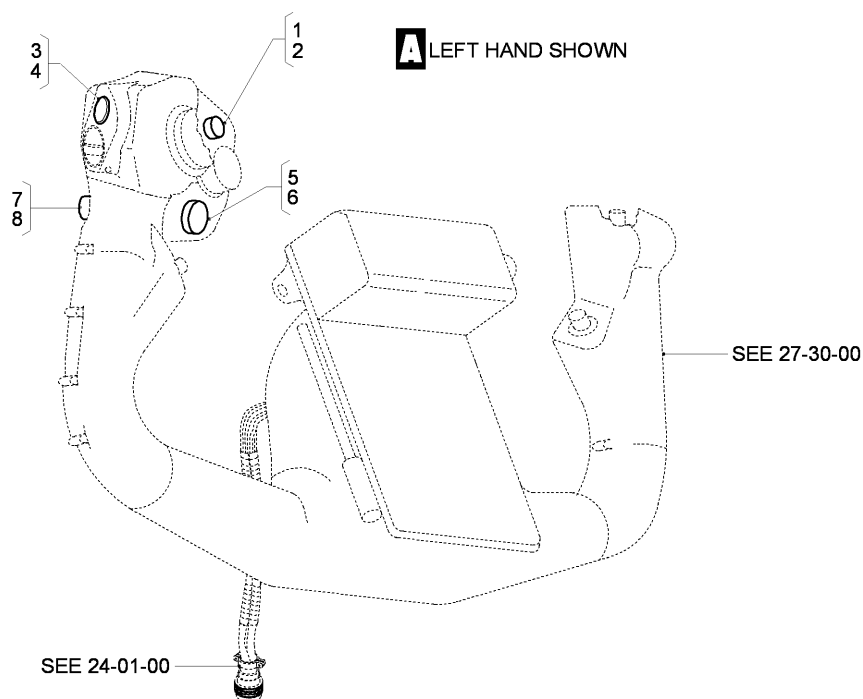
FIG 05 AUTOPILOT SWITCH INSTL, Z31AA, LH-RH (SHEET 1 OF 1)
