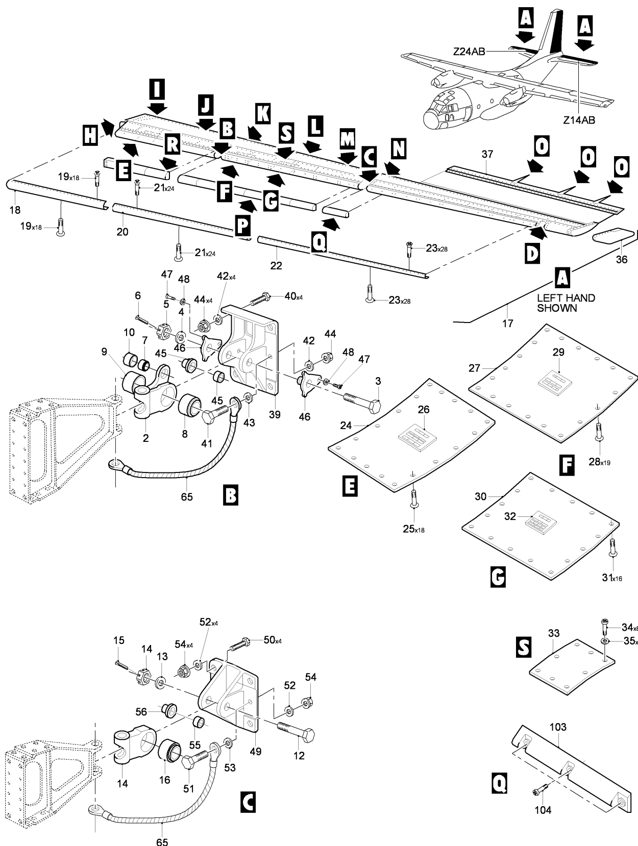
FIG 01 ELEVATOR CONTROL STRUCTURE INSTL, Z14AB-24AB, LH-RH (SHEET 1 OF 2)
