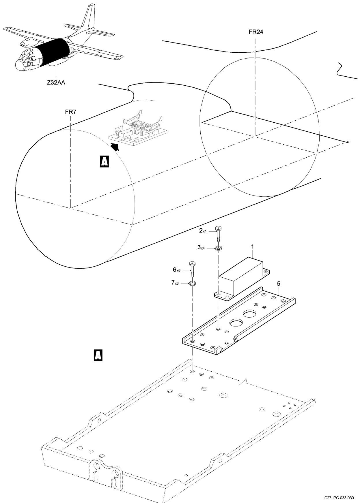
FIG 04 EMERGENCY EXIT BOX INSTL - INTERNAL LIGHT, Z32AA (SHEET 1 OF 1)
