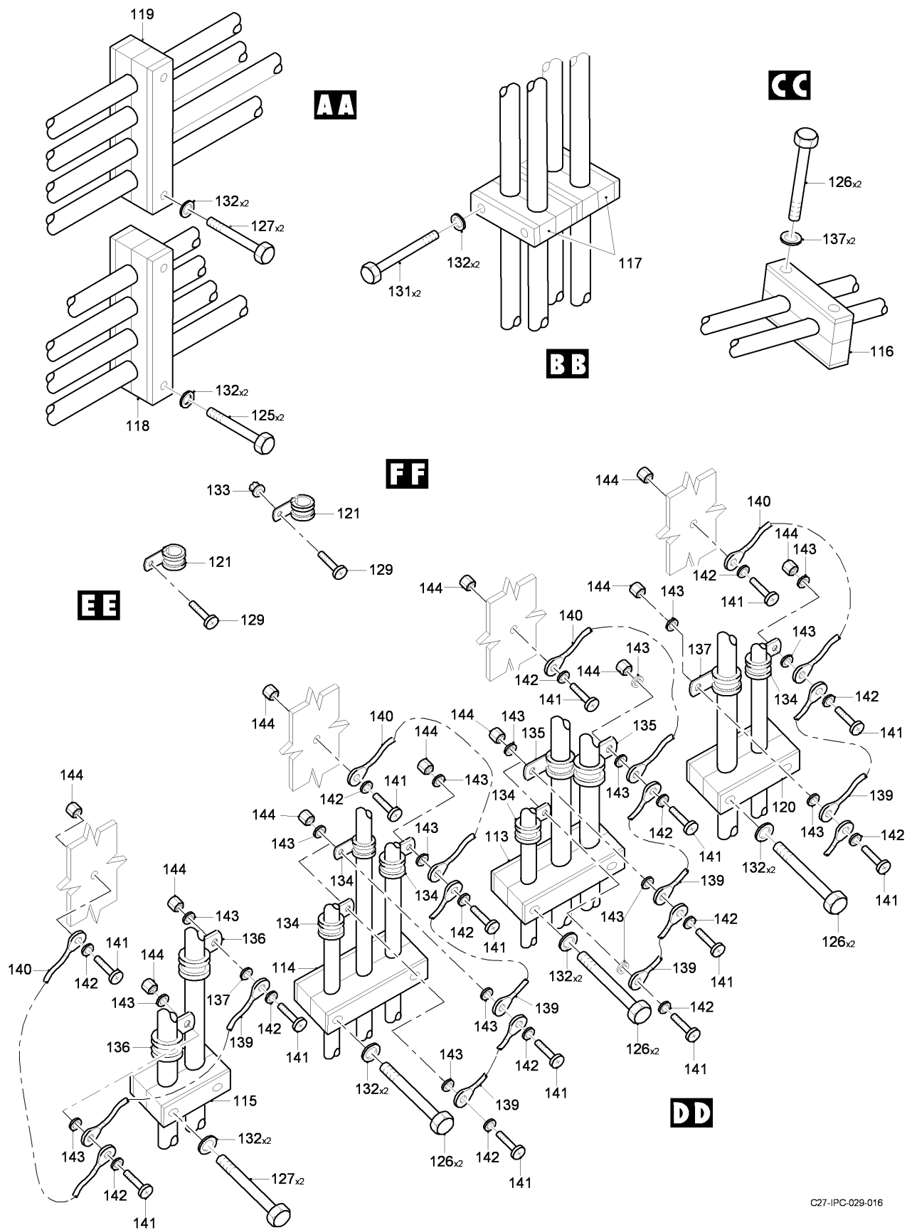
FIG 04 HYDRAULIC INSTL - CENTER FUSELAGE, Z32AC-32AD (SHEET 5 OF 6)
