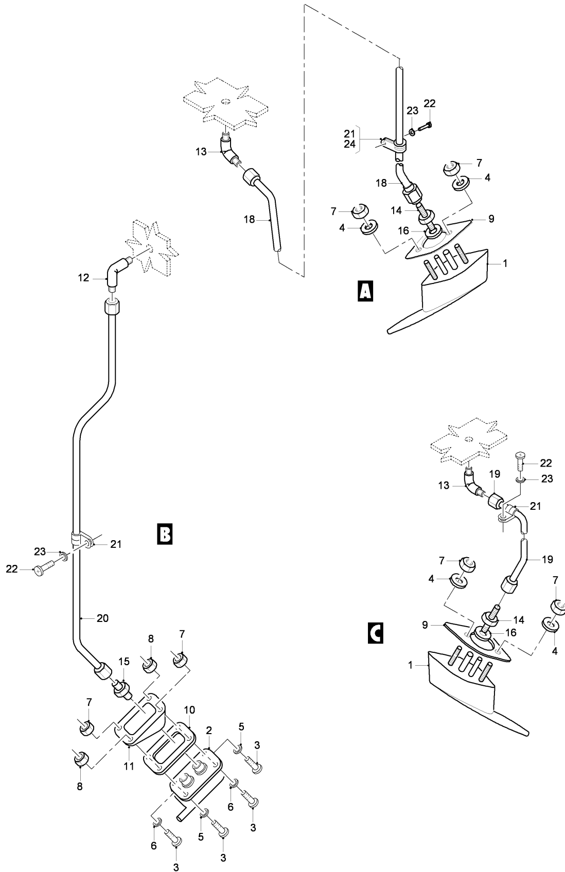
FIG 07 PITOT PROBE INSTL, Z31AA (SHEET 2 OF 2)
