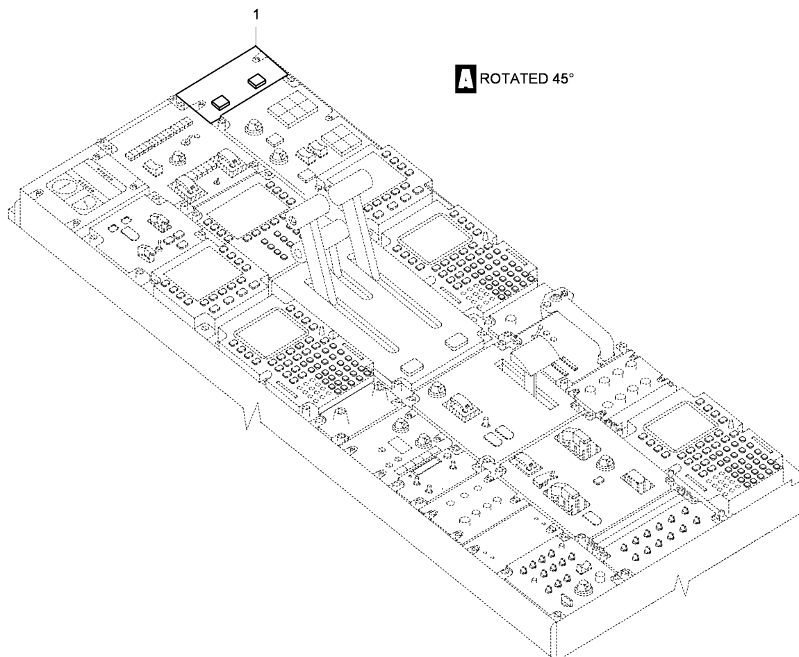
FIG 01 OBIGGS CONTROL PANEL INSTL, Z31AA (SHEET 1 OF 1)
