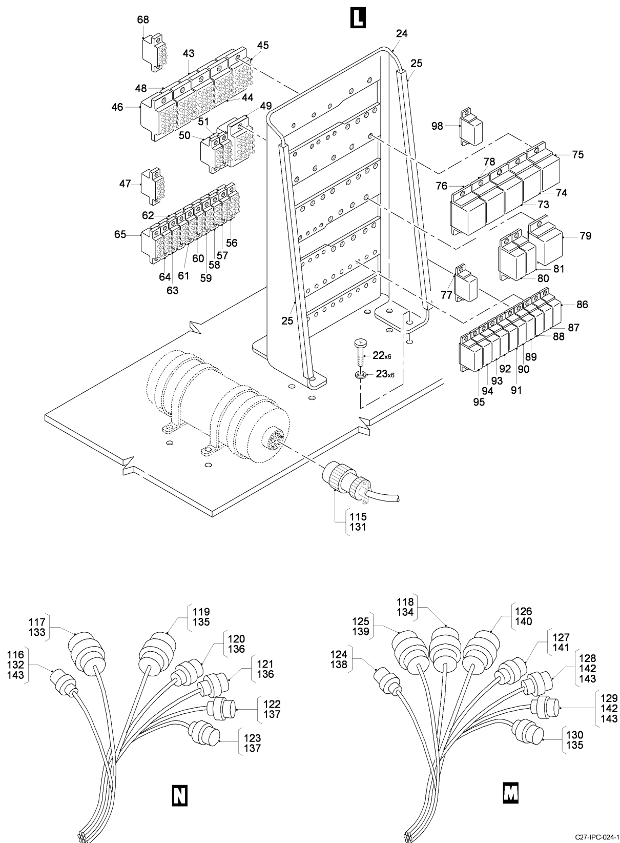
FIG 02 SECOND SHELF INSTL - ELECTRONIC COMPARTMENT, Z31AA (SHEET 3 OF 3)
