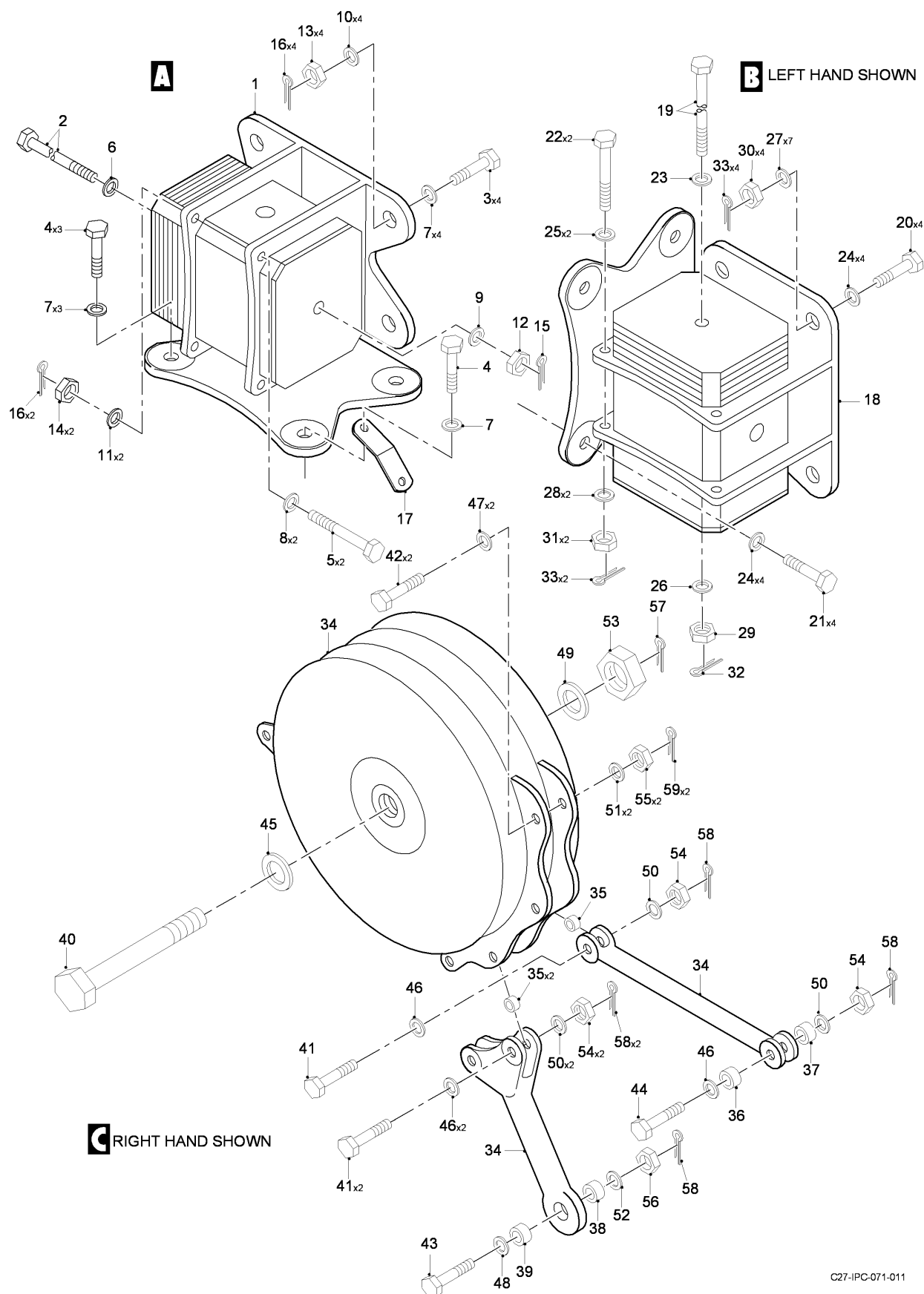
FIG 01 ENGINE MOUNTING INSTL, Z12AC-22AC (SHEET 2 OF 2)
