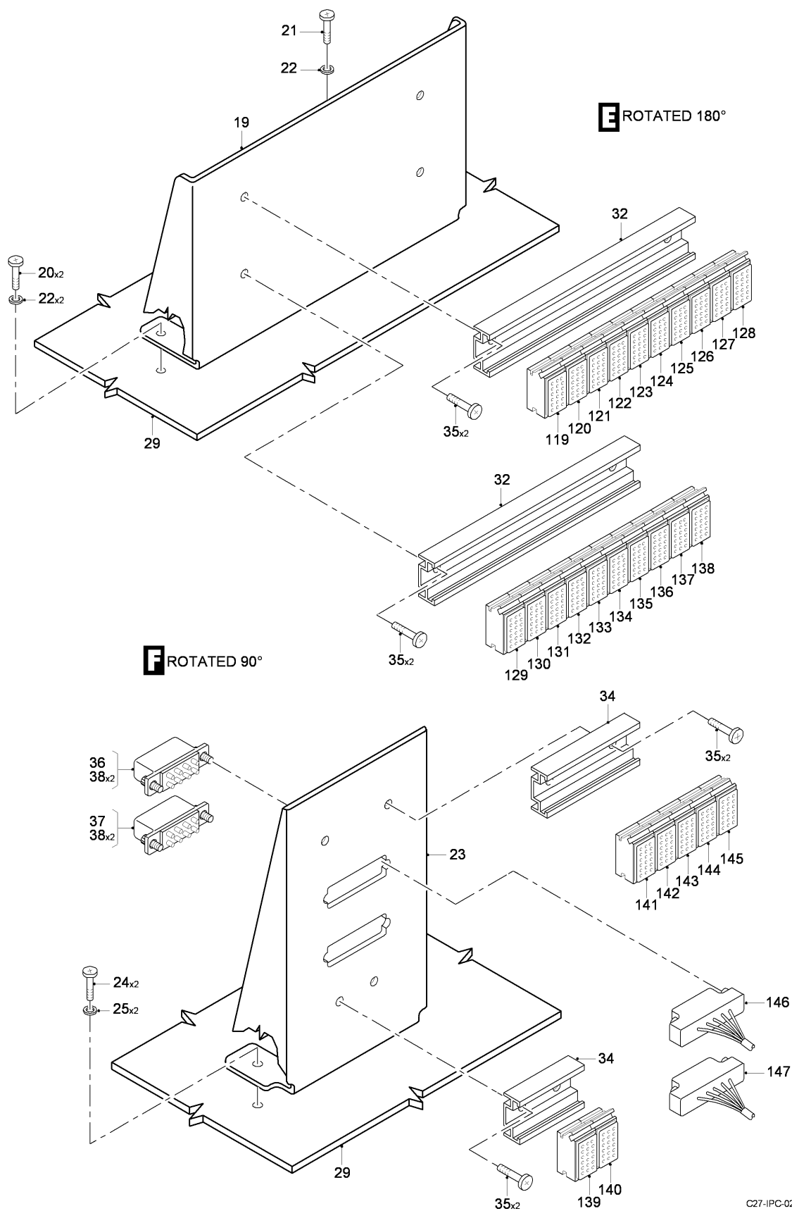
FIG 08 SECOND SHELF INSTL - ELECTRICAL COMPARTMENT, Z31AA (SHEET 3 OF 4)
