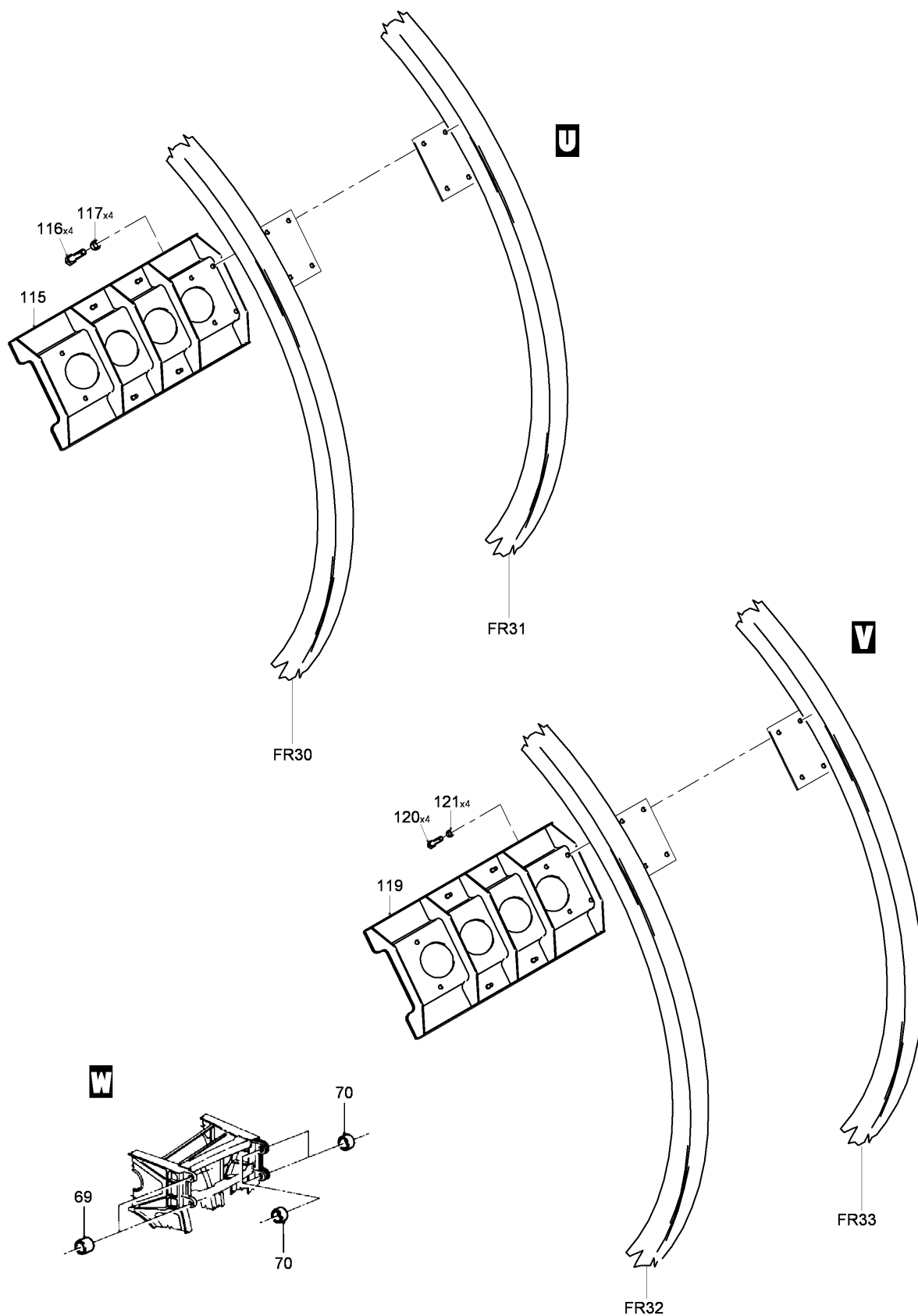
FIG 02 STRUCTURE INSTL, Z34AA (SHEET 4 OF 4)
