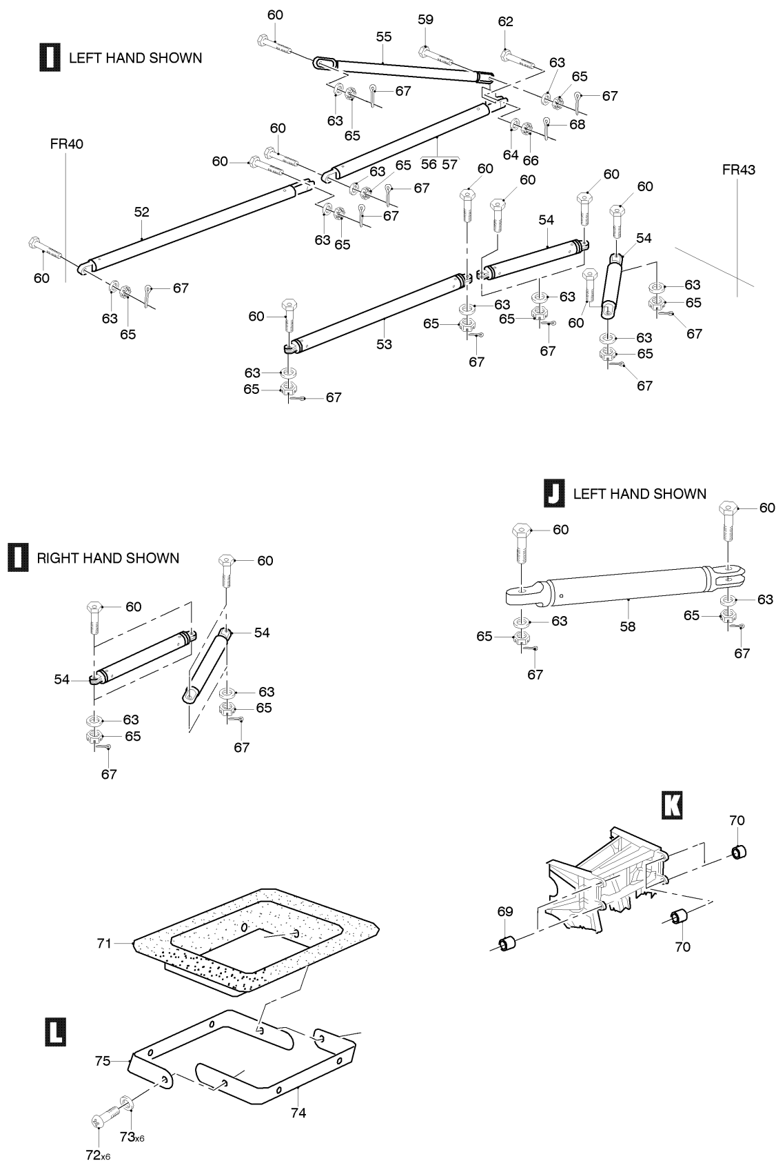
FIG 02 STRUCTURE INSTL, Z34AA (SHEET 2 OF 4)
