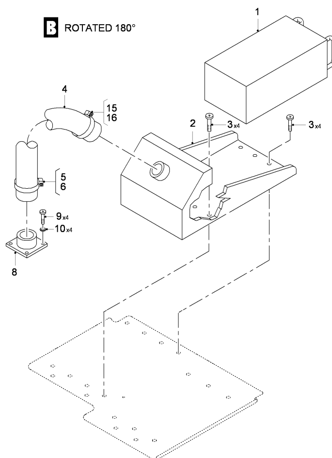
FIG 02 MISSION COMPUTER INSTL - ELECTRONIC COMPARTMENT, Z31AA (SHEET 1 OF 1)
