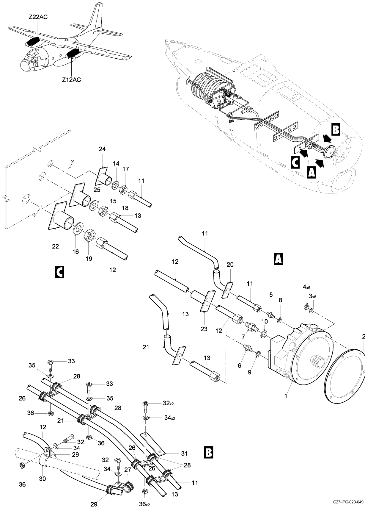
FIG 10 HYDRAULIC INSTL - FWD ENGINE, Z12AC-22AC, LH-RH (SHEET 1 OF 1)
