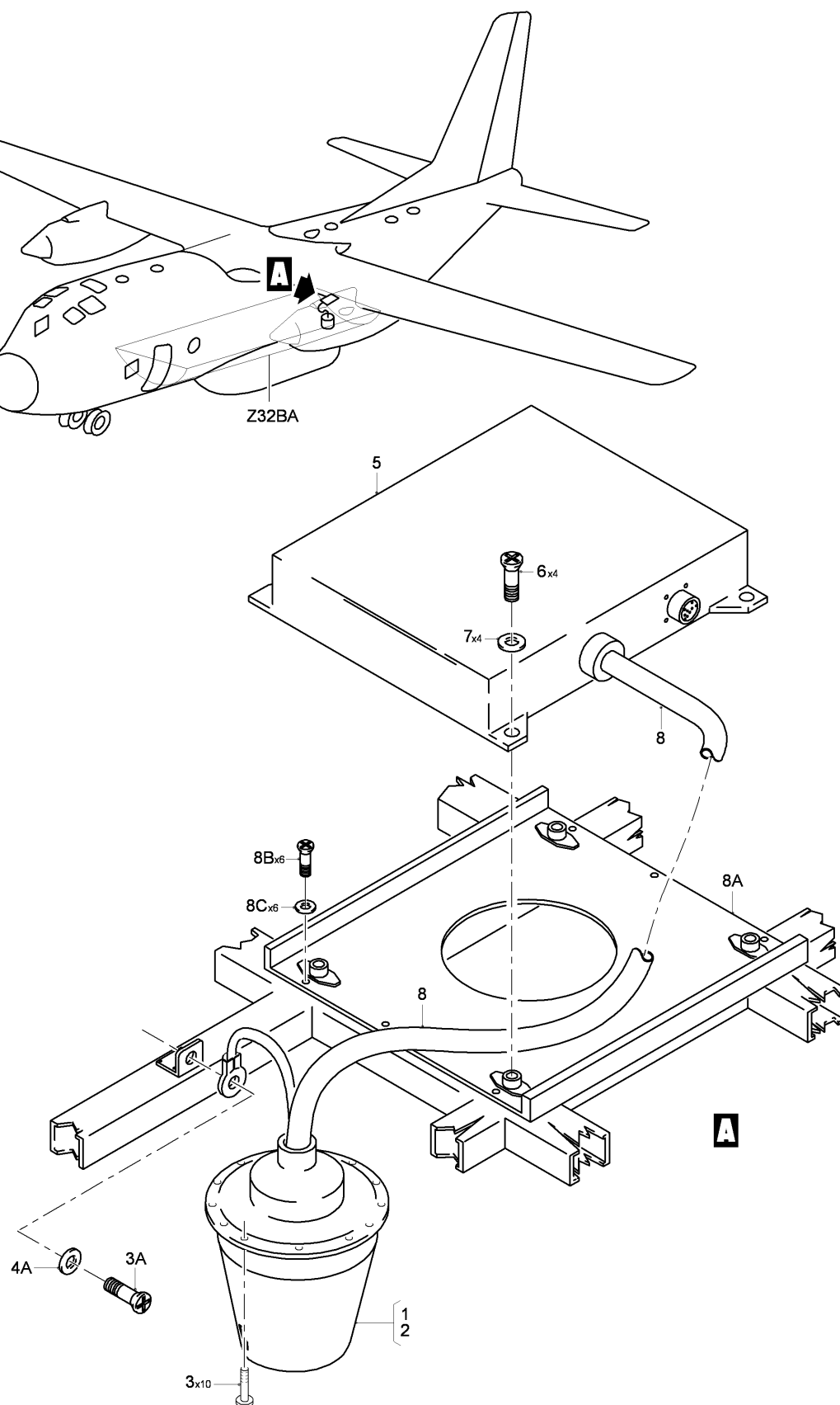
FIG 06 ANTICOLLISION LIGHT INSTL, Z32BA (SHEET 1 OF 1)
