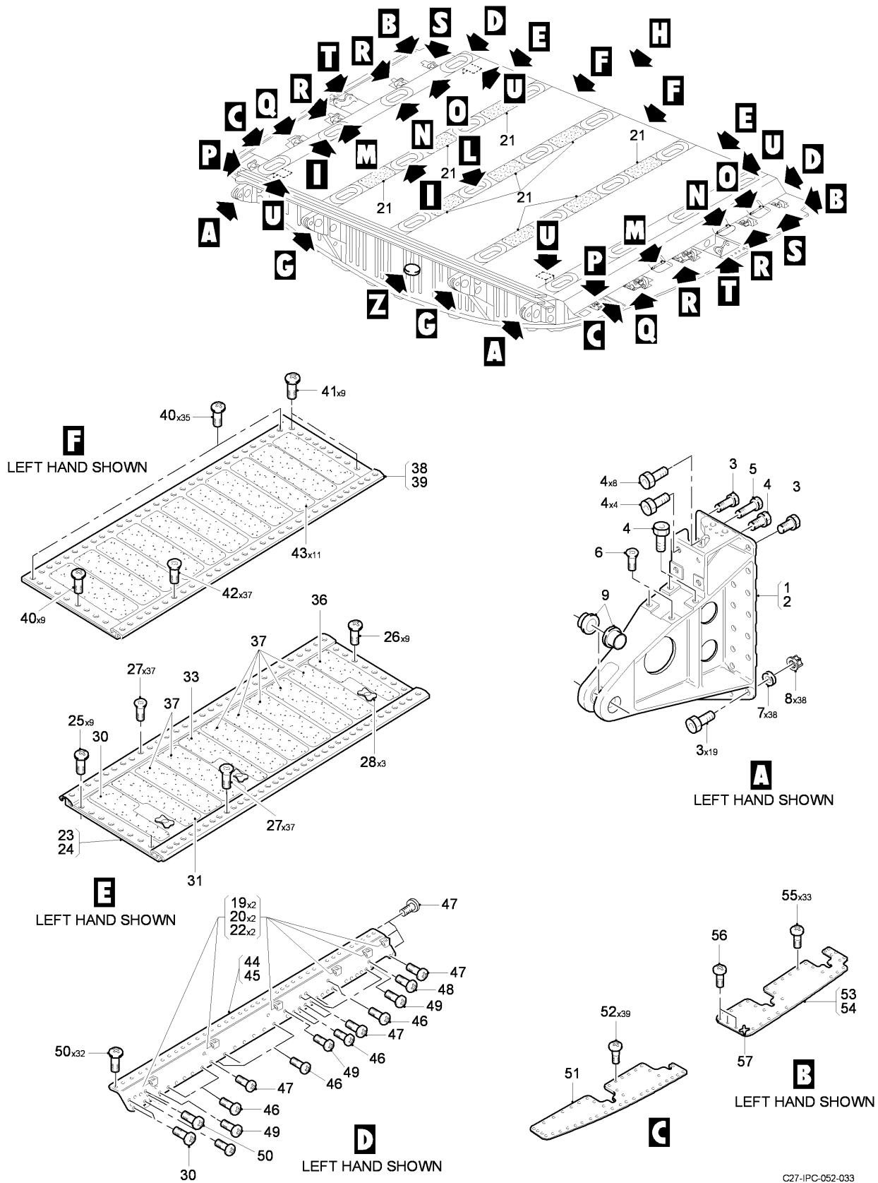
FIG 02 CARGO RAMP ASSY (SHEET 1 OF 6)
