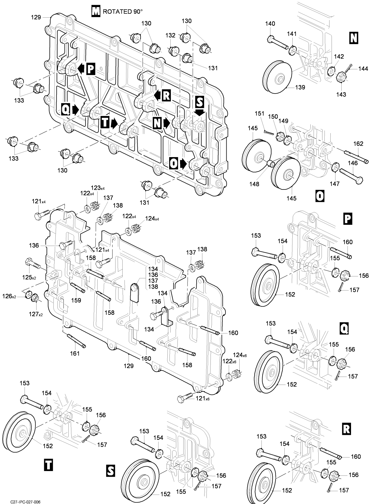
FIG 02 AILERON CONTROLS INSTL, Z31AA-31AB (SHEET 4 OF 5)
