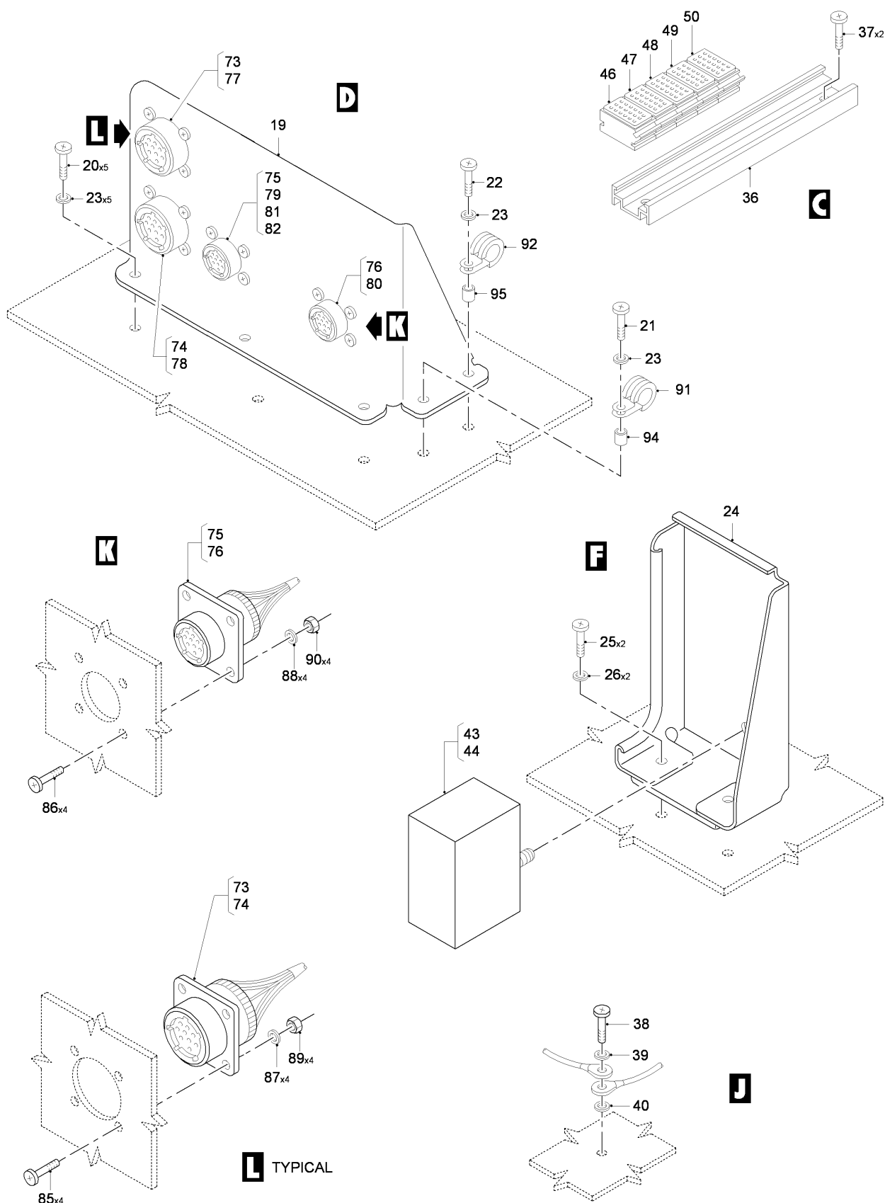
FIG 06 SIXTH SHELF INSTL - ELECTRONIC COMPARTMENT, Z31AA (SHEET 2 OF 3)
