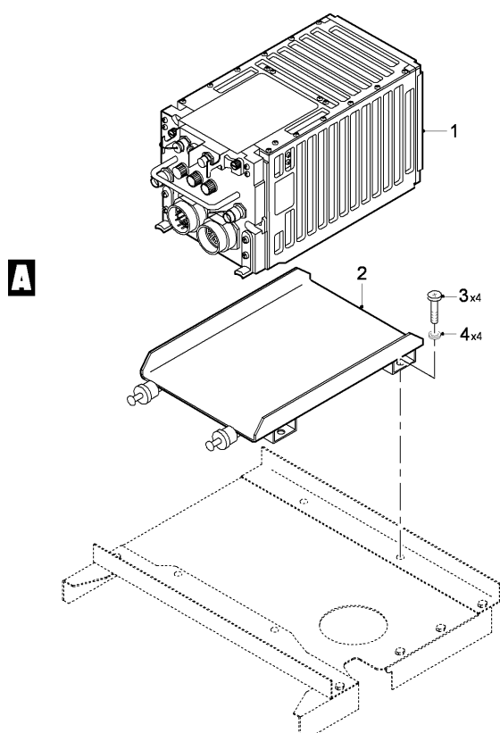
FIG 06 IFF SECOND INSTL, Z31BC (SHEET 1 OF 1)
