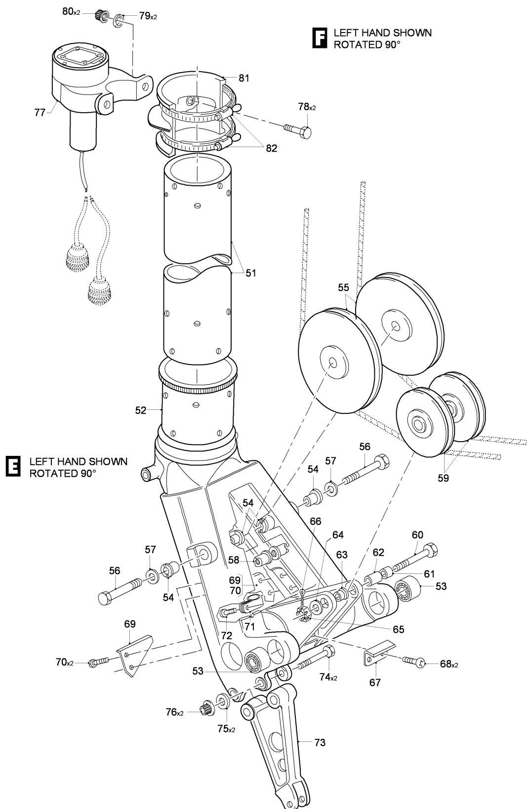
FIG 01 CONTROL COLUMN INSTL, Z31AA, LH-RH (SHEET 3 OF 3)
