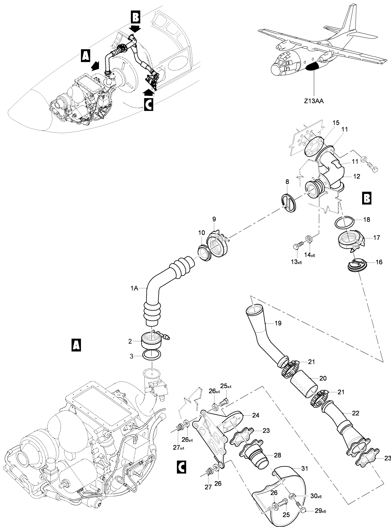
FIG 01 APU ENGINE STARTING INSTL, Z13AA (SHEET 1 OF 1)
