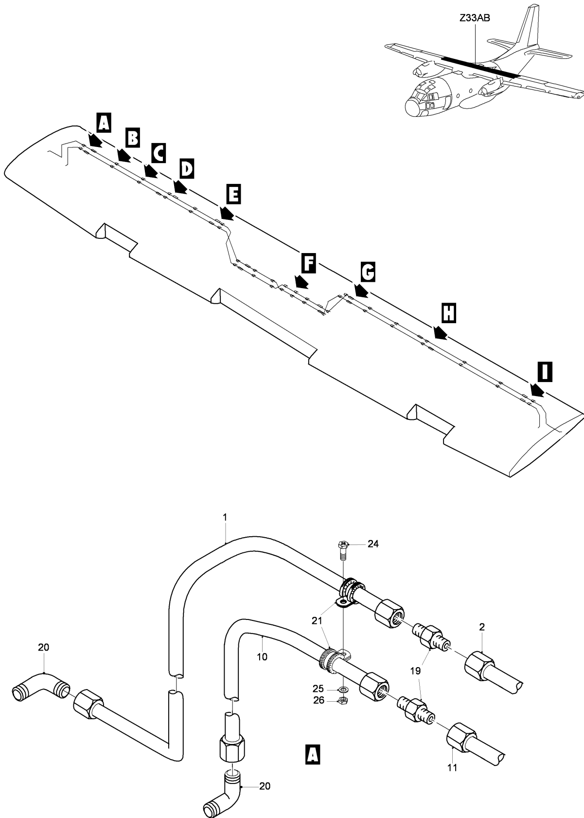
FIG 01 ENGINE FIRE EXTINGUISHING INSTL - CENTER WING, Z33AB (SHEET 1 OF 4)
