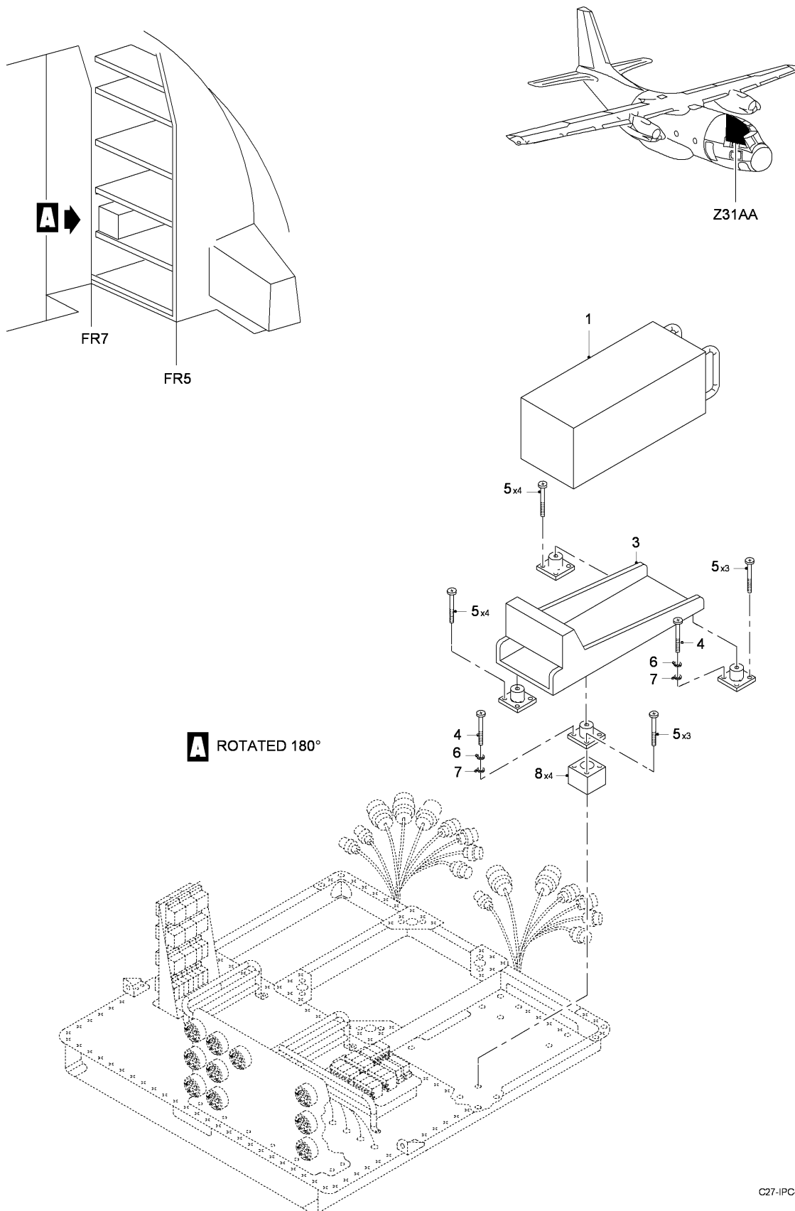
FIG 01 BUS INTERFACE UNIT INSTL - ELECTRONIC COMPARTMENT, Z31AA (SHEET 1 OF 1)
