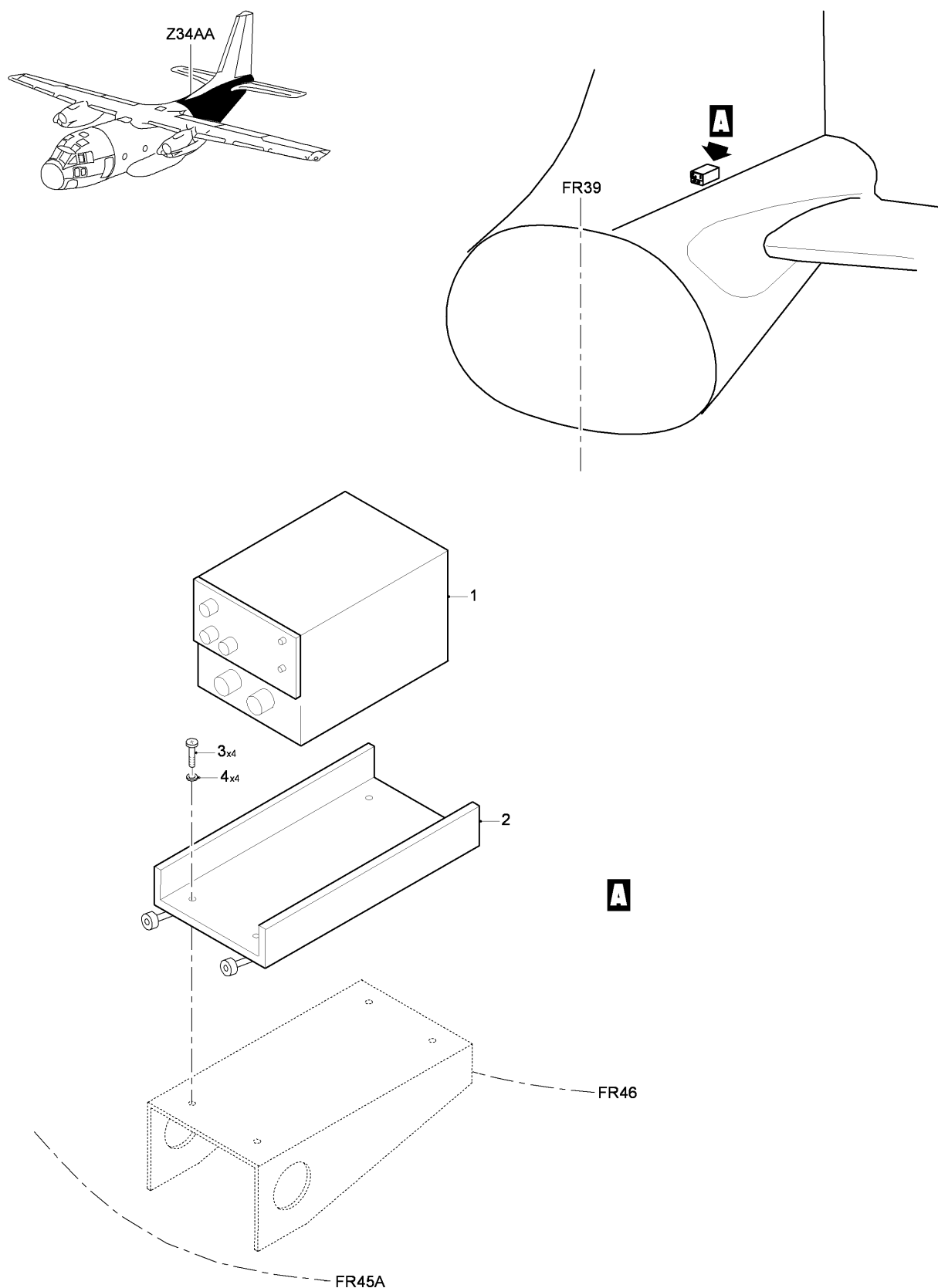
FIG 11 VHF/UHF RECEIVER/TRANSMITTER INSTL, Z34AA (SHEET 1 OF 1)
