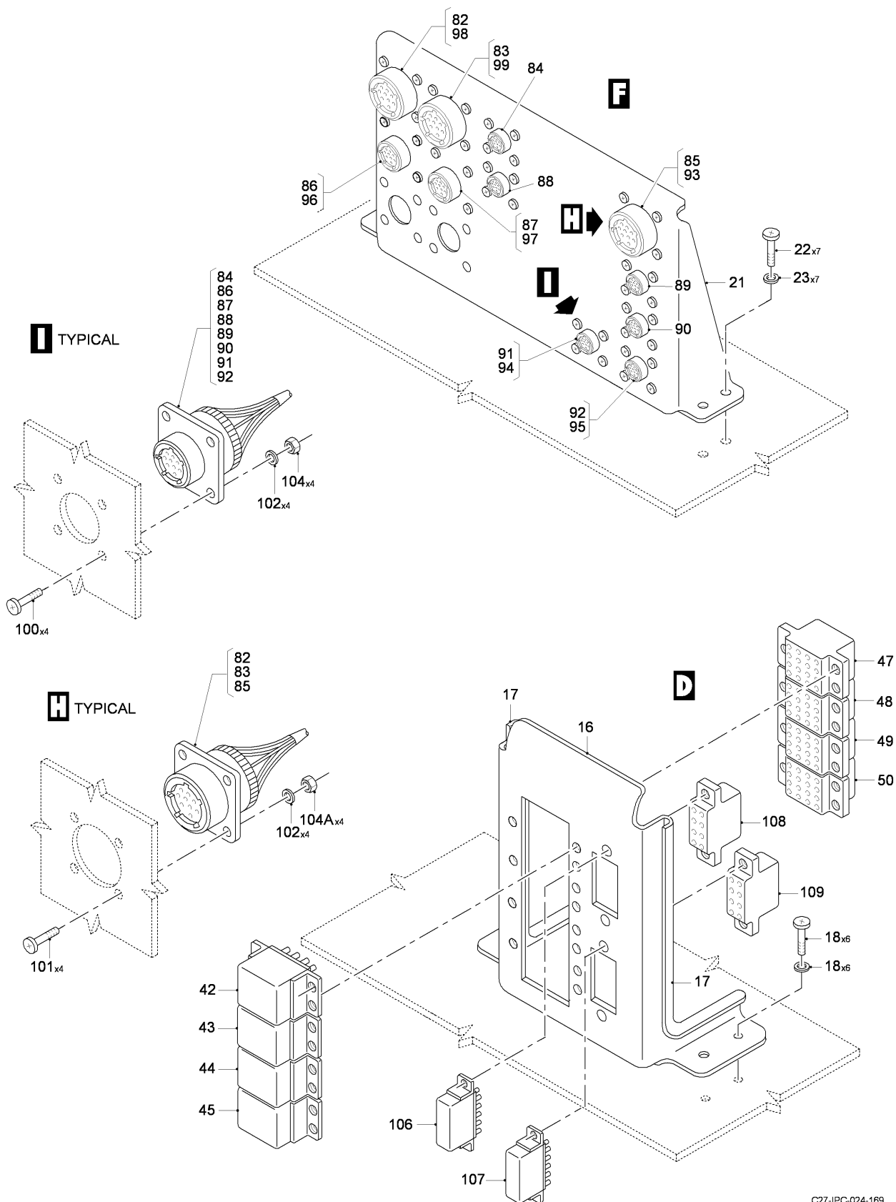
FIG 03 THIRD SHELF INSTL - ELECTRONIC COMPARTMENT, Z31AA (SHEET 3 OF 3)
