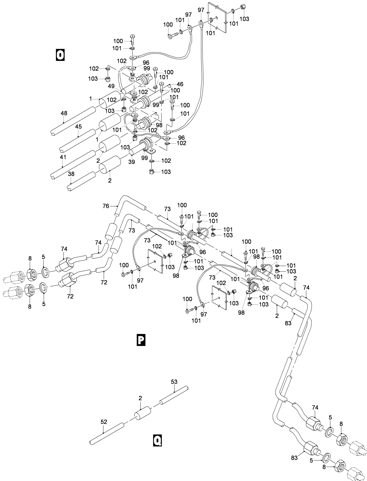
FIG 02 HYDRAULIC INSTL - CENTER FUSELAGE, LOWER, Z32BA (SHEET 6 OF 8)
