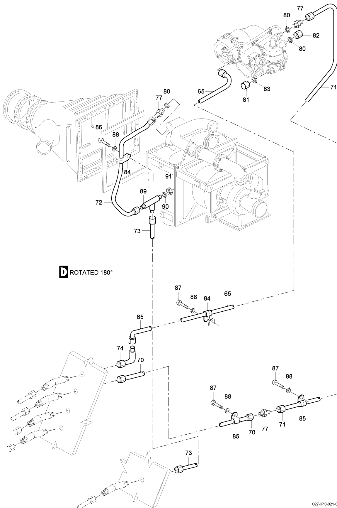
FIG 02 AIR CONDITIONING INSTL - MLG RH FAIRING, Z23AA (SHEET 3 OF 3)
