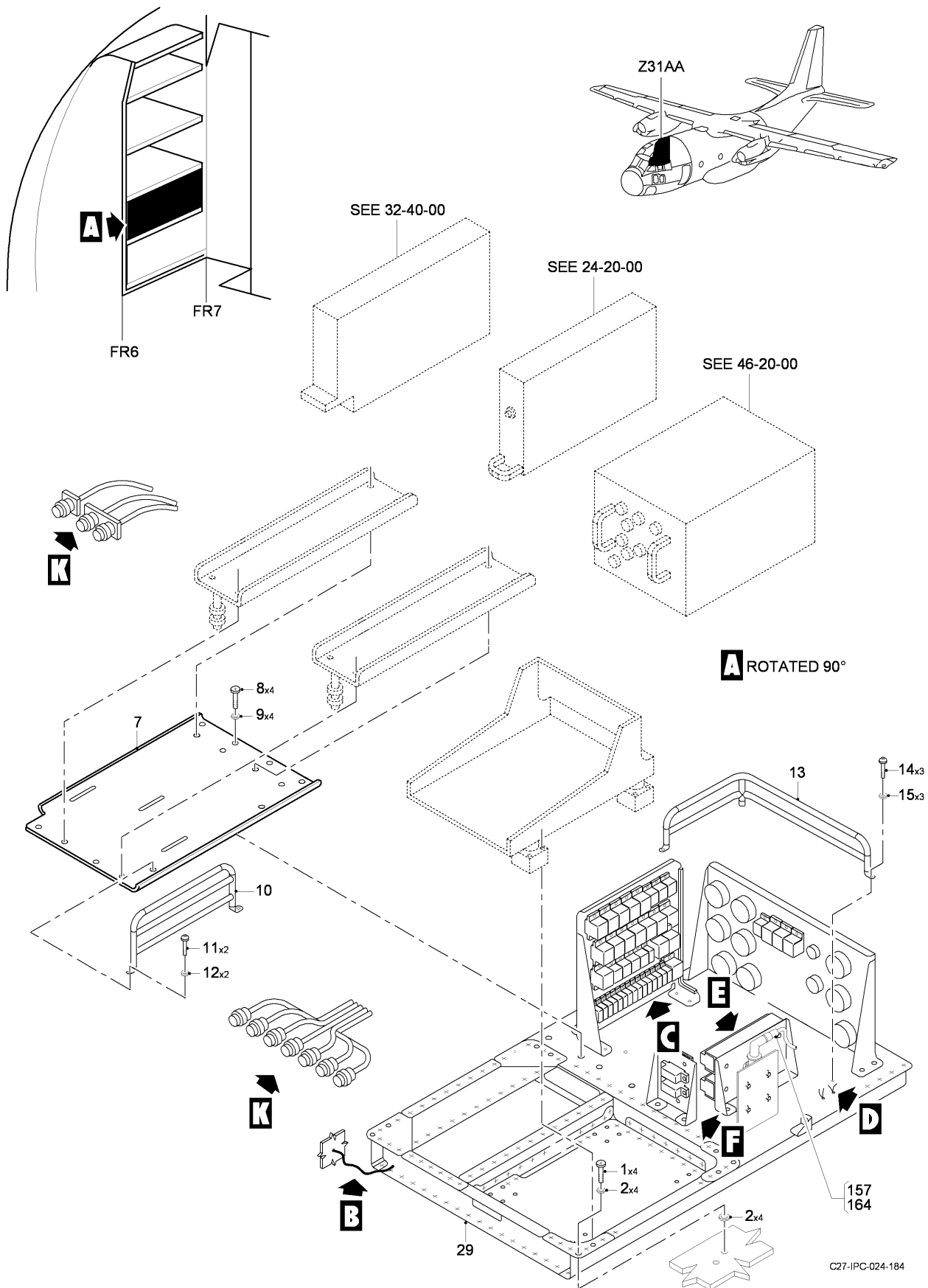
FIG 08 SECOND SHELF INSTL - ELECTRICAL COMPARTMENT, Z31AA (SHEET 1 OF 4)
