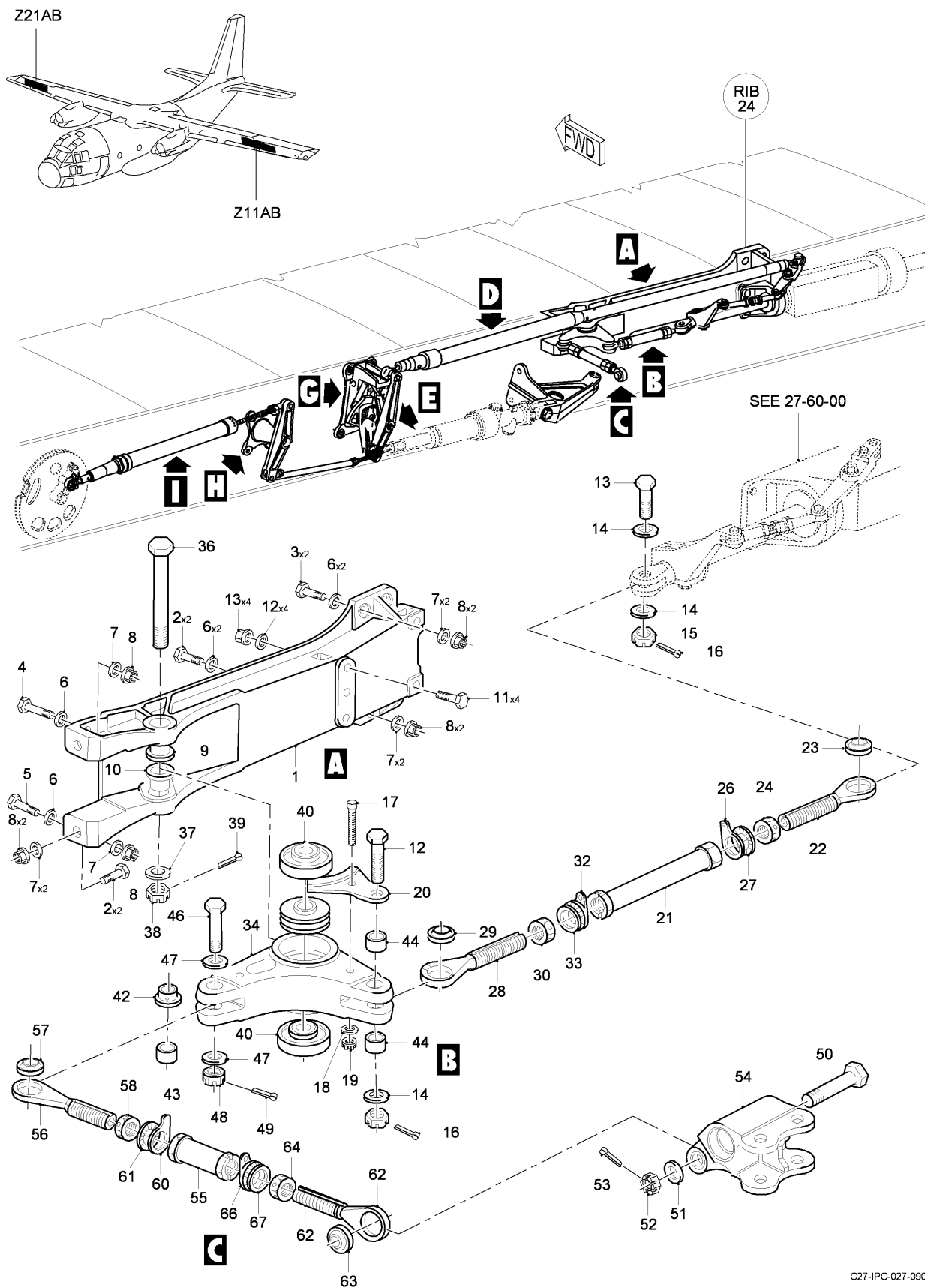
FIG 03 SPOILER CONTROLS INSTL, Z11AB-21AB, LH-RH (SHEET 1 OF 3)
