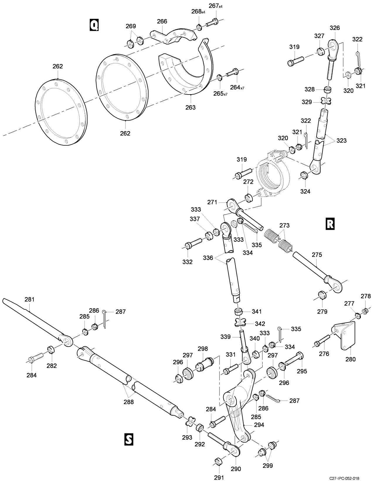
FIG 03 PARATROOPS DOOR ASSY, LH-RH (SHEET 7 OF 8)
