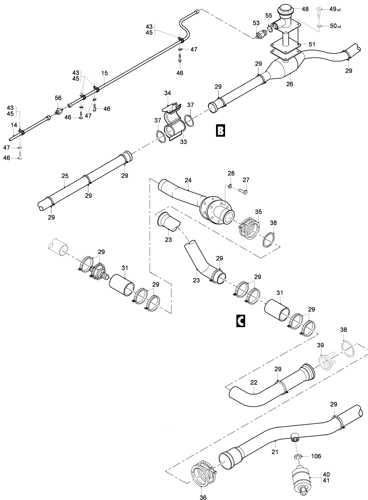
FIG 01 FUEL TANK EXPLOSION PROTECTION SYSTEM INSTL, Z32BA (SHEET 2 OF 3)
