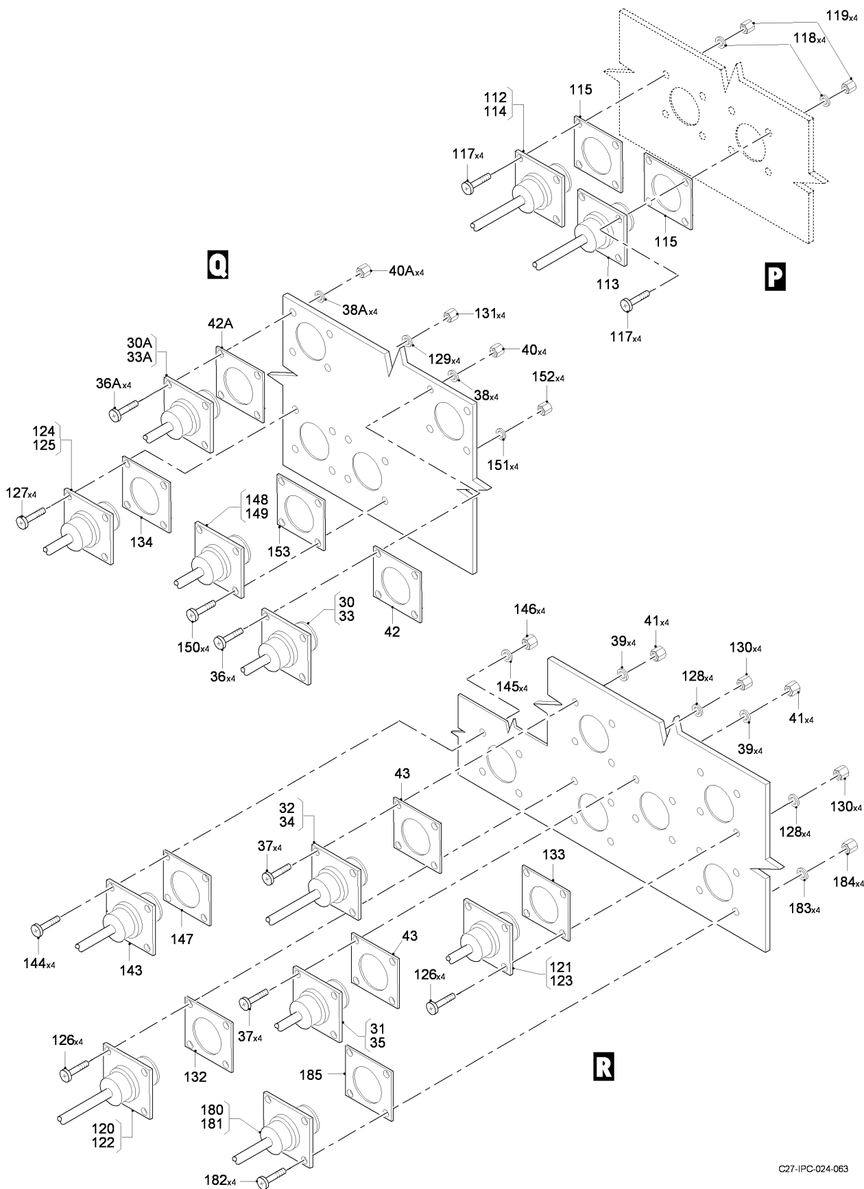
FIG 15 ELECTRICAL AND ELECTRONICS INSTL, Z31AB-32AA-32AB-32AC, LH (SHEET 7 OF 9)
