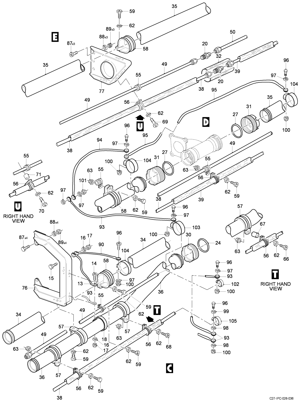
FIG 08 SINGLE POINT REFUEL AND FUEL SUPPLY INSTL, Z11AA-21AA, LH-RH (SHEET 2 OF 6)
