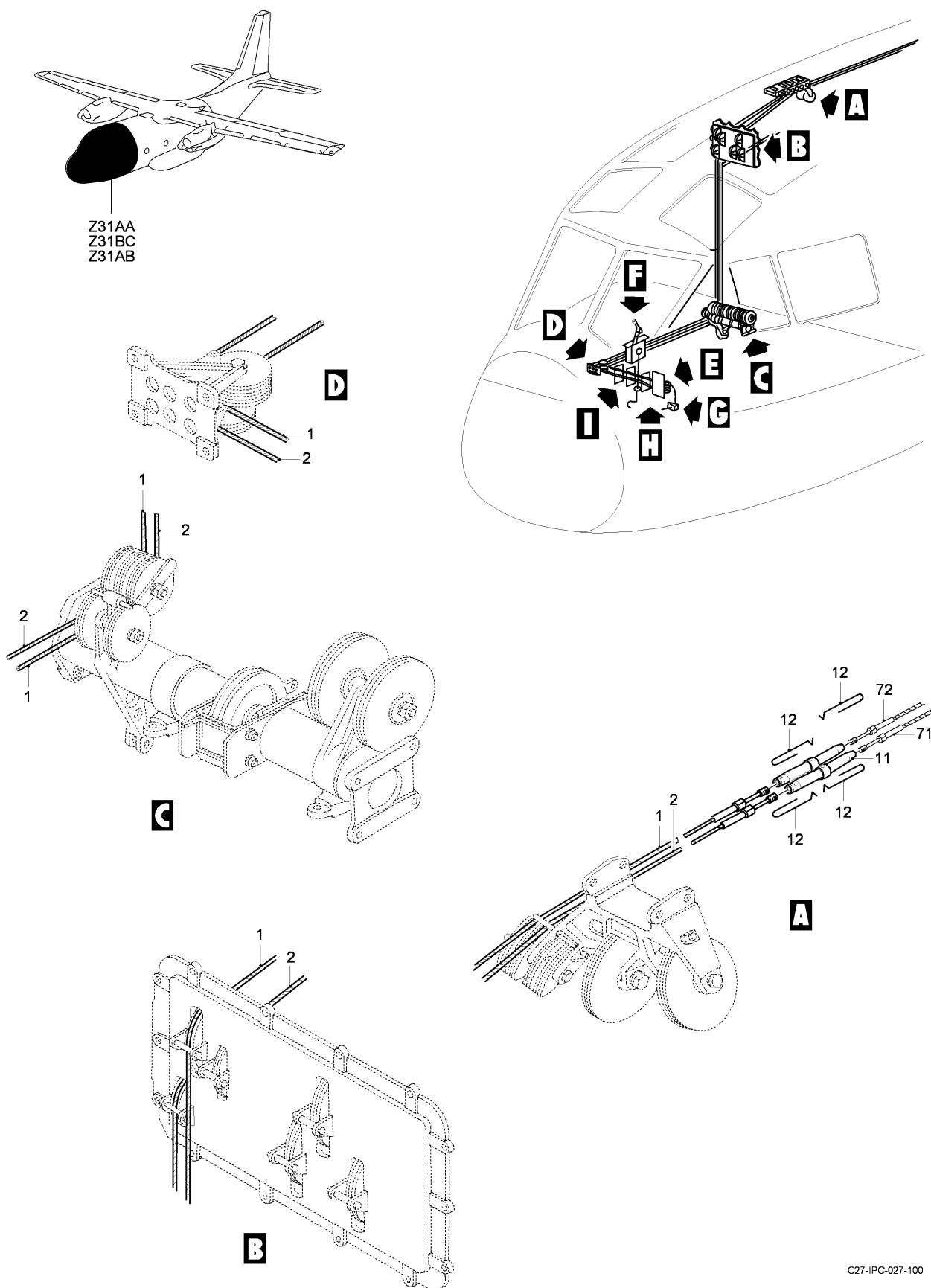
FIG 01 CONTROLS LOKING INSTL, Z31AB-31BB (SHEET 1 OF 4)
