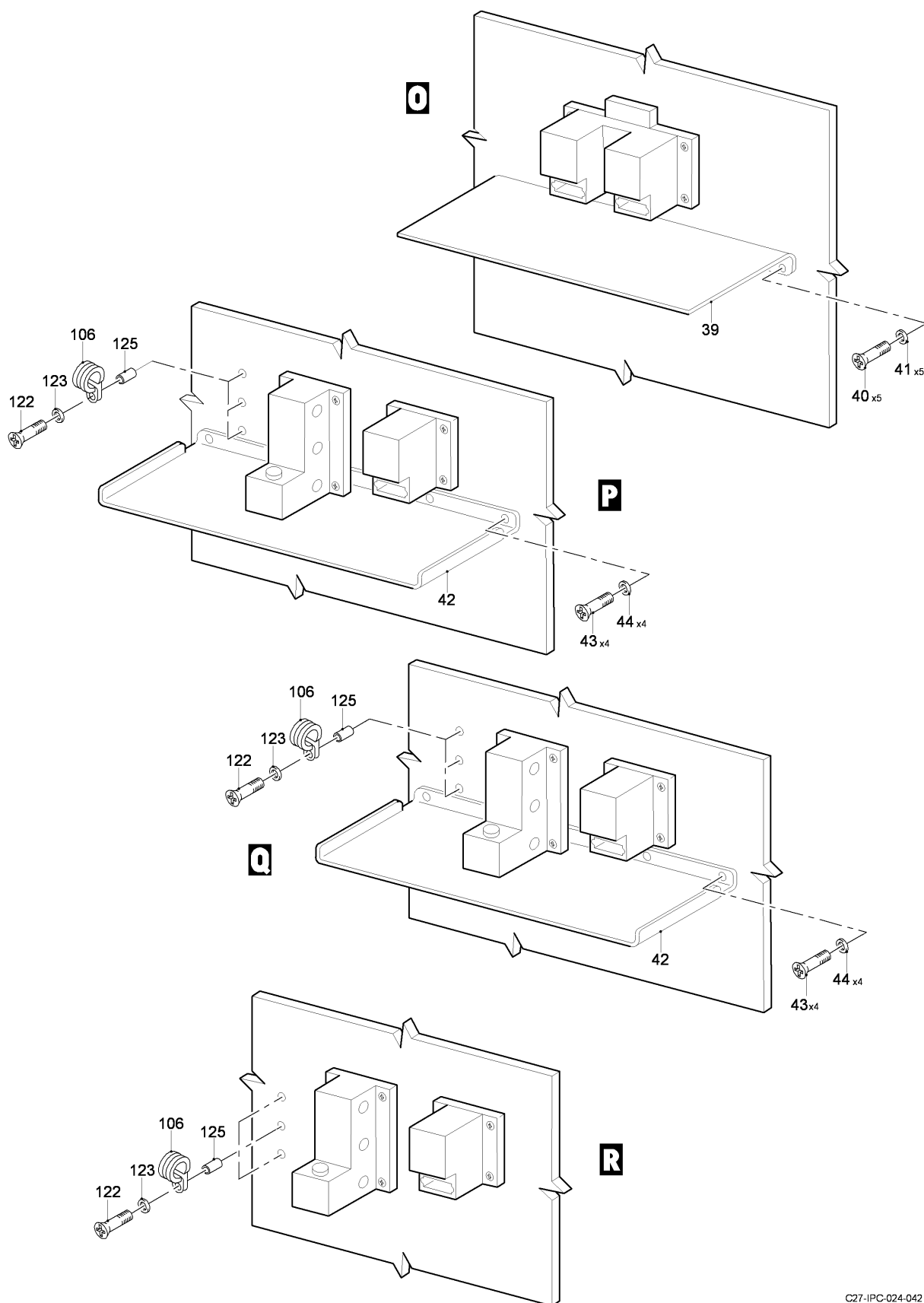
FIG 11 ELECTRICAL AND ELECTRONICS INSTL, Z31AA (SHEET 6 OF 6)
