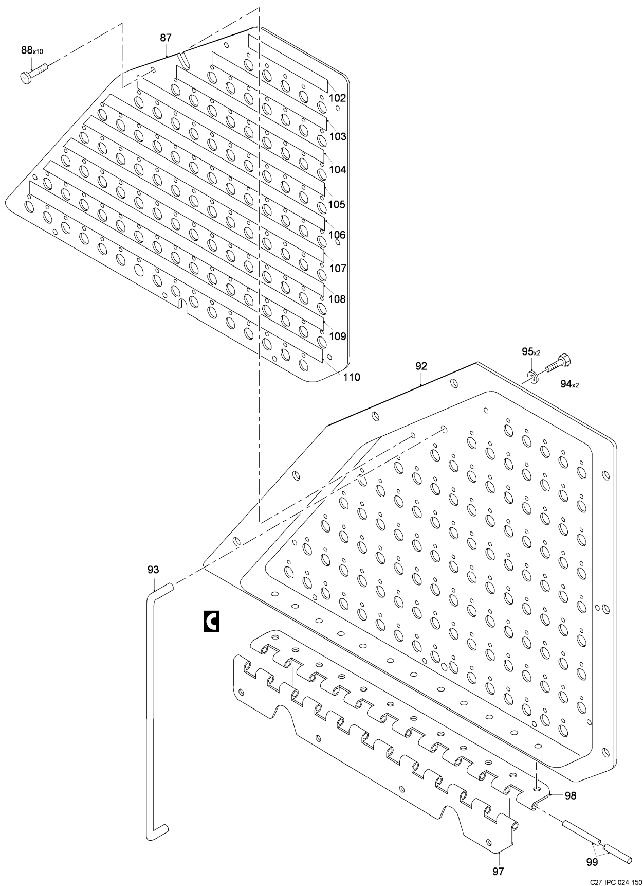
FIG 02 CIRCUIT BREAKER PANEL NO. 1 INSTL, Z31AA (SHEET 2 OF 3)
