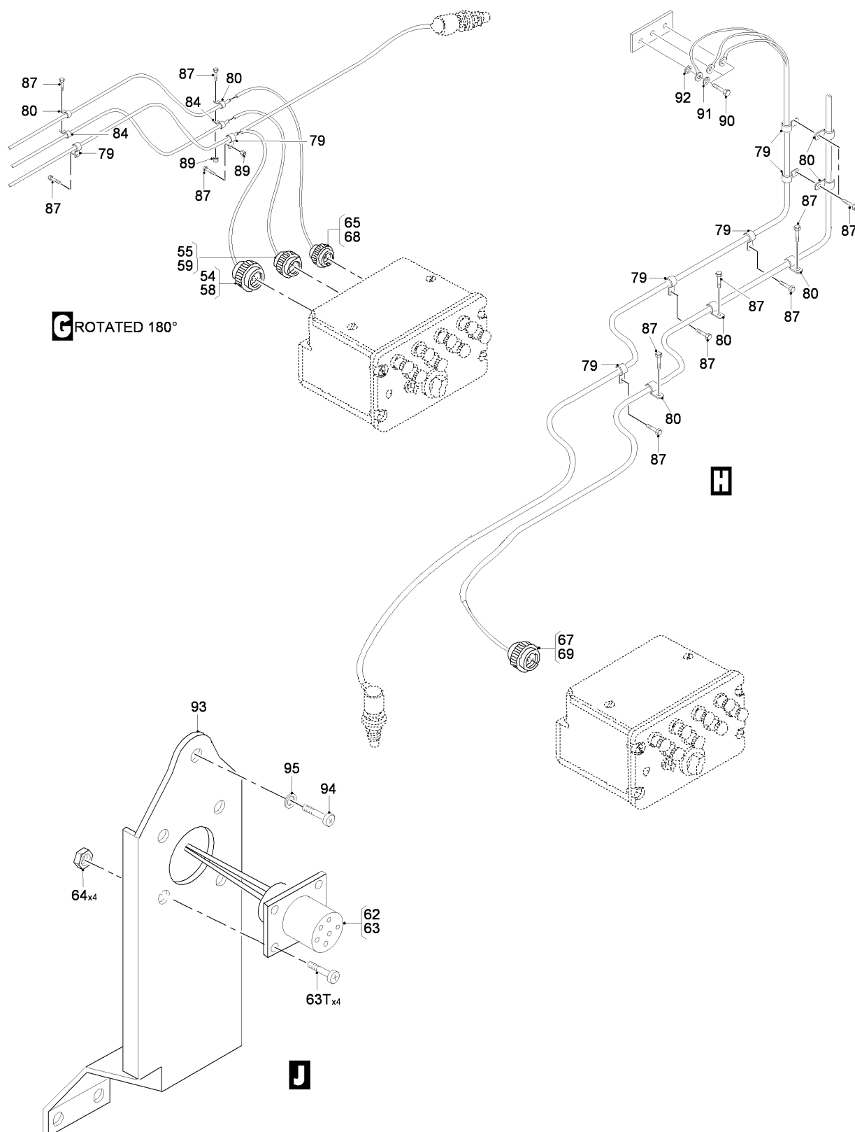
FIG 19 ELECTRICAL AND ELECTRONICS INSTL, Z32AD (SHEET 4 OF 5)
