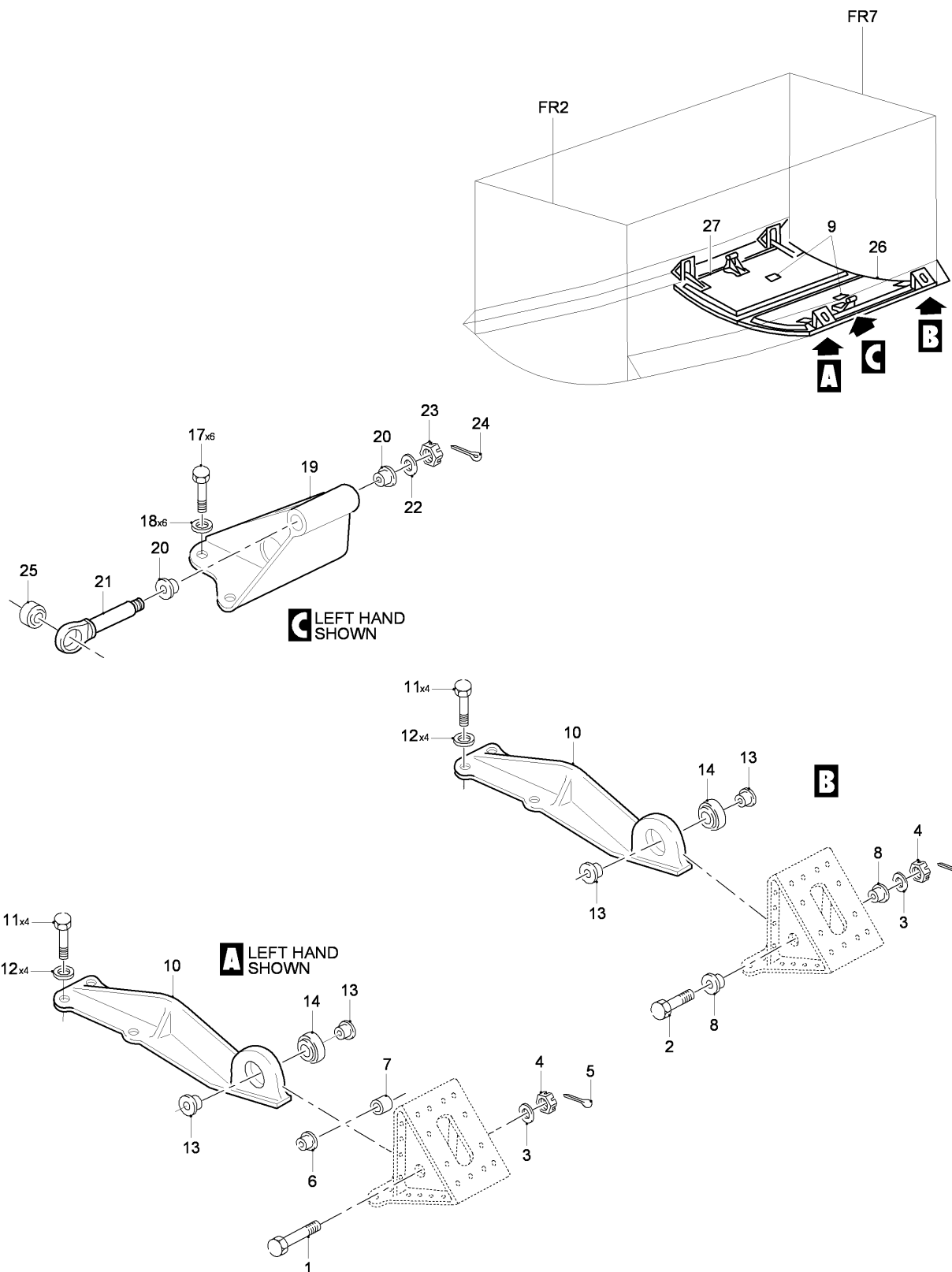
FIG 04 FITTING BAY DOOR INSTL - NLG, Z31BB, LH-RH (SHEET 1 OF 1)
