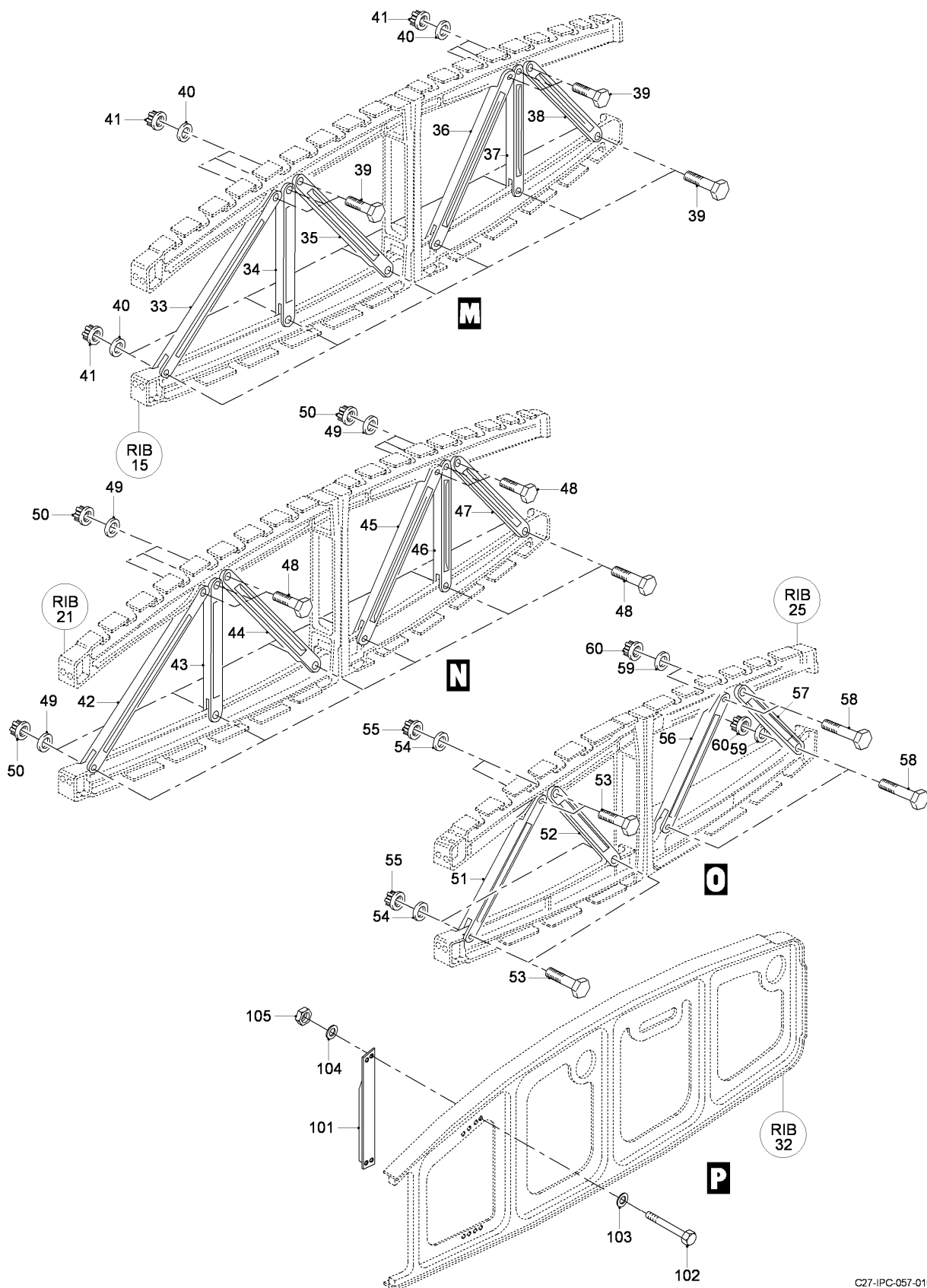
FIG 02 STRUCTURE INSTL - OUTER WING, Z11AB-21AB, LH-RH (SHEET 3 OF 4)
