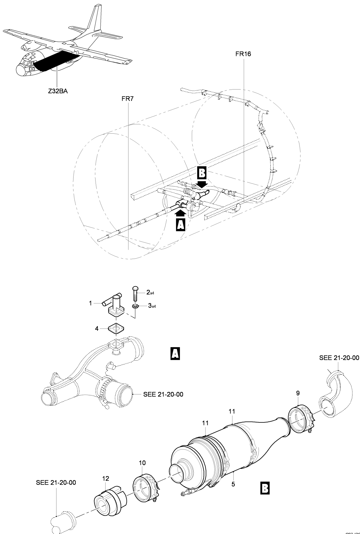
FIG 01 AIR CONDITIONING COOLING INSTL - CENTER FUSELAGE, Z32BA (SHEET 1 OF 1)
