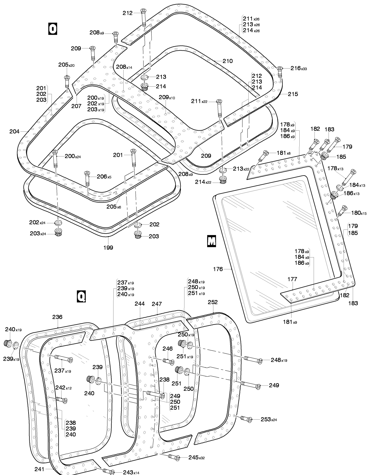
FIG 01 WINDOWS CABIN INSTL, Z31AA (SHEET 5 OF 6)
