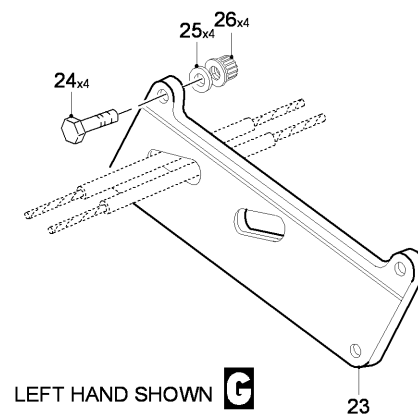
FIG 04 ELEVATOR CONTROLS INSTL, Z32AA-32AB-32AC-32AD-34AA (SHEET 2 OF 5)
