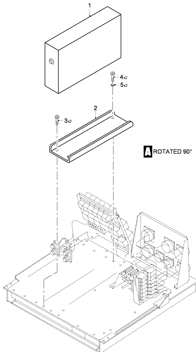
FIG 04 GCU ALTERNATOR INSTL, Z31AA (SHEET 1 OF 1)
