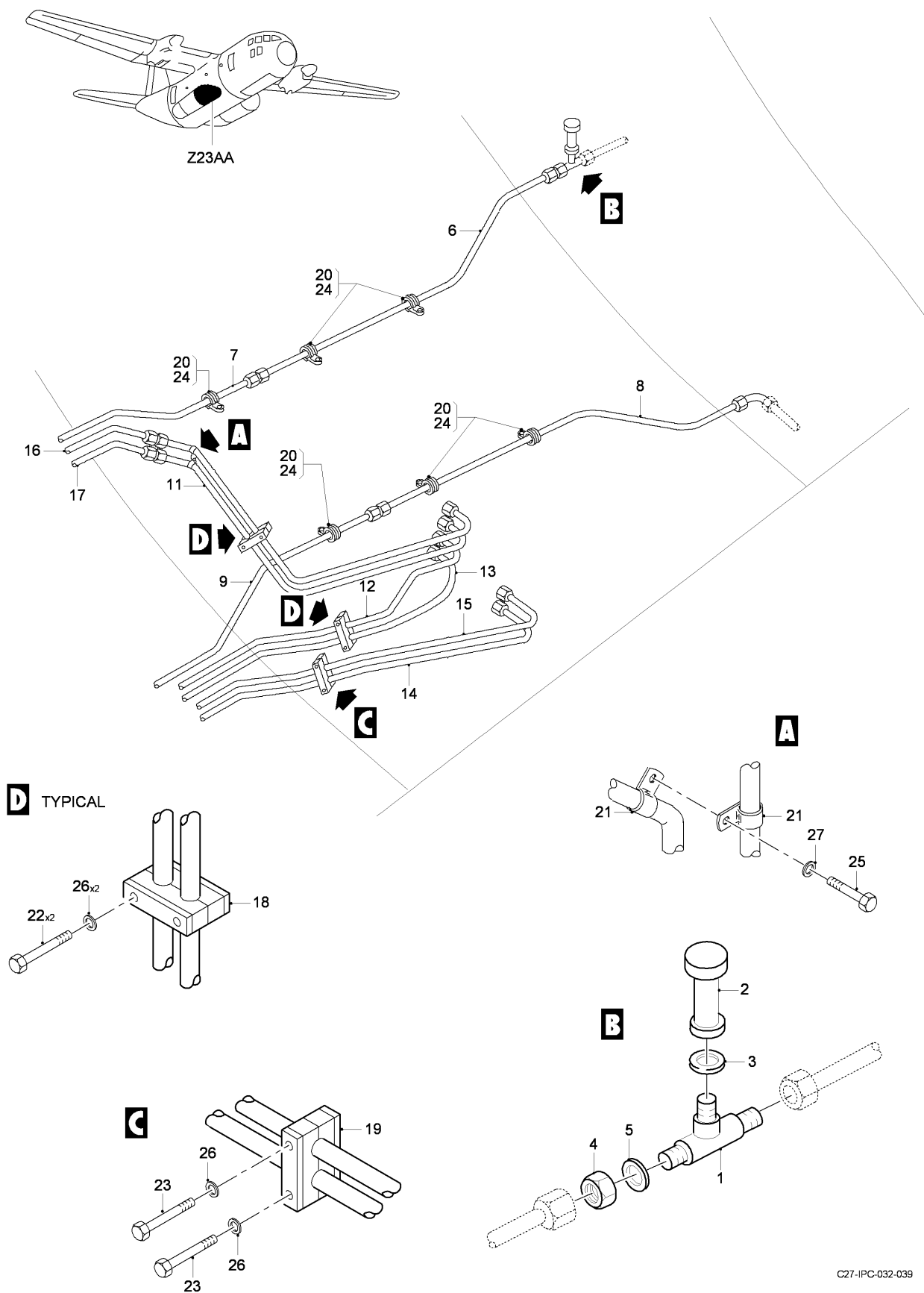
FIG 04 HYDRAULIC INSTL - MLG FRAME 16 TO 21, Z23AA, RH (SHEET 1 OF 1)
