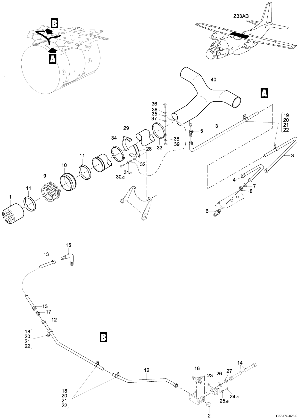
FIG 01 IN-FLIGHT REFUELLING RECEIVER SYSTEM INSTL, Z33AB (SHEET 1 OF 1)
