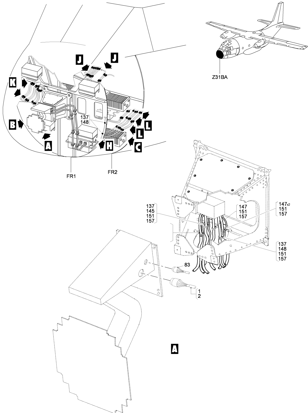
FIG 01 ELECTRICAL AND ELECTRONICS INSTL - RADOME AND FWD BAY, Z31BA (SHEET 1 OF 5)
