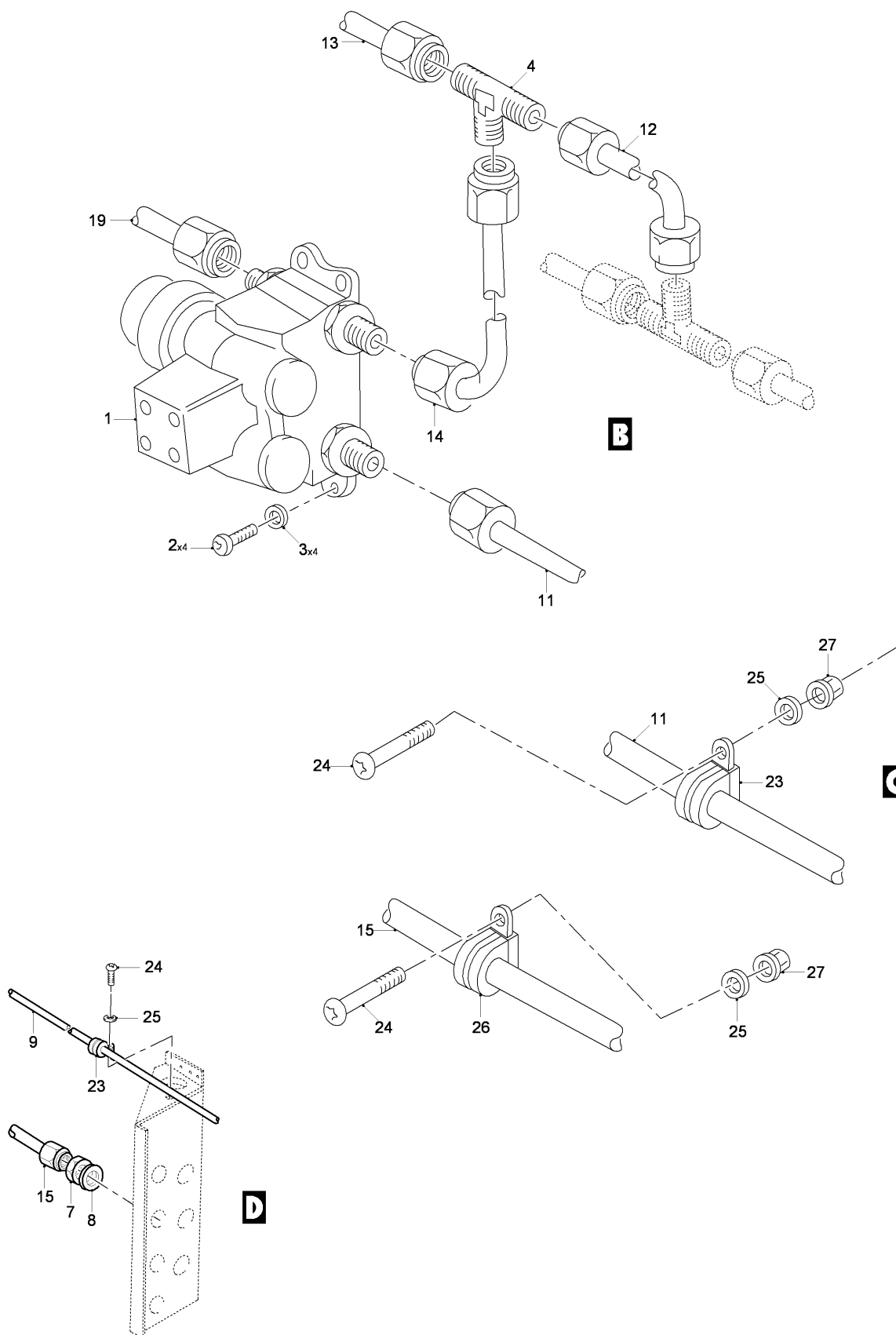
FIG 01 VALVE LIFT DUMPER CONTROLS INSTL, Z33AB (SHEET 2 OF 2)
