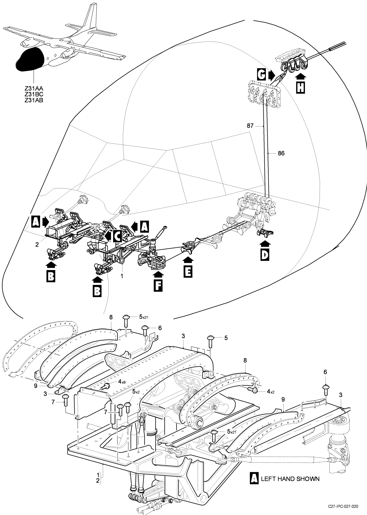
FIG 03 RUDDER CONTROLS INSTL, Z31AA-31BC-31AB (SHEET 1 OF 5)
