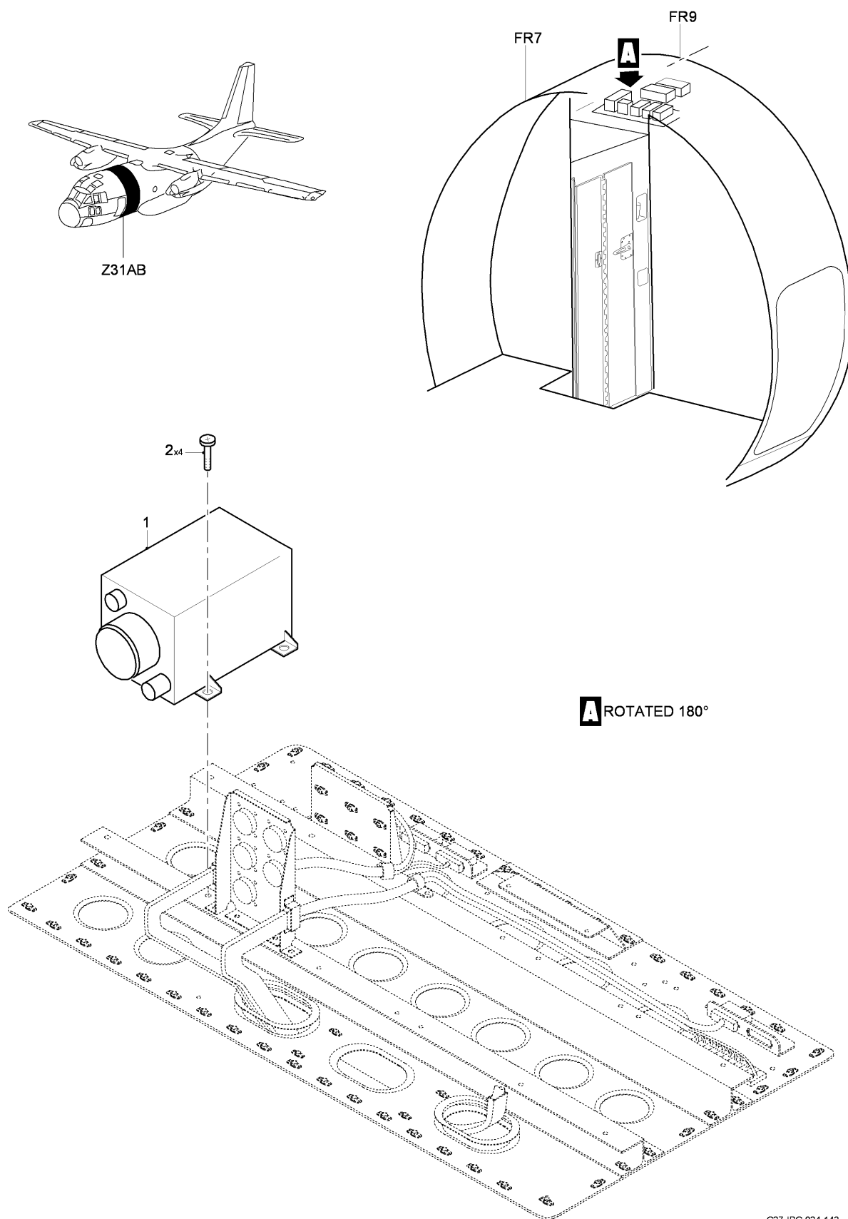
FIG 05 TRU INSTL, Z31AB (SHEET 1 OF 1)
