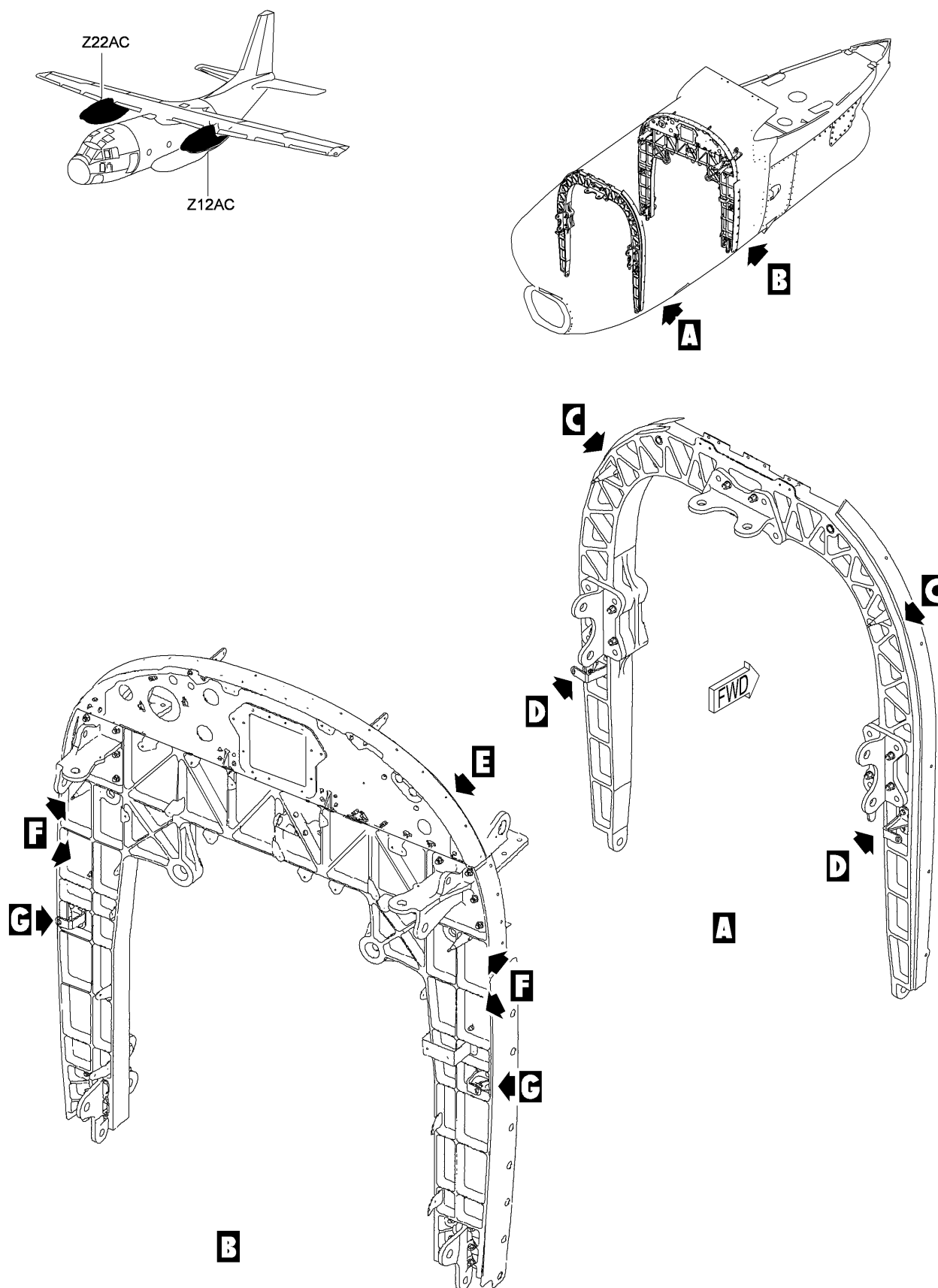
FIG 02 FITTING INSTL - NACELLE ENGINE, Z12AC-22AC (SHEET 1 OF 2)
