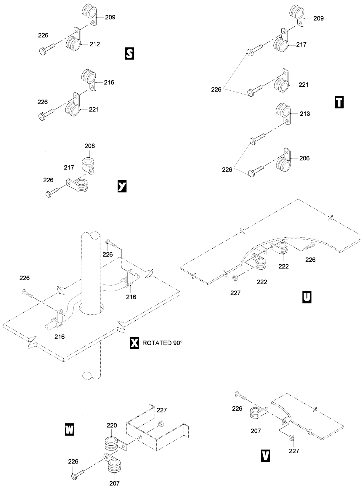
FIG 15 ELECTRICAL AND ELECTRONICS INSTL, Z31AB-32AA-32AB-32AC, LH (SHEET 8 OF 9)
