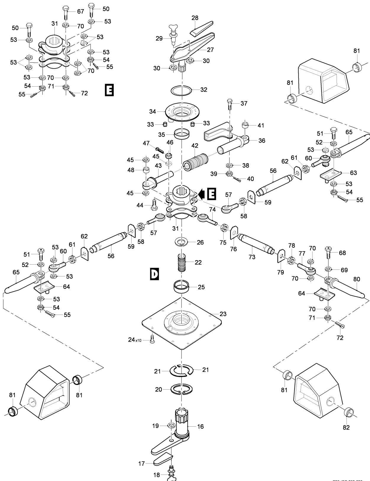
FIG 01 EMERGENCY EXIT DOOR INSTL - TOP FWD, Z31AA (SHEET 2 OF 2)
