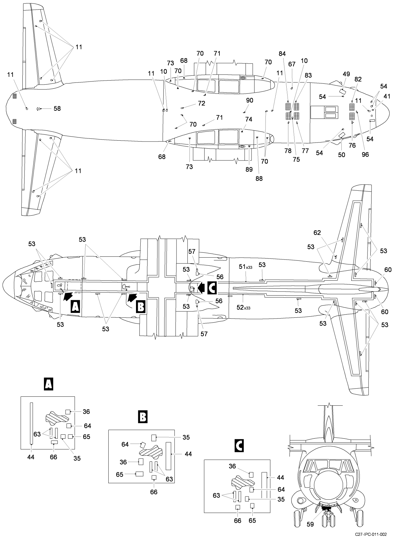
FIG 01 FUSELAGE OUTSIDE MARKING INSTL, Z31-32-33-34-35-14-24 (SHEET 2 OF 2)
