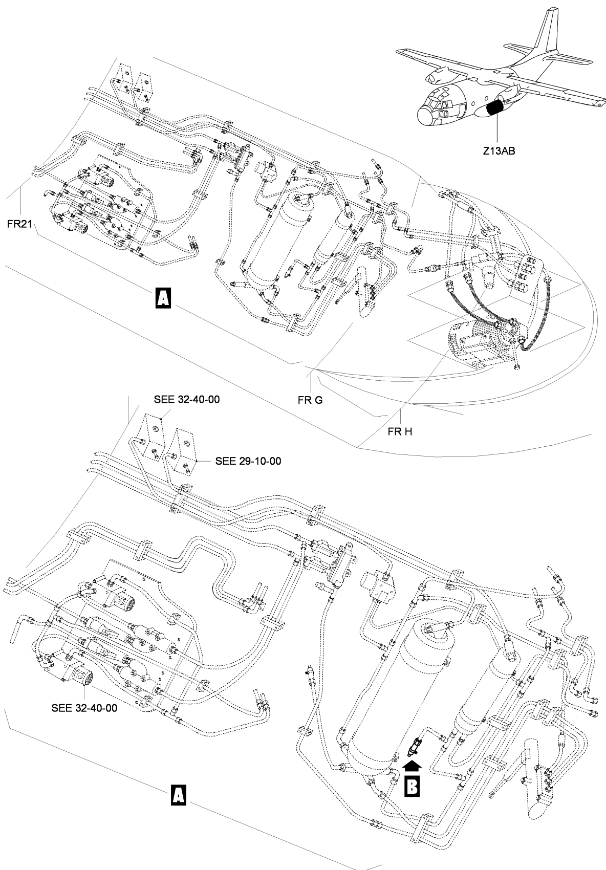
FIG 03 TRANSMITTER PRESSURE INSTL - MLG, Z13AB (SHEET 1 OF 2)
