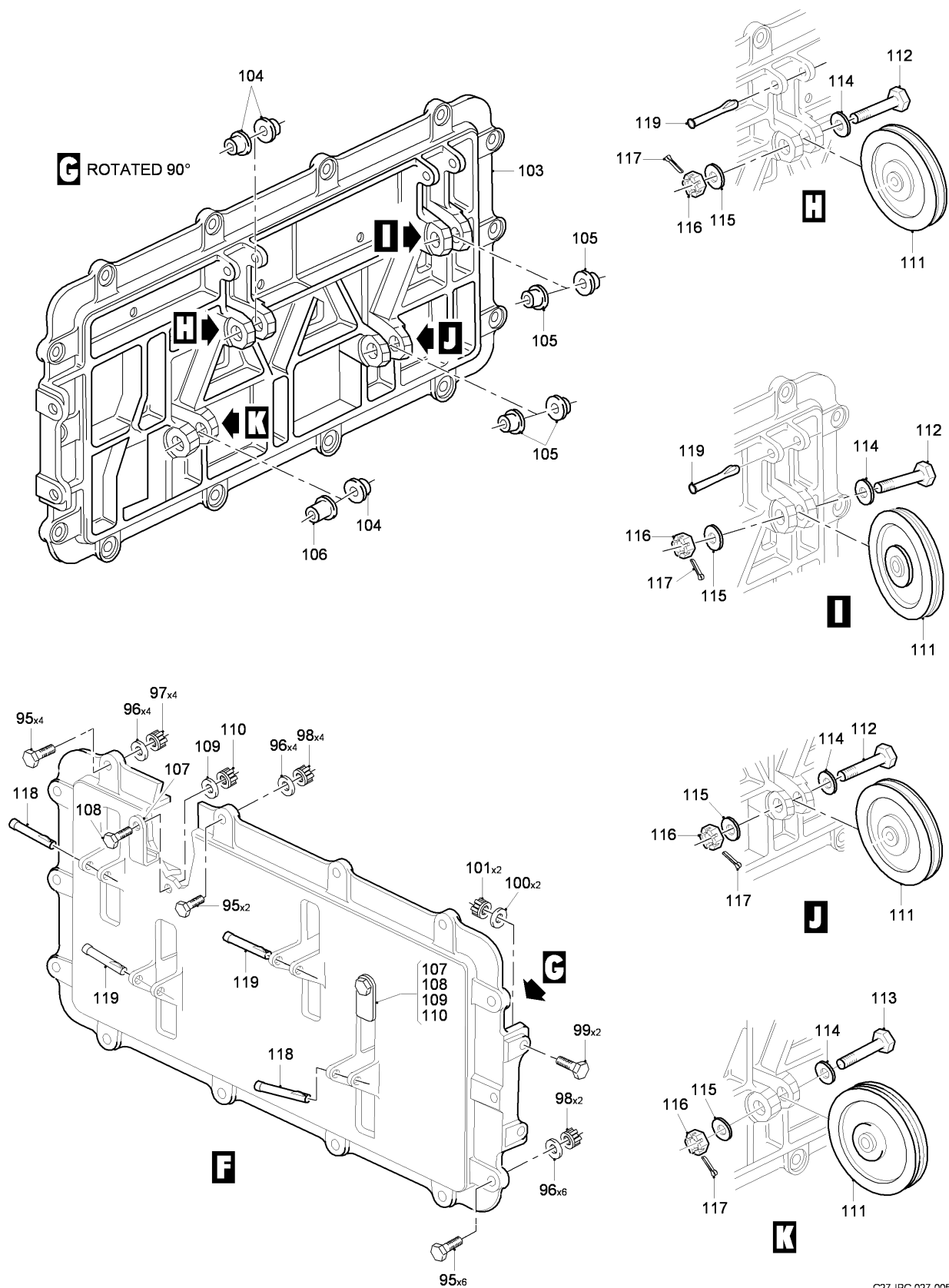
FIG 02 AILERON CONTROLS INSTL, Z31AA-31AB (SHEET 3 OF 5)
