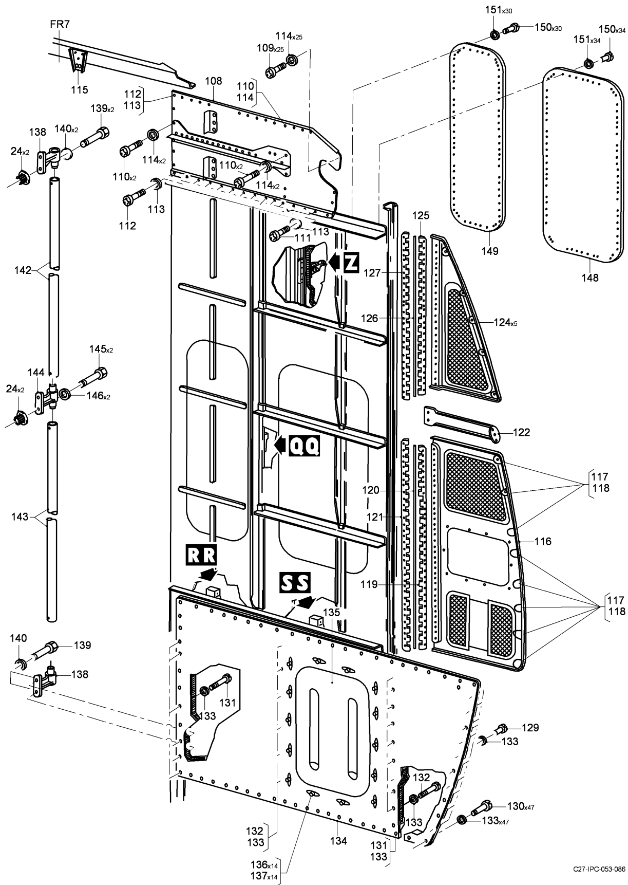
FIG 06 STRUCTURE INSTL, Z31AA (SHEET 6 OF 10)
