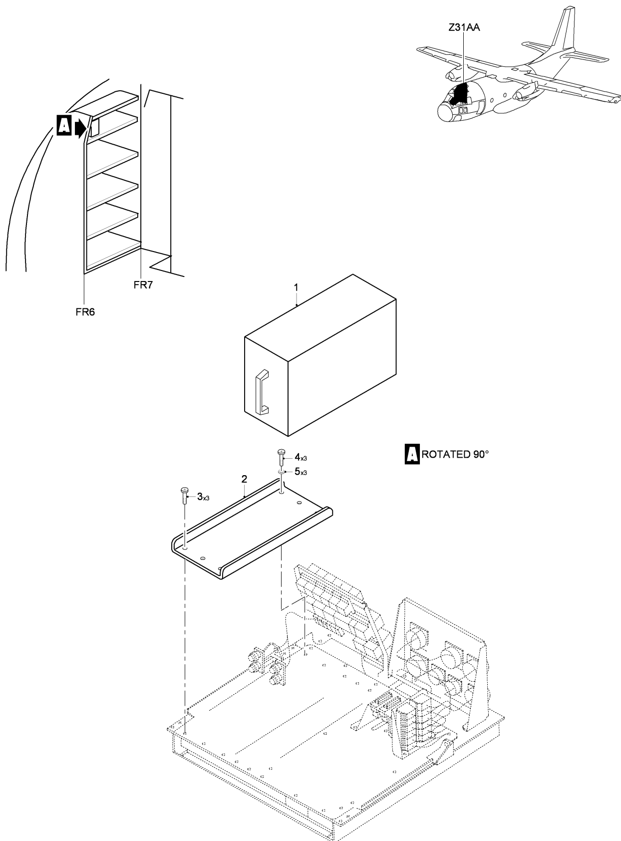
FIG 01 PROXIMITY SWITCHES INSTL - ELECTRONIC PANEL, Z31AA (SHEET 1 OF 1)
