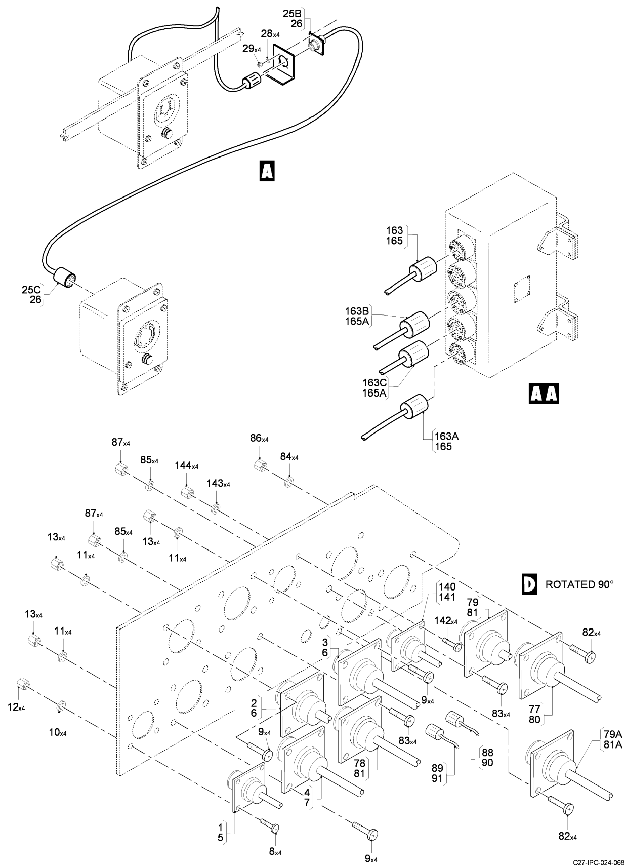
FIG 16 ELECTRICAL AND ELECTRONICS INSTL, Z31AB-32AA-32AB-32AC, RH (SHEET 4 OF 8)
