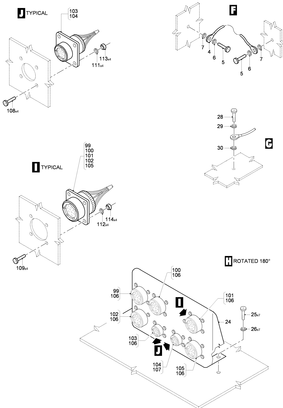
FIG 11 FIFTH AND SIXTH SHELF INSTL - ELECTRICAL COMPARTMENT, Z31AA (SHEET 4 OF 4)
