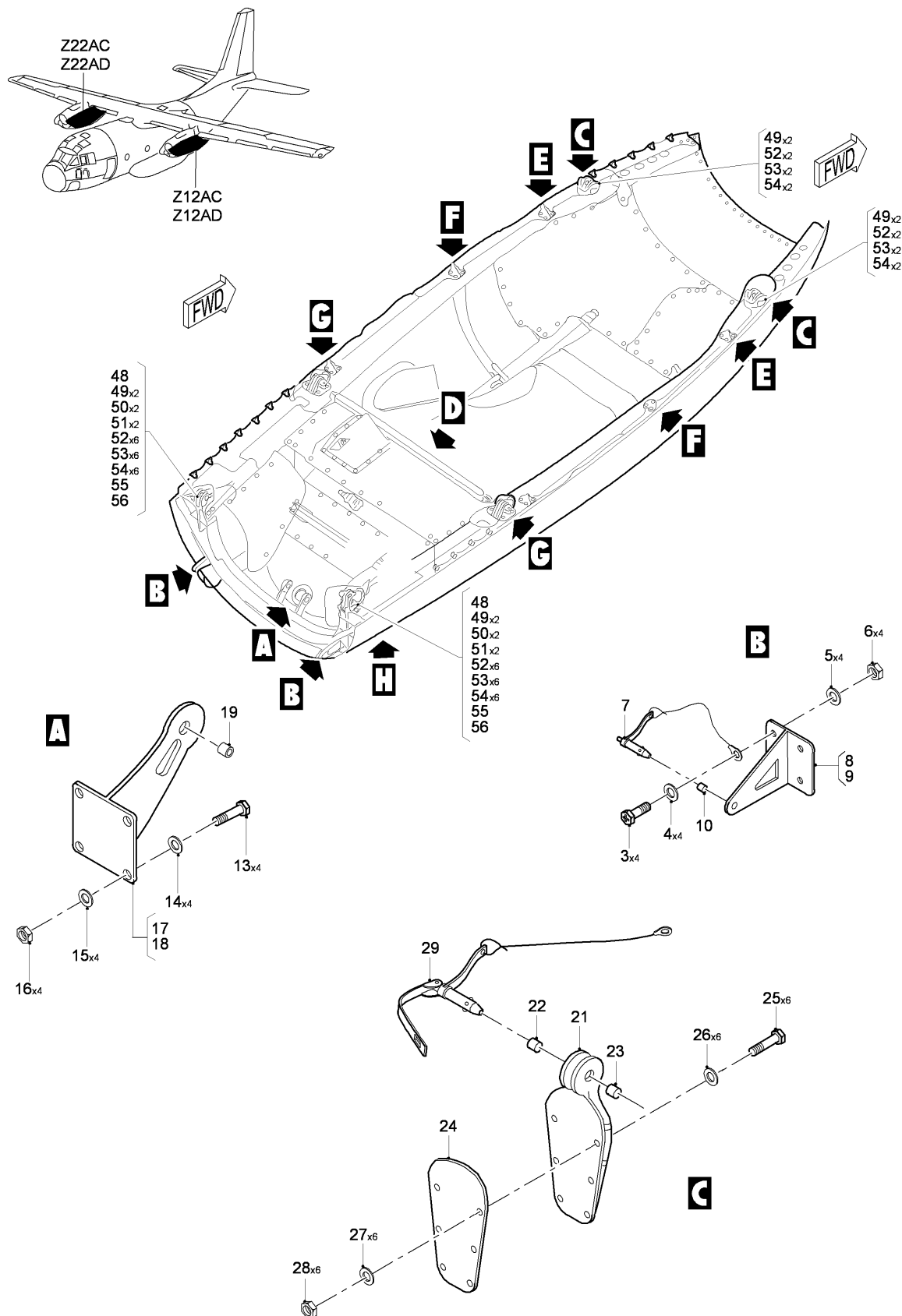
FIG 01 NACELLE ENGINE LWR PANEL INSTL, Z12AC-12AD-22AC-22AD, LH-RH (SHEET 1 OF 3)
