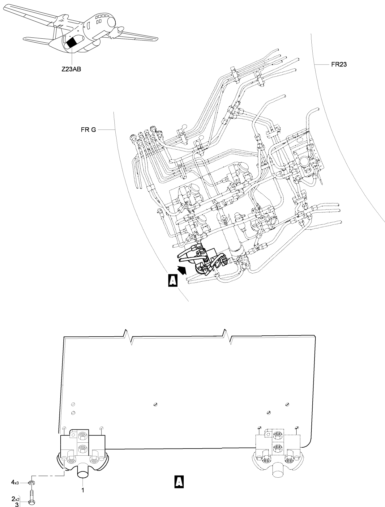
FIG 05 SELECTOR FLOW INSTL - MAIN LANDING GEAR, Z23AB (SHEET 1 OF 1)
