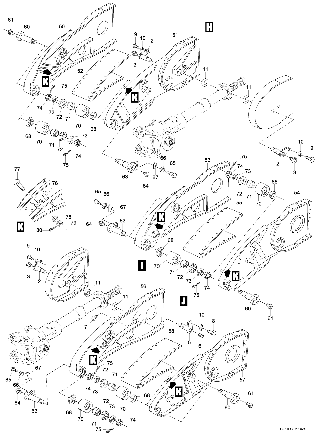
FIG 02 FLAP INSTL - OUTER WING, Z11AD-21AD, LH-RH (SHEET 2 OF 2)
