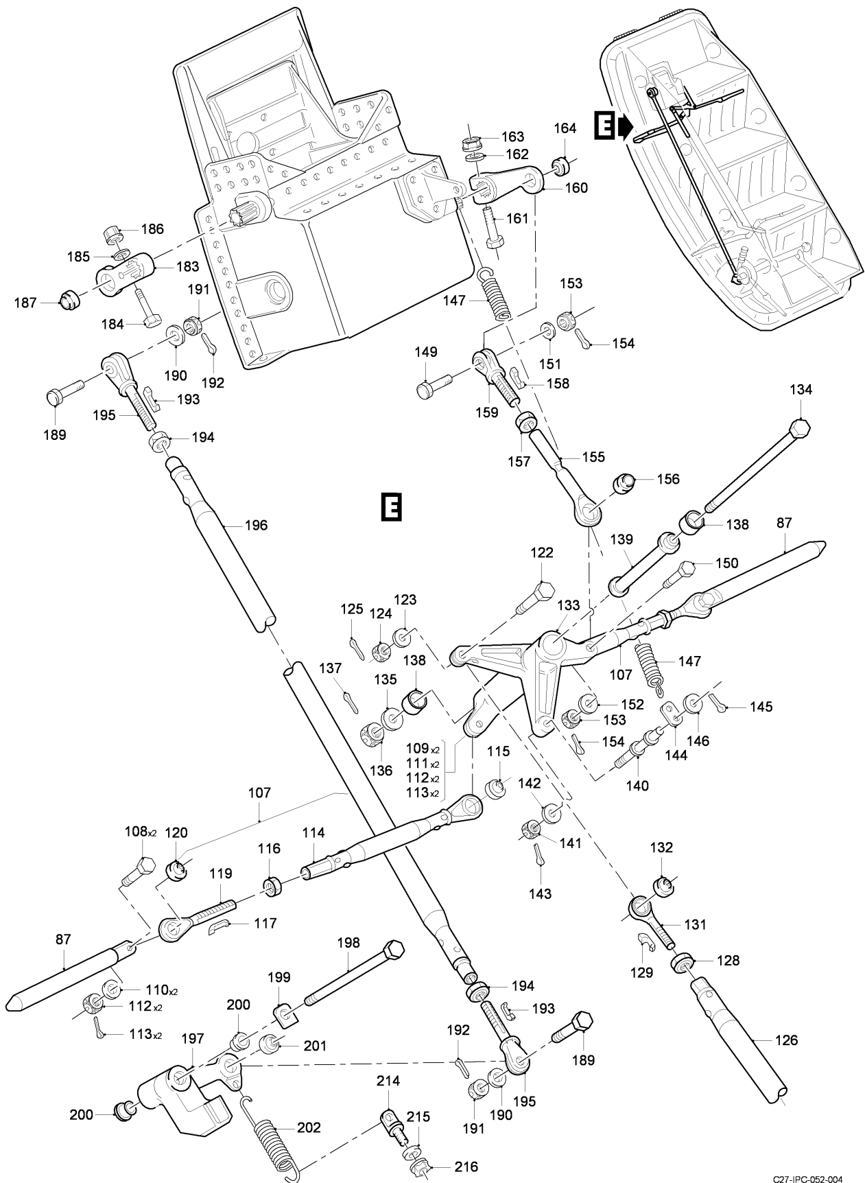
FIG 01 CREW DOOR INSTL, Z31AB (SHEET 4 OF 7)
