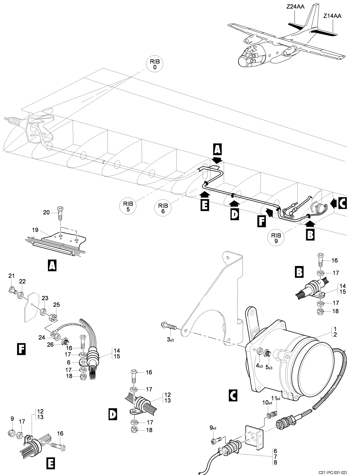
FIG 09 ELEVATOR TRANSMITTER INSTL - TRIM POSITION, Z14AA-24AA,LH-RH (SHEET 1 OF 1)
