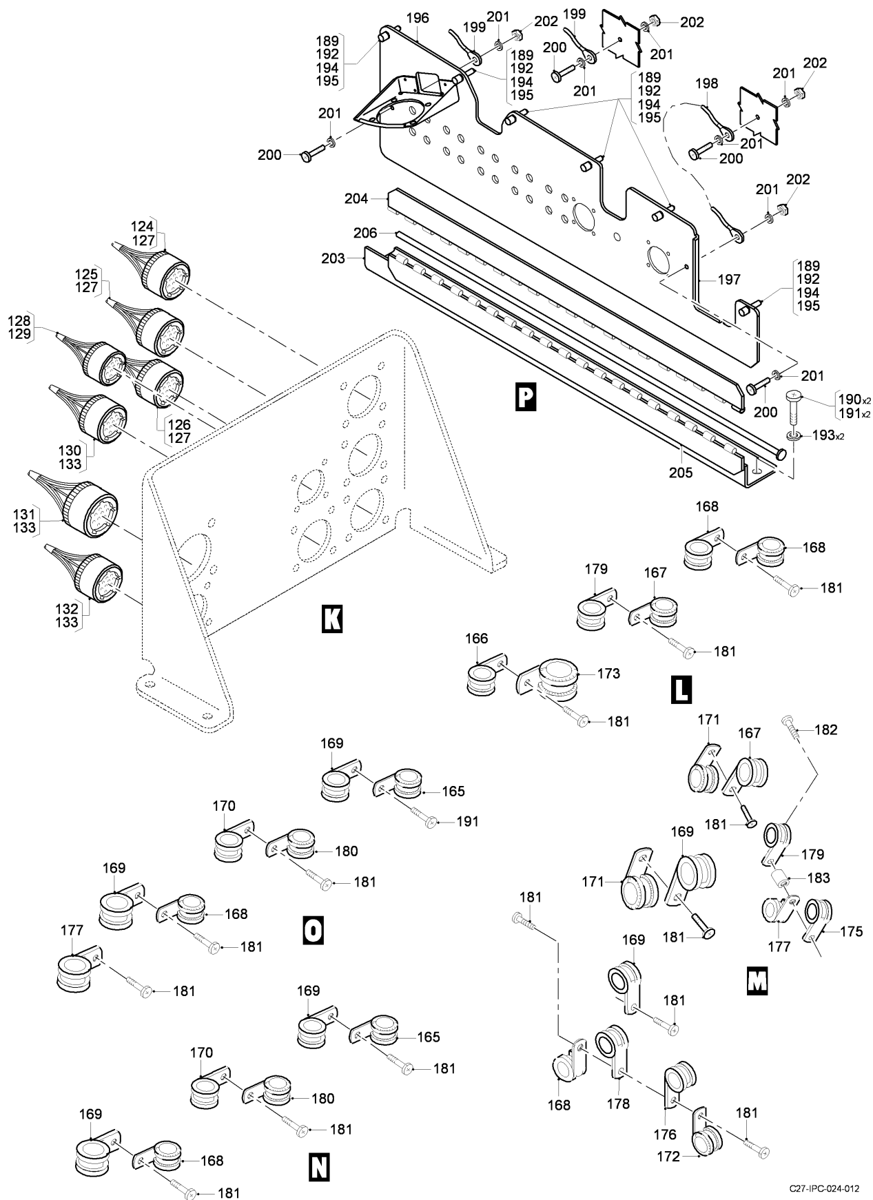
FIG 04 ELECTRICAL AND ELECTRONICS INSTL - CABIN, Z31AA, LH (SHEET 5 OF 5)
