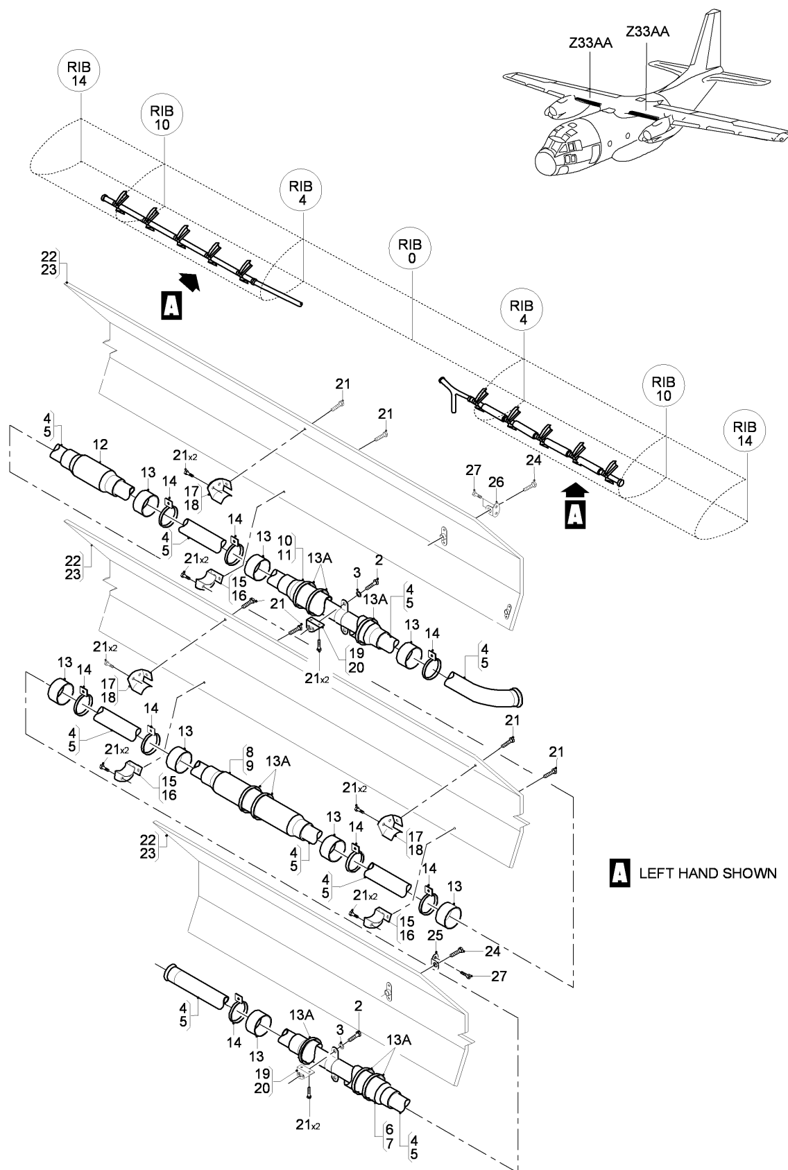
FIG 06 AIR CONDITIONING INSTL - CENTER WING, Z33AA, LH-RH (SHEET 1 OF 1)
