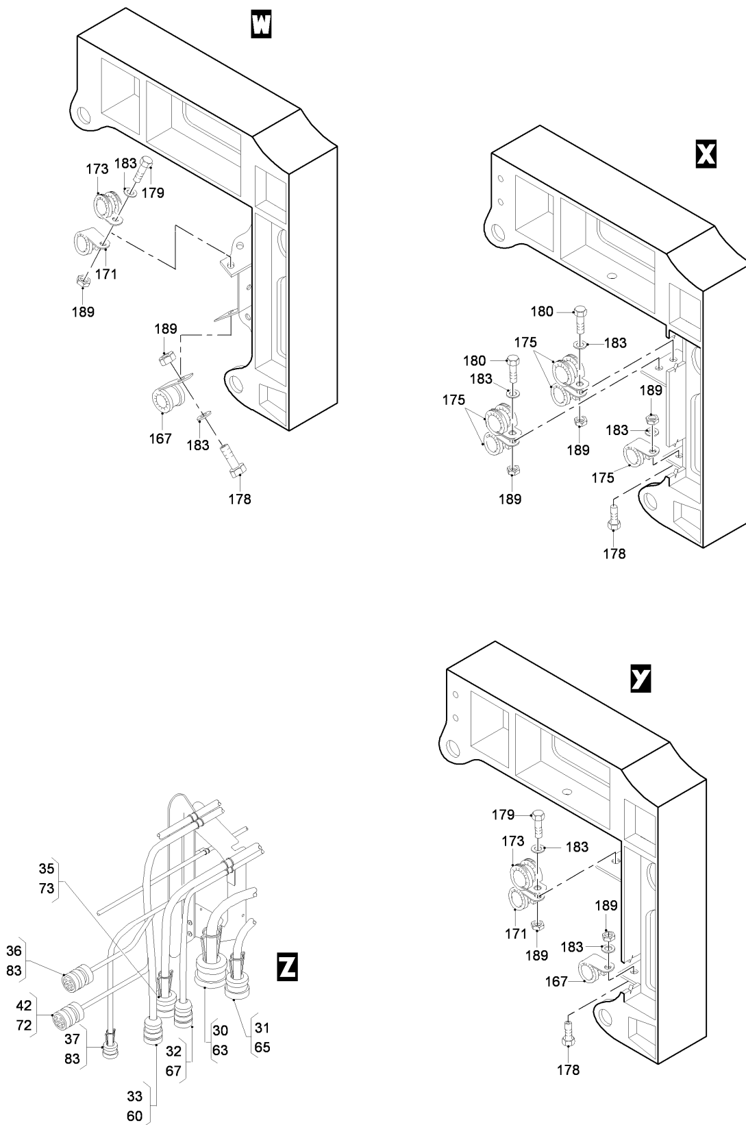
FIG 22 ELECTRICAL AND ELECTRONICS INSTL - CENTER WING, Z33AB, LH (SHEET 6 OF 7)
