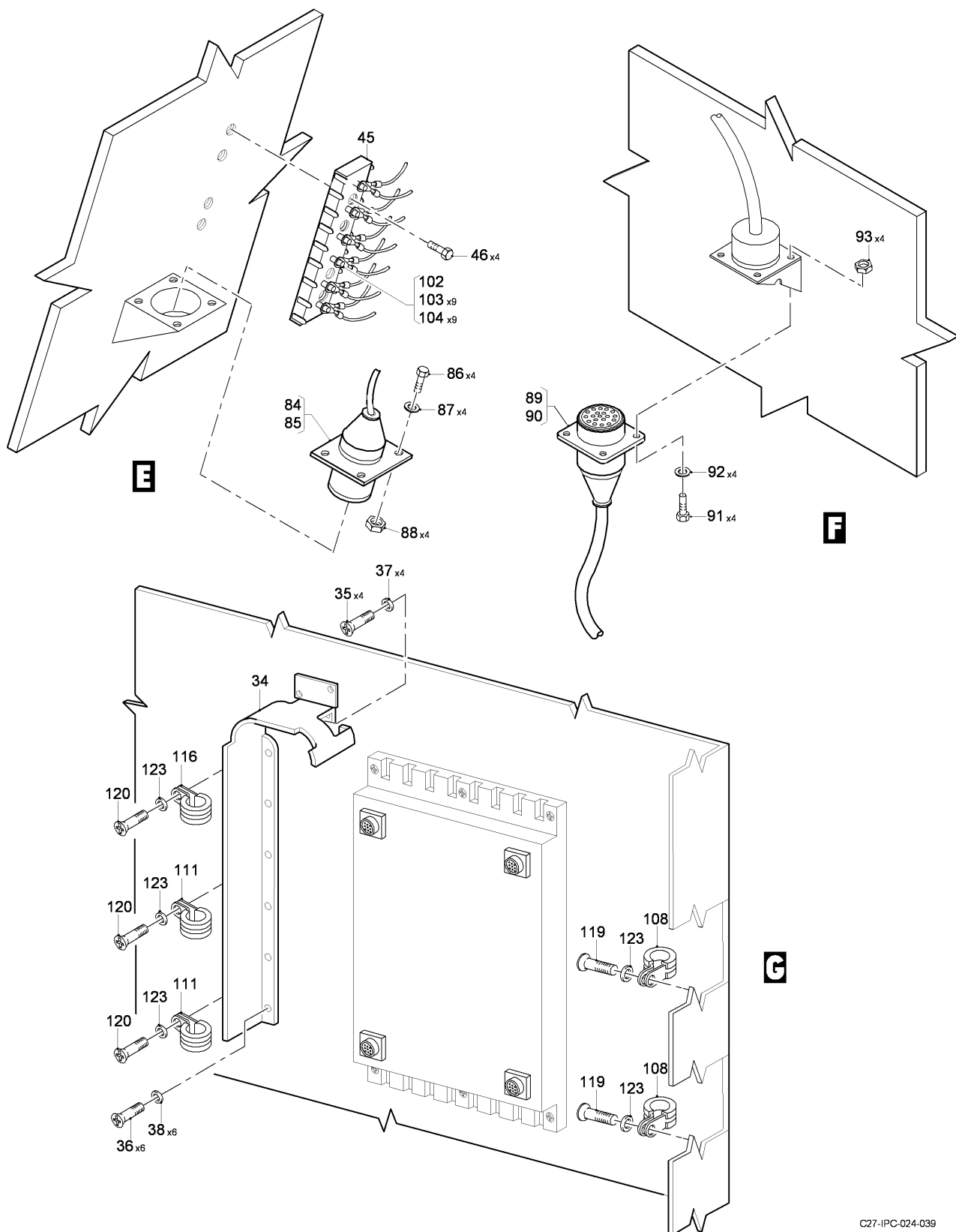
FIG 11 ELECTRICAL AND ELECTRONICS INSTL, Z31AA (SHEET 3 OF 6)
