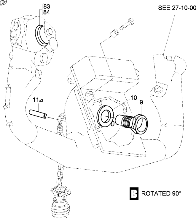
FIG 01 CONTROL COLUMN INSTL, Z31AA, LH-RH (SHEET 1 OF 3)
