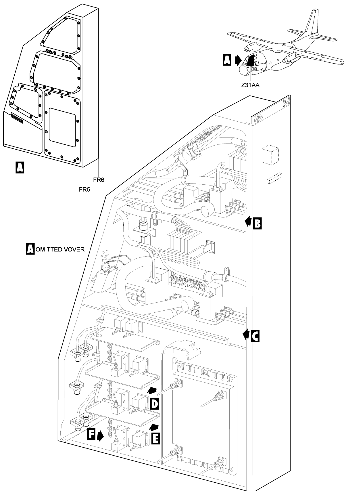
FIG 01 POWER DISTRUBTION UNIT INSTL, Z31AA (SHEET 1 OF 3)
