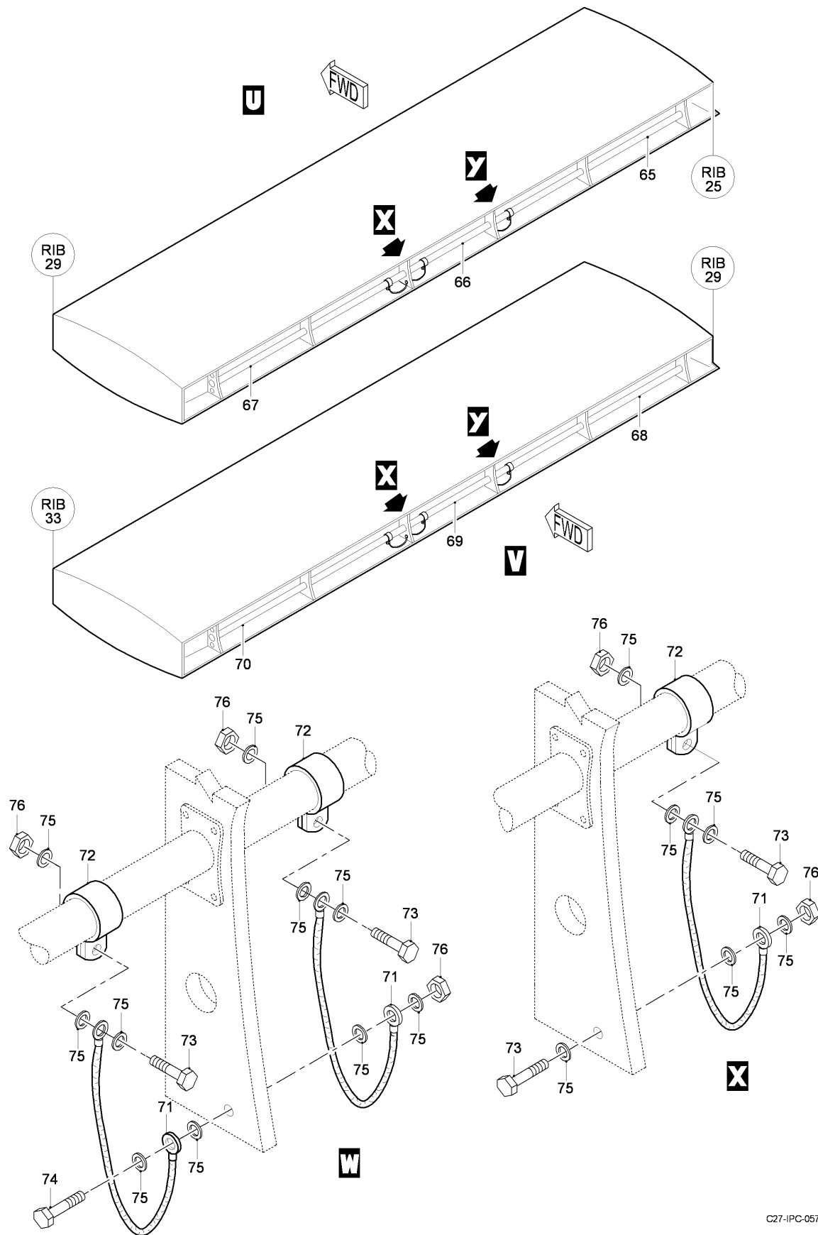
FIG 04 TRAILING EDGE INSTL, Z11AC-11AD-21AC-21AD, LH-RH (SHEET 5 OF 5)
