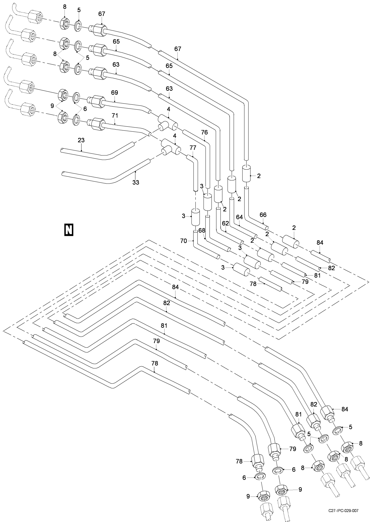
FIG 02 HYDRAULIC INSTL - CENTER FUSELAGE, LOWER, Z32BA (SHEET 5 OF 8)
