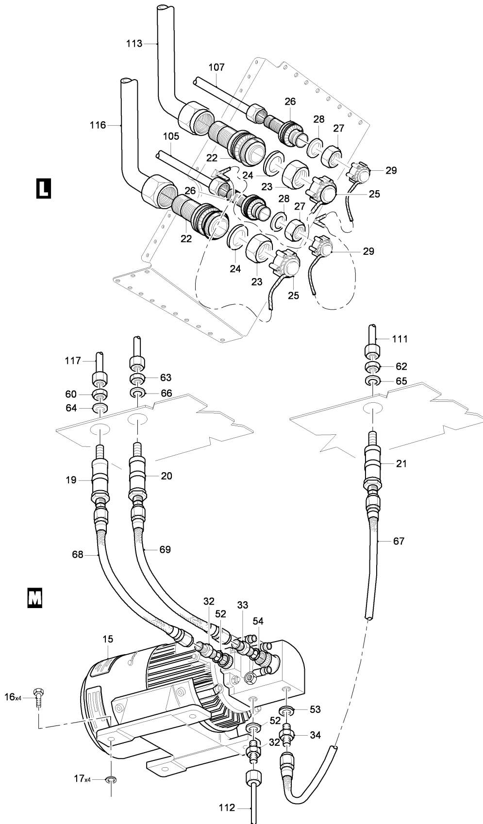
FIG 07 HYDRAULIC INSTL - MLG, Z13AB, LH (SHEET 6 OF 8)
