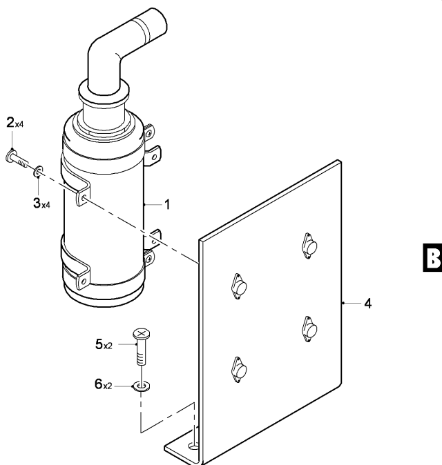
FIG 04 IFF DATA CONVERSION UNIT INSTL, Z31AA (SHEET 1 OF 1)
