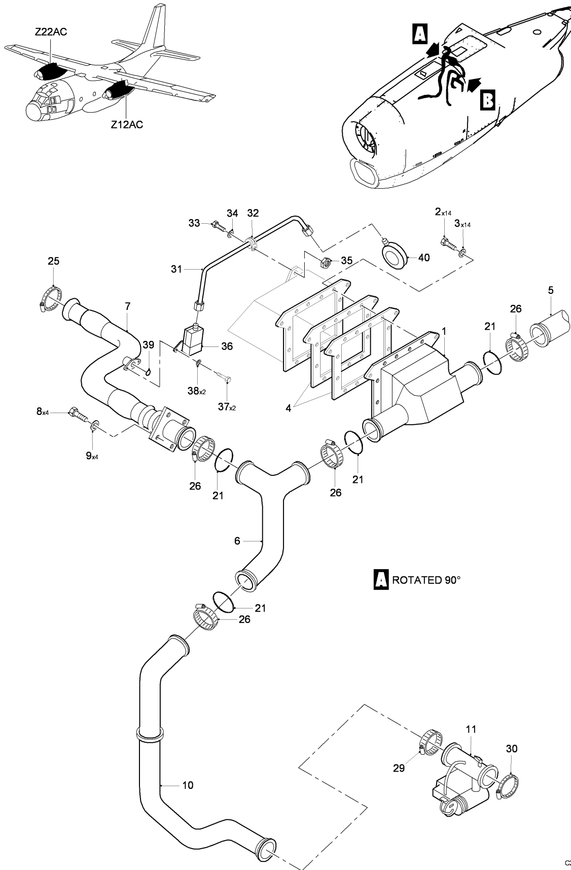
FIG 02 PNEUMATIC SYSTEM INSTL - ENGINE, Z12AC-22AC (SHEET 1 OF 2)
