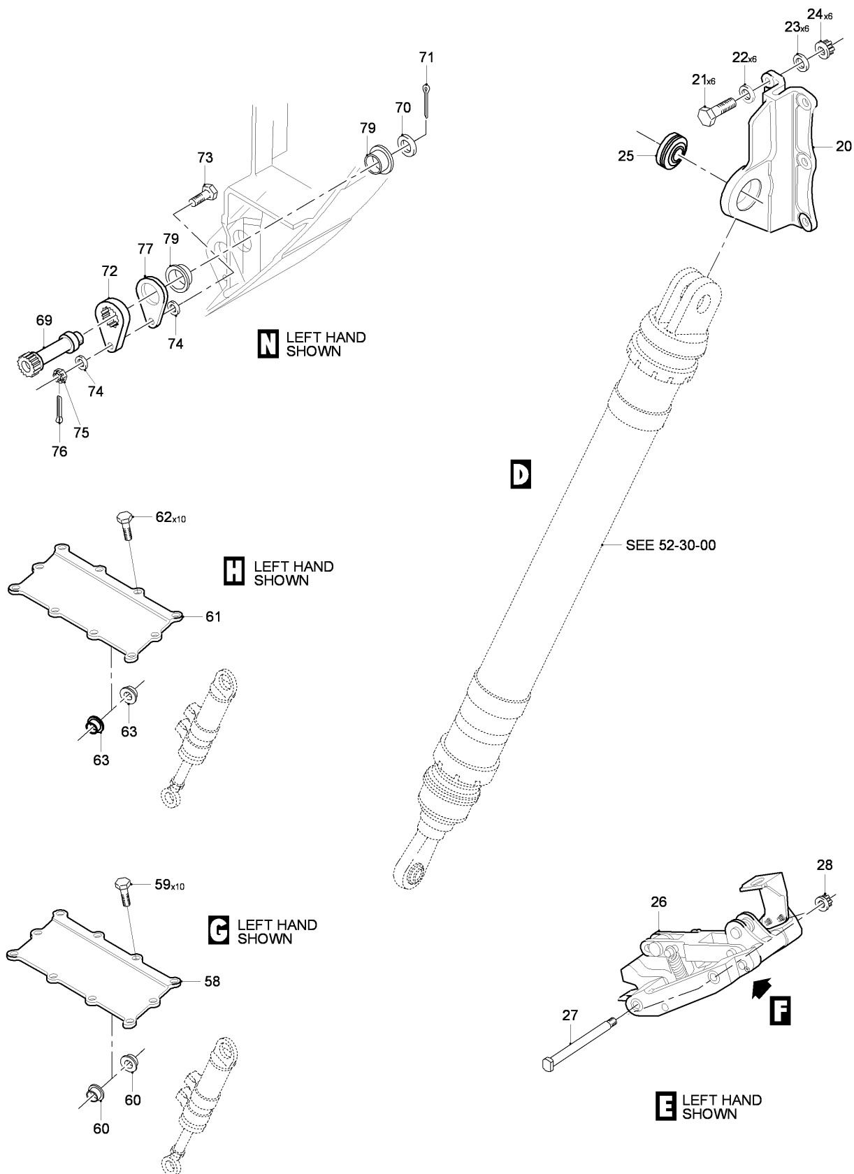
FIG 11 CARGO DOOR INSTL, Z34AA-34BB (SHEET 2 OF 3)
