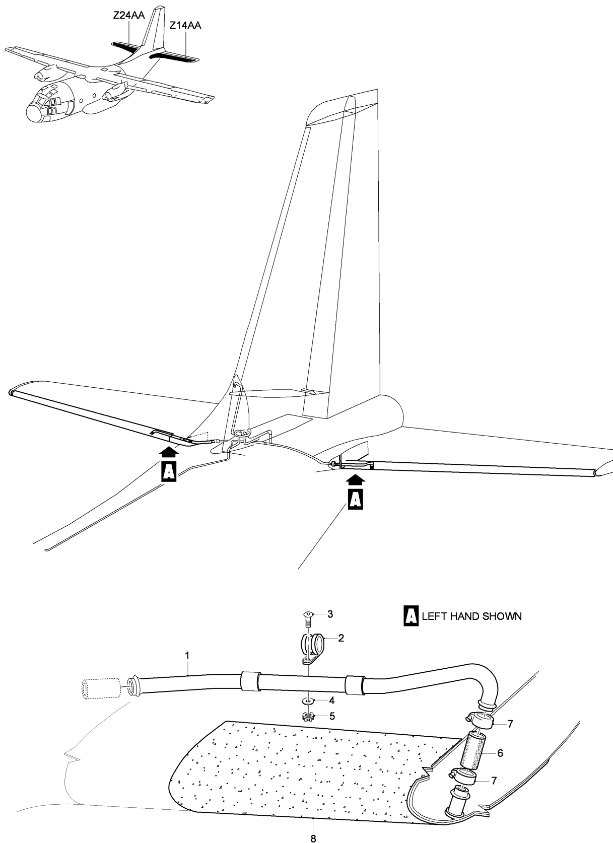
FIG 05 ANTI-ICING INSTL - HORIZONTAL STABILIZER, Z14AA-24AA, LH-RH (SHEET 1 OF 1)
