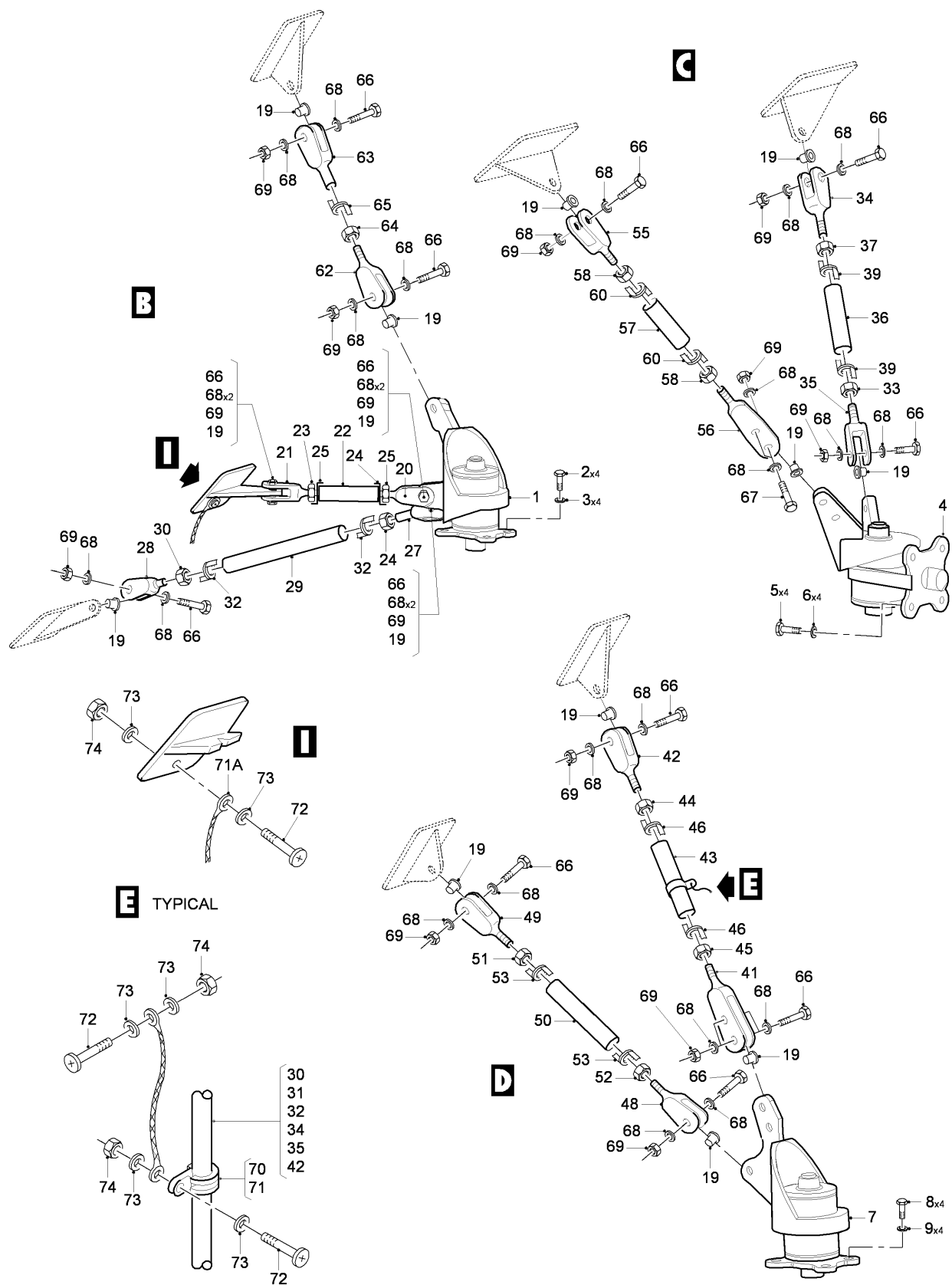
FIG 01 APU INSTL, Z13AA (SHEET 2 OF 3)
