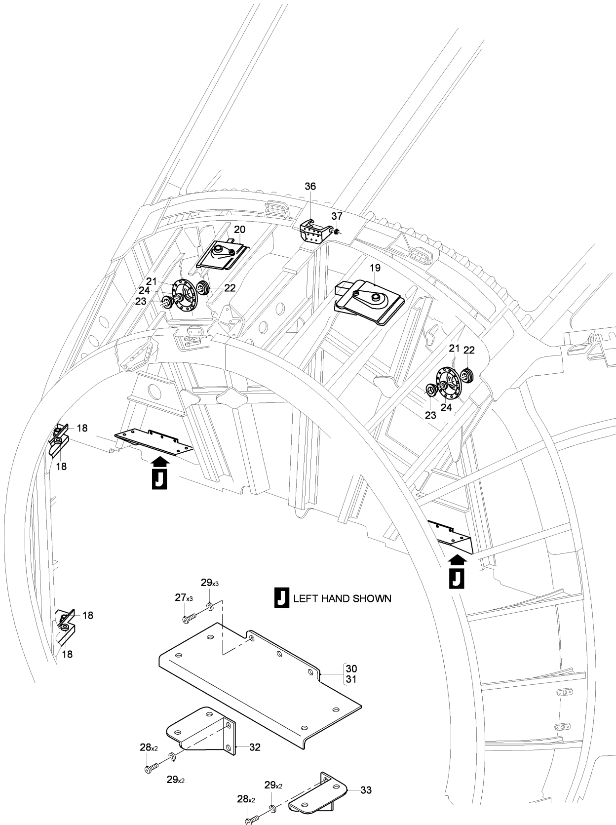
FIG 06 STRUCTURE INSTL, Z31AA (SHEET 2 OF 10)
