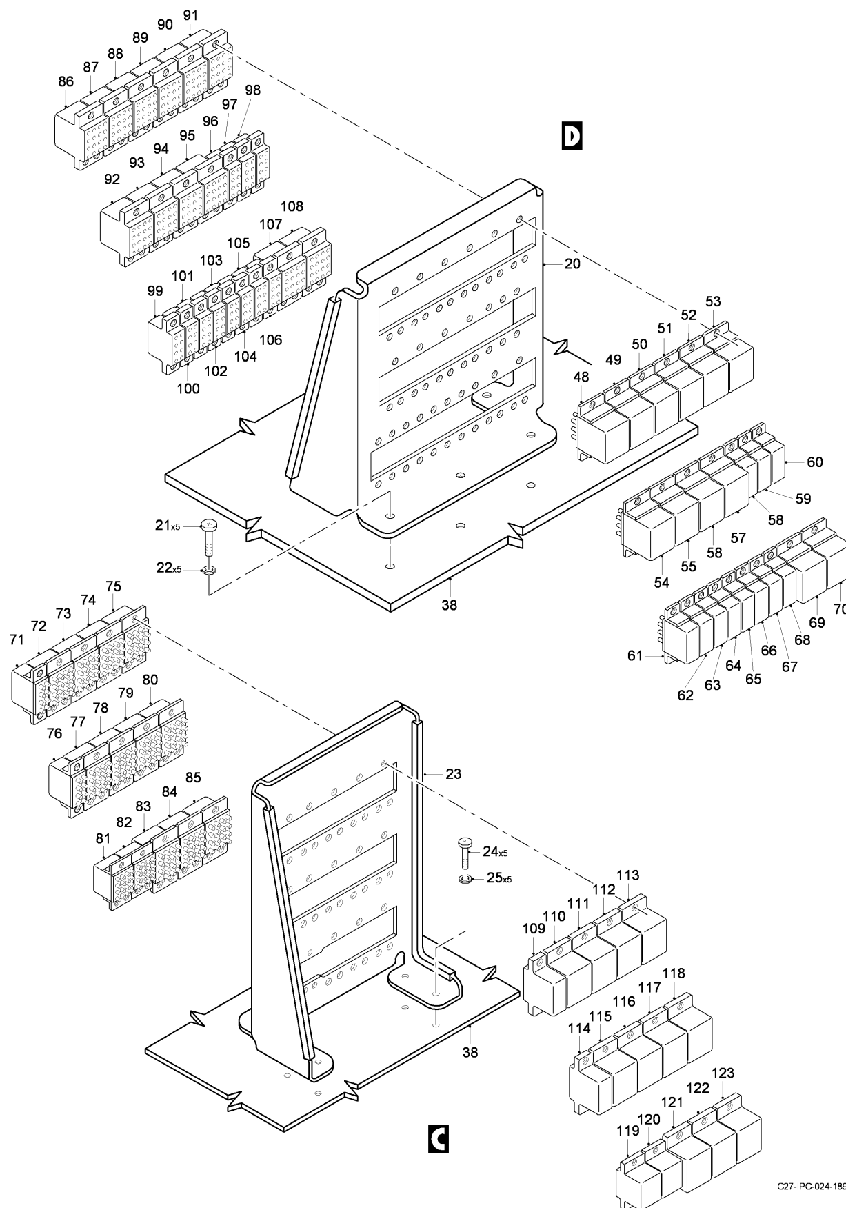
FIG 09 THIRD SHELF INSTL - ELECTRICAL COMPARTMENT, Z31AA (SHEET 2 OF 4)
