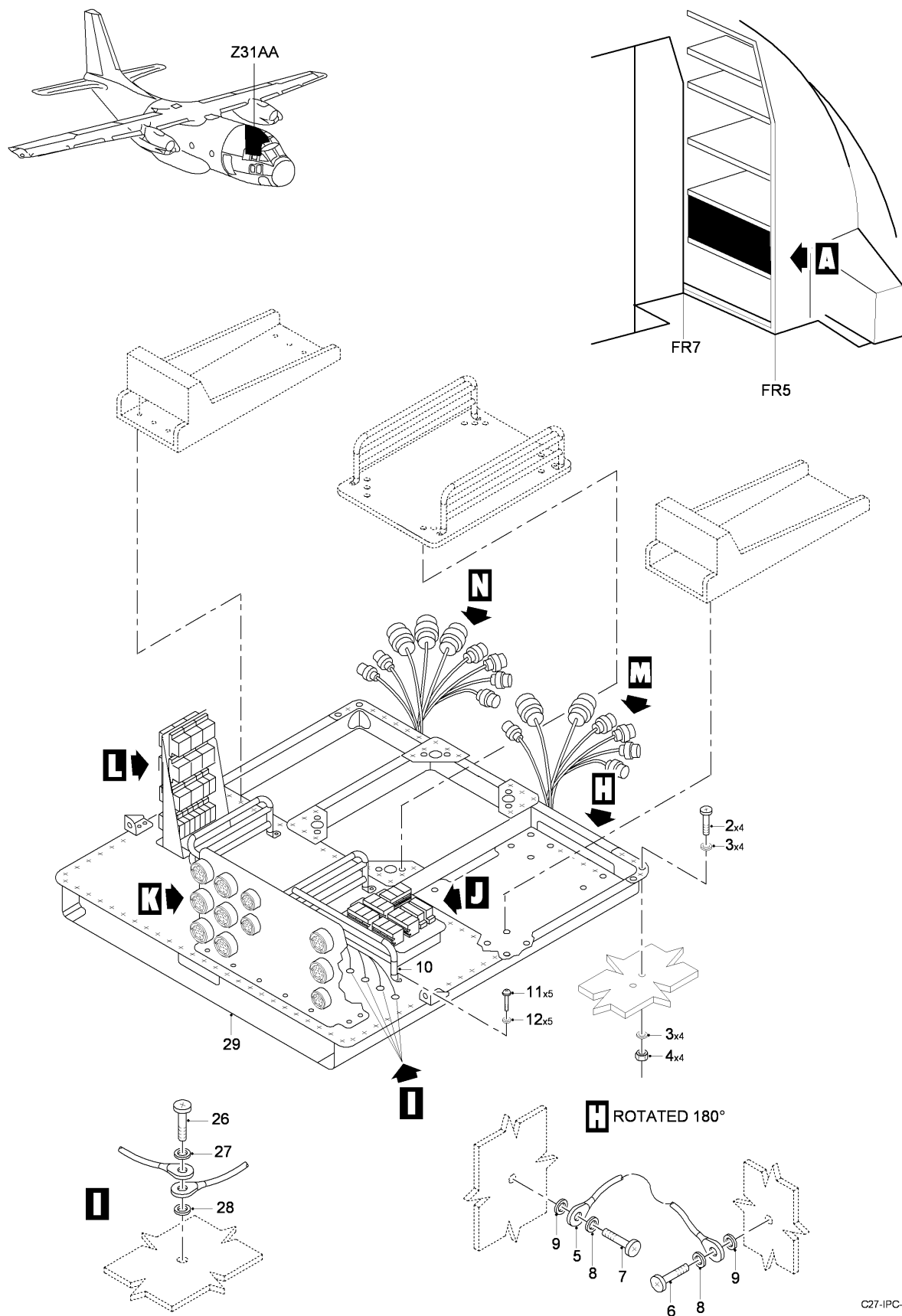
FIG 02 SECOND SHELF INSTL - ELECTRONIC COMPARTMENT, Z31AA (SHEET 1 OF 3)
