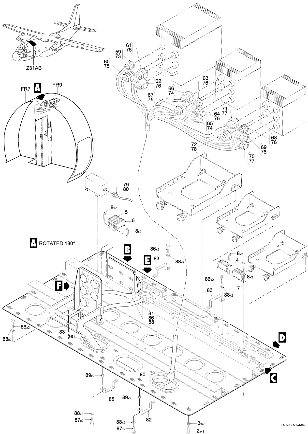
FIG 12 ELECTRONIC INSTL - SHELF FRAME 7 TO 8, Z31AB (SHEET 1 OF 2)
