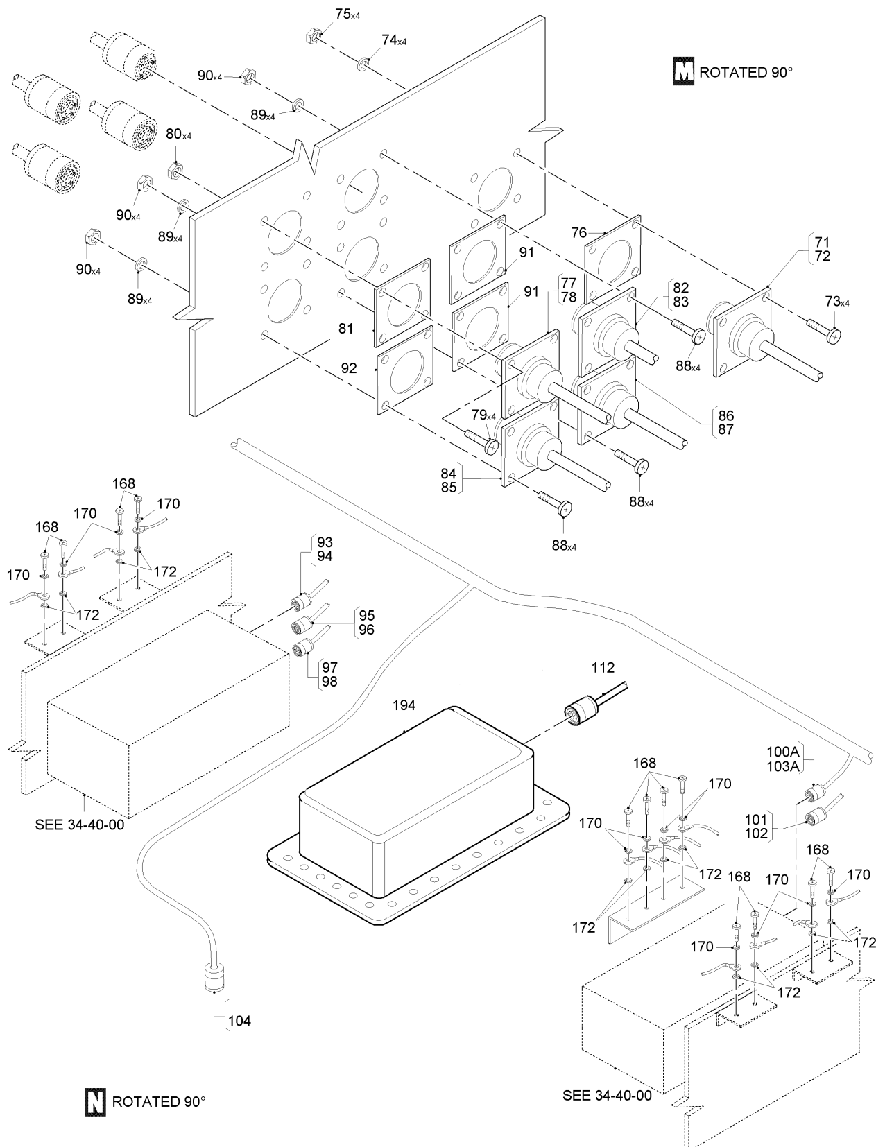
FIG 14 ELECTRICAL AND ELECTRONICS INSTL, Z31BC-31BD-32BA (SHEET 6 OF 11)
