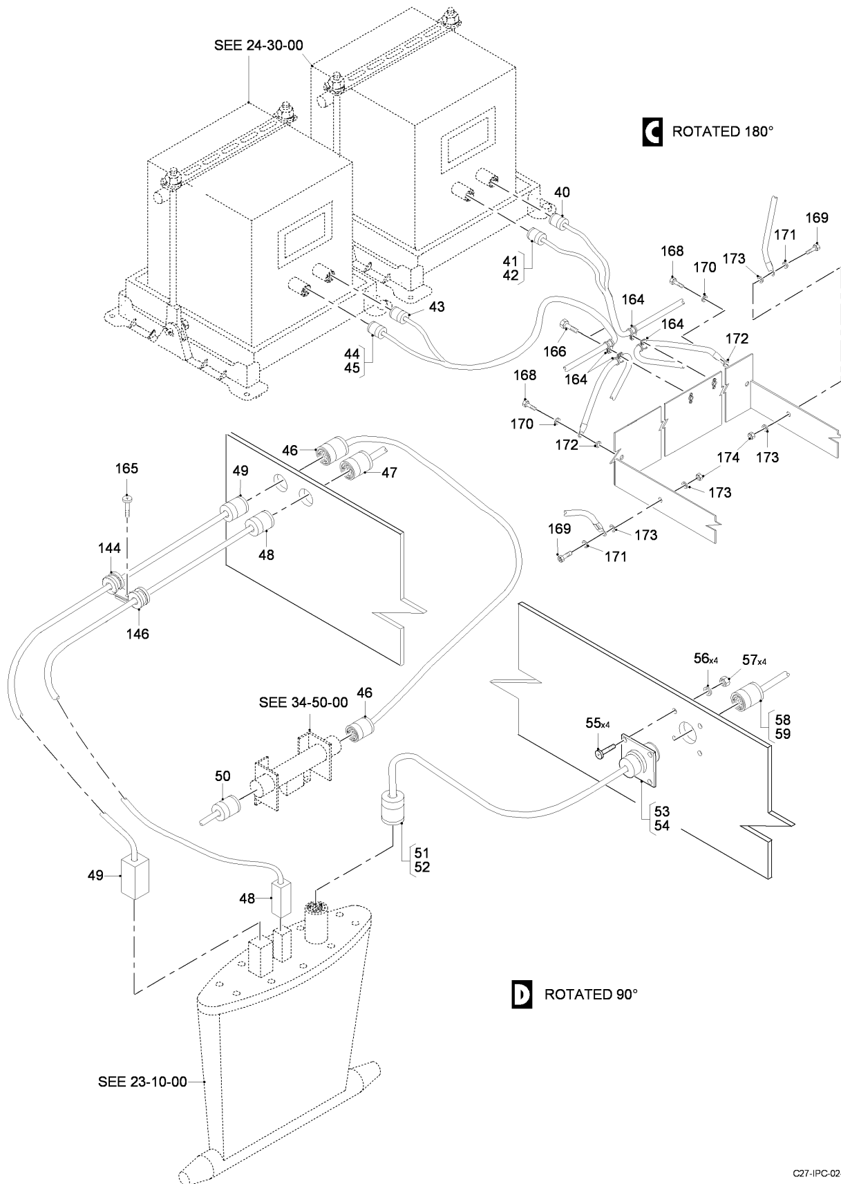
FIG 14 ELECTRICAL AND ELECTRONICS INSTL, Z31BC-31BD-32BA (SHEET 4 OF 11)
