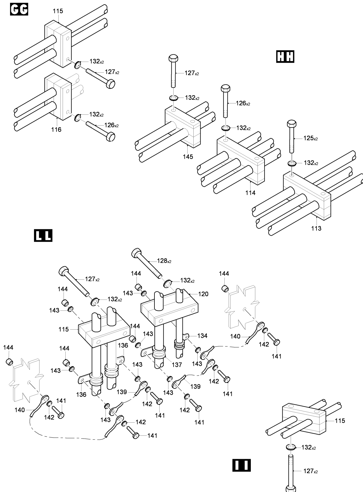
FIG 04 HYDRAULIC INSTL - CENTER FUSELAGE, Z32AC-32AD (SHEET 6 OF 6)
