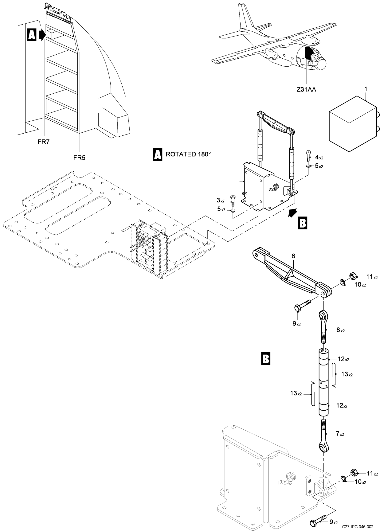
FIG 02 BUS ADAPTER UNIT TYPE I INSTL, Z31AA (SHEET 1 OF 1)
