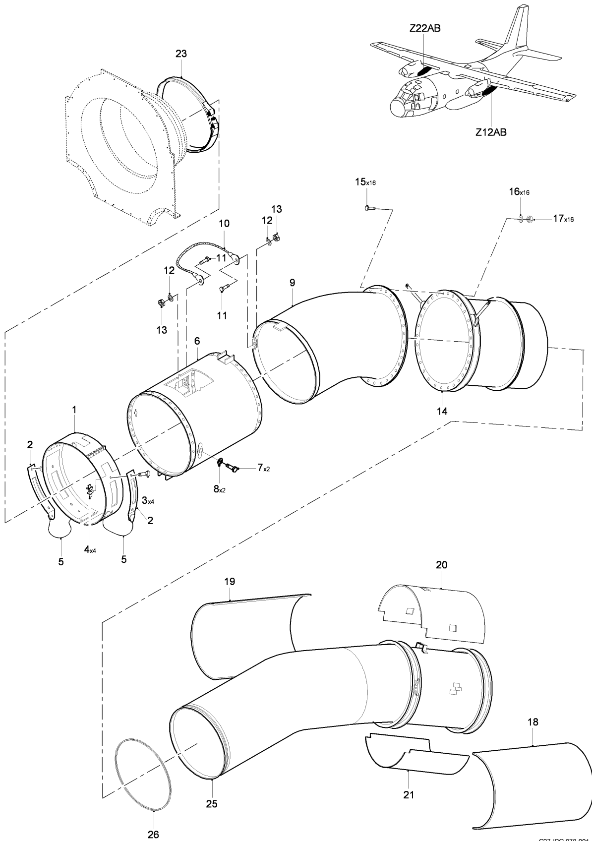
FIG 01 EXHAUST DUCT INSTL - ENGINE, Z12AB-22AB (SHEET 1 OF 1)
