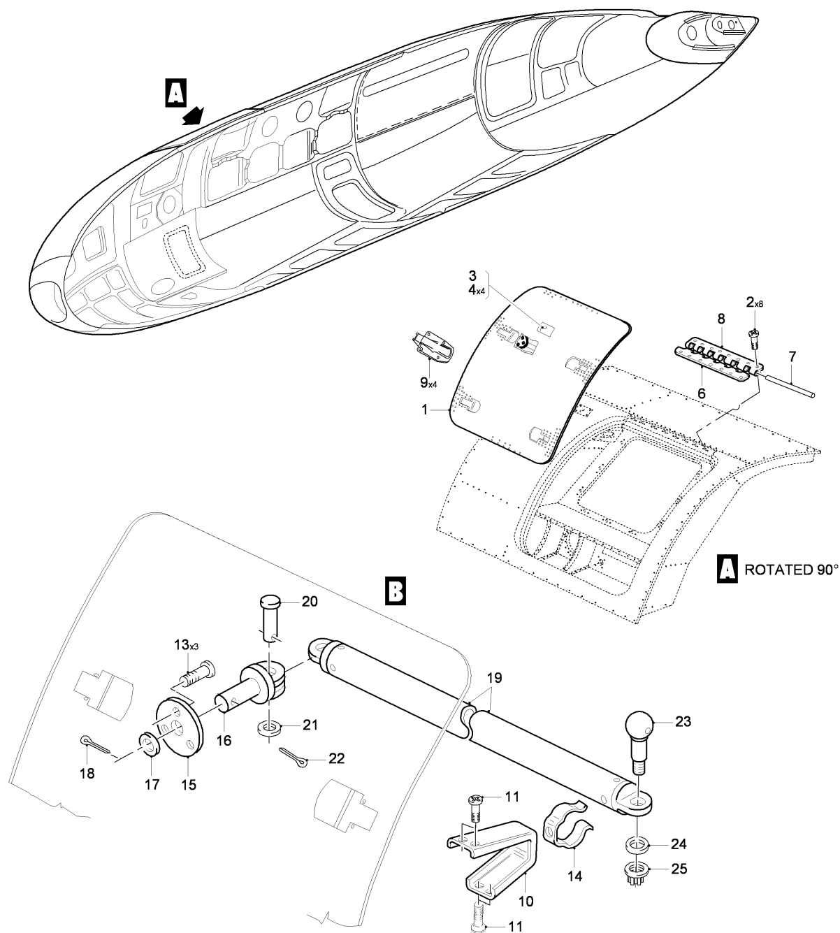
FIG 05 DOOR INSTL - REFUELLING ACCESS, Z23AA, RH (SHEET 1 OF 1)
