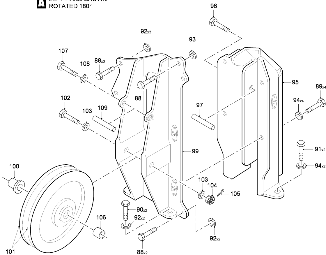
FIG 03 ELEVATOR CONTROLS PULLEYS INSTL, Z31AA-31BB-31AB (SHEET 1 OF 4)
