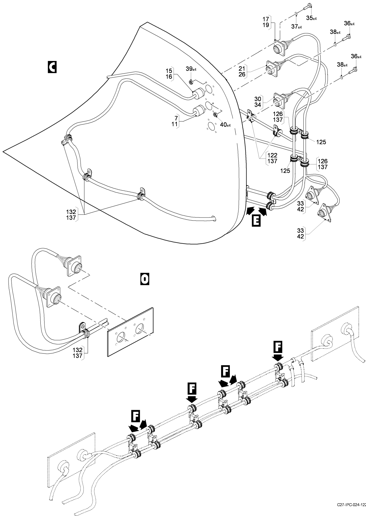
FIG 26 ELECTRICAL AND ELECTRONICS INSTL - MLG, Z13AA-13AB-13AC, LH (SHEET 2 OF 5)
