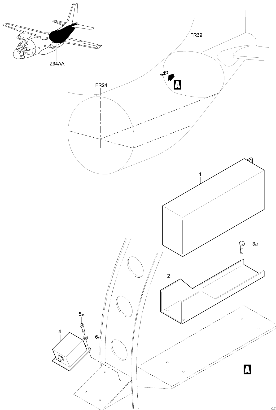
FIG 04 FLIGHT DATA RECORDER INSTL, Z34AA (SHEET 1 OF 1)
