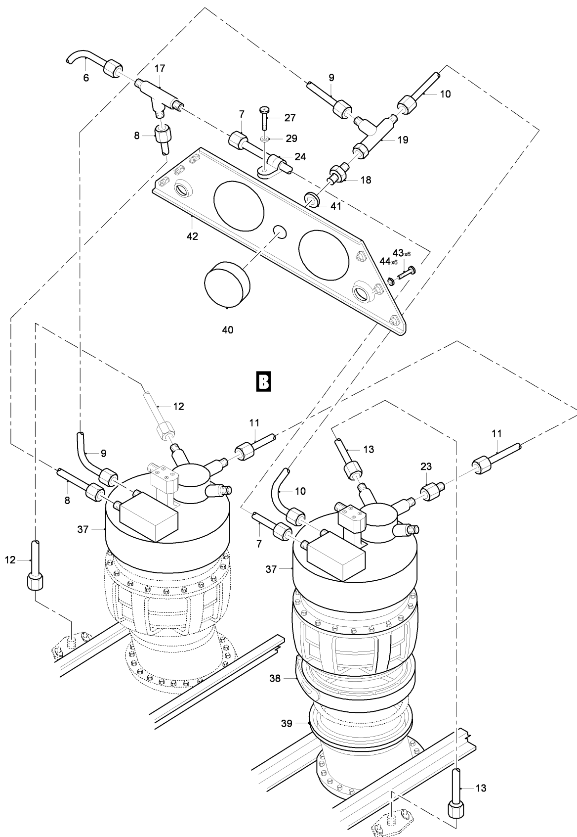
FIG 03 PRESSURIZATION INSTL - FWD FUSELAGE, Z32AB-32AC (SHEET 2 OF 3)
