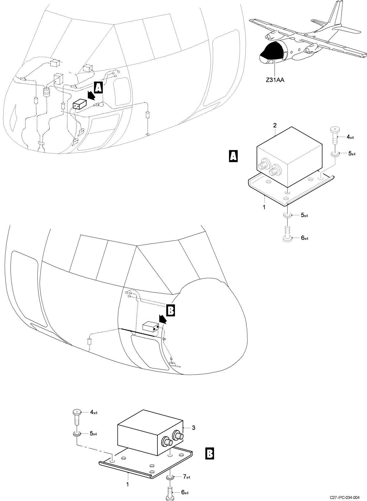
FIG 04 COMPUTER AID DATA 1 AND 2 INSTL, Z31AA (SHEET 1 OF 1)
