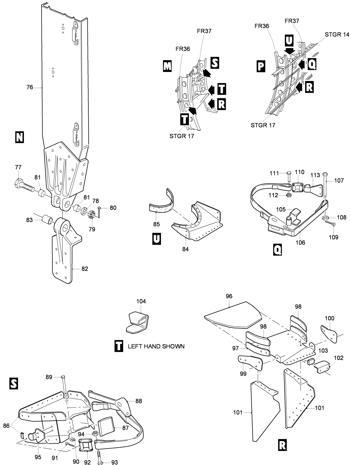
FIG 02 STRUCTURE INSTL, Z34AA (SHEET 3 OF 4)
