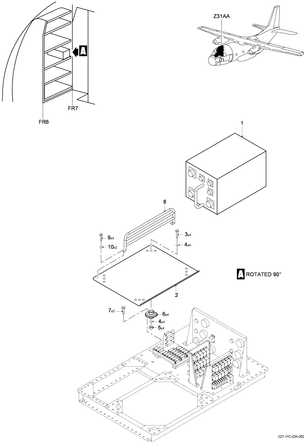
FIG 03 CNI SIGNAL PROCESSOR NO. 2 INSTL, Z31AA (SHEET 1 OF 1)
