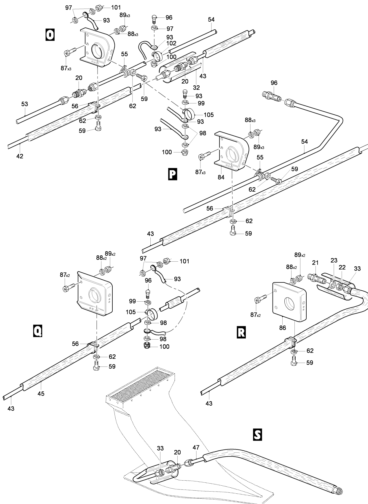
FIG 08 SINGLE POINT REFUEL AND FUEL SUPPLY INSTL, Z11AA-21AA, LH-RH (SHEET 5 OF 6)
