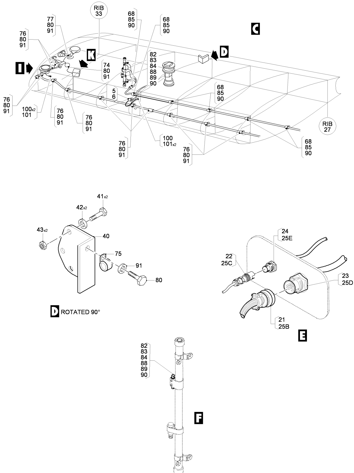
FIG 25 ELECTRICAL AND ELECTRONICS INSTL, Z21AA-21AB, RH (SHEET 2 OF 3)
