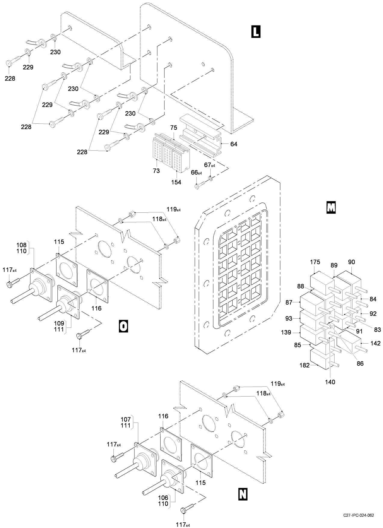
FIG 15 ELECTRICAL AND ELECTRONICS INSTL, Z31AB-32AA-32AB-32AC, LH (SHEET 6 OF 9)
