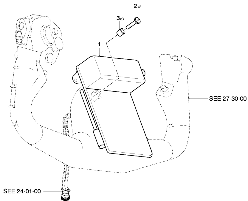
FIG 04 CHART HOLDER INSTL, Z31AA, LH-RH (SHEET 1 OF 1)
