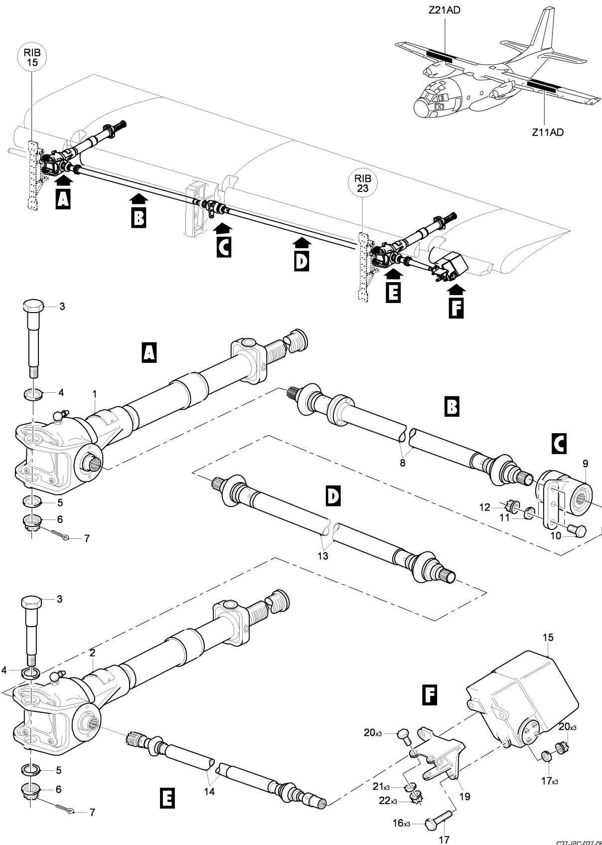
FIG 07 FLAP CONTROLS INSTL, Z11AD-21AD, LH-RH (SHEET 1 OF 1)
