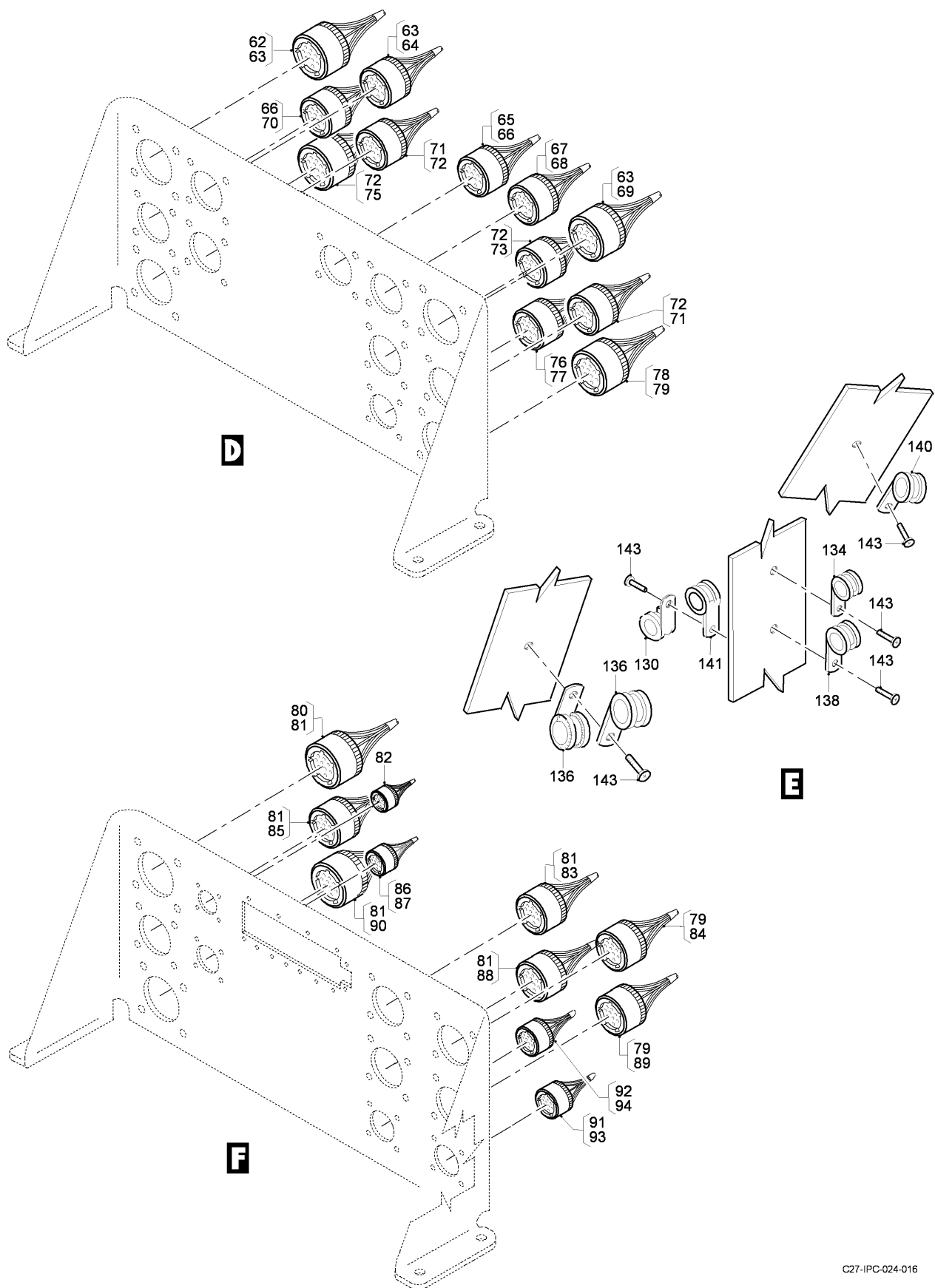
FIG 05 ELECTRICAL AND ELECTRONICS INSTL - CABIN, Z31AA, RH (SHEET 4 OF 5)
