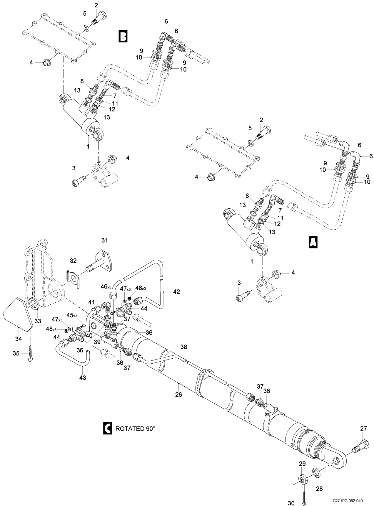
FIG 09 HYDRAULIC PIPING INSTL - CARGO DOOR, Z34AA, RH (SHEET 2 OF 3)
