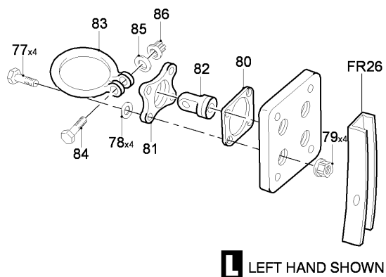
FIG 01 STRUCTURE INSTL, Z34AA (SHEET 3 OF 6)
