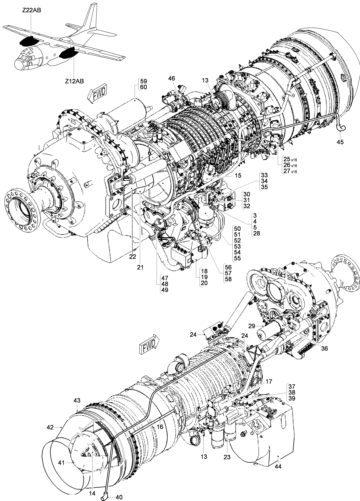
FIG 01 ENGINE INSTL, Z12AB-22AB (SHEET 1 OF 1)
