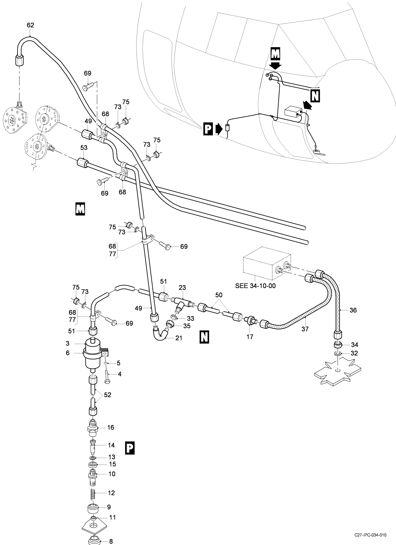
FIG 06 STATIC AND DYNAMIC PRESSURE INSTRUMENTS INSTL, Z31AA (SHEET 5 OF 5)
