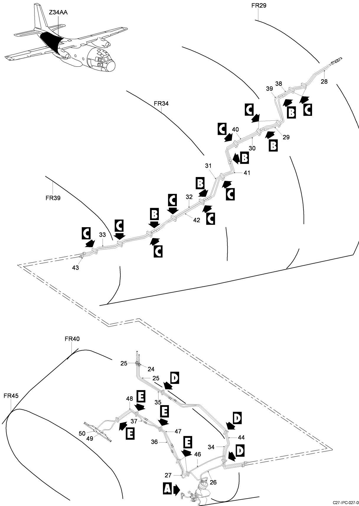
FIG 06 ELEVATOR HYDRAULIC ACCUMULATOR INSTL, Z34AA, RH (SHEET 1 OF 3)
