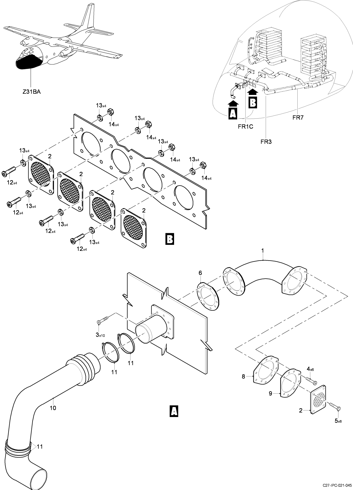
FIG 03 DUCT ASSY WEATHER RADAR COOLING INSTL, Z31BA (SHEET 1 OF 1)
