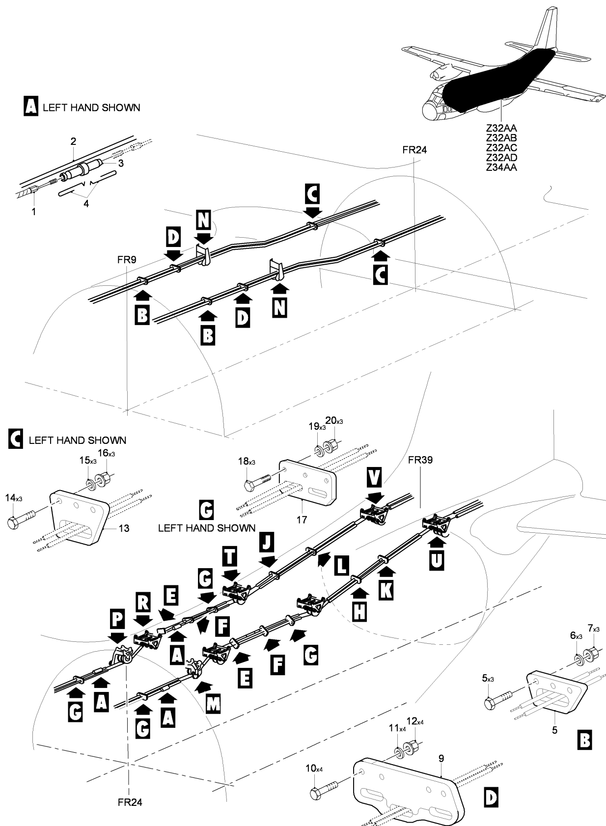
FIG 04 ELEVATOR CONTROLS INSTL, Z32AA-32AB-32AC-32AD-34AA (SHEET 1 OF 5)
