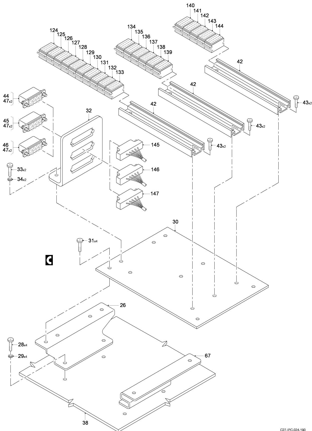
FIG 09 THIRD SHELF INSTL - ELECTRICAL COMPARTMENT, Z31AA (SHEET 3 OF 4)
