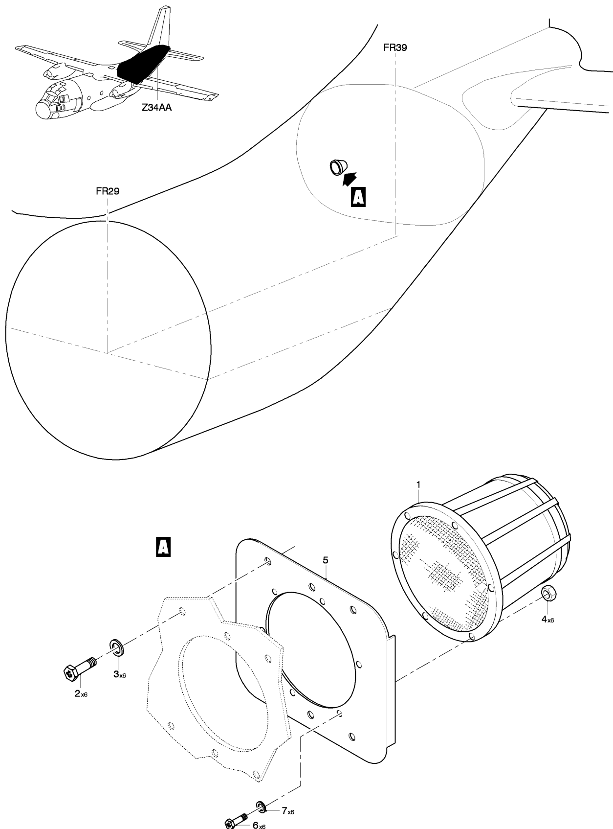
FIG 04 LOUDSPEAKER INSTL, Z34AA (SHEET 1 OF 1)
