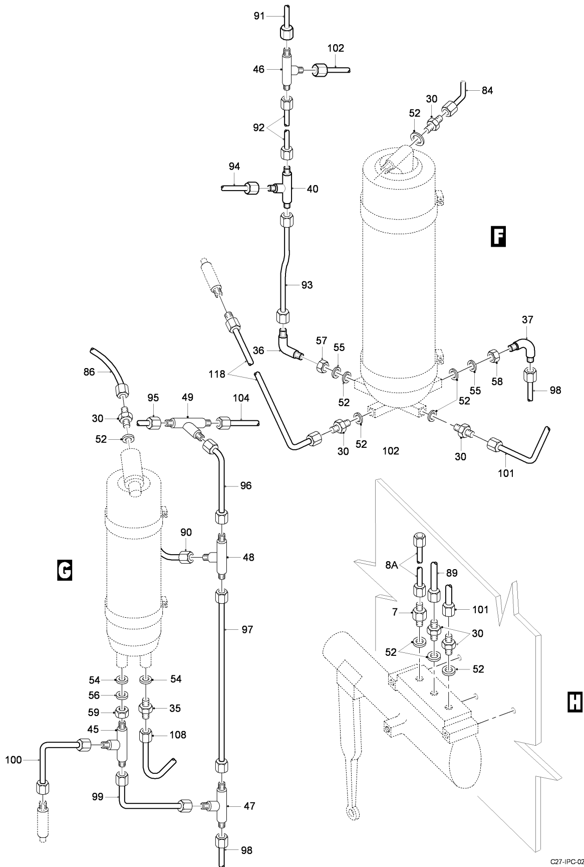
FIG 07 HYDRAULIC INSTL - MLG, Z13AB, LH (SHEET 3 OF 8)
