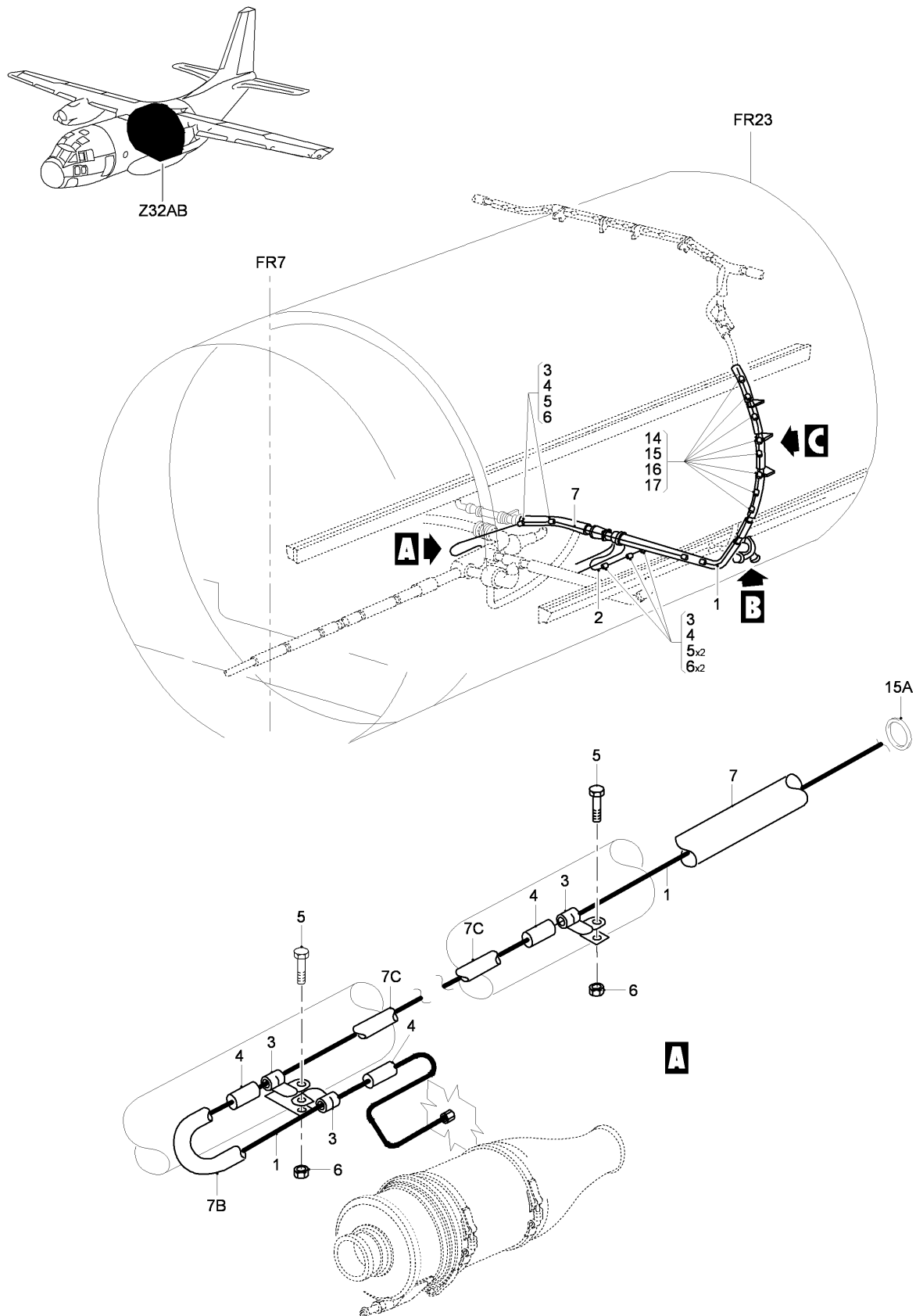
FIG 02 LEAK DETECTOR INSTL - CENTER FUSELAGE LOWER, Z32AB (SHEET 1 OF 2)
