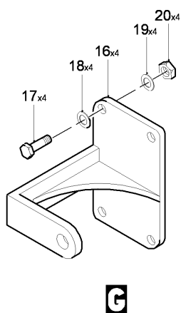
FIG 02 FITTING INSTL - NACELLE ENGINE, Z12AC-22AC (SHEET 2 OF 2)
