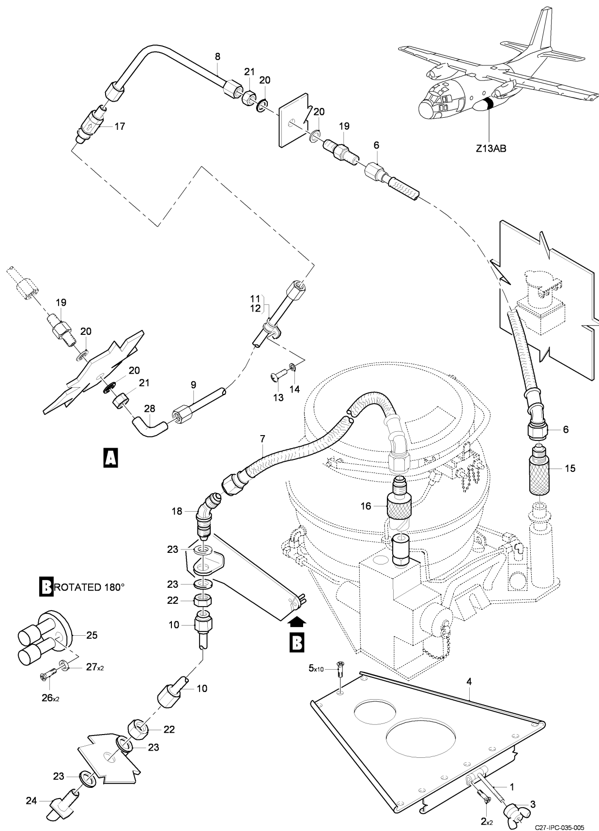
FIG 05 OXYGEN INSTL - MLG FARING, Z13AB, LH (SHEET 1 OF 1)
