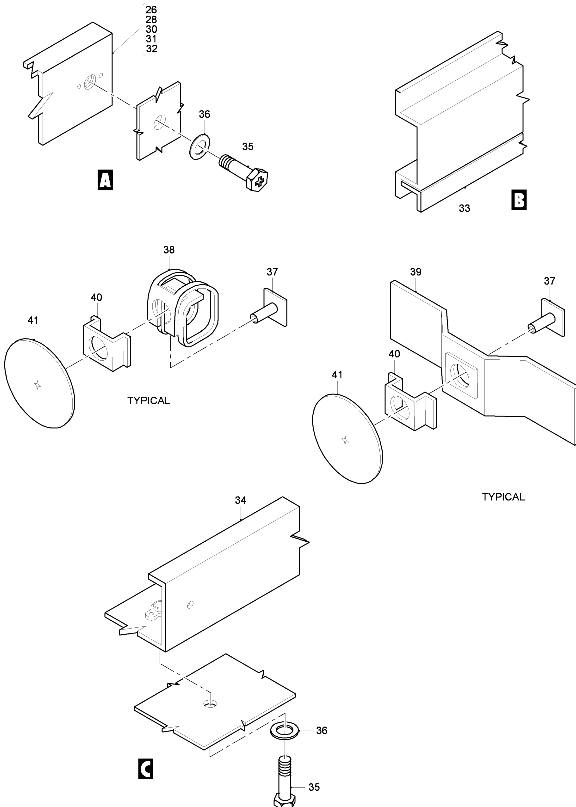
FIG 35 SECONDARY THERMAL INSULATION INSTL, RH SIDE, Z34AA (SHEET 2 OF 2)
