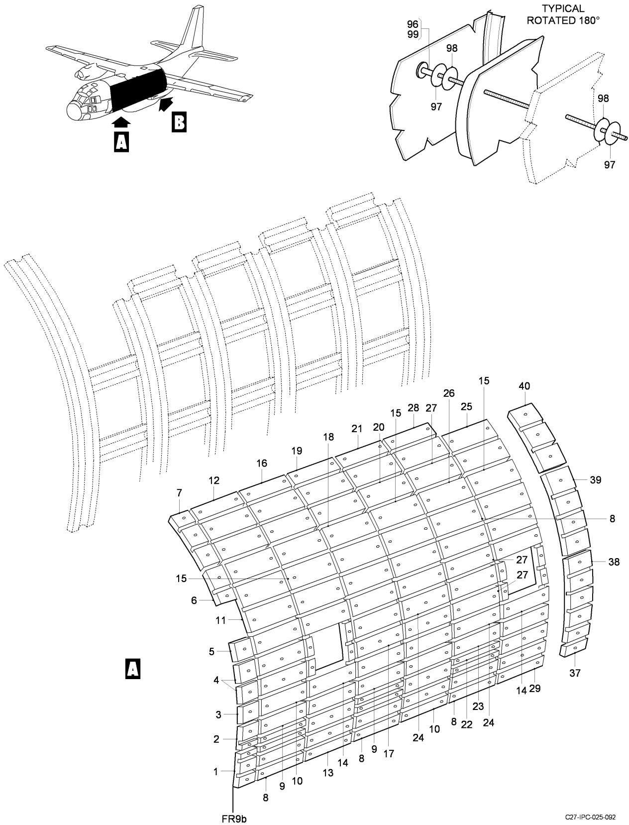
FIG 16 PRIMARY THERMAL INSULATION INSTL, Z32AA-32AB-32AC-32AD (SHEET 1 OF 2)
