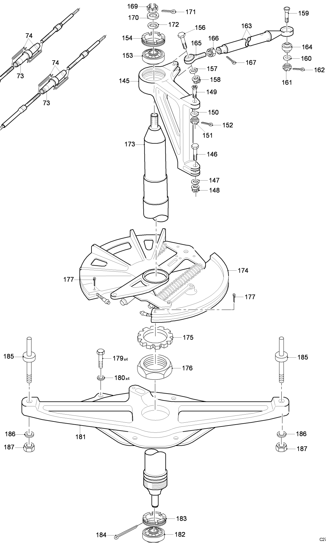
FIG 02 ELEVATOR CONTROLS INSTL, Z31AA-31BB-31AB (SHEET 3 OF 5)
