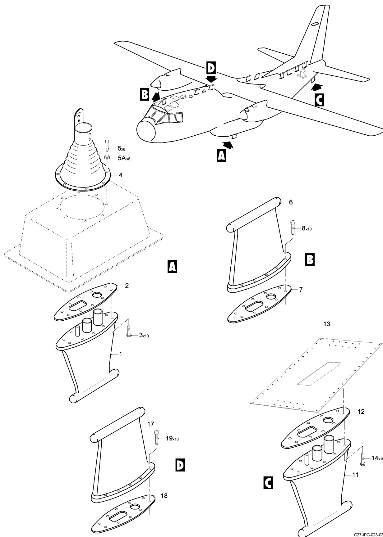
FIG 14 V/UHF ANTENNA, Z31AA-Z32AB-Z32BA-Z34BB (SHEET 1 OF 1)
