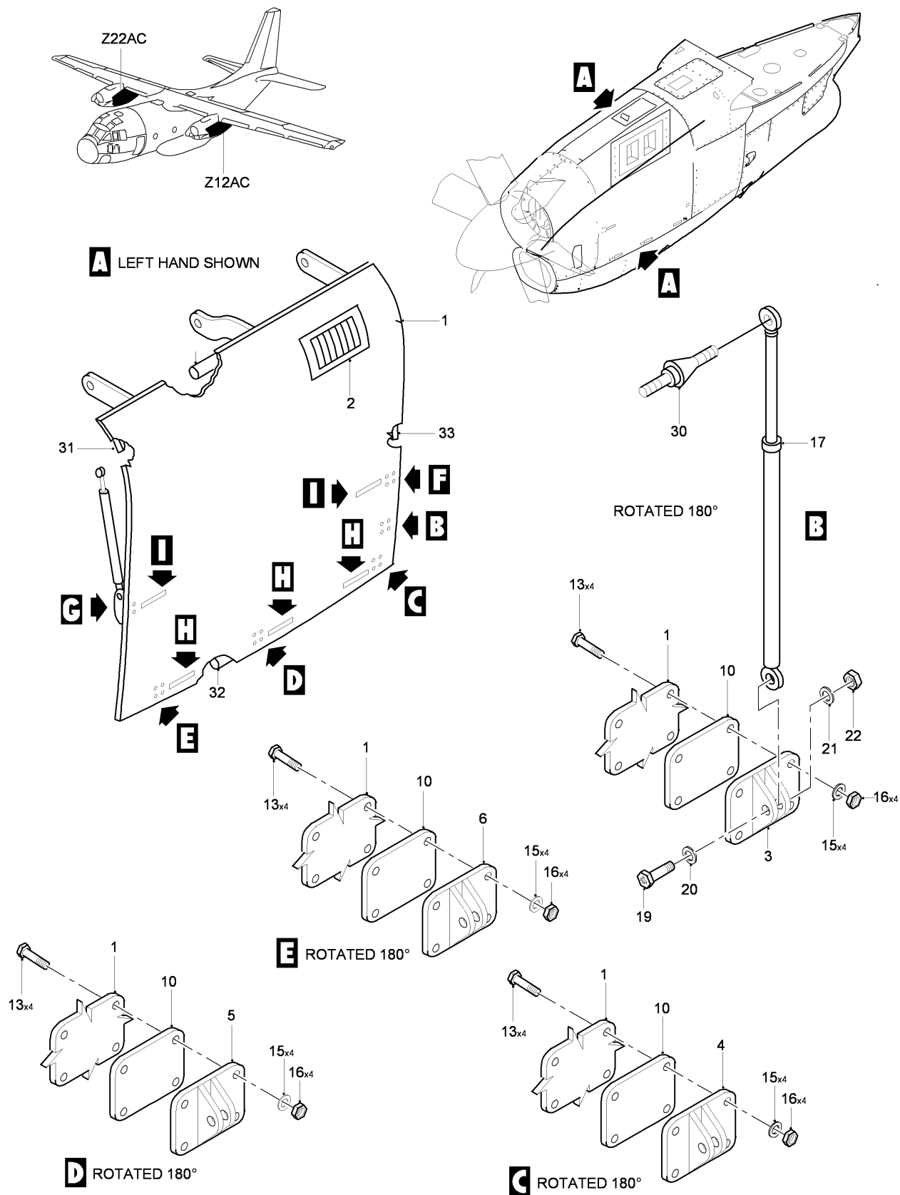
FIG 04 PANEL ASSY INSTL - SIDE FWD, Z12AC-22AC, LH-RH (SHEET 1 OF 2)
