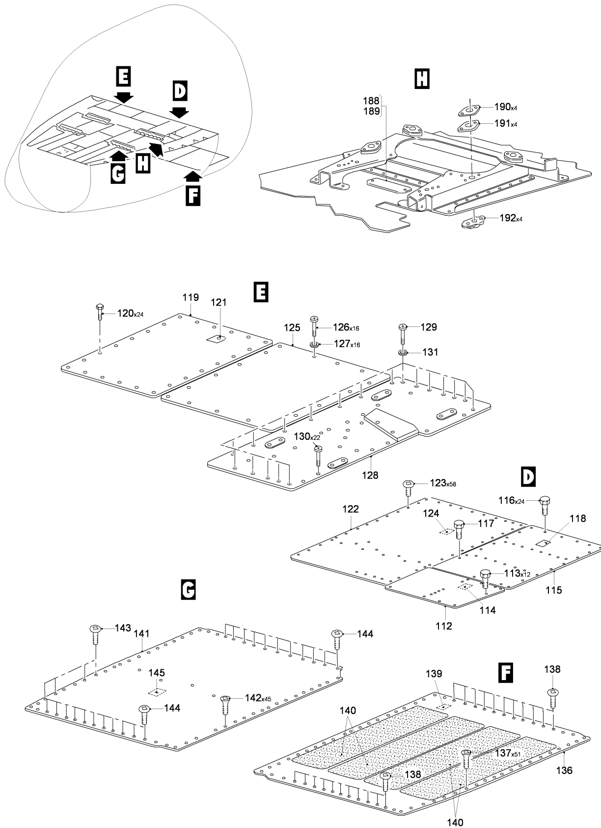
FIG 08 FLOOR FWD FUSELAGE INSTL, Z31AA (SHEET 3 OF 3)
