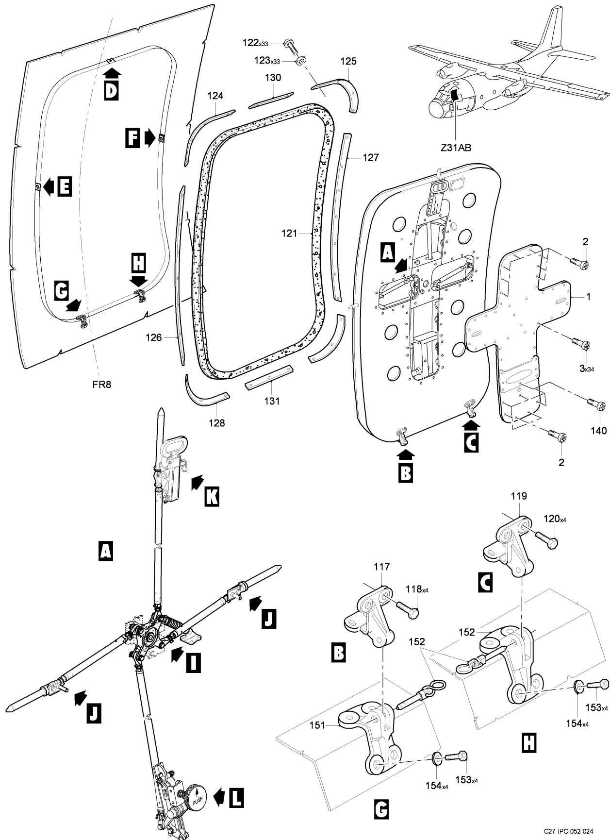
FIG 02 EMERGENCY EXIT DOOR INSTL - RH SIDE, Z31AB (SHEET 1 OF 2)
