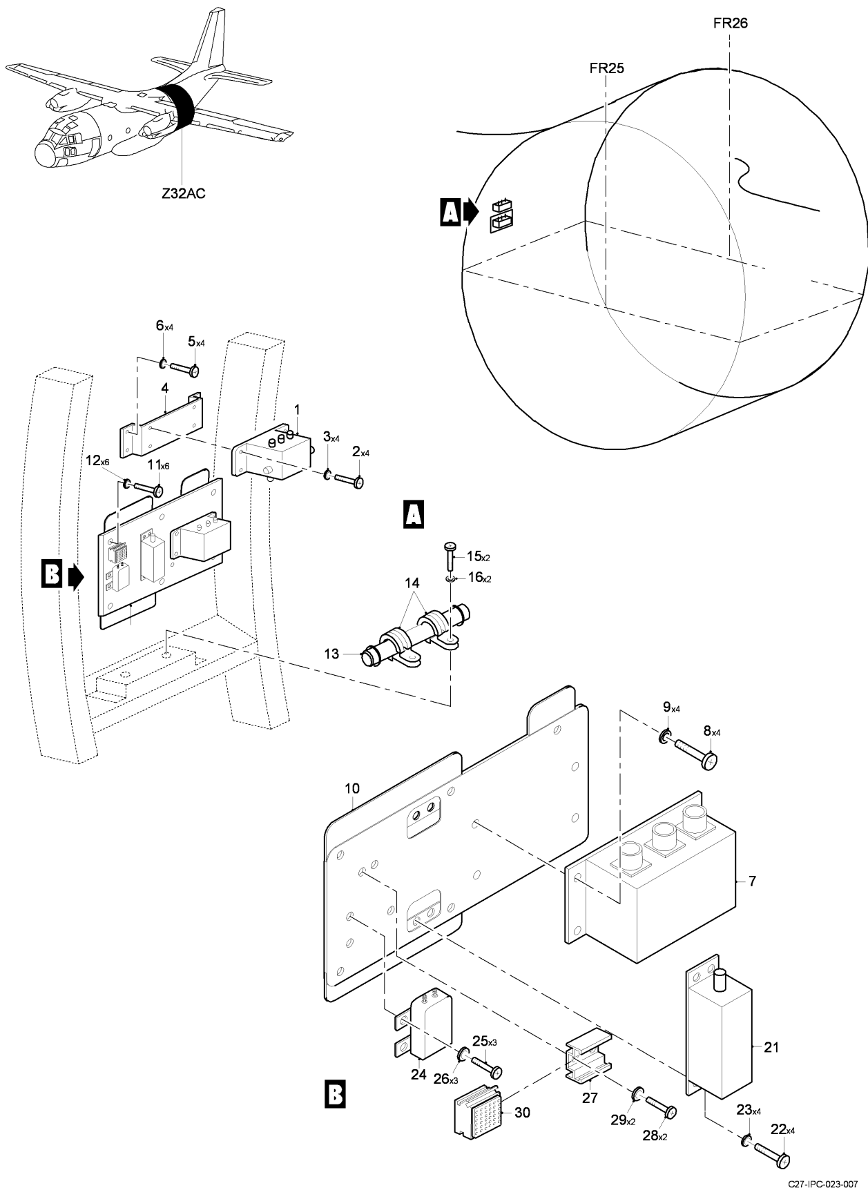
FIG 07 VHF/UHF NO. 2 AND NO. 3 INSTL, Z32AC (SHEET 1 OF 1)
