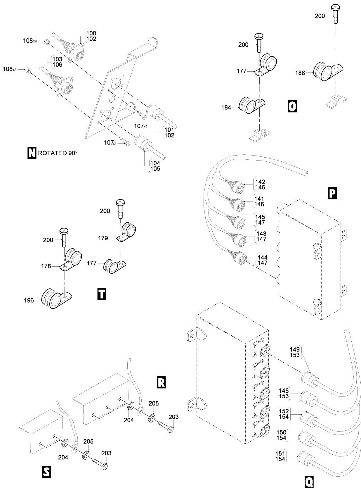
FIG 09 ELECTRICAL AND ELECTRONICS INSTL, Z31AA-31BC, RH (SHEET 6 OF 7)
