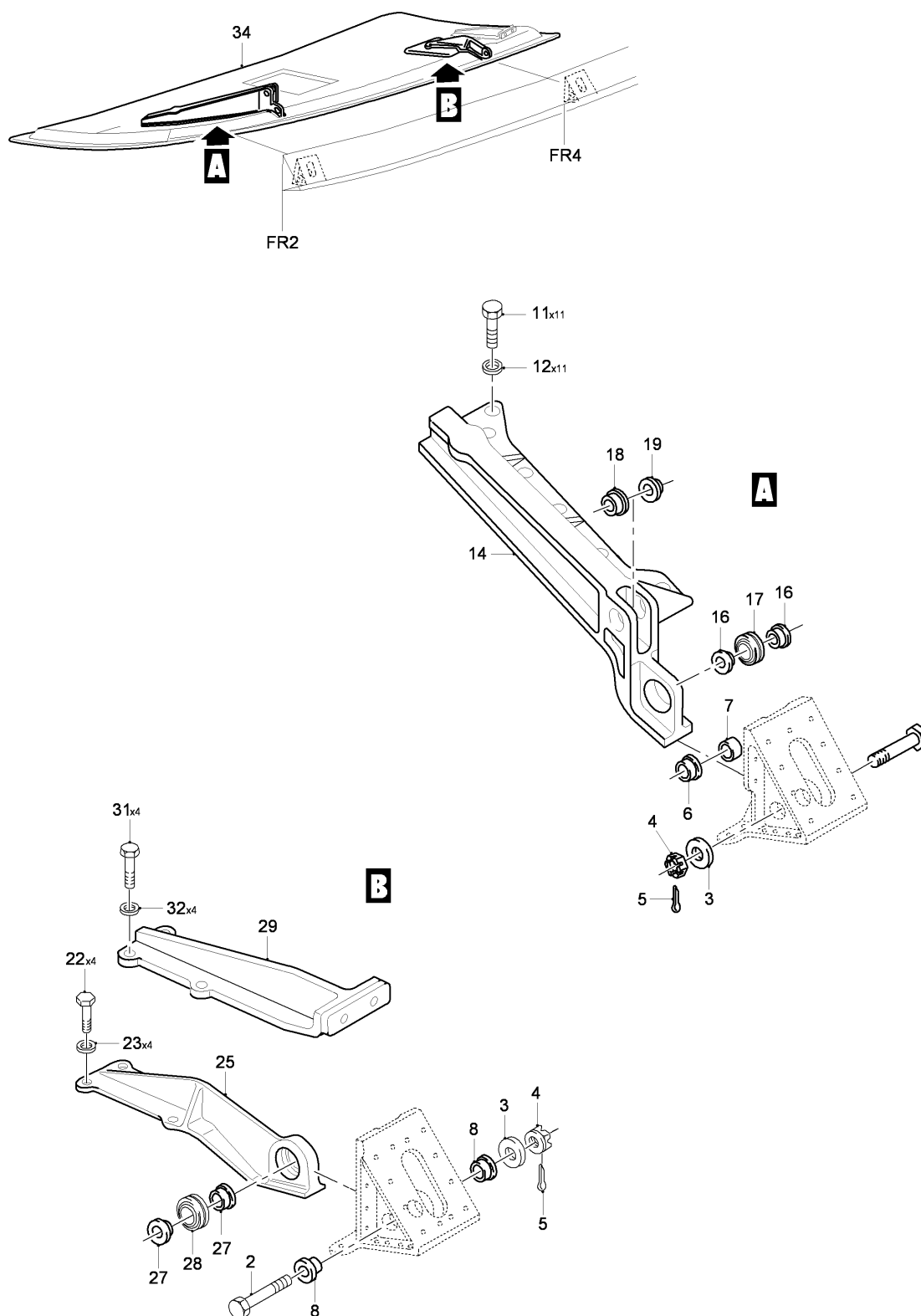
FIG 03 FITTING WHEEL BAY DOOR INSTL - NLG, Z31BB, LH-RH (SHEET 1 OF 1)
