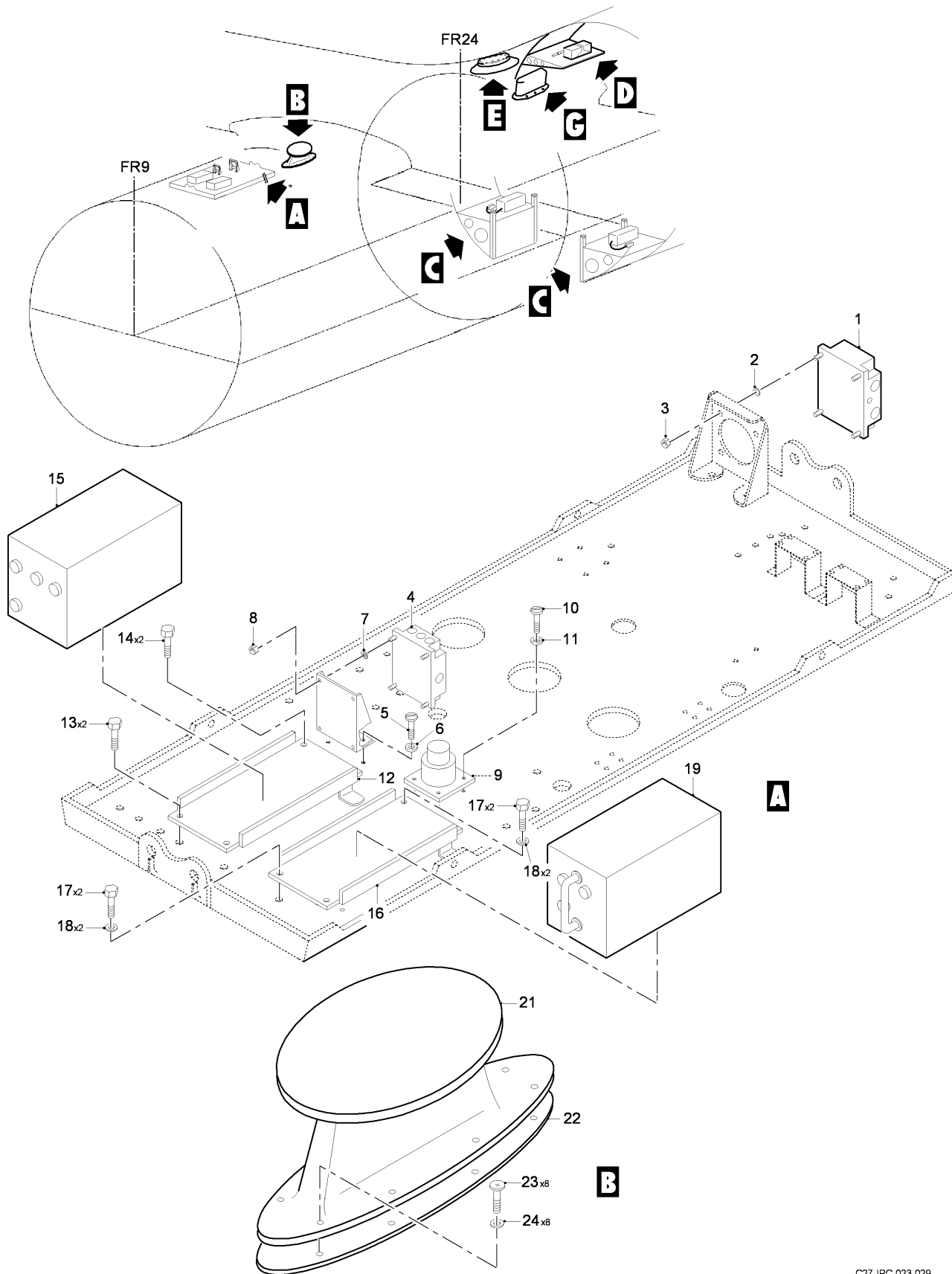
FIG 01 SATELLITE COMMUNICATION SYSTEM, Z32AA, Z32AD, Z32BA, Z34AA (SHEET 1 OF 3)
