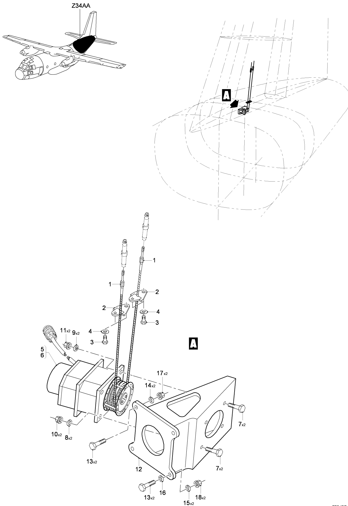
FIG 08 AUTOPILOT ACTUATOR INSTL - RUDDER CONTROL, Z34AA (SHEET 1 OF 1)
