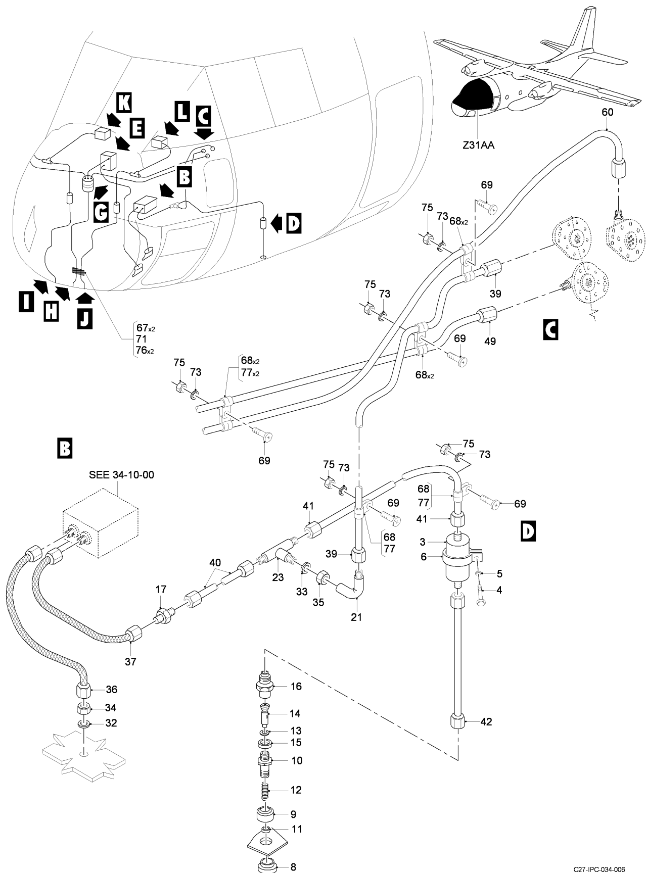
FIG 06 STATIC AND DYNAMIC PRESSURE INSTRUMENTS INSTL, Z31AA (SHEET 1 OF 5)
