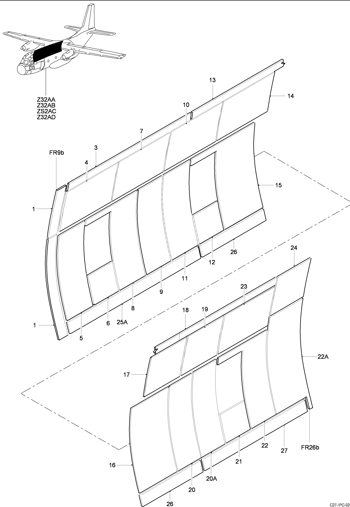
FIG 24 SECONDARY THERMAL INSULATION INSTL, Z32AA-32AB-32AC-32AD (SHEET 1 OF 3)
