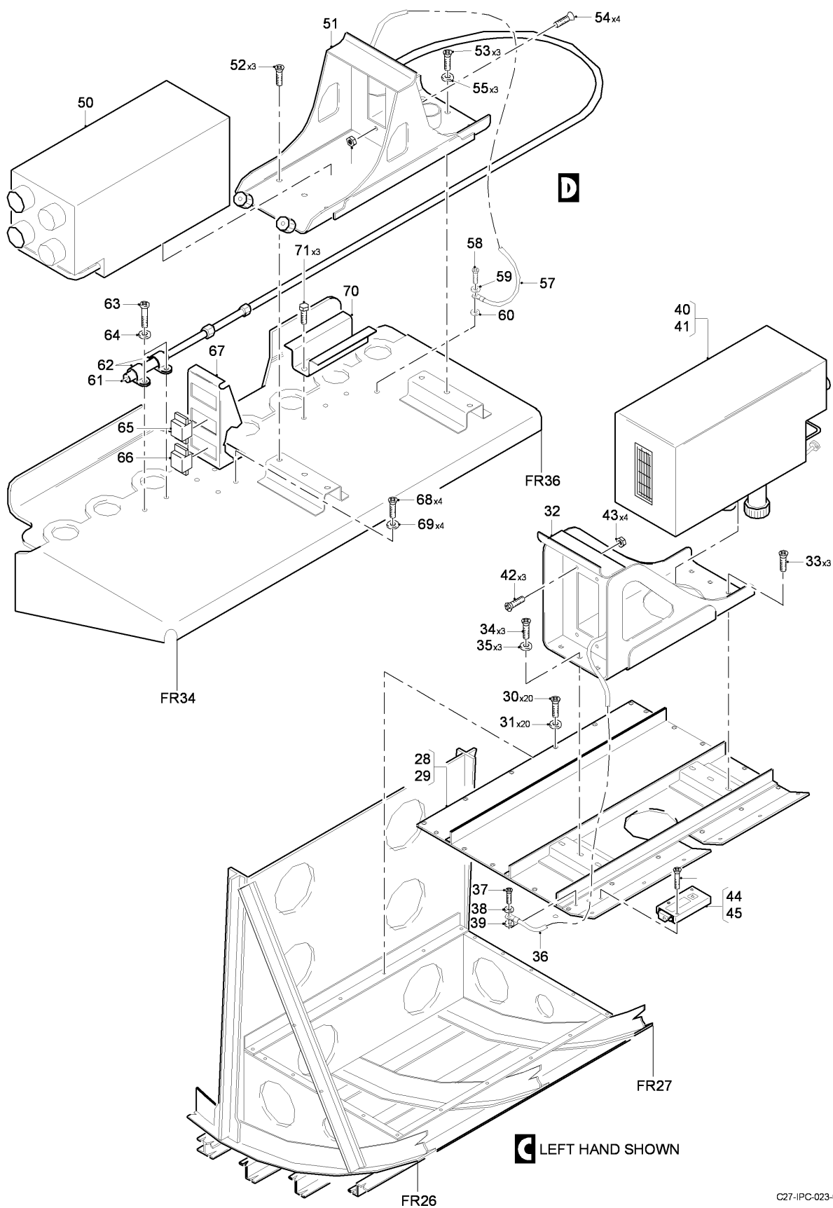
FIG 01 SATELLITE COMMUNICATION SYSTEM, Z32AA, Z32AD, Z32BA, Z34AA (SHEET 2 OF 3)
