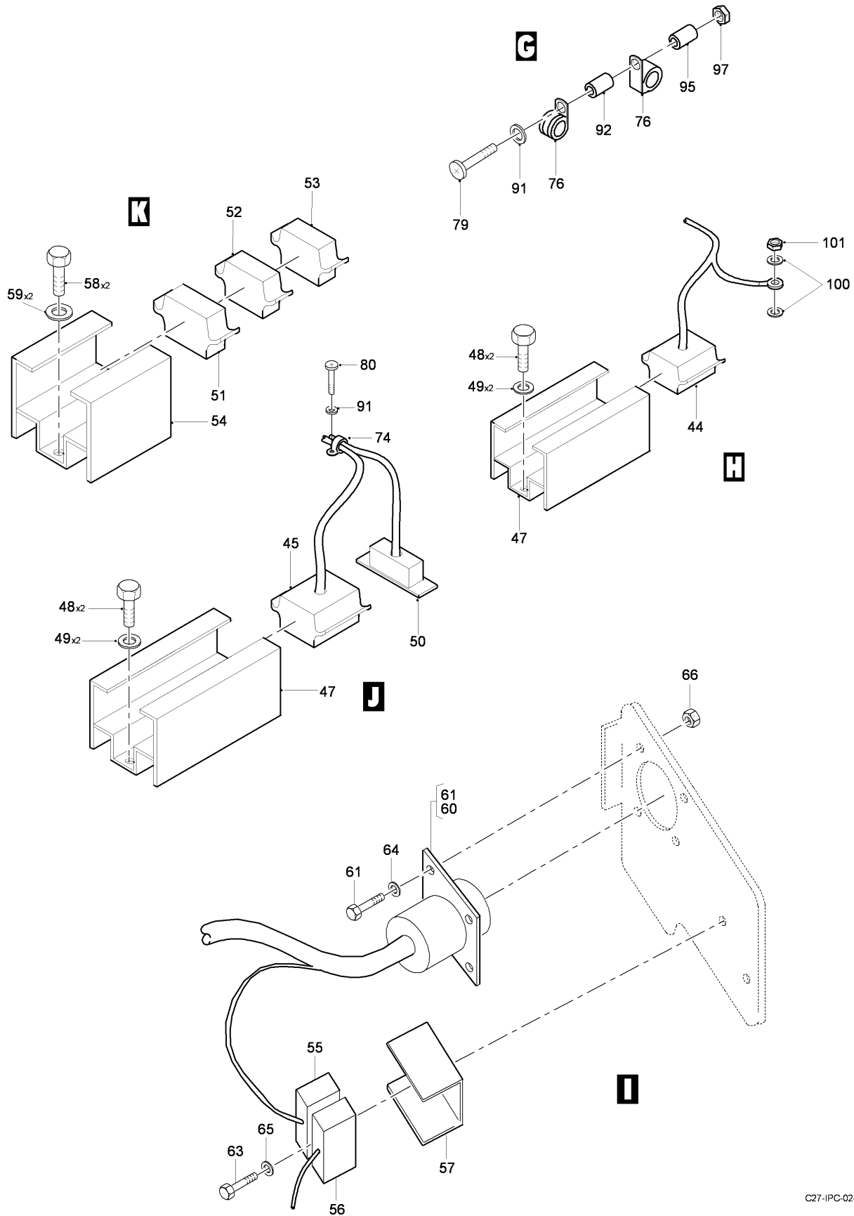
FIG 25 ELECTRICAL AND ELECTRONICS INSTL, Z21AA-21AB, RH (SHEET 3 OF 3)
