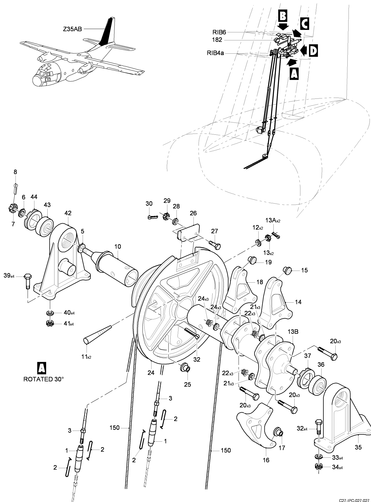
FIG 06 RUDDER CONTROL INSTL, Z35AB (SHEET 1 OF 4)
