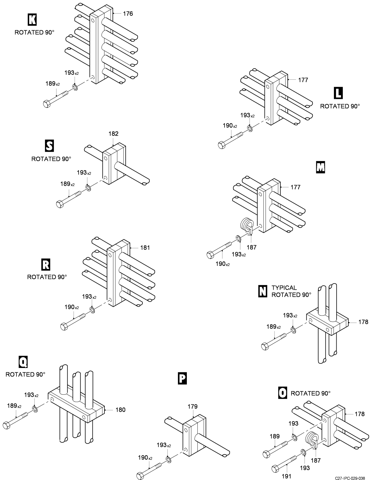
FIG 08 HYDRAULIC INSTL - MLG, Z23AB, RH (SHEET 6 OF 11)
