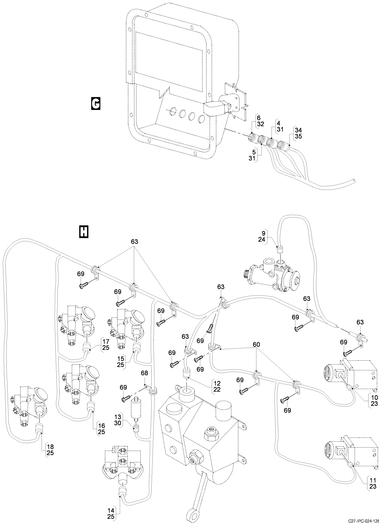
FIG 27 ELECTRICAL AND ELECTRONICS INSTL - MLG, Z23AA-23AB-23AC, RH (SHEET 3 OF 5)
