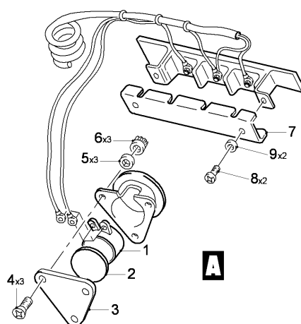
FIG 05 SWITCH THERMOSTATIC INSTL, Z31AA, RH (SHEET 1 OF 1)
