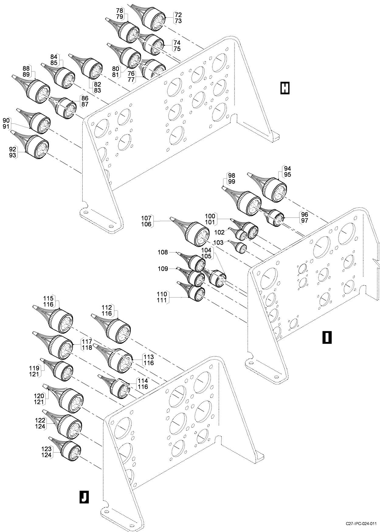
FIG 04 ELECTRICAL AND ELECTRONICS INSTL - CABIN, Z31AA, LH (SHEET 4 OF 5)
