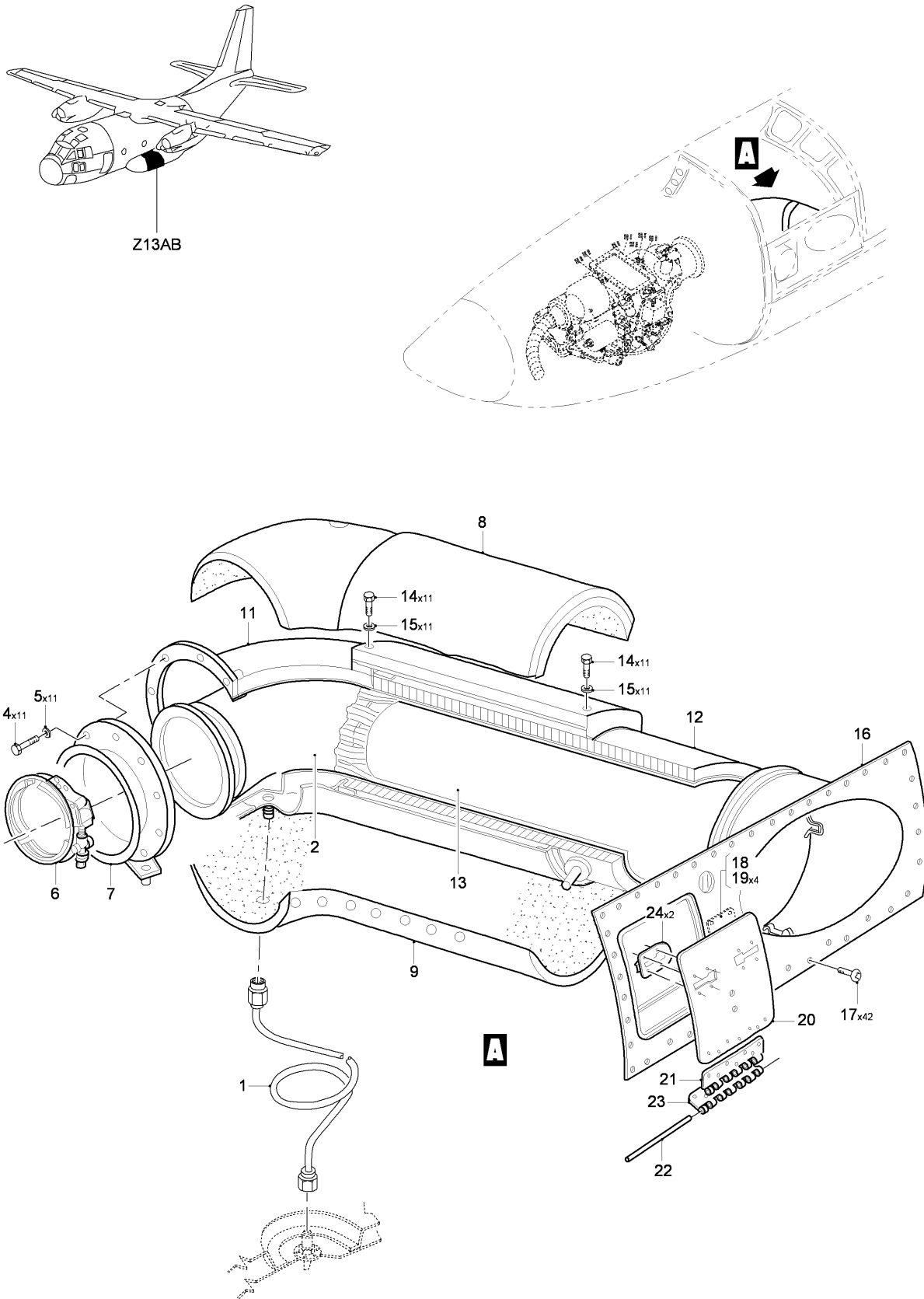
FIG 01 EXHAUST DUCT INSTL, APU, Z13AB (SHEET 1 OF 1)
