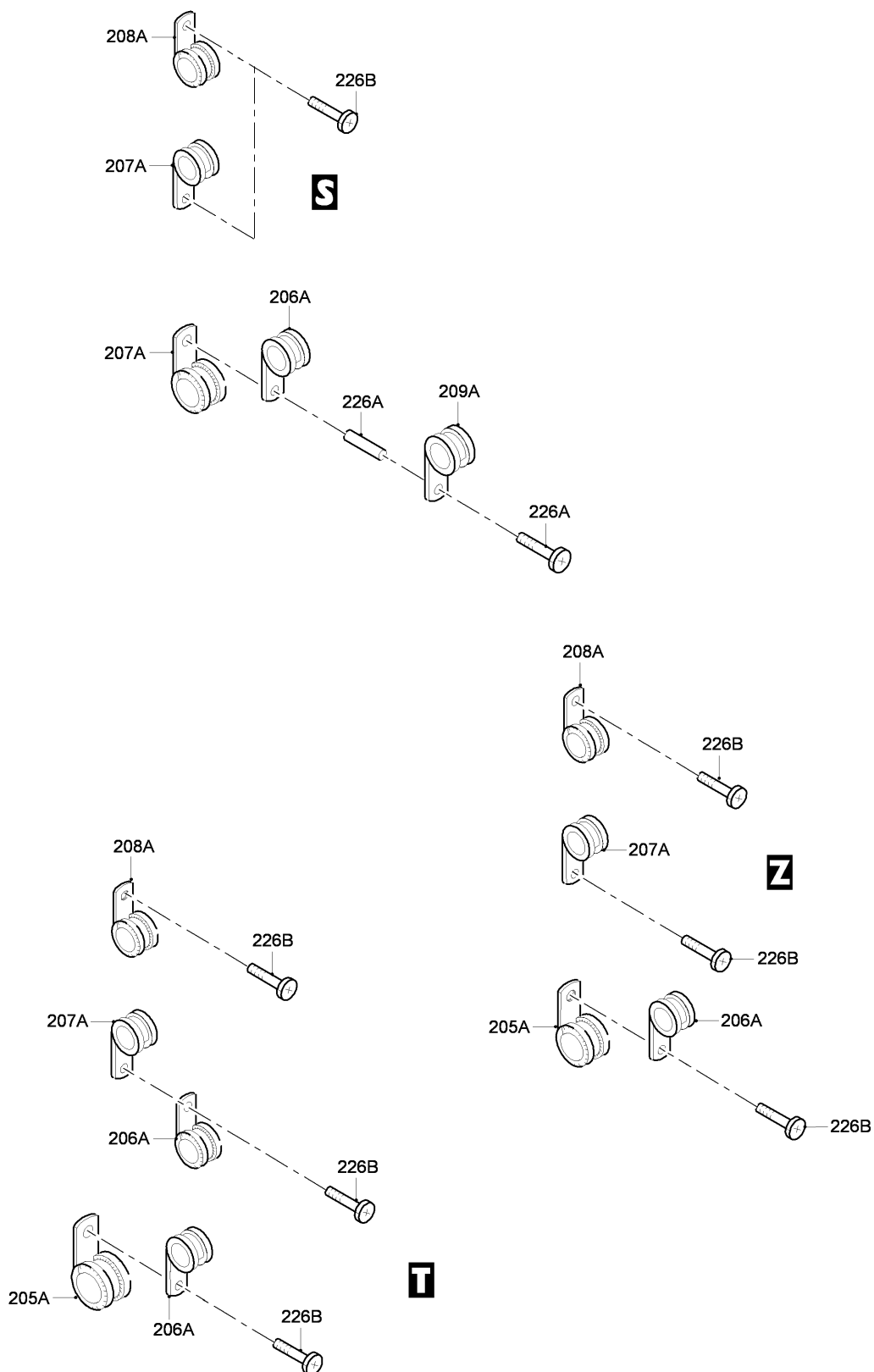
FIG 15 ELECTRICAL AND ELECTRONICS INSTL, Z31AB-32AA-32AB-32AC, LH (SHEET 9 OF 9)
