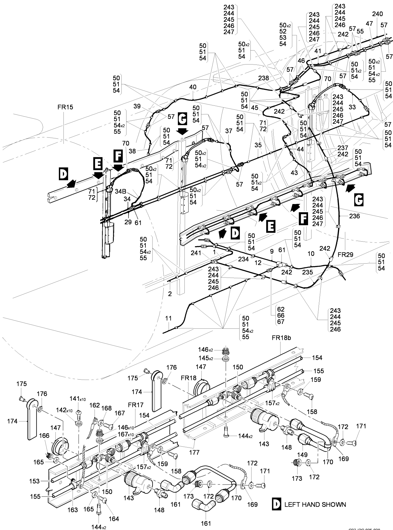
FIG 03 OXYGEN INSTL - CENTER FUSELAGE, Z32AA-32AB-32AC-32AD (SHEET 3 OF 5)
