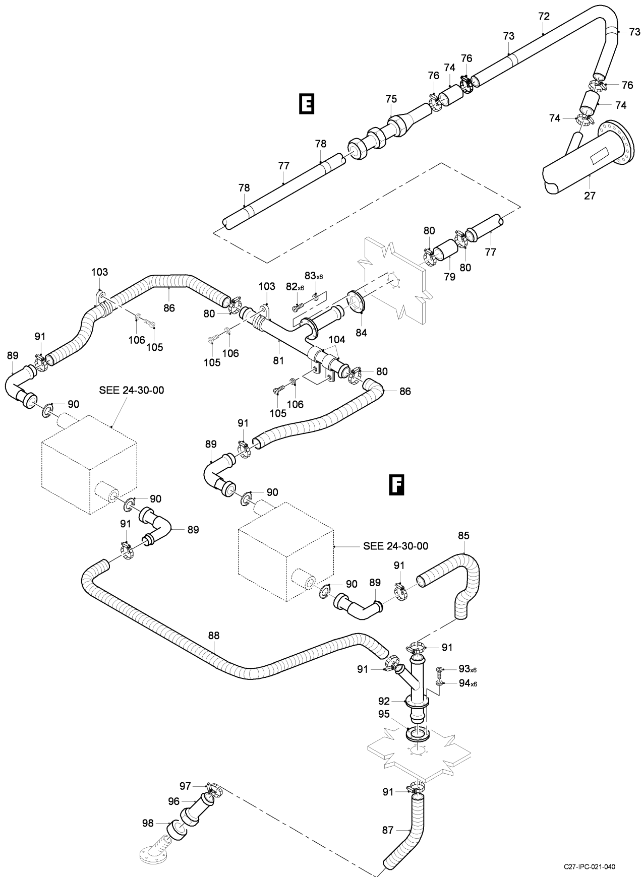
FIG 01 VENTILATION INSTL - CENTER FUSELAGE, Z32BA (SHEET 3 OF 3)
