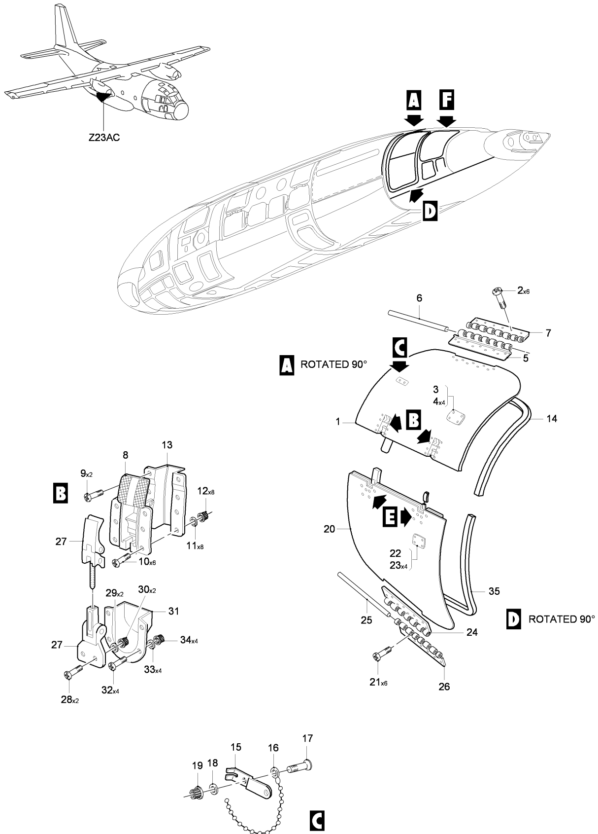
FIG 11 DOOR INSTL - MLG REAR, Z23AC, RH (SHEET 1 OF 2)
