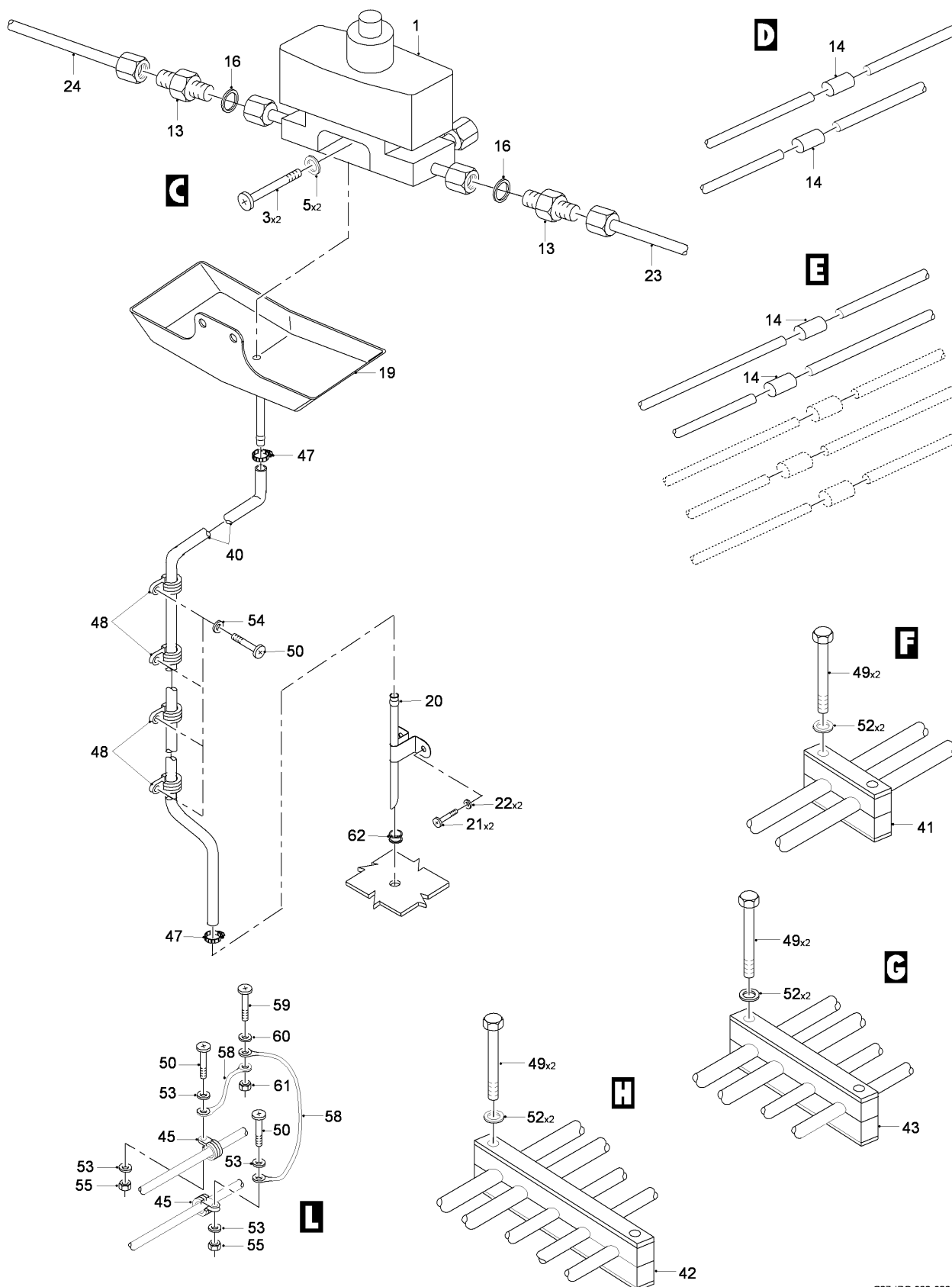
FIG 01 BRAKE HYDRAULIC SYSTEM INSTL, Z31BA-31BB (SHEET 3 OF 4)
