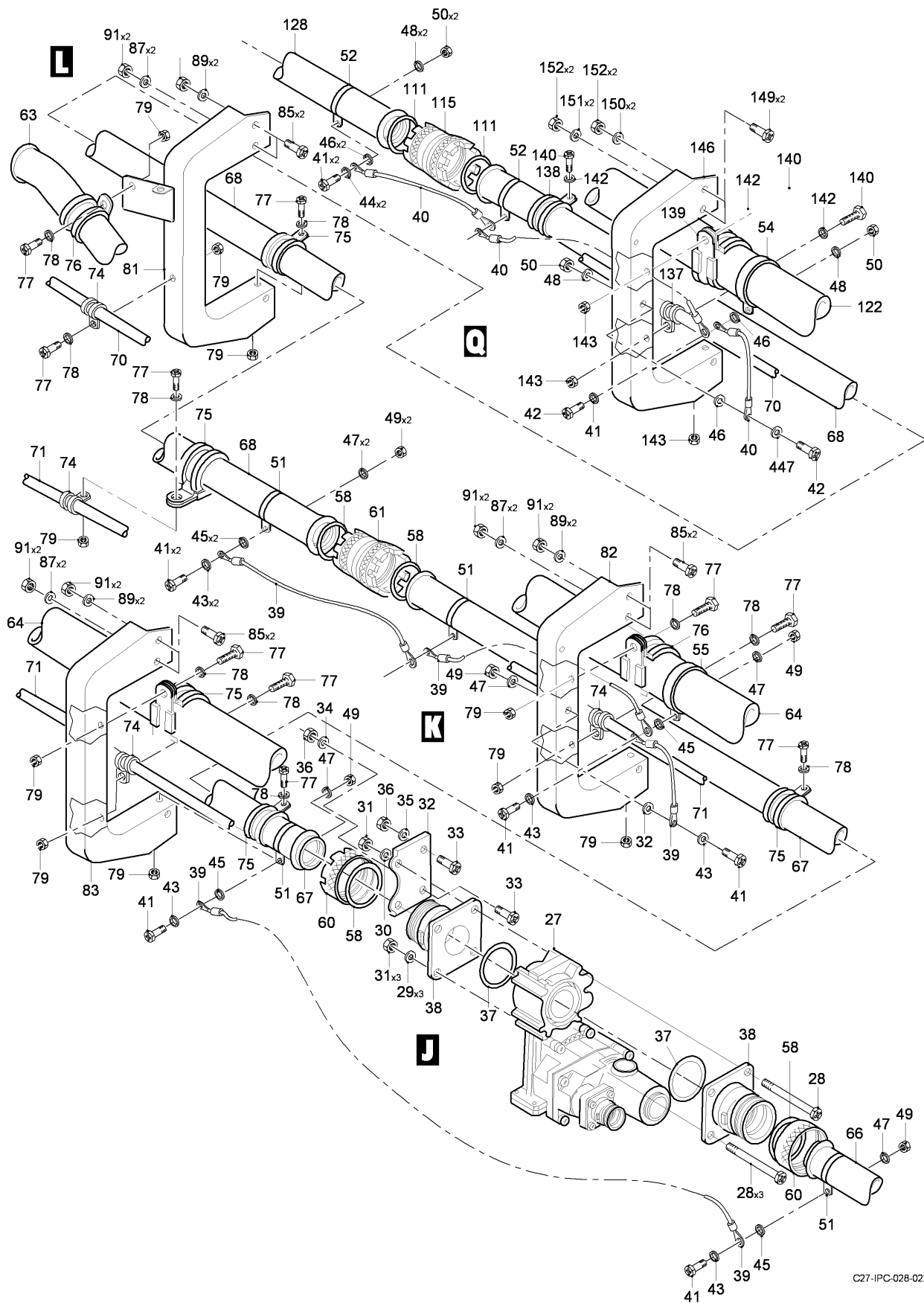
FIG 04 SINGLE POINT REFUELLING AND FUEL SUPPLY INSTL, Z33AB, LH-RH (SHEET 2 OF 6)
