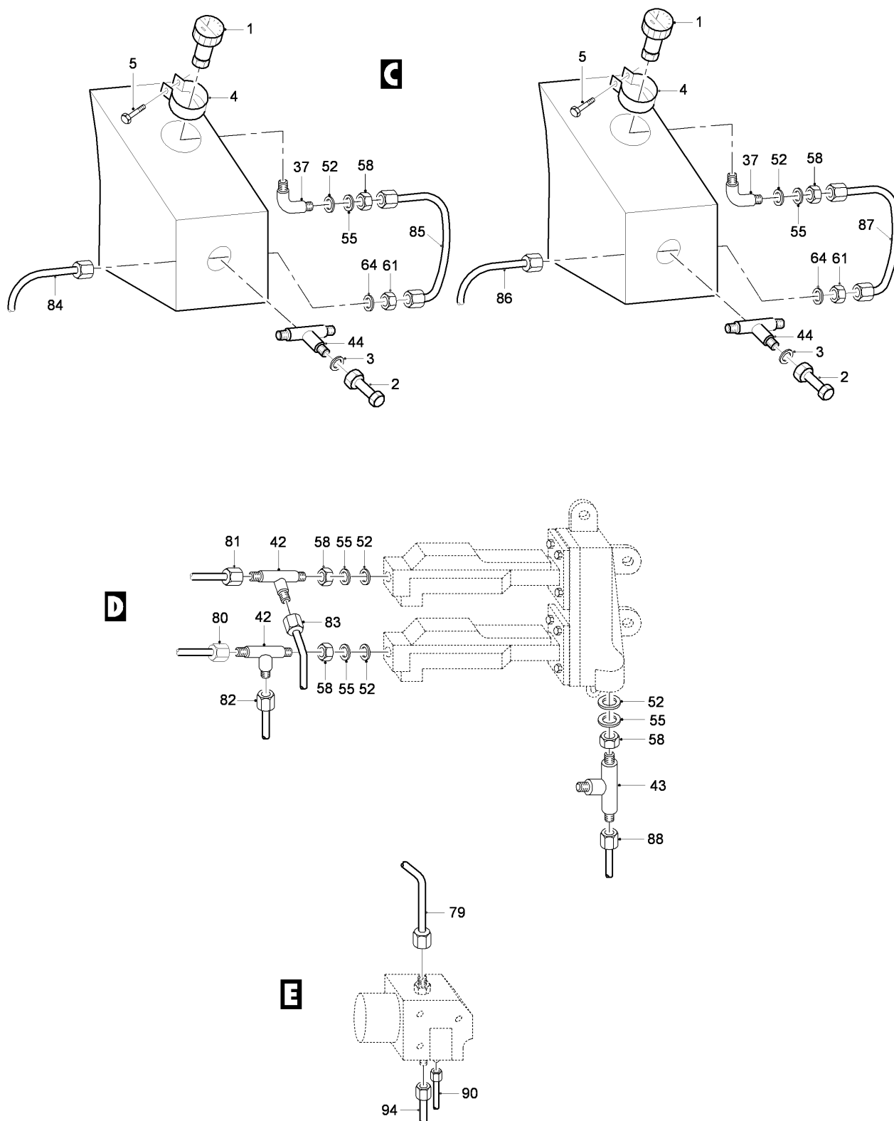
FIG 07 HYDRAULIC INSTL - MLG, Z13AB, LH (SHEET 2 OF 8)
