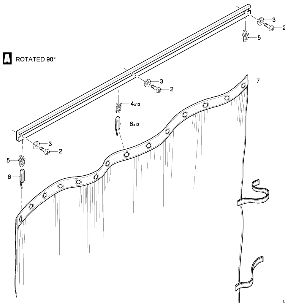
FIG 03 CABIN CURTAIN INSTL, Z31AB (SHEET 1 OF 1)
