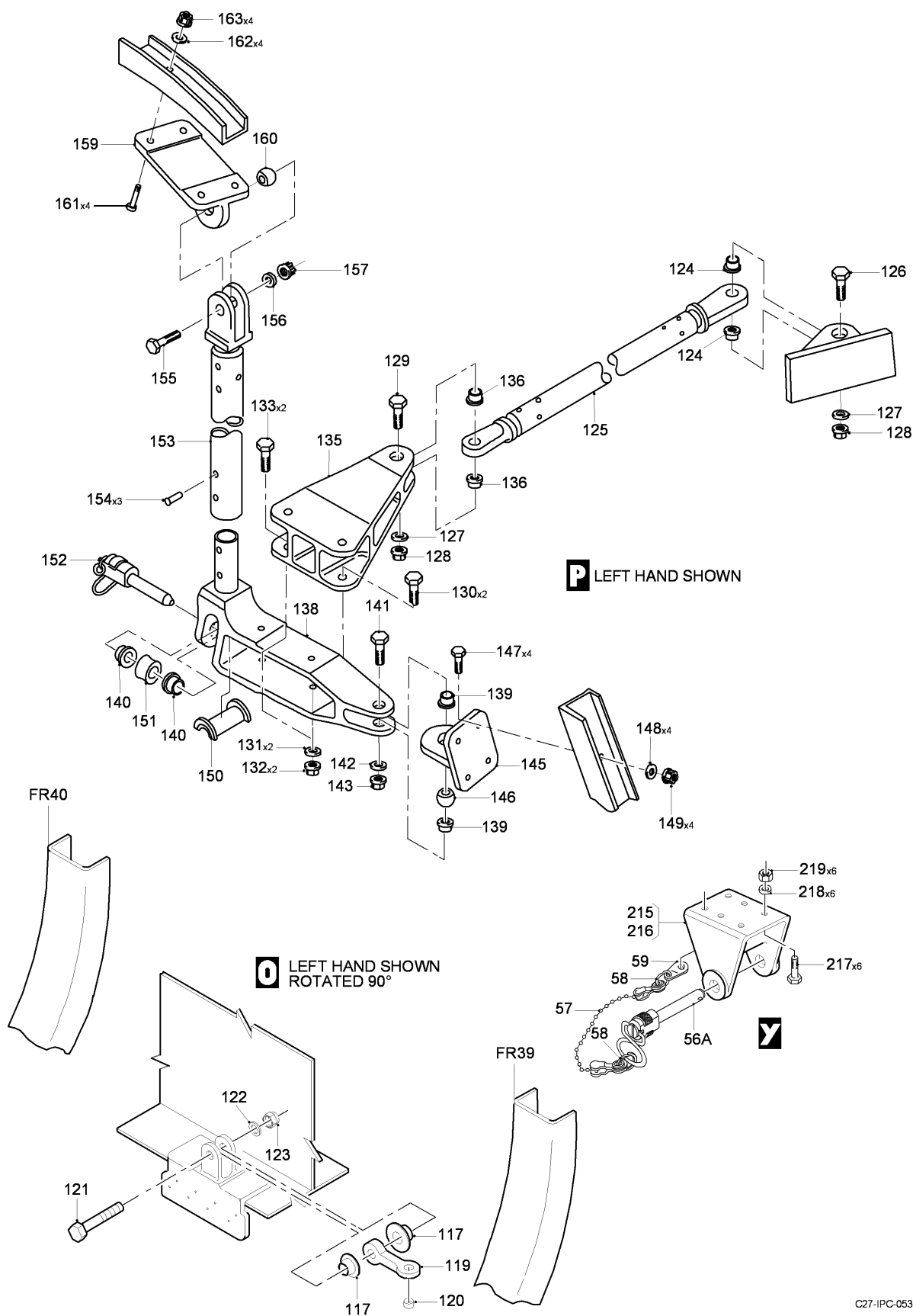
FIG 01 STRUCTURE INSTL, Z34AA (SHEET 4 OF 6)
