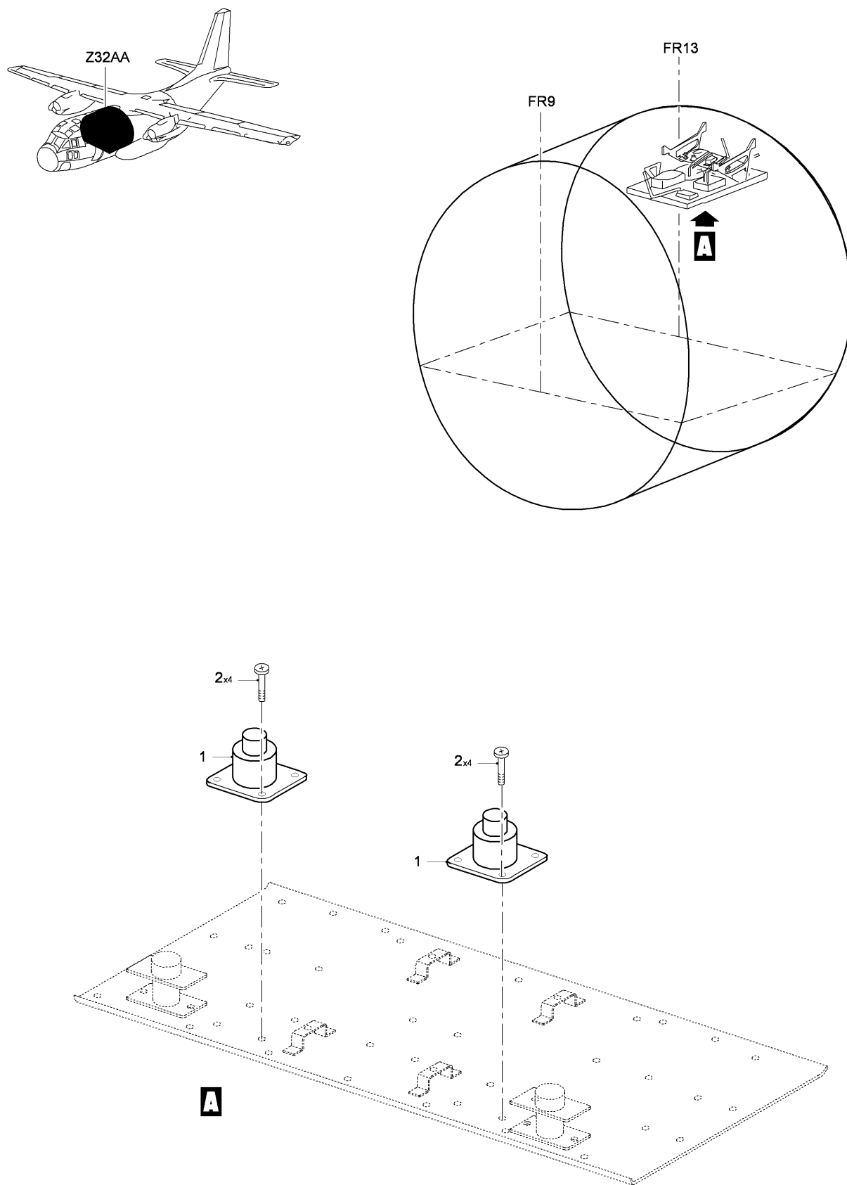
FIG 02 PROPELLER DE-ICING CONTACTOR INSTL, Z32AA (SHEET 1 OF 1)
