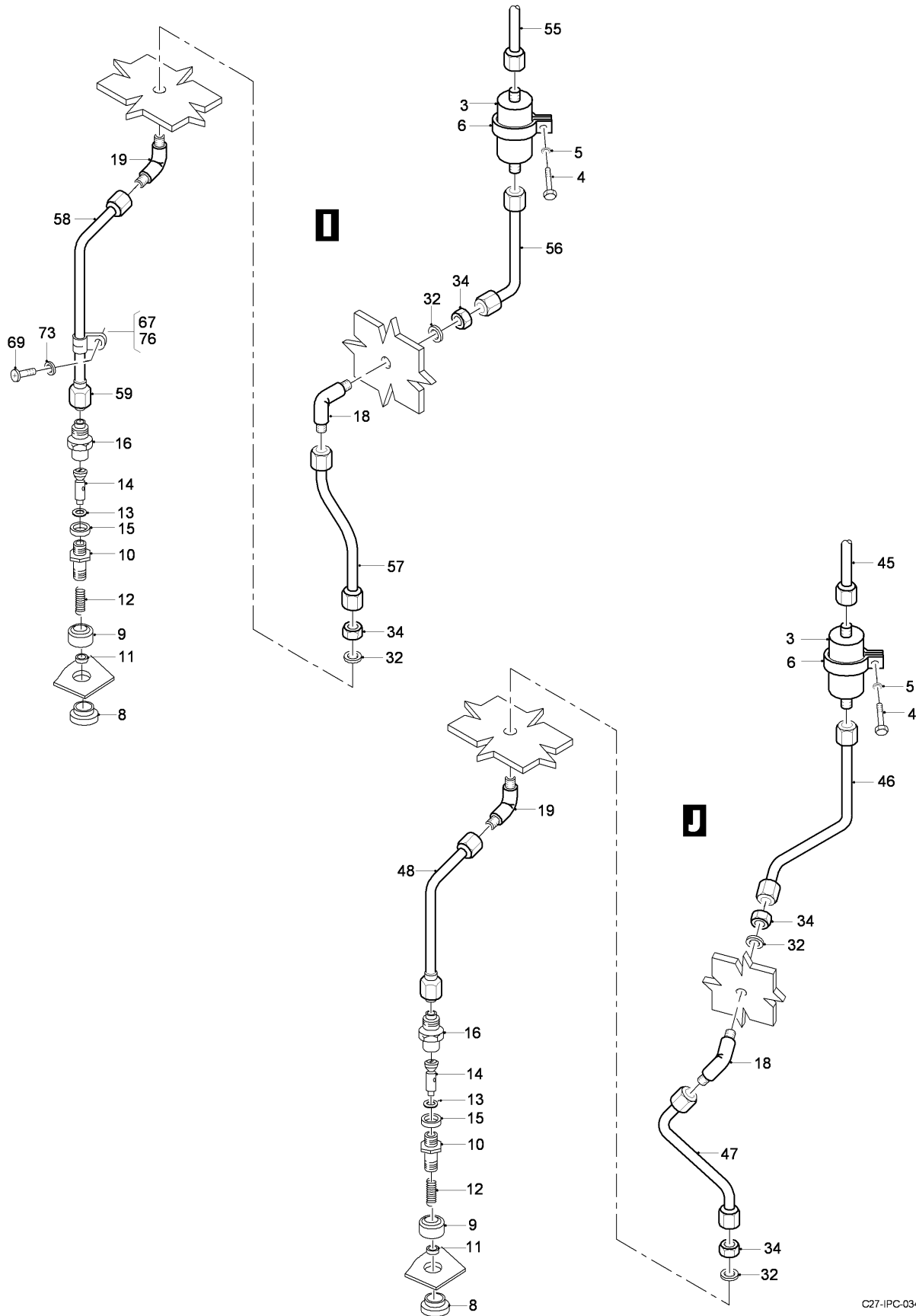
FIG 06 STATIC AND DYNAMIC PRESSURE INSTRUMENTS INSTL, Z31AA (SHEET 3 OF 5)
