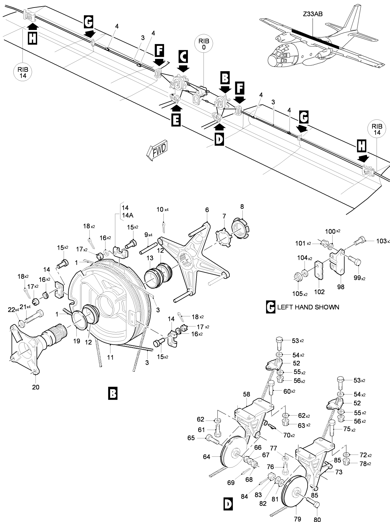
FIG 04 AILERON CONTROLS INSTL, Z33AB (SHEET 1 OF 2)
