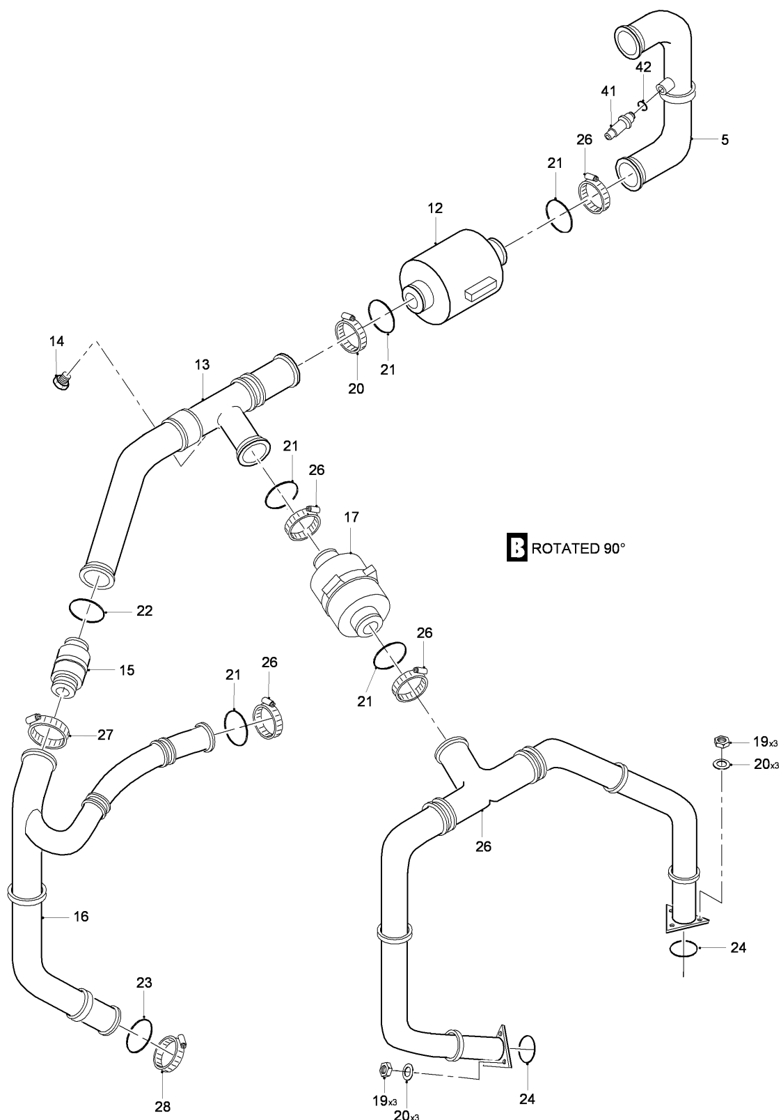
FIG 02 PNEUMATIC SYSTEM INSTL - ENGINE, Z12AC-22AC (SHEET 2 OF 2)
