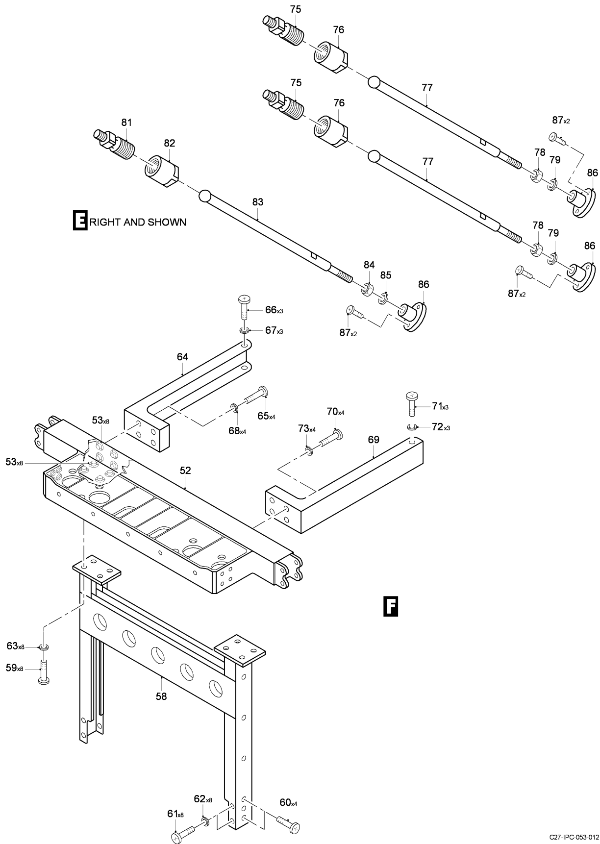
FIG 03 INSTRUMENTS PANELS INSTL, Z31AA (SHEET 3 OF 5)
